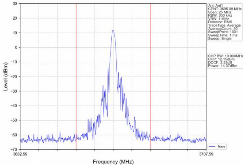
Band48_10MHz_256QAM_HCH_3695MHz_RB_1_49_NTNV
