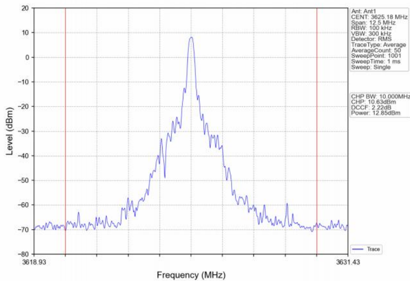
Band48_5MHz_256QAM_MCH_3625MHz_RB_1_13_NTNV
