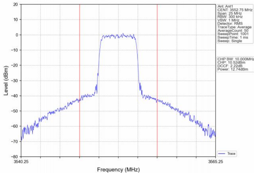
Band48_10MHz_256QAM_LCH_3555MHz_RB_25_13_NTNV
