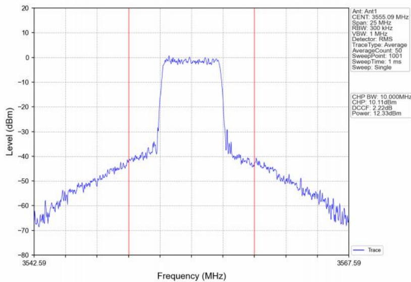
Band48_10MHz_256QAM_LCH_3555MHz_RB_25_13_NTNV
