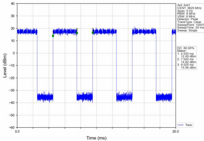
Band48_20MHz_64QAM_MCH_3625MHz_RB_100_0_NTNV
