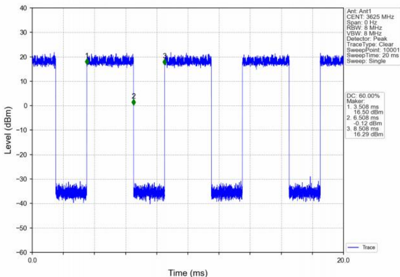
Band48_15MHz_64QAM_MCH_3625MHz_RB_75_0_NTNV
