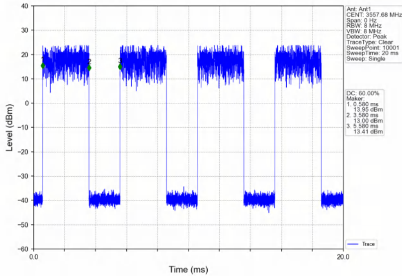
Band48_15MHz_16QAM_LCH_3557.5MHz_RB_1_74_NTNV
