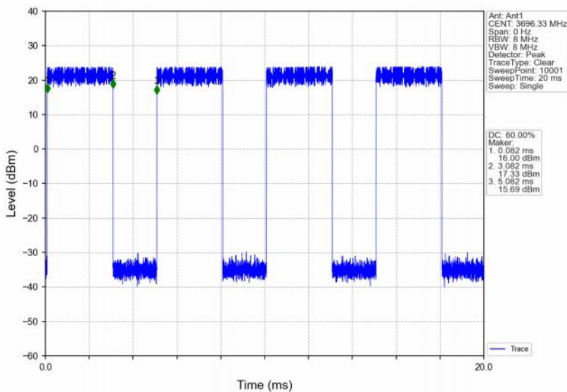
Band48_5MHz_QPSK_HCH_3697.5MHz_RB_12_0_NTV
