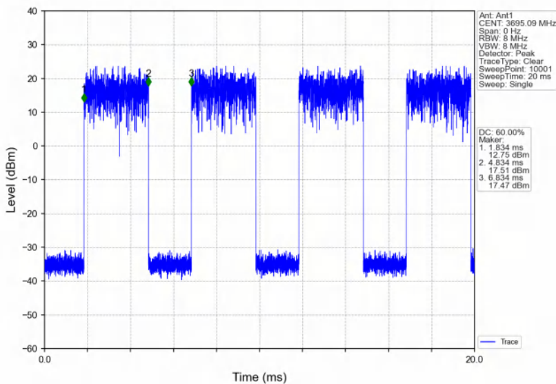
Band48_10MHz_64QAM_HCH_3695MHz_RB_1_25_NTNV
