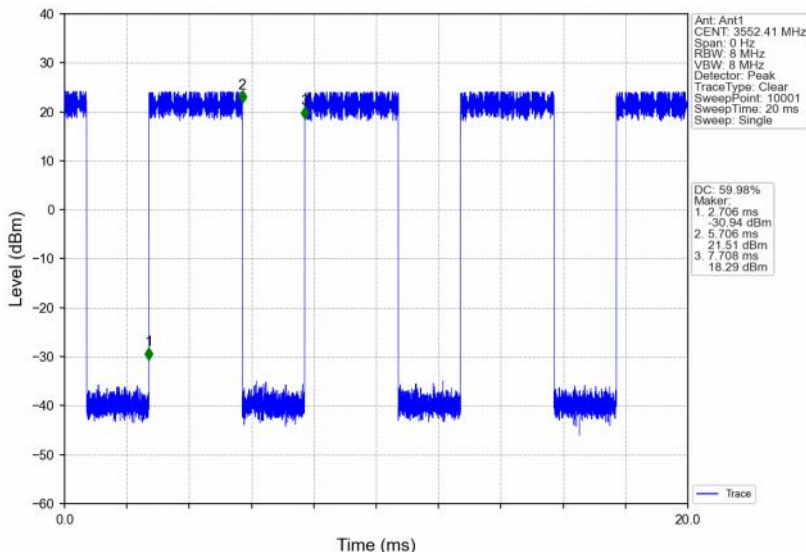
Band48_5MHz_QPSK_LCH_3552.5MHz_RB_12_13_NTNV
