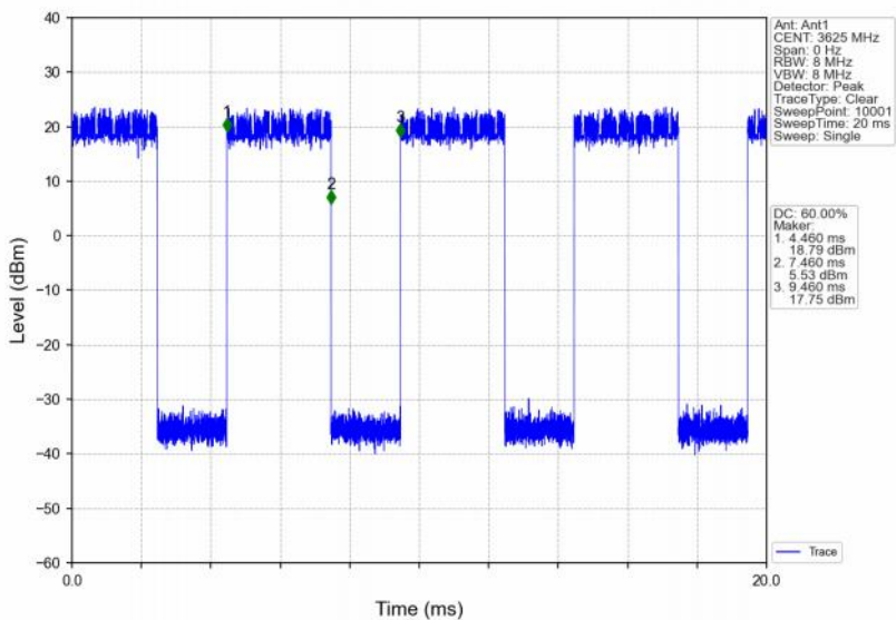
Band48_5MHz_64QAM_MCH_3625MHz_RB_25_0_NTNV
