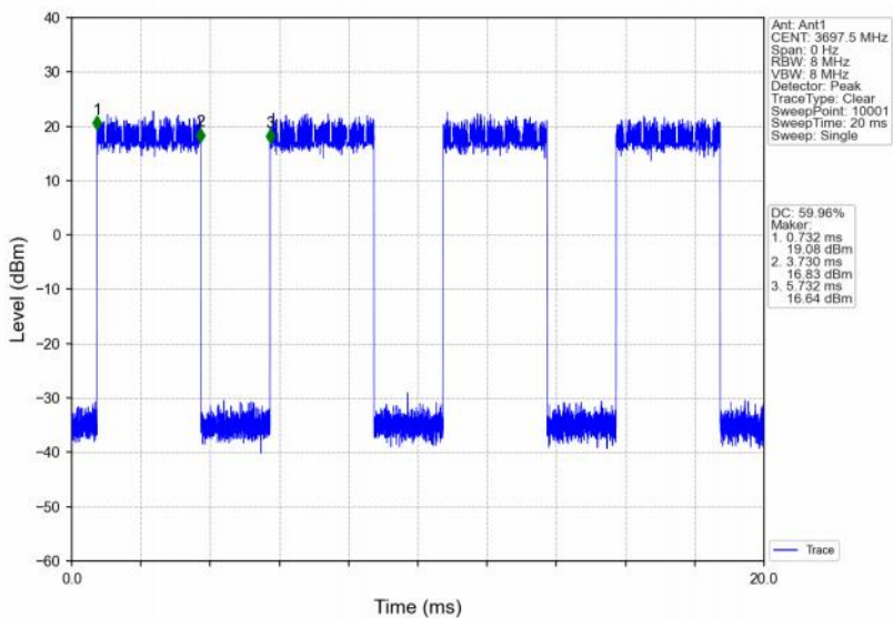
Band48_5MHz_256QAM_HCH_3697.5MHz_RB_25_0_NTNV
