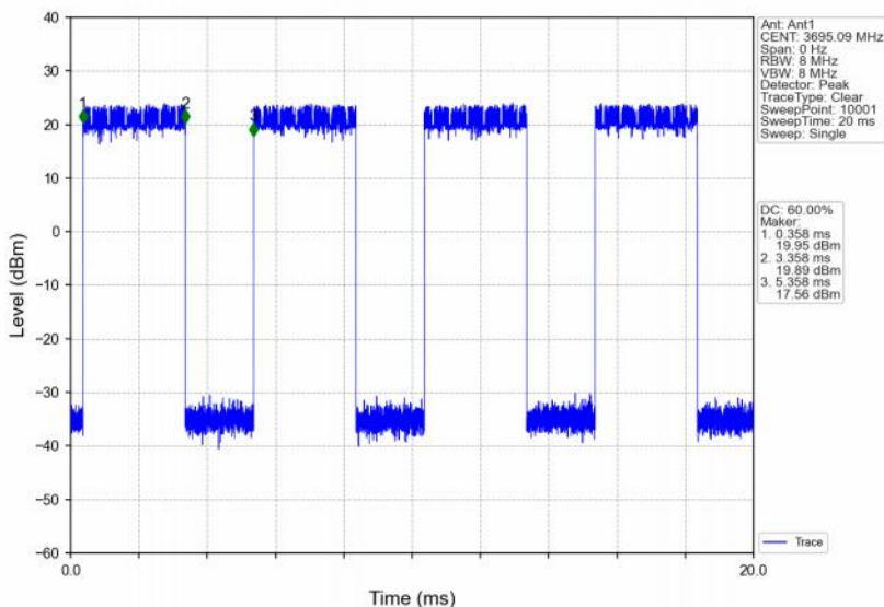
Band48_10MHz_16QAM_HCH_3695MHz_RB_25_13_NTNV
