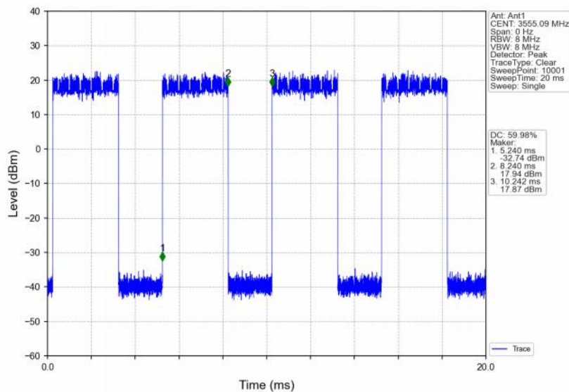
Band48_10MHz_256QAM_LCH_3555MHz_RB_25_13_NTNV
