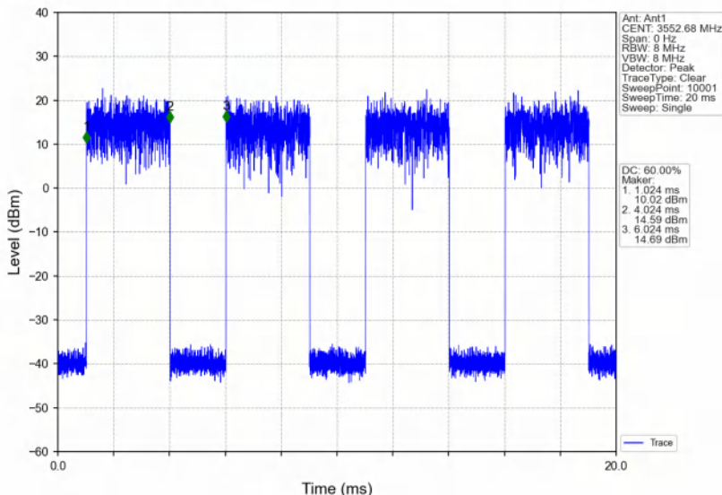
Band48_5MHz_256QAM_LCH_3552.5MHz_RB_1_24_NTNV
