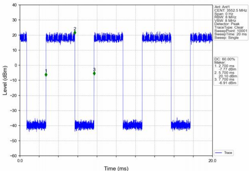
Band48_5MHz_256QAM_LCH_3552.5MHz_RB_25_0_NTNV
