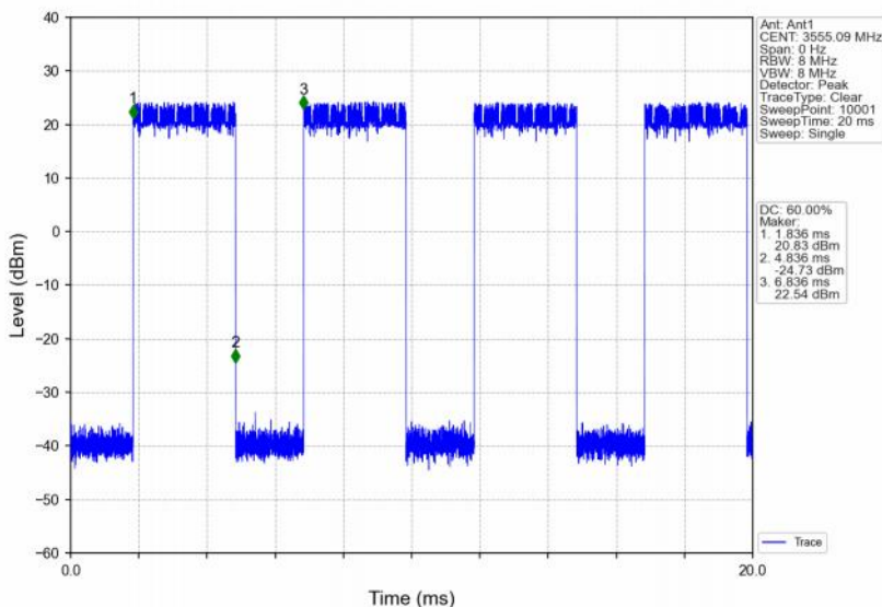
Band48_10MHz_16QAM_LCH_3555MHz_RB_25_13_NTNV
