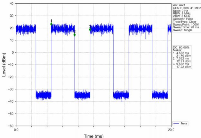
Band48_5MHz_64QAM_HCH_3697.5MHz_RB_12_13_NTNV
