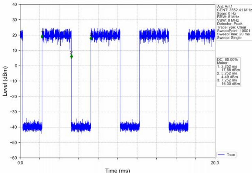
Band48_5MHz_64QAM_LCH_3552.5MHz_RB_12_13_NTNV
