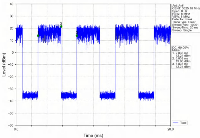
Band48_5MHz_16QAM_MCH_3625MHz_RB_1_13_NTNV
