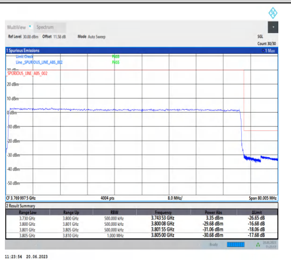
1-N78-3700-3800-PC2-30-70-H-3-CP-QPSK-Outer _Full-189@0-Ant2-1--PASS-see graph
