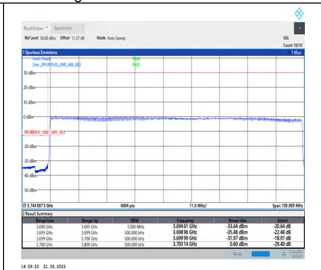
1-N78-3700-3800-PC2-30-100-L-3-CP-QPSK-Out er_Full-273@0-Ant2-1--PASS-see graph
