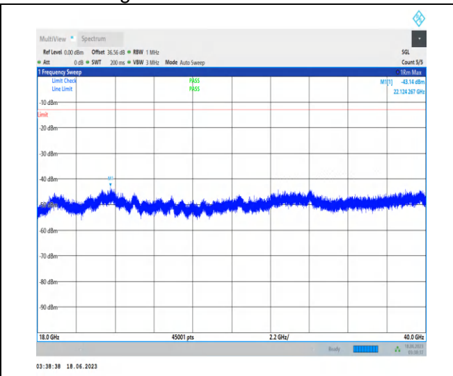
1-N78-3700-3800-PC2-30-100-L-1-N/A-DFT-PI2BPS K-Inner_1RB_Left-1@1-18000-40000-Ant2-22124.27 --43.14--13-PASS
