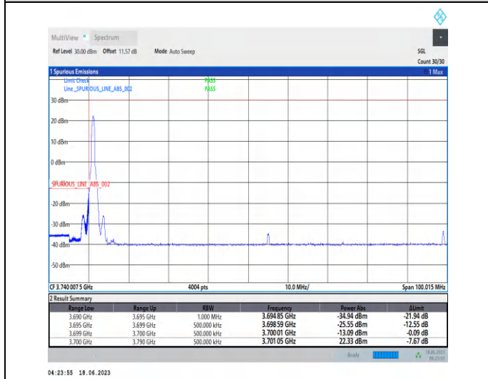
1-N78-3700-3800-PC2-30-90-L-4-CP-QPSK-Edge_1RB_Left-1@0-Ant2-1--PASS-see graph
