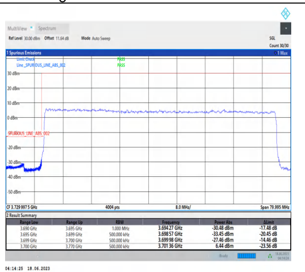
1-N78-3700-3800-PC2-30-70-L-3-DFT-PI2BPSK-Outer_Full-180@0-Ant2-1--PASS-see graph
