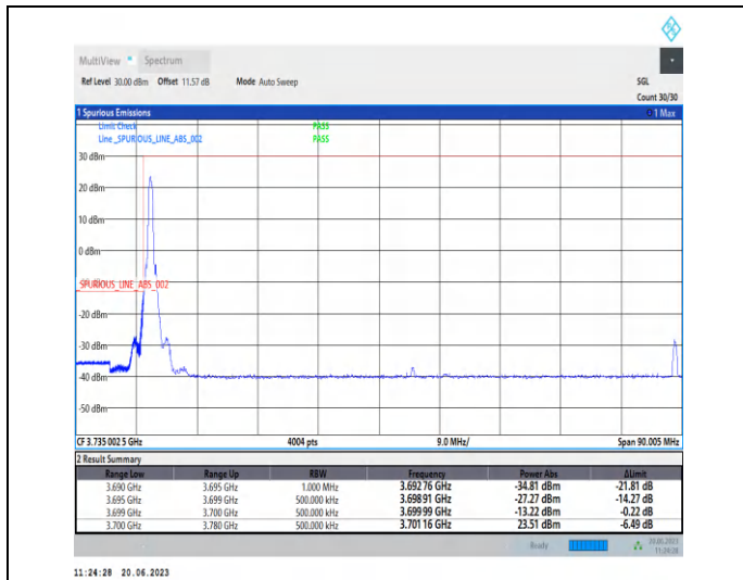
1-N78-3700-3800-PC2-30-80-L-1-CP-QPSK-Edge_1R B_Left-1@0-Ant2-1--PASS-see graph
