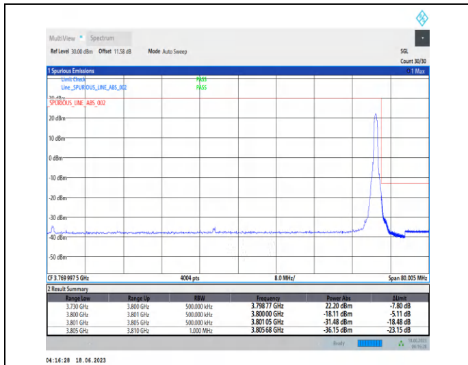
1-N78-3700-3800-PC2-30-70-H-2-DFT-PI2BPSK-Edge_1RB_Right-1@188-Ant2-1--PASS-see graph
