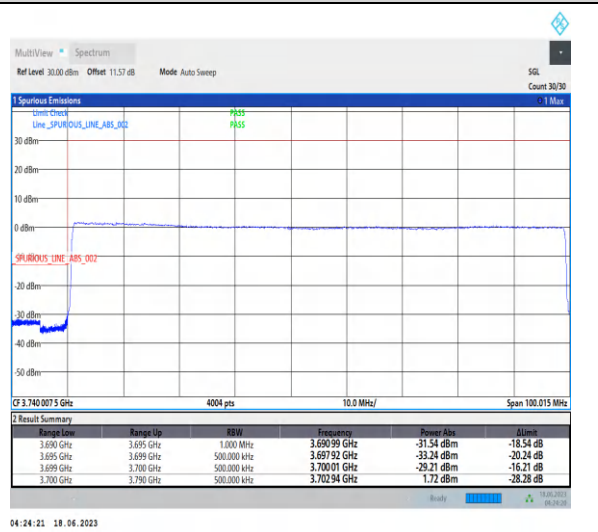
1-N78-3700-3800-PC2-30-90-L-6-CP-QPSK-Outer_Full-245@0-Ant2-1--PASS-see graph
