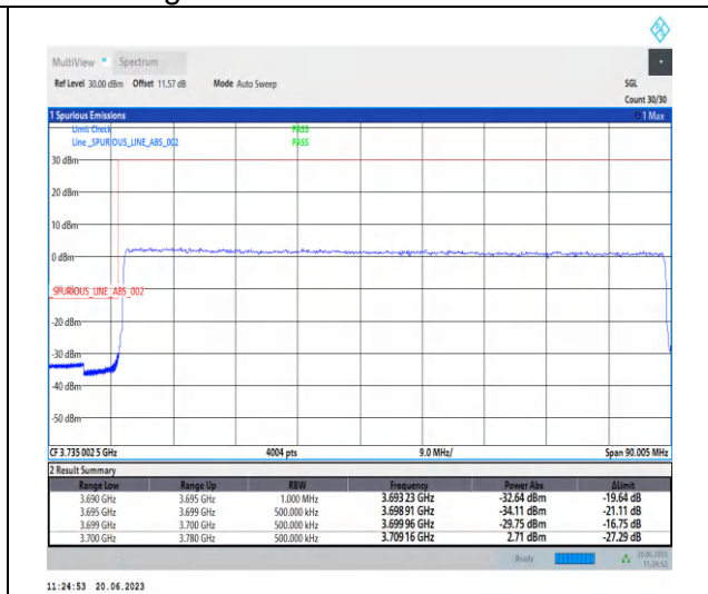
1-N78-3700-3800-PC2-30-80-L-3-CP-QPSK-Outer _Full-217@0-Ant2-1--PASS-see graph
