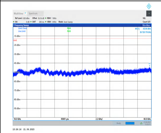
1-N78-3700-3800-PC2-30-100-M-1-N/A-DFT-QPSK-Edge_1RB_Left-1@0-18000-40000-Ant2-39728.18--43.94--13-PASS
