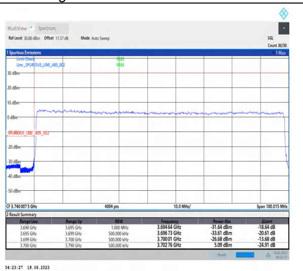
1-N78-3700-3800-PC2-30-90-L-3-DFT-PI2BPSK-Outer_Full-243@0-Ant2-1--PASS-see graph
