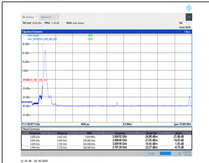
1-N78-3700-3800-PC2-30-70-L-1-CP-QPSK-Edge_1R B_Left-1@0-Ant2-1--PASS-see graph
