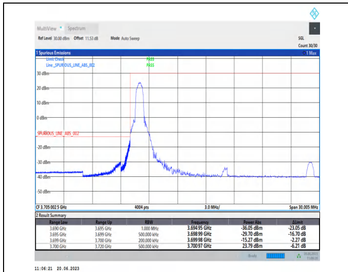
1-N78-3700-3800-PC2-30-20-L-1-CP-QPSK-Edge_1R B_Left-1@0-Ant2-1--PASS-see graph
