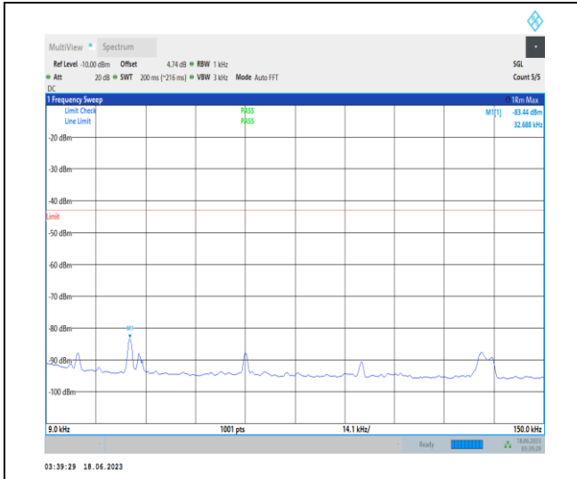
1-N78-3700-3800-PC2-30-100-H-1-N/A-DFT-PI2BP SK-Inner_1RB_Left-1@1-0.009-0.15-Ant2-0.03--83. 44--43-PASS
