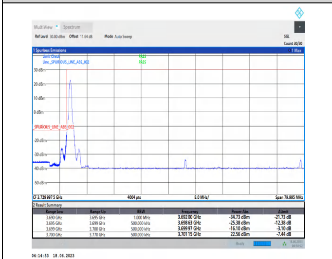
1-N78-3700-3800-PC2-30-70-L-4-CP-QPSK-Edge_1RB_Left-1@0-Ant2-1--PASS-see graph
