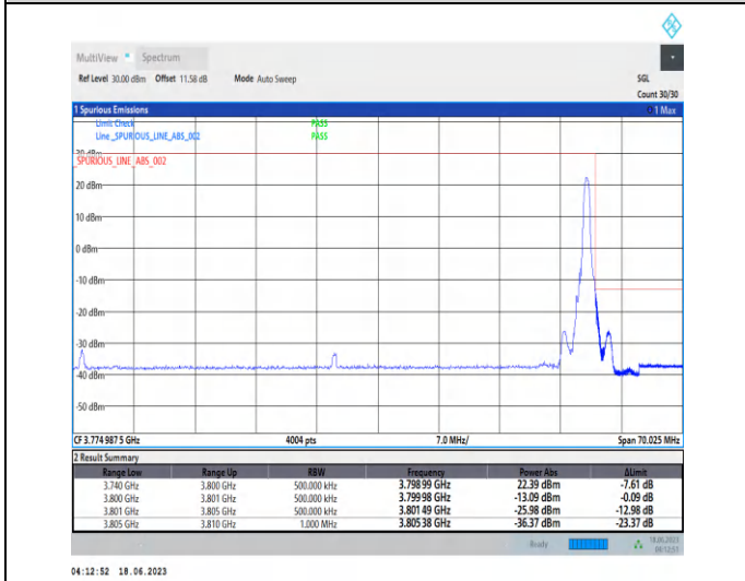
1-N78-3700-3800-PC2-30-60-H-5-CP-QPSK-Edge_1RB_Right-1@161-Ant2-1--PASS-see graph
