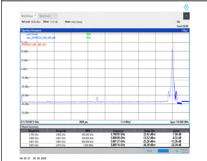
1-N78-3700-3800-PC2-30-100-H-5-CP-QPSK-Edge_1RB_Right-1@272-Ant2-1--PASS-see graph
