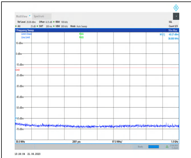
1-N78-3700-3800-PC2-30-100-M-1-N/A-DFT-QPSK-Edge_1RB_Left-1@0-30-1000-Ant2-30.00--63.27--1 3-PASS
