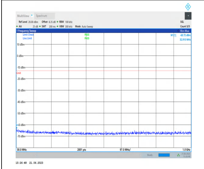
1-N78-3700-3800-PC2-30-100-H-1-N/A-DFT-QPSK-Edge_1RB_Left-1@0-30-1000-Ant2-32.91--63.72--13-PASS
