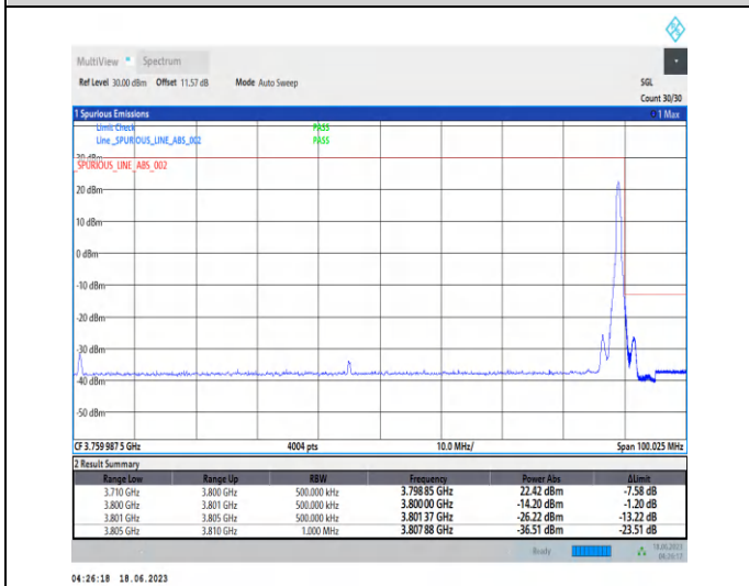
1-N78-3700-3800-PC2-30-90-H-5-CP-QPSK-Edge_1RB_Right-1@244-Ant2-1--PASS-see graph
