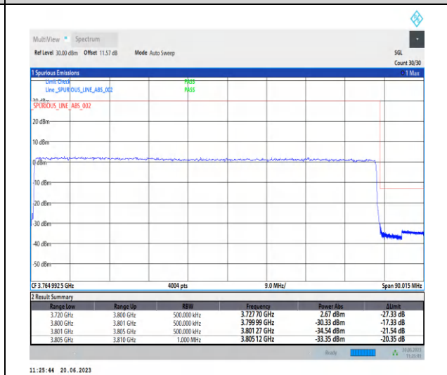
1-N78-3700-3800-PC2-30-80-H-3-CP-QPSK-Outer _Full-217@0-Ant2-1--PASS-see graph
