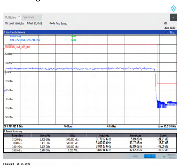
1-N78-3700-3800-PC2-30-80-H-3-DFT-PI2BPSK-Outer_Full-216@0-Ant2-1--PASS-see graph
