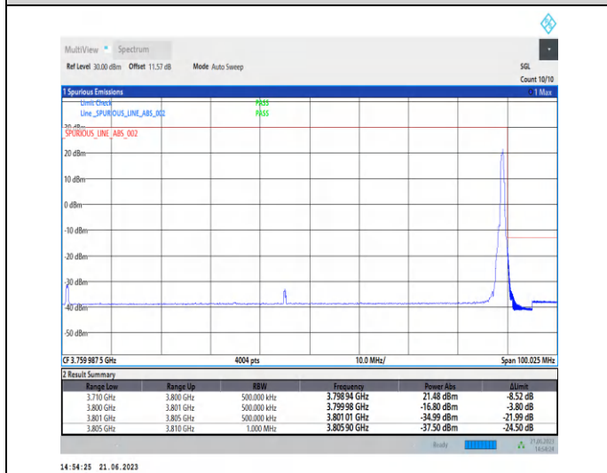
1-N78-3700-3800-PC2-30-90-H-2-CP-QPSK-Edge_1R B_Right-1@244-Ant2-1--PASS-see graph
