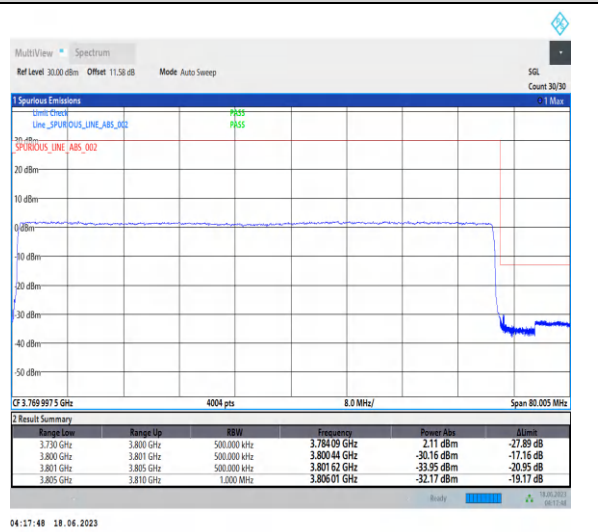
1-N78-3700-3800-PC2-30-70-H-6-CP-QPSK-Outer_Full-189@0-Ant2-1--PASS-see graph
