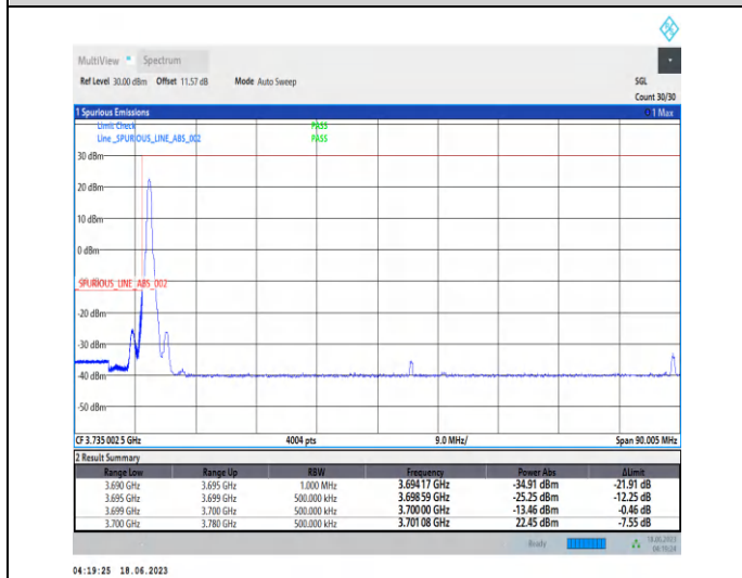
1-N78-3700-3800-PC2-30-80-L-4-CP-QPSK-Edge_1RB_Left-1@0-Ant2-1--PASS-see graph
