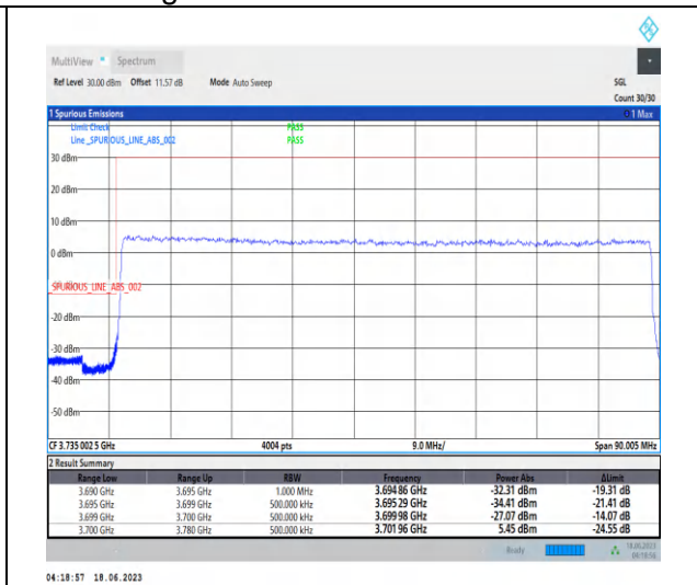
1-N78-3700-3800-PC2-30-80-L-3-DFT-PI2BPSK-Outer_Full-216@0-Ant2-1--PASS-see graph
