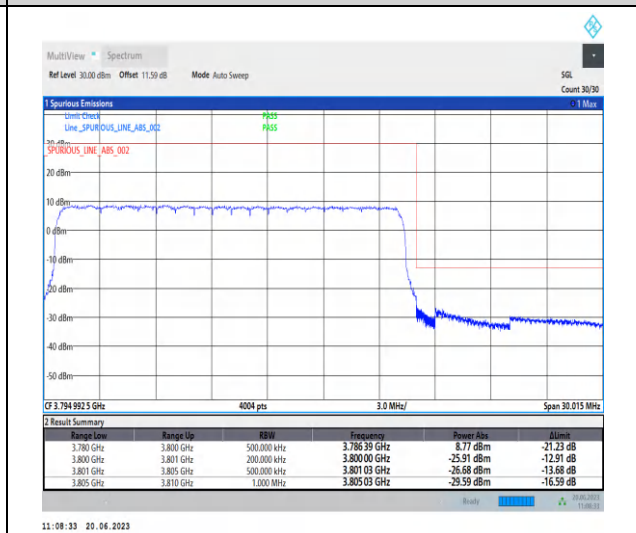
1-N78-3700-3800-PC2-30-20-H-3-CP-QPSK-Outer _Full-51@0-Ant2-1--PASS-see graph
