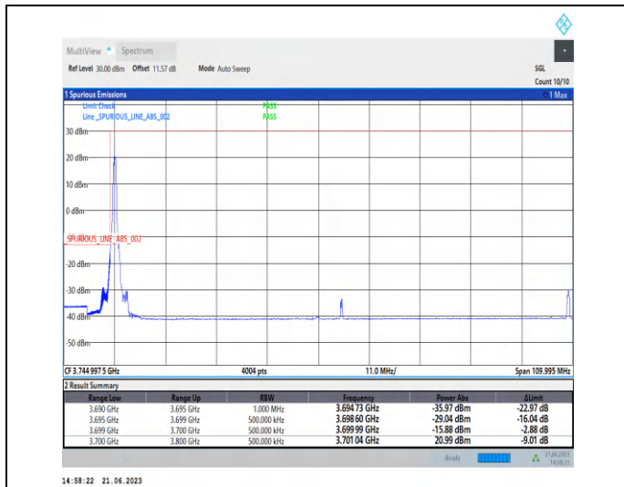
1-N78-3700-3800-PC2-30-100-L-1-CP-QPSK-Edge_1 RB_Left-1@0-Ant2-1--PASS-see graph
