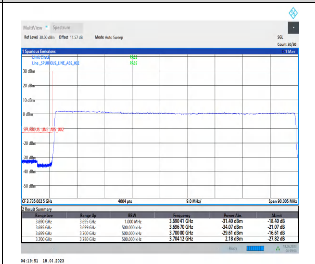
1-N78-3700-3800-PC2-30-80-L-6-CP-QPSK-Outer_Full-217@0-Ant2-1--PASS-see graph
