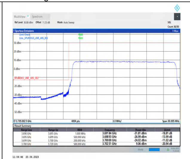
1-N78-3700-3800-PC2-30-20-L-3-CP-QPSK-Outer _Full-51@0-Ant2-1--PASS-see graph
