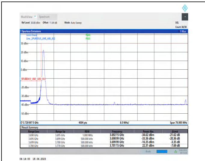
1-N78-3700-3800-PC2-30-70-L-1-DFT-PI2BPSK-Edge_1RB_Left-1@0-Ant2-1--PASS-see graph
