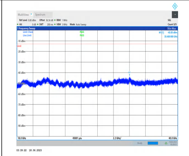
1-N78-3700-3800-PC2-30-100-M-1-N/A-DFT-PI2BPS K-Inner_1RB_Left-1@1-18000-40000-Ant2-33400.00 --43.05--13-PASS
