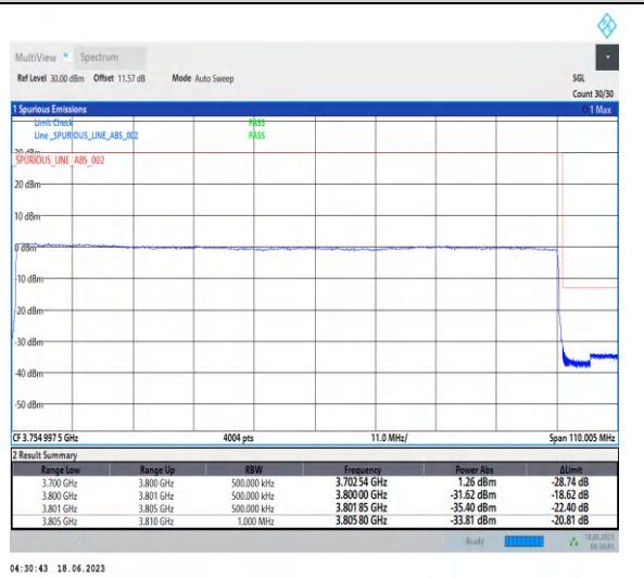
1-N78-3700-3800-PC2-30-100-H-6-CP-QPSK-Outer_Full-273@0-Ant2-1--PASS-see graph
