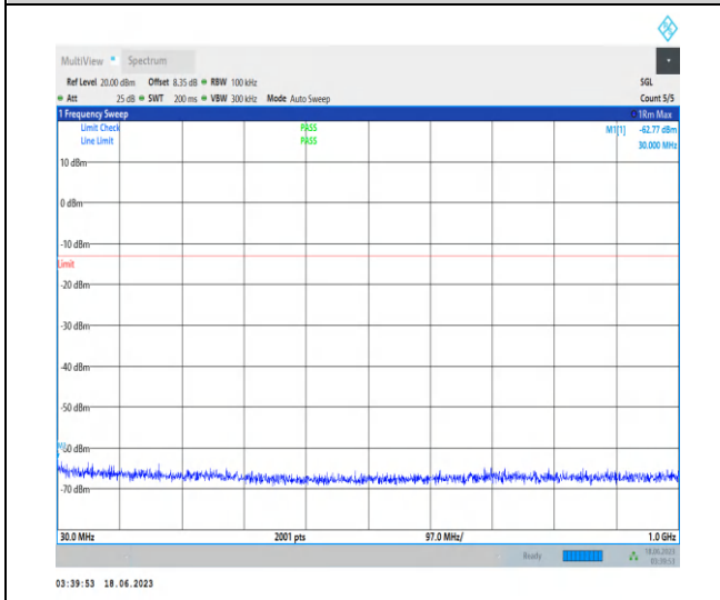
1-N78-3700-3800-PC2-30-100-H-1-N/A-DFT-PI2BP SK-Inner_1RB_Left-1@1-30-1000-Ant2-30.00--62.7 7--13-PASS
