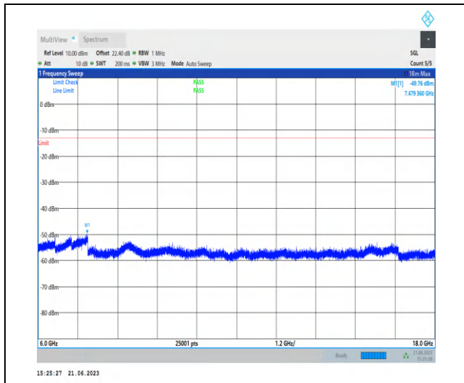
1-N78-3700-3800-PC2-30-100-L-1-N/A-DFT-QPSK-Edge_1RB_Left-1@0-6000-18000-Ant2-7479.36--49.76--13-PASS
