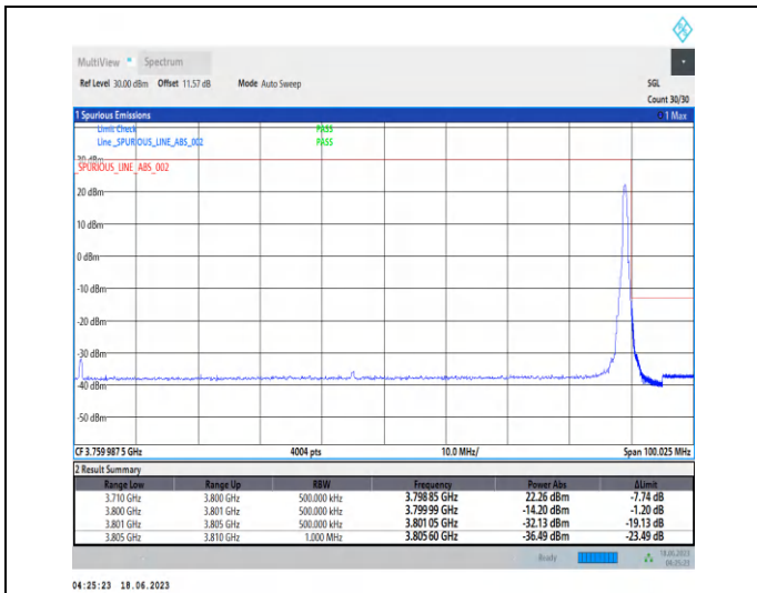
1-N78-3700-3800-PC2-30-90-H-2-DFT-PI2BPSK-Edge_1RB_Right-1@244-Ant2-1--PASS-see graph
