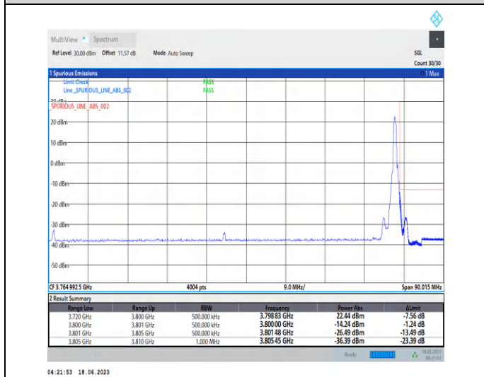
1-N78-3700-3800-PC2-30-80-H-5-CP-QPSK-Edge_1RB_Right-1@216-Ant2-1--PASS-see graph
