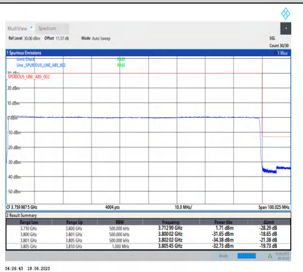
1-N78-3700-3800-PC2-30-90-H-6-CP-QPSK-Outer_Full-245@0-Ant2-1--PASS-see graph
