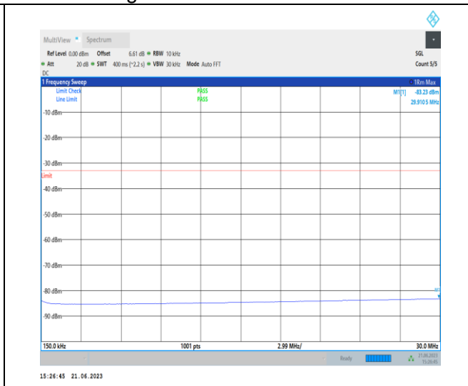
1-N78-3700-3800-PC2-30-100-H-1-N/A-DFT-QPSK-Edge_1RB_Left-1@0-0.15-30-Ant2-29.91--83.23--33-PASS
