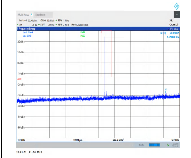
1-N78-3700-3800-PC2-30-100-H-1-N/A-DFT-QPSK-Edge_1RB_Left-1@0-1000-6000-Ant2-5570.00--28.09--9--13-PASS
