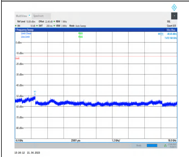
1-N78-3700-3800-PC2-30-100-M-1-N/A-DFT-QPSK-Edge_1RB_Left-1@0-6000-18000-Ant2-7472.16--49 .45--13-PASS
