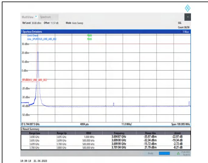
1-N78-3700-3800-PC2-30-100-L-1-DFT-PI2BPSK-Edge_1RB_Left-1@0-Ant2-1--PASS-see graph
