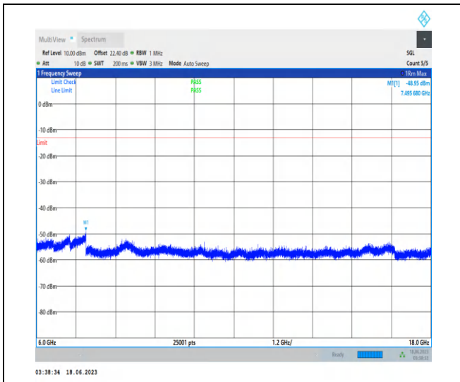
1-N78-3700-3800-PC2-30-100-L-1-N/A-DFT-PI2BP SK-Inner_1RB_Left-1@1-6000-18000-Ant2-7495.68 --48.95--13-PASS
