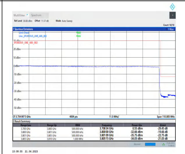
1-N78-3700-3800-PC2-30-100-H-3-CP-QPSK-Out er_Full-273@0-Ant2-1--PASS-see graph
