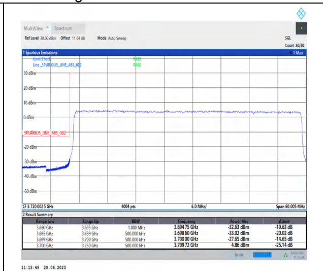
1-N78-3700-3800-PC2-30-50-L-3-CP-QPSK-Outer _Full-133@0-Ant2-1--PASS-see graph
