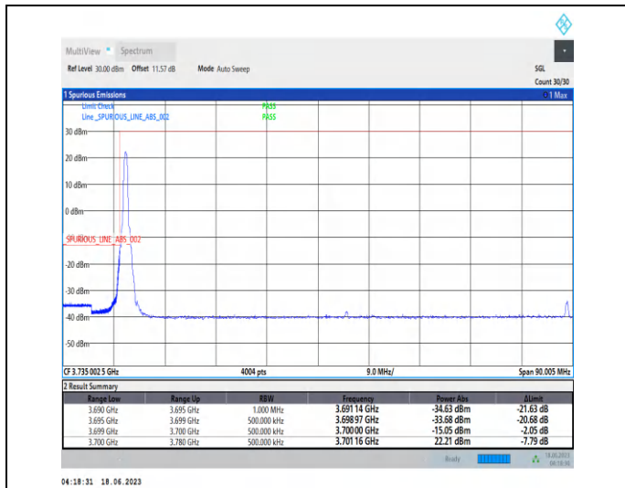
1-N78-3700-3800-PC2-30-80-L-1-DFT-PI2BPSK-Edge_1RB_Left-1@0-Ant2-1--PASS-see graph
