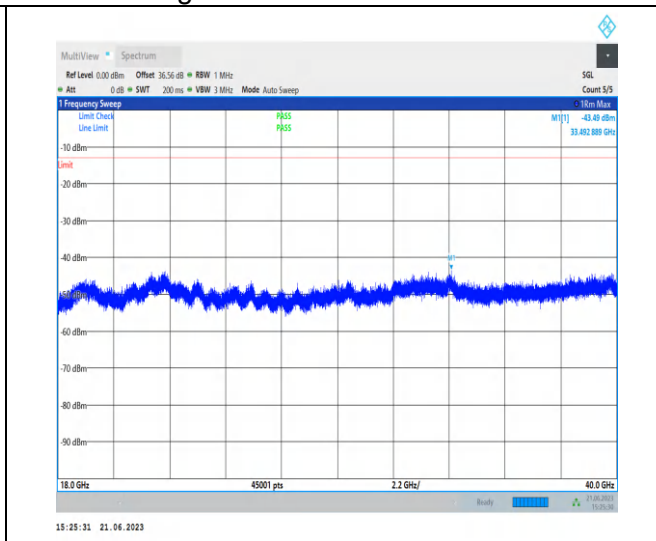
1-N78-3700-3800-PC2-30-100-L-1-N/A-DFT-QPSK-E dge_1RB_Left-1@0-18000-40000-Ant2-33492.89--43.49--13-PASS
