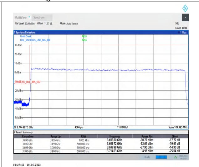
1-N78-3700-3800-PC2-30-100-L-3-DFT-PI2BPSK-Outer_Full-270@0-Ant2-1--PASS-see graph
