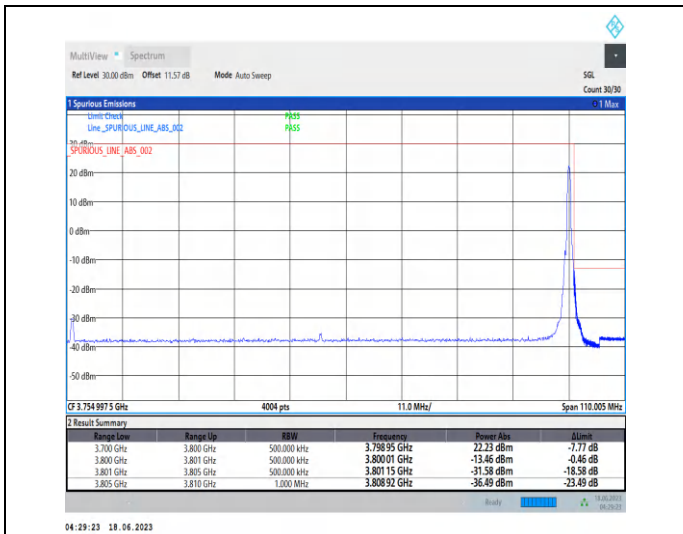
1-N78-3700-3800-PC2-30-100-H-2-DFT-PI2BPSK-Edge_1RB_Right-1@272-Ant2-1--PASS-see graph
