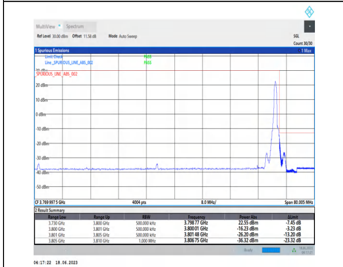
1-N78-3700-3800-PC2-30-70-H-5-CP-QPSK-Edge_1RB_Right-1@188-Ant2-1--PASS-see graph
