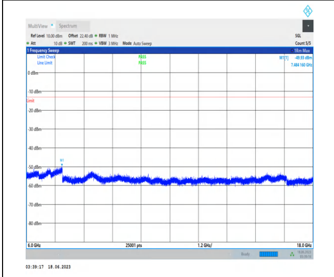
1-N78-3700-3800-PC2-30-100-M-1-N/A-DFT-PI2BP SK-Inner_1RB_Left-1@1-6000-18000-Ant2-7484.16 --49.93--13-PASS
