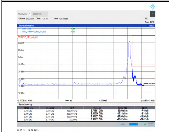
1-N78-3700-3800-PC2-30-50-H-2-CP-QPSK-Edge_1R B_Right-1@132-Ant2-1--PASS-see graph
