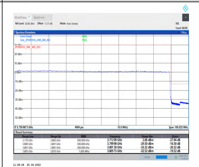
1-N78-3700-3800-PC2-30-90-H-3-CP-QPSK-Outer _Full-245@0-Ant2-1--PASS-see graph
