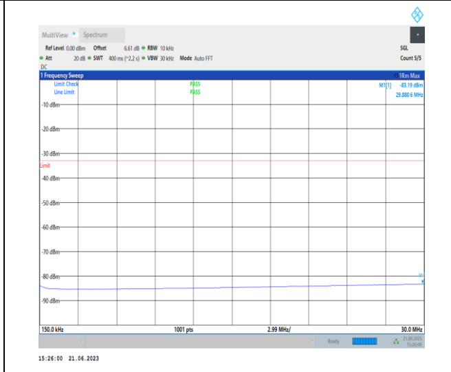
1-N78-3700-3800-PC2-30-100-M-1-N/A-DFT-QPSK-Edge_1RB_Left-1@0-0.15-30-Ant2-29.88--83.19--33-PASS
