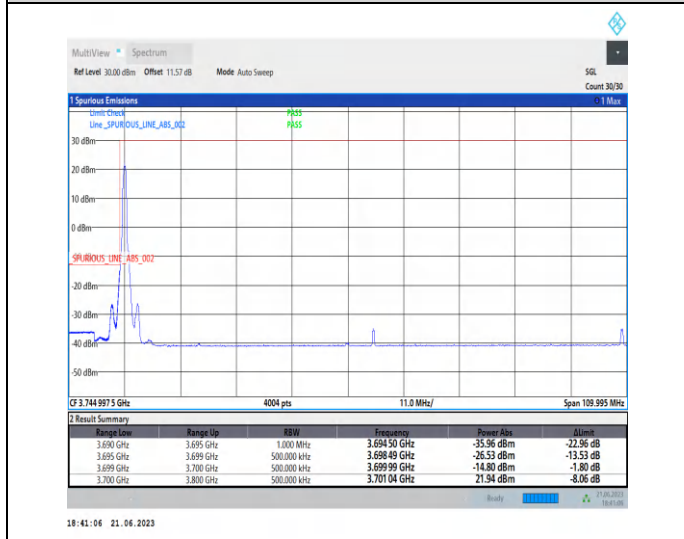
1-N78-3700-3800-PC2-30-100-L-4-CP-QPSK-Edge_1RB_Left-1@0-Ant2-1--PASS-see graph
