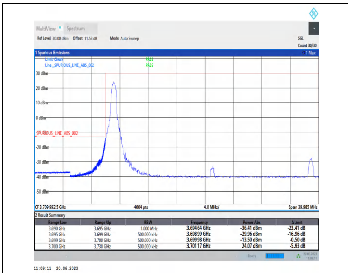
1-N78-3700-3800-PC2-30-30-L-1-CP-QPSK-Edge_1R B_Left-1@0-Ant2-1--PASS-see graph
