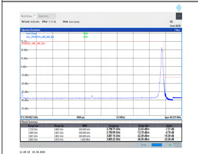
1-N78-3700-3800-PC2-30-80-H-2-CP-QPSK-Edge_1R B_Right-1@216-Ant2-1--PASS-see graph
