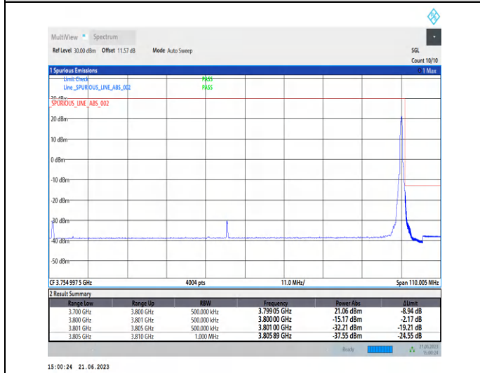
1-N78-3700-3800-PC2-30-100-H-2-CP-QPSK-Edge_1 RB_Right-1@272-Ant2-1--PASS-see graph
