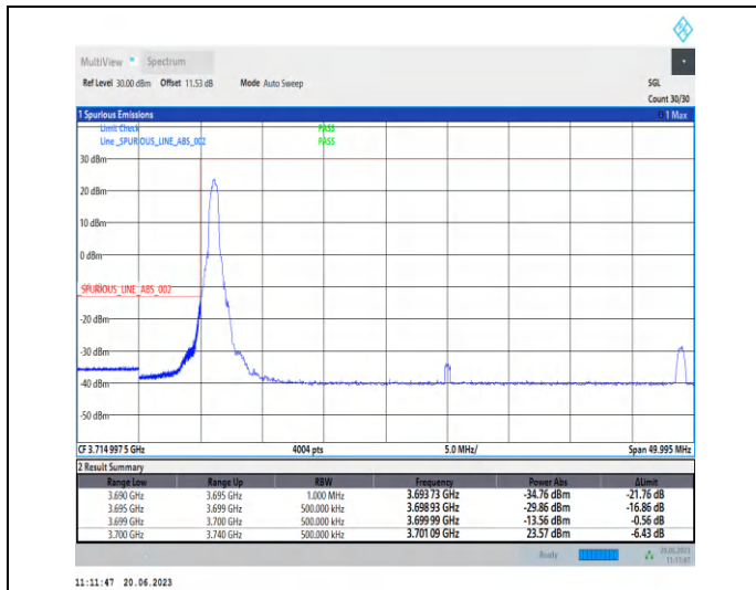
1-N78-3700-3800-PC2-30-40-L-1-CP-QPSK-Edge_1R B_Left-1@0-Ant2-1--PASS-see graph
