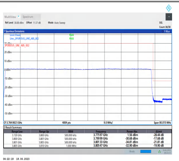
1-N78-3700-3800-PC2-30-80-H-6-CP-QPSK-Outer_Full-217@0-Ant2-1--PASS-see graph
