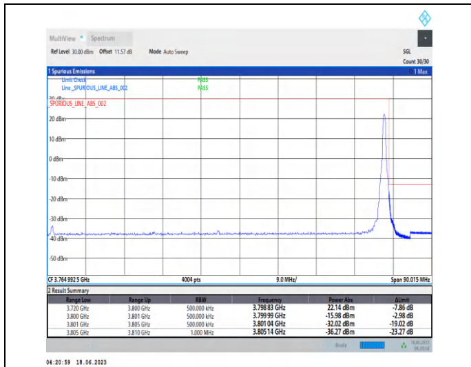
1-N78-3700-3800-PC2-30-80-H-2-DFT-PI2BPSK-Edge_1RB_Right-1@216-Ant2-1--PASS-see graph
