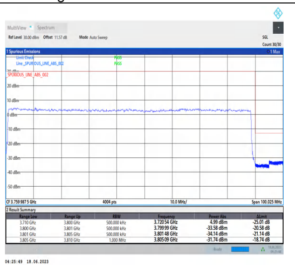
1-N78-3700-3800-PC2-30-90-H-3-DFT-PI2BPSK-Outer_Full-243@0-Ant2-1--PASS-see graph
