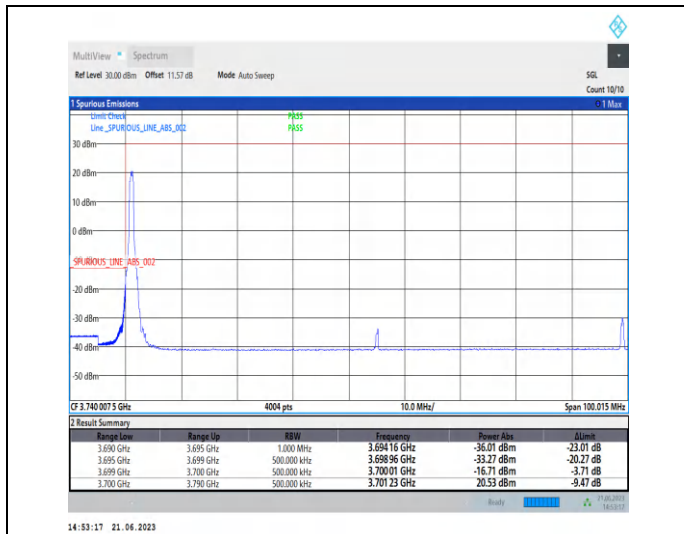
1-N78-3700-3800-PC2-30-90-L-1-CP-QPSK-Edge_1R B_Left-1@0-Ant2-1--PASS-see graph
