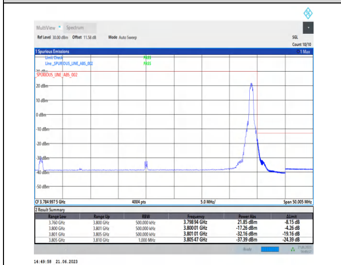
1-N78-3700-3800-PC2-30-40-H-2-CP-QPSK-Edge_1R B_Right-1@105-Ant2-1--PASS-see graph
