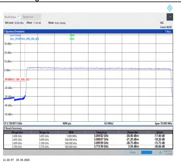
1-N78-3700-3800-PC2-30-70-L-3-CP-QPSK-Outer _Full-189@0-Ant2-1--PASS-see graph
