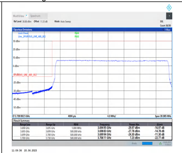
1-N78-3700-3800-PC2-30-30-L-3-CP-QPSK-Outer _Full-78@0-Ant2-1--PASS-see graph
