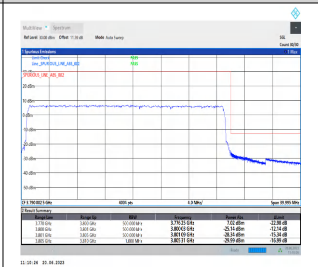
1-N78-3700-3800-PC2-30-30-H-3-CP-QPSK-Outer _Full-78@0-Ant2-1--PASS-see graph
