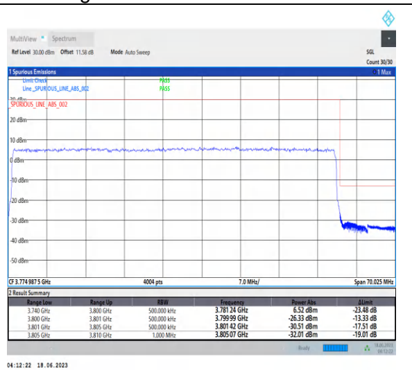
1-N78-3700-3800-PC2-30-60-H-3-DFT-PI2BPSK-Outer_Full-162@0-Ant2-1--PASS-see graph
