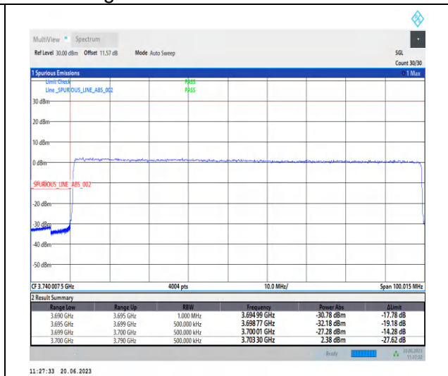
1-N78-3700-3800-PC2-30-90-L-3-CP-QPSK-Outer _Full-245@0-Ant2-1--PASS-see graph
