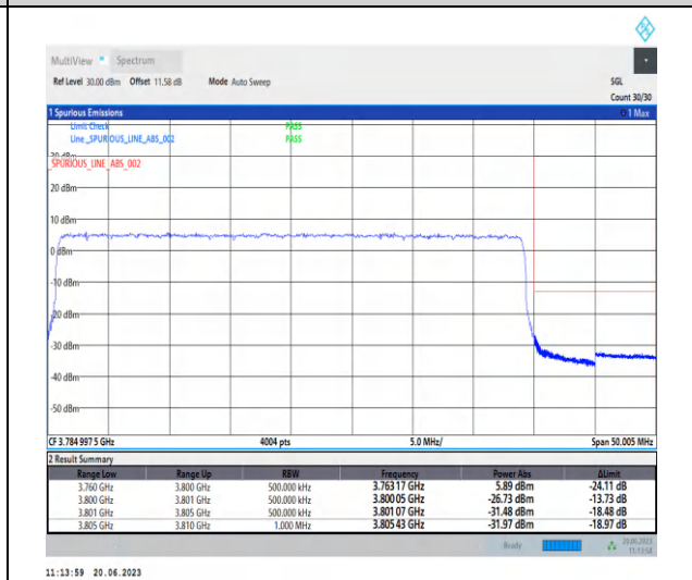
1-N78-3700-3800-PC2-30-40-H-3-CP-QPSK-Outer _Full-106@0-Ant2-1--PASS-see graph
