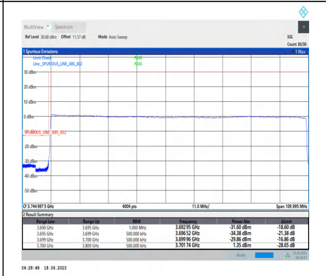
1-N78-3700-3800-PC2-30-100-L-6-CP-QPSK-Outer_Full-273@0-Ant2-1--PASS-see graph
