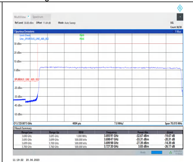
1-N78-3700-3800-PC2-30-60-L-3-CP-QPSK-Outer _Full-162@0-Ant2-1--PASS-see graph
