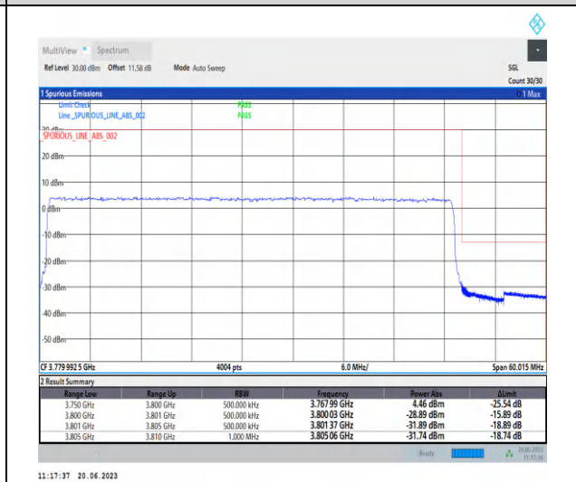
1-N78-3700-3800-PC2-30-50-H-3-CP-QPSK-Outer _Full-133@0-Ant2-1--PASS-see graph
