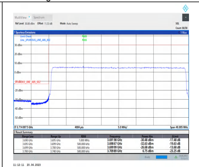
1-N78-3700-3800-PC2-30-40-L-3-CP-QPSK-Outer _Full-106@0-Ant2-1--PASS-see graph
