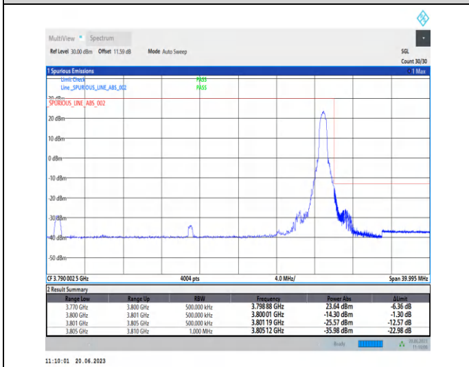
1-N78-3700-3800-PC2-30-30-H-2-CP-QPSK-Edge_1R B_Right-1@77-Ant2-1--PASS-see graph
