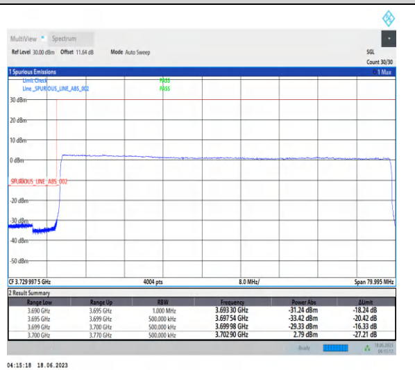
1-N78-3700-3800-PC2-30-70-L-6-CP-QPSK-Outer_Full-189@0-Ant2-1--PASS-see graph
