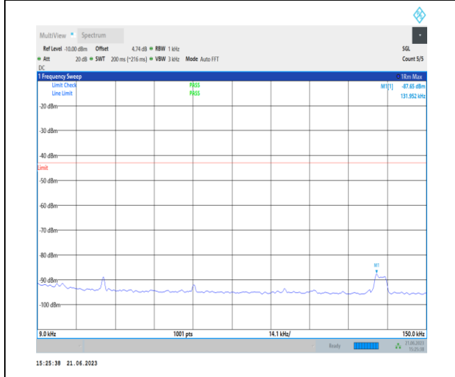
1-N78-3700-3800-PC2-30-100-M-1-N/A-DFT-QPSK-Edge_1RB_Left-1@0-0.009-0.15-Ant2-0.13--87.65--43-PASS
