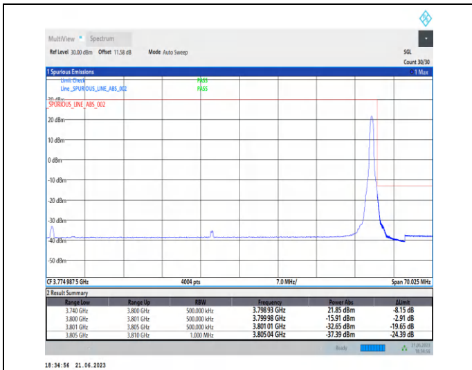
1-N78-3700-3800-PC2-30-60-H-2-DFT-PI2BPSK-Edge_1RB_Right-1@161-Ant2-1--PASS-see graph
