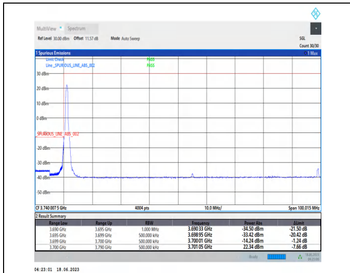
1-N78-3700-3800-PC2-30-90-L-1-DFT-PI2BPSK-Edge_1RB_Left-1@0-Ant2-1--PASS-see graph
