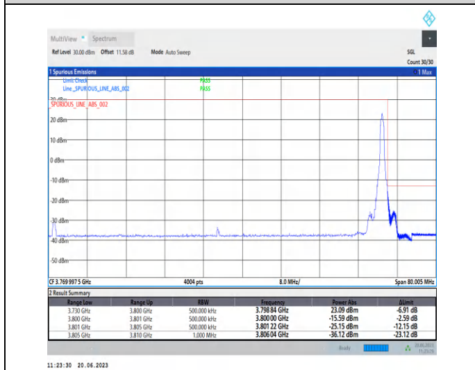
1-N78-3700-3800-PC2-30-70-H-2-CP-QPSK-Edge_1R B_Right-1@188-Ant2-1--PASS-see graph
