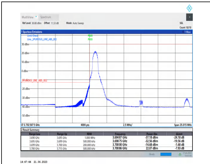
1-N78-3700-3800-PC2-30-15-L-1-CP-QPSK-Edge_1R B_Left-1@0-Ant2-1--PASS-see graph
