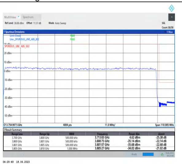
1-N78-3700-3800-PC2-30-100-H-3-DFT-PI2BPSK-Outer_Full-270@0-Ant2-1--PASS-see graph
