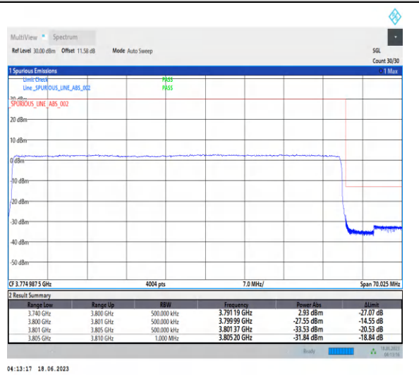
1-N78-3700-3800-PC2-30-60-H-6-CP-QPSK-Outer_Full-162@0-Ant2-1--PASS-see graph
