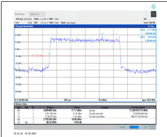
1-N78-3700-3800-PC2-30-80-L-1-DFT-PI2BPSK-Out er_Full-216@0-Ant2-77.241-80.320-≤80-PASS
