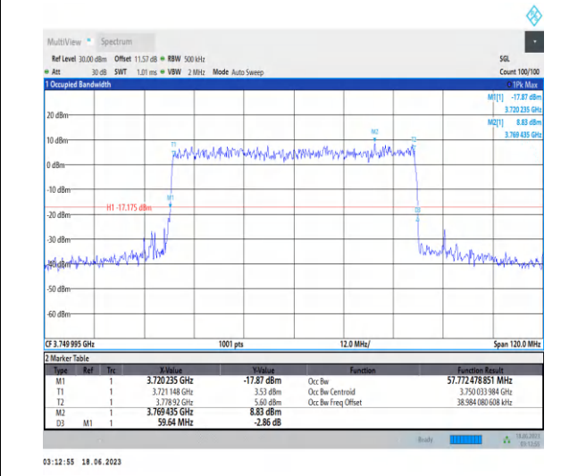
1-N78-3700-3800-PC2-30-60-M-9-CP-256QAM-Outer_Full-162@0-Ant2-57.772-59.640-≤60-PASS
