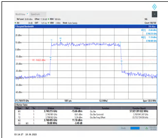
1-N78-3700-3800-PC2-30-60-H-5-DFT-256QAM-Out er_Full-162@0-Ant2-57.921-59.880-≤60-PASS
