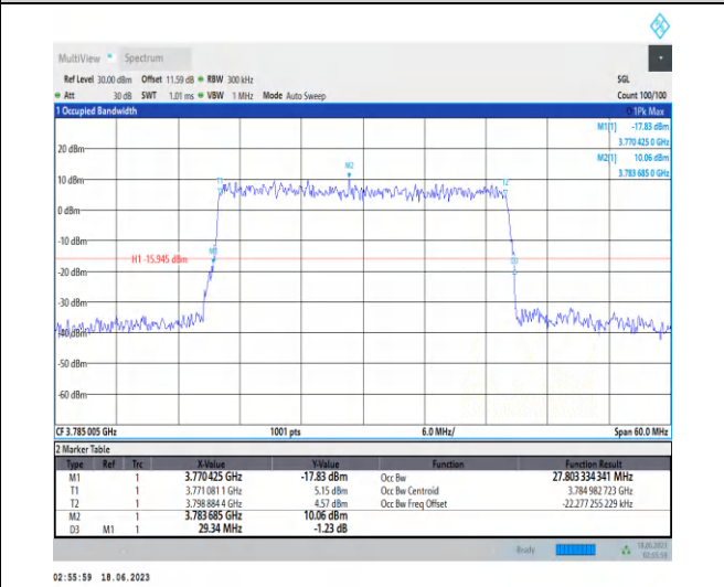
1-N78-3700-3800-PC2-30-30-H-9-CP-256QAM-Outer_Full-78@0-Ant2-27.803-29.340-≤30-PASS
