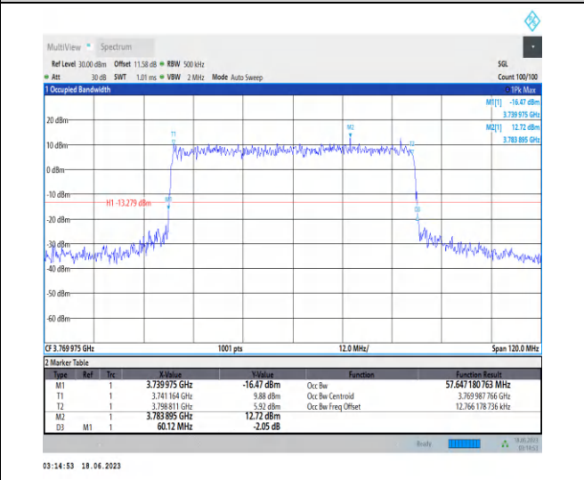
1-N78-3700-3800-PC2-30-60-H-8-CP-64QAM-Outer_Full-162@0-Ant2-57.647-60.120-≤60-PASS
