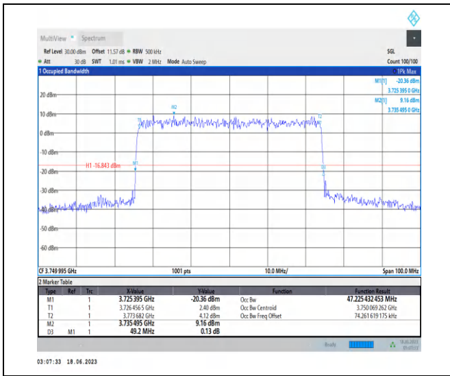
1-N78-3700-3800-PC2-30-50-M-9-CP-256QAM-Out er_Full-133@0-Ant2-47.225-49.200-≤50-PASS
