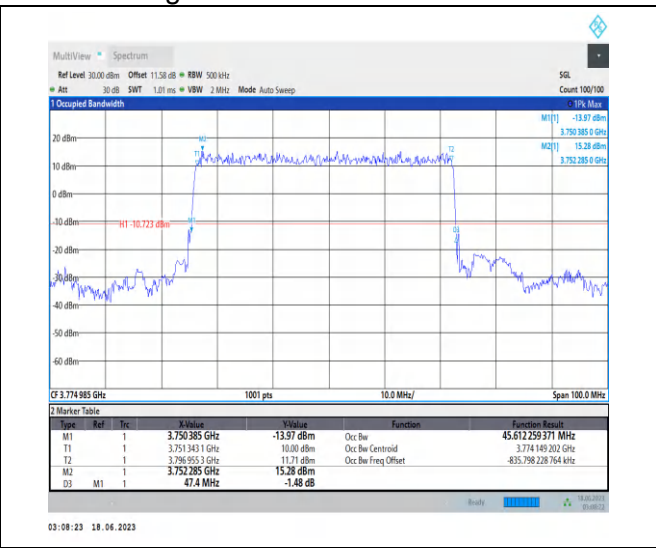
1-N78-3700-3800-PC2-30-50-H-1-DFT-PI2BPSK-Ou ter_Full-128@0-Ant2-45.612-47.400-≤50-PASS
