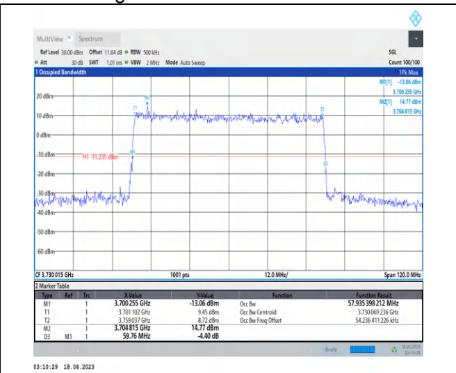
1-N78-3700-3800-PC2-30-60-L-4-DFT-64QAM-Outer_Full-162@0-Ant2-57.935-59.760-≤60-PASS
