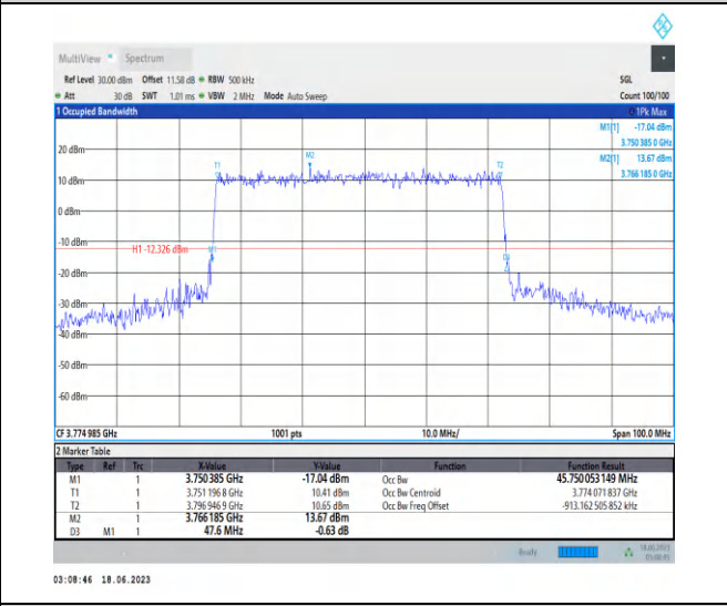
1-N78-3700-3800-PC2-30-50-H-3-DFT-16QAM-Out er_Full-128@0-Ant2-45.75-47.600-≤50-PASS
