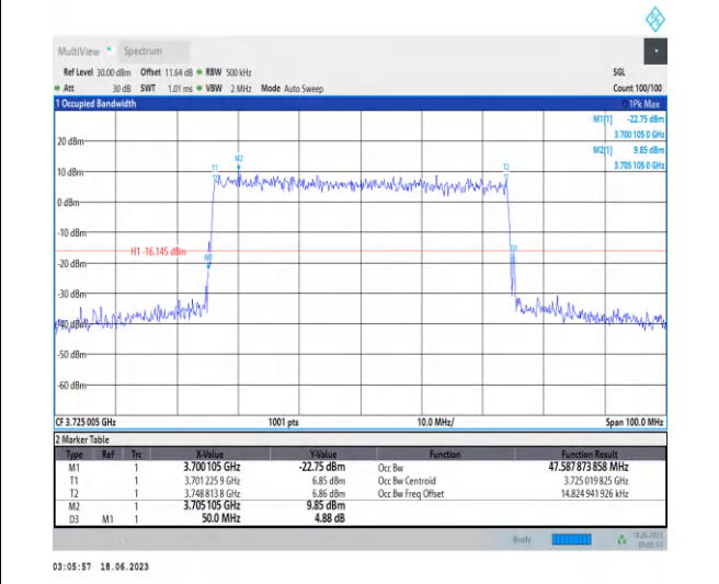
1-N78-3700-3800-PC2-30-50-L-9-CP-256QAM-Outer_Full-133@0-Ant2-47.588-50.000-≤50-PASS
