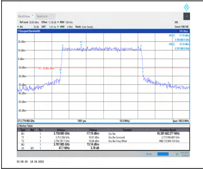
1-N78-3700-3800-PC2-30-50-H-2-DFT-QPSK-Out er_Full-128@0-Ant2-45.582-47.700-≤50-PASS
