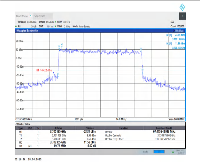
1-N78-3700-3800-PC2-30-70-L-7-CP-16QAM-Outer_Full-189@0-Ant2-67.475-69.720-≤70-PASS
