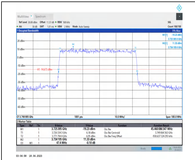
1-N78-3700-3800-PC2-30-50-M-5-DFT-256QAM-Out_Full-128@0-Ant2-45.46-47.400-≤50-PASS
