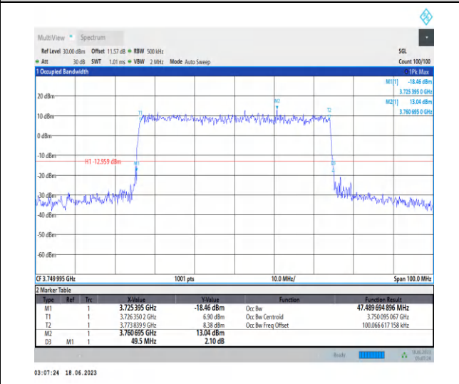
1-N78-3700-3800-PC2-30-50-M-8-CP-64QAM-Outer_Full-133@0-Ant2-47.49-49.500-≤50-PASS
