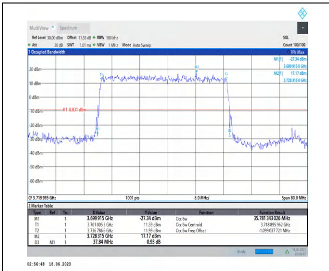
1-N78-3700-3800-PC2-30-40-L-1-DFT-PI2BPSK-Out er_Full-100@0-Ant2-35.781-37.840-≤40-PASS
