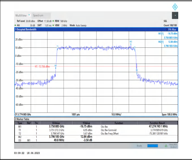
1-N78-3700-3800-PC2-30-50-H-7-CP-16QAM-Outer_Full-133@0-Ant2-47.275-49.800-≤50-PASS
