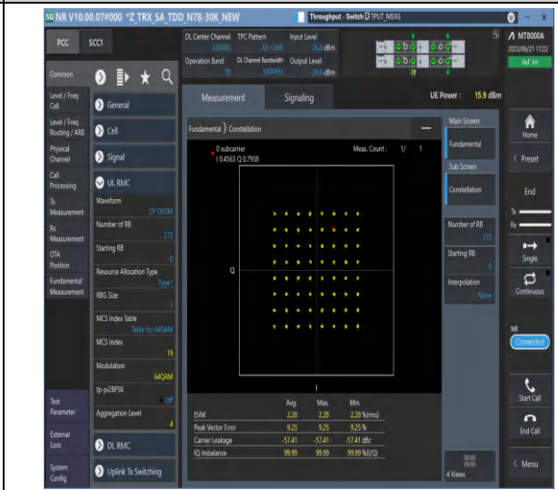
1-N78-3700-3800-PC2-30-100-M-8-CP-64QAM-Outer_Full-273@0-Ant2-see graph-PASS
