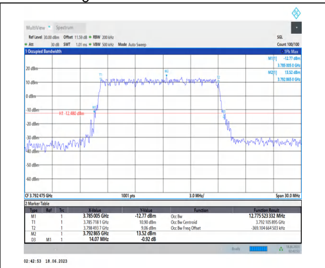
1-N78-3700-3800-PC2-30-15-H-5-DFT-256QAM-Outer_Full-36@0-Ant2-12.776-14.070-≤15-PASS
