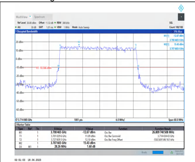
1-N78-3700-3800-PC2-30-30-L-1-DFT-PI2BPSK-Outer_Full-75@0-Ant2-26.81-28.260-<=30-PASS
