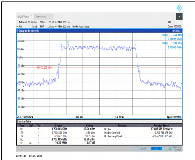
1-N78-3700-3800-PC2-30-20-L-3-DFT-16QAM-Outer_Full-50@0-Ant2-17.886-19.240-≤20-PASS
