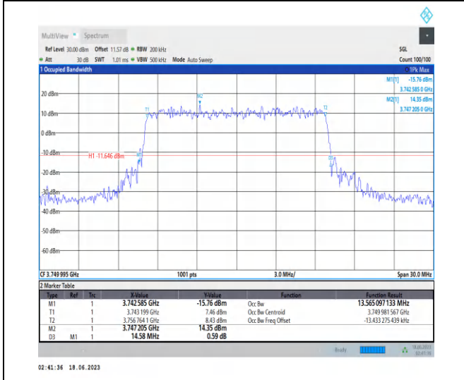
1-N78-3700-3800-PC2-30-15-M-7-CP-16QAM-Outer _Full-38@0-Ant2-13.565-14.580-≤15-PASS
