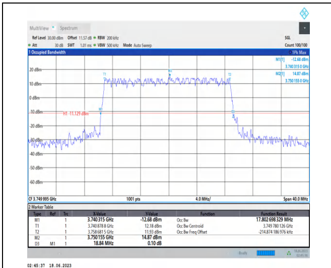
1-N78-3700-3800-PC2-30-20-M-2-DFT-QPSK-Outer_Full-50@0-Ant2-17.803-18.840-≤20-PASS
