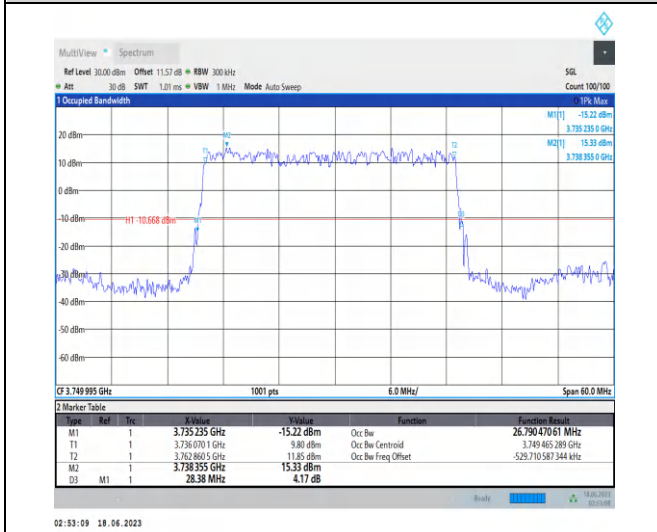
1-N78-3700-3800-PC2-30-30-M-1-DFT-PI2BPSK-Outer_Full-75@0-Ant2-26.79-28.380-≤30-PASS
