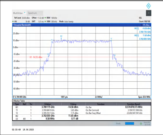
1-N78-3700-3800-PC2-30-10-L-8-CP-64QAM-Outer _Full-24@0-Ant2-8.575-9.580-≤10-PASS
