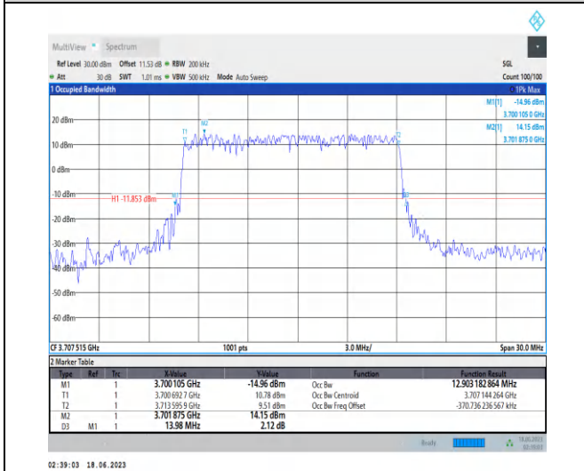
1-N78-3700-3800-PC2-30-15-L-4-DFT-64QAM-Outer_Full-36@0-Ant2-12.903-13.980-≤15-PASS
