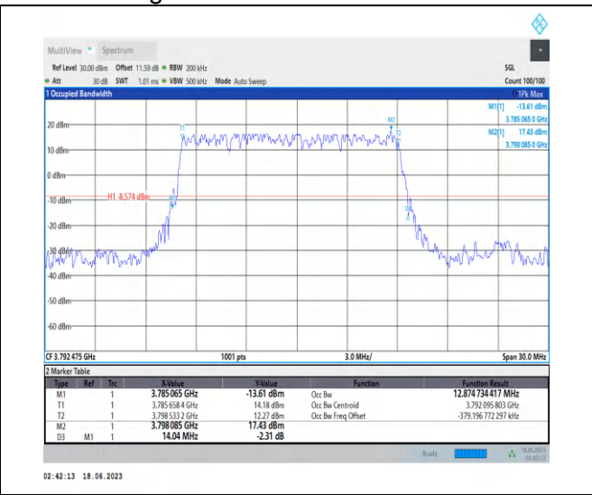
1-N78-3700-3800-PC2-30-15-H-1-DFT-PI2BPSK-Ou_Full-36@0-Ant2-12.875-14.040-≤15-PASS
