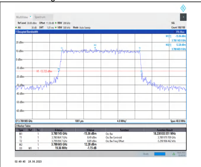
1-N78-3700-3800-PC2-30-20-H-6-CP-QPSK-Outer_Full-51@0-Ant2-18.23-19.360-≤20-PASS
