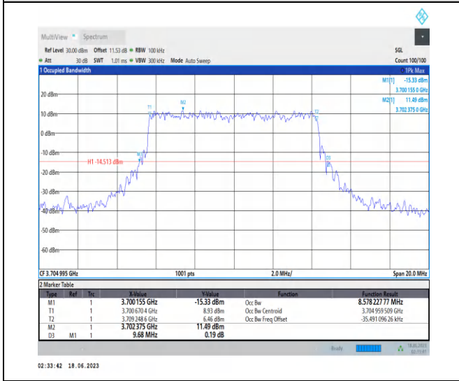
1-N78-3700-3800-PC2-30-10-L-7-CP-16QAM-Outer _Full-24@0-Ant2-8.578-9.680-≤10-PASS
