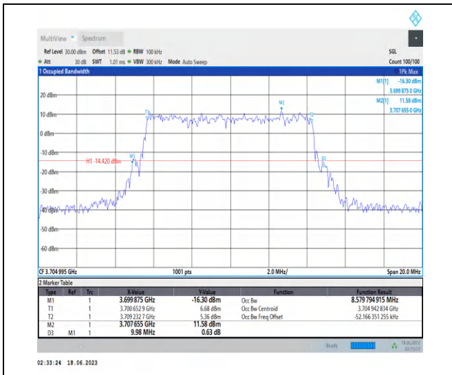
1-N78-3700-3800-PC2-30-10-L-5-DFT-256QAM-Out er_Full-24@0-Ant2-8.58-9.980-≤10-PASS
