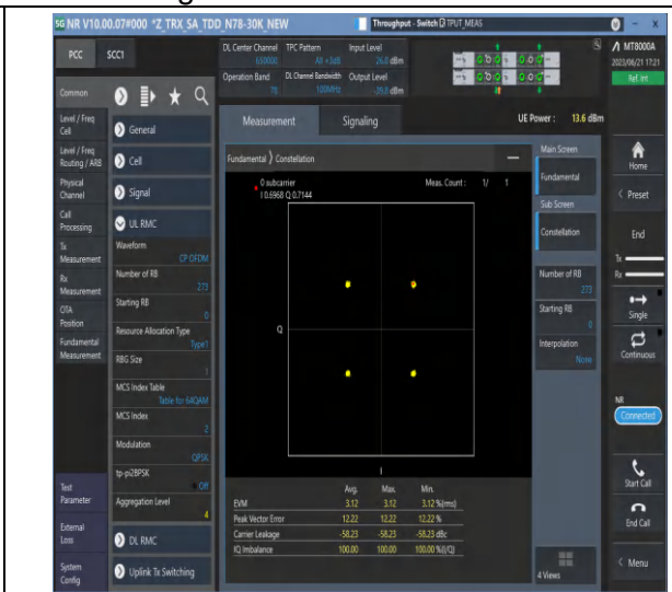
1-N78-3700-3800-PC2-30-100-M-6-CP-QPSK-Outer_Full-273@0-Ant2-see graph-PASS
