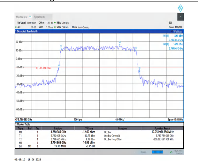
1-N78-3700-3800-PC2-30-20-H-2-DFT-QPSK-Outer_Full-50@0-Ant2-17.752-19.160-≤20-PASS
