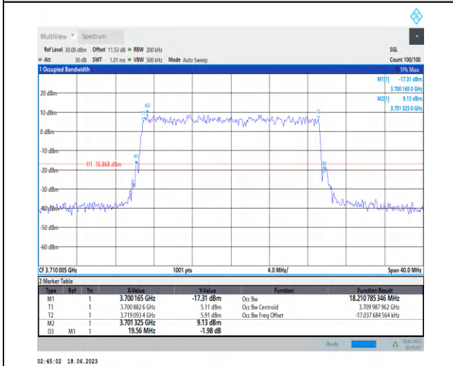
1-N78-3700-3800-PC2-30-20-L-9-CP-256QAM-Outer_Full-51@0-Ant2-18.211-19.560-≤20-PASS
