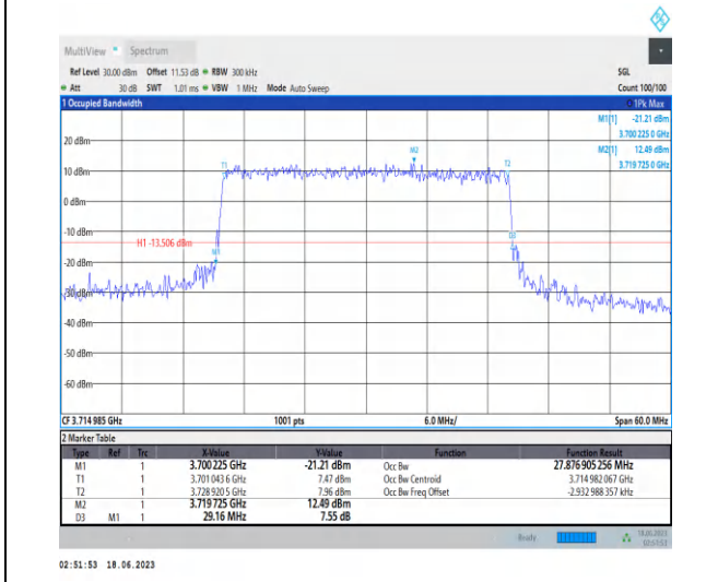
1-N78-3700-3800-PC2-30-30-L-6-CP-QPSK-Outer_Full-78@0-Ant2-27.877-29.160-≤30-PASS
