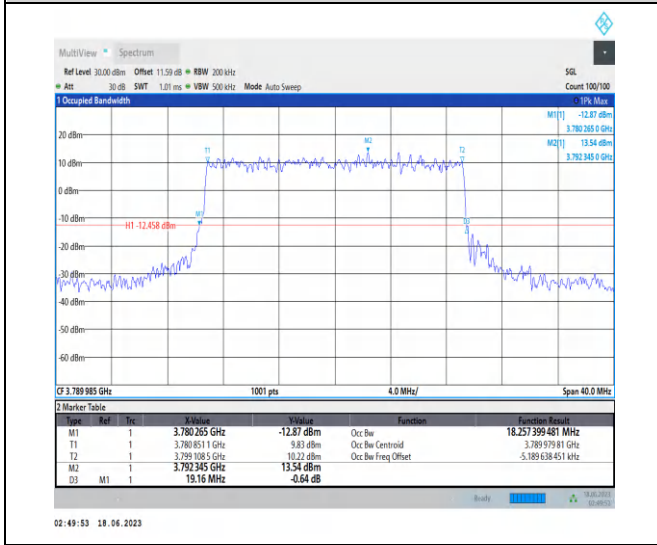
1-N78-3700-3800-PC2-30-20-H-7-CP-16QAM-Outer_Full-51@0-Ant2-18.257-19.160-≤20-PASS
