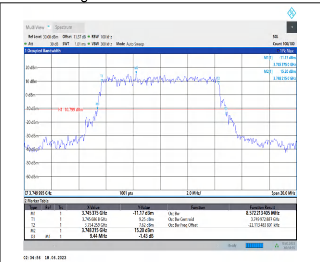
1-N78-3700-3800-PC2-30-10-M-1-DFT-PI2BPSK-Outer_Full-24@0-Ant2-8.572-9.440-≤10-PASS
