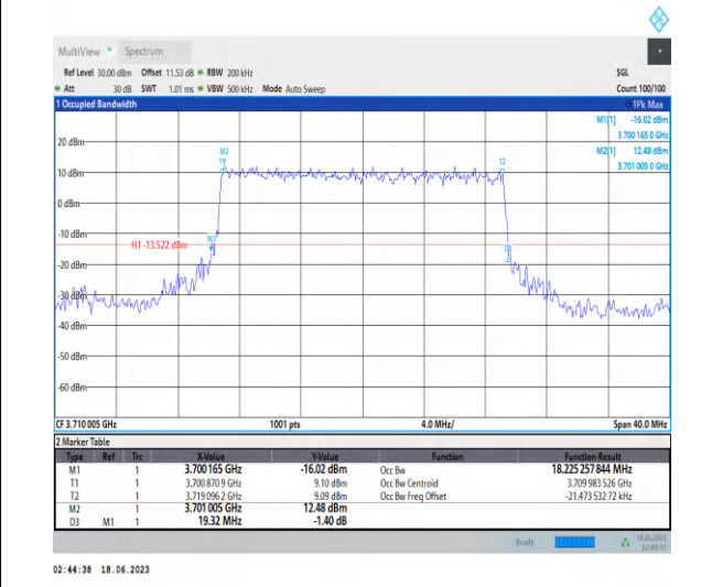
1-N78-3700-3800-PC2-30-20-L-6-CP-QPSK-Outer_Full-51@0-Ant2-18.225-19.320-≤20-PASS
