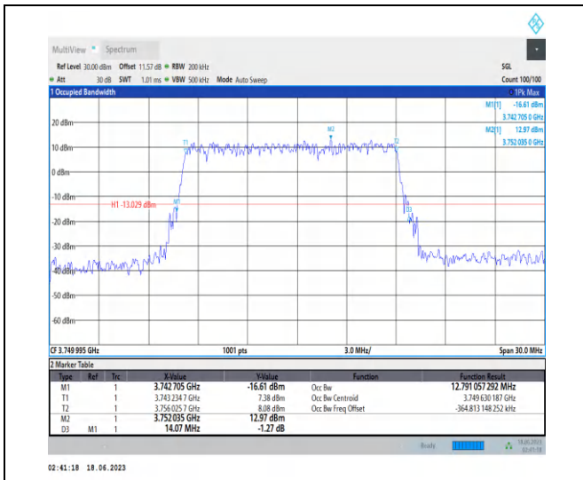
1-N78-3700-3800-PC2-30-15-M-5-DFT-256QAM-Out er_Full-36@0-Ant2-12.791-14.070-≤15-PASS
