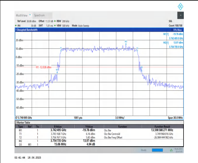
1-N78-3700-3800-PC2-30-15-M-8-CP-64QAM-Outer _Full-38@0-Ant2-13.599-15.060-≤15-PASS
