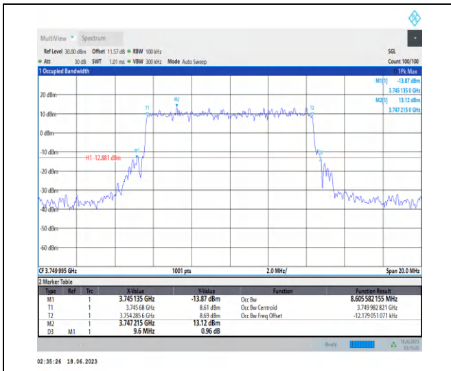
1-N78-3700-3800-PC2-30-10-M-4-DFT-64QAM-Outer_Full-24@0-Ant2-8.606-9.600-≤10-PASS
