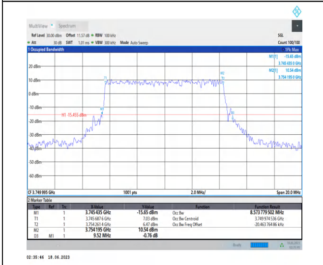
1-N78-3700-3800-PC2-30-10-M-6-CP-QPSK-Outer_Full-24@0-Ant2-8.574-9.520-≤10-PASS
