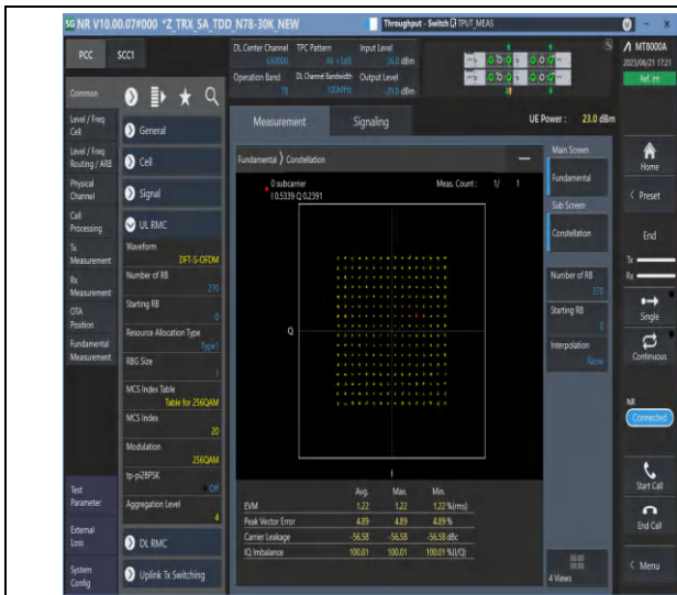
1-N78-3700-3800-PC2-30-100-M-5-DFT-256QAM-Outer_Full-270@0-Ant2-see graph-PASS
