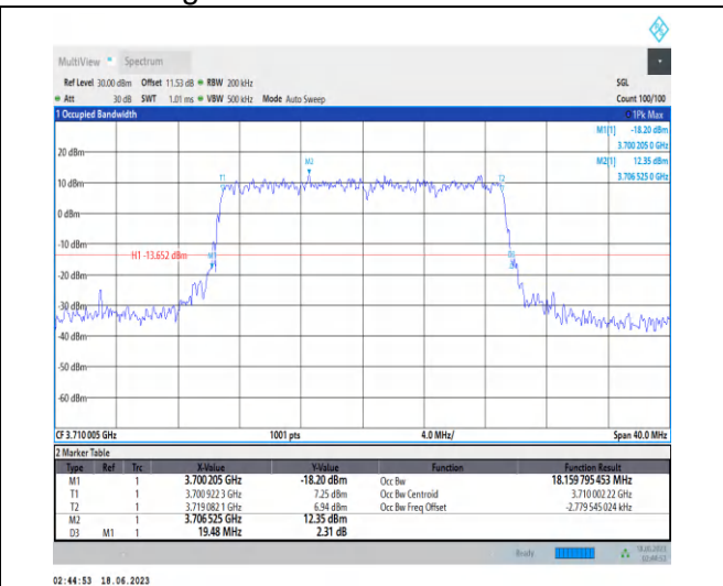
1-N78-3700-3800-PC2-30-20-L-8-CP-64QAM-Outer_Full-51@0-Ant2-18.16-19.480-≤20-PASS
