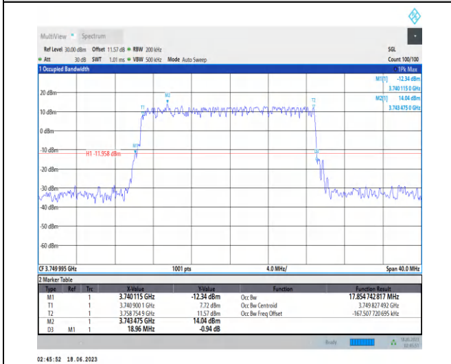
1-N78-3700-3800-PC2-30-20-M-4-DFT-64QAM-Outer_Full-50@0-Ant2-17.855-18.960-≤20-PASS
