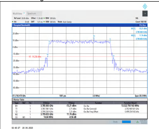
1-N78-3700-3800-PC2-30-15-H-9-CP-256QAM-Outer_Full-38@0-Ant2-13.523-14.640-≤15-PASS
