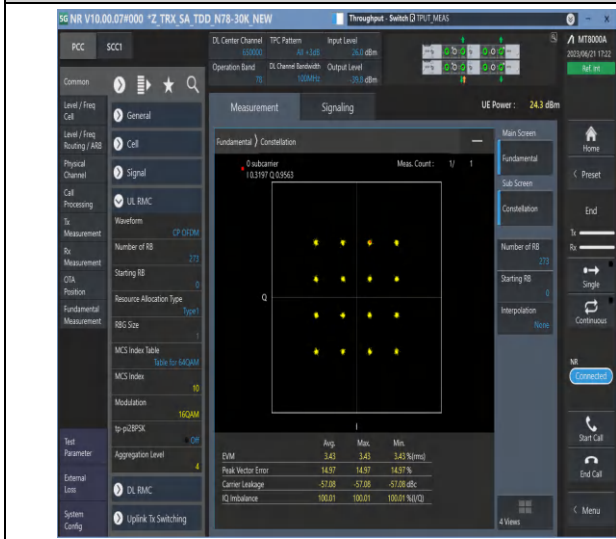
1-N78-3700-3800-PC2-30-100-M-7-CP-16QAM-Outer_Full-273@0-Ant2-see graph-PASS
