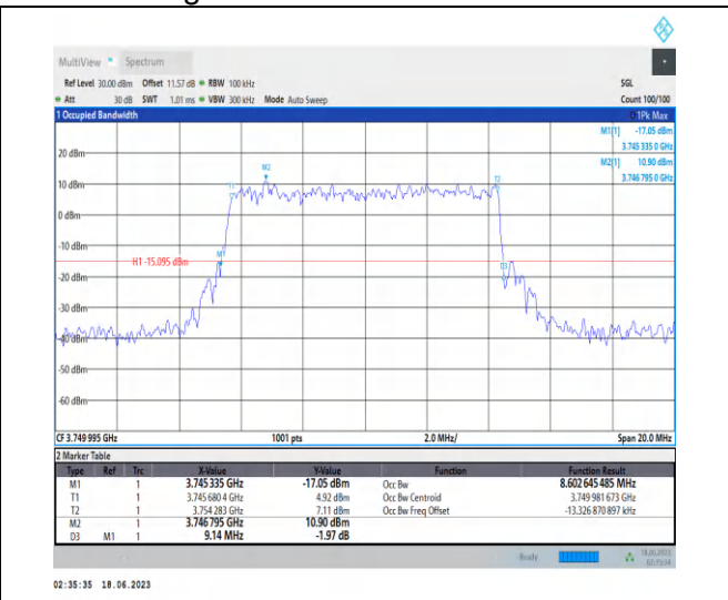
1-N78-3700-3800-PC2-30-10-M-5-DFT-256QAM-Outer_Full-24@0-Ant2-8.603-9.140-≤10-PASS
