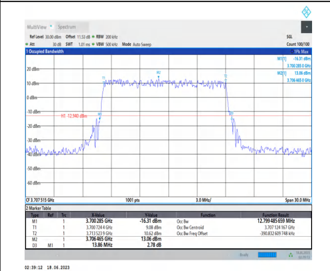
1-N78-3700-3800-PC2-30-15-L-5-DFT-256QAM-Outer_Full-36@0-Ant2-12.799-13.860-≤15-PASS
