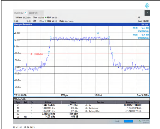
1-N78-3700-3800-PC2-30-15-M-3-DFT-16QAM-Outer_Full-36@0-Ant2-12.899-14.070-≤15-PASS
