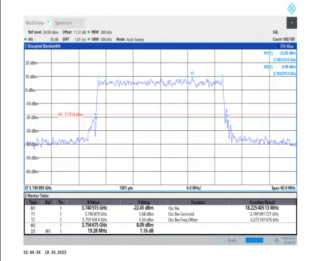
1-N78-3700-3800-PC2-30-20-M-9-CP-256QAM-Outer_Full-51@0-Ant2-18.225-19.280-≤20-PASS
