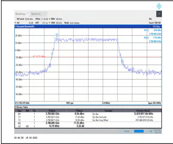
1-N78-3700-3800-PC2-30-15-H-2-DFT-QPSK-Outer_Full-36@0-Ant2-12.82-14.190-≤15-PASS
