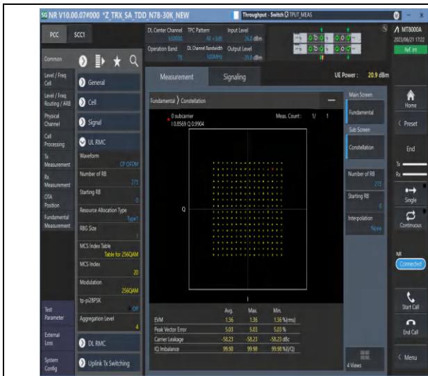
1-N78-3700-3800-PC2-30-100-M-9-CP-256QAM-Outer_Full-273@0-Ant2-see graph-PASS
