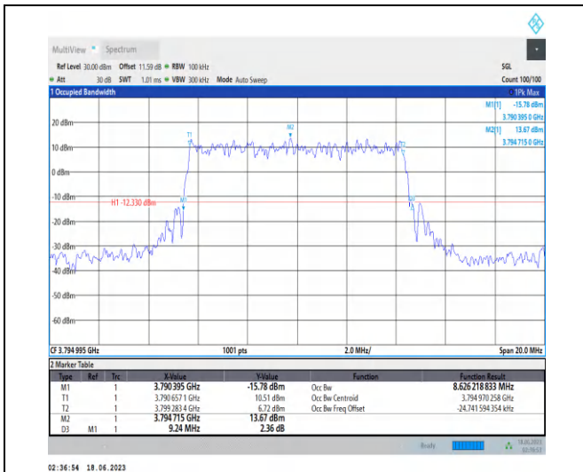
1-N78-3700-3800-PC2-30-10-H-3-DFT-16QAM-Outer_Full-24@0-Ant2-8.626-9.240-≤10-PASS
