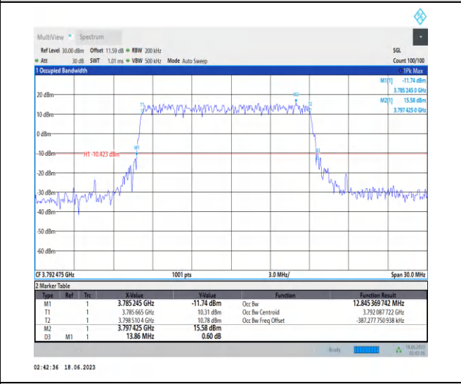
1-N78-3700-3800-PC2-30-15-H-3-DFT-16QAM-Outer_Full-36@0-Ant2-12.845-13.860-≤15-PASS
