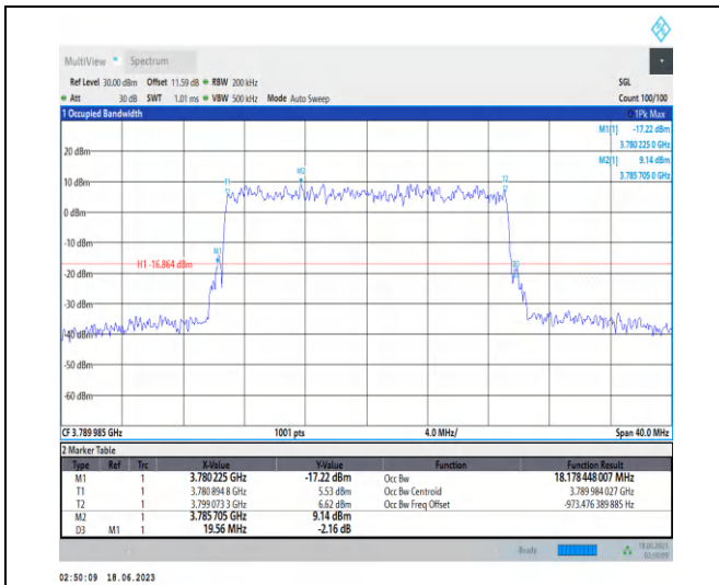
1-N78-3700-3800-PC2-30-20-H-9-CP-256QAM-Outer_Full-51@0-Ant2-18.178-19.560-<=20-PASS
