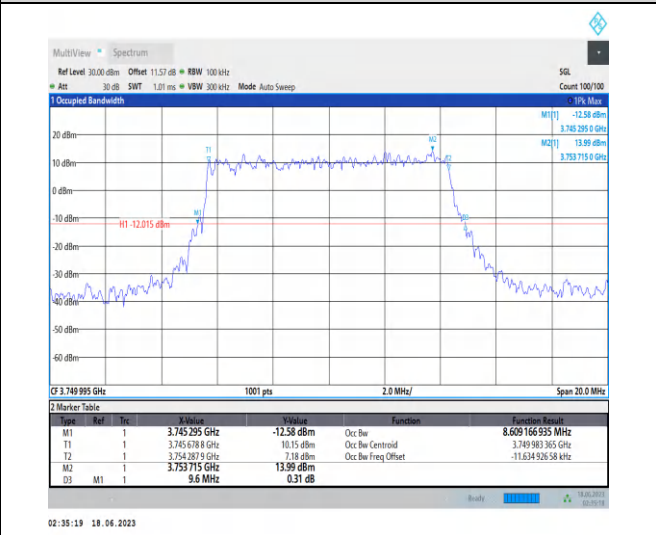
1-N78-3700-3800-PC2-30-10-M-3-DFT-16QAM-Outer_Full-24@0-Ant2-8.609-9.600-≤10-PASS
