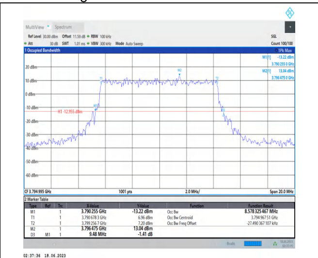
1-N78-3700-3800-PC2-30-10-H-8-CP-64QAM-Outer_Full-24@0-Ant2-8.578-9.480-≤10-PASS
