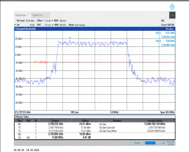
1-N78-3700-3800-PC2-30-15-L-1-DFT-PI2BPSK-Outer_Full-36@0-Ant2-12.841-13.860-≤15-PASS
