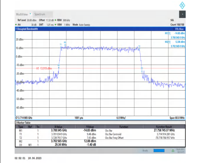
1-N78-3700-3800-PC2-30-30-L-7-CP-16QAM-Outer_Full-78@0-Ant2-27.759-29.340-≤30-PASS
