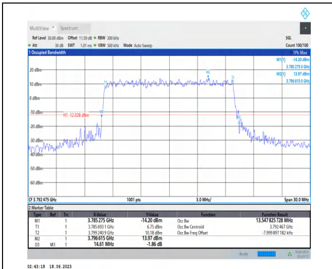
1-N78-3700-3800-PC2-30-15-H-8-CP-64QAM-Outer_Full-38@0-Ant2-13.548-14.610-≤15-PASS
