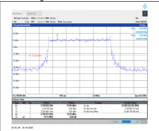
1-N78-3700-3800-PC2-30-15-M-6-CP-QPSK-Outer Full-38@0-Ant2-13.596-14.730-≤15-PASS
