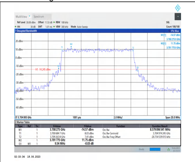
1-N78-3700-3800-PC2-30-10-L-6-CP-QPSK-Outer Full-24@0-Ant2-8.579-9.540-≤10-PASS
