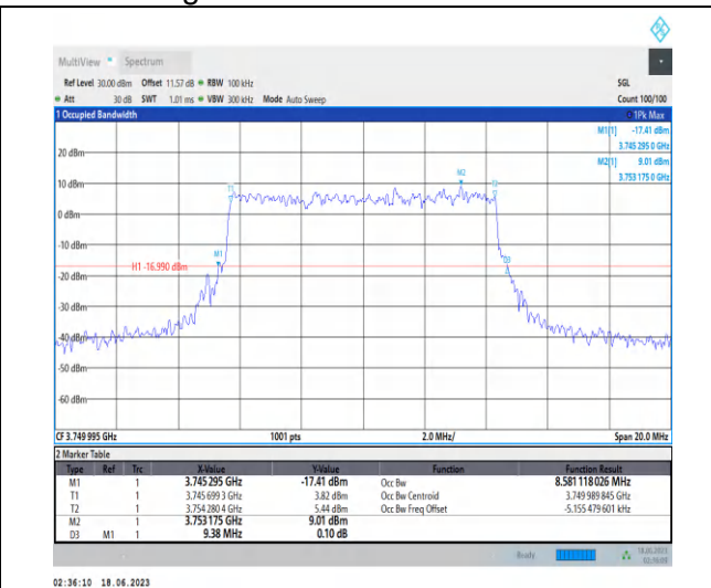
1-N78-3700-3800-PC2-30-10-M-9-CP-256QAM-Outer_Full-24@0-Ant2-8.581-9.380-≤10-PASS
