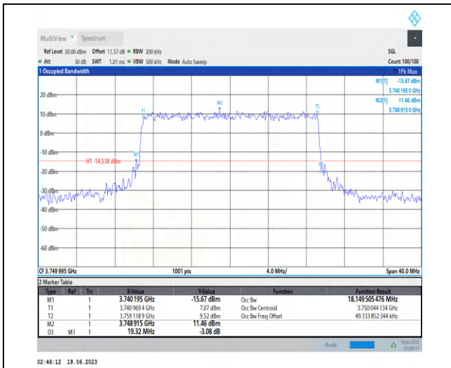
1-N78-3700-3800-PC2-30-20-M-6-CP-QPSK-Outer_Full-51@0-Ant2-18.15-19.320-≤20-PASS
