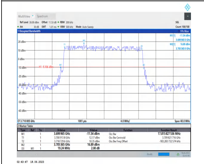
1-N78-3700-3800-PC2-30-20-L-1-DFT-PI2BPSK-Outer_Full-50@0-Ant2-17.816-19.240-≤20-PASS
