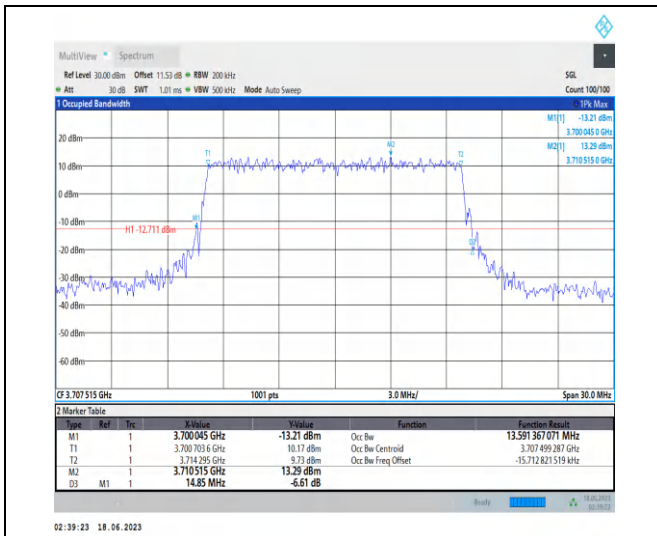
1-N78-3700-3800-PC2-30-15-L-6-CP-QPSK-Outer_Full-38@0-Ant2-13.591-14.850-≤15-PASS
