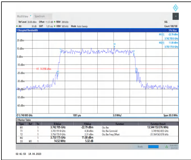
1-N78-3700-3800-PC2-30-15-M-9-CP-256QAM-Out_Full-38@0-Ant2-13.544-14.520-≤15-PASS
