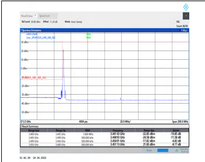
1-N78-3450-3550-PC2-30-70-L-1-DFT-PI2BPSK-Edge_1RB_Left-1@0-Ant2-1--PASS-see graph
