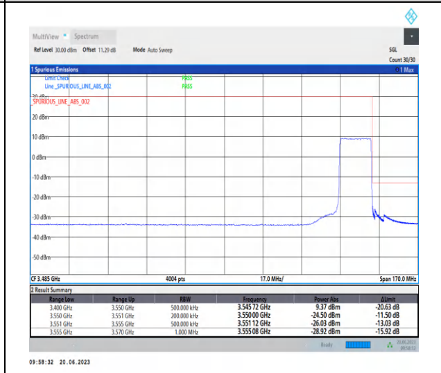
1-N78-3450-3550-PC2-30-15-H-3-CP-QPSK-Outer _Full-38@0-Ant2-1--PASS-see graph
