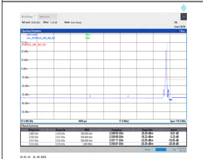
1-N78-3450-3550-PC2-30-80-H-5-CP-QPSK-Edge_1RB_Right-1@216-Ant2-1--PASS-see graph
