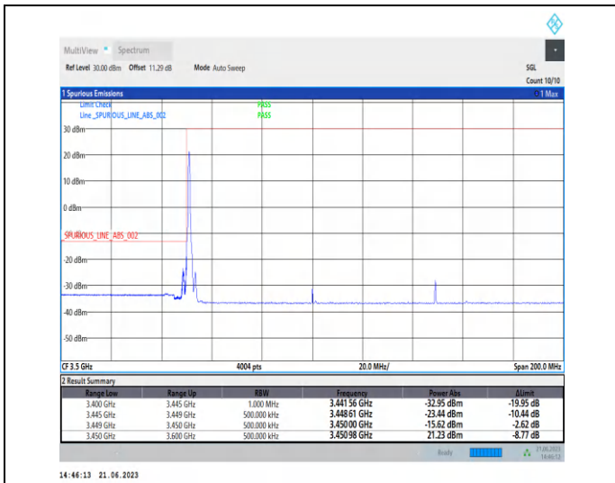
1-N78-3450-3550-PC2-30-100-L-1-CP-QPSK-Edge_1 RB_Left-1@0-Ant2-1--PASS-see graph
