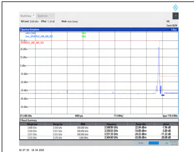
1-N78-3450-3550-PC2-30-100-H-2-DFT-PI2BPSK-Edge_1RB_Right-1@272-Ant2-1--PASS-see graph
