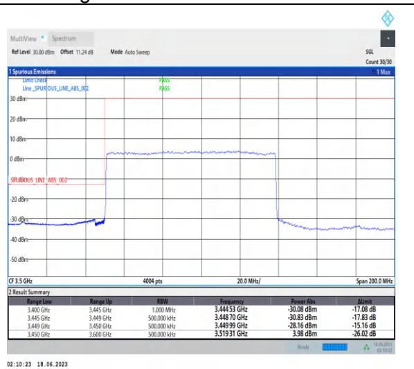
1-N78-3450-3550-PC2-30-90-L-3-DFT-PI2BPSK-Outer_Full-243@0-Ant2-1--PASS-see graph
