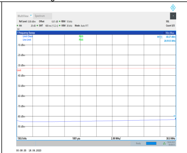
1-N78-3450-3550-PC2-30-100-H-1-N/A-DFT-PI2BPS K-Inner_1RB_Left-1@1-0.15-30-Ant2-29.91--83.27--33-PASS
