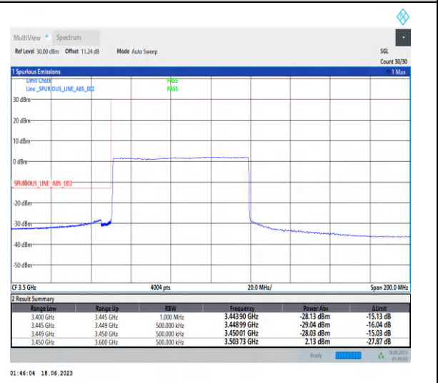
1-N78-3450-3550-PC2-30-70-L-6-CP-QPSK-Outer_Full-189@0-Ant2-1--PASS-see graph
