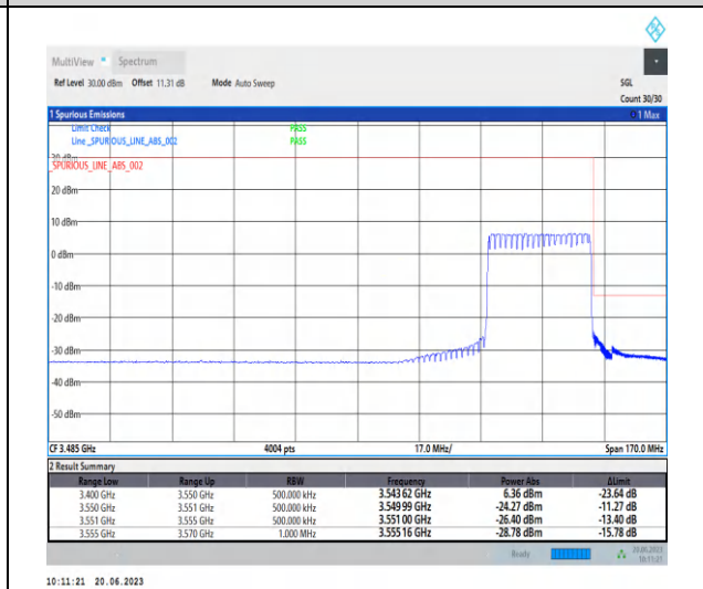
1-N78-3450-3550-PC2-30-30-H-3-CP-QPSK-Outer_Full-78@0-Ant2-1--PASS-see graph
