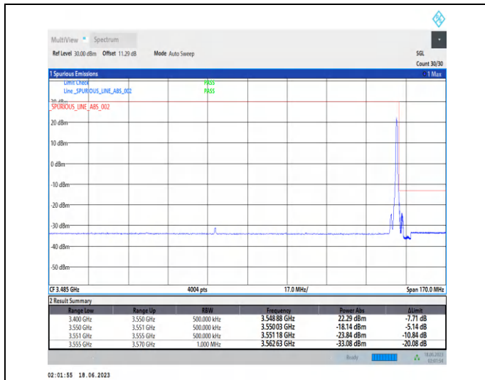
1-N78-3450-3550-PC2-30-80-H-2-DFT-PI2BPSK-Edge_1RB_Right-1@216-Ant2-1--PASS-see graph
