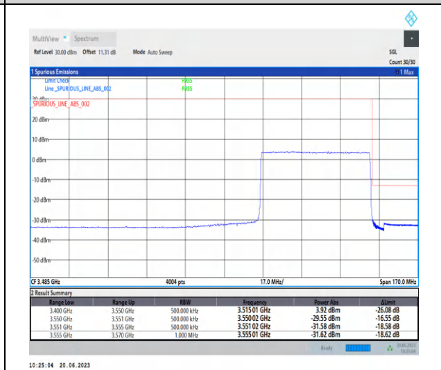
1-N78-3450-3550-PC2-30-50-H-3-CP-QPSK-Outer _Full-133@0-Ant2-1--PASS-see graph
