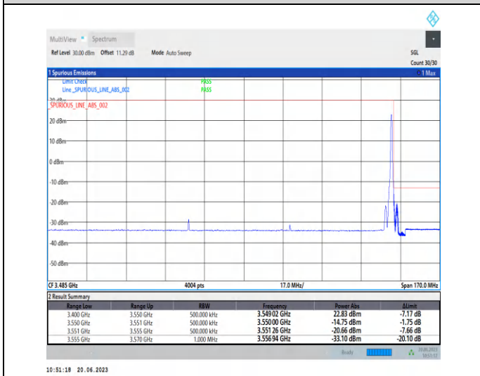
1-N78-3450-3550-PC2-30-90-H-2-CP-QPSK-Edge_1R B_Right-1@244-Ant2-1--PASS-see graph
