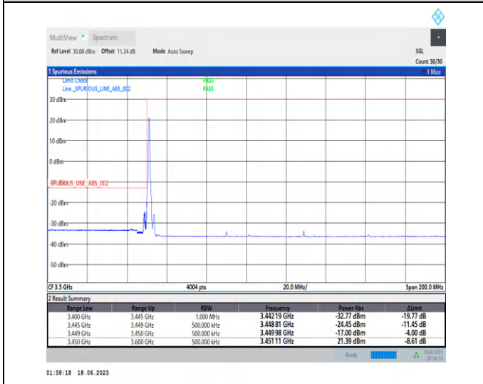
1-N78-3450-3550-PC2-30-80-L-4-CP-QPSK-Edge_1RB_Left-1@0-Ant2-1--PASS-see graph
