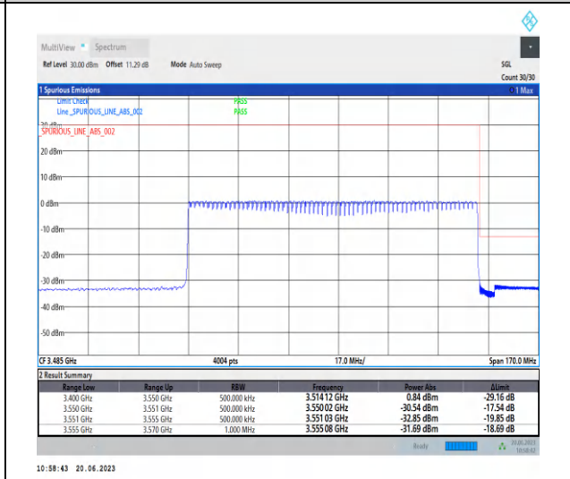
1-N78-3450-3550-PC2-30-100-H-3-CP-QPSK-Out er_Full-273@0-Ant2-1--PASS-see graph
