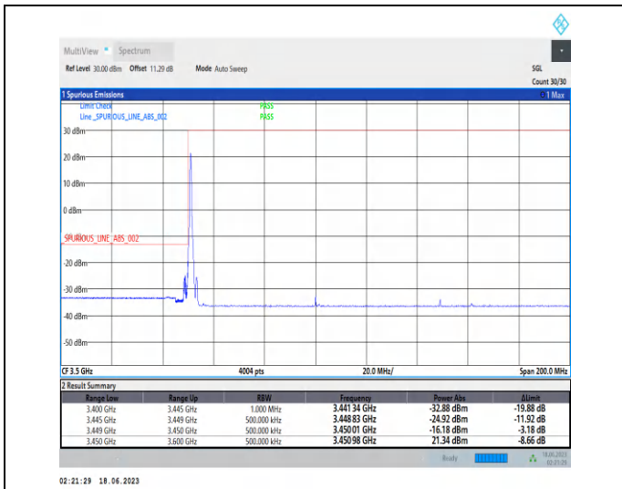
1-N78-3450-3550-PC2-30-100-L-1-DFT-PI2BPSK-Edge_1RB_Left-1@0-Ant2-1--PASS-see graph
