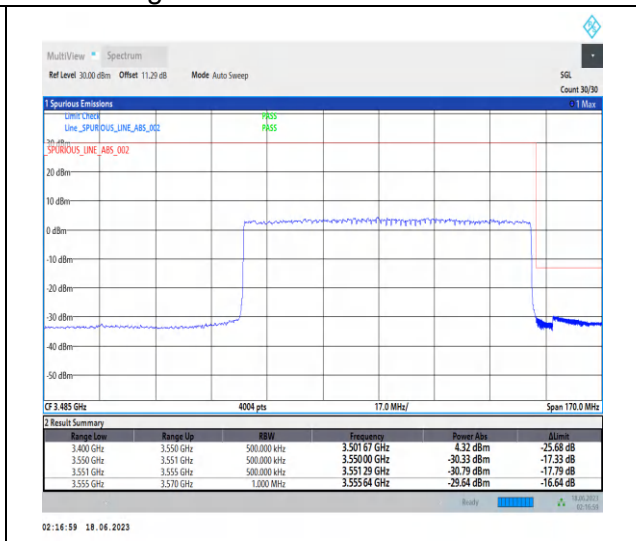
1-N78-3450-3550-PC2-30-90-H-3-DFT-PI2BPSK-Outer_Full-243@0-Ant2-1--PASS-see graph
