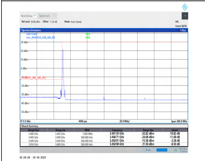
1-N78-3450-3550-PC2-30-100-L-4-CP-QPSK-Edge_1RB_Left-1@0-Ant2-1--PASS-see graph
