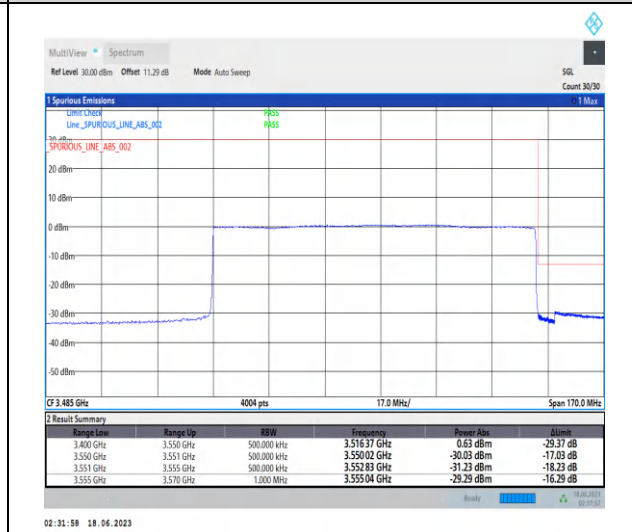
1-N78-3450-3550-PC2-30-100-H-6-CP-QPSK-Outer_Full-273@0-Ant2-1--PASS-see graph
