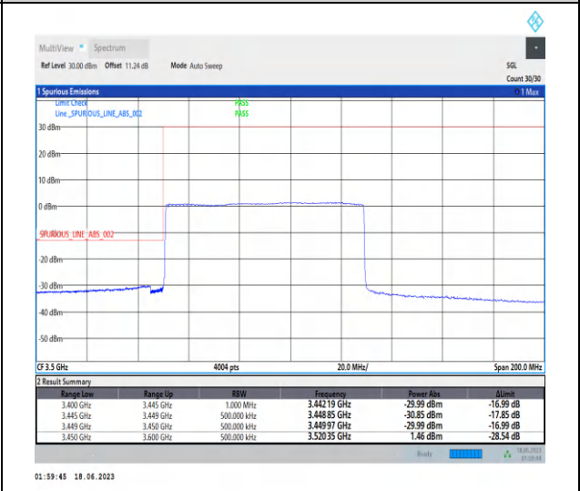
1-N78-3450-3550-PC2-30-80-L-6-CP-QPSK-Outer_Full-217@0-Ant2-1--PASS-see graph
