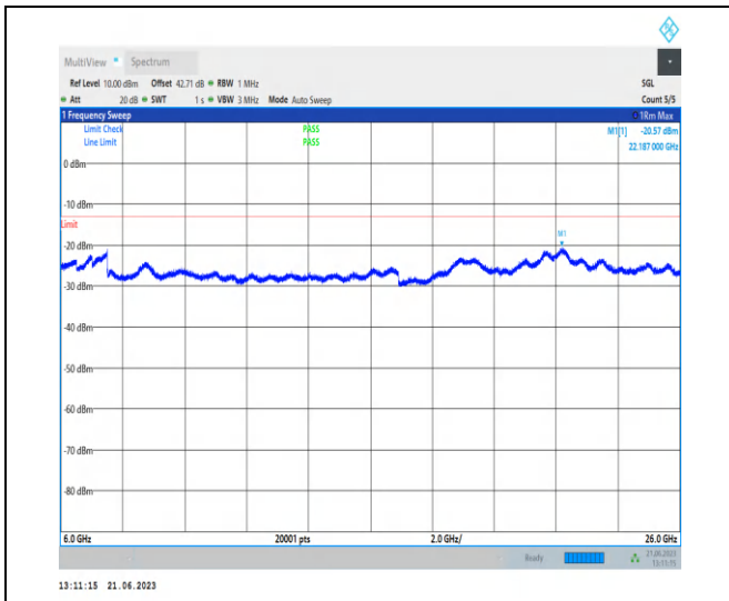
1-N78-3450-3550-PC2-30-100-M-1-N/A-DFT-QPSK-Edge_1RB_Left-1@0-6000-26000-Ant2-22187.00--2.057--13-PASS
