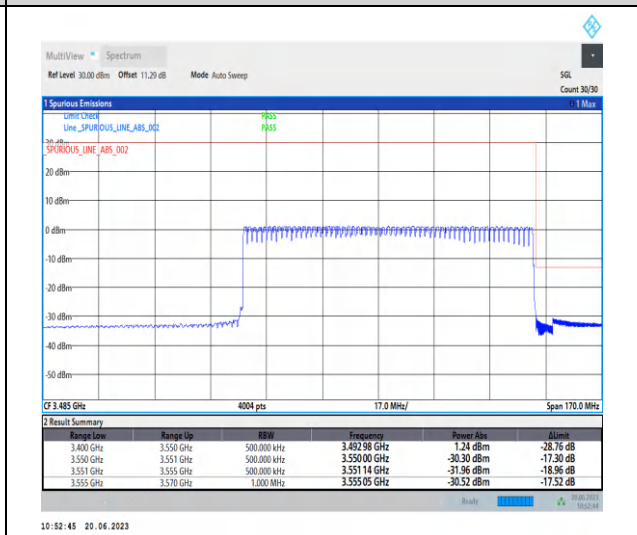
1-N78-3450-3550-PC2-30-90-H-3-CP-QPSK-Outer _Full-245@0-Ant2-1--PASS-see graph
