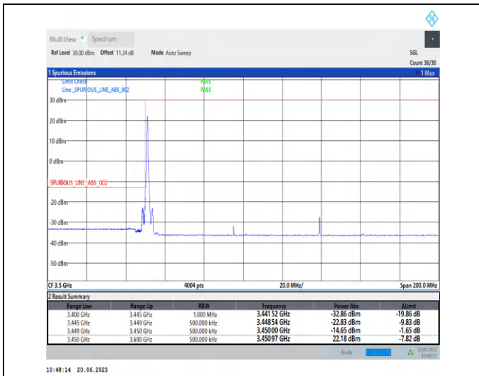
1-N78-3450-3550-PC2-30-90-L-1-CP-QPSK-Edge_1R B_Left-1@0-Ant2-1--PASS-see graph
