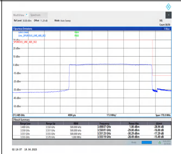
1-N78-3450-3550-PC2-30-90-H-6-CP-QPSK-Outer_Full-245@0-Ant2-1--PASS-see graph
