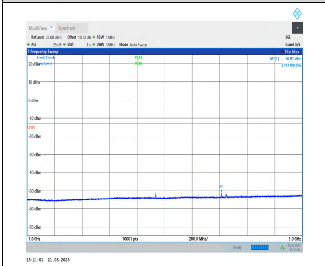
1-N78-3450-3550-PC2-30-100-M-1-N/A-DFT-QPSK-Edge_1RB_Left-1@0-1000-3000-Ant2-2414.40--50.97--13-PASS
