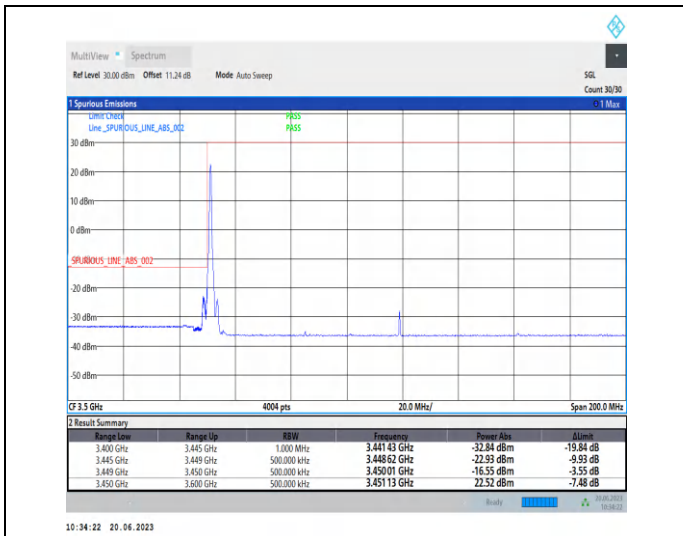
1-N78-3450-3550-PC2-30-70-L-1-CP-QPSK-Edge_1R B_Left-1@0-Ant2-1--PASS-see graph
