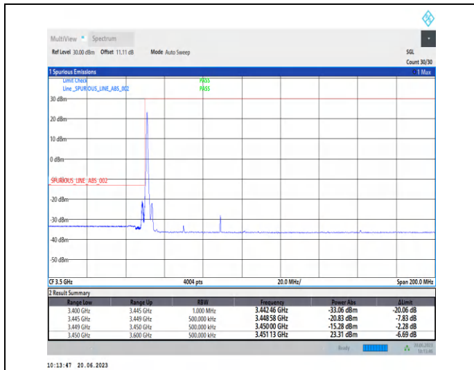
1-N78-3450-3550-PC2-30-40-L-1-CP-QPSK-Edge_1R B_Left-1@0-Ant2-1--PASS-see graph
