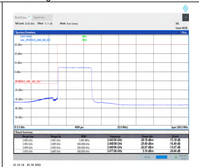
1-N78-3450-3550-PC2-30-40-L-3-CP-QPSK-Outer _Full-106@0-Ant2-1--PASS-see graph
