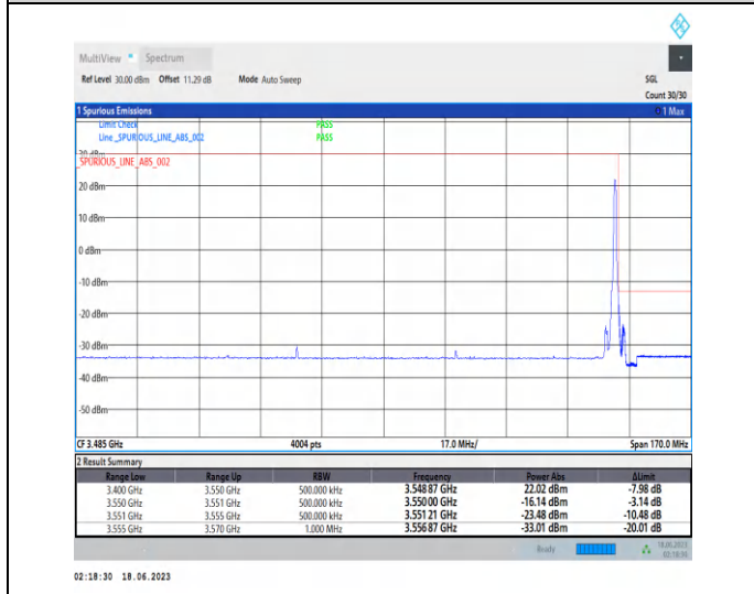
1-N78-3450-3550-PC2-30-90-H-5-CP-QPSK-Edge_1RB_Right-1@244-Ant2-1--PASS-see graph
