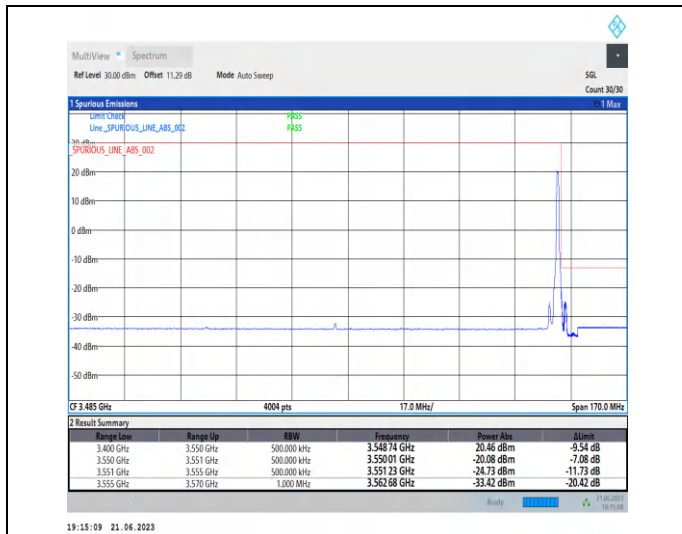
1-N78-3450-3550-PC2-30-70-H-2-DFT-PI2BPSK-Edge_1RB_Right-1@188-Ant2-1--PASS-see graph
