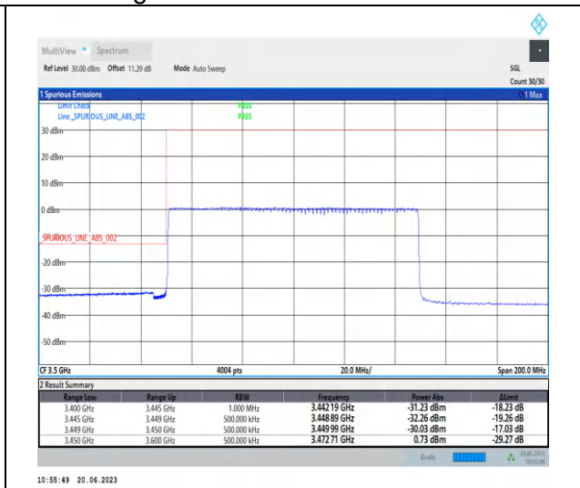
1-N78-3450-3550-PC2-30-100-L-3-CP-QPSK-Out er_Full-273@0-Ant2-1--PASS-see graph
