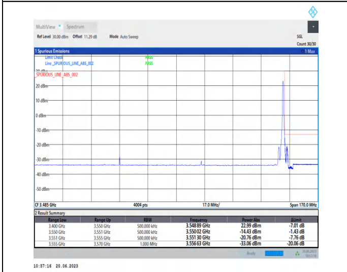
1-N78-3450-3550-PC2-30-100-H-2-CP-QPSK-Edge_1 RB_Right-1@272-Ant2-1--PASS-see graph
