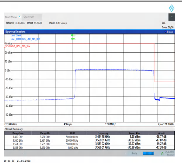
1-N78-3450-3550-PC2-30-80-H-6-CP-QPSK-Outer_Full-217@0-Ant2-1--PASS-see graph
