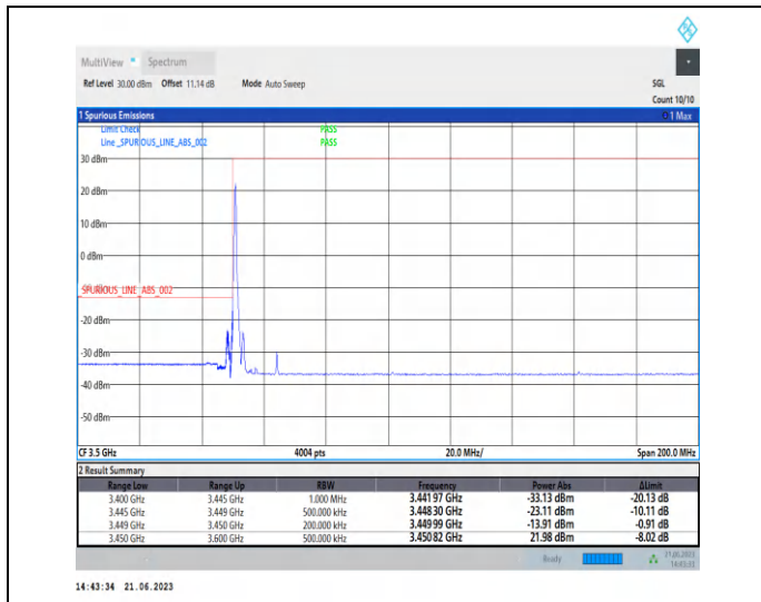
1-N78-3450-3550-PC2-30-15-L-1-CP-QPSK-Edge_1R B_Left-1@0-Ant2-1--PASS-see graph
