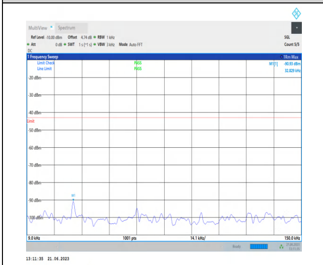
1-N78-3450-3550-PC2-30-100-H-1-N/A-DFT-QPSK-Edge_1RB_Left-1@0-0.009-0.15-Ant2-0.03--90.93--43-PASS
