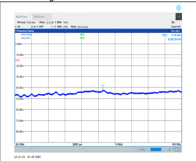
1-N78-3450-3550-PC2-30-100-M-1-N/A-DFT-QPSK-Edge_1RB_Left-1@0-26000-40000-Ant2-33382.20--41.65--13-PASS
