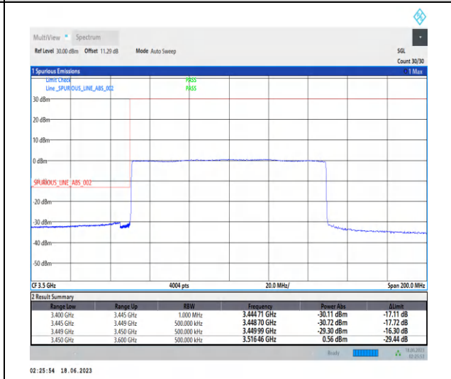
1-N78-3450-3550-PC2-30-100-L-6-CP-QPSK-Outer_Full-273@0-Ant2-1--PASS-see graph
