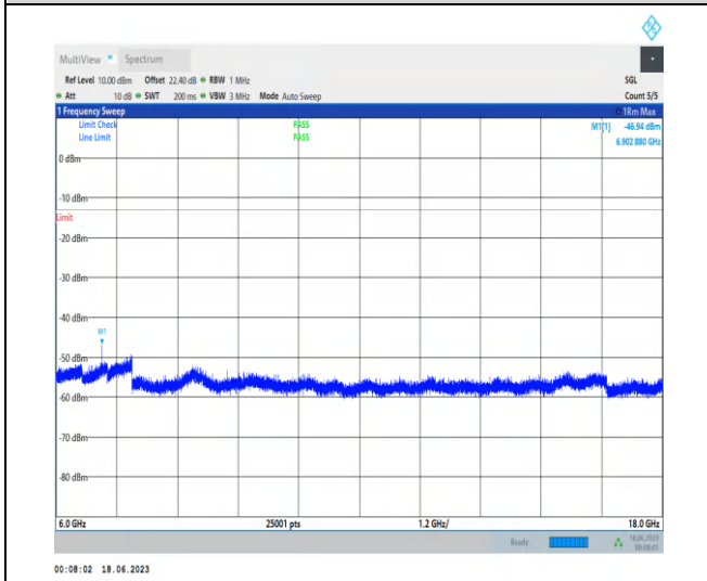
1-N78-3450-3550-PC2-30-100-M-1-N/A-DFT-PI2BP SK-Inner_1RB_Left-1@1-6000-18000-Ant2-6902.88 --46.94--13-PASS
