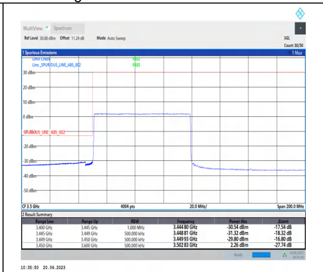
1-N78-3450-3550-PC2-30-70-L-3-CP-QPSK-Outer _Full-189@0-Ant2-1--PASS-see graph
