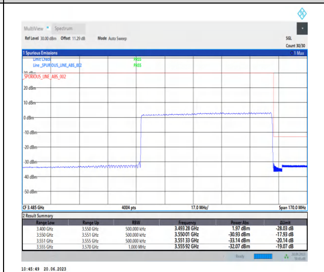
1-N78-3450-3550-PC2-30-80-H-3-CP-QPSK-Outer _Full-217@0-Ant2-1--PASS-see graph
