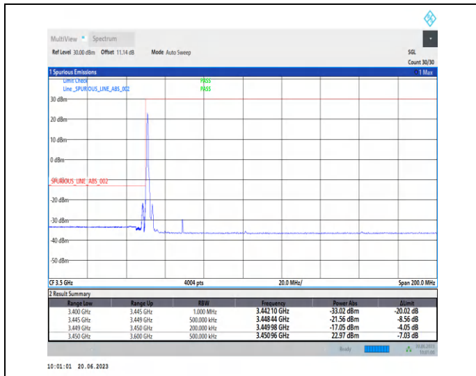
1-N78-3450-3550-PC2-30-20-L-1-CP-QPSK-Edge_1R B_Left-1@0-Ant2-1--PASS-see graph
