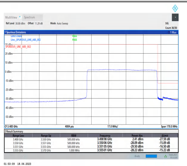
1-N78-3450-3550-PC2-30-70-H-6-CP-QPSK-Outer_Full-189@0-Ant2-1--PASS-see graph
