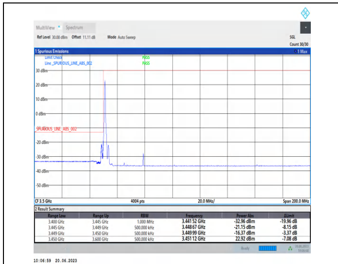
1-N78-3450-3550-PC2-30-30-L-1-CP-QPSK-Edge_1R_B_Left-1@0-Ant2-1--PASS-see graph
