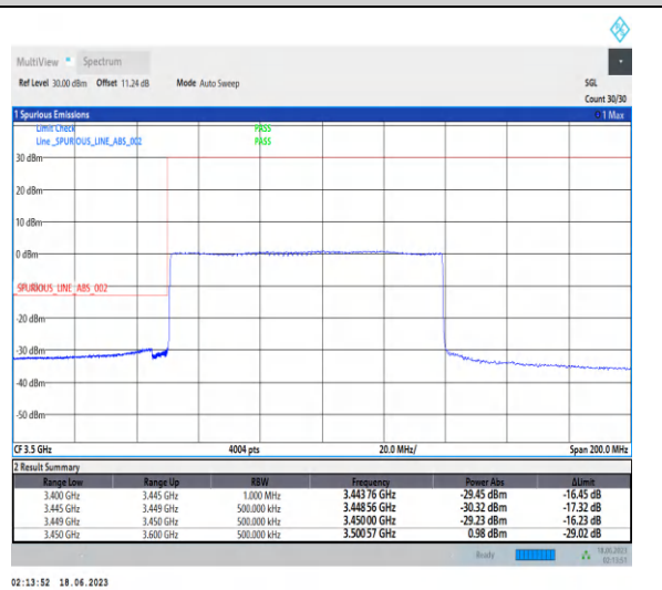
1-N78-3450-3550-PC2-30-90-L-6-CP-QPSK-Outer_Full-245@0-Ant2-1--PASS-see graph
