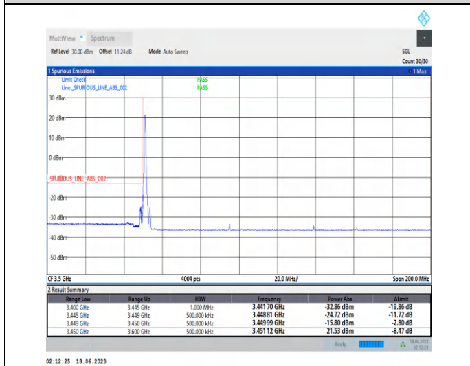
1-N78-3450-3550-PC2-30-90-L-4-CP-QPSK-Edge_1RB_Left-1@0-Ant2-1--PASS-see graph
