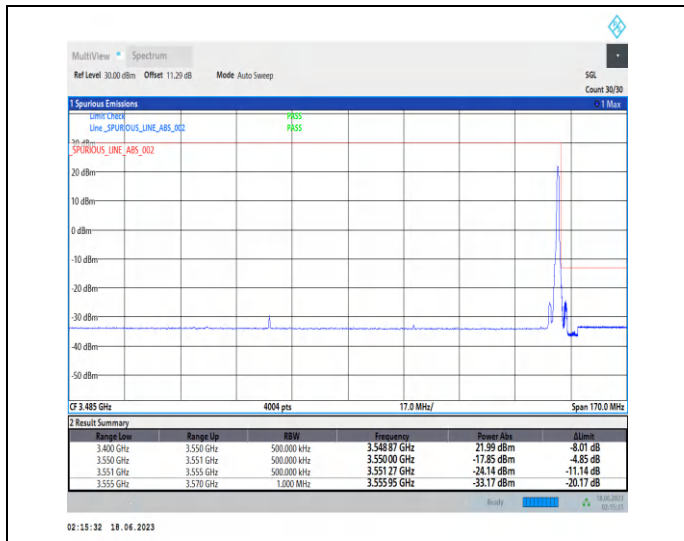
1-N78-3450-3550-PC2-30-90-H-2-DFT-PI2BPSK-Edge_1RB_Right-1@244-Ant2-1--PASS-see graph
