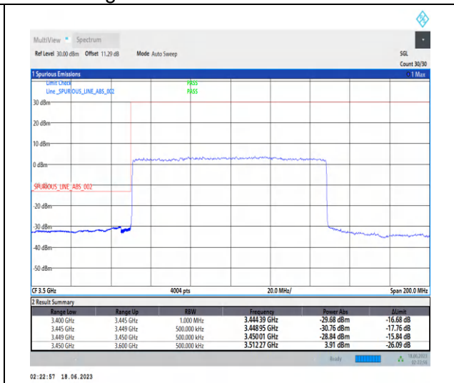
1-N78-3450-3550-PC2-30-100-L-3-DFT-PI2BPSK-Outer_Full-270@0-Ant2-1--PASS-see graph
