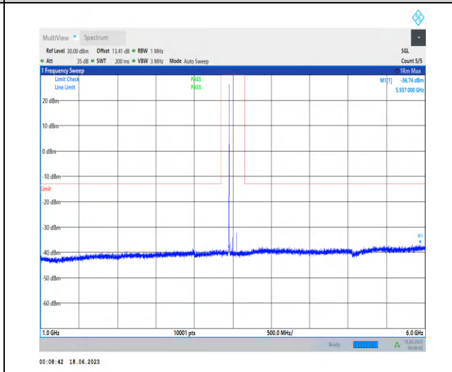
1-N78-3450-3550-PC2-30-100-H-1-N/A-DFT-PI2BPS K-Inner_1RB_Left-1@1-1000-6000-Ant2-5937.00--36.74--13-PASS
