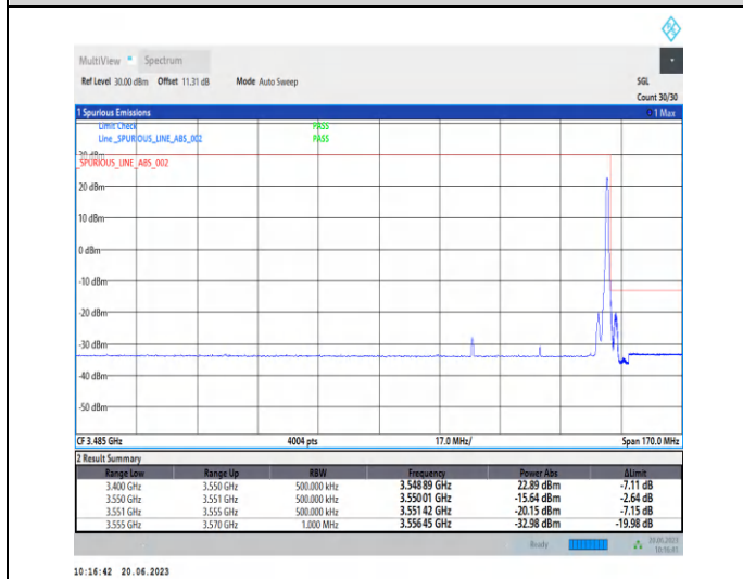
1-N78-3450-3550-PC2-30-40-H-2-CP-QPSK-Edge_1R B_Right-1@105-Ant2-1--PASS-see graph
