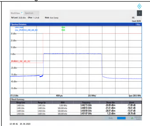
1-N78-3450-3550-PC2-30-90-L-3-CP-QPSK-Outer _Full-245@0-Ant2-1--PASS-see graph
