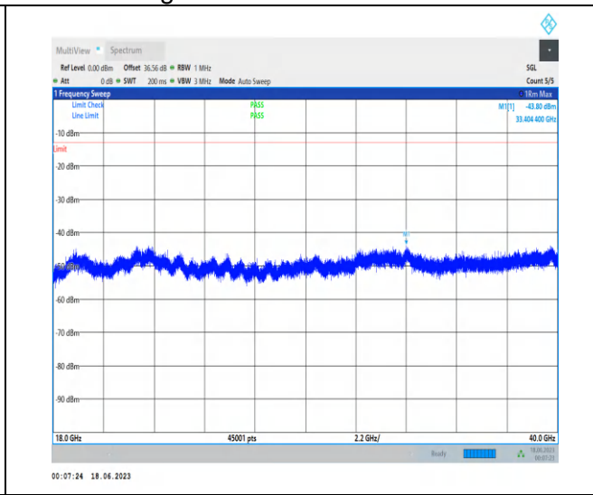
1-N78-3450-3550-PC2-30-100-L-1-N/A-DFT-PI2BPS K-Inner_1RB_Left-1@1-18000-40000-Ant2-33404.40 --43.80--13-PASS
