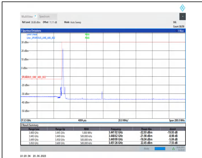
1-N78-3450-3550-PC2-30-50-L-1-CP-QPSK-Edge_1R B_Left-1@0-Ant2-1--PASS-see graph
