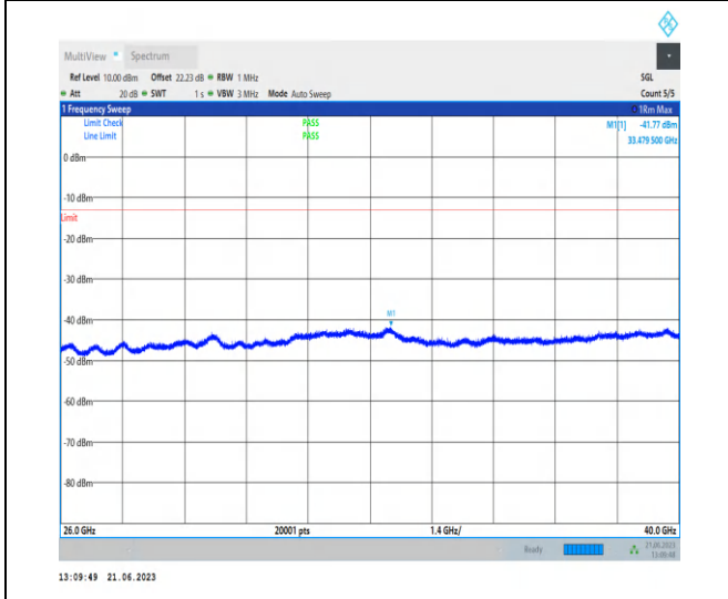
1-N78-3450-3550-PC2-30-100-L-1-N/A-DFT-QPSK-Edge_1RB_Left-1@0-26000-40000-Ant2-33479.50--41.77--13-PASS
