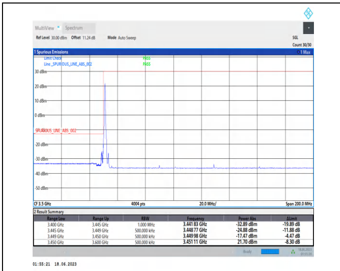
1-N78-3450-3550-PC2-30-80-L-1-DFT-PI2BPSK-Edge_1RB_Left-1@0-Ant2-1--PASS-see graph
