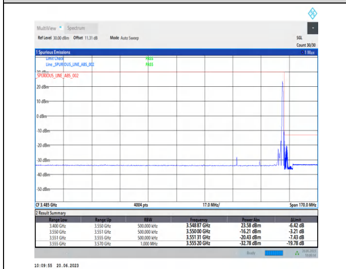
1-N78-3450-3550-PC2-30-30-H-2-CP-QPSK-Edge_1R_B_Right-1@77-Ant2-1--PASS-see graph
