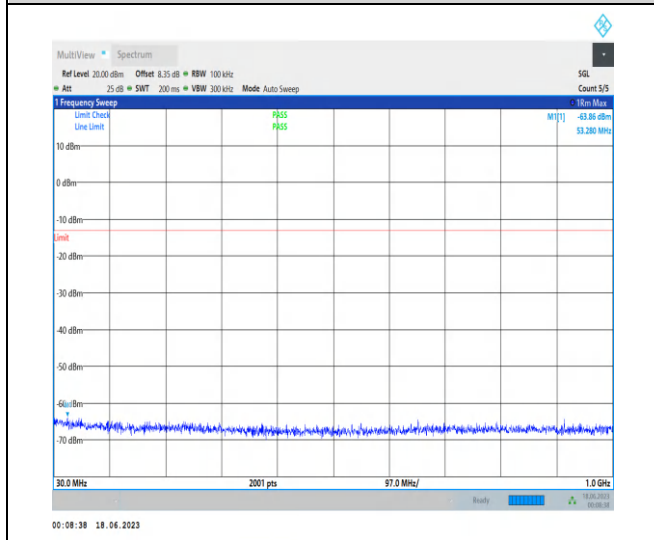
1-N78-3450-3550-PC2-30-100-H-1-N/A-DFT-PI2BP SK-Inner_1RB_Left-1@1-30-1000-Ant2-53.28--63.86--13-PASS
