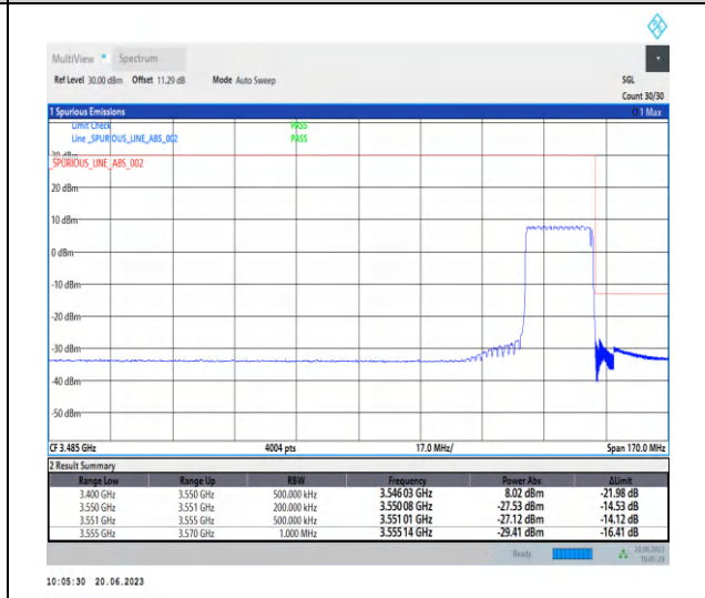
1-N78-3450-3550-PC2-30-20-H-3-CP-QPSK-Outer _Full-51@0-Ant2-1--PASS-see graph
