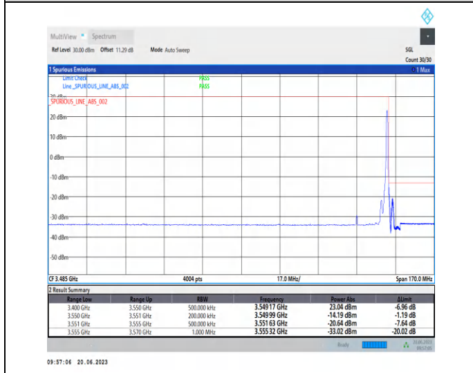
1-N78-3450-3550-PC2-30-15-H-2-CP-QPSK-Edge_1R B_Right-1@37-Ant2-1--PASS-see graph
