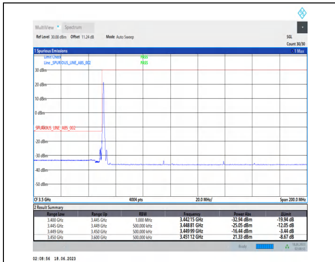
1-N78-3450-3550-PC2-30-90-L-1-DFT-PI2BPSK-Edge_1RB_Left-1@0-Ant2-1--PASS-see graph
