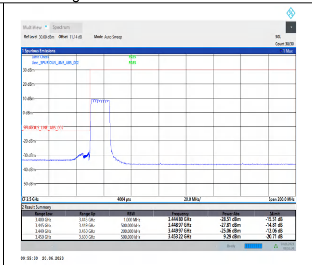
1-N78-3450-3550-PC2-30-15-L-3-CP-QPSK-Outer _Full-38@0-Ant2-1--PASS-see graph
