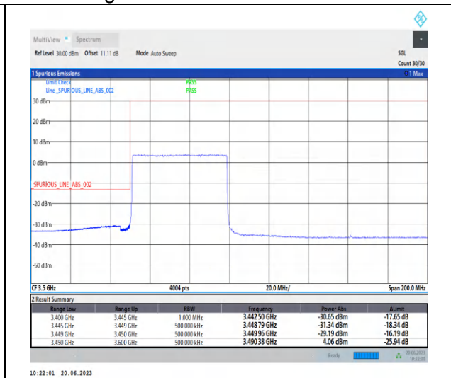
1-N78-3450-3550-PC2-30-50-L-3-CP-QPSK-Outer _Full-133@0-Ant2-1--PASS-see graph
