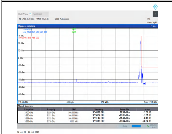
1-N78-3450-3550-PC2-30-80-H-2-CP-QPSK-Edge_1R B_Right-1@216-Ant2-1--PASS-see graph
