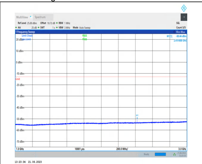
1-N78-3450-3550-PC2-30-100-H-1-N/A-DFT-QPSK-Edge_1RB_Left-1@0-1000-3000-Ant2-2462.80--50.44--44--13-PASS
