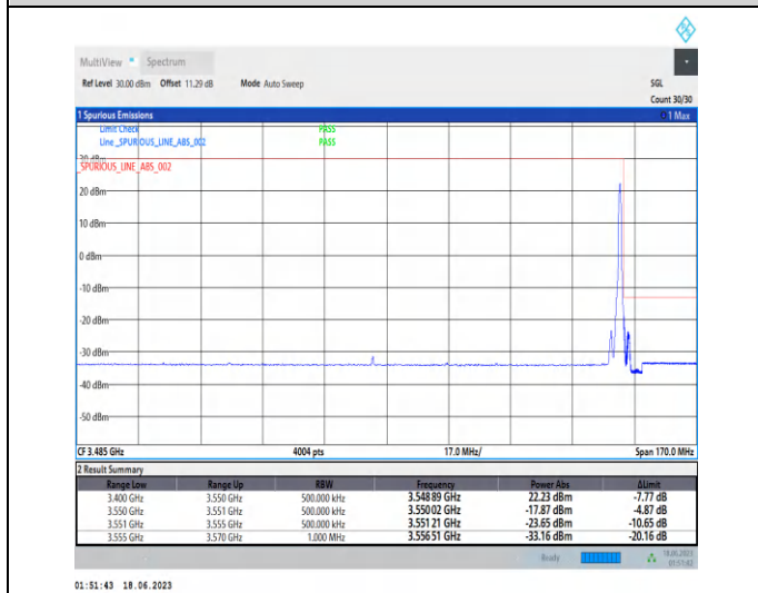
1-N78-3450-3550-PC2-30-70-H-5-CP-QPSK-Edge_1RB_Right-1@188-Ant2-1--PASS-see graph
