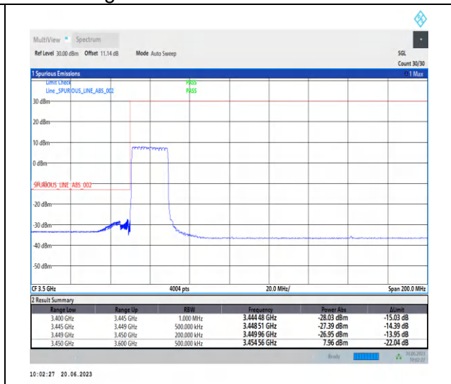
1-N78-3450-3550-PC2-30-20-L-3-CP-QPSK-Outer _Full-51@0-Ant2-1--PASS-see graph
