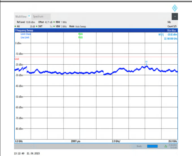
1-N78-3450-3550-PC2-30-100-H-1-N/A-DFT-QPSK-Edge_1RB_Left-1@0-6000-26000-Ant2-22180.00--20.82--13-PASS
