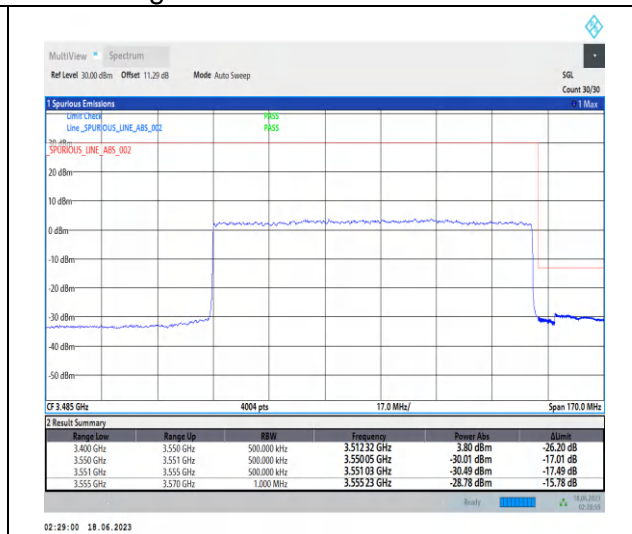
1-N78-3450-3550-PC2-30-100-H-3-DFT-PI2BPSK-Outer_Full-270@0-Ant2-1--PASS-see graph
