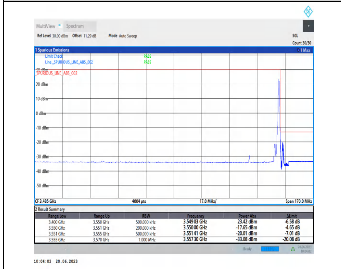
1-N78-3450-3550-PC2-30-20-H-2-CP-QPSK-Edge_1R B_Right-1@50-Ant2-1--PASS-see graph
