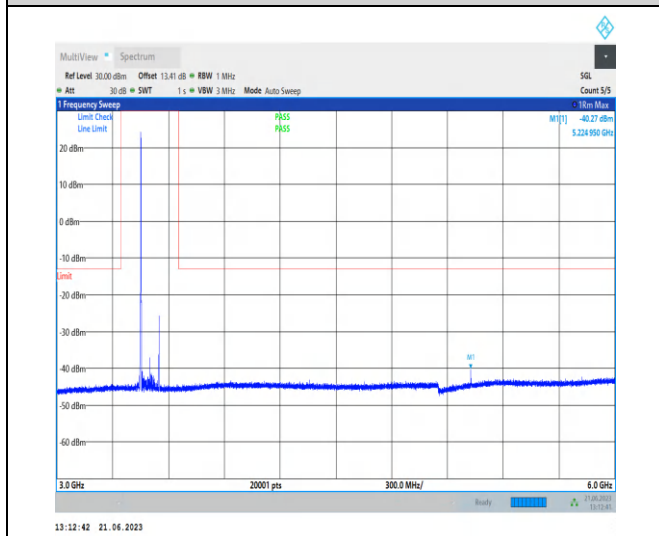
1-N78-3450-3550-PC2-30-100-H-1-N/A-DFT-QPSK-Edge_1RB_Left-1@0-3000-6000-Ant2-5224.95--40.27--13-PASS
