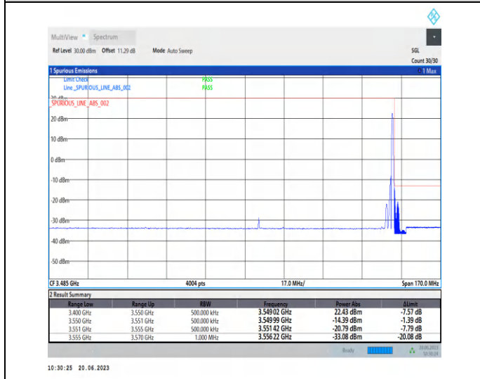
1-N78-3450-3550-PC2-30-60-H-2-CP-QPSK-Edge_1R B_Right-1@161-Ant2-1--PASS-see graph
