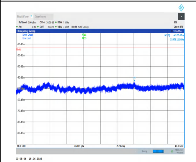
1-N78-3450-3550-PC2-30-100-M-1-N/A-DFT-PI2BPS K-Inner_1RB_Left-1@1-18000-40000-Ant2-33478.22 --43.55--13-PASS
