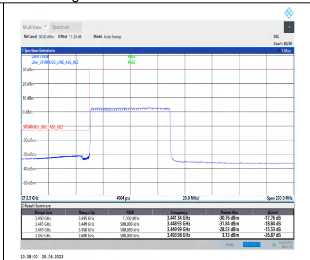
1-N78-3450-3550-PC2-30-60-L-3-CP-QPSK-Outer _Full-162@0-Ant2-1--PASS-see graph
