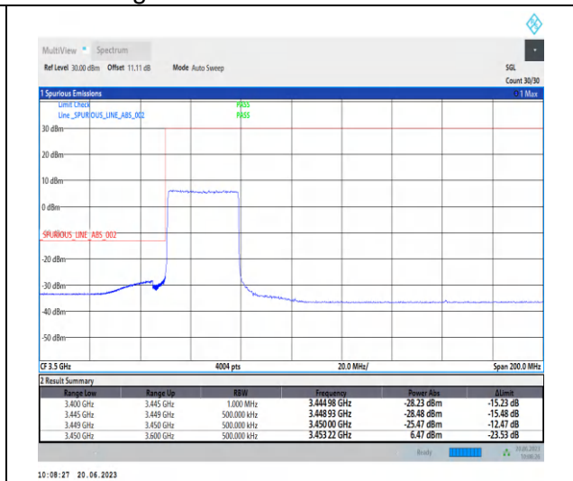
1-N78-3450-3550-PC2-30-30-L-3-CP-QPSK-Outer_Full-78@0-Ant2-1--PASS-see graph
