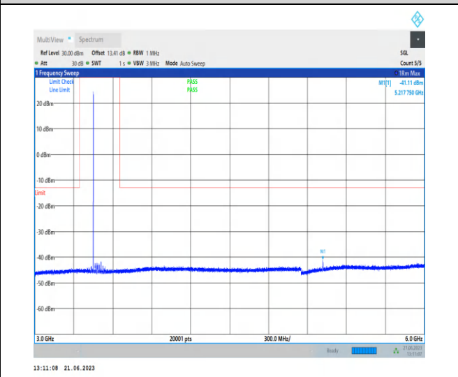
1-N78-3450-3550-PC2-30-100-M-1-N/A-DFT-QPSK-Edge_1RB_Left-1@0-3000-6000-Ant2-5217.75--41.11--13-PASS
