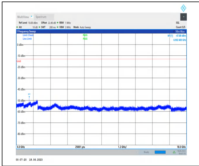
1-N78-3450-3550-PC2-30-100-L-1-N/A-DFT-PI2BP SK-Inner_1RB_Left-1@1-6000-18000-Ant2-6902.40 --47.89--13-PASS
