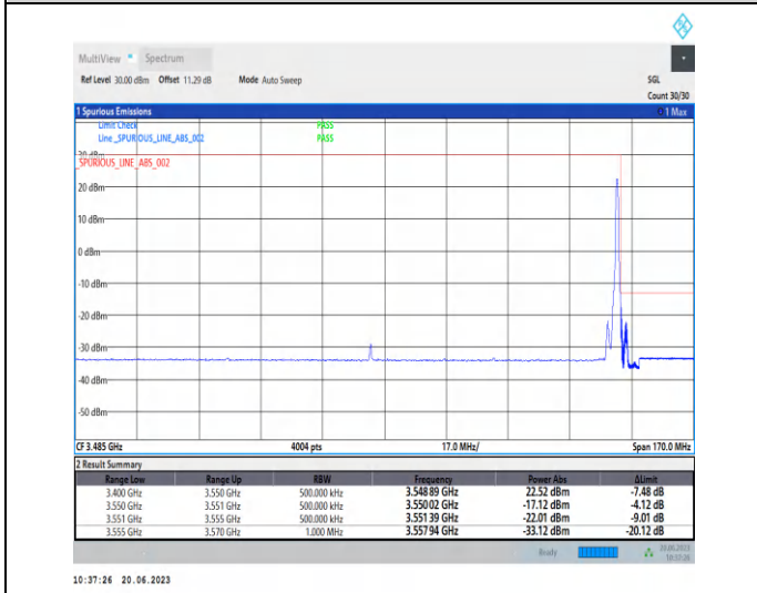
1-N78-3450-3550-PC2-30-70-H-2-CP-QPSK-Edge_1R B_Right-1@188-Ant2-1--PASS-see graph
