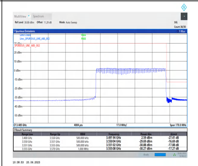
1-N78-3450-3550-PC2-30-70-H-3-CP-QPSK-Outer _Full-189@0-Ant2-1--PASS-see graph
