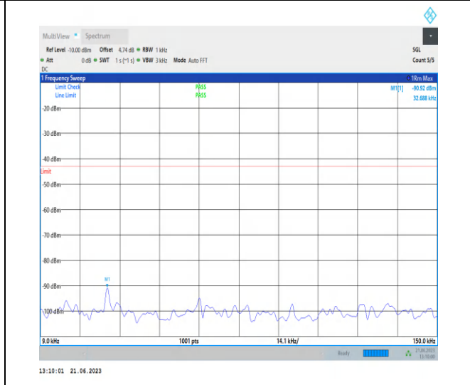
1-N78-3450-3550-PC2-30-100-M-1-N/A-DFT-QPSK-Edge_1RB_Left-1@0-0.009-0.15-Ant2-0.03--90.92--43-PASS
