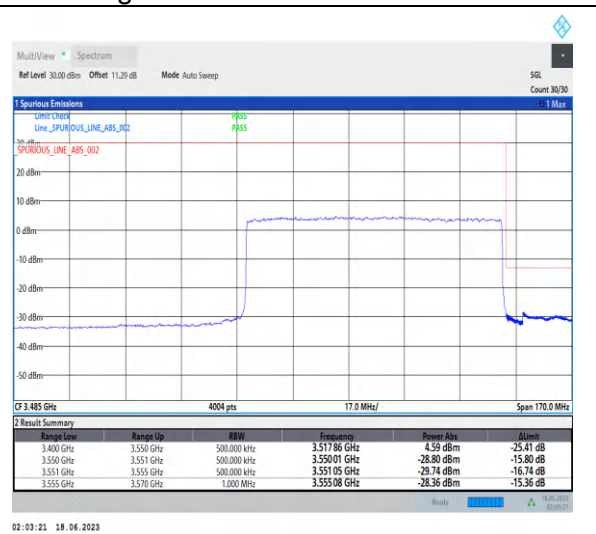
1-N78-3450-3550-PC2-30-80-H-3-DFT-PI2BPSK-Outer_Full-216@0-Ant2-1--PASS-see graph
