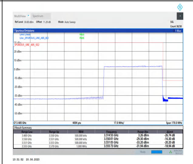
1-N78-3450-3550-PC2-30-60-H-3-CP-QPSK-Outer _Full-162@0-Ant2-1--PASS-see graph
