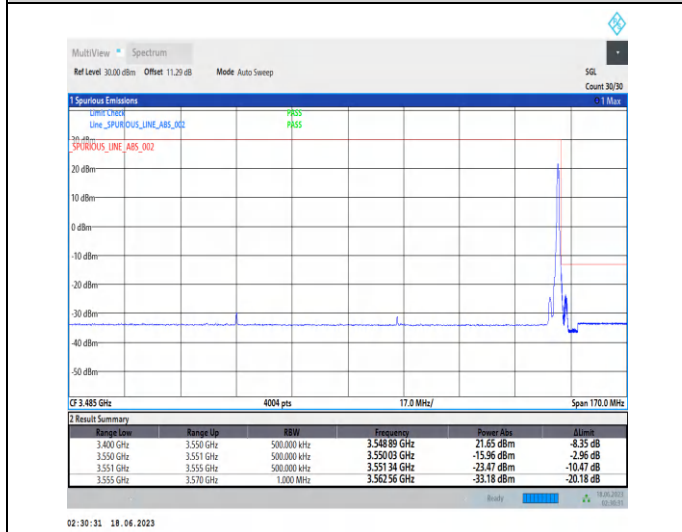
1-N78-3450-3550-PC2-30-100-H-5-CP-QPSK-Edge_1RB_Right-1@272-Ant2-1--PASS-see graph
