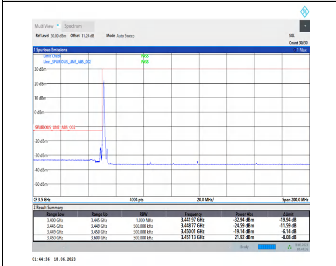
1-N78-3450-3550-PC2-30-70-L-4-CP-QPSK-Edge_1RB_Left-1@0-Ant2-1--PASS-see graph
