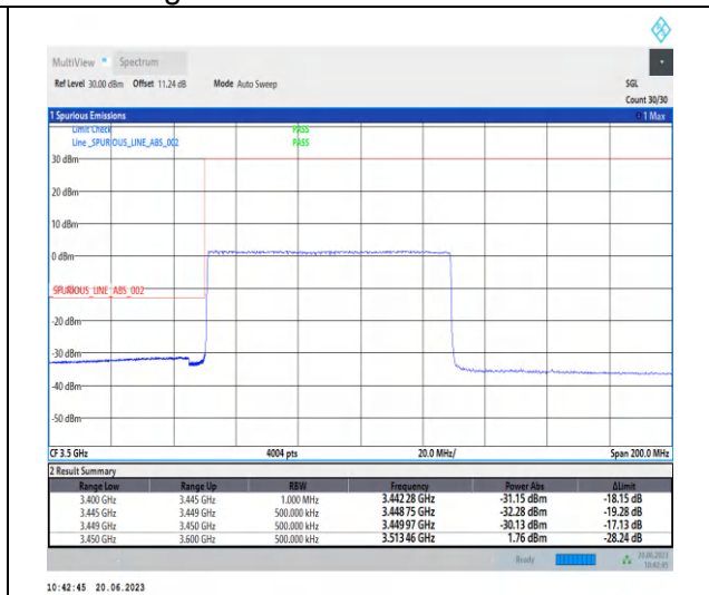
1-N78-3450-3550-PC2-30-80-L-3-CP-QPSK-Outer _Full-217@0-Ant2-1--PASS-see graph
