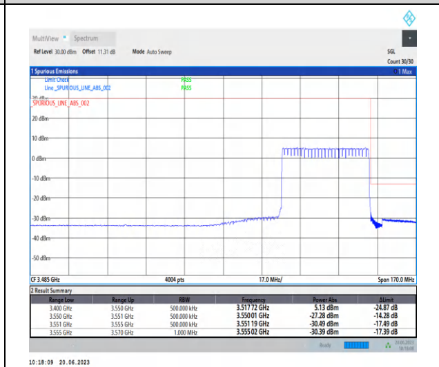
1-N78-3450-3550-PC2-30-40-H-3-CP-QPSK-Outer _Full-106@0-Ant2-1--PASS-see graph
