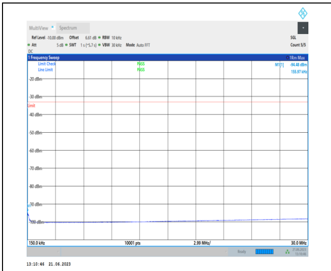
1-N78-3450-3550-PC2-30-100-M-1-N/A-DFT-QPSK-Edge_1RB_Left-1@0-0.15-30-Ant2-0.16--94.48--33-PASS
