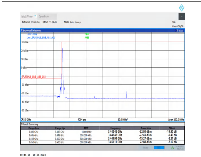
1-N78-3450-3550-PC2-30-80-L-1-CP-QPSK-Edge_1R B_Left-1@0-Ant2-1--PASS-see graph
