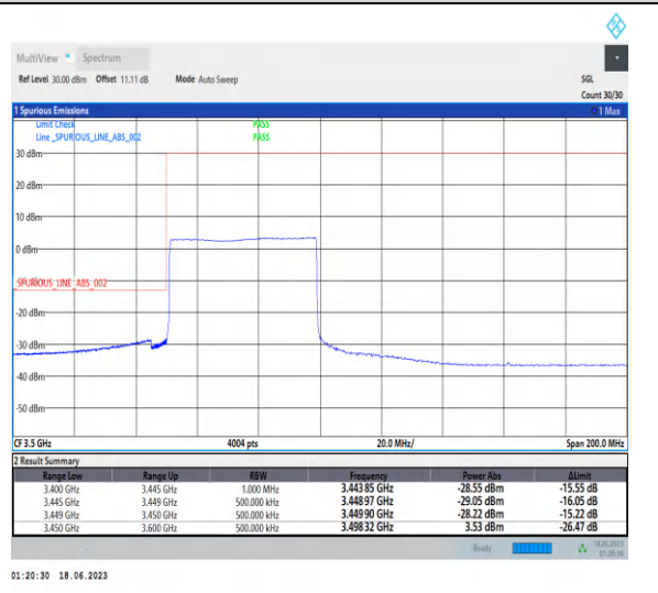
1-N78-3450-3550-PC2-30-50-L-6-CP-QPSK-Outer_Full-133@0-Ant2-1--PASS-see graph
