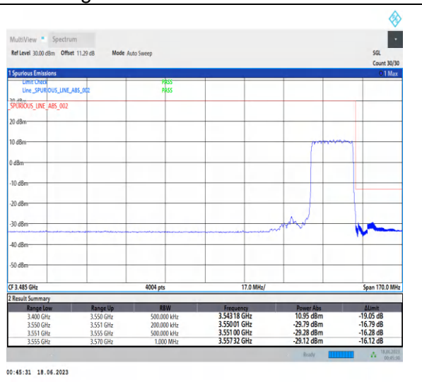
1-N78-3450-3550-PC2-30-20-H-3-DFT-PI2BPSK-Outer_Full-50@0-Ant2-1--PASS-see graph
