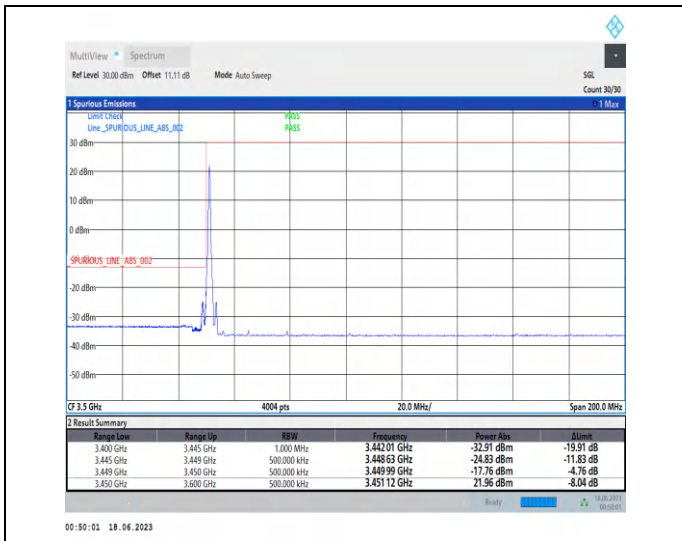
1-N78-3450-3550-PC2-30-30-L-1-DFT-PI2BPSK-Edge_1RB_Left-1@0-Ant2-1--PASS-see graph
