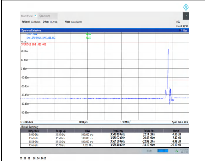
1-N78-3450-3550-PC2-30-10-H-5-CP-QPSK-Edge_1RB_Right-1@23-Ant2-1--PASS-see graph
