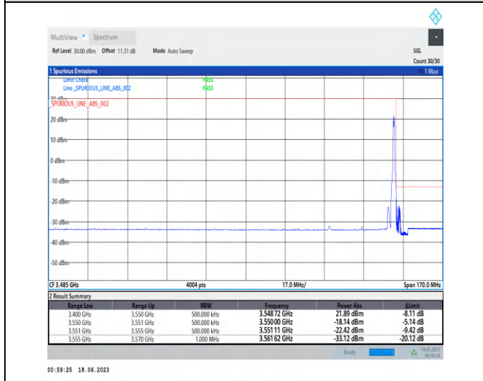
1-N78-3450-3550-PC2-30-30-H-5-CP-QPSK-Edge_1RB_Right-1@77-Ant2-1--PASS-see graph
