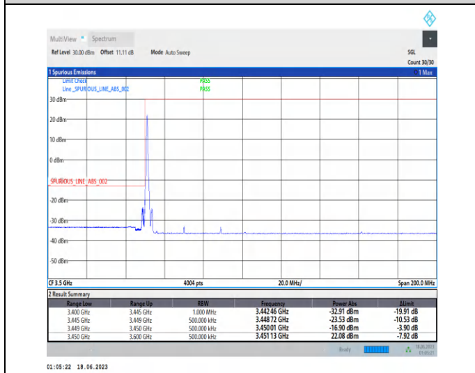
1-N78-3450-3550-PC2-30-40-L-4-CP-QPSK-Edge_1RB_Left-1@0-Ant2-1--PASS-see graph
