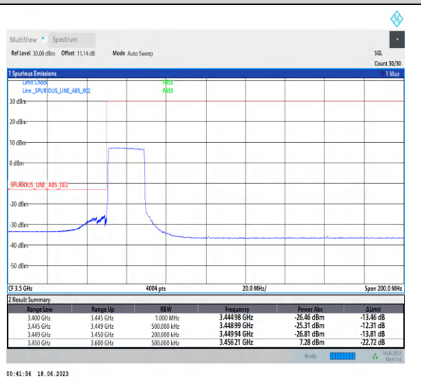
1-N78-3450-3550-PC2-30-20-L-6-CP-QPSK-Outer_Full-51@0-Ant2-1--PASS-see graph
