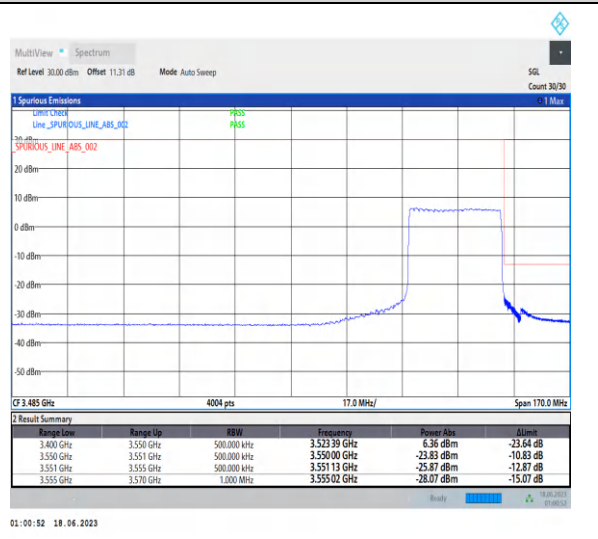
1-N78-3450-3550-PC2-30-30-H-6-CP-QPSK-Outer_Full-78@0-Ant2-1--PASS-see graph
