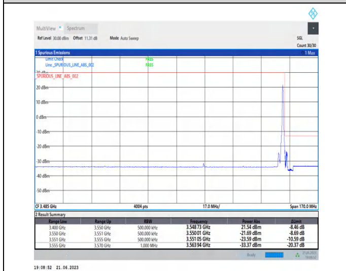
1-N78-3450-3550-PC2-30-50-H-5-CP-QPSK-Edge_1RB_Right-1@132-Ant2-1--PASS-see graph
