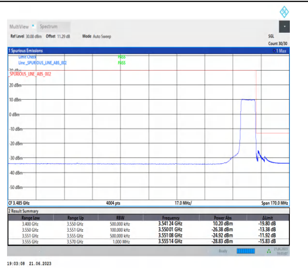
1-N78-3450-3550-PC2-30-10-H-6-CP-QPSK-Outer_Full-24@0-Ant2-1--PASS-see graph
