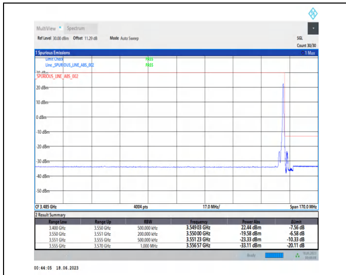
1-N78-3450-3550-PC2-30-20-H-2-DFT-PI2BPSK-Edge_1RB_Right-1@50-Ant2-1--PASS-see graph
