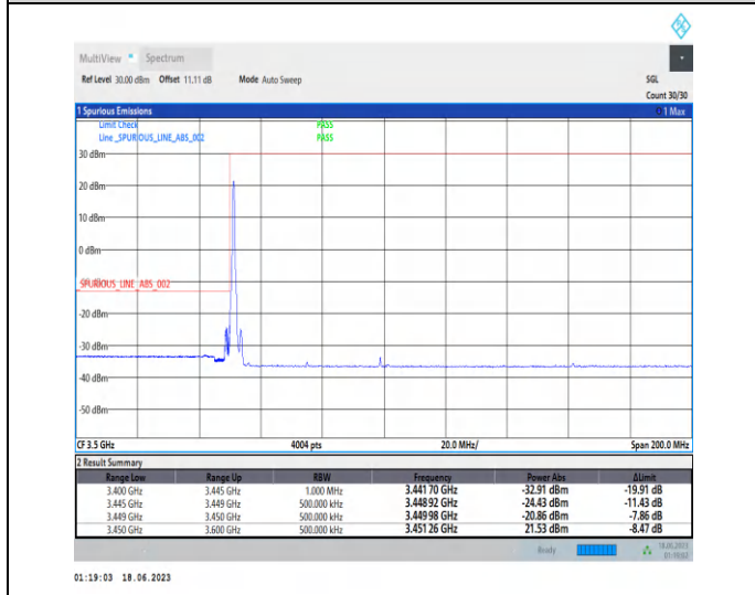
1-N78-3450-3550-PC2-30-50-L-4-CP-QPSK-Edge_1RB_Left-1@0-Ant2-1--PASS-see graph
