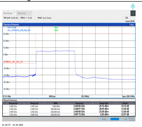
1-N78-3450-3550-PC2-30-60-L-3-DFT-PI2BPSK-Outer_Full-162@0-Ant2-1--PASS-see graph
