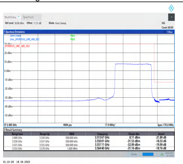
1-N78-3450-3550-PC2-30-40-H-3-DFT-PI2BPSK-Outer_Full-100@0-Ant2-1--PASS-see graph
