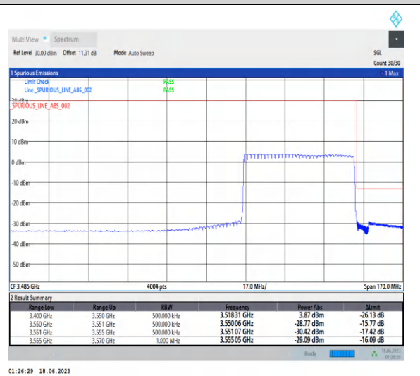
1-N78-3450-3550-PC2-30-50-H-6-CP-QPSK-Outer_Full-133@0-Ant2-1--PASS-see graph
