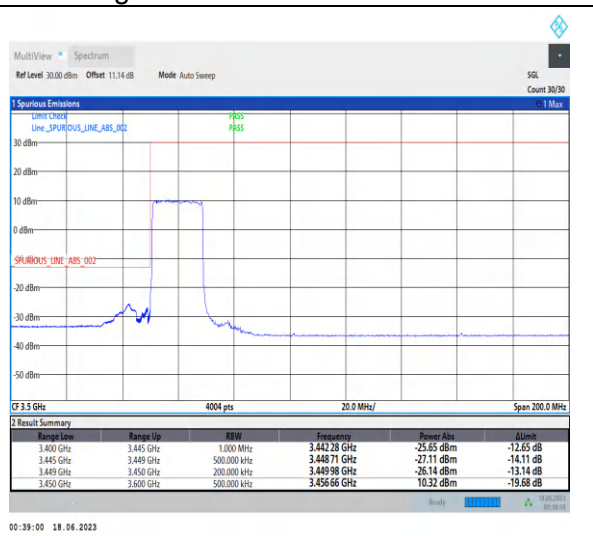
1-N78-3450-3550-PC2-30-20-L-3-DFT-PI2BPSK-Outer_Full-50@0-Ant2-1--PASS-see graph
