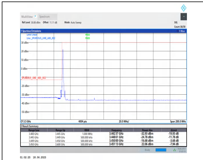
1-N78-3450-3550-PC2-30-40-L-1-DFT-PI2BPSK-Edge_1RB_Left-1@0-Ant2-1--PASS-see graph
