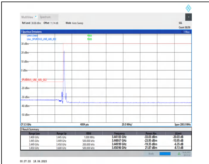
1-N78-3450-3550-PC2-30-20-L-1-DFT-PI2BPSK-Edge_1RB_Left-1@0-Ant2-1--PASS-see graph
