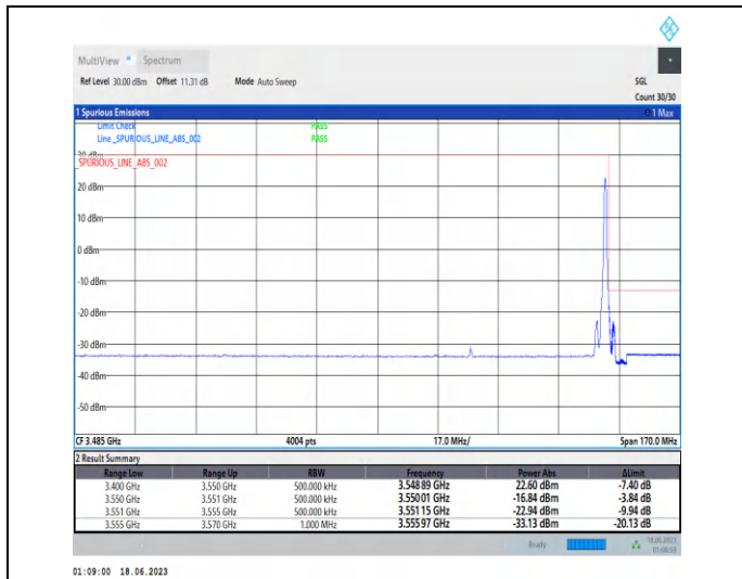
1-N78-3450-3550-PC2-30-40-H-2-DFT-PI2BPSK-Edge_1RB_Right-1@105-Ant2-1--PASS-see graph
