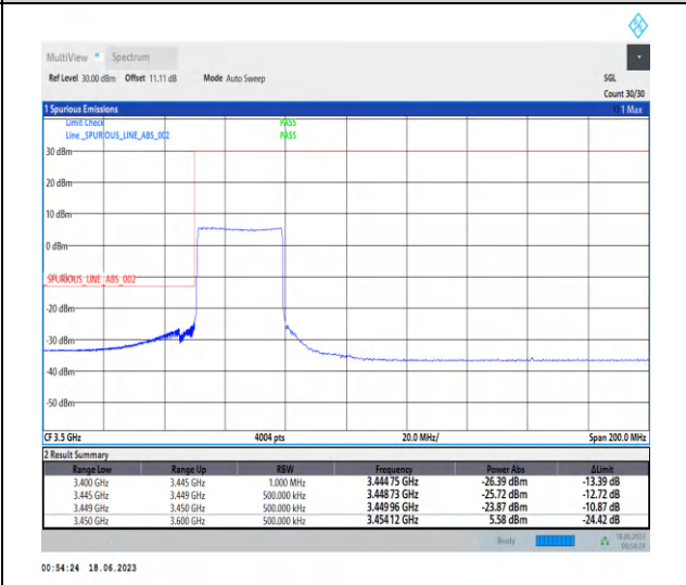
1-N78-3450-3550-PC2-30-30-L-6-CP-QPSK-Outer_Full-78@0-Ant2-1--PASS-see graph
