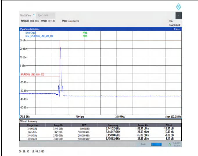
1-N78-3450-3550-PC2-30-15-L-4-CP-QPSK-Edge_1RB_Left-1@0-Ant2-1--PASS-see graph
