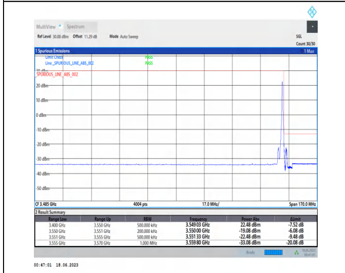
1-N78-3450-3550-PC2-30-20-H-5-CP-QPSK-Edge_1RB_Right-1@50-Ant2-1--PASS-see graph
