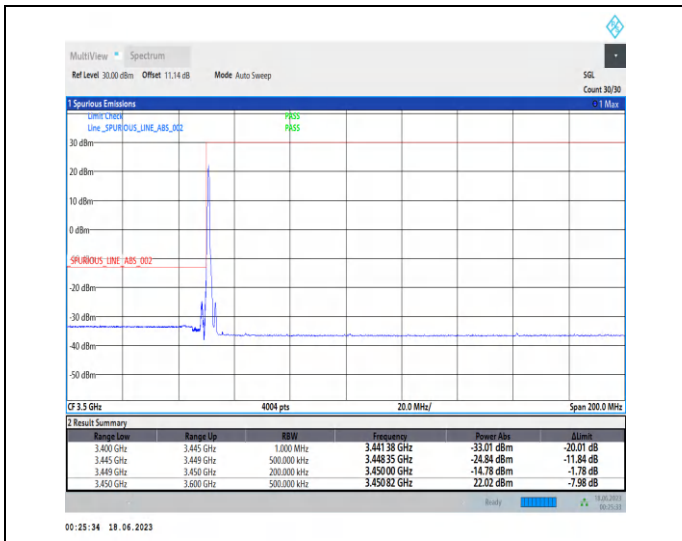
1-N78-3450-3550-PC2-30-15-L-1-DFT-PI2BPSK-Edge_1RB_Left-1@0-Ant2-1--PASS-see graph
