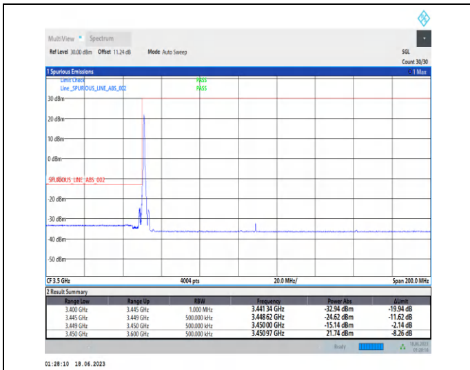
1-N78-3450-3550-PC2-30-60-L-1-DFT-PI2BPSK-Edge_1RB_Left-1@0-Ant2-1--PASS-see graph
