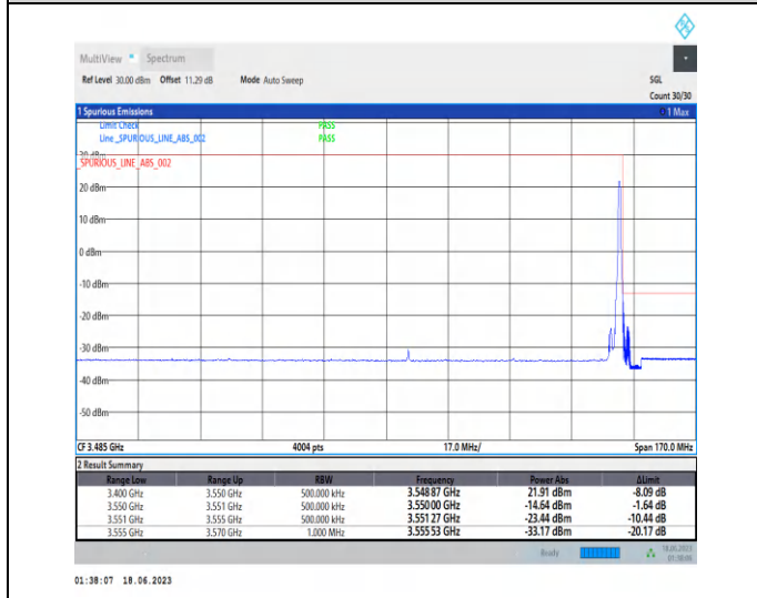
1-N78-3450-3550-PC2-30-60-H-5-CP-QPSK-Edge_1RB_Right-1@161-Ant2-1--PASS-see graph
