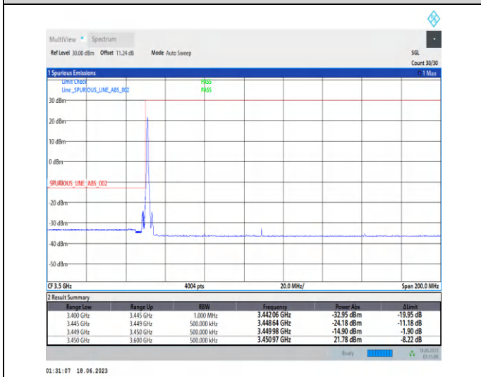
1-N78-3450-3550-PC2-30-60-L-4-CP-QPSK-Edge_1RB_Left-1@0-Ant2-1--PASS-see graph
