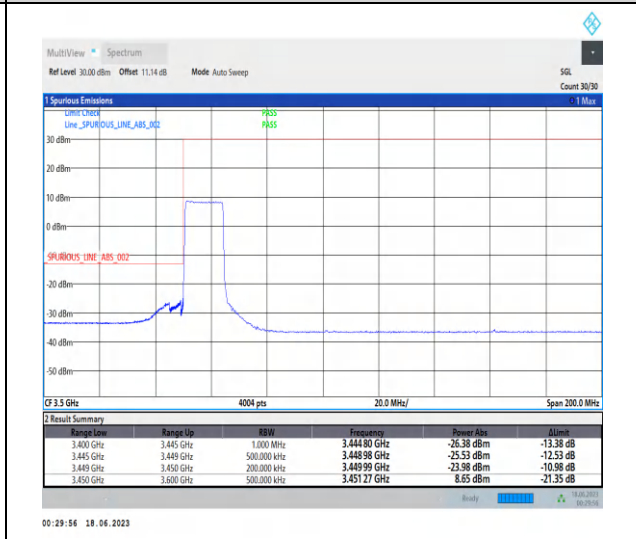
1-N78-3450-3550-PC2-30-15-L-6-CP-QPSK-Outer_Full-38@0-Ant2-1--PASS-see graph
