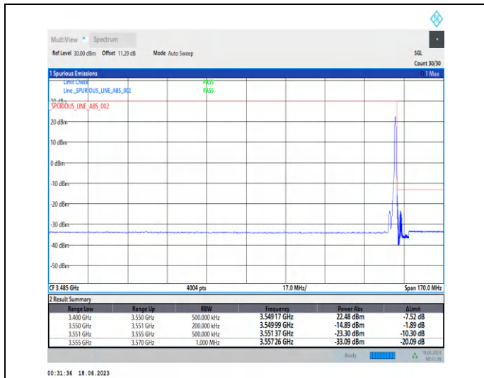
1-N78-3450-3550-PC2-30-15-H-2-DFT-PI2BPSK-Edge_1RB_Right-1@37-Ant2-1--PASS-see graph
