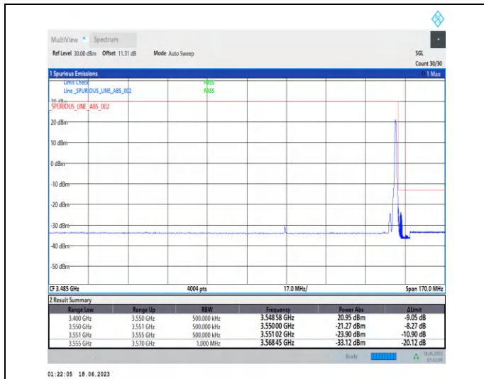
1-N78-3450-3550-PC2-30-50-H-2-DFT-PI2BPSK-Edge_1RB_Right-1@132-Ant2-1--PASS-see graph
