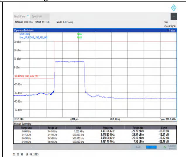
1-N78-3450-3550-PC2-30-40-L-3-DFT-PI2BPSK-Outer_Full-100@0-Ant2-1--PASS-see graph
