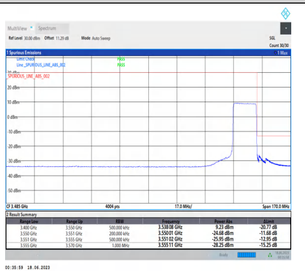
1-N78-3450-3550-PC2-30-15-H-6-CP-QPSK-Outer_Full-38@0-Ant2-1--PASS-see graph
