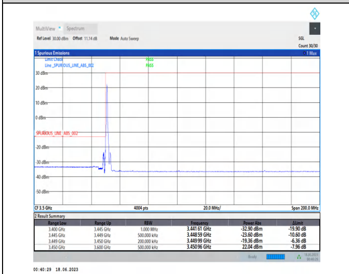
1-N78-3450-3550-PC2-30-20-L-4-CP-QPSK-Edge_1RB_Left-1@0-Ant2-1--PASS-see graph
