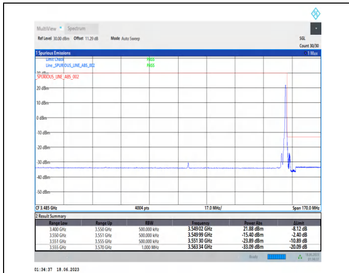
1-N78-3450-3550-PC2-30-60-H-2-DFT-PI2BPSK-Edge_1RB_Right-1@161-Ant2-1--PASS-see graph
