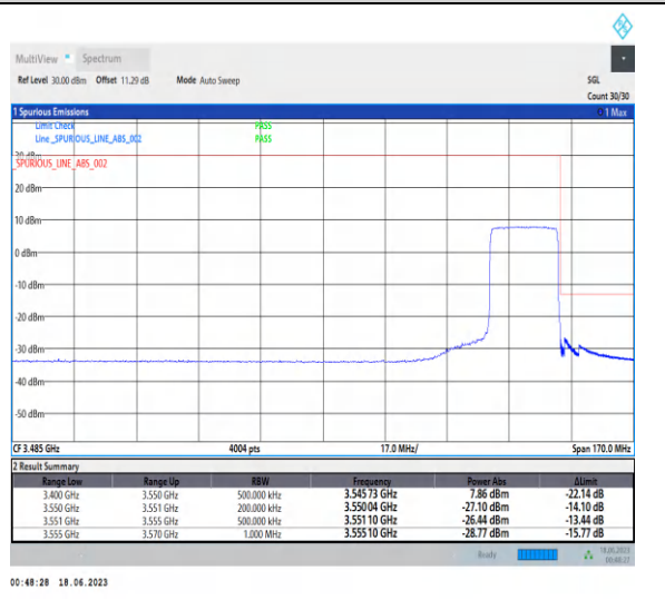
1-N78-3450-3550-PC2-30-20-H-6-CP-QPSK-Outer_Full-51@0-Ant2-1--PASS-see graph
