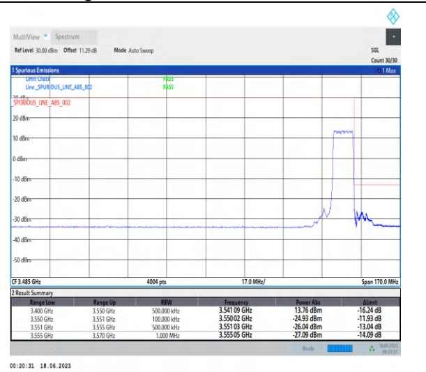
1-N78-3450-3550-PC2-30-10-H-3-DFT-PI2BPSK-Outer_Full-24@0-Ant2-1--PASS-see graph
