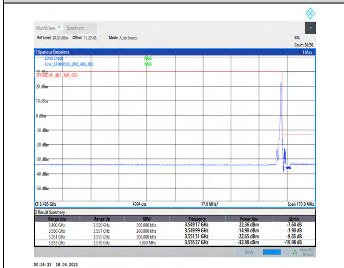
1-N78-3450-3550-PC2-30-15-H-5-CP-QPSK-Edge_1RB_Right-1@37-Ant2-1--PASS-see graph
