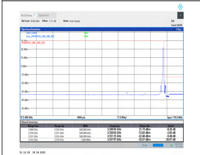
1-N78-3450-3550-PC2-30-40-H-5-CP-QPSK-Edge_1RB_Right-1@105-Ant2-1--PASS-see graph
