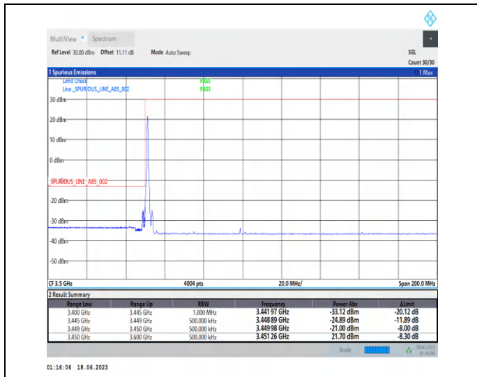
1-N78-3450-3550-PC2-30-50-L-1-DFT-PI2BPSK-Edge_1RB_Left-1@0-Ant2-1--PASS-see graph
