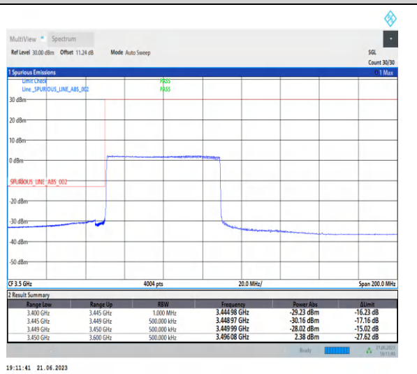
1-N78-3450-3550-PC2-30-60-L-6-CP-QPSK-Outer_Full-162@0-Ant2-1--PASS-see graph
