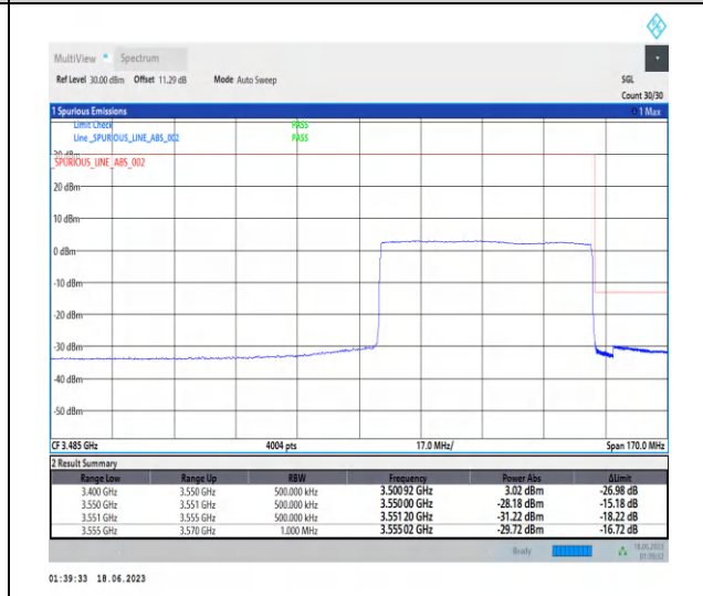
1-N78-3450-3550-PC2-30-60-H-6-CP-QPSK-Outer_Full-162@0-Ant2-1--PASS-see graph
