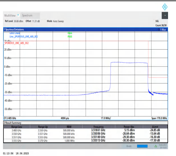
1-N78-3450-3550-PC2-30-40-H-6-CP-QPSK-Outer_Full-106@0-Ant2-1--PASS-see graph
