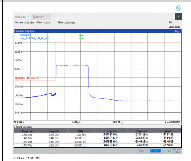
1-N78-3450-3550-PC2-30-40-L-6-CP-QPSK-Outer_Full-106@0-Ant2-1--PASS-see graph
