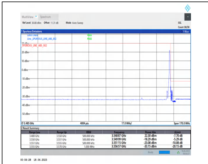
1-N78-3450-3550-PC2-30-30-H-2-DFT-PI2BPSK-Edge_1RB_Right-1@77-Ant2-1--PASS-see graph
