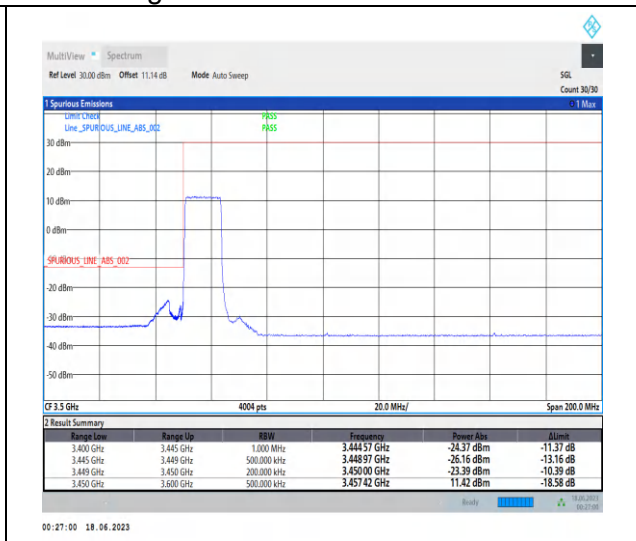
1-N78-3450-3550-PC2-30-15-L-3-DFT-PI2BPSK-Outer_Full-36@0-Ant2-1--PASS-see graph
