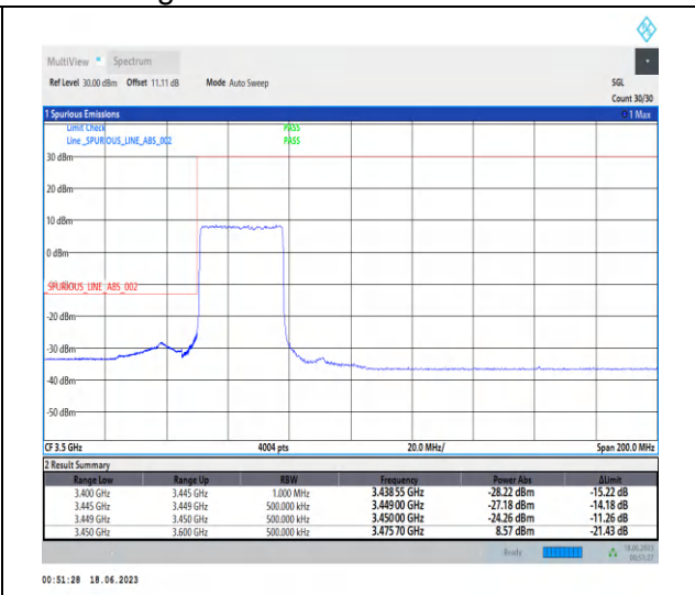
1-N78-3450-3550-PC2-30-30-L-3-DFT-PI2BPSK-Outer_Full-75@0-Ant2-1--PASS-see graph
