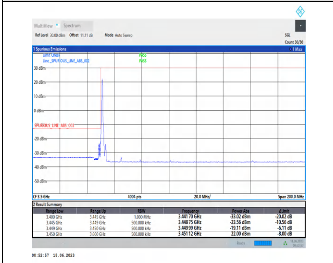
1-N78-3450-3550-PC2-30-30-L-4-CP-QPSK-Edge_1RB_Left-1@0-Ant2-1--PASS-see graph
