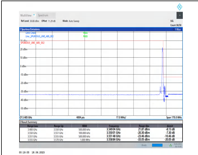
1-N78-3450-3550-PC2-30-10-H-2-DFT-PI2BPSK-Edge_1RB_Right-1@23-Ant2-1--PASS-see graph
