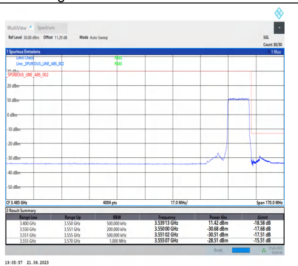
1-N78-3450-3550-PC2-30-15-H-3-DFT-PI2BPSK-Outer_Full-36@0-Ant2-1--PASS-see graph
