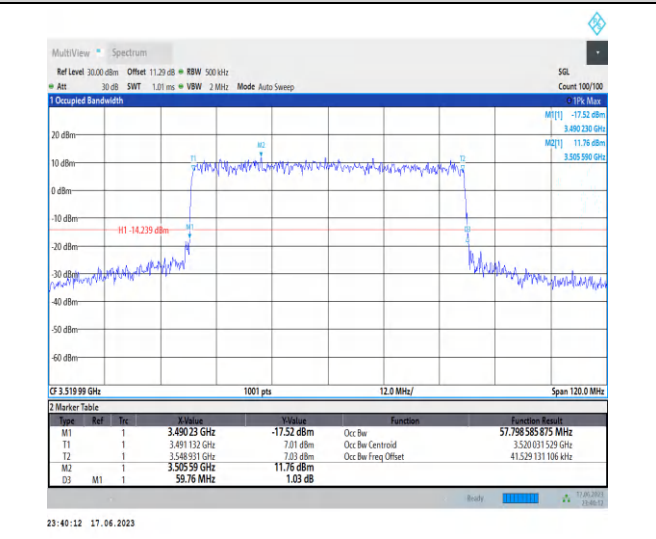
1-N78-3450-3550-PC2-30-60-H-8-CP-64QAM-Outer_Full-162@0-Ant2-57.799-59.760-≤60-PASS
