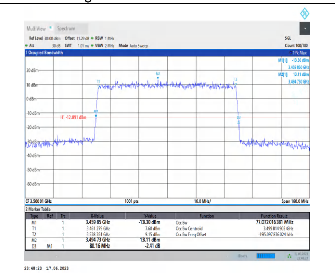
1-N78-3450-3550-PC2-30-80-M-5-DFT-256QAM-Out_er_Full-216@0-Ant2-77.072-80.160-≤80-PASS
