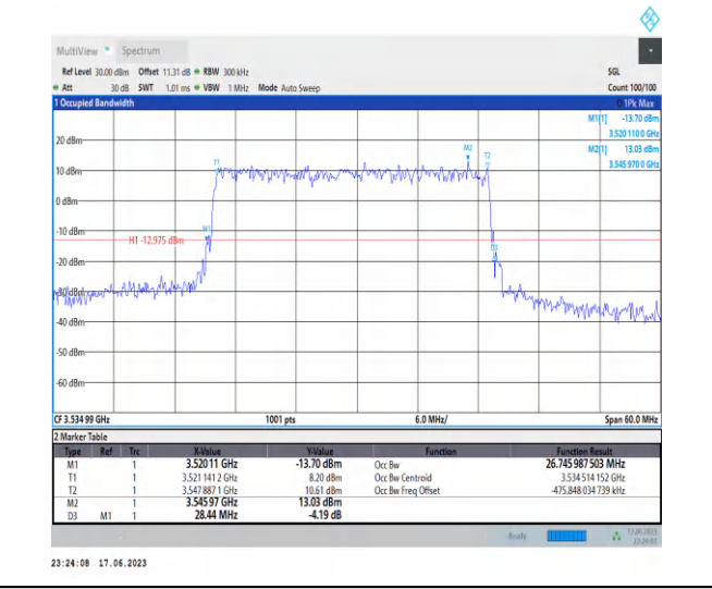
1-N78-3450-3550-PC2-30-30-H-5-DFT-256QAM-Outer_Full-75@0-Ant2-26.746-28.440-≤30-PASS
