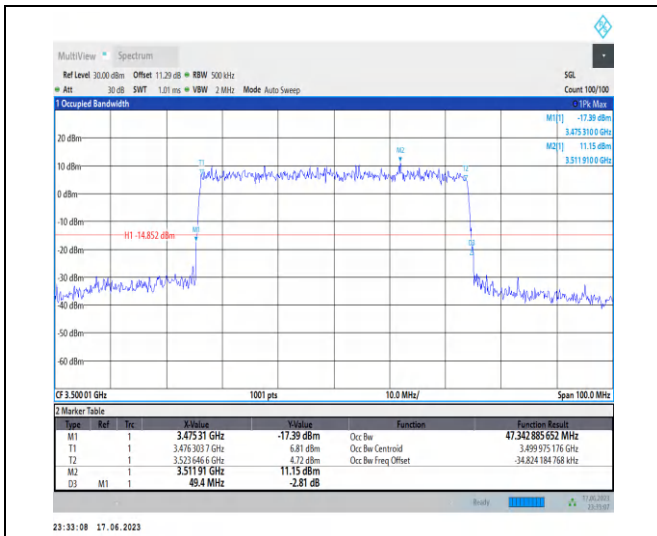
1-N78-3450-3550-PC2-30-50-M-9-CP-256QAM-Out er_Full-133@0-Ant2-47.343-49.400-≤50-PASS
