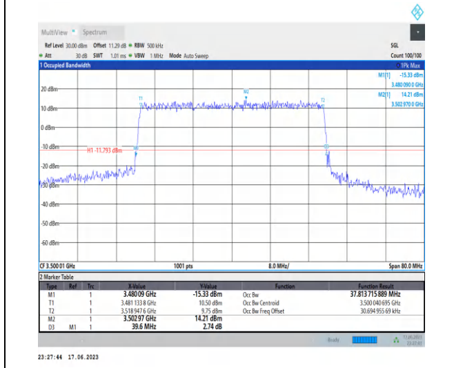
1-N78-3450-3550-PC2-30-40-M-6-CP-QPSK-Outer_Full-106@0-Ant2-37.814-39.600-≤40-PASS
