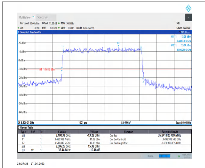
1-N78-3450-3550-PC2-30-40-M-4-DFT-64QAM-Out er_Full-100@0-Ant2-35.842-37.440-≤40-PASS
