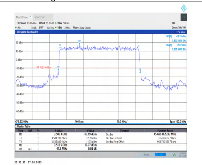
1-N78-3450-3550-PC2-30-50-H-1-DFT-PI2BPSK-Out er_Full-128@0-Ant2-45.696-47.500-≤50-PASS
