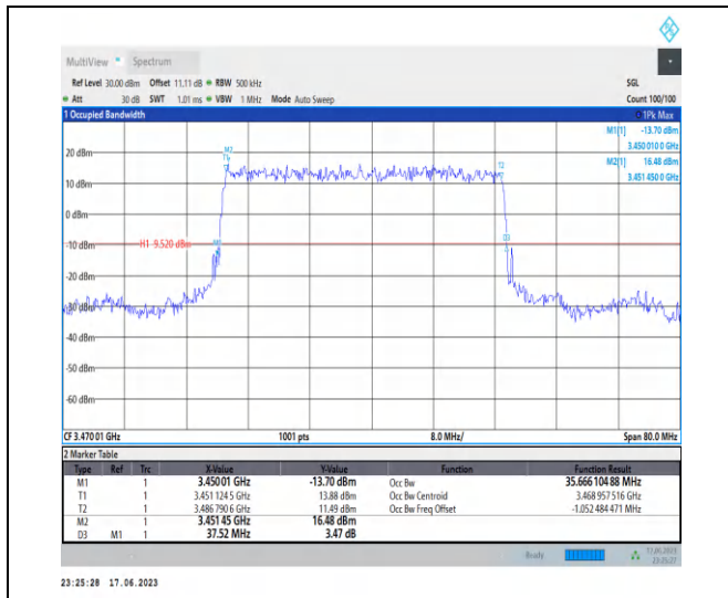
1-N78-3450-3550-PC2-30-40-L-1-DFT-PI2BPSK-Out er_Full-100@0-Ant2-35.666-37.520-≤40-PASS
