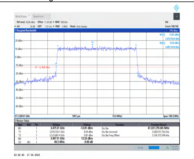
1-N78-3450-3550-PC2-30-50-M-6-CP-QPSK-Outer_Full-133@0-Ant2-47.331-49.500-≤50-PASS
