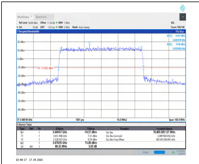
1-N78-3450-3550-PC2-30-80-L-1-DFT-PI2BPSK-Out er_Full-216@0-Ant2-76.805-80.320-≤80-PASS
