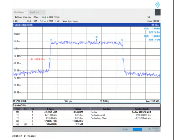
1-N78-3450-3550-PC2-30-60-M-5-DFT-256QAM-Outer_Full-162@0-Ant2-57.822-59.640-≤60-PASS
