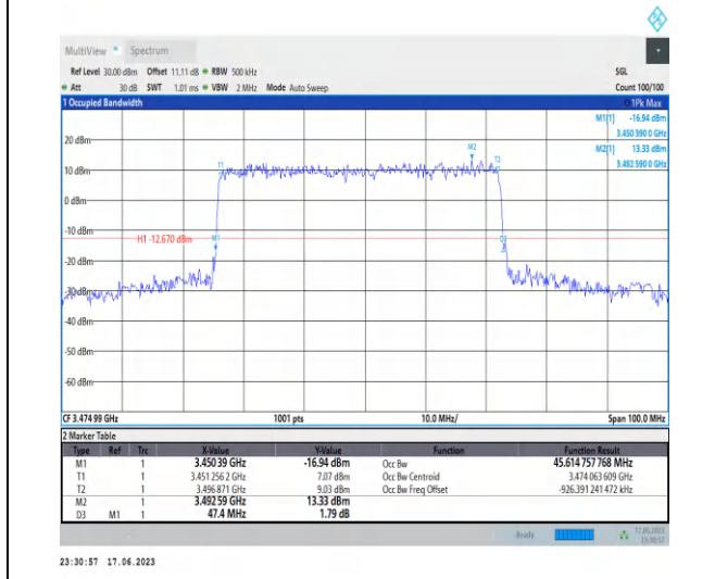
1-N78-3450-3550-PC2-30-50-L-4-DFT-64QAM-Outer_Full-128@0-Ant2-45.615-47.400-≤50-PASS
