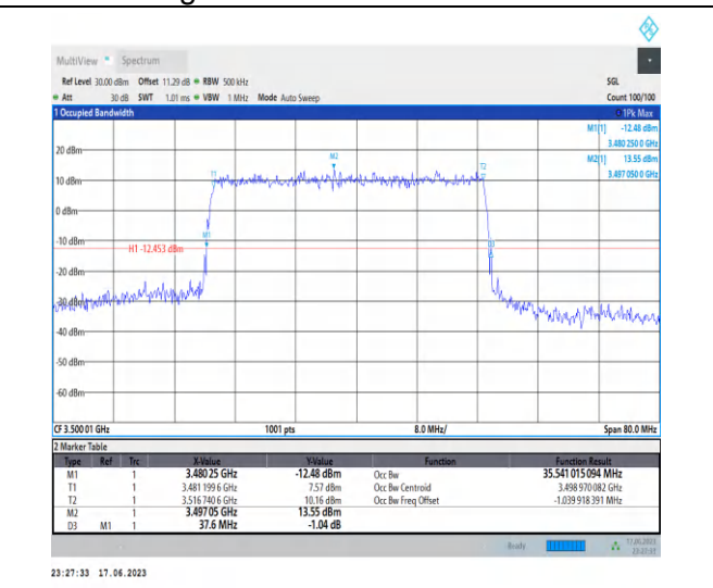
1-N78-3450-3550-PC2-30-40-M-5-DFT-256QAM-Out er_Full-100@0-Ant2-35.541-37.600-≤40-PASS
