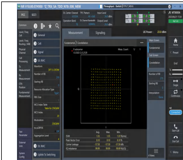
1-N78-3450-3550-PC2-30-100-M-5-DFT-256QAM-Outer_Full-270@0-Ant2-see graph-PASS
