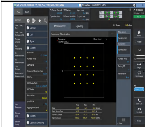
1-N78-3450-3550-PC2-30-100-M-7-CP-16QAM-Outer_Full-273@0-Ant2-see graph-PASS
