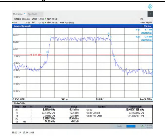
1-N78-3450-3550-PC2-30-15-H-1-DFT-PI2BPSK-Out er_Full-36@0-Ant2-12.909-14.250-≤15-PASS
