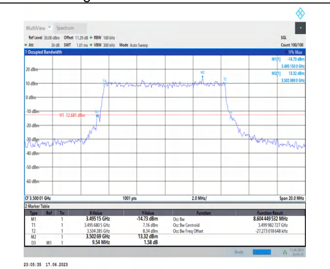
1-N78-3450-3550-PC2-30-10-M-5-DFT-256QAM-Out er_Full-24@0-Ant2-8.604-9.540-≤10-PASS
