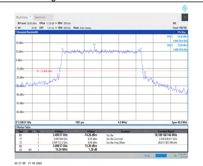
1-N78-3450-3550-PC2-30-20-M-7-CP-16QAM-Outer_Full-51 @0-Ant2-18.189-19.240-≤20-PASS
