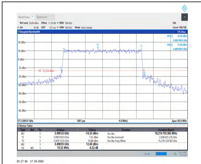
1-N78-3450-3550-PC2-30-20-M-6-CP-QPSK-Outer_Full-51 @0-Ant2-18.217-19.520-≤20-PASS
