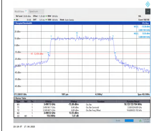
1-N78-3450-3550-PC2-30-20-M-8-CP-64QAM-Outer_Full-51 @0-Ant2-18.126-19.600-≤20-PASS
