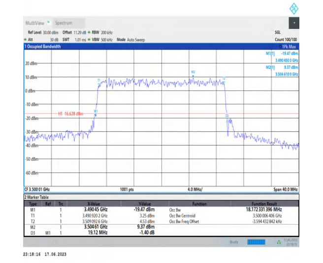
1-N78-3450-3550-PC2-30-20-M-9-CP-256QAM-Outer_Full-51 @0-Ant2-18.172-19.120-≤20-PASS
