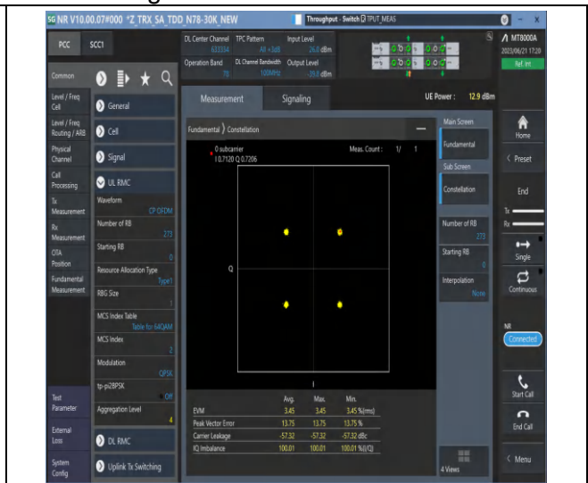
1-N78-3450-3550-PC2-30-100-M-6-CP-QPSK-Outer_Full-273@0-Ant2-see graph-PASS
