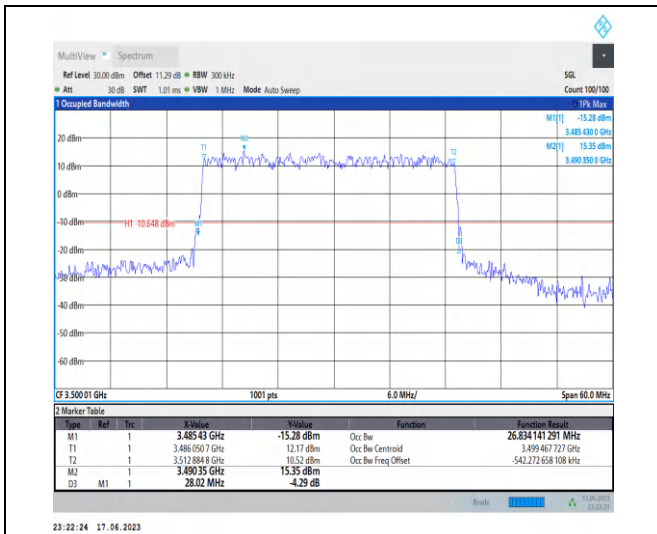
1-N78-3450-3550-PC2-30-30-M-3-DFT-16QAM-Out er_Full-75@0-Ant2-26.834-28.020-≤30-PASS
