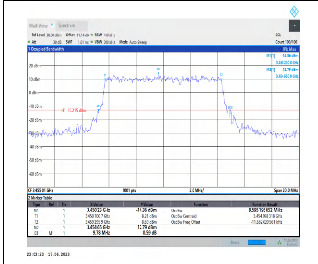
1-N78-3450-3550-PC2-30-10-L-3-DFT-16QAM-Outer r_Full-24@0-Ant2-8.595-9.780-≤10-PASS
