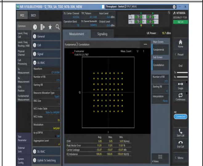
1-N78-3450-3550-PC2-30-100-M-8-CP-64QAM-Outer_Full-273@0-Ant2-see graph-PASS
