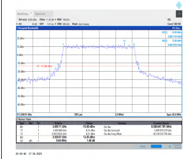
1-N78-3450-3550-PC2-30-10-M-6-CP-QPSK-Outer Full-24@0-Ant2-8.581-9.640-≤10-PASS
