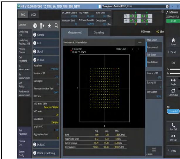
1-N78-3450-3550-PC2-30-100-M-9-CP-256QAM-Out er_Full-273@0-Ant2-see graph-PASS
