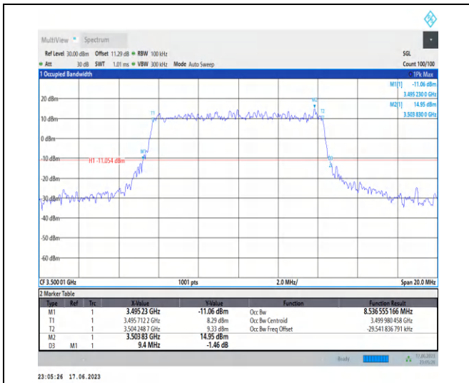
1-N78-3450-3550-PC2-30-10-M-4-DFT-64QAM-Out er_Full-24@0-Ant2-8.537-9.400-≤10-PASS
