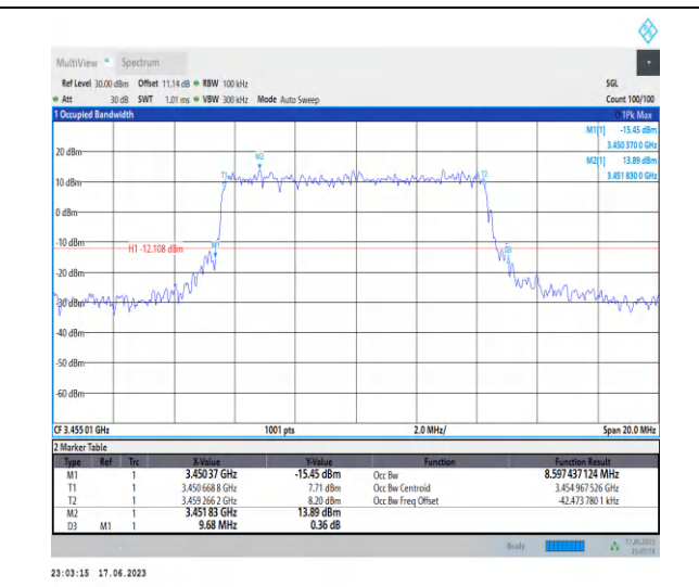
1-N78-3450-3550-PC2-30-10-L-2-DFT-QPSK-Outer Full-24@0-Ant2-8.597-9.680-≤10-PASS
