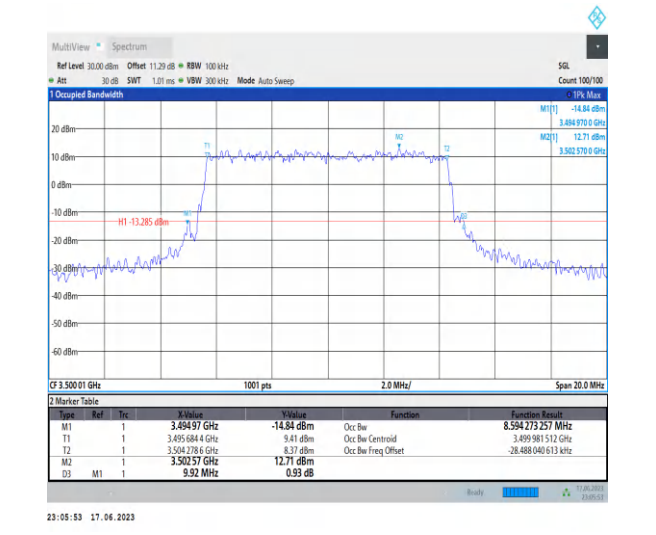
1-N78-3450-3550-PC2-30-10-M-7-CP-16QAM-Outer _Full-24@0-Ant2-8.594-9.920-≤10-PASS
