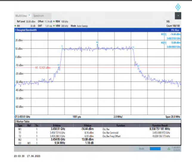
1-N78-3450-3550-PC2-30-10-L-4-DFT-64QAM-Outer _Full-24@0-Ant2-8.559-9.540-≤10-PASS
