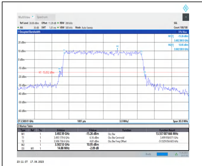
1-N78-3450-3550-PC2-30-15-M-9-CP-256QAM-Out er_Full-38@0-Ant2-13.557-14.880-≤15-PASS
