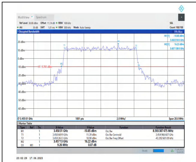
1-N78-3450-3550-PC2-30-10-L-1-DFT-PI2BPSK-Out er_Full-24@0-Ant2-8.593-9.260-≤10-PASS
