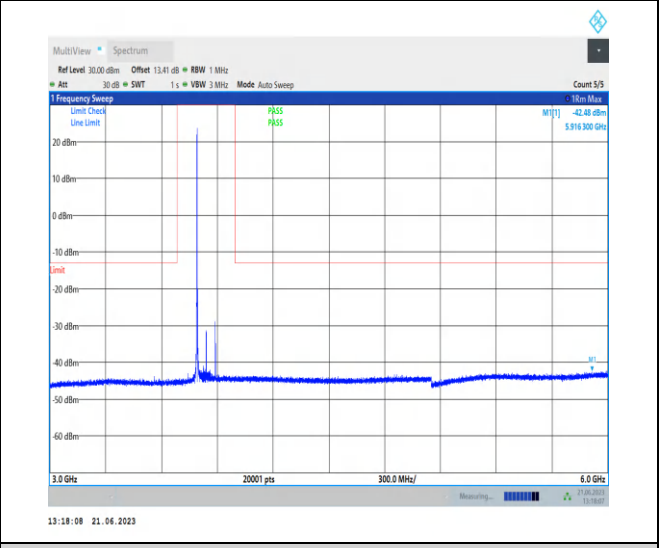
1-N77-3700-3980-PC2-30-100-M-1-NS_01-DFT-QP SK-Edge_1RB_Left-1@0-3000-6000-Ant2-5177.85-- 42.48--13-PASS
