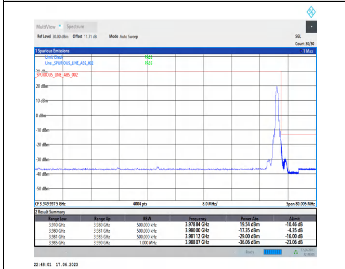
1-N77-3700-3980-PC3-30-70-H-5-CP-QPSK-Edge_1RB_Right-1@188-Ant2-1--PASS-see graph
