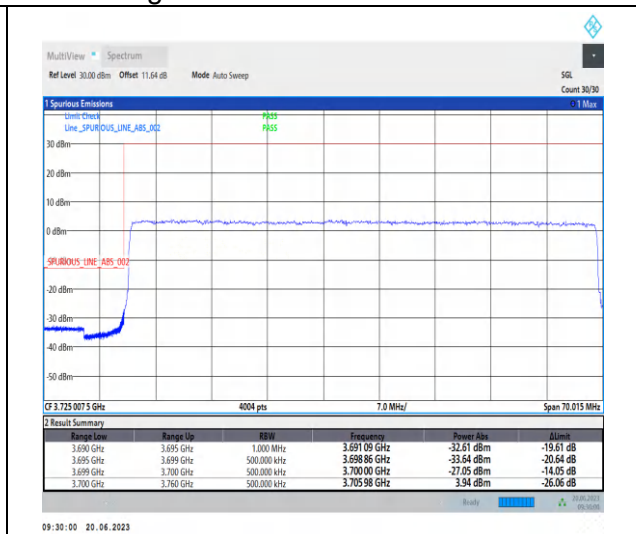
1-N77-3700-3980-PC2-30-60-L-3-CP-QPSK-Outer _Full-162@0-Ant2-1--PASS-see graph
