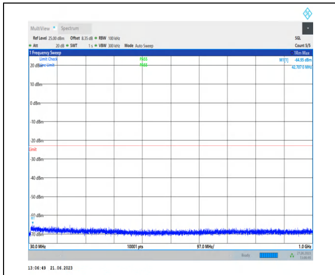
1-N77-3700-3980-PC2-30-100-H-1-NS_01-DFT-QP SK-Edge_1RB_Left-1@0-30-1000-Ant2-42.71--64.9 5--23-PASS
