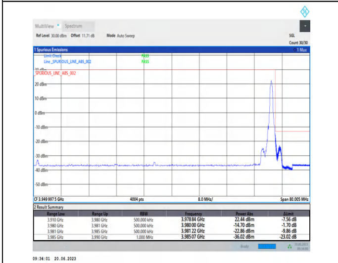
1-N77-3700-3980-PC2-30-70-H-2-CP-QPSK-Edge_1R B_Right-1@188-Ant2-1--PASS-see graph
