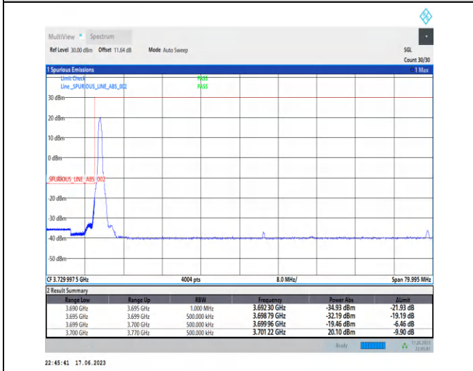
1-N77-3700-3980-PC3-30-70-L-4-CP-QPSK-Edge_1RB_Left-1@0-Ant2-1--PASS-see graph
