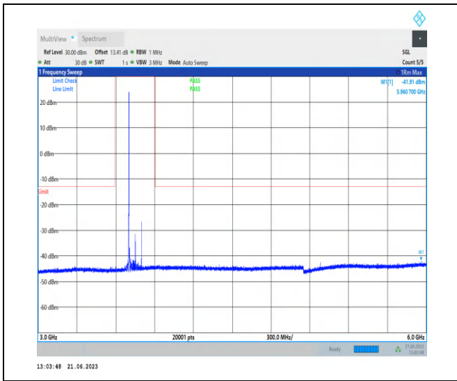
1-N77-3700-3980-PC2-30-100-L-1-NS_01-DFT-QPS K-Edge_1RB_Left-1@0-3000-6000-Ant2-5227.65--4 1.91--13-PASS
