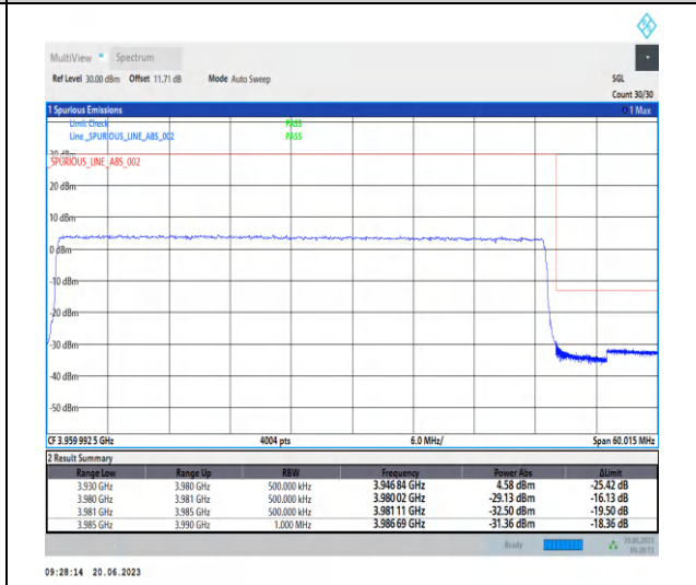
1-N77-3700-3980-PC2-30-50-H-3-CP-QPSK-Outer _Full-133@0-Ant2-1--PASS-see graph
