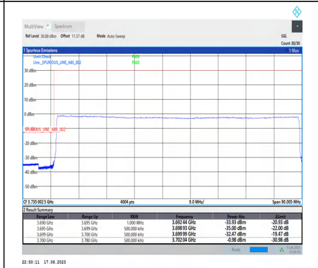
1-N77-3700-3980-PC3-30-80-L-6-CP-QPSK-Outer_Full-217@0-Ant2-1--PASS-see graph
