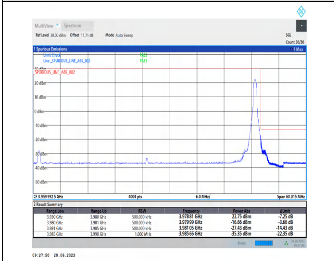
1-N77-3700-3980-PC2-30-50-H-2-CP-QPSK-Edge_1R B_Right-1@132-Ant2-1--PASS-see graph
