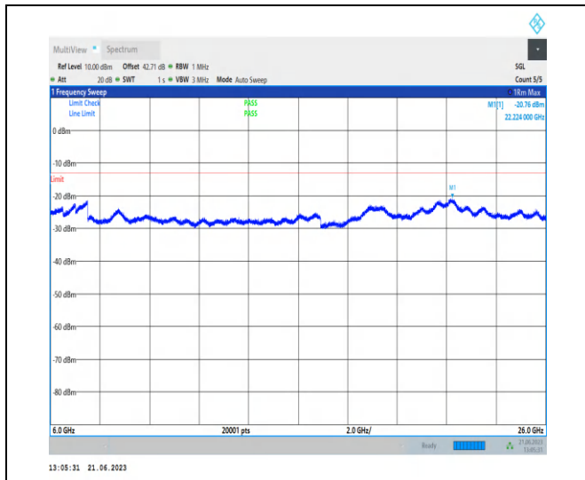
1-N77-3700-3980-PC2-30-100-M-1-NS_01-DFT-QP SK-Edge_1RB_Left-1@0-6000-26000-Ant2-22224.0 0--20.76--13-PASS
