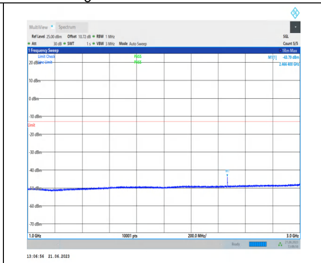
1-N77-3700-3980-PC2-30-100-H-1-NS_01-DFT-QPS K-Edge_1RB_Left-1@0-1000-3000-Ant2-2466.40--4 3.79--13-PASS
