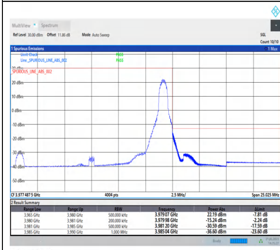
1-N77-3700-3980-PC2-30-15-H-2-CP-QPSK-Edge_1R_B_Right-1@37-Ant2-1--PASS-see graph
