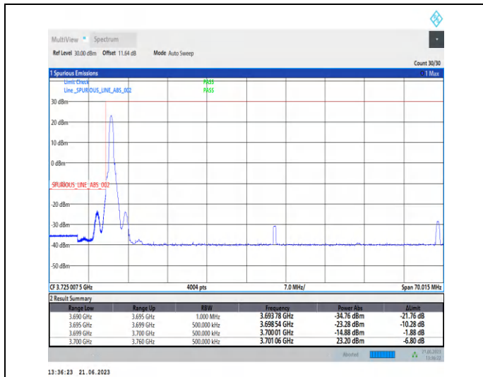
1-N77-3700-3980-PC2-30-60-L-1-CP-QPSK-Edge_1R B_Left-1@0-Ant2-1--PASS-see graph
