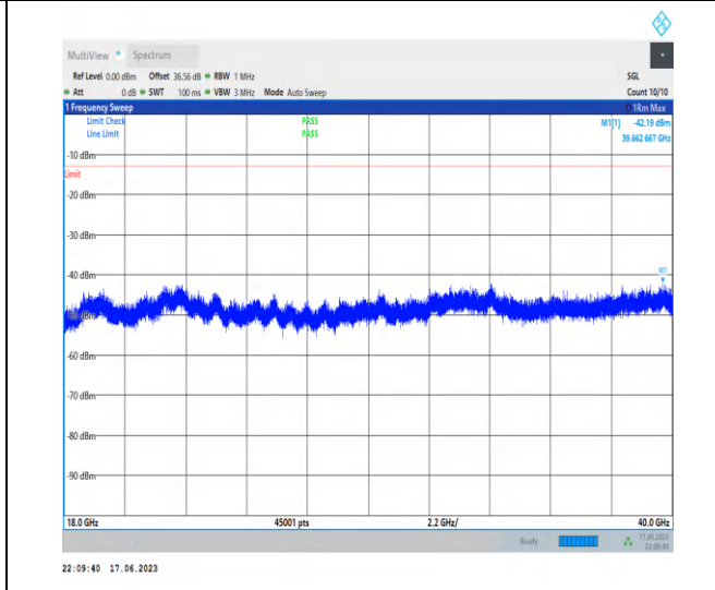
1-N77-3700-3980-PC3-30-100-M-1-N/A-DFT-PI2BPS K-Inner_1RB_Left-1@1-18000-40000-Ant2-39662.67 --42.19--13-PASS
