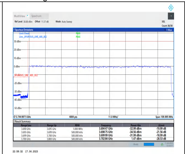
1-N77-3700-3980-PC3-30-100-L-3-DFT-PI2BPSK-Outer_Full-270@0-Ant2-1--PASS-see graph
