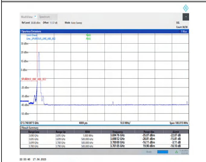
1-N77-3700-3980-PC3-30-90-L-4-CP-QPSK-Edge_1RB_Left-1@0-Ant2-1--PASS-see graph
