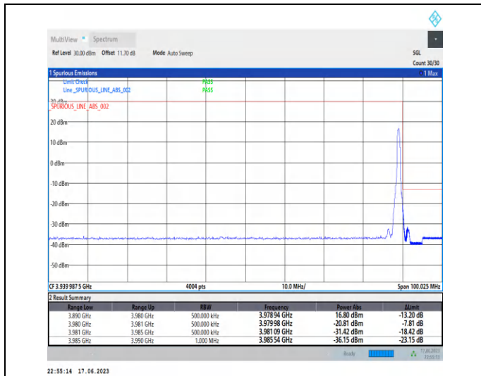
1-N77-3700-3980-PC3-30-90-H-2-DFT-PI2BPSK-Edge_1RB_Right-1@244-Ant2-1--PASS-see graph
