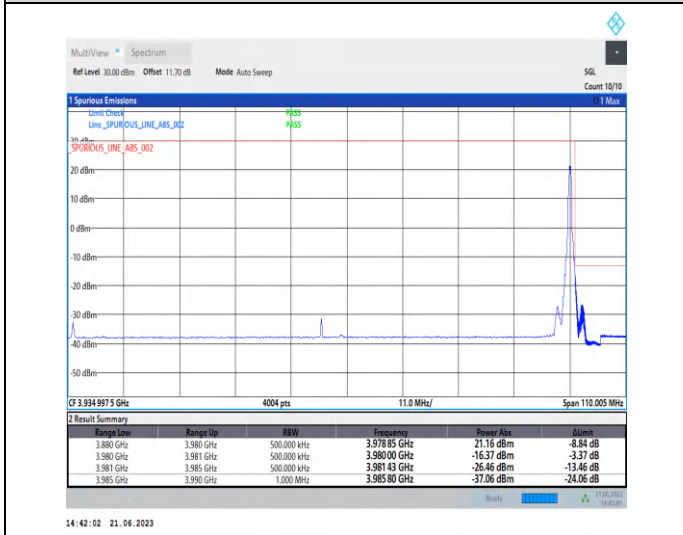
1-N77-3700-3980-PC2-30-100-H-2-CP-QPSK-Edge_1 RB_Right-1@272-Ant2-1--PASS-see graph
