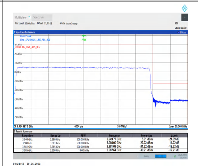
1-N77-3700-3980-PC2-30-40-H-3-CP-QPSK-Outer _Full-106@0-Ant2-1--PASS-see graph
