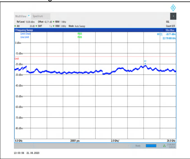
1-N77-3700-3980-PC2-30-100-L-1-NS_01-DFT-QPS K-Edge_1RB_Left-1@0-6000-26000-Ant2-22151.00-- -20.71--13-PASS
