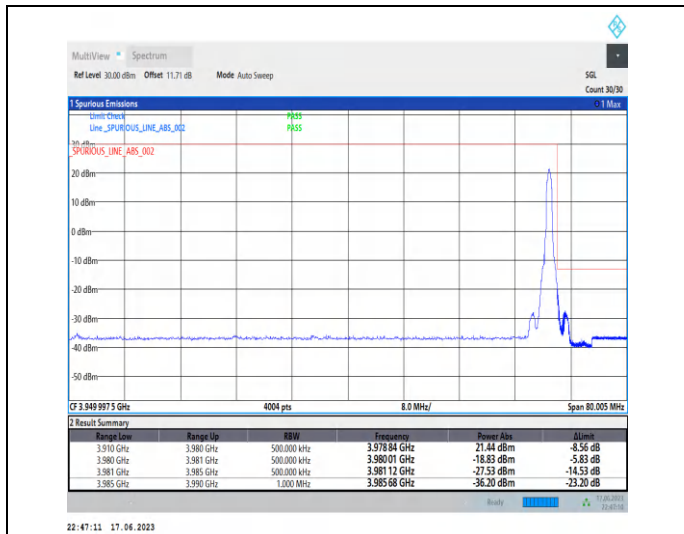
1-N77-3700-3980-PC3-30-70-H-2-DFT-PI2BPSK-Edge_1RB_Right-1@188-Ant2-1--PASS-see graph
