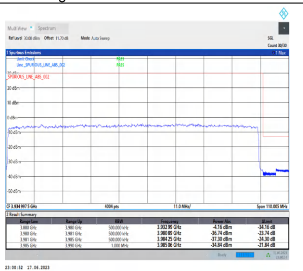
1-N77-3700-3980-PC3-30-100-H-3-DFT-PI2BPSK-Outer_Full-270@0-Ant2-1--PASS-see graph
