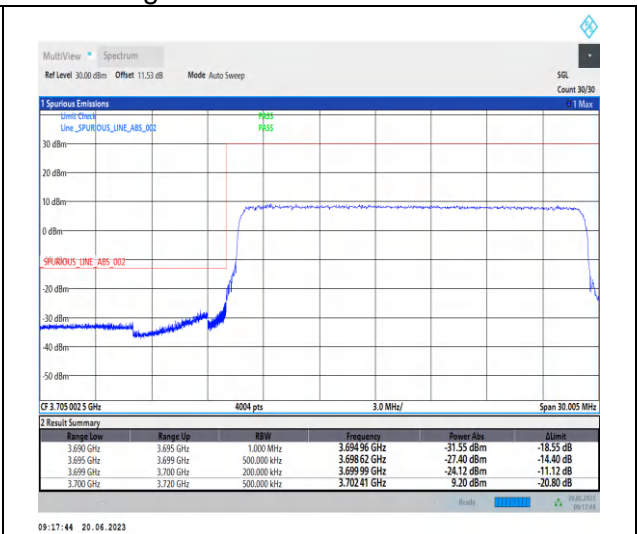
1-N77-3700-3980-PC2-30-20-L-3-CP-QPSK-Outer _Full-51@0-Ant2-1--PASS-see graph
