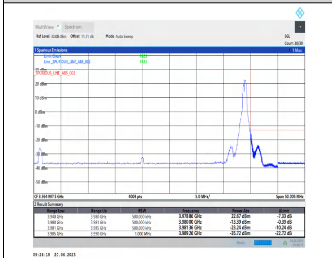
1-N77-3700-3980-PC2-30-40-H-2-CP-QPSK-Edge_1R B_Right-1@105-Ant2-1--PASS-see graph
