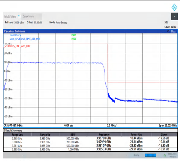
1-N77-3700-3980-PC2-30-15-H-3-CP-QPSK-Outer_Full-38@0-Ant2-1--PASS-see graph
