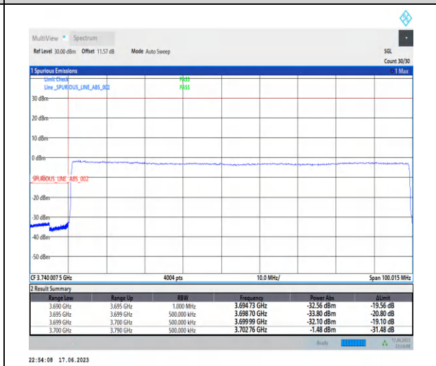
1-N77-3700-3980-PC3-30-90-L-6-CP-QPSK-Outer_Full-245@0-Ant2-1--PASS-see graph
