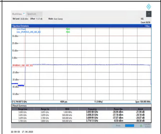
1-N77-3700-3980-PC3-30-100-L-6-CP-QPSK-Outer_Full-273@0-Ant2-1--PASS-see graph
