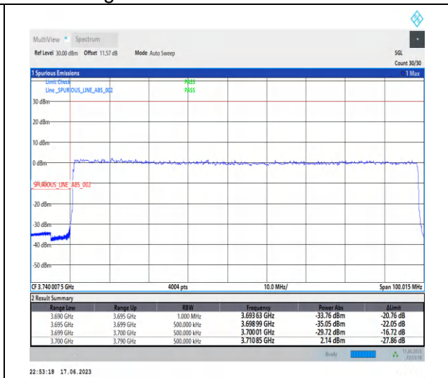
1-N77-3700-3980-PC3-30-90-L-3-DFT-PI2BPSK-Outer_Full-243@0-Ant2-1--PASS-see graph
