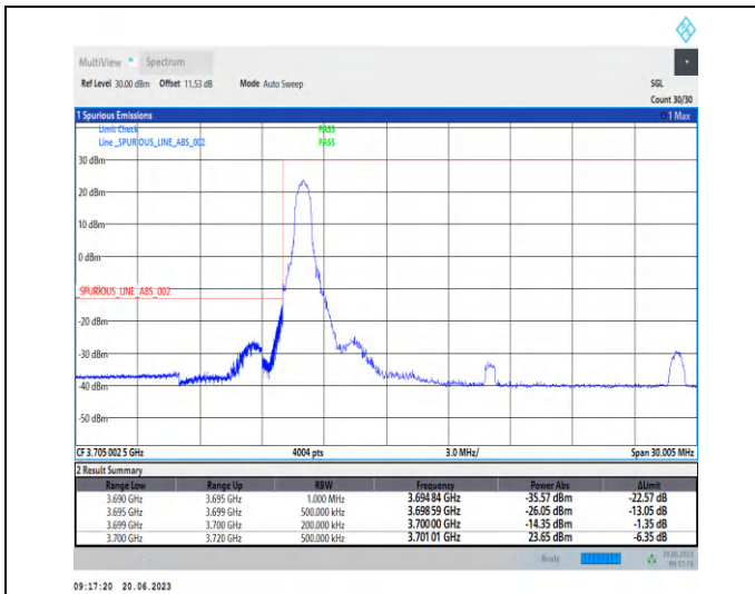
1-N77-3700-3980-PC2-30-20-L-1-CP-QPSK-Edge_1R B_Left-1@0-Ant2-1--PASS-see graph
