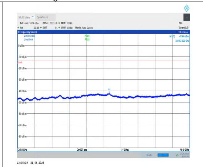
1-N77-3700-3980-PC2-30-100-M-1-NS_01-DFT-QP SK-Edge_1RB_Left-1@0-26000-40000-Ant2-33452. 90--42.00--13-PASS
