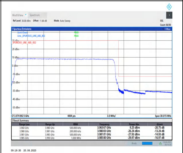
1-N77-3700-3980-PC2-30-20-H-3-CP-QPSK-Outer _Full-51@0-Ant2-1--PASS-see graph
