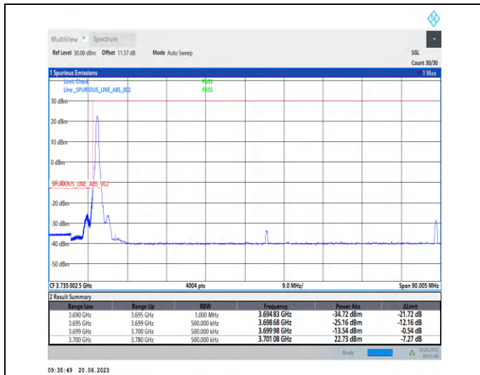
1-N77-3700-3980-PC2-30-80-L-1-CP-QPSK-Edge_1R B_Left-1@0-Ant2-1--PASS-see graph
