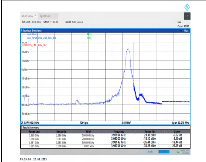
1-N77-3700-3980-PC2-30-20-H-2-CP-QPSK-Edge_1R B_Right-1@50-Ant2-1--PASS-see graph
