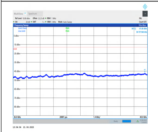
1-N77-3700-3980-PC2-30-100-L-1-NS_01-DFT-QPS K-Edge_1RB_Left-1@0-26000-40000-Ant2-33436.8 0--41.69--13-PASS
