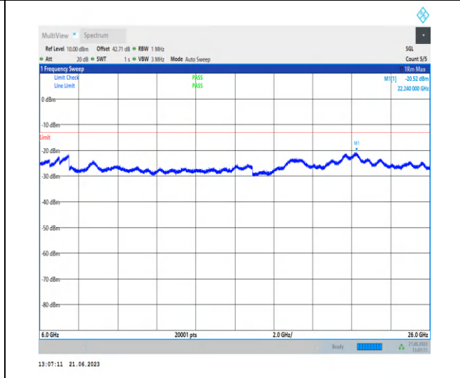
1-N77-3700-3980-PC2-30-100-H-1-NS_01-DFT-QPS K-Edge_1RB_Left-1@0-6000-26000-Ant2-22240.00-- 20.52--13-PASS
