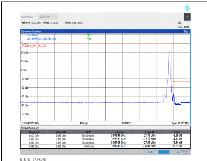
1-N77-3700-3980-PC3-30-80-H-2-DFT-PI2BPSK-Edge_1RB_Right-1@216-Ant2-1--PASS-see graph
