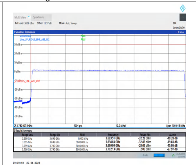
1-N77-3700-3980-PC2-30-90-L-3-CP-QPSK-Outer _Full-245@0-Ant2-1--PASS-see graph
