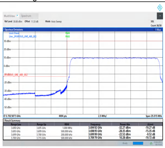
1-N77-3700-3980-PC2-30-15-L-3-CP-QPSK-Outer_Full-38@0-Ant2-1--PASS-see graph
