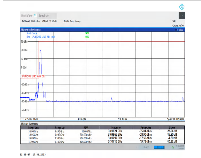
1-N77-3700-3980-PC3-30-80-L-4-CP-QPSK-Edge_1RB_Left-1@0-Ant2-1--PASS-see graph
