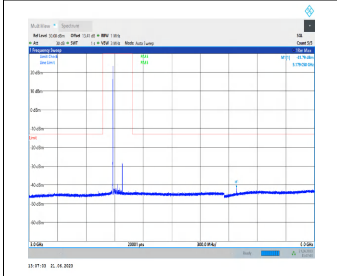
1-N77-3700-3980-PC2-30-100-H-1-NS_01-DFT-QP SK-Edge_1RB_Left-1@0-3000-6000-Ant2-5179.05-- 41.79--13-PASS
