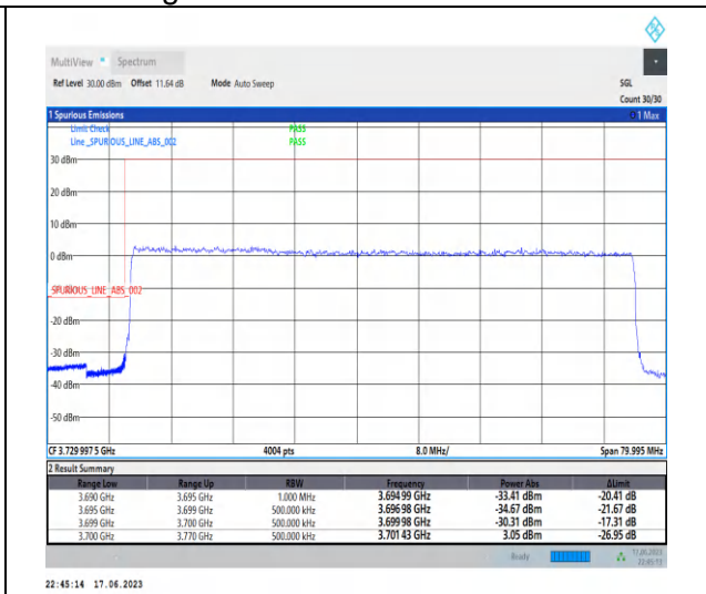
1-N77-3700-3980-PC3-30-70-L-3-DFT-PI2BPSK-Outer_Full-180@0-Ant2-1--PASS-see graph
