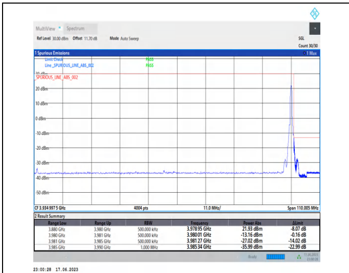
1-N77-3700-3980-PC3-30-100-H-2-DFT-PI2BPSK-Edge_1_RB_Right-1@272-Ant2-1--PASS-see graph
