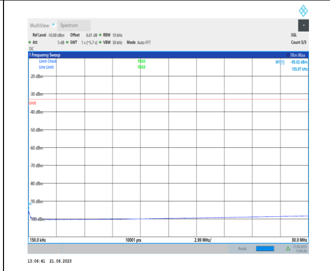
1-N77-3700-3980-PC2-30-100-H-1-NS_01-DFT-QPS K-Edge_1RB_Left-1@0-0.15-30-Ant2-0.16--95.02--3 3-PASS
