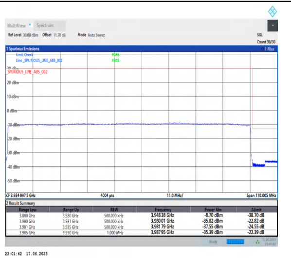
1-N77-3700-3980-PC3-30-100-H-6-CP-QPSK-Outer_Full-273@0-Ant2-1--PASS-see graph
