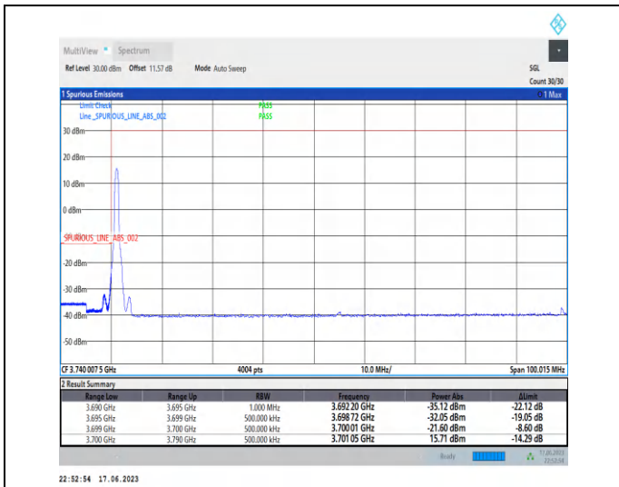
1-N77-3700-3980-PC3-30-90-L-1-DFT-PI2BPSK-Edge_1RB_Left-1@0-Ant2-1--PASS-see graph
