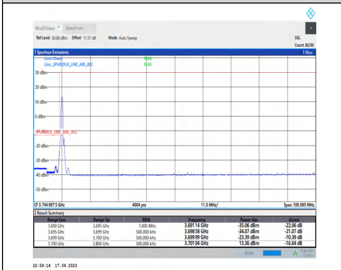
1-N77-3700-3980-PC3-30-100-L-4-CP-QPSK-Edge_1_RB_Left-1@0-Ant2-1--PASS-see graph
