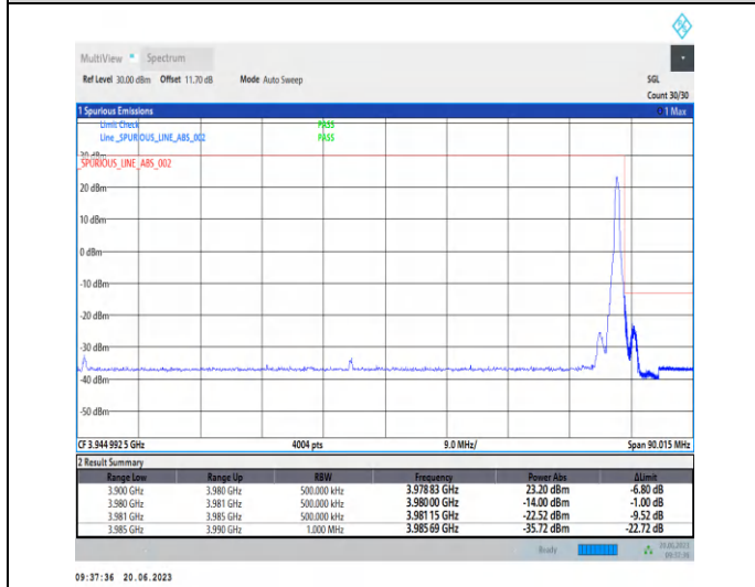
1-N77-3700-3980-PC2-30-80-H-2-CP-QPSK-Edge_1R B_Right-1@216-Ant2-1--PASS-see graph
