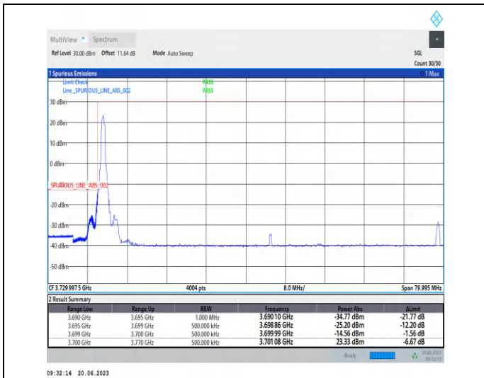
1-N77-3700-3980-PC2-30-70-L-1-CP-QPSK-Edge_1R B_Left-1@0-Ant2-1--PASS-see graph
