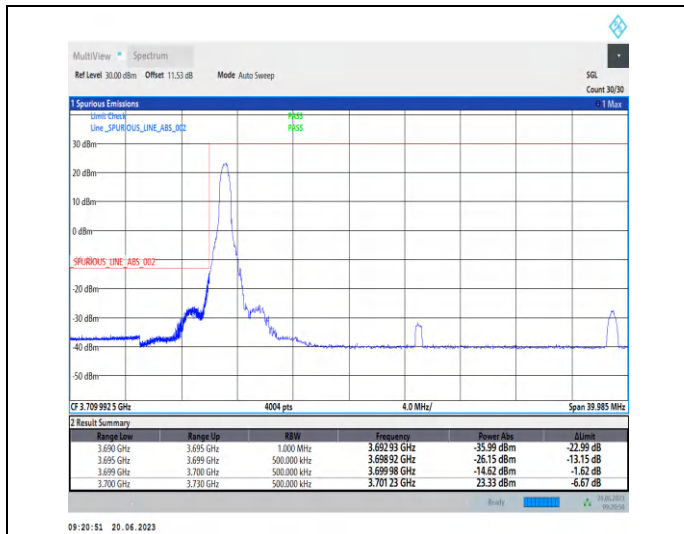
1-N77-3700-3980-PC2-30-30-L-1-CP-QPSK-Edge_1R B_Left-1@0-Ant2-1--PASS-see graph
