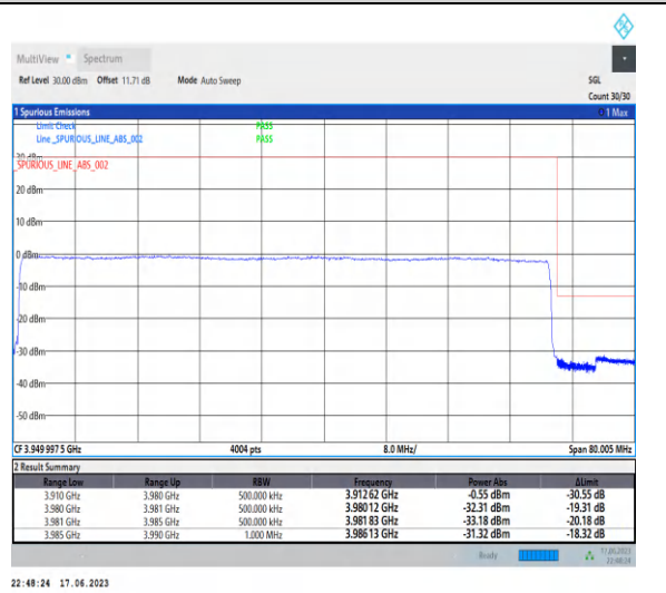
1-N77-3700-3980-PC3-30-70-H-6-CP-QPSK-Outer_Full-189@0-Ant2-1--PASS-see graph
