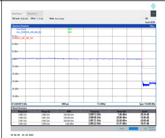
1-N77-3700-3980-PC2-30-100-H-3-CP-QPSK-Out er_Full-273@0-Ant2-1--PASS-see graph
