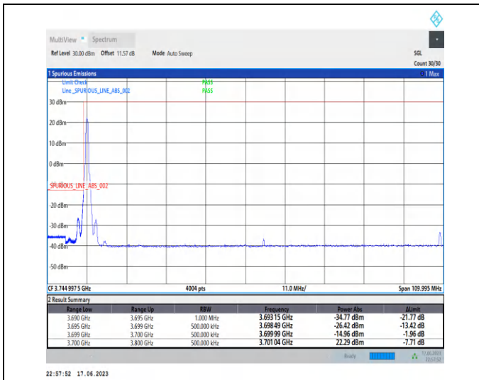
1-N77-3700-3980-PC3-30-100-L-1-DFT-PI2BPSK-Edge_1_RB_Left-1@0-Ant2-1--PASS-see graph
