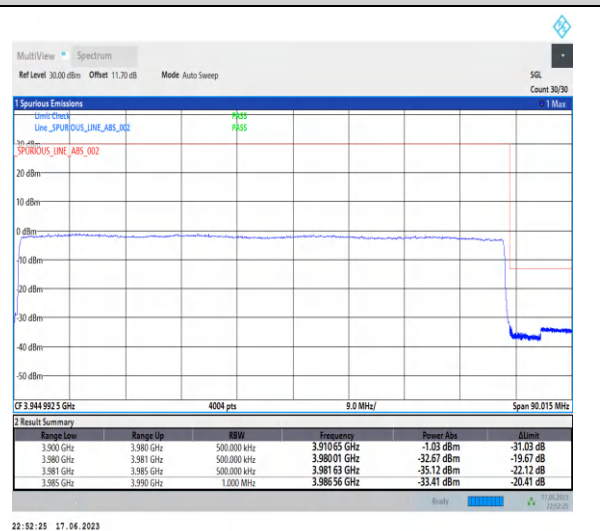
1-N77-3700-3980-PC3-30-80-H-6-CP-QPSK-Outer_Full-217@0-Ant2-1--PASS-see graph
