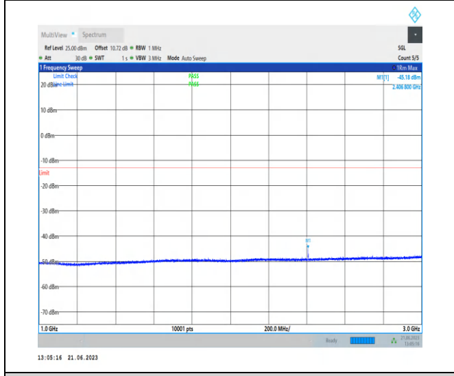
1-N77-3700-3980-PC2-30-100-M-1-NS_01-DFT-QP SK-Edge_1RB_Left-1@0-1000-3000-Ant2-2406.80-- 45.18--13-PASS
