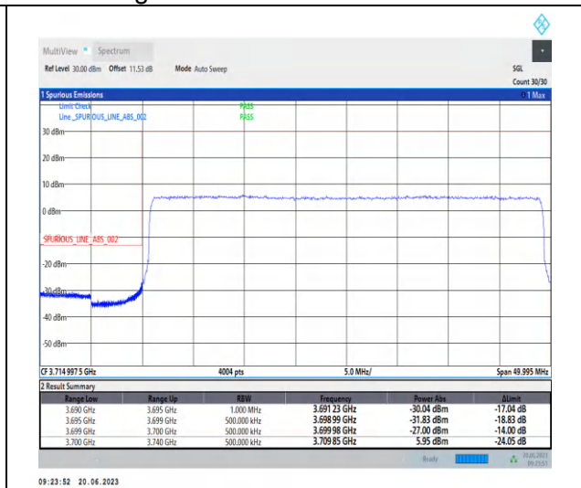
1-N77-3700-3980-PC2-30-40-L-3-CP-QPSK-Outer _Full-106@0-Ant2-1--PASS-see graph
