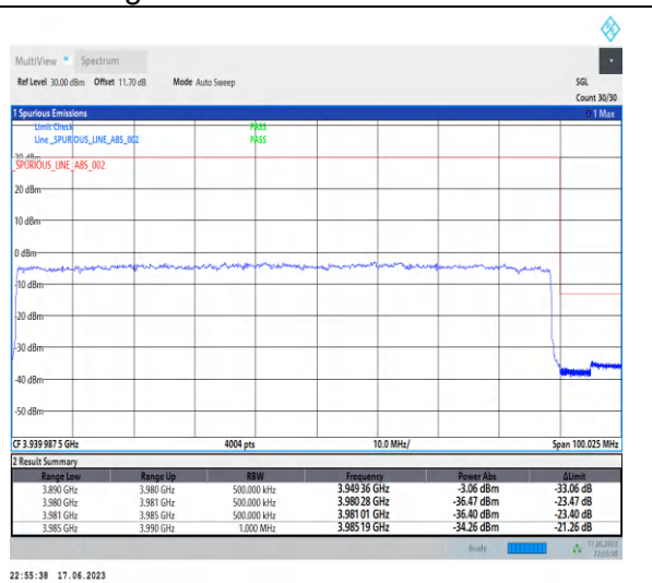
1-N77-3700-3980-PC3-30-90-H-3-DFT-PI2BPSK-Outer_Full-243@0-Ant2-1--PASS-see graph
