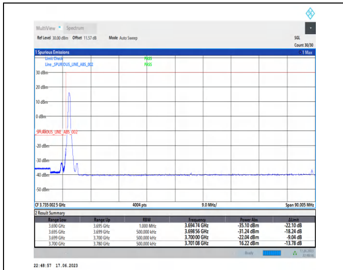
1-N77-3700-3980-PC3-30-80-L-1-DFT-PI2BPSK-Edge_1RB_Left-1@0-Ant2-1--PASS-see graph
