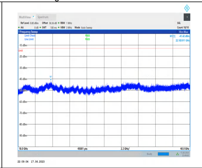
1-N77-3700-3980-PC3-30-100-L-1-N/A-DFT-PI2BPS K-Inner_1RB_Left-1@1-18000-40000-Ant2-22183.91 --41.42--13-PASS
