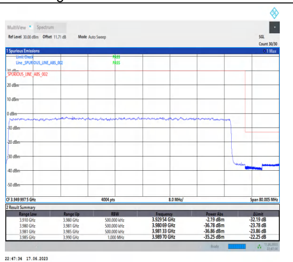
1-N77-3700-3980-PC3-30-70-H-3-DFT-PI2BPSK-Outer_Full-180@0-Ant2-1--PASS-see graph
