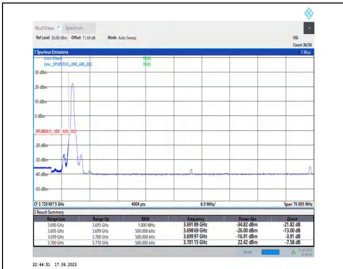
1-N77-3700-3980-PC3-30-70-L-1-DFT-PI2BPSK-Edge_1RB_Left-1@0-Ant2-1--PASS-see graph
