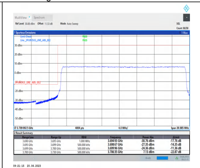
1-N77-3700-3980-PC2-30-30-L-3-CP-QPSK-Outer _Full-78@0-Ant2-1--PASS-see graph
