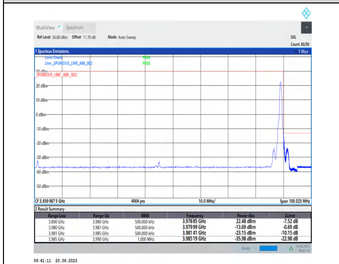
1-N77-3700-3980-PC2-30-90-H-2-CP-QPSK-Edge_1R B_Right-1@244-Ant2-1--PASS-see graph
