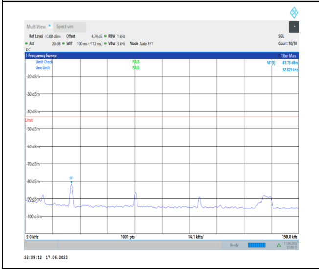
1-N77-3700-3980-PC3-30-100-M-1-N/A-DFT-PI2BP SK-Inner_1RB_Left-1@1-0.009-0.15-Ant2-0.03--81. 73--43-PASS
