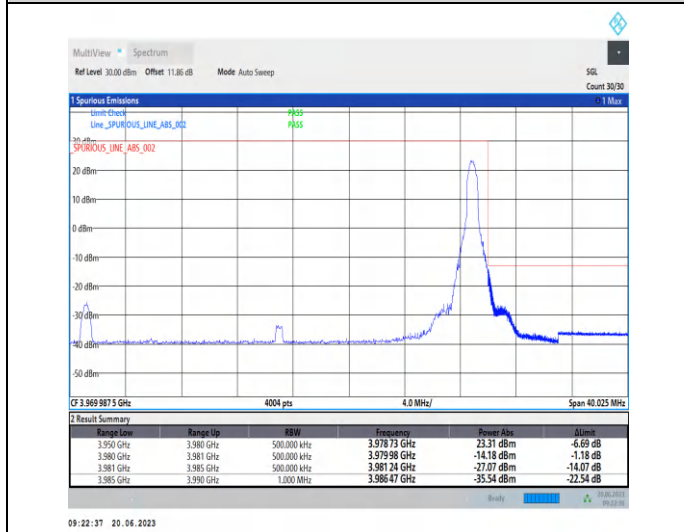
1-N77-3700-3980-PC2-30-30-H-2-CP-QPSK-Edge_1R B_Right-1@77-Ant2-1--PASS-see graph
