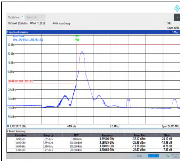
1-N77-3700-3980-PC2-30-15-L-1-CP-QPSK-Edge_1R_B_Left-1@0-Ant2-1--PASS-see graph
