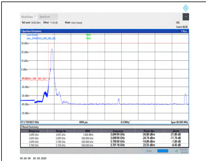
1-N77-3700-3980-PC2-30-50-L-1-CP-QPSK-Edge_1R B_Left-1@0-Ant2-1--PASS-see graph
