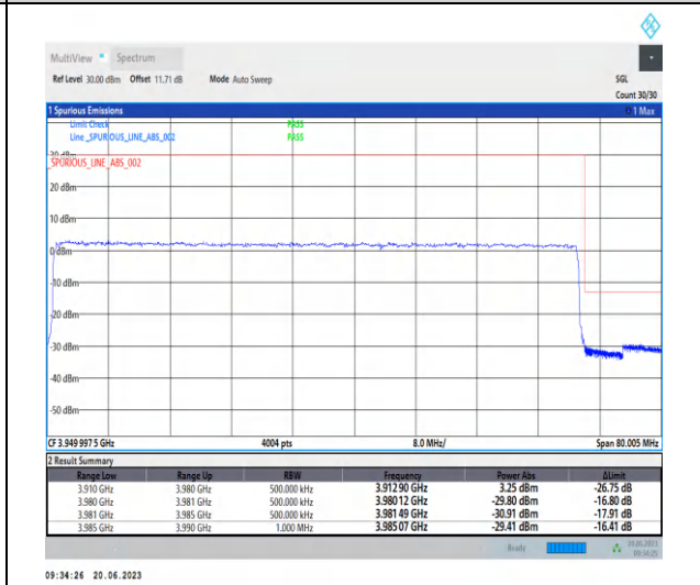
1-N77-3700-3980-PC2-30-70-H-3-CP-QPSK-Outer _Full-189@0-Ant2-1--PASS-see graph
