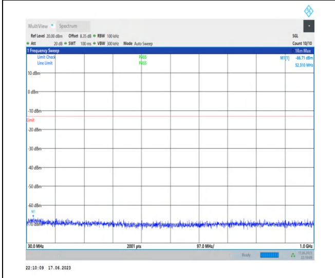
1-N77-3700-3980-PC3-30-100-H-1-N/A-DFT-PI2BP SK-Inner_1RB_Left-1@1-30-1000-Ant2-52.31--66.7 1--13-PASS
