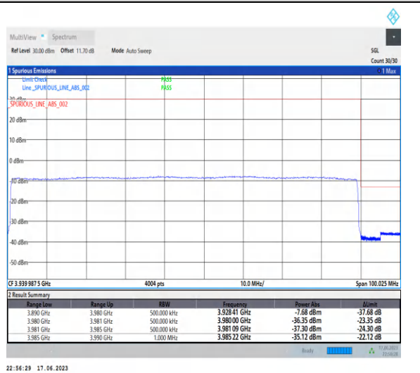
1-N77-3700-3980-PC3-30-90-H-6-CP-QPSK-Outer_Full-245@0-Ant2-1--PASS-see graph
