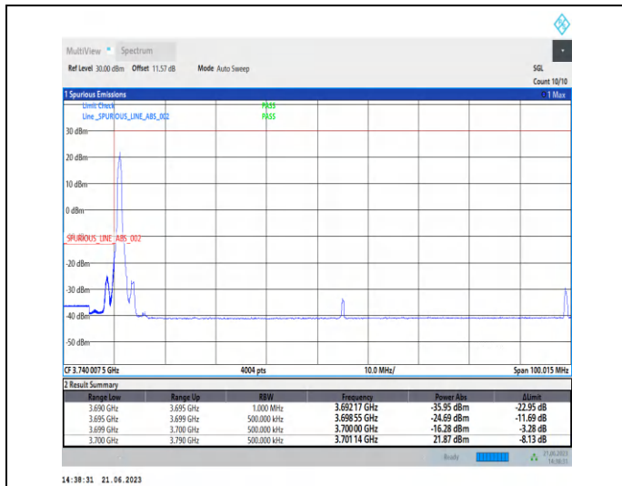
1-N77-3700-3980-PC2-30-90-L-1-CP-QPSK-Edge_1R B_Left-1@0-Ant2-1--PASS-see graph
