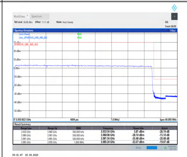
1-N77-3700-3980-PC2-30-60-H-3-CP-QPSK-Outer _Full-162@0-Ant2-1--PASS-see graph
