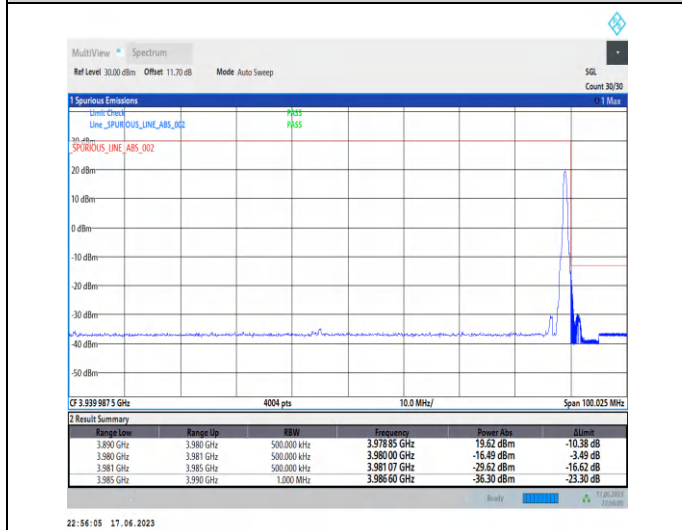
1-N77-3700-3980-PC3-30-90-H-5-CP-QPSK-Edge_1RB_Right-1@244-Ant2-1--PASS-see graph
