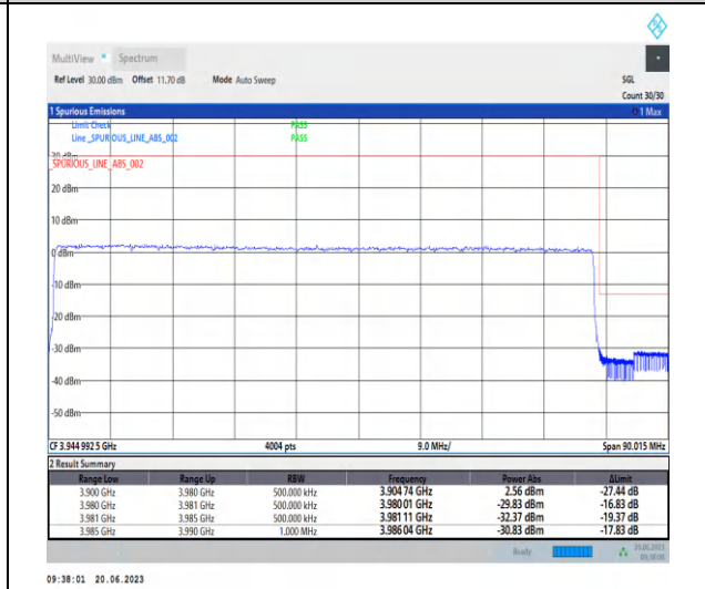
1-N77-3700-3980-PC2-30-80-H-3-CP-QPSK-Outer _Full-217@0-Ant2-1--PASS-see graph
