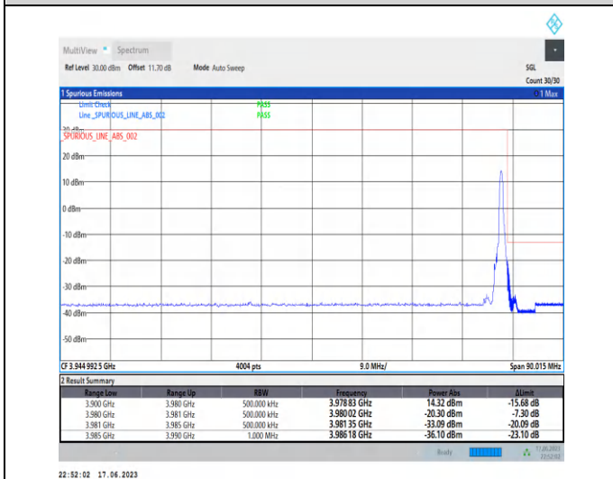
1-N77-3700-3980-PC3-30-80-H-5-CP-QPSK-Edge_1RB_Right-1@216-Ant2-1--PASS-see graph
