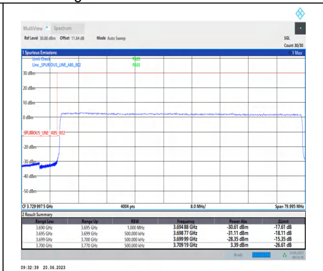
1-N77-3700-3980-PC2-30-70-L-3-CP-QPSK-Outer _Full-189@0-Ant2-1--PASS-see graph
