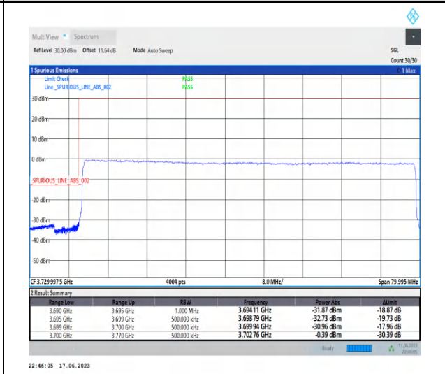
1-N77-3700-3980-PC3-30-70-L-6-CP-QPSK-Outer_Full-189@0-Ant2-1--PASS-see graph
