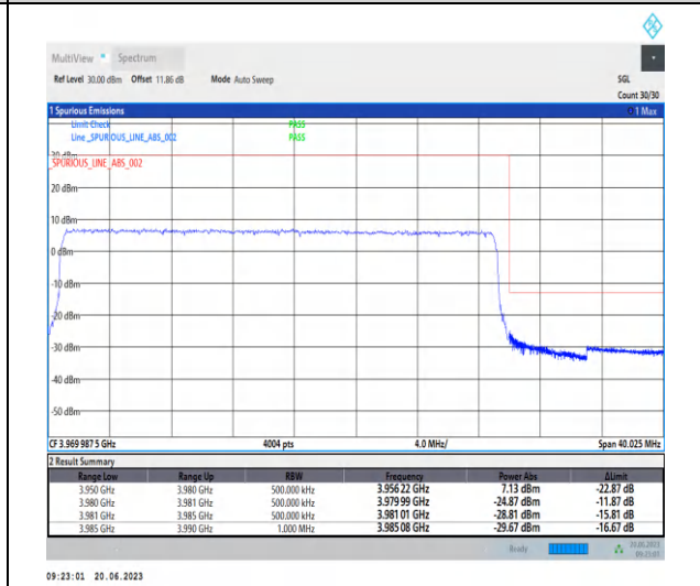
1-N77-3700-3980-PC2-30-30-H-3-CP-QPSK-Outer _Full-78@0-Ant2-1--PASS-see graph
