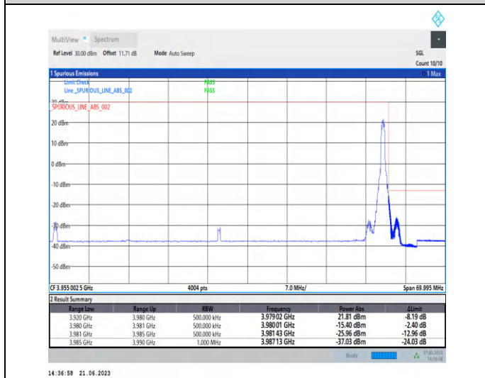
1-N77-3700-3980-PC2-30-60-H-2-CP-QPSK-Edge_1R B_Right-1@161-Ant2-1--PASS-see graph
