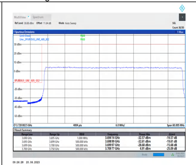
1-N77-3700-3980-PC2-30-50-L-3-CP-QPSK-Outer _Full-133@0-Ant2-1--PASS-see graph
