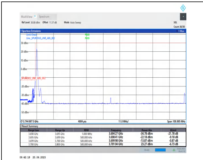
1-N77-3700-3980-PC2-30-100-L-1-CP-QPSK-Edge_1 RB_Left-1@0-Ant2-1--PASS-see graph
