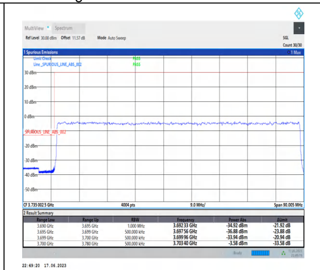
1-N77-3700-3980-PC3-30-80-L-3-DFT-PI2BPSK-Outer_Full-216@0-Ant2-1--PASS-see graph
