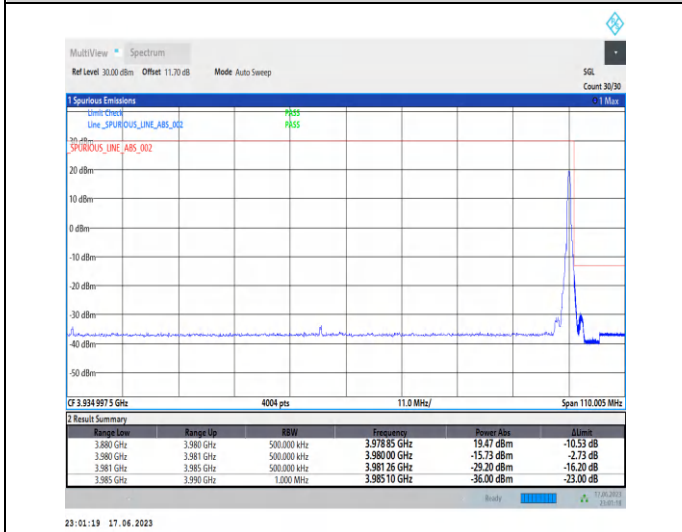
1-N77-3700-3980-PC3-30-100-H-5-CP-QPSK-Edge_1_RB_Right-1@272-Ant2-1--PASS-see graph
