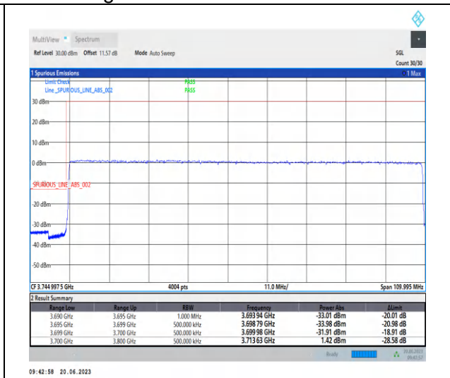
1-N77-3700-3980-PC2-30-100-L-3-CP-QPSK-Out er_Full-273@0-Ant2-1--PASS-see graph
