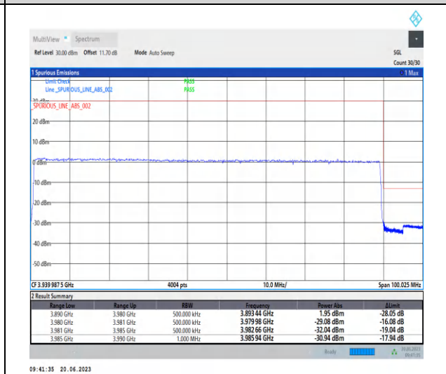
1-N77-3700-3980-PC2-30-90-H-3-CP-QPSK-Outer _Full-245@0-Ant2-1--PASS-see graph
