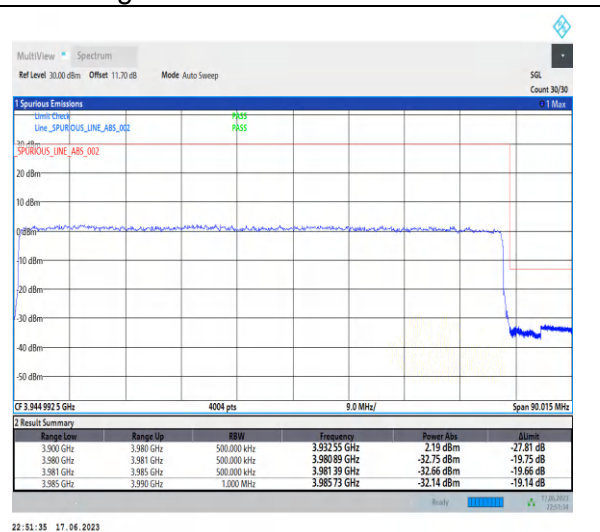
1-N77-3700-3980-PC3-30-80-H-3-DFT-PI2BPSK-Outer_Full-216@0-Ant2-1--PASS-see graph
