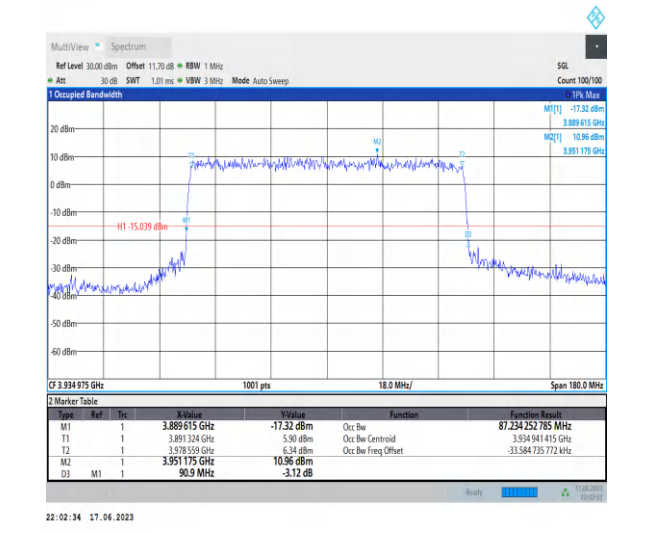
1-N77-3700-3980-PC3-30-90-H-7-CP-16QAM-Outer Full-245@0-Ant2-87.234-90.900-≤90-PASS
