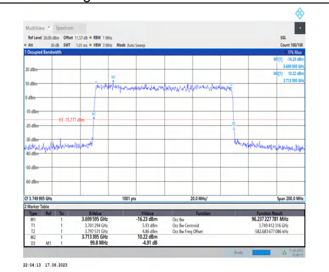
1-N77-3700-3980-PC3-30-100-L-4-DFT-64QAM-Out er_Full-270@0-Ant2-96.237-99.800-≤100-PASS
