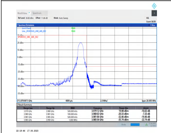
1-N77-3700-3980-PC3-30-10-H-5-CP-QPSK-Edge_1RB_Right-1@23-Ant2-1--PASS-see graph
