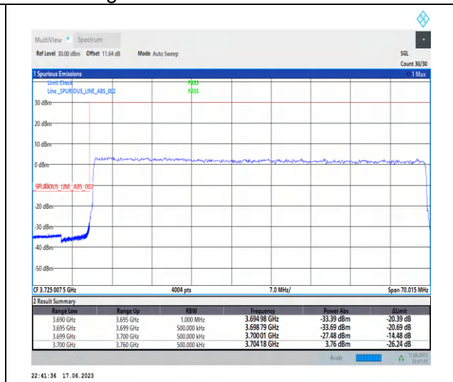
1-N77-3700-3980-PC3-30-60-L-3-DFT-PI2BPSK-Outer_Full-162@0-Ant2-1--PASS-see graph
