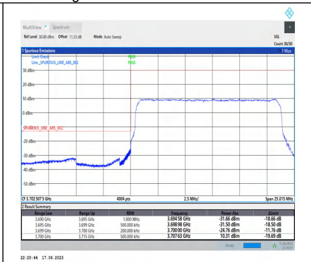
1-N77-3700-3980-PC3-30-15-L-3-DFT-PI2BPSK-Outer_Full-36@0-Ant2-1--PASS-see graph
