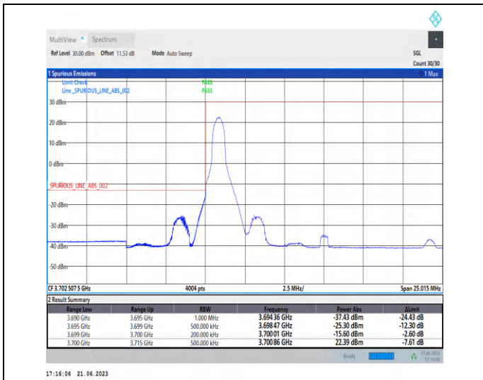
1-N77-3700-3980-PC3-30-15-L-1-DFT-PI2BPSK-Edge_1RB_Left-1@0-Ant2-1--PASS-see graph
