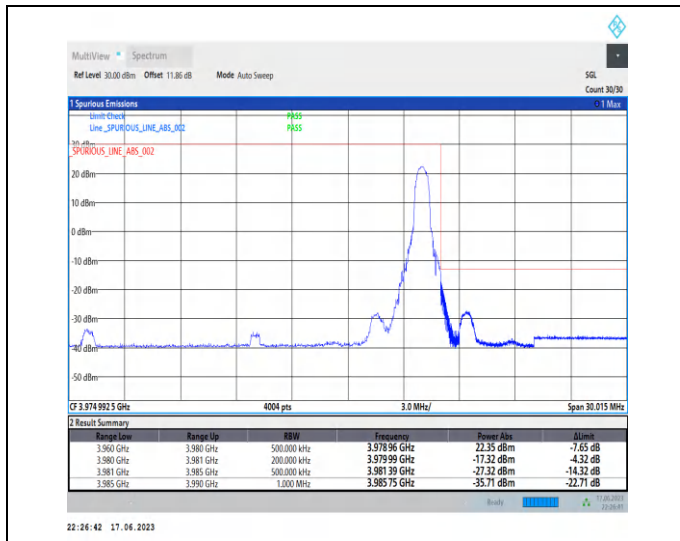
1-N77-3700-3980-PC3-30-20-H-2-DFT-PI2BPSK-Edge_1RB_Right-1@50-Ant2-1--PASS-see graph
