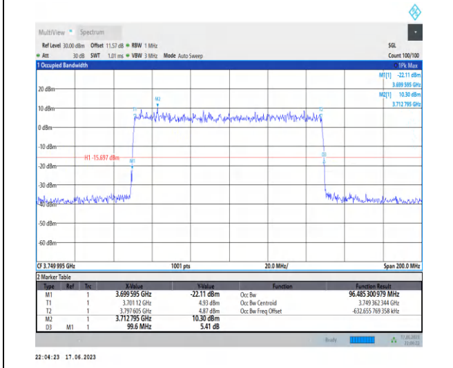
1-N77-3700-3980-PC3-30-100-L-5-DFT-256QAM-Out er_Full-270@0-Ant2-96.485-99.600-≤100-PASS
