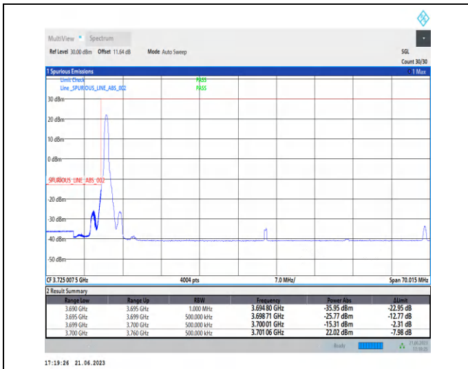
1-N77-3700-3980-PC3-30-60-L-1-DFT-PI2BPSK-Edge_1RB_Left-1@0-Ant2-1--PASS-see graph
