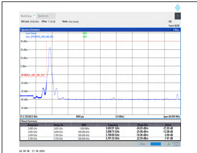
1-N77-3700-3980-PC3-30-50-L-1-DFT-PI2BPSK-Edge_1RB_Left-1@0-Ant2-1--PASS-see graph
