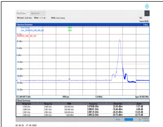
1-N77-3700-3980-PC3-30-40-H-2-DFT-PI2BPSK-Edge_1RB_Right-1@105-Ant2-1--PASS-see graph
