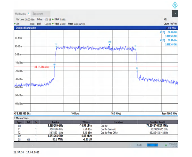
1-N77-3700-3980-PC3-30-80-H-6-CP-QPSK-Out er_Full-217@0-Ant2-77.265-80.800-≤80-PASS
