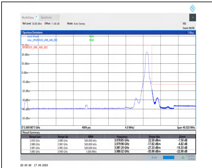
1-N77-3700-3980-PC3-30-30-H-2-DFT-PI2BPSK-Edge_1RB_Right-1@77-Ant2-1--PASS-see graph
