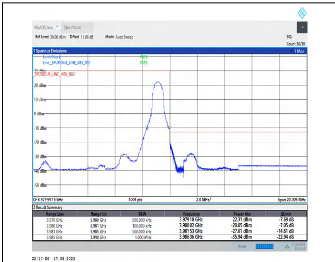
1-N77-3700-3980-PC3-30-10-H-2-DFT-PI2BPSK-Edge_1RB_Right-1@23-Ant2-1--PASS-see graph
