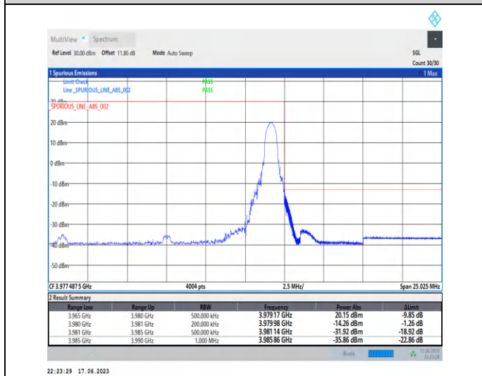
1-N77-3700-3980-PC3-30-15-H-5-CP-QPSK-Edge_1RB_Right-1@37-Ant2-1--PASS-see graph
