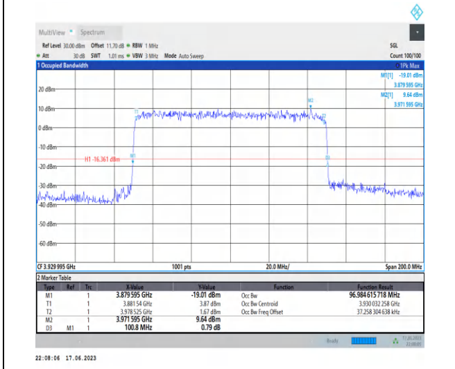
1-N77-3700-3980-PC3-30-100-H-7-CP-16QAM-Outer_Full-273@0-Ant2-96.985-100.800-≤100-PASS
