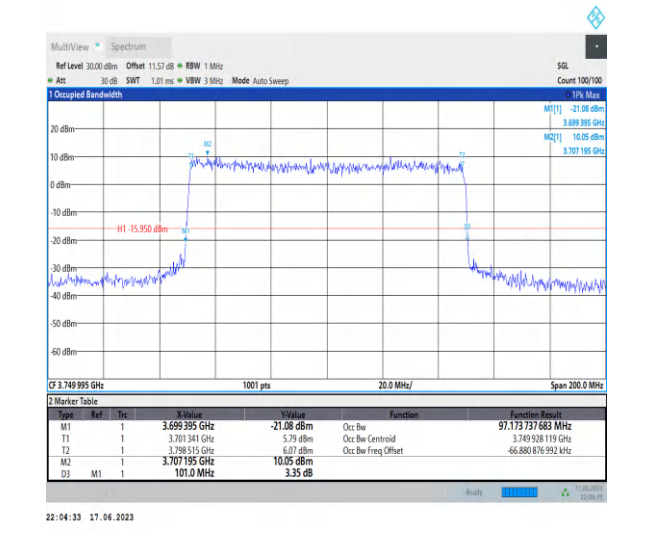
1-N77-3700-3980-PC3-30-100-L-6-CP-QPSK-Outer Full-273@0-Ant2-97.174-101.000-≤100-PASS
