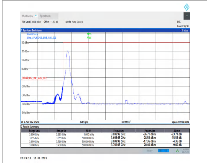
1-N77-3700-3980-PC3-30-30-L-4-CP-QPSK-Edge_1RB_Left-1@0-Ant2-1--PASS-see graph
