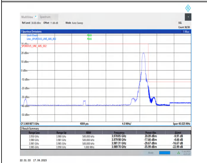
1-N77-3700-3980-PC3-30-30-H-5-CP-QPSK-Edge_1RB_Right-1@77-Ant2-1--PASS-see graph
