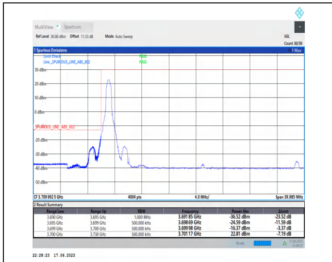
1-N77-3700-3980-PC3-30-30-L-1-DFT-PI2BPSK-Edge_1RB_Left-1@0-Ant2-1--PASS-see graph
