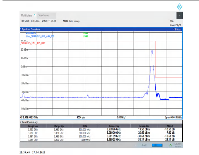
1-N77-3700-3980-PC3-30-50-H-5-CP-QPSK-Edge_1RB_Right-1@132-Ant2-1--PASS-see graph
