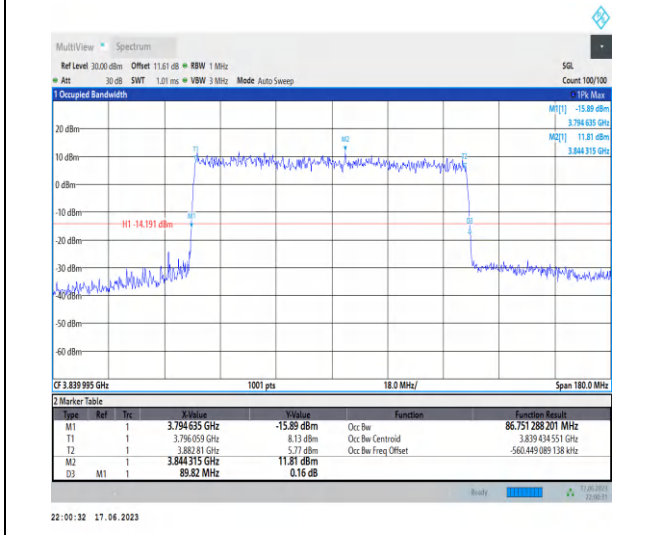
1-N77-3700-3980-PC3-30-90-M-3-DFT-16QAM-Outer_Full-243@0-Ant2-86.751-89.820-≤90-PASS
