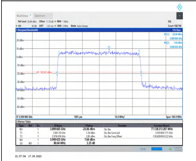
1-N77-3700-3980-PC3-30-80-H-9-CP-256QAM-Outer_Full-217@0-Ant2-77.128-80.640-≤80-PASS
