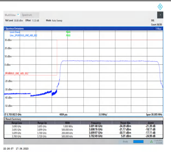
1-N77-3700-3980-PC3-30-20-L-6-CP-QPSK-Outer_Full-51@0-Ant2-1--PASS-see graph
