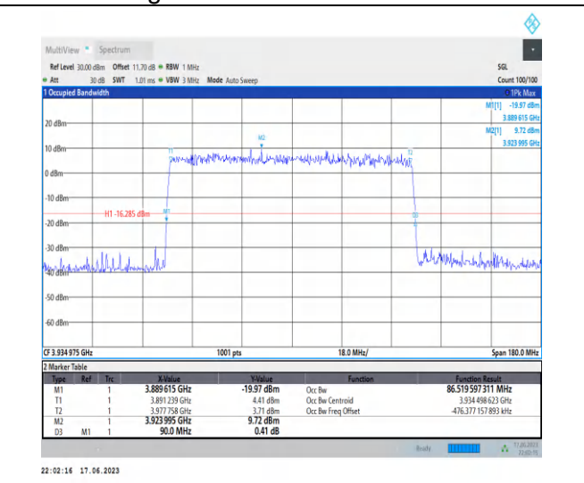
1-N77-3700-3980-PC3-30-90-H-5-DFT-256QAM-Out er_Full-243@0-Ant2-86.52-90.000-≤90-PASS
