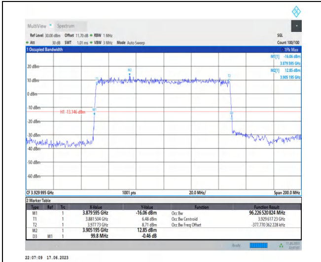
1-N77-3700-3980-PC3-30-100-H-1-DFT-PI2BPSK-Outer_Full-270@0-Ant2-96.227-99.800-≤100-PASS
