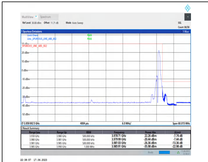
1-N77-3700-3980-PC3-30-50-H-2-DFT-PI2BPSK-Edge_1RB_Right-1@132-Ant2-1--PASS-see graph
