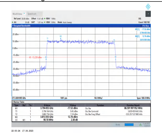
1-N77-3700-3980-PC3-30-90-M-2-DFT-QPSK-Outer_Full-243@0-Ant2-86.592-90.180-≤90-PASS
