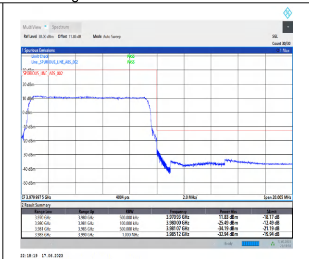
1-N77-3700-3980-PC3-30-10-H-3-DFT-PI2BPSK-Outer_Full-24@0-Ant2-1--PASS-see graph
