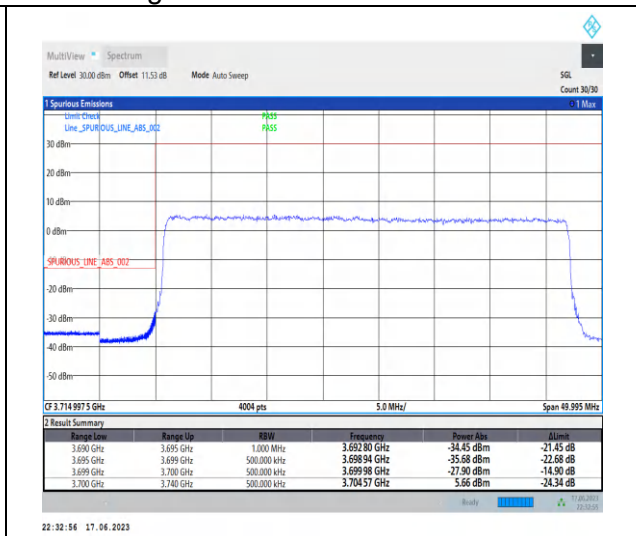
1-N77-3700-3980-PC3-30-40-L-3-DFT-PI2BPSK-Outer_Full-100@0-Ant2-1--PASS-see graph
