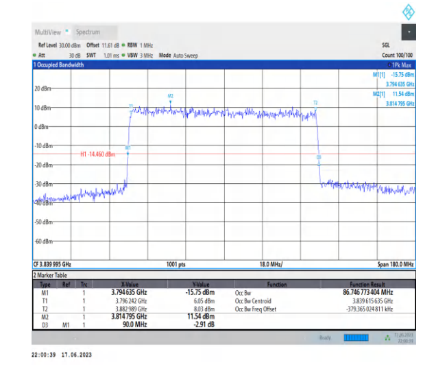
1-N77-3700-3980-PC3-30-90-M-4-DFT-64QAM-Outer_Full-243@0-Ant2-86.747-90.000-≤90-PASS
