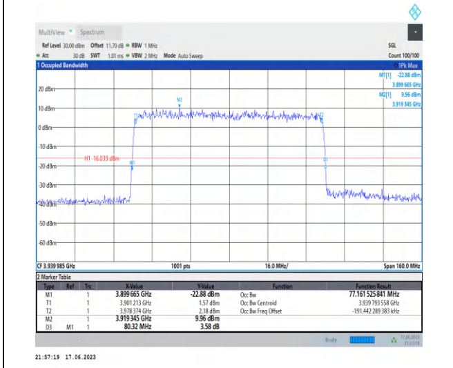
1-N77-3700-3980-PC3-30-80-H-5-DFT-256QAM-Out er_Full-216@0-Ant2-77.162-80.320-≤80-PASS
