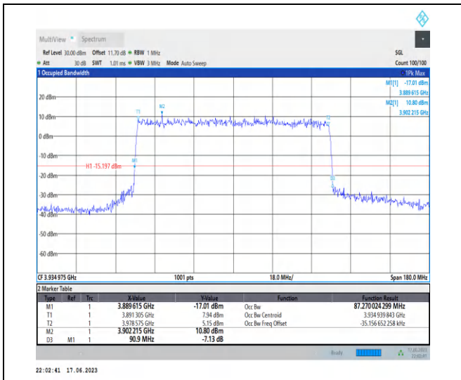
1-N77-3700-3980-PC3-30-90-H-8-CP-64QAM-Outer_Full-245@0-Ant2-87.27-90.900-≤90-PASS
