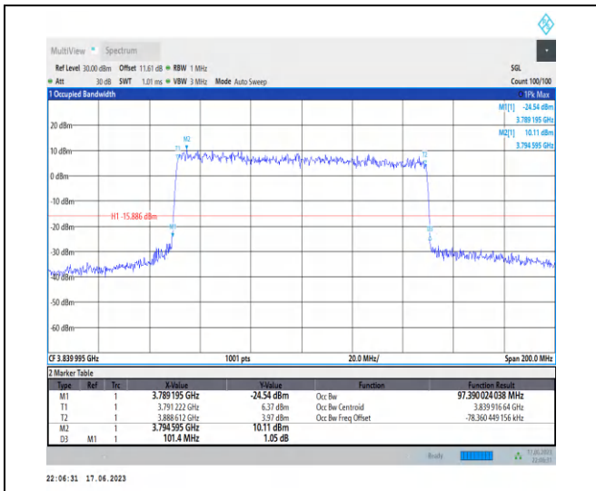
1-N77-3700-3980-PC3-30-100-M-6-CP-QPSK-Outer_Full-273@0-Ant2-97.39-101.400-≤100-PASS
