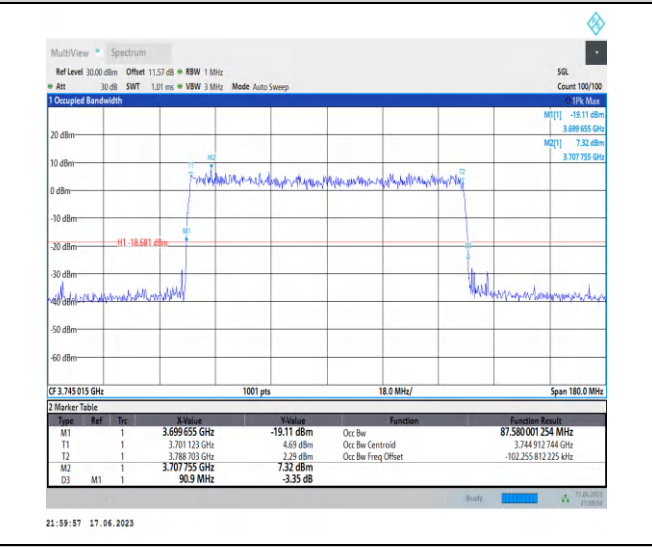
1-N77-3700-3980-PC3-30-90-L-9-CP-256QAM-Outer_Full-245@0-Ant2-87.58-90.900-≤90-PASS
