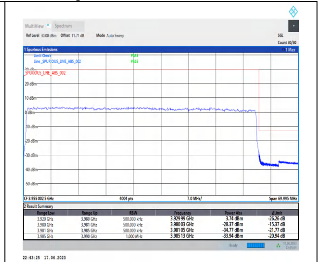
1-N77-3700-3980-PC3-30-60-H-3-DFT-PI2BPSK-Outer_Full-162@0-Ant2-1--PASS-see graph
