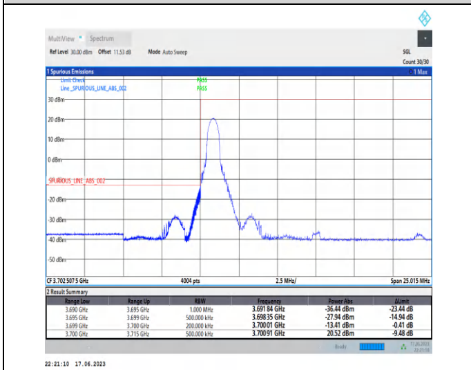
1-N77-3700-3980-PC3-30-15-L-4-CP-QPSK-Edge_1RB_Left-1@0-Ant2-1--PASS-see graph
