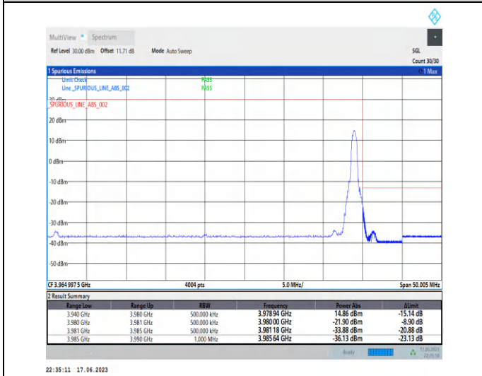
1-N77-3700-3980-PC3-30-40-H-5-CP-QPSK-Edge_1RB_Right-1@105-Ant2-1--PASS-see graph
