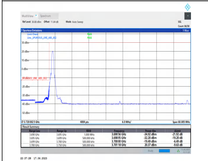
1-N77-3700-3980-PC3-30-50-L-4-CP-QPSK-Edge_1RB_Left-1@0-Ant2-1--PASS-see graph
