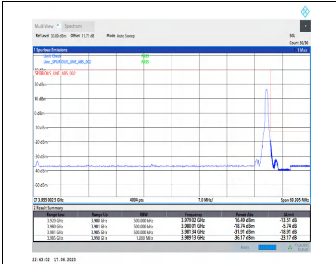
1-N77-3700-3980-PC3-30-60-H-2-DFT-PI2BPSK-Edge_1RB_Right-1@161-Ant2-1--PASS-see graph
