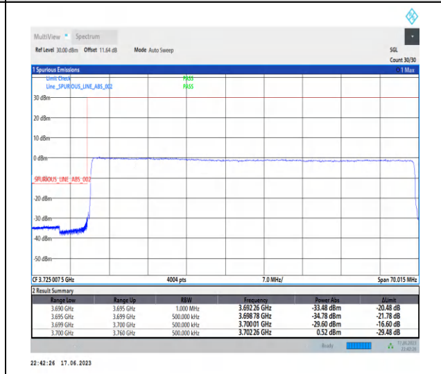
1-N77-3700-3980-PC3-30-60-L-6-CP-QPSK-Outer_Full-162@0-Ant2-1--PASS-see graph
