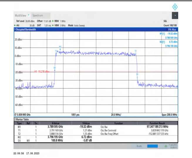
1-N77-3700-3980-PC3-30-100-M-9-CP-256QAM-Outer_Full-273@0-Ant2-97.347-100.800-≤100-PASS
