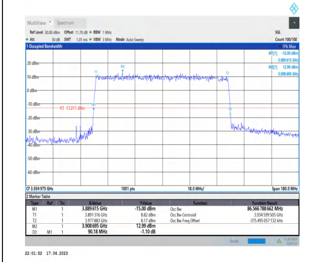
1-N77-3700-3980-PC3-30-90-H-2-DFT-QPSK-Outer _Full-243@0-Ant2-86.567-90.180-≤90-PASS
