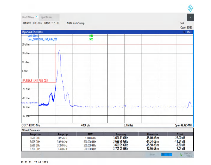
1-N77-3700-3980-PC3-30-40-L-1-DFT-PI2BPSK-Edge_1RB_Left-1@0-Ant2-1--PASS-see graph
