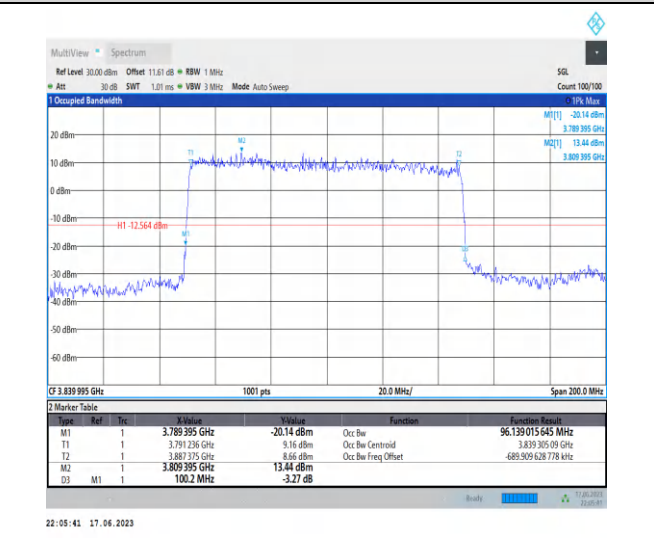
1-N77-3700-3980-PC3-30-100-M-1-DFT-PI2BPSK-Outer_Full-270@0-Ant2-96.139-100.200-≤100-PASS
