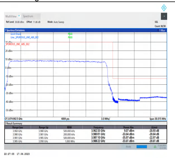
1-N77-3700-3980-PC3-30-20-H-3-DFT-PI2BPSK-Outer_Full-50@0-Ant2-1--PASS-see graph
