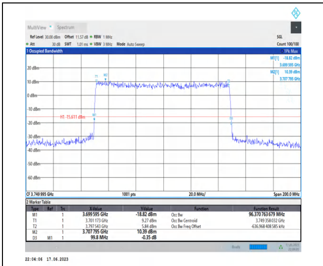
1-N77-3700-3980-PC3-30-100-L-3-DFT-16QAM-Out er_Full-270@0-Ant2-96.371-99.800-≤100-PASS
