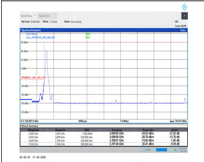
1-N77-3700-3980-PC3-30-60-L-4-CP-QPSK-Edge_1RB_Left-1@0-Ant2-1--PASS-see graph
