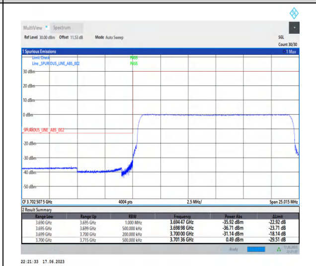
1-N77-3700-3980-PC3-30-15-L-6-CP-QPSK-Outer_Full-38@0-Ant2-1--PASS-see graph
