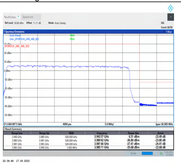
1-N77-3700-3980-PC3-30-40-H-3-DFT-PI2BPSK-Outer_Full-100@0-Ant2-1--PASS-see graph
