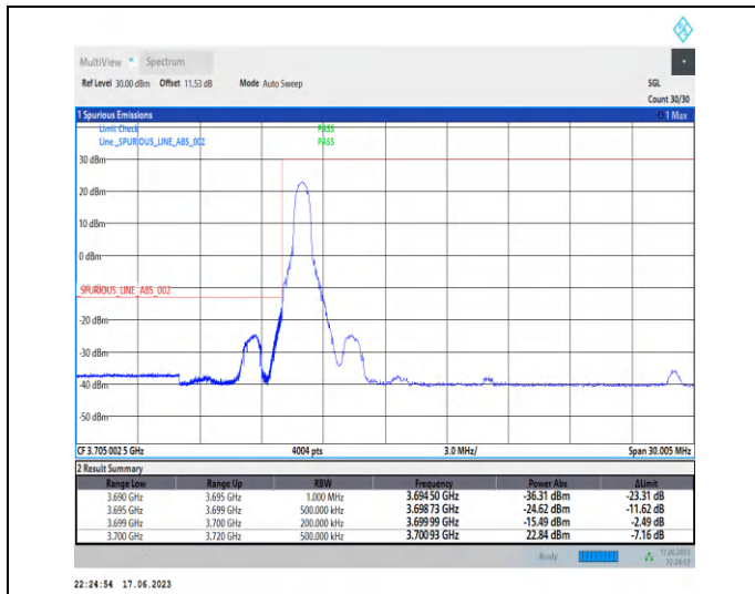
1-N77-3700-3980-PC3-30-20-L-1-DFT-PI2BPSK-Edge_1RB_Left-1@0-Ant2-1--PASS-see graph
