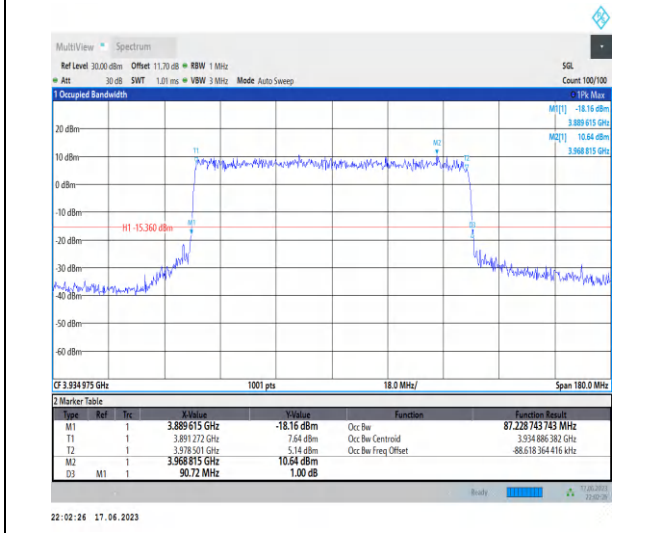
1-N77-3700-3980-PC3-30-90-H-6-CP-QPSK-Outer Full-245@0-Ant2-87.229-90.720-≤90-PASS
