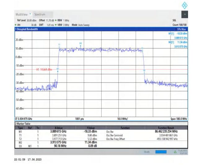
1-N77-3700-3980-PC3-30-90-H-3-DFT-16QAM-Outer _Full-243@0-Ant2-86.462-90.180-≤90-PASS
