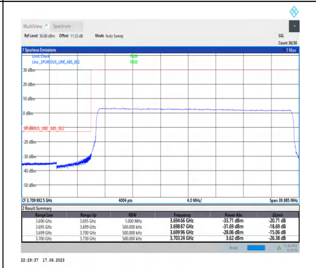
1-N77-3700-3980-PC3-30-30-L-6-CP-QPSK-Outer_Full-78@0-Ant2-1--PASS-see graph
