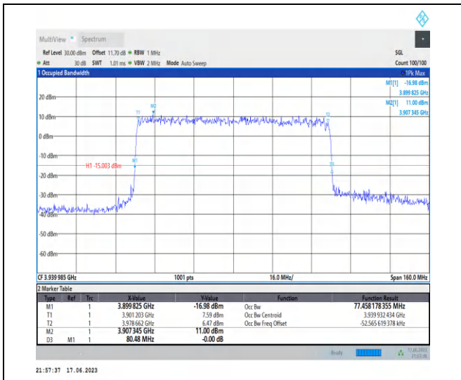
1-N77-3700-3980-PC3-30-80-H-7-CP-16QAM-Outer_Full-217@0-Ant2-77.458-80.480-≤80-PASS
