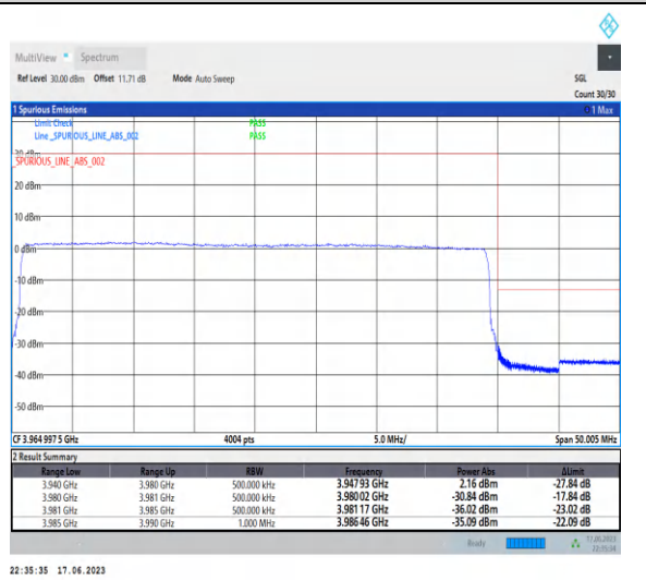
1-N77-3700-3980-PC3-30-40-H-6-CP-QPSK-Outer_Full-106@0-Ant2-1--PASS-see graph
