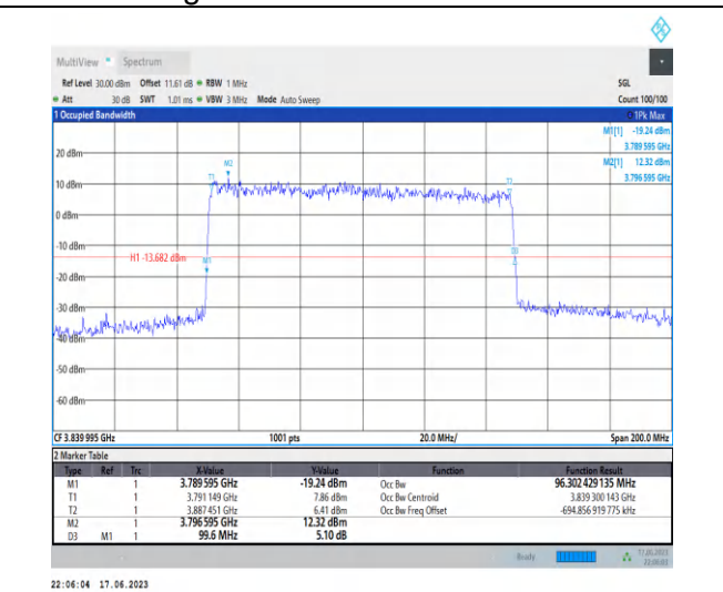
1-N77-3700-3980-PC3-30-100-M-3-DFT-16QAM-Out er_Full-270@0-Ant2-96.302-99.600-≤100-PASS
