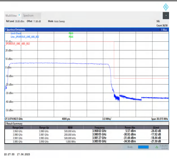
1-N77-3700-3980-PC3-30-20-H-6-CP-QPSK-Outer_Full-51@0-Ant2-1--PASS-see graph
