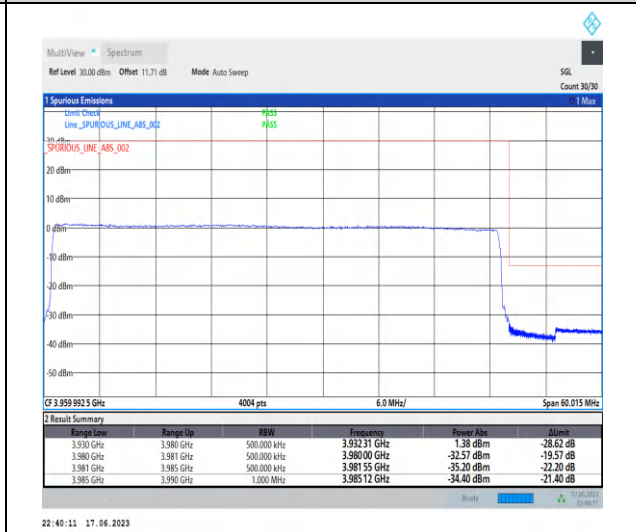
1-N77-3700-3980-PC3-30-50-H-6-CP-QPSK-Outer_Full-133@0-Ant2-1--PASS-see graph
