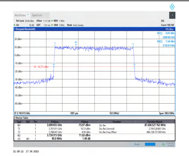
1-N77-3700-3980-PC3-30-90-L-1-DFT-PI2BPSK-Outer_Full-243@0-Ant2-87.037-90.000-≤90-PASS
