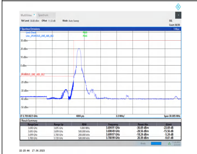
1-N77-3700-3980-PC3-30-20-L-4-CP-QPSK-Edge_1RB_Left-1@0-Ant2-1--PASS-see graph
