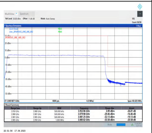
1-N77-3700-3980-PC3-30-30-H-6-CP-QPSK-Outer_Full-78@0-Ant2-1--PASS-see graph
