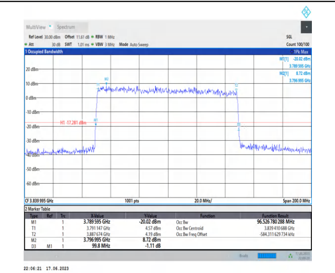
1-N77-3700-3980-PC3-30-100-M-5-DFT-256QAM-Out er_Full-270@0-Ant2-96.527-99.800-≤100-PASS
