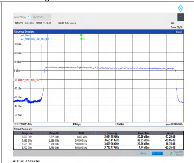
1-N77-3700-3980-PC3-30-50-L-3-DFT-PI2BPSK-Outer_Full-128@0-Ant2-1--PASS-see graph
