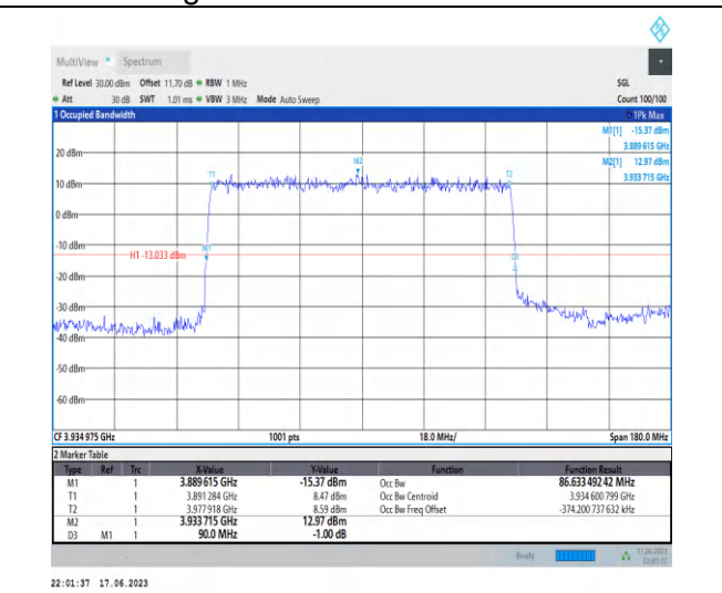
1-N77-3700-3980-PC3-30-90-H-1-DFT-PI2BPSK-Out er_Full-243@0-Ant2-86.633-90.000-≤90-PASS
