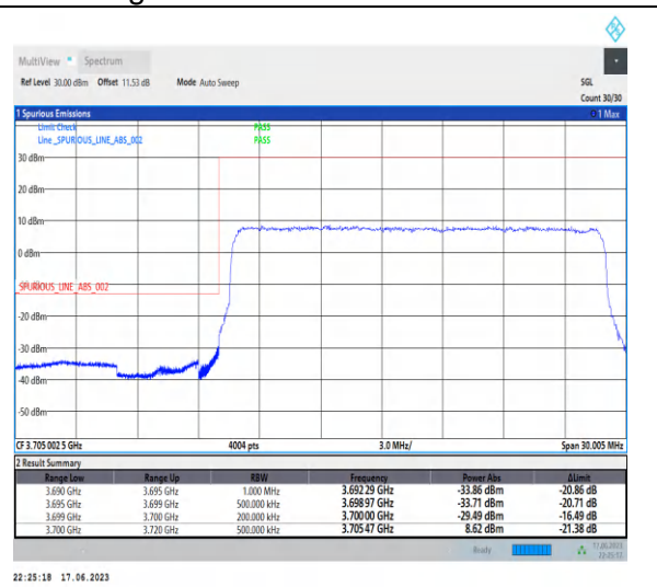
1-N77-3700-3980-PC3-30-20-L-3-DFT-PI2BPSK-Outer_Full-50@0-Ant2-1--PASS-see graph
