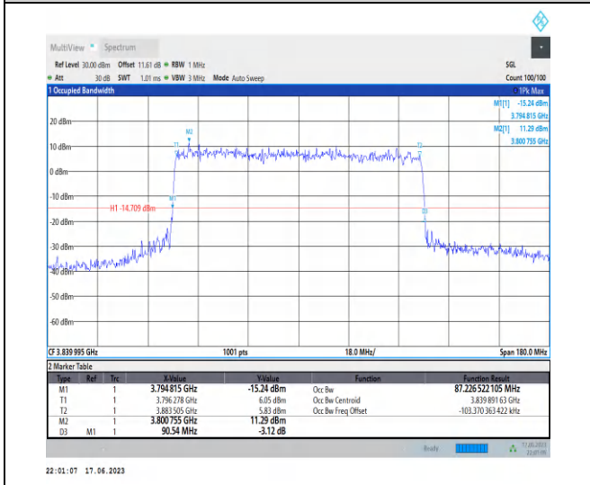
1-N77-3700-3980-PC3-30-90-M-7-CP-16QAM-Outer_Full-245@0-Ant2-87.227-90.540-≤90-PASS
