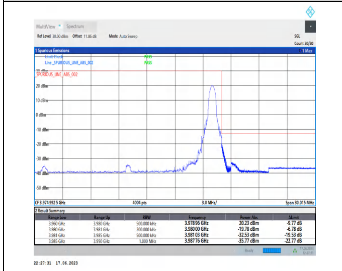
1-N77-3700-3980-PC3-30-20-H-5-CP-QPSK-Edge_1RB_Right-1@50-Ant2-1--PASS-see graph
