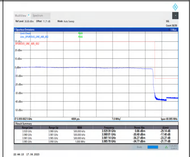
1-N77-3700-3980-PC3-30-60-H-6-CP-QPSK-Outer_Full-162@0-Ant2-1--PASS-see graph
