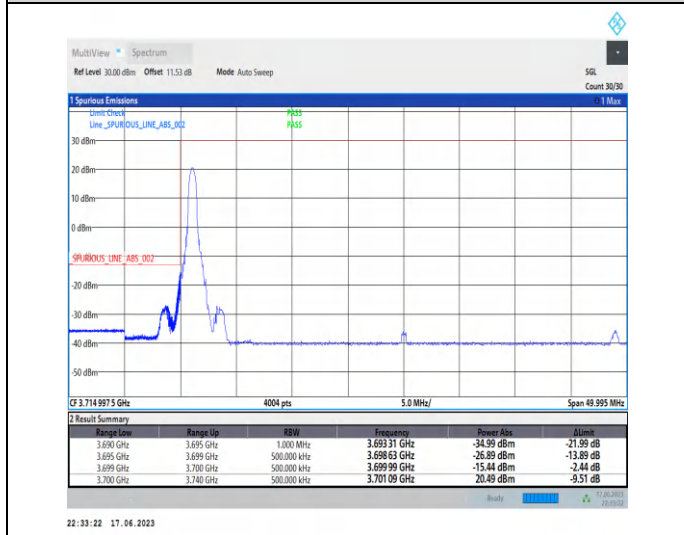
1-N77-3700-3980-PC3-30-40-L-4-CP-QPSK-Edge_1RB_Left-1@0-Ant2-1--PASS-see graph
