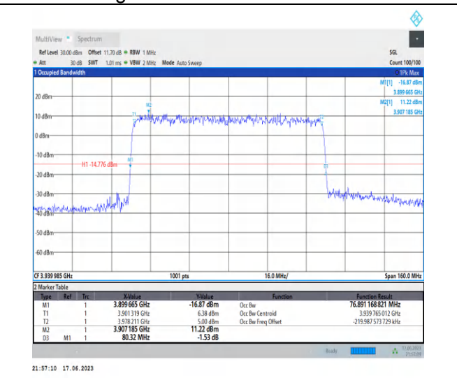
1-N77-3700-3980-PC3-30-80-H-4-DFT-64QAM-Out er_Full-216@0-Ant2-76.891-80.320-≤80-PASS
