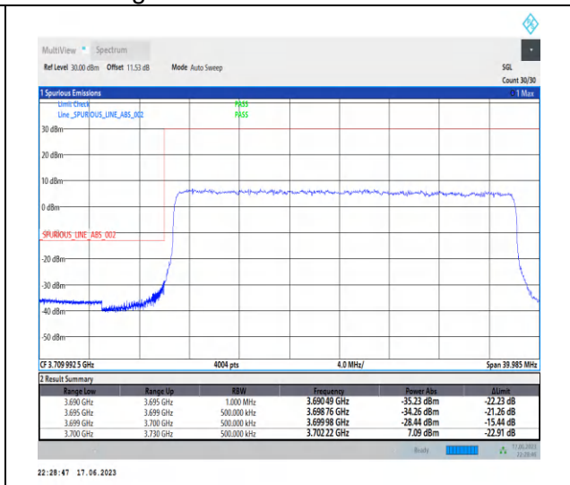
1-N77-3700-3980-PC3-30-30-L-3-DFT-PI2BPSK-Outer_Full-75@0-Ant2-1--PASS-see graph
