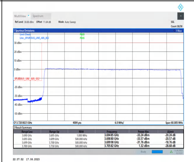
1-N77-3700-3980-PC3-30-50-L-6-CP-QPSK-Outer_Full-133@0-Ant2-1--PASS-see graph
