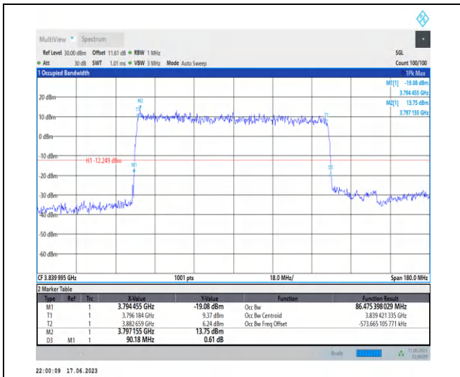
1-N77-3700-3980-PC3-30-90-M-1-DFT-PI2BPSK-Outer_Full-243@0-Ant2-86.475-90.180-≤90-PASS
