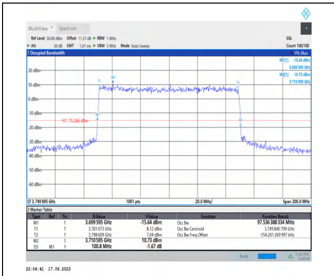
1-N77-3700-3980-PC3-30-100-L-7-CP-16QAM-Outer_Full-273@0-Ant2-97.536-100.800-≤100-PASS
