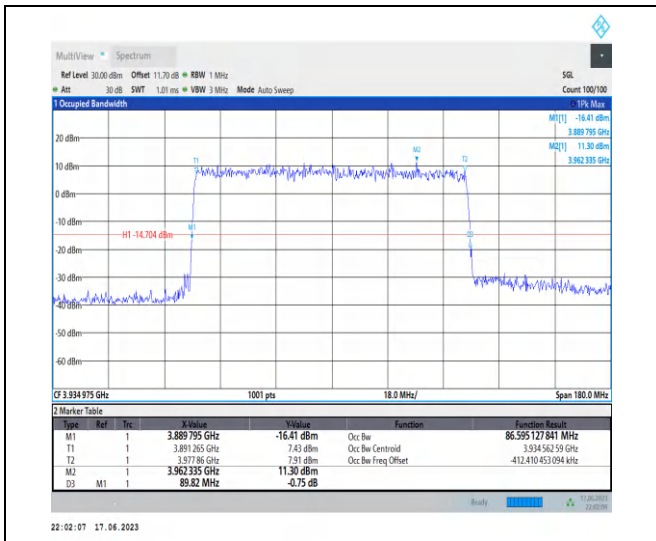
1-N77-3700-3980-PC3-30-90-H-4-DFT-64QAM-Out er_Full-243@0-Ant2-86.595-89.820-≤90-PASS
