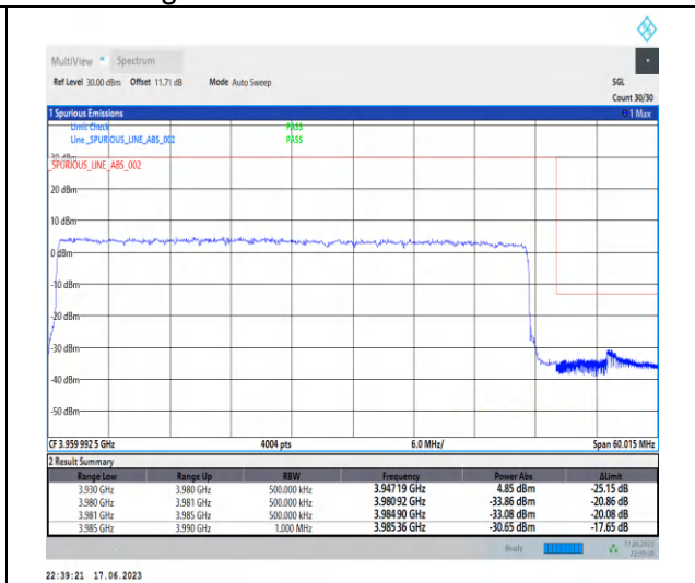
1-N77-3700-3980-PC3-30-50-H-3-DFT-PI2BPSK-Outer_Full-128@0-Ant2-1--PASS-see graph
