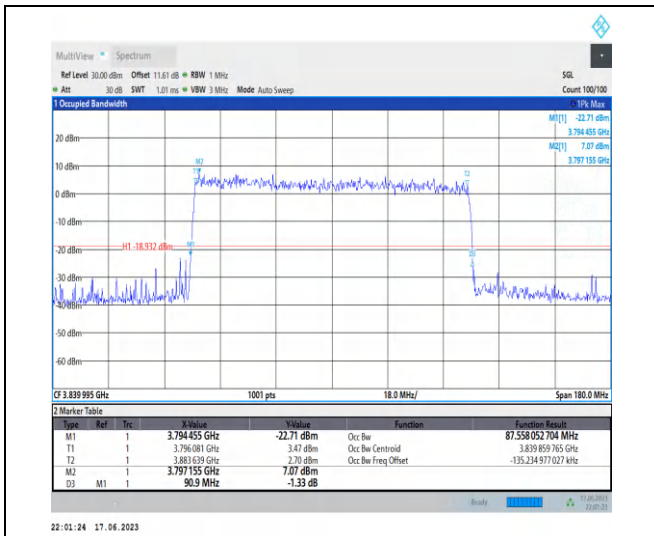
1-N77-3700-3980-PC3-30-90-M-9-CP-256QAM-Out er_Full-245@0-Ant2-87.558-90.900-≤90-PASS
