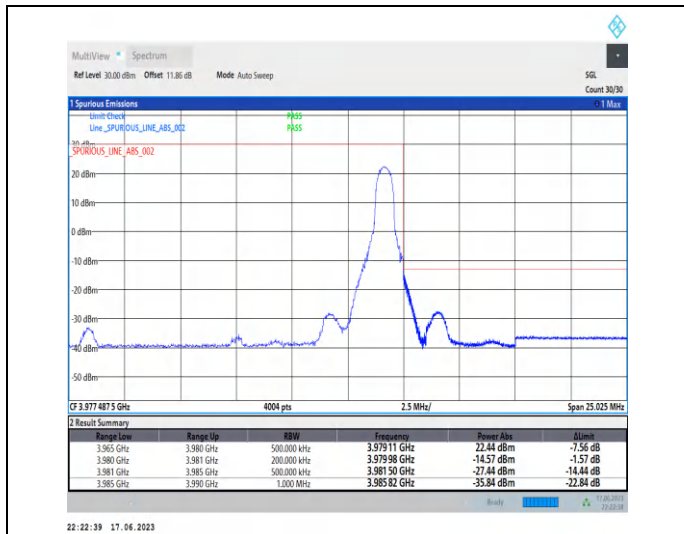
1-N77-3700-3980-PC3-30-15-H-2-DFT-PI2BPSK-Edge_1RB_Right-1@37-Ant2-1--PASS-see graph
