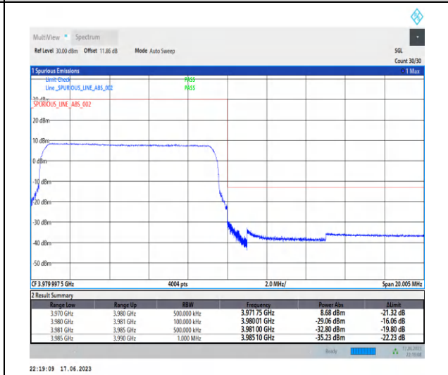
1-N77-3700-3980-PC3-30-10-H-6-CP-QPSK-Outer_Full-24@0-Ant2-1--PASS-see graph
