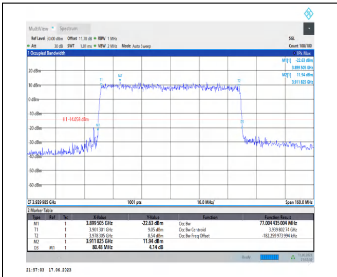
1-N77-3700-3980-PC3-30-80-H-3-DFT-16QAM-Out er_Full-216@0-Ant2-77.004-80.480-≤80-PASS
