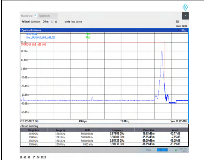
1-N77-3700-3980-PC3-30-60-H-5-CP-QPSK-Edge_1RB_Right-1@161-Ant2-1--PASS-see graph
