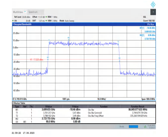
1-N77-3700-3980-PC3-30-90-L-5-DFT-256QAM-Outer_Full-243@0-Ant2-86.845-90.000-≤90-PASS
