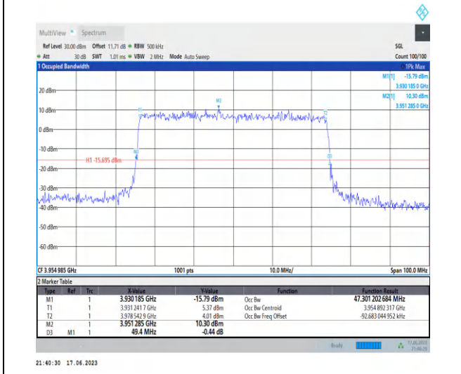
1-N77-3700-3980-PC3-30-50-H-6-CP-QPSK-Outer Full-133@0-Ant2-47.301-49.400-≤50-PASS
