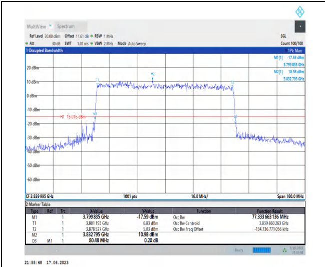
1-N77-3700-3980-PC3-30-80-M-8-CP-64QAM-Outer_Full-217@0-Ant2-77.334-80.480-≤80-PASS
