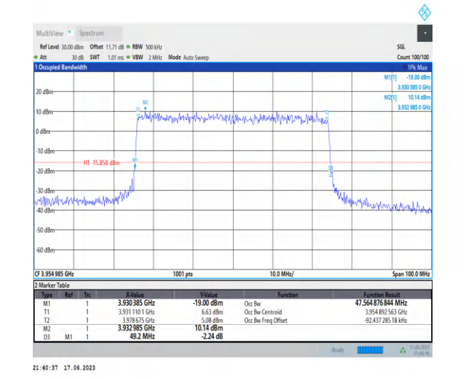
1-N77-3700-3980-PC3-30-50-H-7-CP-16QAM-Outer Full-133@0-Ant2-47.565-49.200-≤50-PASS
