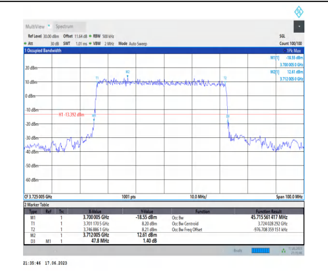
1-N77-3700-3980-PC3-30-50-L-1-DFT-PI2BPSK-Outer_Full-128@0-Ant2-45.716-47.800-≤50-PASS
