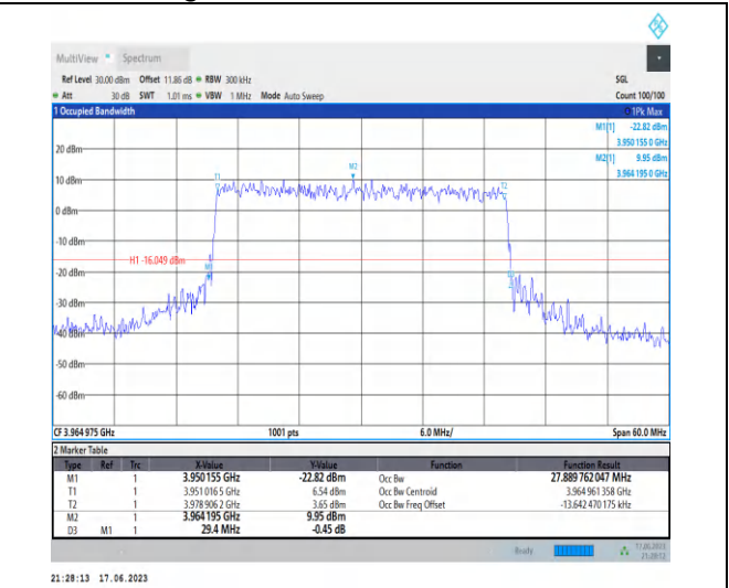
1-N77-3700-3980-PC3-30-30-H-7-CP-16QAM-Outer_Full-78@0-Ant2-27.89-29.400-≤30-PASS
