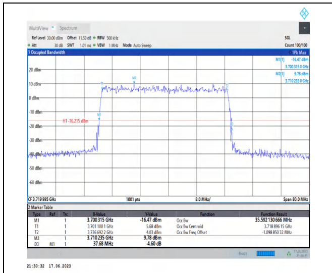
1-N77-3700-3980-PC3-30-40-L-5-DFT-256QAM-Out er_Full-100@0-Ant2-35.592-37.680-≤40-PASS
