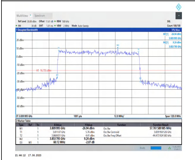
1-N77-3700-3980-PC3-30-60-M-8-CP-64QAM-Outer_Full-162@0-Ant2-57.762-60.120-≤60-PASS
