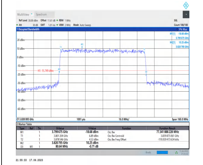
1-N77-3700-3980-PC3-30-80-M-6-CP-QPSK-Outer Full-217@0-Ant2-77.342-80.640-≤80-PASS
