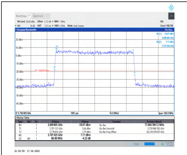
1-N77-3700-3980-PC3-30-80-L-9-CP-256QAM-Outer_Full-217@0-Ant2-77.695-80.480-≤80-PASS
