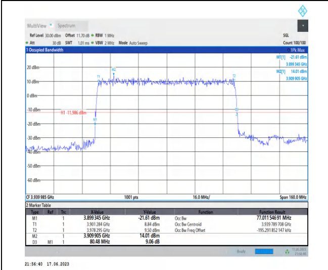
1-N77-3700-3980-PC3-30-80-H-1-DFT-PI2BPSK-Outer_Full-216@0-Ant2-77.012-80.480-≤80-PASS
