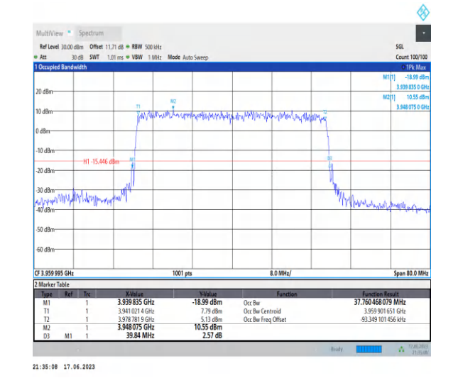
1-N77-3700-3980-PC3-30-40-H-6-CP-QPSK-Out er_Full-106@0-Ant2-37.76-39.840-≤40-PASS
