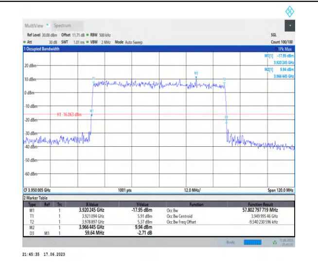
1-N77-3700-3980-PC3-30-60-H-4-DFT-64QAM-Outer_Full-162@0-Ant2-57.803-59.640-≤60-PASS
