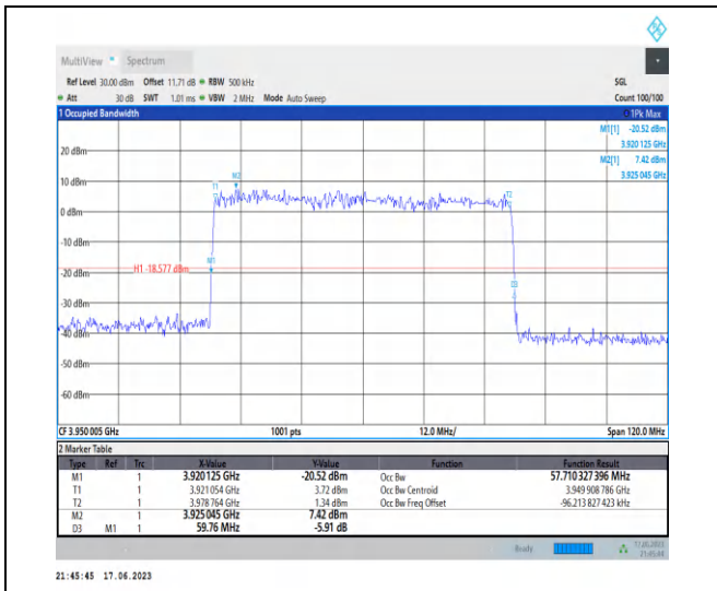
1-N77-3700-3980-PC3-30-60-H-5-DFT-256QAM-Outer_Full-162@0-Ant2-57.71-59.760-≤60-PASS
