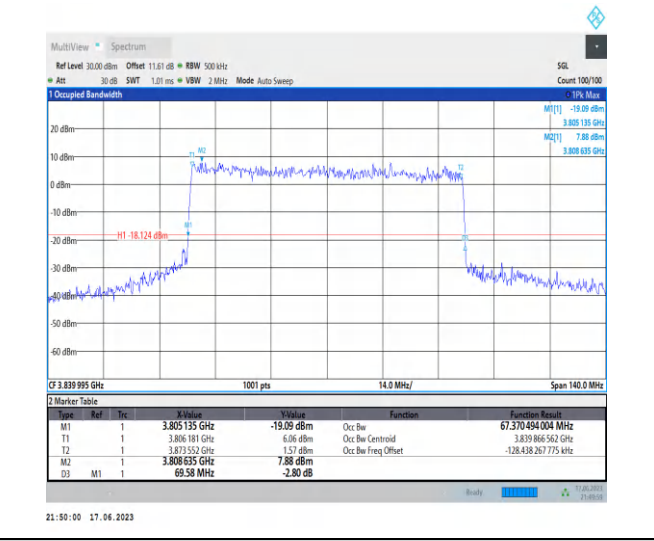
1-N77-3700-3980-PC3-30-70-M-6-CP-QPSK-Out er_Full-189@0-Ant2-67.37-69.580-≤70-PASS
