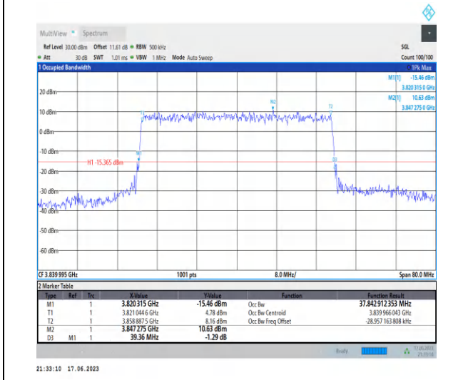
1-N77-3700-3980-PC3-30-40-M-6-CP-QPSK-Outer Full-106@0-Ant2-37.843-39.360-≤40-PASS
