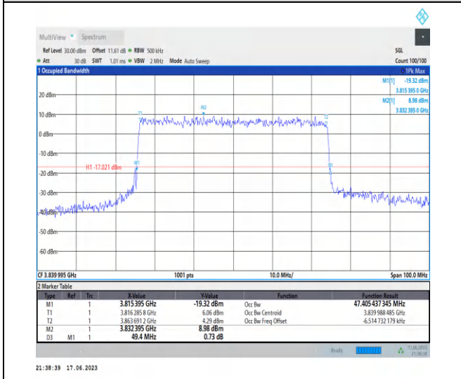
1-N77-3700-3980-PC3-30-50-M-7-CP-16QAM-Outer_Full-133@0-Ant2-47.405-49.400-≤50-PASS
