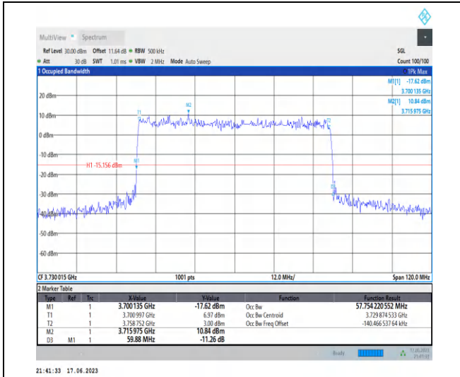
1-N77-3700-3980-PC3-30-60-L-3-DFT-16QAM-Outer_Full-162@0-Ant2-57.754-59.880-≤60-PASS
