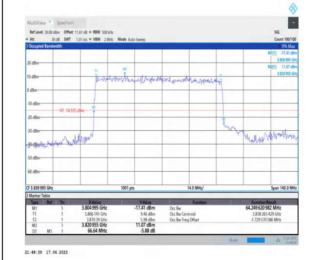
1-N77-3700-3980-PC3-30-70-M-1-DFT-PI2BPSK-Outer _Full-180@0-Ant2-64.25-66.640-≤70-PASS
