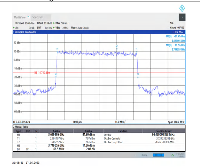
1-N77-3700-3980-PC3-30-70-L-1-DFT-PI2BPSK-Out er_Full-180@0-Ant2-64.45-66.500-≤70-PASS
