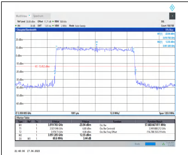
1-N77-3700-3980-PC3-30-60-H-1-DFT-PI2BPSK-Outer_Full-162@0-Ant2-57.684-60.600-≤60-PASS
