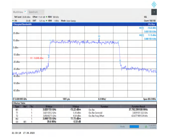
1-N77-3700-3980-PC3-30-40-M-7-CP-16QAM-Outer _Full-106@0-Ant2-37.792-39.600-≤40-PASS
