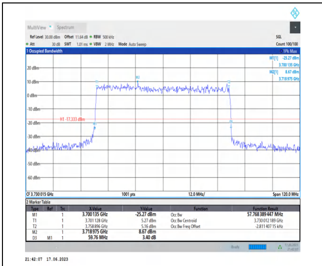
1-N77-3700-3980-PC3-30-60-L-7-CP-16QAM-Outer_Full-162@0-Ant2-57.768-59.760-≤60-PASS
