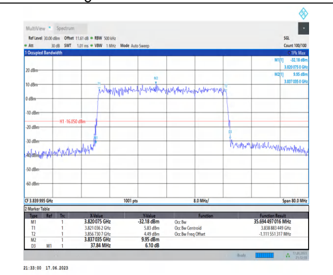
1-N77-3700-3980-PC3-30-40-M-5-DFT-256QAM-Out er_Full-100@0-Ant2-35.694-37.840-≤40-PASS
