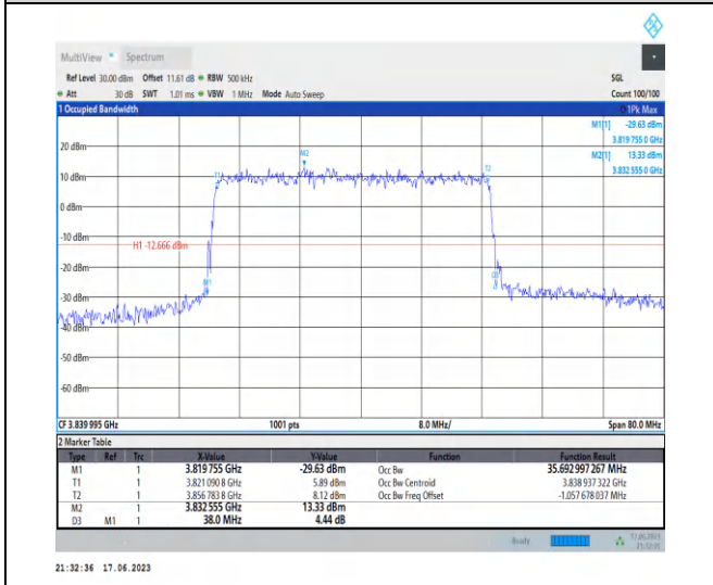
1-N77-3700-3980-PC3-30-40-M-2-DFT-QPSK-Outer_Full-100@0-Ant2-35.693-38.000-≤40-PASS
