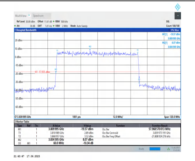
1-N77-3700-3980-PC3-30-60-M-5-DFT-256QAM-Outer_Full-162@0-Ant2-57.969-60.000-≤60-PASS
