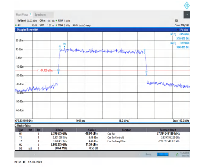
1-N77-3700-3980-PC3-30-80-M-7-CP-16QAM-Outer _Full-217@0-Ant2-77.395-80.640-≤80-PASS
