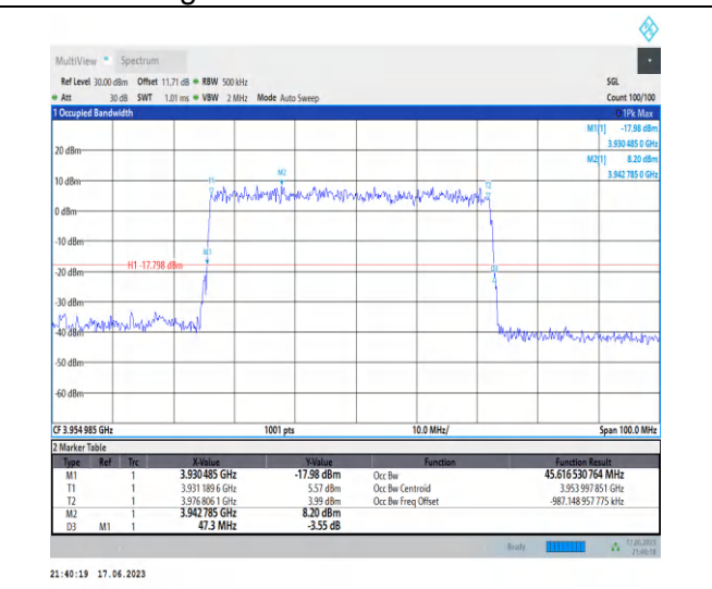
1-N77-3700-3980-PC3-30-50-H-5-DFT-256QAM-Out er_Full-128@0-Ant2-45.617-47.300-≤50-PASS
