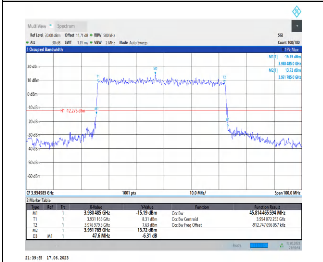
1-N77-3700-3980-PC3-30-50-H-2-DFT-QPSK-Outer_Full-128@0-Ant2-45.814-47.600-≤50-PASS
