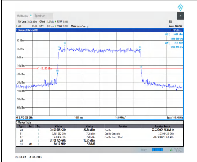
1-N77-3700-3980-PC3-30-80-L-3-DFT-16QAM-Outer_Full-216@0-Ant2-77.222-80.160-≤80-PASS
