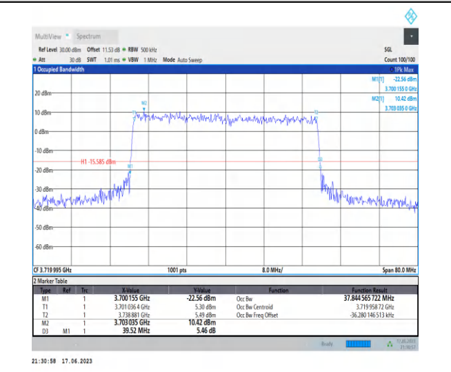
1-N77-3700-3980-PC3-30-40-L-8-CP-64QAM-Outer_Full-106@0-Ant2-37.845-39.520-≤40-PASS
