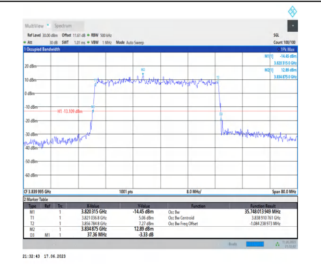
1-N77-3700-3980-PC3-30-40-M-3-DFT-16QAM-Outer_Full-100@0-Ant2-35.748-37.360-≤40-PASS
