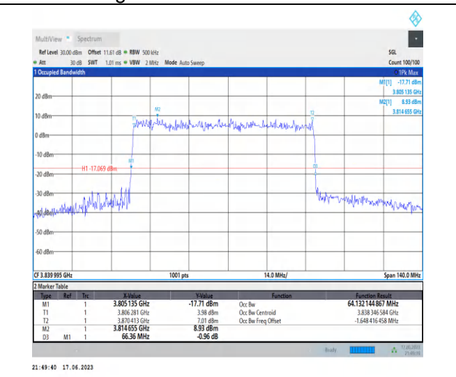
1-N77-3700-3980-PC3-30-70-M-4-DFT-64QAM-Out er_Full-180@0-Ant2-64.132-66.360-≤70-PASS
