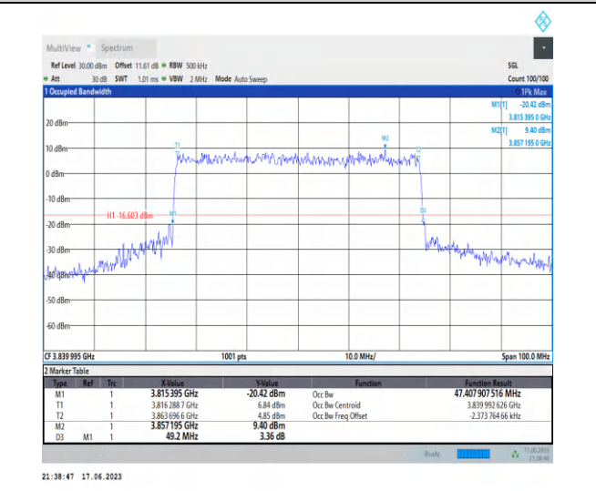
1-N77-3700-3980-PC3-30-50-M-8-CP-64QAM-Outer_Full-133@0-Ant2-47.408-49.200-≤50-PASS
