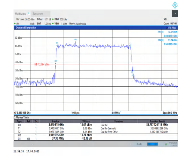
1-N77-3700-3980-PC3-30-40-H-2-DFT-QPSK-Outer_Full-100@0-Ant2-35.798-37.360-≤40-PASS
