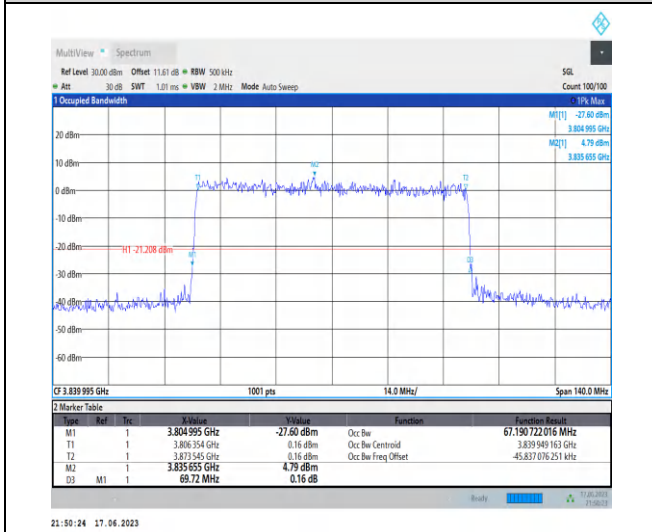
1-N77-3700-3980-PC3-30-70-M-9-CP-256QAM-Outer_Full-189@0-Ant2-67.191-69.720-≤70-PASS
