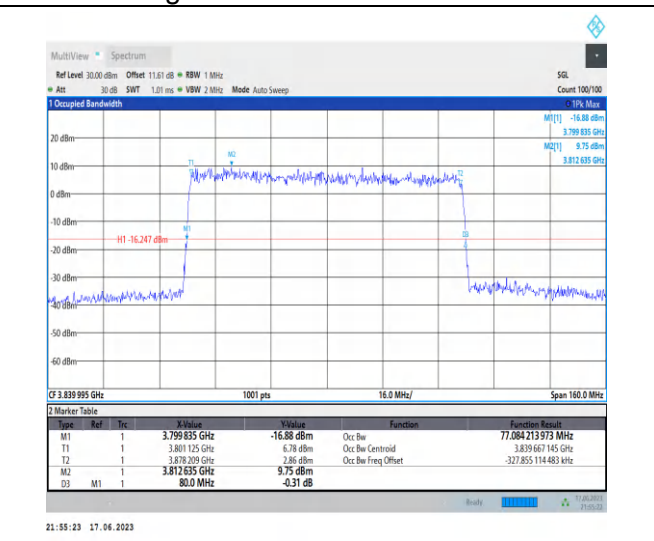
1-N77-3700-3980-PC3-30-80-M-5-DFT-256QAM-Out er_Full-216@0-Ant2-77.084-80.000-≤80-PASS
