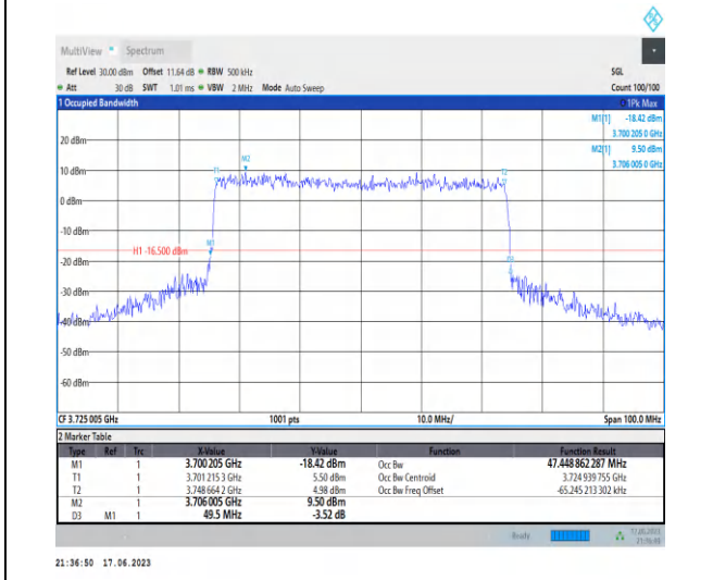
1-N77-3700-3980-PC3-30-50-L-8-CP-64QAM-Outer_Full-133@0-Ant2-47.449-49.500-≤50-PASS
