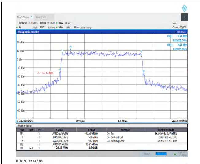
1-N77-3700-3980-PC3-30-30-M-7-CP-16QAM-Outer_Full-78@0-Ant2-27.745-29.460-≤30-PASS
