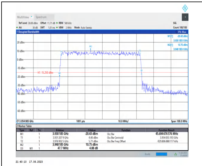
1-N77-3700-3980-PC3-30-50-H-4-DFT-64QAM-Out er_Full-128@0-Ant2-45.695-47.700-≤50-PASS
