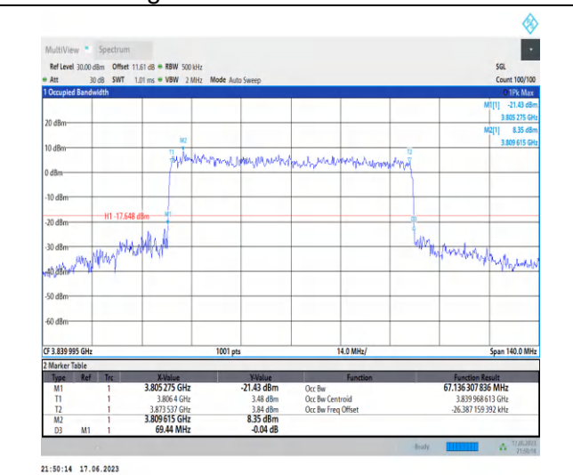
1-N77-3700-3980-PC3-30-70-M-8-CP-64QAM-Outer_Full-189@0-Ant2-67.136-69.440-≤70-PASS
