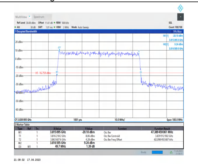
1-N77-3700-3980-PC3-30-50-M-6-CP-QPSK-Outer_Full-133@0-Ant2-47.389-49.700-≤50-PASS
