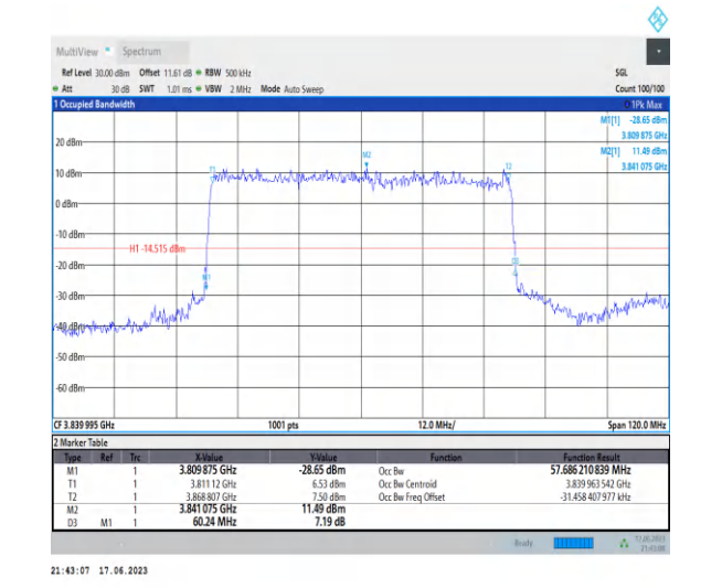
1-N77-3700-3980-PC3-30-60-M-1-DFT-PI2BPSK-Outer_Full-162@0-Ant2-57.686-60.240-≤60-PASS
