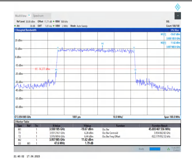
1-N77-3700-3980-PC3-30-50-H-3-DFT-16QAM-Outer_Full-128@0-Ant2-45.693-47.600-≤50-PASS
