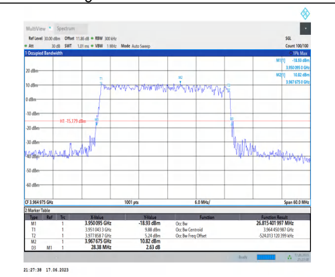
1-N77-3700-3980-PC3-30-30-H-3-DFT-16QAM-Outer_Full-75@0-Ant2-26.815-28.380-≤30-PASS
