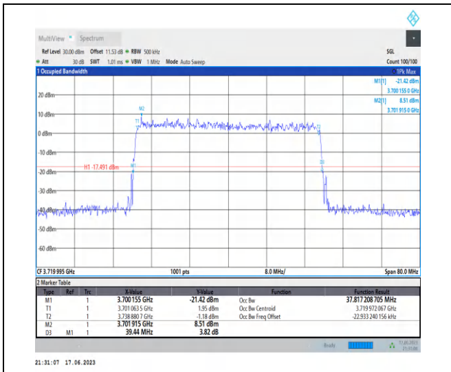
1-N77-3700-3980-PC3-30-40-L-9-CP-256QAM-Outer_Full-106@0-Ant2-37.817-39.440-≤40-PASS
