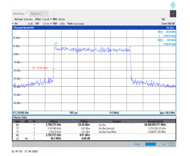
1-N77-3700-3980-PC3-30-70-L-3-DFT-16QAM-Outer _Full-180@0-Ant2-64.507-66.500-≤70-PASS
