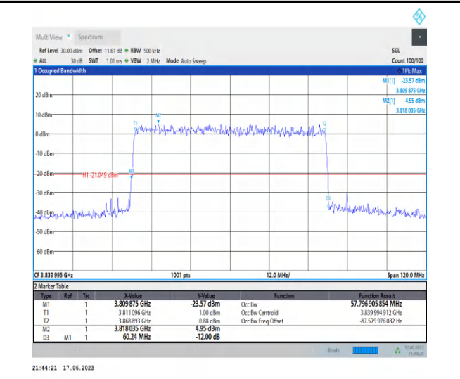
1-N77-3700-3980-PC3-30-60-M-9-CP-256QAM-Outer_Full-162@0-Ant2-57.797-60.240-≤60-PASS
