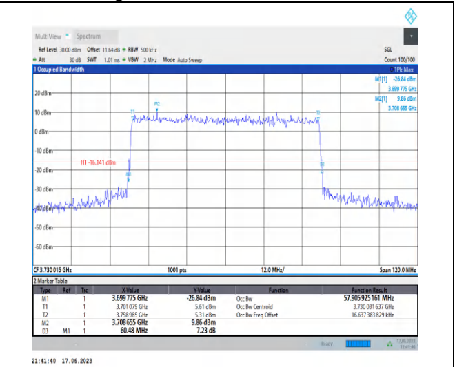
1-N77-3700-3980-PC3-30-60-L-4-DFT-64QAM-Outer_Full-162@0-Ant2-57.906-60.480-≤60-PASS
