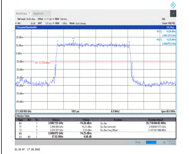
1-N77-3700-3980-PC3-30-40-H-1-DFT-PI2BPSK-Outer_Full-100@0-Ant2-35.718-37.920-≤40-PASS
