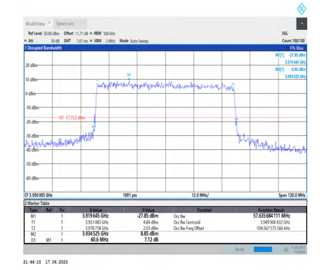
1-N77-3700-3980-PC3-30-60-H-8-CP-64QAM-Outer_Full-162@0-Ant2-57.636-60.600-≤60-PASS
