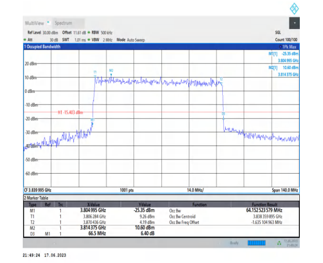
1-N77-3700-3980-PC3-30-70-M-2-DFT-QPSK-Outer _Full-180@0-Ant2-64.153-66.500-≤70-PASS
