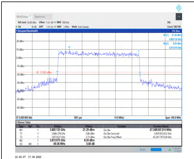
1-N77-3700-3980-PC3-30-70-M-7-CP-16QAM-Outer_Full-189@0-Ant2-67.349-69.580-≤70-PASS
