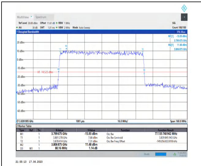
1-N77-3700-3980-PC3-30-80-M-4-DFT-64QAM-Out er_Full-216@0-Ant2-77.136-80.160-≤80-PASS
