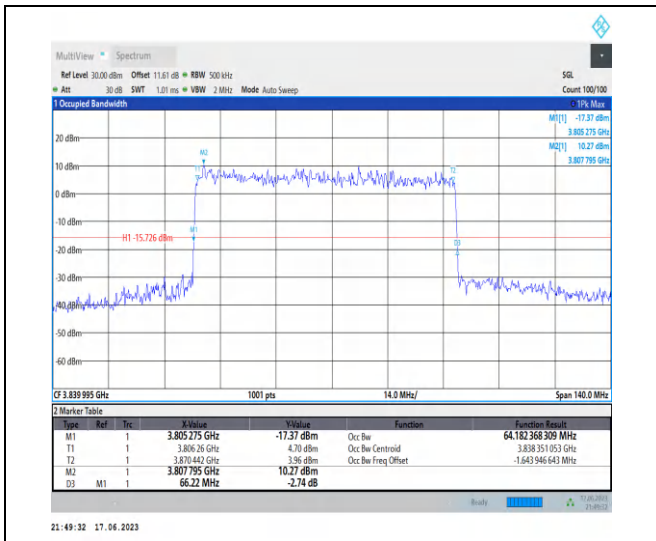
1-N77-3700-3980-PC3-30-70-M-3-DFT-16QAM-Out er_Full-180@0-Ant2-64.182-66.220-≤70-PASS
