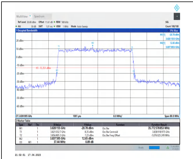
1-N77-3700-3980-PC3-30-40-M-4-DFT-64QAM-Out er_Full-100@0-Ant2-35.773-37.440-≤40-PASS
