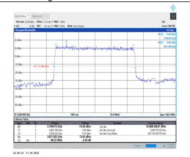
1-N77-3700-3980-PC3-30-80-M-1-DFT-PI2BPSK-Outer_Full-216@0-Ant2-76.908-80.320-≤80-PASS
