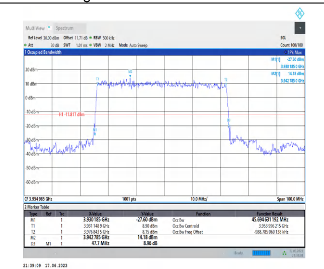
1-N77-3700-3980-PC3-30-50-H-1-DFT-PI2BPSK-Out er_Full-128@0-Ant2-45.695-47.700-≤50-PASS
