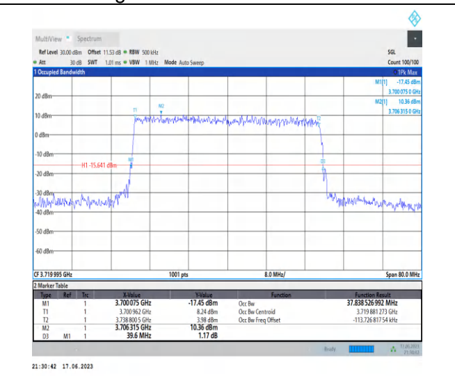
1-N77-3700-3980-PC3-30-40-L-6-CP-QPSK-Outer_Full-106@0-Ant2-37.839-39.600-≤40-PASS
