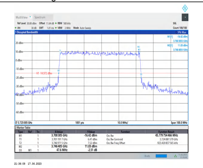
1-N77-3700-3980-PC3-30-50-L-3-DFT-16QAM-Outer_Full-128@0-Ant2-45.78-47.600-≤50-PASS
