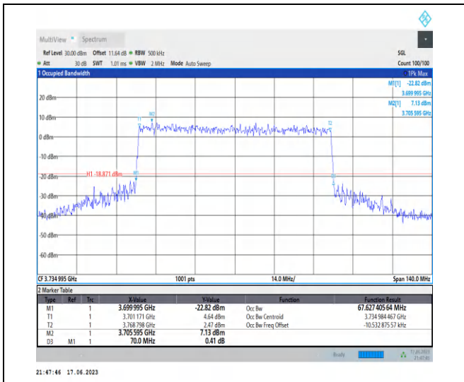
1-N77-3700-3980-PC3-30-70-L-8-CP-64QAM-Outer _Full-189@0-Ant2-67.627-70.000-≤70-PASS
