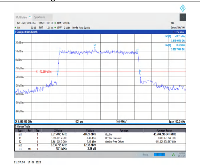
1-N77-3700-3980-PC3-30-50-M-2-DFT-QPSK-Outer_Full-128@0-Ant2-45.704-48.100-≤50-PASS
