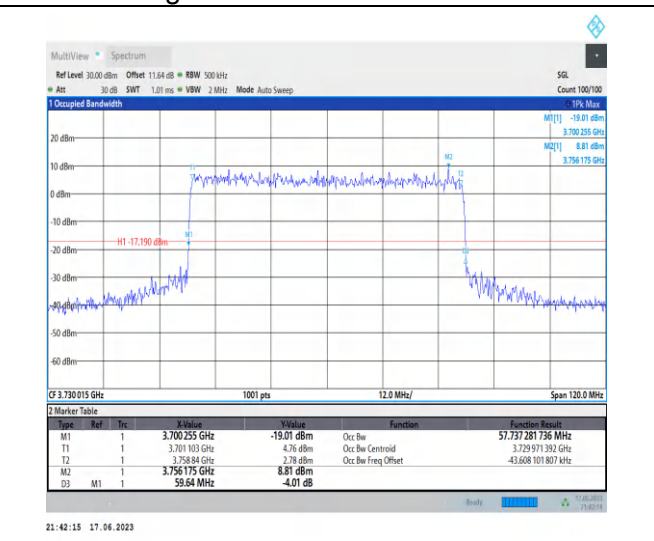
1-N77-3700-3980-PC3-30-60-L-8-CP-64QAM-Outer_Full-162@0-Ant2-57.737-59.640-≤60-PASS
