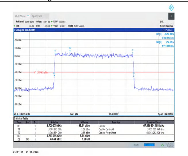
1-N77-3700-3980-PC3-30-70-L-9-CP-256QAM-Outer _Full-189@0-Ant2-67.557-69.440-≤70-PASS
