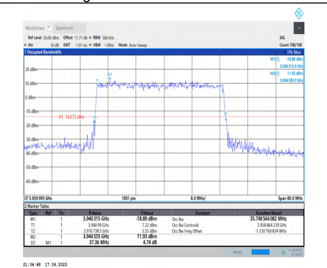
1-N77-3700-3980-PC3-30-40-H-4-DFT-64QAM-Out er_Full-100@0-Ant2-35.749-37.360-≤40-PASS
