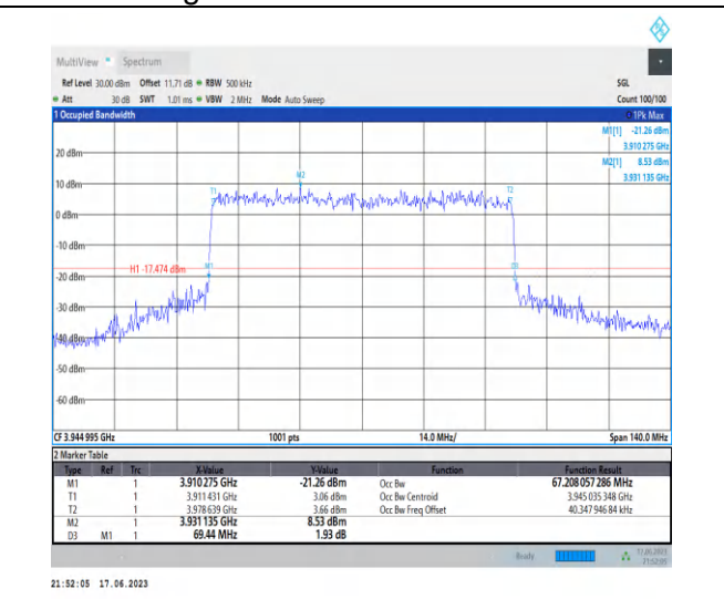
1-N77-3700-3980-PC3-30-70-H-7-CP-16QAM-Outer_Full-189@0-Ant2-67.208-69.440-≤70-PASS
