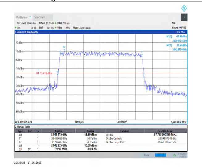
1-N77-3700-3980-PC3-30-40-H-8-CP-64QAM-Outer_Full-106@0-Ant2-37.783-39.920-≤40-PASS
