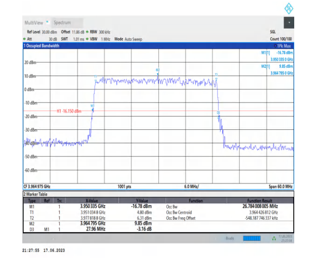
1-N77-3700-3980-PC3-30-30-H-5-DFT-256QAM-Outer_Full-75@0-Ant2-26.784-27.960-≤30-PASS
