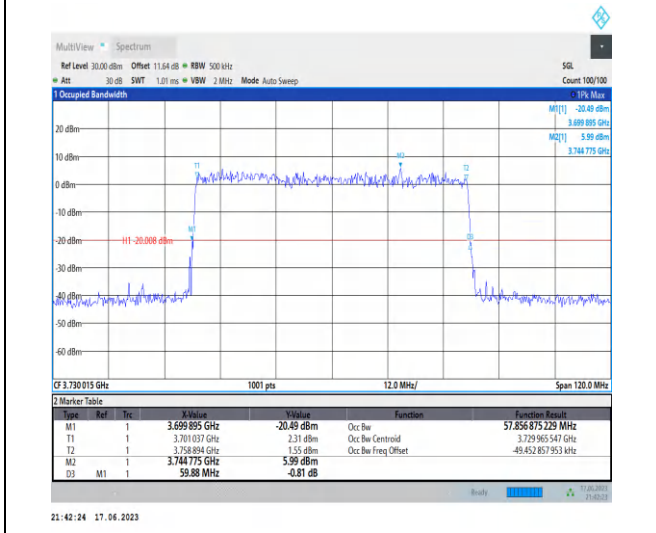
1-N77-3700-3980-PC3-30-60-L-9-CP-256QAM-Outer_Full-162@0-Ant2-57.857-59.880-≤60-PASS
