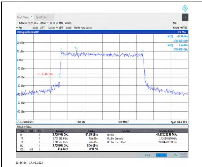
1-N77-3700-3980-PC3-30-50-L-6-CP-QPSK-Outer_Full-133@0-Ant2-47.372-49.400-≤50-PASS
