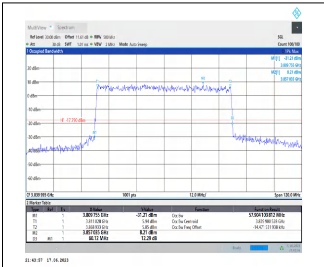
1-N77-3700-3980-PC3-30-60-M-6-CP-QPSK-Outer_Full-162@0-Ant2-57.904-60.120-≤60-PASS
