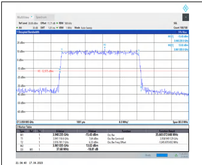
1-N77-3700-3980-PC3-30-40-H-3-DFT-16QAM-Out er_Full-100@0-Ant2-35.665-37.680-≤40-PASS
