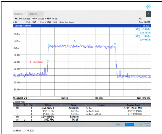
1-N77-3700-3980-PC3-30-60-H-9-CP-256QAM-Out er_Full-162@0-Ant2-57.691-59.520-≤60-PASS
