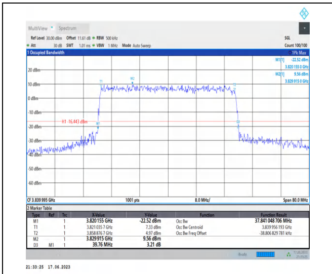
1-N77-3700-3980-PC3-30-40-M-8-CP-64QAM-Outer_Full-106@0-Ant2-37.841-39.760-≤40-PASS
