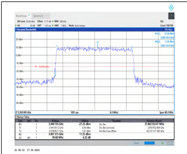
1-N77-3700-3980-PC3-30-40-H-7-CP-16QAM-Outer_Full-106@0-Ant2-37.803-39.680-≤40-PASS
