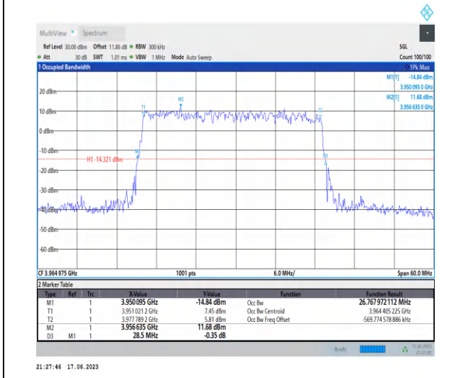
1-N77-3700-3980-PC3-30-30-H-4-DFT-64QAM-Outer_Full-75@0-Ant2-26.768-28.500-≤30-PASS
