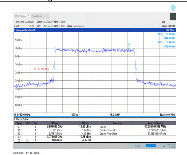
1-N77-3700-3980-PC3-30-80-L-6-CP-QPSK-Outer_Full-217@0-Ant2-77.536-80.800-≤80-PASS
