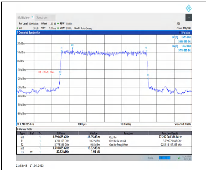
1-N77-3700-3980-PC3-30-80-L-1-DFT-PI2BPSK-Outer_Full-216@0-Ant2-77.233-80.320-≤80-PASS
