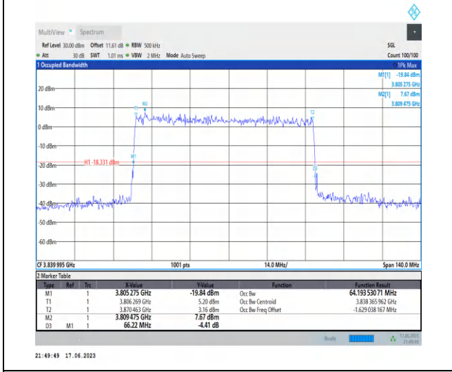
1-N77-3700-3980-PC3-30-70-M-5-DFT-256QAM-Out er_Full-180@0-Ant2-64.194-66.220-≤70-PASS
