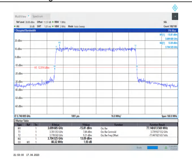
1-N77-3700-3980-PC3-30-80-L-2-DFT-QPSK-Outer_Full-216@0-Ant2-77.149-80.320-≤80-PASS
