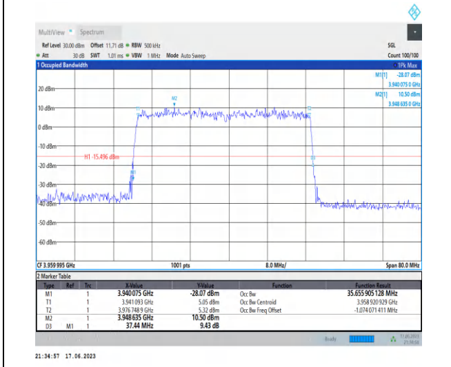
1-N77-3700-3980-PC3-30-40-H-5-DFT-256QAM-Out er_Full-100@0-Ant2-35.656-37.440-≤40-PASS
