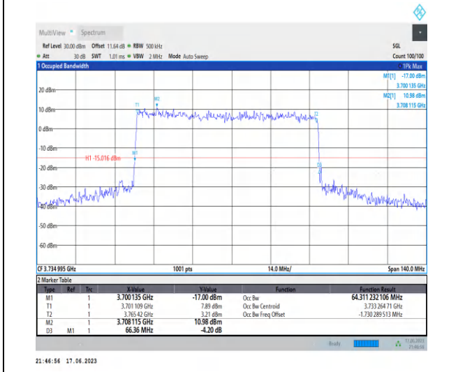
1-N77-3700-3980-PC3-30-70-L-2-DFT-QPSK-Outer _Full-180@0-Ant2-64.311-66.360-≤70-PASS
