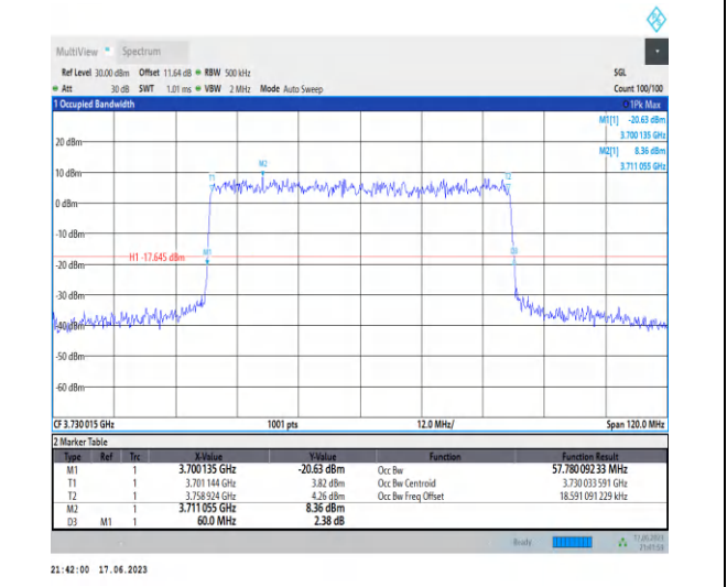
1-N77-3700-3980-PC3-30-60-L-6-CP-QPSK-Outer_Full-162@0-Ant2-57.78-60.000-≤60-PASS
