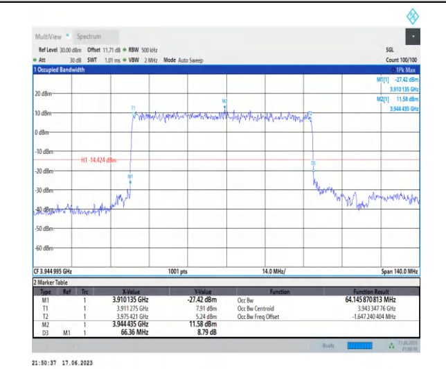
1-N77-3700-3980-PC3-30-70-H-1-DFT-PI2BPSK-Outer_Full-180@0-Ant2-64.146-66.360-≤70-PASS
