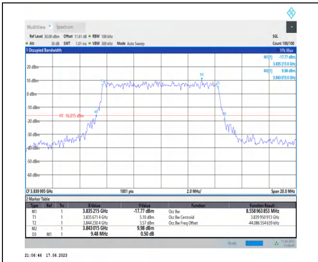
1-N77-3700-3980-PC3-30-10-M-4-DFT-64QAM-Out er_Full-24@0-Ant2-8.559-9.480-≤10-PASS
