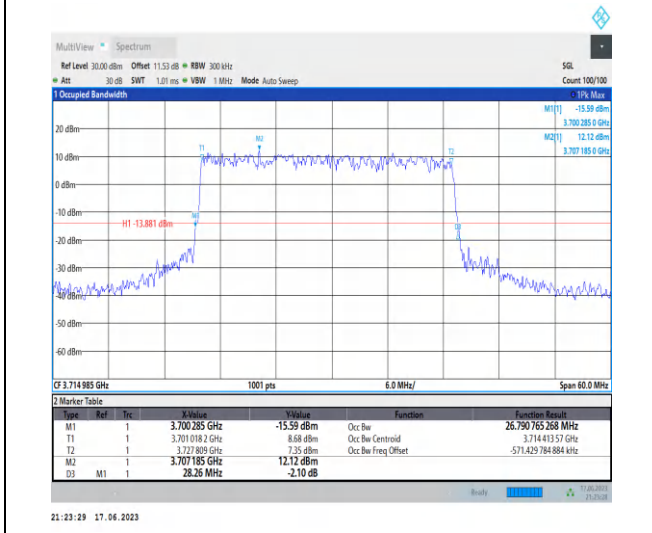
1-N77-3700-3980-PC3-30-30-L-2-DFT-QPSK-Outer_Full-75@0-Ant2-26.791-28.260-≤30-PASS
