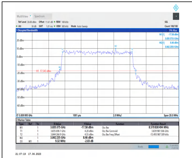
1-N77-3700-3980-PC3-30-10-M-8-CP-64QAM-Outer_Full-24@0-Ant2-8.571-9.320-≤10-PASS
