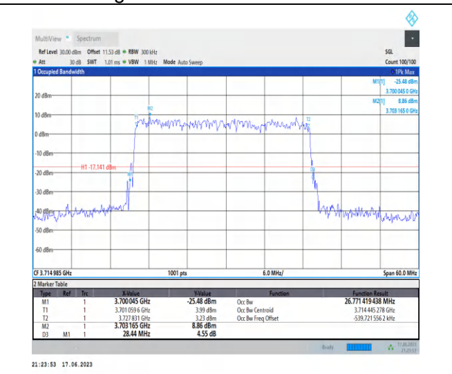
1-N77-3700-3980-PC3-30-30-L-5-DFT-256QAM-Outer_Full-75@0-Ant2-26.771-28.440-≤30-PASS
