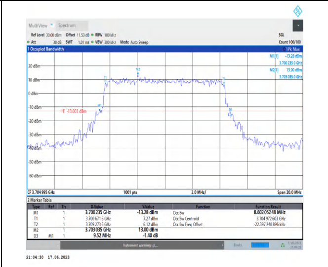
1-N77-3700-3980-PC3-30-10-L-2-DFT-QPSK-Outer_Full-24@0-Ant2-8.602-9.520-≤10-PASS
