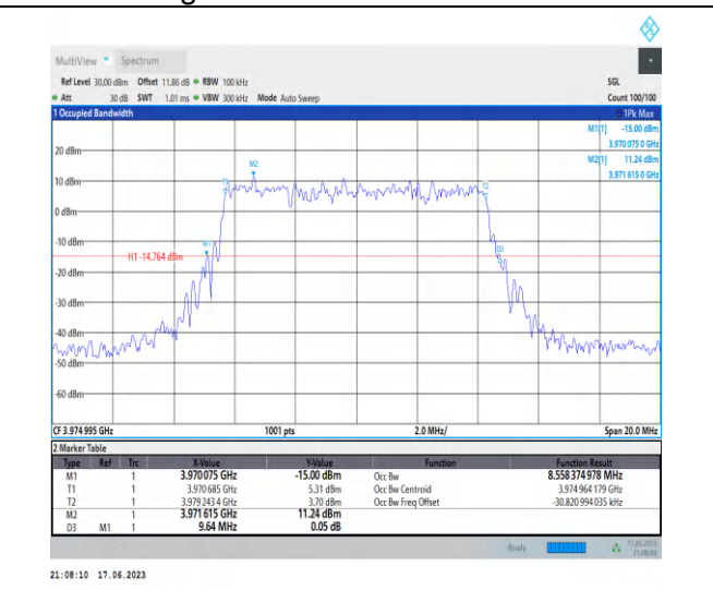
1-N77-3700-3980-PC3-30-10-H-4-DFT-64QAM-Out r_Full-24@0-Ant2-8.558-9.640-≤10-PASS
