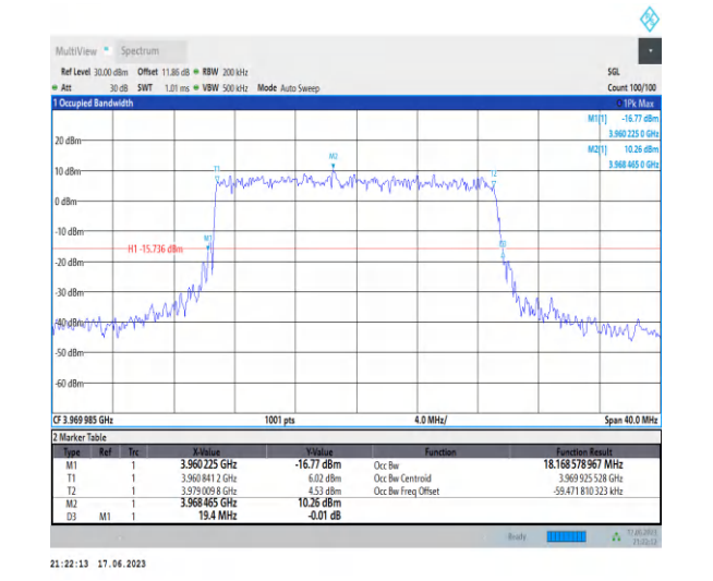
1-N77-3700-3980-PC3-30-20-H-8-CP-64QAM-Outer_Full-51@0-Ant2-18.169-19.400-≤20-PASS
