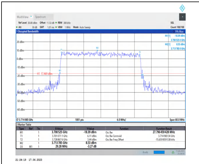
1-N77-3700-3980-PC3-30-30-L-8-CP-64QAM-Outer _Full-78@0-Ant2-27.796-29.280-≤30-PASS
