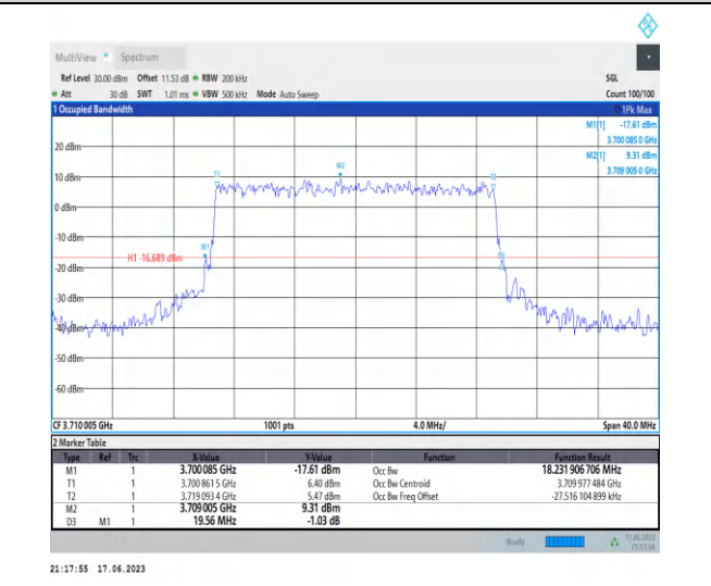
1-N77-3700-3980-PC3-30-20-L-6-CP-QPSK-Outer_Full-51@0-Ant2-18.232-19.560-≤20-PASS
