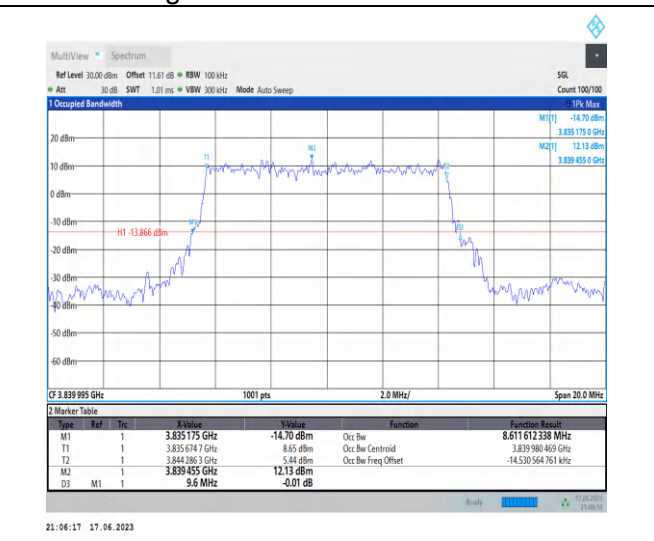
1-N77-3700-3980-PC3-30-10-M-1-DFT-PI2BPSK-Outer_Full-24@0-Ant2-8.612-9.600-≤10-PASS
