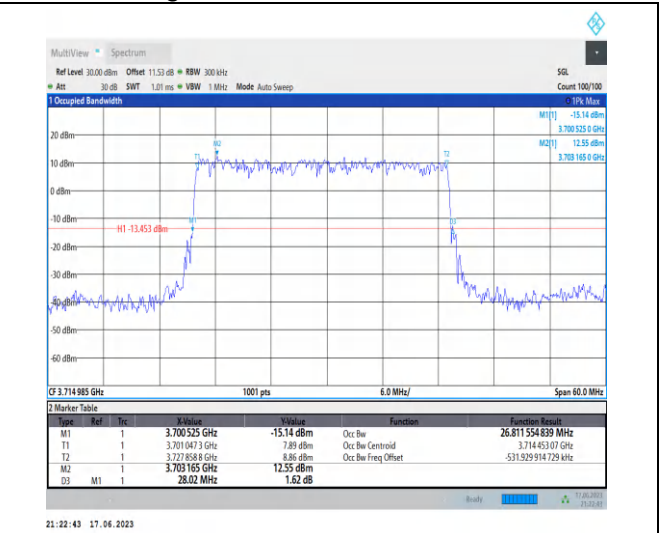
1-N77-3700-3980-PC3-30-30-L-1-DFT-PI2BPSK-Out er_Full-75@0-Ant2-26.812-28.020-≤30-PASS
