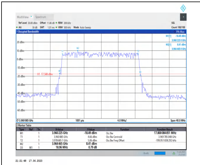
1-N77-3700-3980-PC3-30-20-H-5-DFT-256QAM-Outer_Full-50@0-Ant2-17.8-18.960-≤20-PASS
