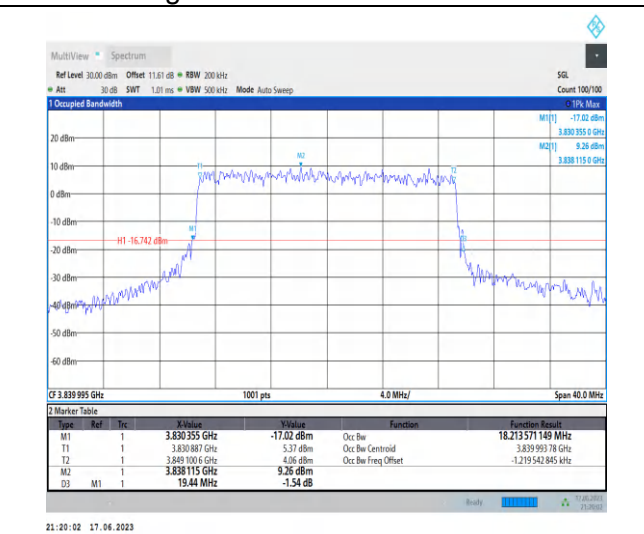
1-N77-3700-3980-PC3-30-20-M-7-CP-16QAM-Outer_Full-51 @0-Ant2-18.214-19.440-≤20-PASS
