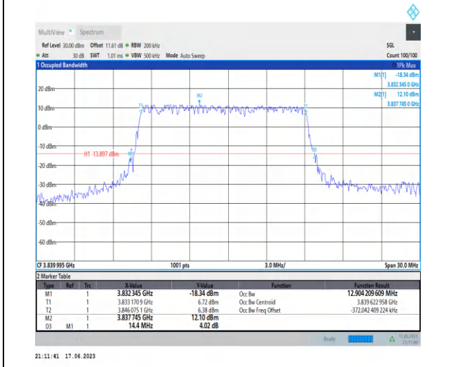
1-N77-3700-3980-PC3-30-15-M-3-DFT-16QAM-Outer_Full-36@0-Ant2-12.904-14.400-≤15-PASS
