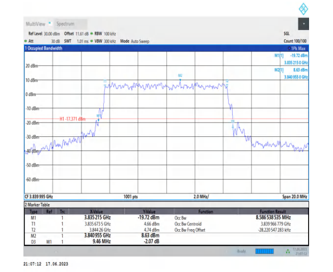
1-N77-3700-3980-PC3-30-10-M-7-CP-16QAM-Outer _Full-24@0-Ant2-8.587-9.460-≤10-PASS
