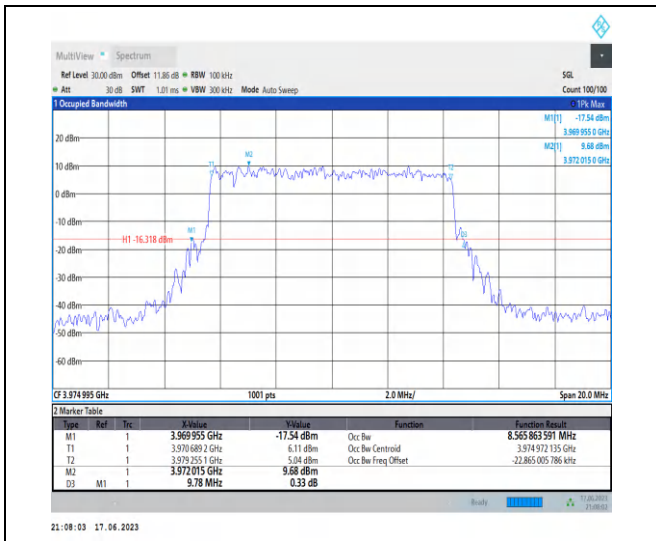
1-N77-3700-3980-PC3-30-10-H-3-DFT-16QAM-Out er_Full-24@0-Ant2-8.566-9.780-≤10-PASS
