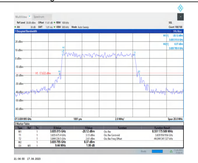
1-N77-3700-3980-PC3-30-10-M-5-DFT-256QAM-Out er_Full-24@0-Ant2-8.551-9.440-≤10-PASS
