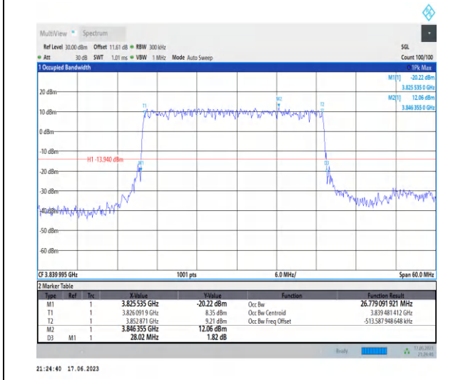
1-N77-3700-3980-PC3-30-30-M-1-DFT-PI2BPSK-Outer _Full-75@0-Ant2-26.779-28.020-≤30-PASS
