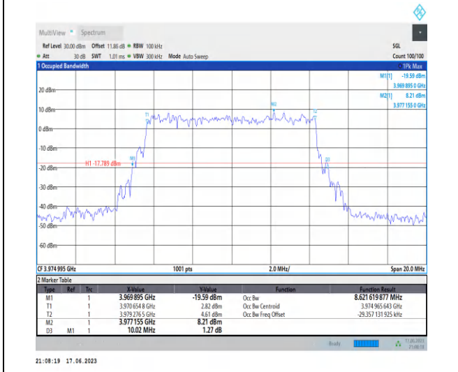
1-N77-3700-3980-PC3-30-10-H-5-DFT-256QAM-Out er_Full-24@0-Ant2-8.622-10.020-≤10-PASS
