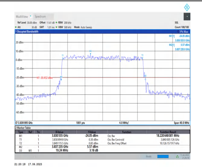
1-N77-3700-3980-PC3-30-20-M-9-CP-256QAM-Outer_Full-51 @0-Ant2-18.221-19.240-≤20-PASS
