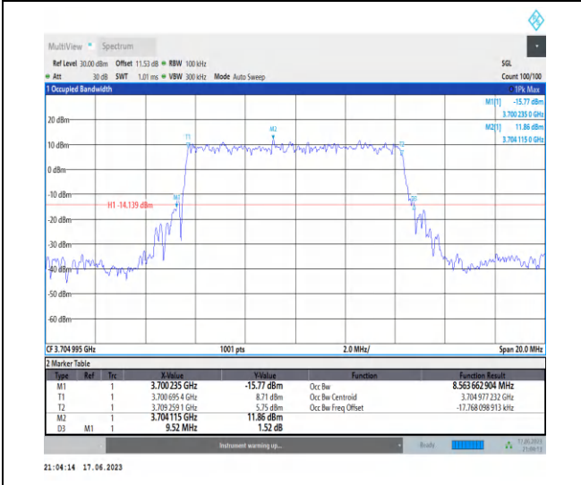
1-N77-3700-3980-PC3-30-10-L-1-DFT-PI2BPSK-Outer_Full-24@0-Ant2-8.564-9.520-≤10-PASS
