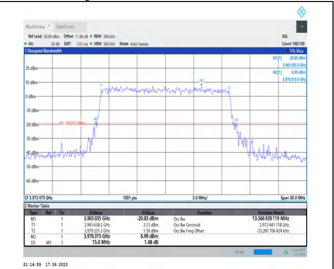
1-N77-3700-3980-PC3-30-15-H-9-CP-256QAM-Outer_Full-38@0-Ant2-13.567-15.000-≤15-PASS
