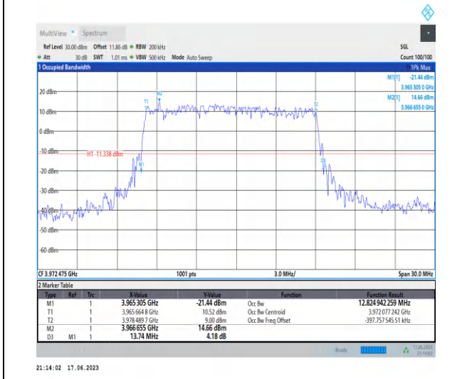
1-N77-3700-3980-PC3-30-15-H-2-DFT-QPSK-Outer_Full-36@0-Ant2-12.825-13.740-≤15-PASS
