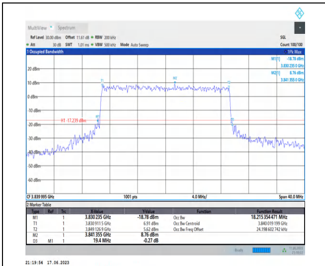
1-N77-3700-3980-PC3-30-20-M-6-CP-QPSK-Outer_Full-51 @0-Ant2-18.215-19.400-≤20-PASS
