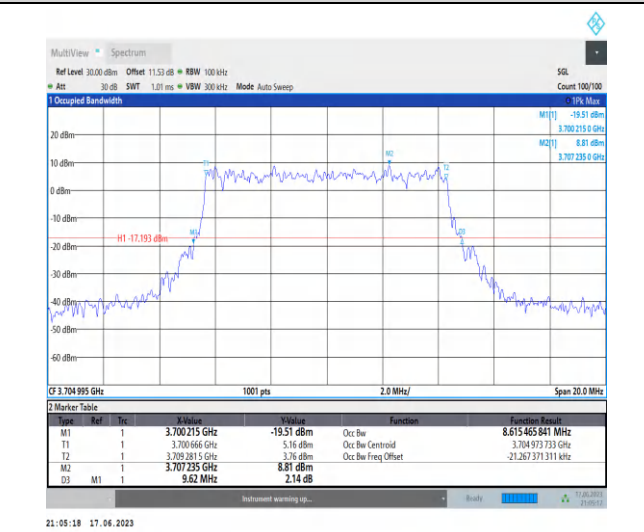
1-N77-3700-3980-PC3-30-10-L-8-CP-64QAM-Outer_Full-24@0-Ant2-8.615-9.620-≤10-PASS
