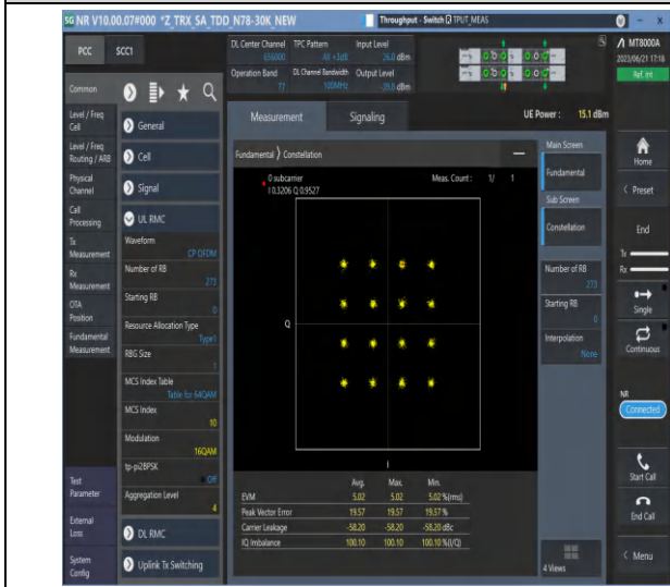
1-N77-3700-3980-PC3-30-100-M-7-CP-16QAM-Outer_Full-273@0-Ant2-see graph-PASS
