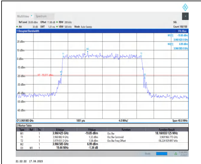
1-N77-3700-3980-PC3-30-20-H-9-CP-256QAM-Out er_Full-51@0-Ant2-18.169-19.440-≤20-PASS
