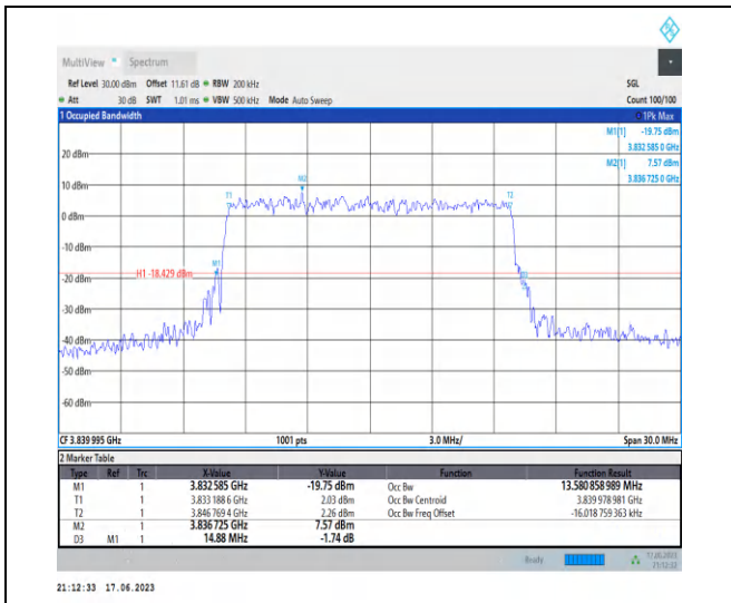
1-N77-3700-3980-PC3-30-15-M-9-CP-256QAM-Out er_Full-38@0-Ant2-13.581-14.880-≤15-PASS
