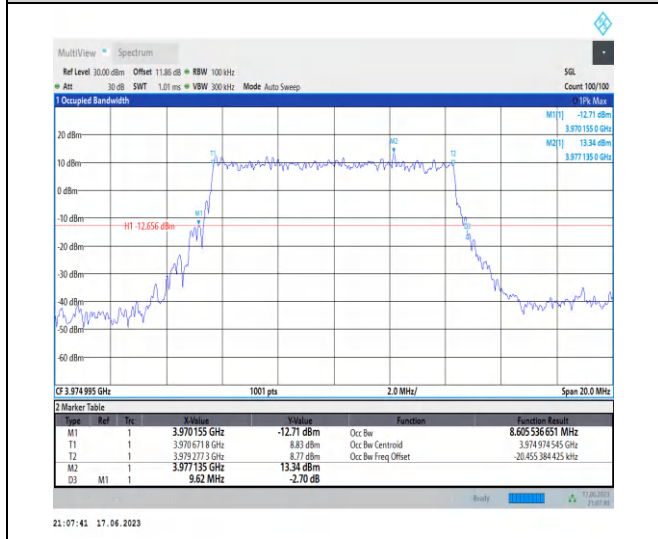
1-N77-3700-3980-PC3-30-10-H-1-DFT-PI2BPSK-Outer_Full-24@0-Ant2-8.606-9.620-≤10-PASS
