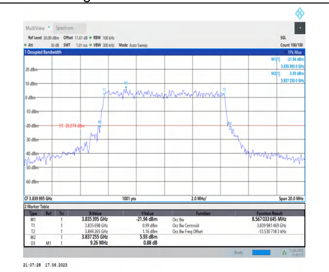
1-N77-3700-3980-PC3-30-10-M-9-CP-256QAM-Outer_Full-24@0-Ant2-8.567-9.260-≤10-PASS
