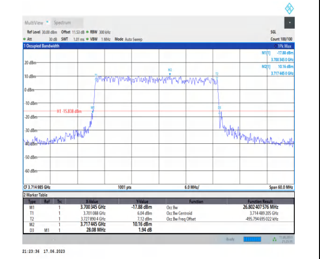
1-N77-3700-3980-PC3-30-30-L-3-DFT-16QAM-Outer_Full-75@0-Ant2-26.802-28.080-≤30-PASS
