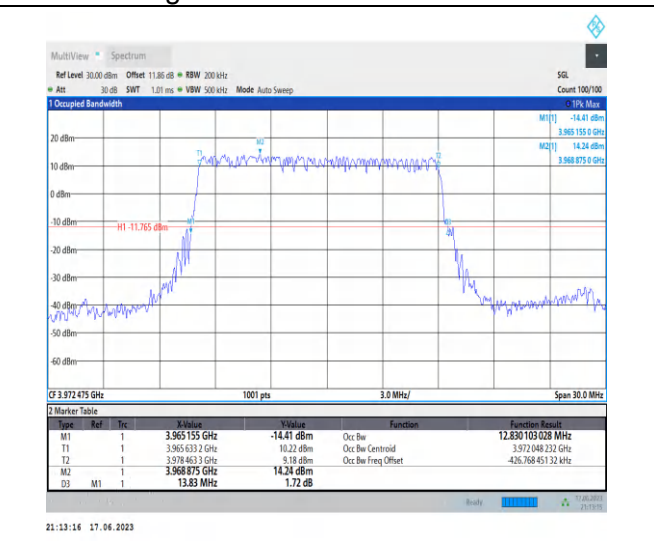
1-N77-3700-3980-PC3-30-15-H-1-DFT-PI2BPSK-Out er_Full-36@0-Ant2-12.83-13.830-≤15-PASS
