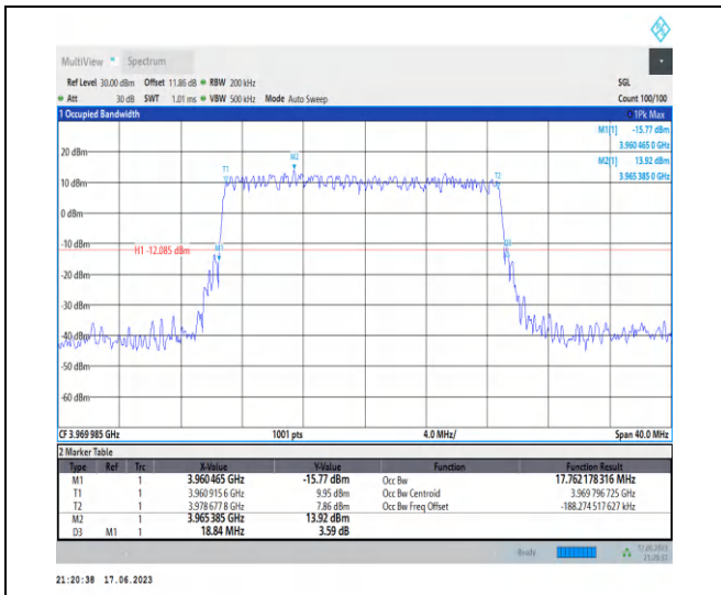
1-N77-3700-3980-PC3-30-20-H-1-DFT-PI2BPSK-Outer_Full-50@0-Ant2-17.762-18.840-≤20-PASS
