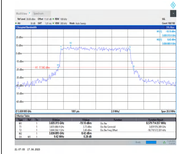
1-N77-3700-3980-PC3-30-10-M-6-CP-QPSK-Outer Full-24@0-Ant2-8.58-9.420-≤10-PASS
