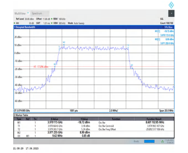
1-N77-3700-3980-PC3-30-10-H-6-CP-QPSK-Out er_Full-24@0-Ant2-8.601-9.620-≤10-PASS
