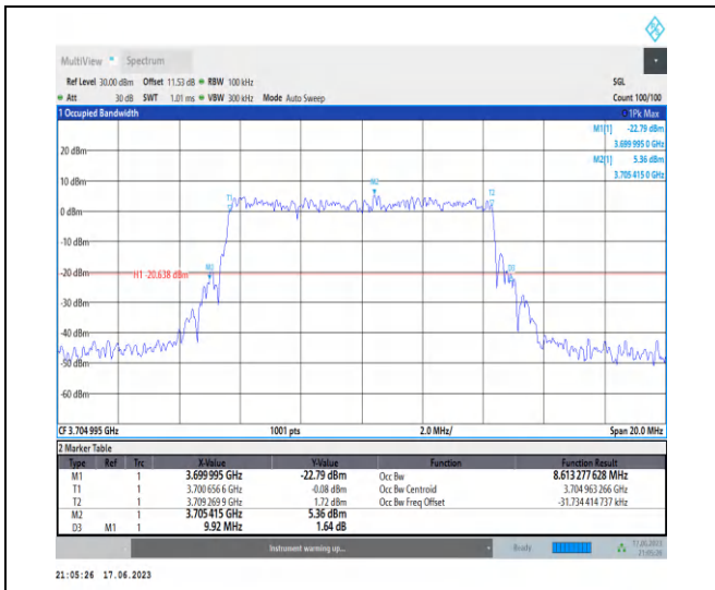
1-N77-3700-3980-PC3-30-10-L-9-CP-256QAM-Outer_Full-24@0-Ant2-8.613-9.920-≤10-PASS
