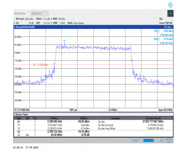
1-N77-3700-3980-PC3-30-30-L-7-CP-16QAM-Outer_Full-78@0-Ant2-27.858-29.340-≤30-PASS
