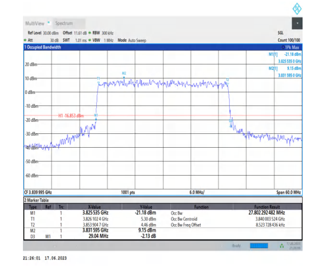
1-N77-3700-3980-PC3-30-30-M-6-CP-QPSK-Outer_Full-78@0-Ant2-27.802-29.040-≤30-PASS
