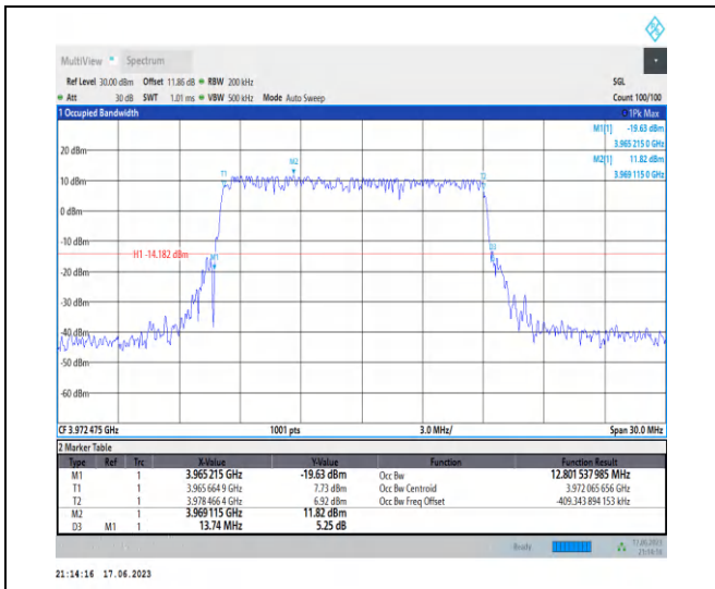
1-N77-3700-3980-PC3-30-15-H-4-DFT-64QAM-Out er_Full-36@0-Ant2-12.802-13.740-≤15-PASS
