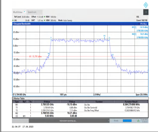
1-N77-3700-3980-PC3-30-10-L-3-DFT-16QAM-Outer_Full-24@0-Ant2-8.584-9.440-≤10-PASS
