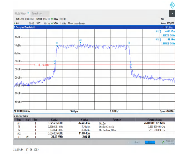
1-N77-3700-3980-PC3-30-30-M-2-DFT-QPSK-Outer _Full-75@0-Ant2-26.806-28.440-≤30-PASS
