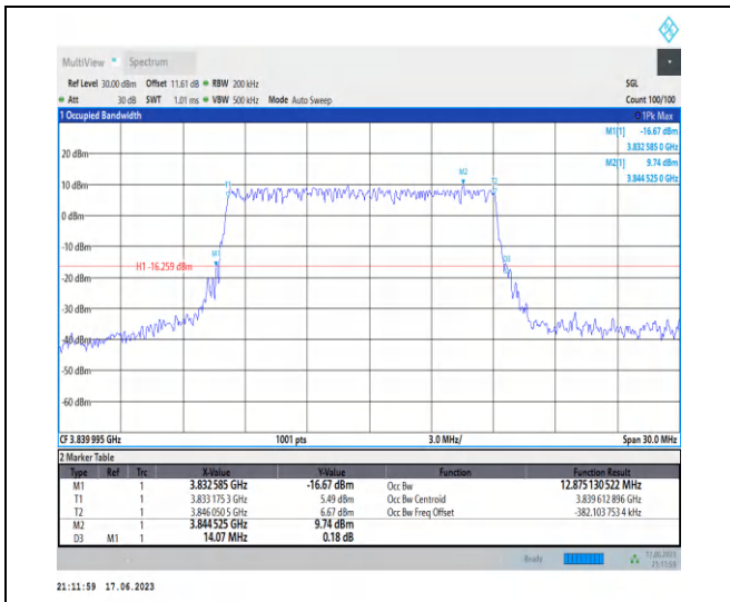
1-N77-3700-3980-PC3-30-15-M-5-DFT-256QAM-Outer_Full-36@0-Ant2-12.875-14.070-≤15-PASS
