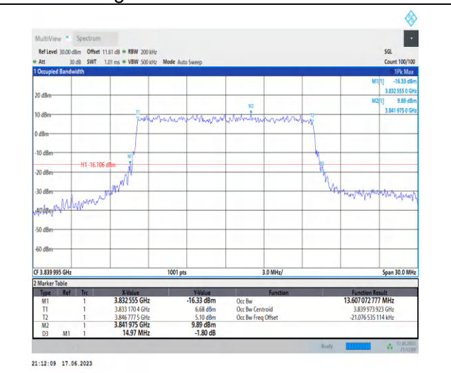
1-N77-3700-3980-PC3-30-15-M-6-CP-QPSK-Outer_Full-38@0-Ant2-13.607-14.970-≤15-PASS
