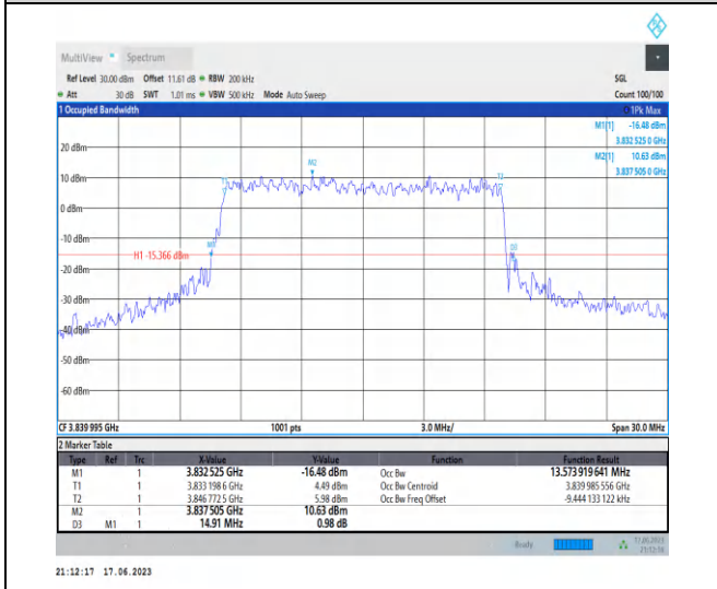
1-N77-3700-3980-PC3-30-15-M-7-CP-16QAM-Outer_Full-38@0-Ant2-13.574-14.910-≤15-PASS
