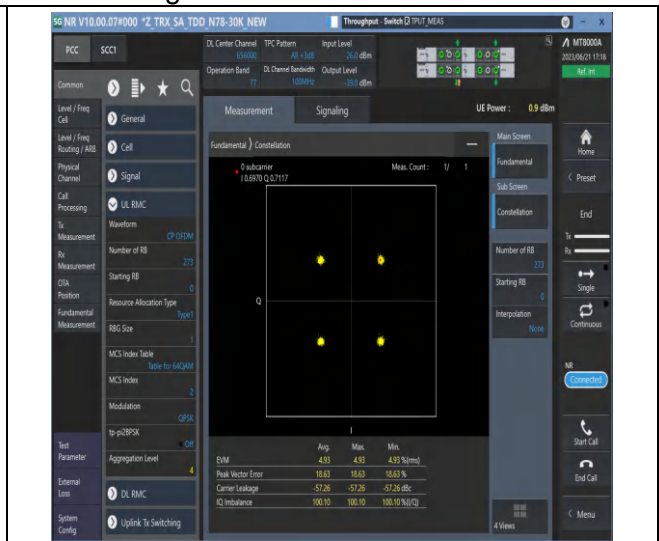
1-N77-3700-3980-PC3-30-100-M-6-CP-QPSK-Outer_Full-273@0-Ant2-see graph-PASS
