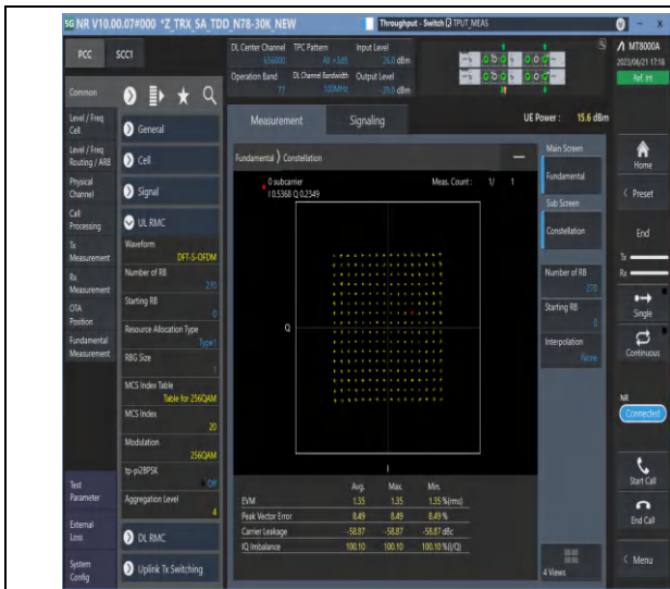
1-N77-3700-3980-PC3-30-100-M-5-DFT-256QAM-Outer_Full-270@0-Ant2-see graph-PASS
