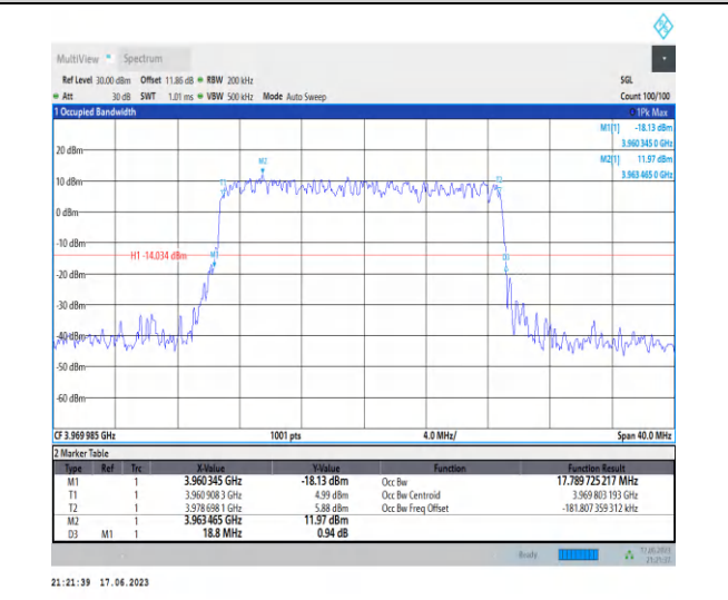
1-N77-3700-3980-PC3-30-20-H-4-DFT-64QAM-Outer_Full-50@0-Ant2-17.79-18.800-≤20-PASS
