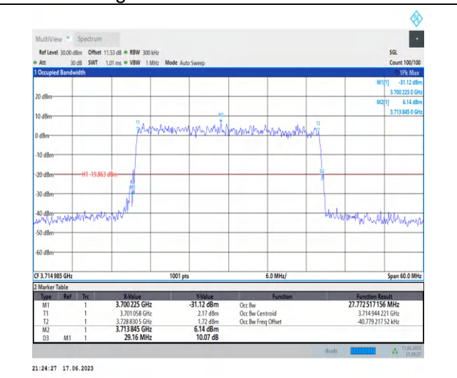
1-N77-3700-3980-PC3-30-30-L-9-CP-256QAM-Outer _Full-78@0-Ant2-27.773-29.160-≤30-PASS
