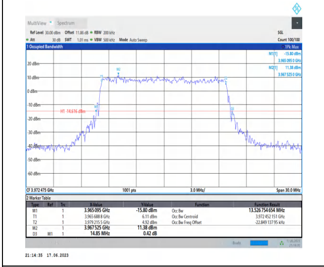
1-N77-3700-3980-PC3-30-15-H-6-CP-QPSK-Outer Full-38@0-Ant2-13.527-14.850-≤15-PASS
