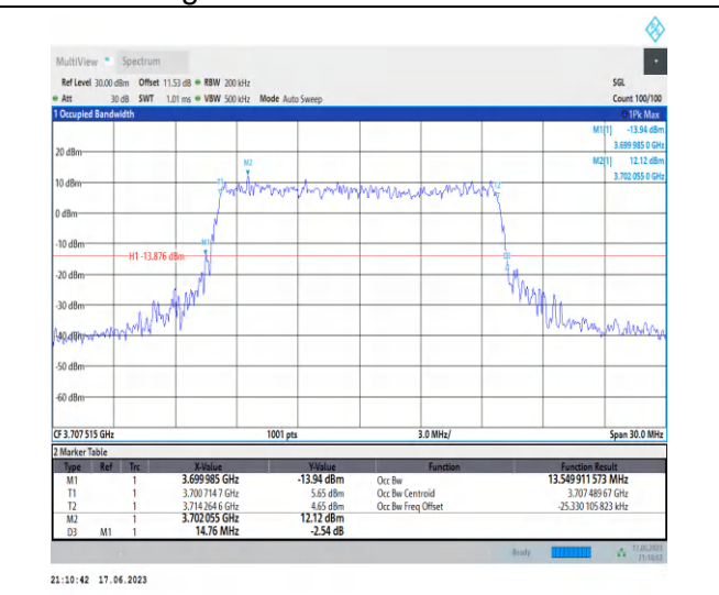
1-N77-3700-3980-PC3-30-15-L-7-CP-16QAM-Outer_Full-38@0-Ant2-13.55-14.760-≤15-PASS
