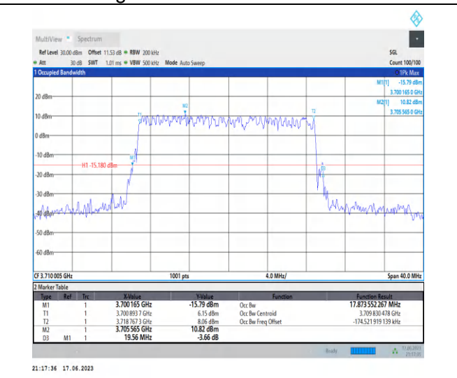
1-N77-3700-3980-PC3-30-20-L-4-DFT-64QAM-Outer_Full-50@0-Ant2-17.874-19.560-≤20-PASS
