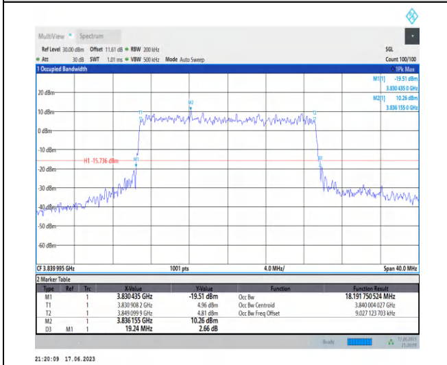
1-N77-3700-3980-PC3-30-20-M-8-CP-64QAM-Outer_Full-51 @0-Ant2-18.192-19.240-≤20-PASS
