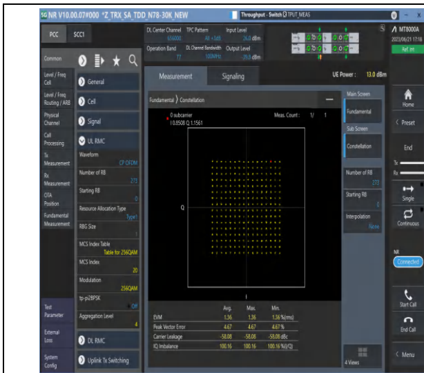
1-N77-3700-3980-PC3-30-100-M-9-CP-256QAM-Outer_Full-273@0-Ant2-see graph-PASS
