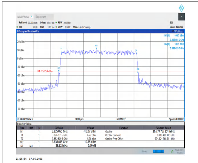
1-N77-3700-3980-PC3-30-30-M-3-DFT-16QAM-Out er_Full-75@0-Ant2-26.778-28.320-≤30-PASS
