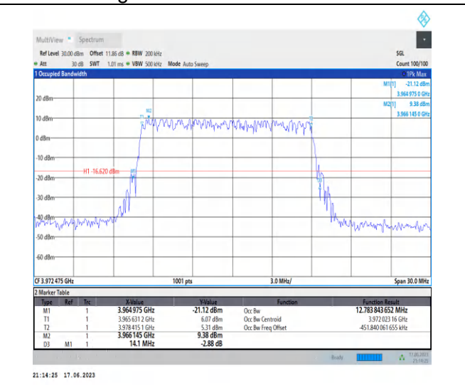
1-N77-3700-3980-PC3-30-15-H-5-DFT-256QAM-Out er_Full-36@0-Ant2-12.784-14.100-≤15-PASS
