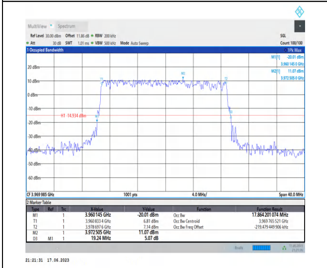
1-N77-3700-3980-PC3-30-20-H-3-DFT-16QAM-Outer_Full-50@0-Ant2-17.864-19.240-≤20-PASS
