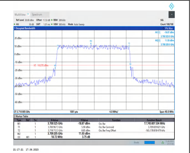
1-N77-3700-3980-PC3-30-20-L-2-DFT-QPSK-Outer_Full-50@0-Ant2-17.745-18.720-≤20-PASS
