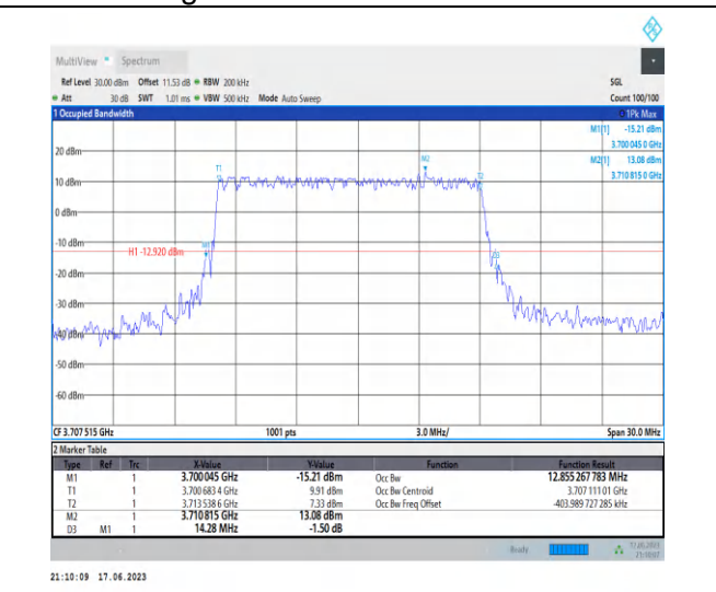
1-N77-3700-3980-PC3-30-15-L-3-DFT-16QAM-Outer_Full-36@0-Ant2-12.855-14.280-≤15-PASS
