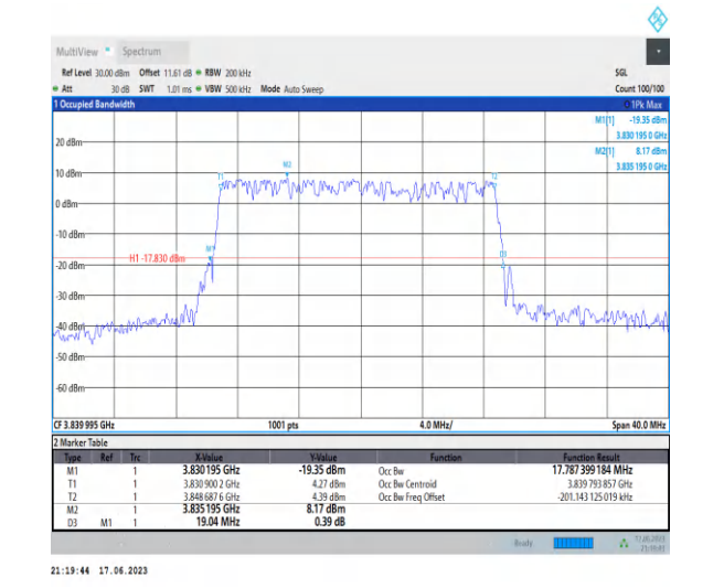
1-N77-3700-3980-PC3-30-20-M-5-DFT-256QAM-Outer_Full-50@0-Ant2-17.787-19.040-≤20-PASS
