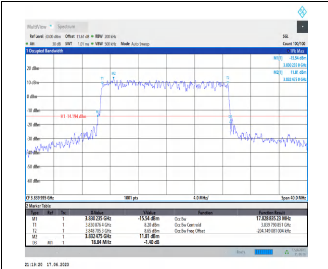
1-N77-3700-3980-PC3-30-20-M-2-DFT-QPSK-Outer_Full-50@0-Ant2-17.829-18.840-≤20-PASS
