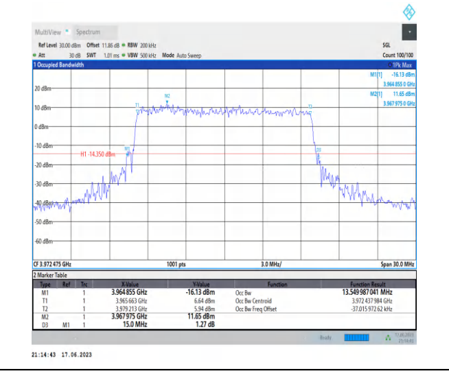
1-N77-3700-3980-PC3-30-15-H-7-CP-16QAM-Outer Full-38@0-Ant2-13.55-15.000-≤15-PASS
