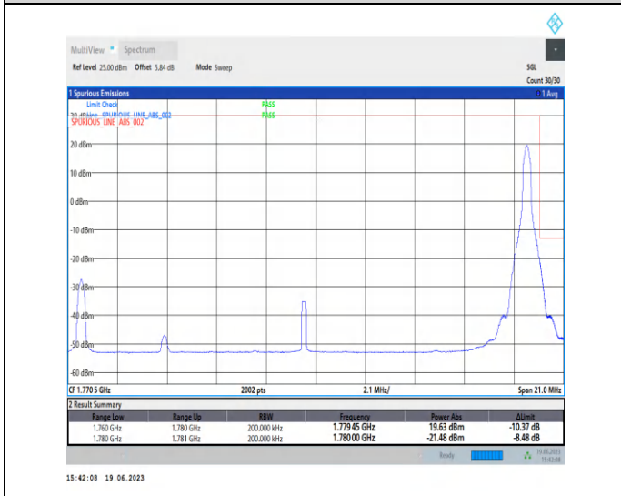
1-N66-PC3-15-20-H-5-CP-QPSK-Edge_1RB_Right-1@105-Ant3-1-seegraph-PASS-see graph
