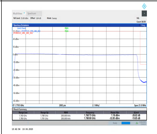
1-N66-PC3-15-20-H-6-CP-QPSK-Outer_Full-106@0-Ant3-1-seegraph-PASS-see graph
