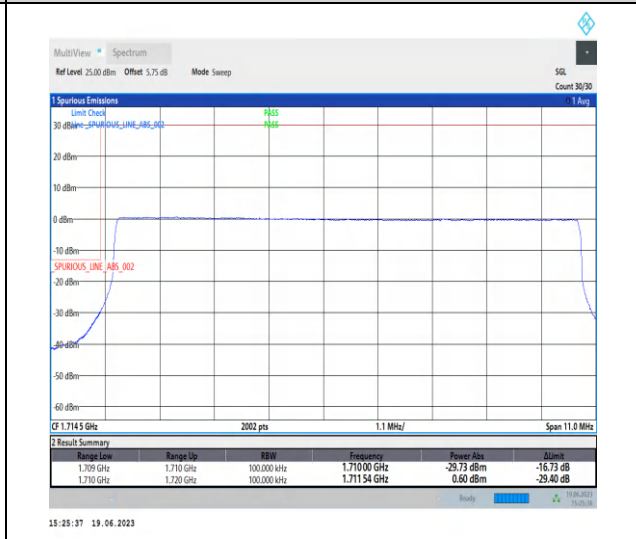
1-N66-PC3-15-10-L-6-CP-QPSK-Outer_Full-52@0-Ant3-1-seegraph-PASS-see graph
