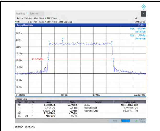
1-N66-PC3-15-30-M-9-CP-256QAM-Outer_Full-160 @0-Ant3-28.612-29.820-≤30-PASS
