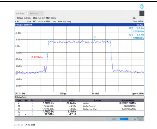
1-N66-PC3-15-30-M-5-DFT-256QAM-Outer_Full-160 @0-Ant3-28.601-29.760-≤30-PASS
