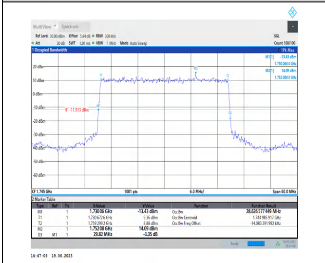
1-N66-PC3-15-30-M-2-DFT-PI2BPSK-Outer_Full-160 @0-Ant3-28.627-29.820-≤30-PASS
