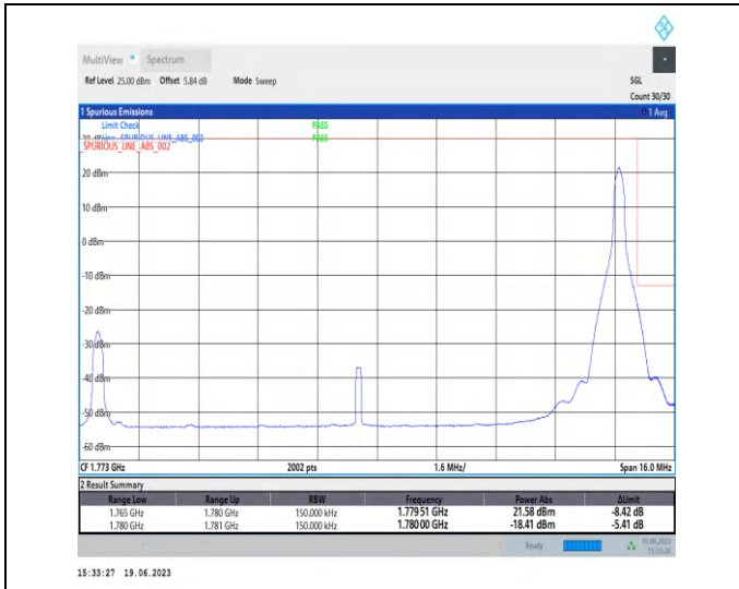
1-N66-PC3-15-15-H-2-DFT-PI2BPSK-Edge_1RB_Right-t-1@78-Ant3-1-seegraph-PASS-see graph
