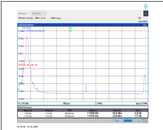
1-N66-PC3-15-20-L-1-DFT-PI2BPSK-Edge_1RB_Left-1@0-Ant3-1-seegraph-PASS-see graph
