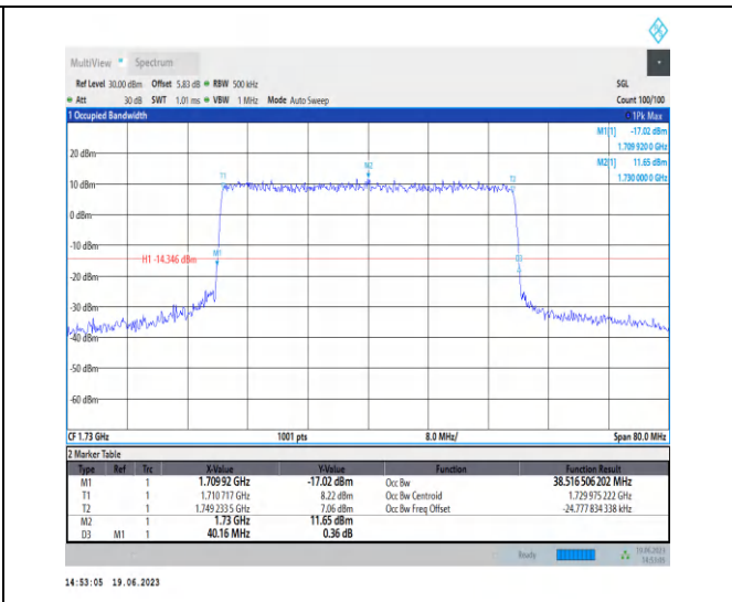
1-N66-PC3-15-40-L-7-CP-16QAM-Outer_Full-216@0 -Ant3-38.517-40.160-<40-PASS
