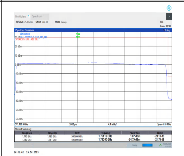
1-N66-PC3-15-40-H-6-CP-QPSK-Outer_Full-216@0-Ant3-1-seegraph-PASS-see graph
