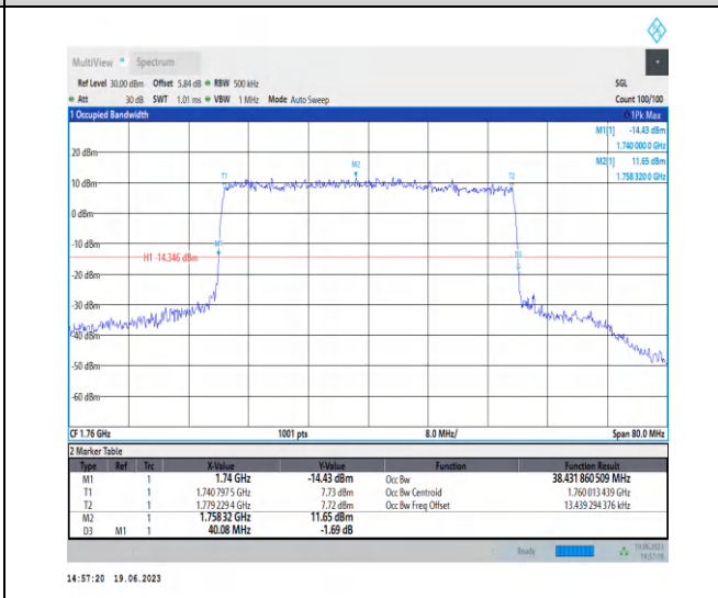
1-N66-PC3-15-40-H-7-CP-16QAM-Outer_Full-216@0 -Ant3-38.432-40.080-<40-PASS
