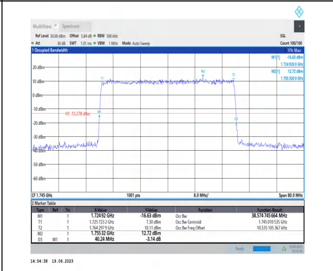
1-N66-PC3-15-40-M-4-DFT-64QAM-Outer_Full-216 @0-Ant3-38.575-40.240-≤40-PASS
