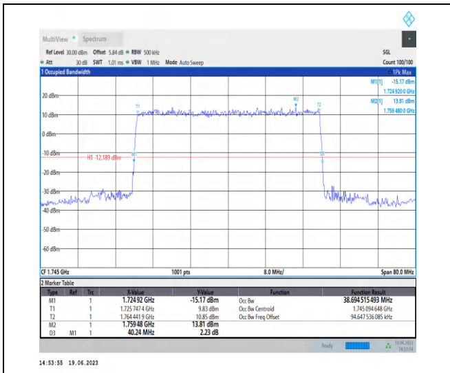
1-N66-PC3-15-40-M-1-DFT-QPSK-Outer_Full-216@ 0-Ant3-38.695-40.240-≤40-PASS
