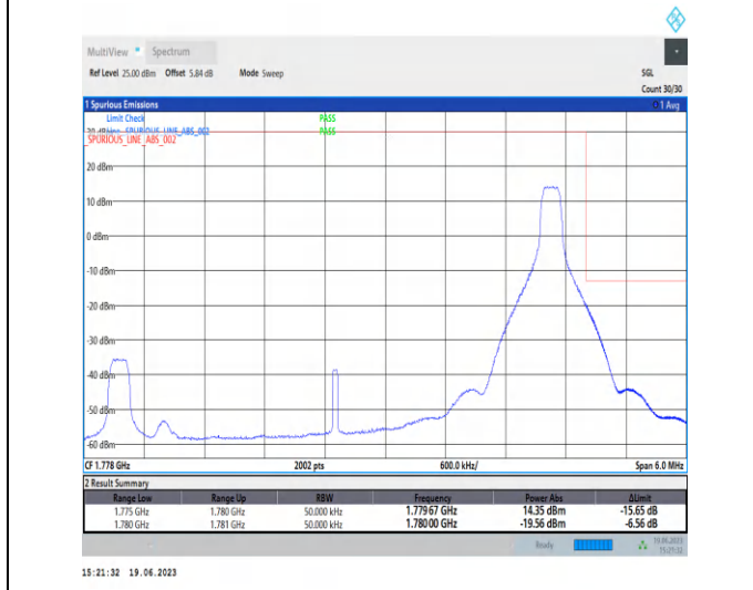
1-N66-PC3-15-5-H-5-CP-QPSK-Edge_1RB_Right-1@ 24-Ant3-1-seegraph-PASS-see graph
