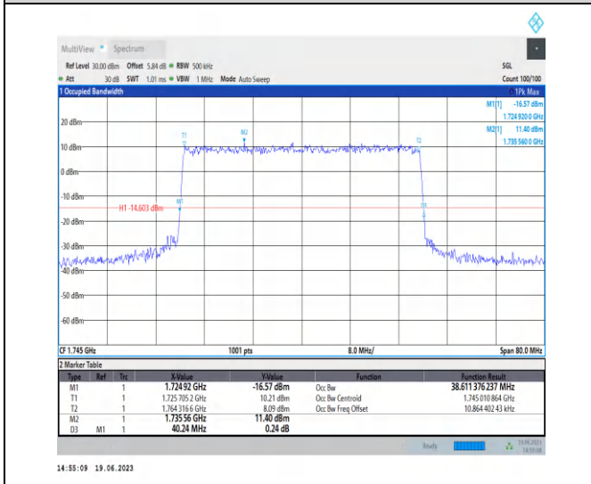
1-N66-PC3-15-40-M-7-CP-16QAM-Outer_Full-216 @0-Ant3-38.611-40.240-≤40-PASS
