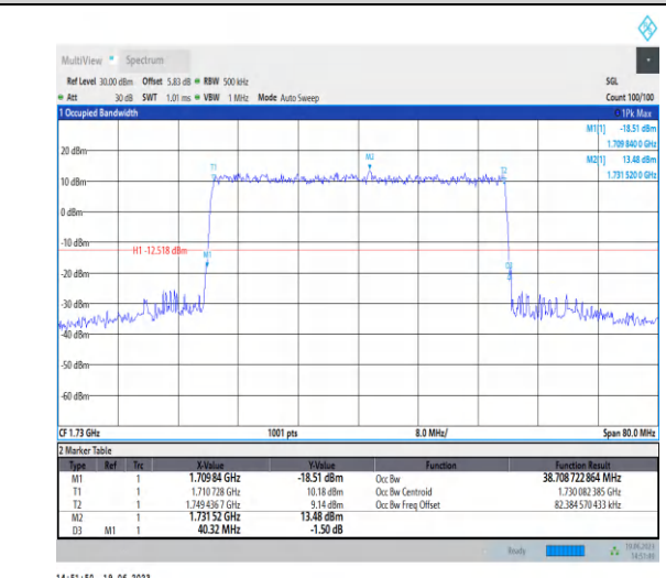
1-N66-PC3-15-40-L-1-DFT-QPSK-Outer_Full-216@ 0-Ant3-38.709-40.320-≤40-PASS
