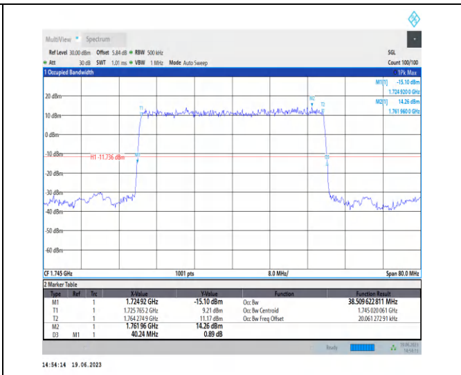
1-N66-PC3-15-40-M-2-DFT-PI2BPSK-Outer_Full-216 @0-Ant3-38.51-40.240-≤40-PASS
