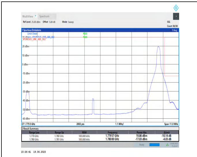
1-N66-PC3-15-10-H-2-DFT-PI2BPSK-Edge_1RB_Right-t-1@51-Ant3-1-seegraph-PASS-see graph
