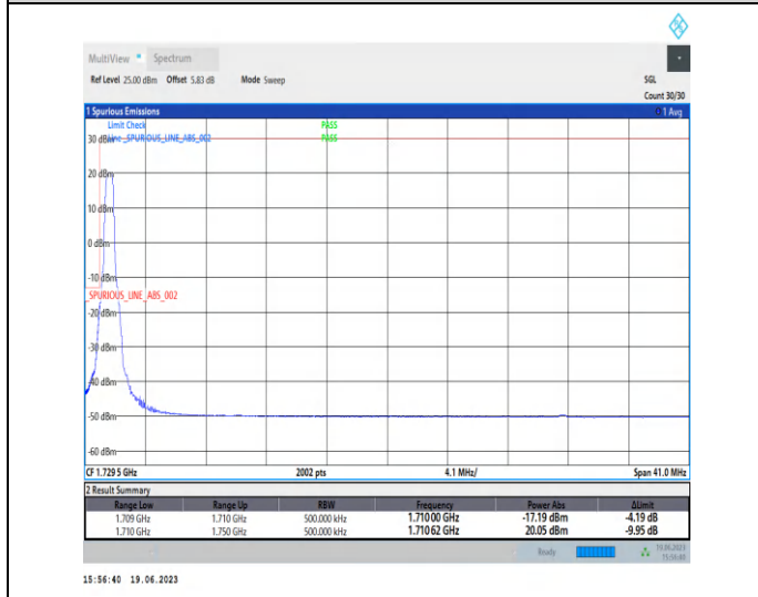
1-N66-PC3-15-40-L-4-CP-QPSK-Edge_1RB_Left-1@0-Ant3-1-seegrph-PASS-see graph
