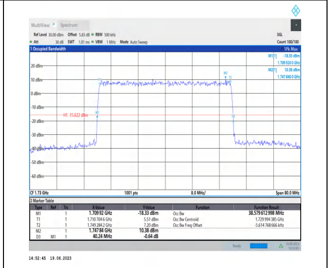
1-N66-PC3-15-40-L-5-DFT-256QAM-Outer_Full-216 @0-Ant3-38.58-40.240-<40-PASS
