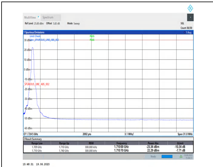
1-N66-PC3-15-30-L-1-DFT-PI2BPSK-Edge_1RB_Left-1@0-Ant3-1-seegrph-PASS-see graph
