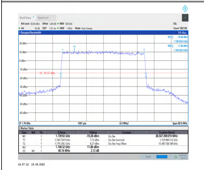
1-N66-PC3-15-40-H-6-CP-QPSK-Outer_Full-216@0 -Ant3-38.507-40.160-<40-PASS
