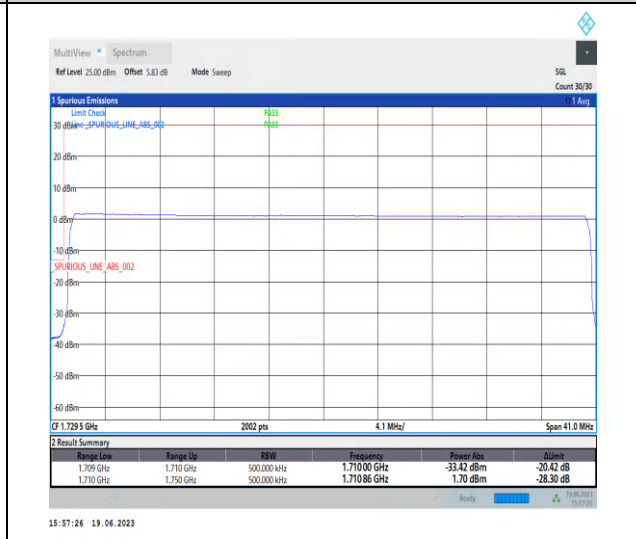
1-N66-PC3-15-40-L-6-CP-QPSK-Outer_Full-216@0-Ant3-1-seegrph-PASS-see graph
