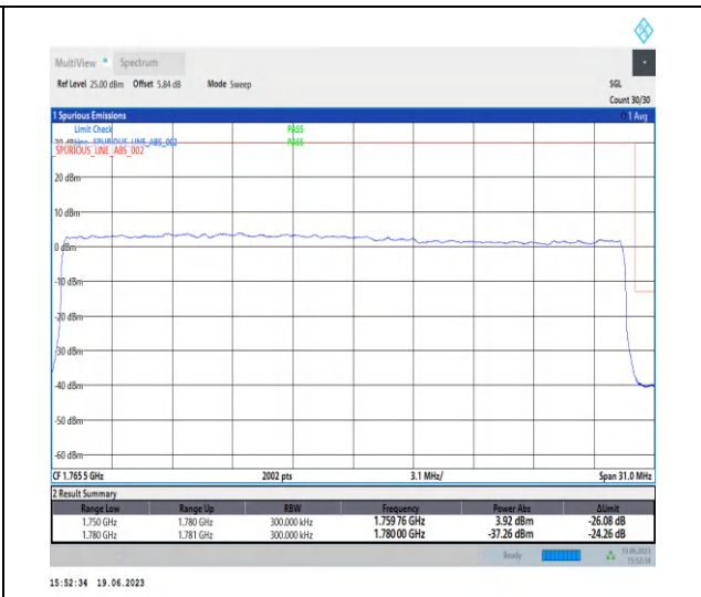
1-N66-PC3-15-30-H-3-DFT-PI2BPSK-Outer_Full-160@0-Ant3-1-seegraph-PASS-see graph
