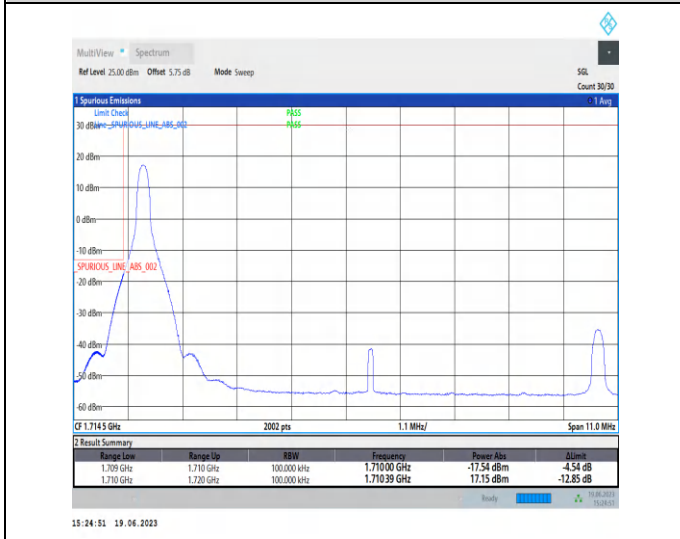
1-N66-PC3-15-10-L-4-CP-QPSK-Edge_1RB_Left-1@0-Ant3-1-seegraph-PASS-see graph
