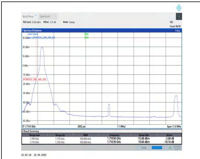
1-N66-PC3-15-10-L-1-DFT-PI2BPSK-Edge_1RB_Left-1@0-Ant3-1-seegraph-PASS-see graph
