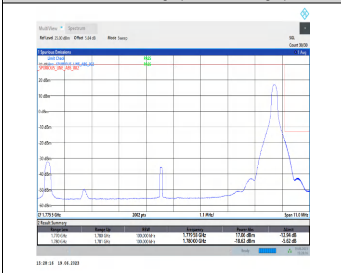
1-N66-PC3-15-10-H-5-CP-QPSK-Edge_1RB_Right-1@51-Ant3-1-seegraph-PASS-see graph
