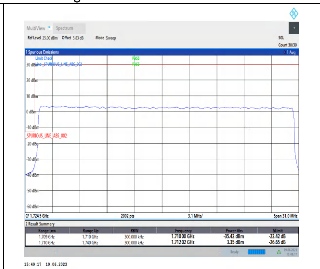
1-N66-PC3-15-30-L-3-DFT-PI2BPSK-Outer_Full-160@0-Ant3-1-seegrph-PASS-see graph
