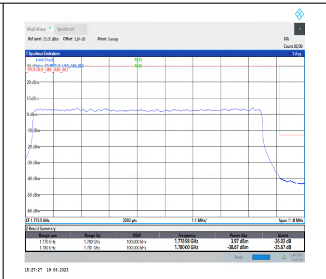
1-N66-PC3-15-10-H-3-DFT-PI2BPSK-Outer_Full-50@0-Ant3-1-seegraph-PASS-see graph
