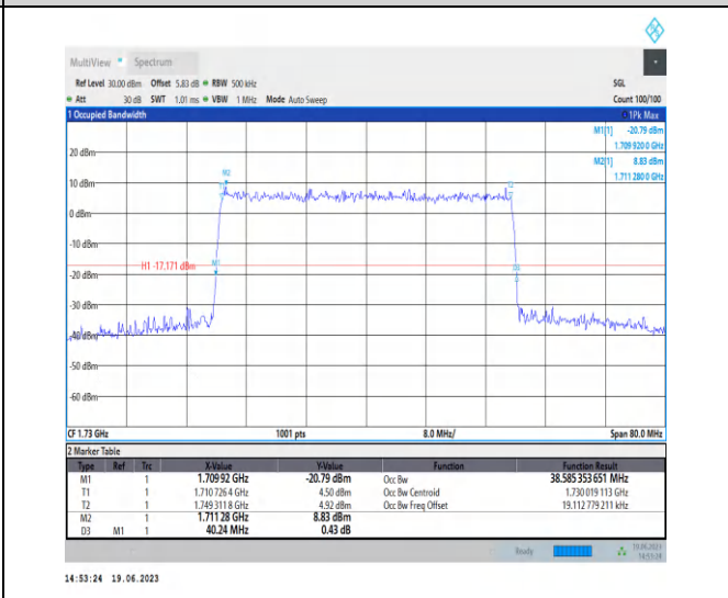
1-N66-PC3-15-40-L-9-CP-256QAM-Outer_Full-216@0 -Ant3-38.585-40.240-<40-PASS
