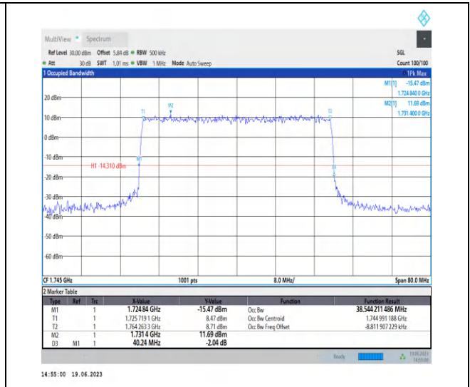
1-N66-PC3-15-40-M-6-CP-QPSK-Outer_Full-216 @0-Ant3-38.544-40.240-≤40-PASS
