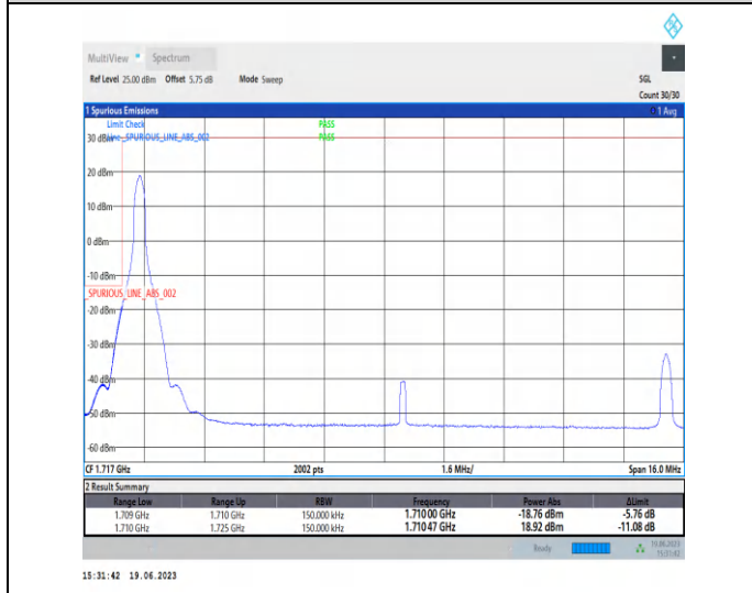
1-N66-PC3-15-15-L-4-CP-QPSK-Edge_1RB_Left-1@0-Ant3-1-seegraph-PASS-see graph
