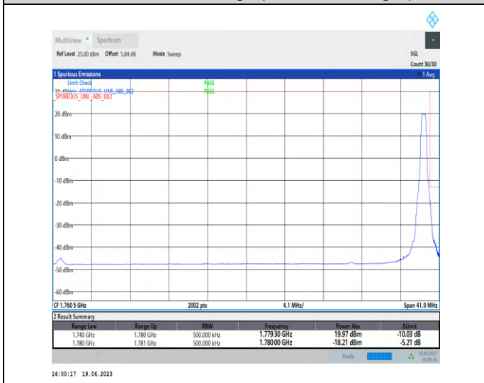
1-N66-PC3-15-40-H-5-CP-QPSK-Edge_1RB_Right-1@215-Ant3-1-seegraph-PASS-see graph
