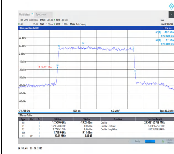
1-N66-PC3-15-30-H-5-DFT-256QAM-Outer_Full-160 @0-Ant3-28.548-29.940-<30-PASS
