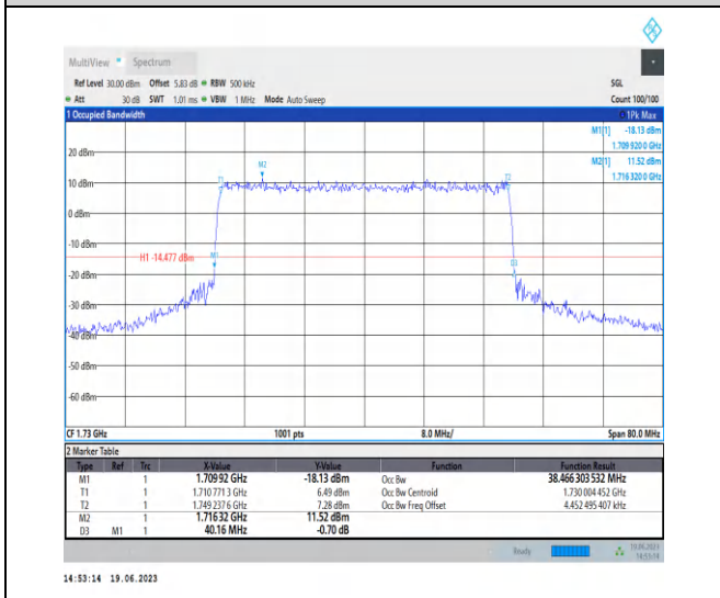
1-N66-PC3-15-40-L-8-CP-64QAM-Outer_Full-216@0 -Ant3-38.466-40.160-<40-PASS
