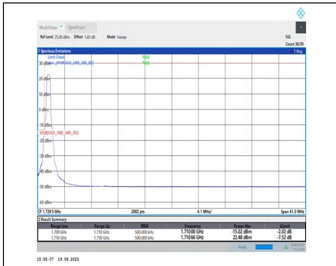
1-N66-PC3-15-40-L-1-DFT-PI2BPSK-Edge_1RB_Left-1@0-Ant3-1-seegrph-PASS-see graph
