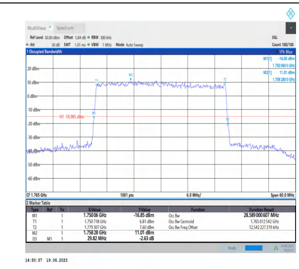
1-N66-PC3-15-30-H-4-DFT-64QAM-Outer_Full-160 @0-Ant3-28.589-29.820-<30-PASS
