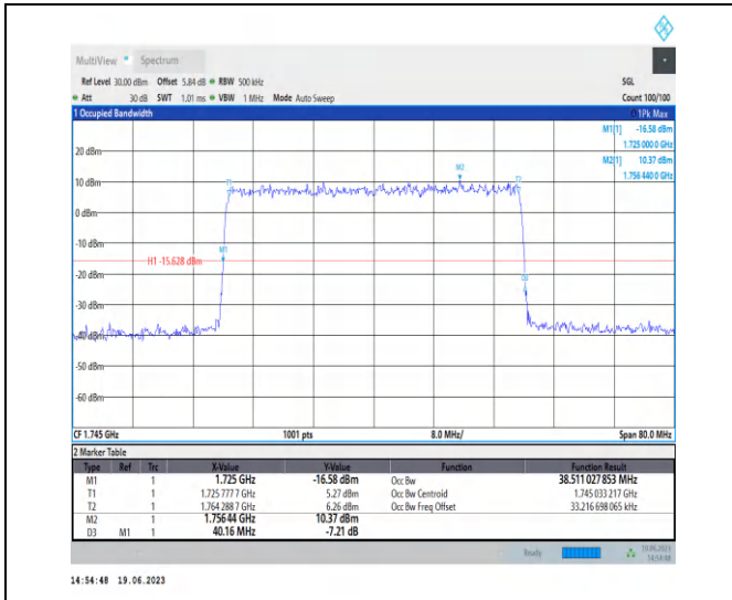
1-N66-PC3-15-40-M-5-DFT-256QAM-Outer_Full-216 @0-Ant3-38.511-40.160-≤40-PASS
