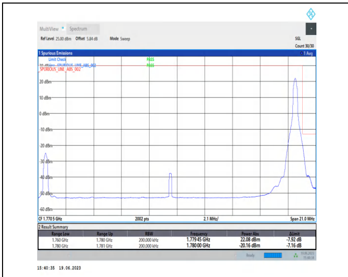
1-N66-PC3-15-20-H-2-DFT-PI2BPSK-Edge_1RB_Right-t-1@105-Ant3-1-seegraph-PASS-see graph
