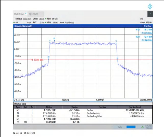
1-N66-PC3-15-30-L-8-CP-64QAM-Outer_Full-160@0 -Ant3-28.592-29.820-≤30-PASS
