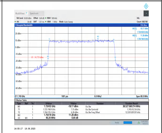
1-N66-PC3-15-40-M-8-CP-64QAM-Outer_Full-216 @0-Ant3-38.527-40.240-≤40-PASS
