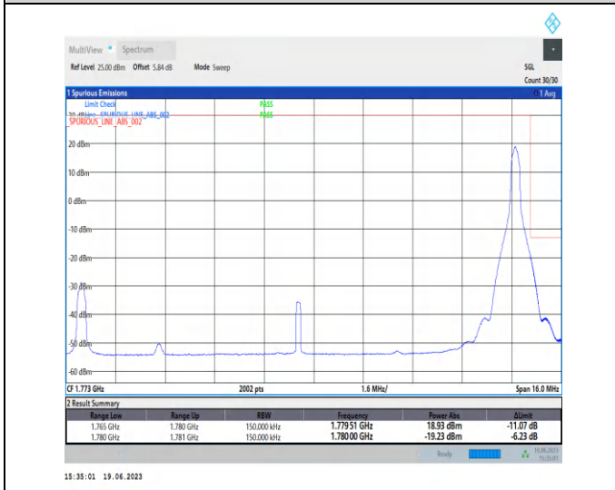
1-N66-PC3-15-15-H-5-CP-QPSK-Edge_1RB_Right-1@78-Ant3-1-seegraph-PASS-see graph
