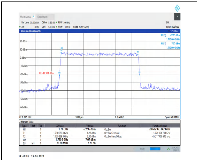
1-N66-PC3-15-30-L-9-CP-256QAM-Outer_Full-160@ 0-Ant3-28.608-29.880-≤30-PASS
