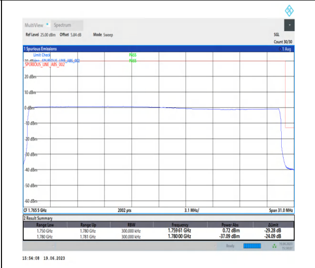
1-N66-PC3-15-30-H-6-CP-QPSK-Outer_Full-160@0-Ant3-1-seegraph-PASS-see graph
