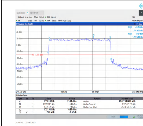
1-N66-PC3-15-30-L-7-CP-16QAM-Outer_Full-160@0 -Ant3-28.628-29.700-≤30-PASS
