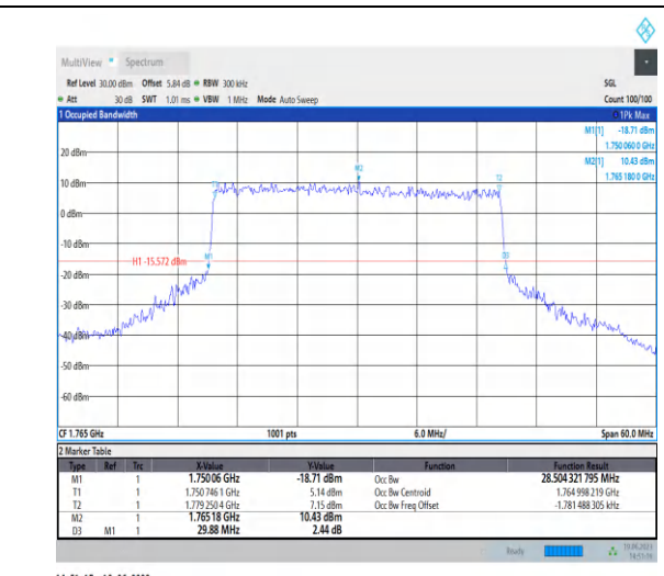
1-N66-PC3-15-30-H-8-CP-64QAM-Outer_Full-160@ 0-Ant3-28.504-29.880-≤30-PASS
