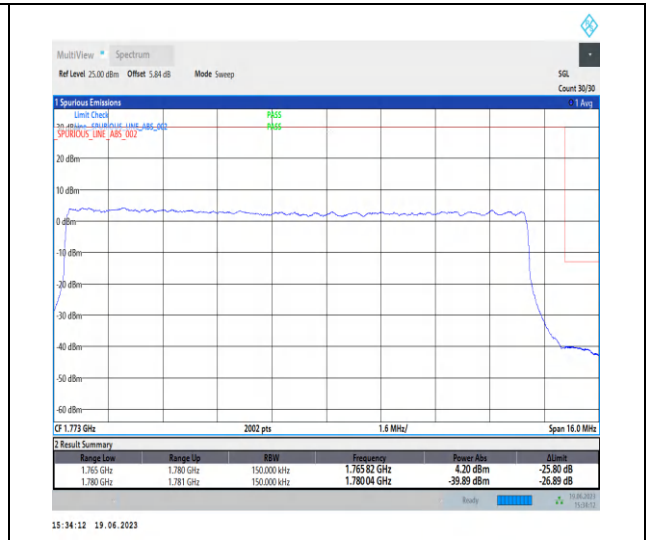
1-N66-PC3-15-15-H-3-DFT-PI2BPSK-Outer_Full-75@0-Ant3-1-seegraph-PASS-see graph
