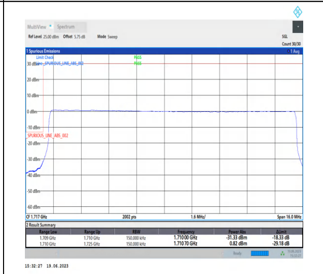
1-N66-PC3-15-15-L-6-CP-QPSK-Outer_Full-79@0-Ant3-1-seegraph-PASS-see graph
