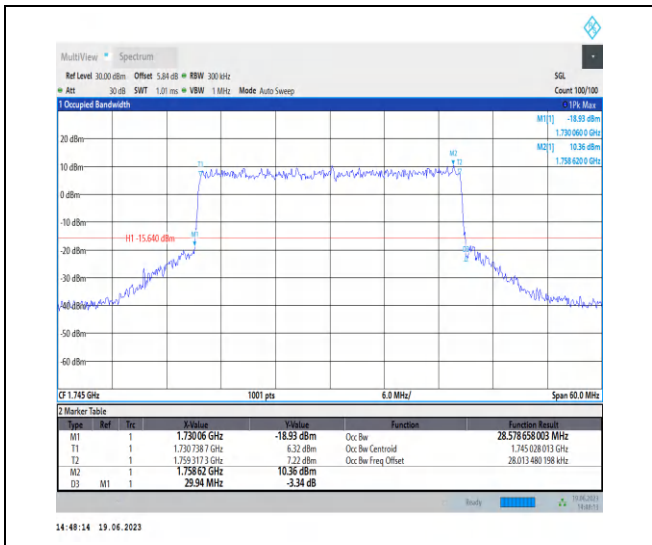
1-N66-PC3-15-30-M-8-CP-64QAM-Outer_Full-160 @0-Ant3-28.579-29.940-≤30-PASS
