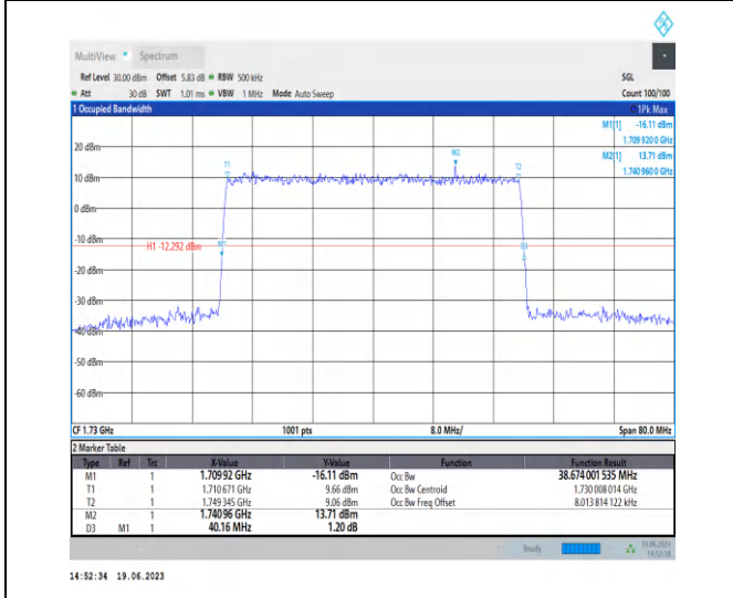
1-N66-PC3-15-40-L-4-DFT-64QAM-Outer_Full-216 @ 0-Ant3-38.674-40.160-<40-PASS
