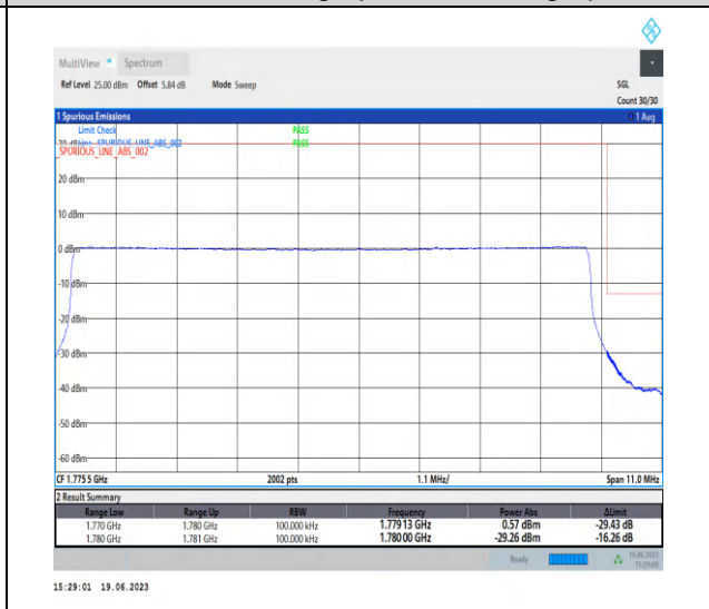
1-N66-PC3-15-10-H-6-CP-QPSK-Outer_Full-52@0-Ant3-1-seegraph-PASS-see graph
