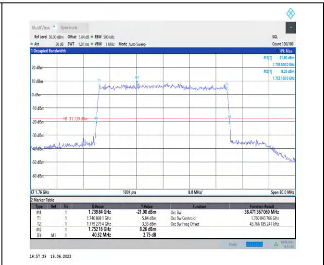
1-N66-PC3-15-40-H-9-CP-256QAM-Outer_Full-216 @0-Ant3-38.471-40.320-<40-PASS
