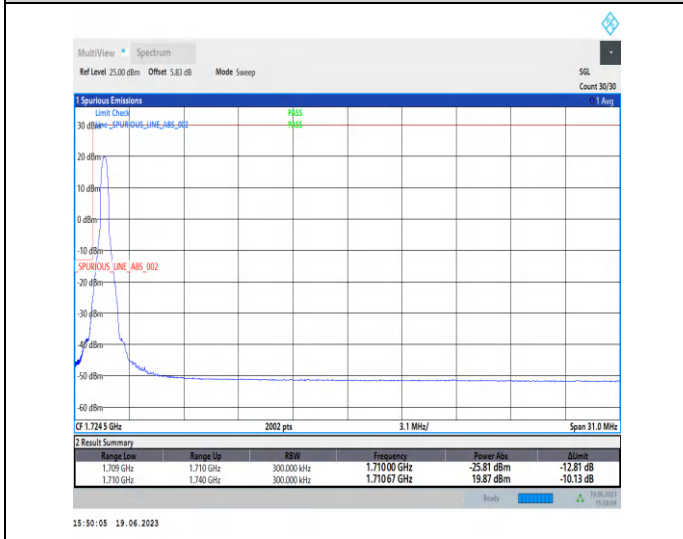
1-N66-PC3-15-30-L-4-CP-QPSK-Edge_1RB_Left-1@0-Ant3-1-seegrph-PASS-see graph
