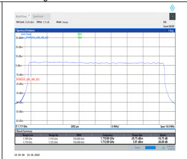
1-N66-PC3-15-15-L-3-DFT-PI2BPSK-Outer_Full-75@0-Ant3-1-seegraph-PASS-see graph
