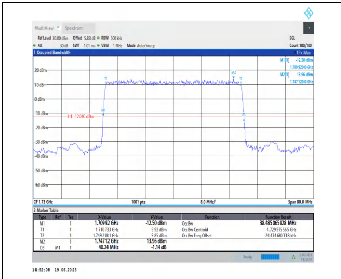
1-N66-PC3-15-40-L-2-DFT-PI2BPSK-Outer_Full-216 @0-Ant3-38.485-40.240-<40-PASS
