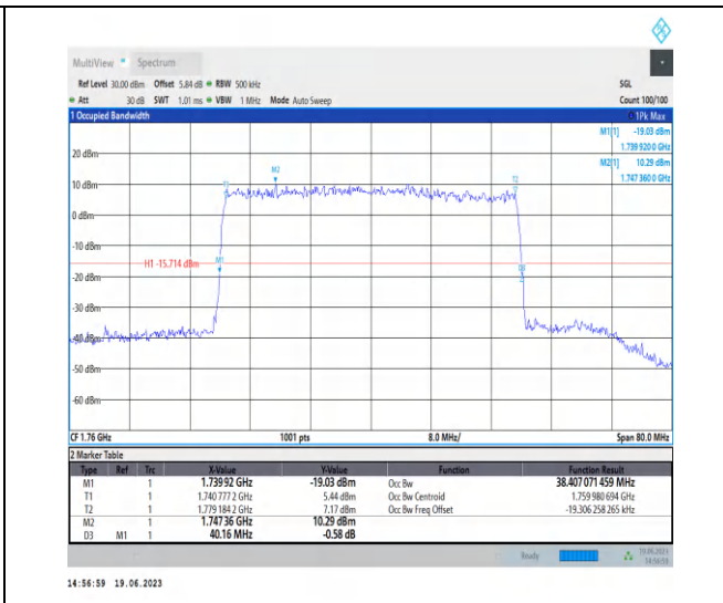
1-N66-PC3-15-40-H-5-DFT-256QAM-Outer_Full-216 @0-Ant3-38.407-40.160-<40-PASS
