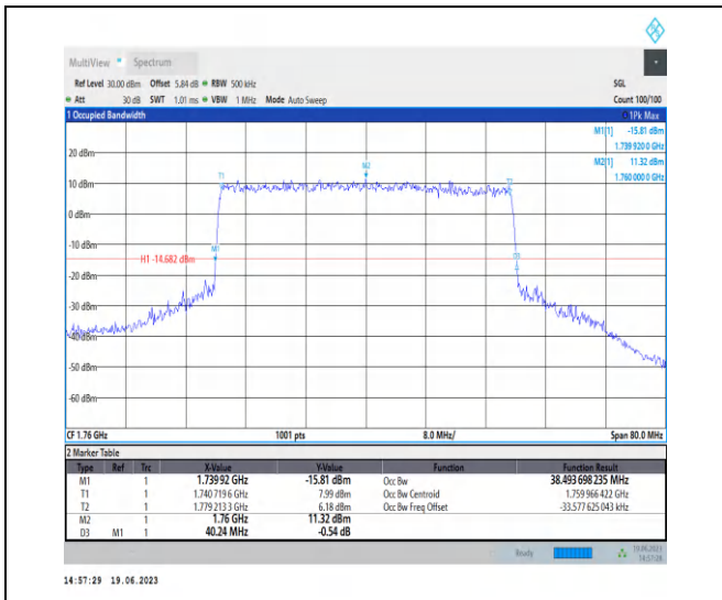
1-N66-PC3-15-40-H-8-CP-64QAM-Outer_Full-216@ 0-Ant3-38.494-40.240-<40-PASS
