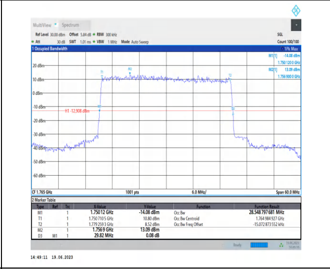
1-N66-PC3-15-30-H-2-DFT-P12BPSK-Outer_Full-160 @0-Ant3-28.549-29.820-≤30-PASS
