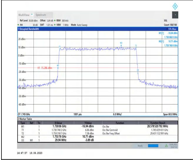
1-N66-PC3-15-30-M-6-CP-QPSK-Outer_Full-160 @0-Ant3-28.579-29.940-≤30-PASS
