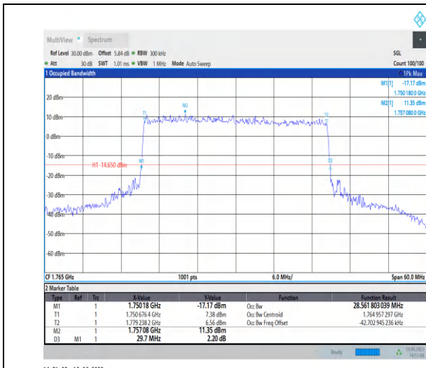
1-N66-PC3-15-30-H-7-CP-16QAM-Outer_Full-160@ 0-Ant3-28.562-29.700-≤30-PASS
