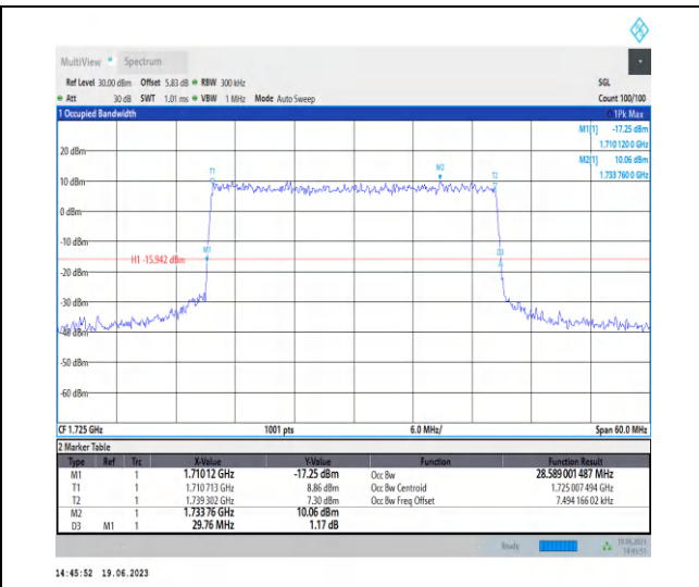
1-N66-PC3-15-30-L-6-CP-QPSK-Outer_Full-160@0 -Ant3-28.589-29.760-≤30-PASS
