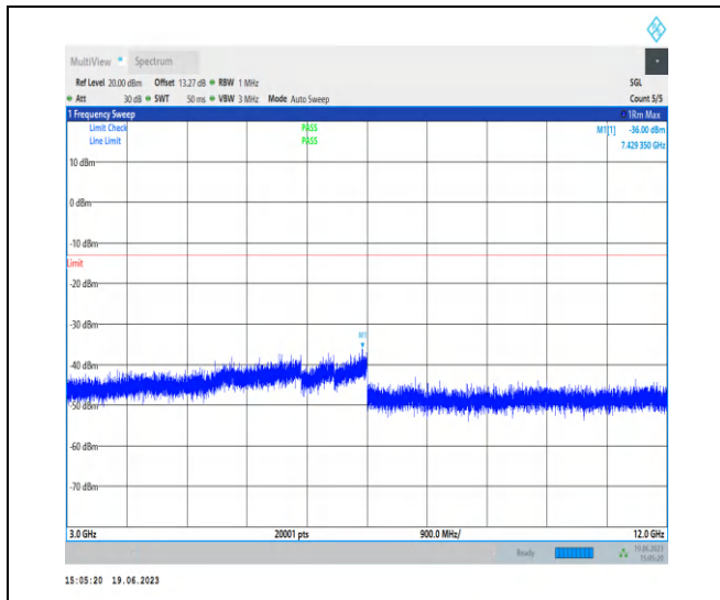
1-N66-PC3-15-40-H-1-DFT-PI2BPSK-Inner_1RB_L eft-1 @ 1-3000-12000-Ant3-7429.35--36.00--13-PAS S
