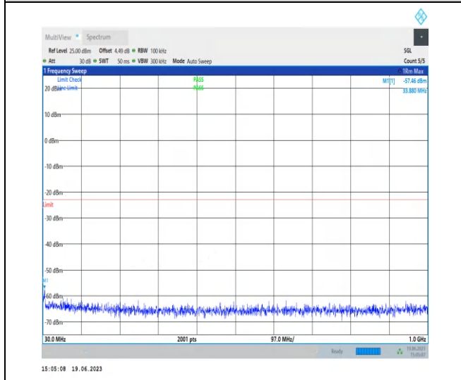
1-N66-PC3-15-40-H-1-DFT-PI2BPSK-Inner_1RB_L eft-1@1-30-1000-Ant3-33.88--57.46--23-PASS
