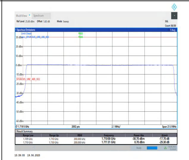
1-N66-PC3-15-20-L-6-CP-QPSK-Outer_Full-106@0-Ant3-1-seegraph-PASS-see graph
