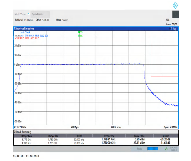
1-N66-PC3-15-5-H-6-CP-QPSK-Outer_Full-25@0-Ant3-1-seegraph-PASS-see graph
