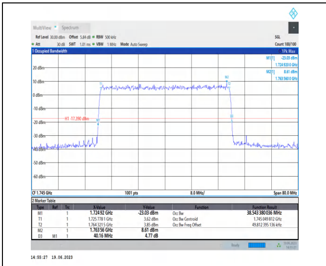
1-N66-PC3-15-40-M-9-CP-256QAM-Outer_Full-216 @0-Ant3-38.543-40.160-<40-PASS
