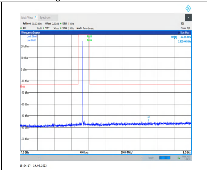
1-N66-PC3-15-40-M-1-DFT-PI2BPSK-Inner_1RB_L ef t-1 @ 1-1000-3000-Ant3-2502.00--44.81--13-PASS
