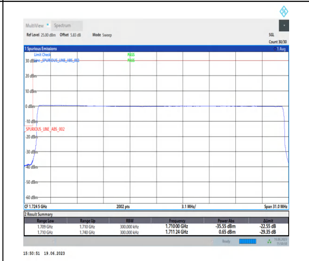
1-N66-PC3-15-30-L-6-CP-QPSK-Outer_Full-160@0-Ant3-1-seegrph-PASS-see graph
