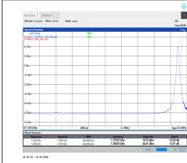
1-N66-PC3-15-30-H-5-CP-QPSK-Edge_1RB_Right-1@159-Ant3-1-seegraph-PASS-see graph
