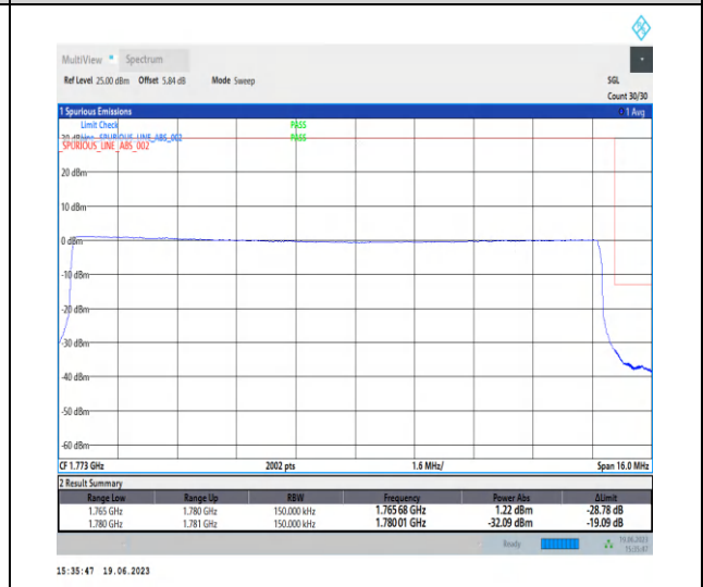
1-N66-PC3-15-15-H-6-CP-QPSK-Outer_Full-79@0-Ant3-1-seegraph-PASS-see graph
