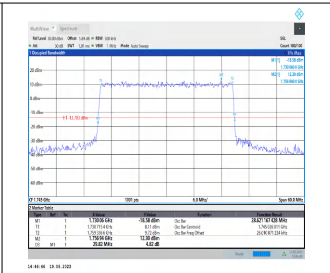
1-N66-PC3-15-30-M-1-DFT-QPSK-Outer_Full-160@ 0-Ant3-28.621-29.820-≤30-PASS
