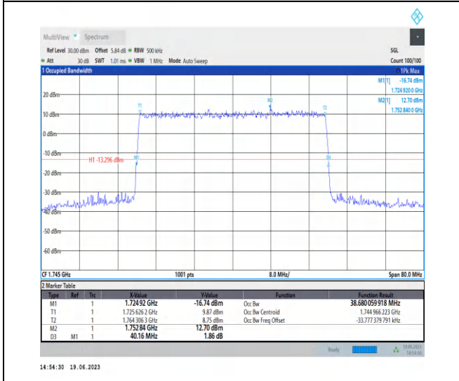
1-N66-PC3-15-40-M-3-DFT-16QAM-Outer_Full-216 @0-Ant3-38.68-40.160-≤40-PASS
