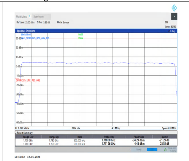
1-N66-PC3-15-40-L-3-DFT-PI2BPSK-Outer_Full-216@0-Ant3-1-seegrph-PASS-see graph
