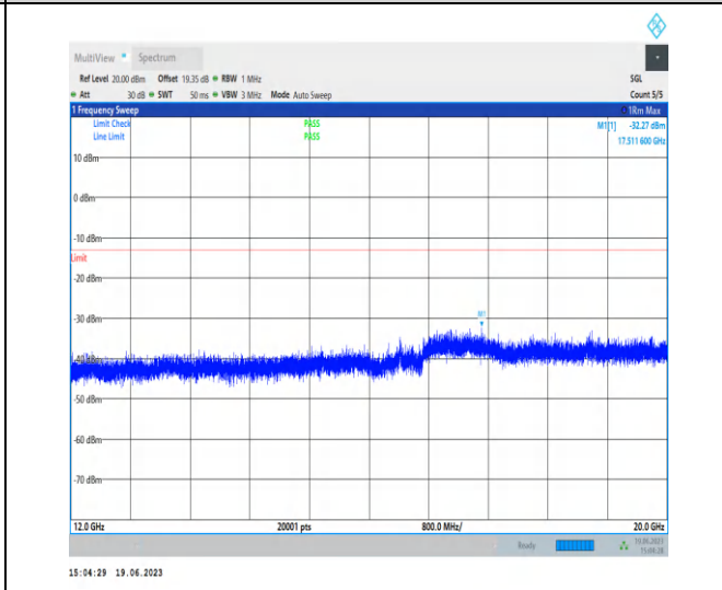
1-N66-PC3-15-40-M-1-DFT-PI2BPSK-Inner_1RB_L ef t-1 @ 1-12000-20000-Ant3-17511.60--32.27--13-PASS
