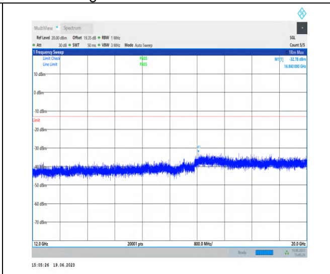
1-N66-PC3-15-40-H-1-DFT-PI2BPSK-Inner_1RB_L ef t-1 @ 1-12000-20000-Ant3-16840.00--32.78--13-PASS
