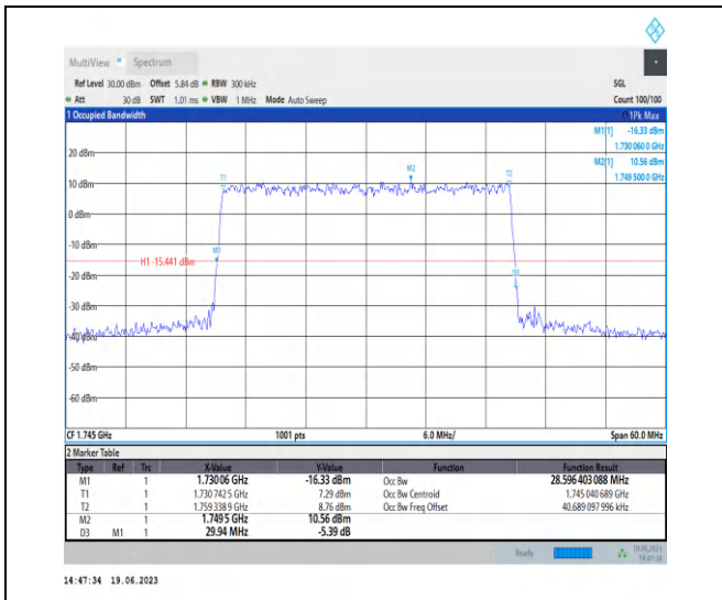
1-N66-PC3-15-30-M-4-DFT-64QAM-Outer_Full-160 @0-Ant3-28.596-29.940-≤30-PASS
