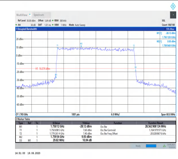
1-N66-PC3-15-30-H-6-CP-QPSK-Outer_Full-160 @0 -Ant3-28.563-29.820-<30-PASS
