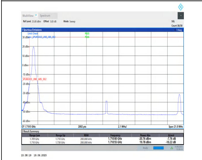
1-N66-PC3-15-20-L-4-CP-QPSK-Edge_1RB_Left-1@0-Ant3-1-seegraph-PASS-see graph
