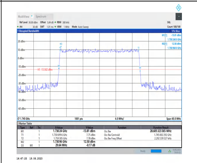
1-N66-PC3-15-30-M-3-DFT-16QAM-Outer_Full-160 @0-Ant3-28.605-29.640-≤30-PASS
