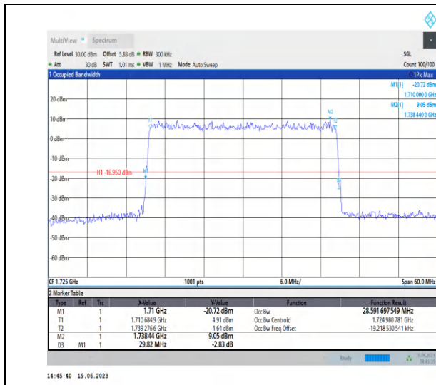
1-N66-PC3-15-30-L-5-DFT-256QAM-Outer_Full-160 @0-Ant3-28.592-29.820-≤30-PASS
