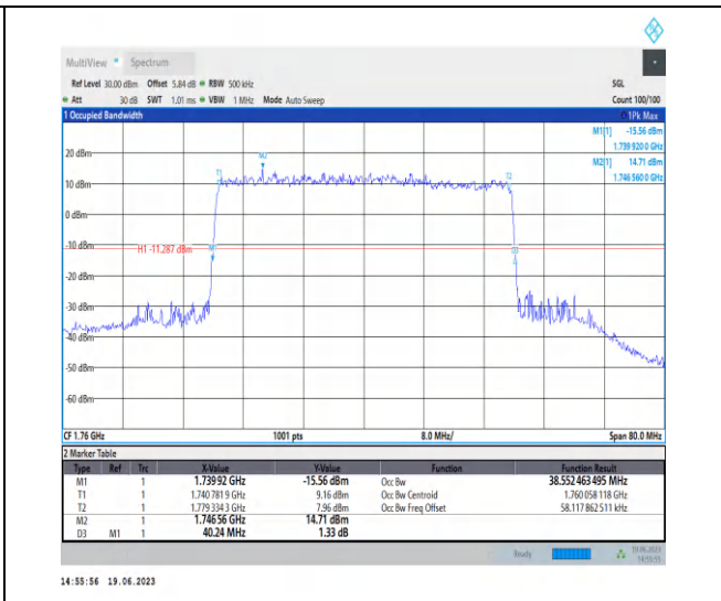
1-N66-PC3-15-40-H-1-DFT-QPSK-Outer_Full-216 @0-Ant3-38.552-40.240-<40-PASS
