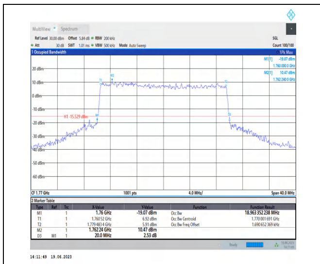
1-N66-PC3-15-20-H-6-CP-QPSK-Outer_Full-106@0 -Ant3-18.963-20.000-≤20-PASS
