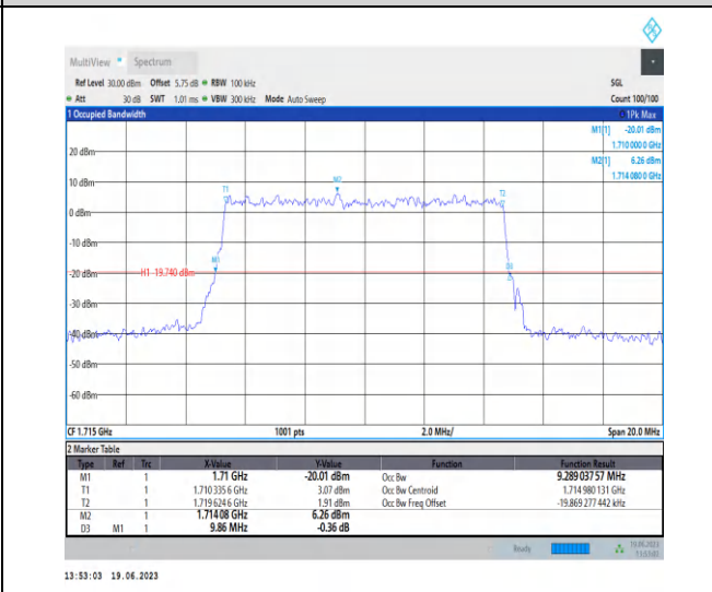
1-N66-PC3-15-10-L-9-CP-256QAM-Outer_Full-52@0 -Ant3-9.289-9.860-≤10-PASS
