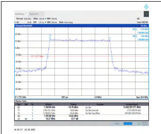
1-N66-PC3-15-15-H-1-DFT-QPSK-Outer_Full-75@0-Ant3-13.464-14.370≤15-PASS
