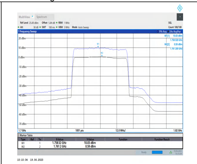
1-N66-PC3-15-40-H-2-CP-256QAM-Outer_Full-216 @0-Ant3-9.44-100%-0.00-9.44-PASS-≤13
