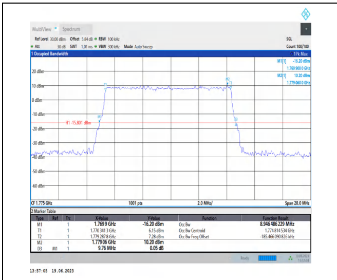
1-N66-PC3-15-10-H-4-DFT-64QAM-Outer_Full-50@ 0-Ant3-8.946-9.760-≤10-PASS
