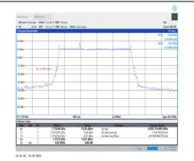
1-N66-PC3-15-10-L-1-DFT-QPSK-Outer_Full-50@0- Ant3-8.925-9.620-≤10-PASS
