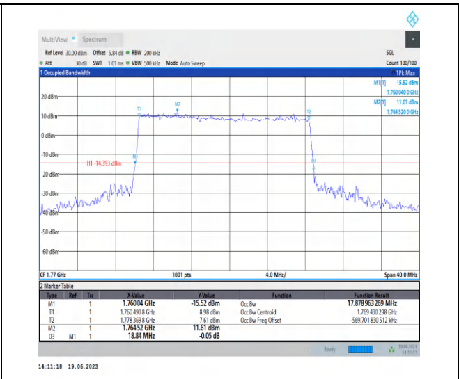
1-N66-PC3-15-20-H-3-DFT-16QAM-Outter_Full-100 @0-Ant3-17.879-18.840-<=20-PASS
