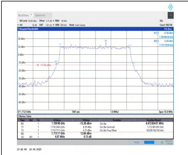
1-N66-PC3-15-5-L-1-DFT-QPSK-Outer_Full-25@0-A nt3-4.473-4.970- \leq 5 -PASS
