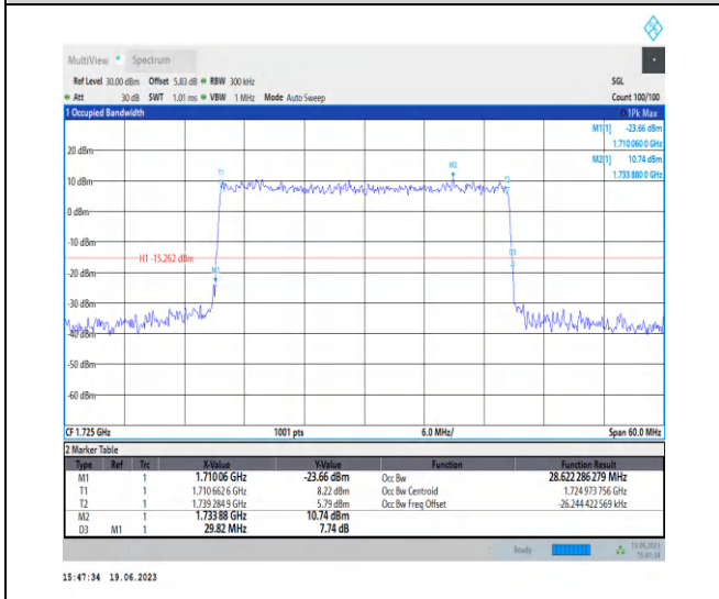
1-N66-PC3-15-30-L-3-DFT-16QAM-Outer_Full-160 @0-Ant3-28.622-29.820-<=30-PASS
