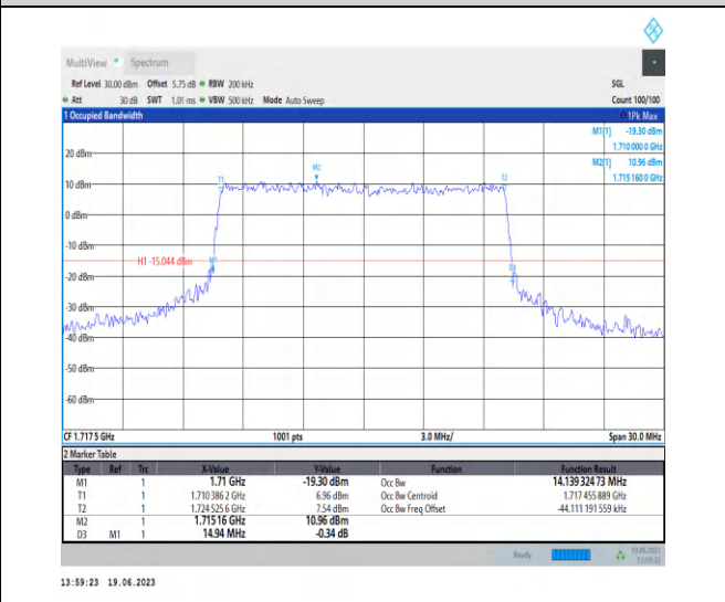
1-N66-PC3-15-15-L-6-CP-QPSK-Outer_Full-79@0-A nt3-14.139-14.940≤15-PASS
