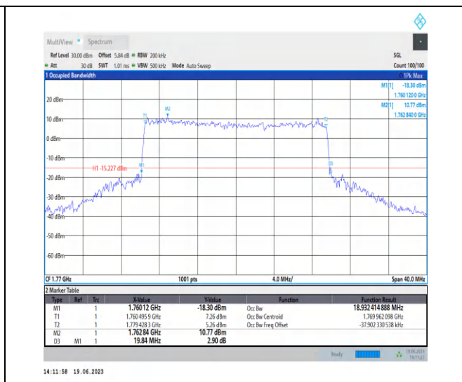
1-N66-PC3-15-20-H-7-CP-16QAM-Outer_Full-106@0 -Ant3-18.932-19.840-≤20-PASS
