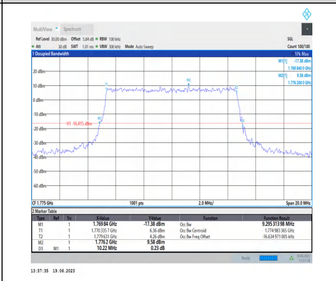
1-N66-PC3-15-10-H-7-CP-16QAM-Outer_Full-52@0- Ant3-9.295-10.220-≤10-PASS
