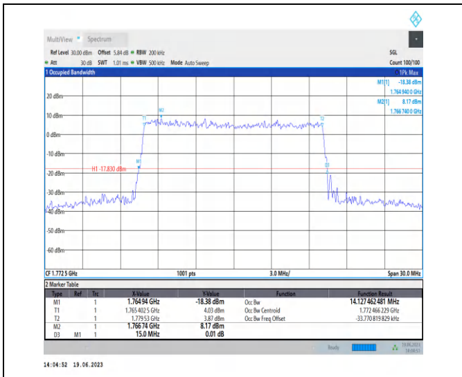
1-N66-PC3-15-15-H-9-CP-256QAM-Outer_Full-79@ 0-Ant3-14.127-15.000-<=15-PASS
