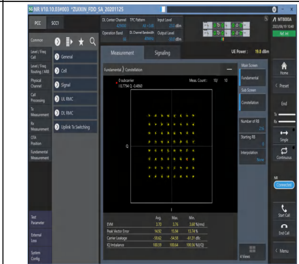
1-N66-PC3-15-40-M-8-CP-64QAM-Outer_Full-216 @0-Ant3-see graph-PASS
