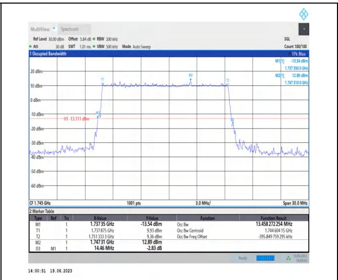
1-N66-PC3-15-15-M-3-DFT-16QAM-Outer_Full-75 @0-Ant3-13.458-14.460-≤15-PASS
