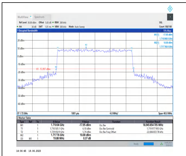
1-N66-PC3-15-20-L-8-CP-64QAM-Outer_Full-106 @0-Ant3-18.946-19.880-<math>\leq 20</math>-PASS
