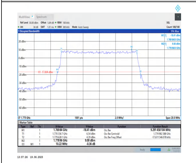
1-N66-PC3-15-10-H-6-CP-QPSK-Outer_Full-52@0- Ant3-9.291-10.220-≤10-PASS
