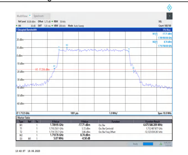
1-N66-PC3-15-5-L-6-CP-QPSK-Outer_Full-25@0-An t3-4.476-5.070-≤5-PASS
