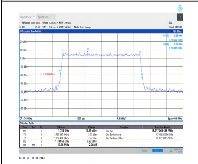
1-N66-PC3-15-20-M-9-CP-256QAM-Outer_Full-106 @-0-Ant3-18.917-19.960-<20-PASS
