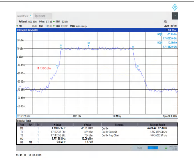
1-N66-PC3-15-5-L-2-DFT-PI2BPSK-Outer_Full-25@ 0-Ant3-4.471-5.000- \leq 5 -PASS
