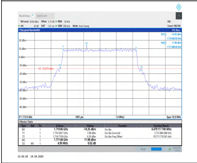
1-N66-PC3-15-5-L-3-DFT-16QAM-Outer_Full-25@0- Ant3-4.479-4.990- \leq 5 -PASS
