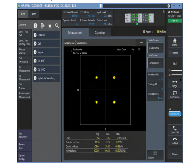
1-N66-PC3-15-40-M-6-CP-QPSK-Outer_Full-216 @0-Ant3-see graph-PASS
