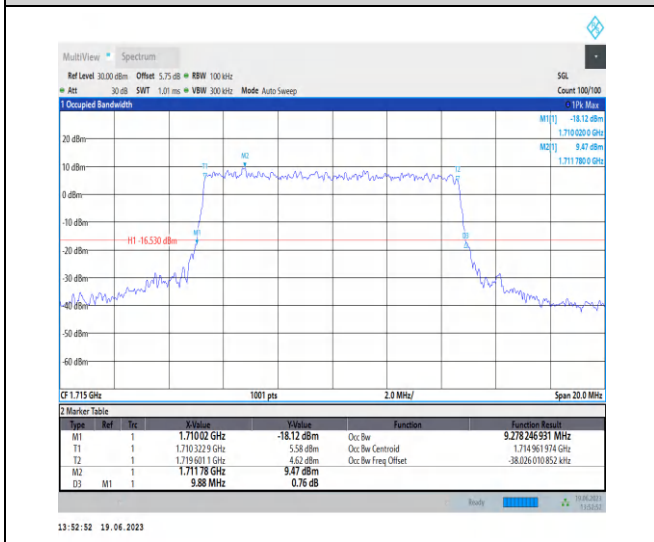
1-N66-PC3-15-10-L-8-CP-64QAM-Outer_Full-52@0 -Ant3-9.278-9.880-≤10-PASS
