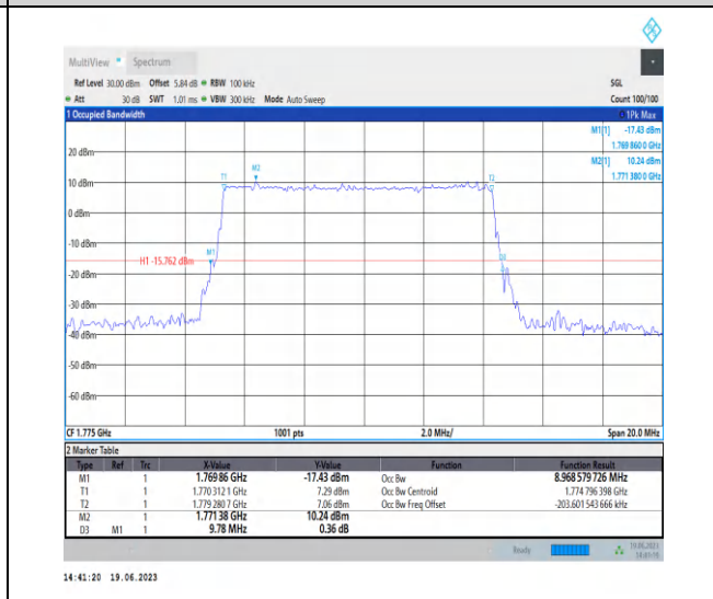
1-N66-PC3-15-10-H-3-DFT-16QAM-Outer_Full-50@ 0-Ant3-8.969-9.780-≤10-PASS
