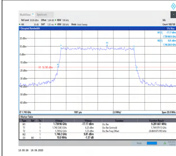
1-N66-PC3-15-10-M-7-CP-16QAM-Outer_Full-52@0-Ant3-9.282-10.000-≤10-PASS
