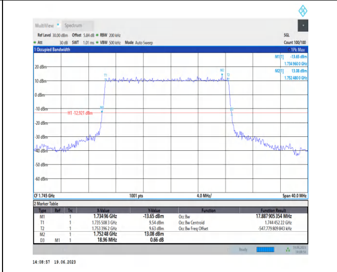
1-N66-PC3-15-20-M-2-DFT-PI2BPSK-Outer_Full-100 @0-Ant3-17.888-18.960-<math>\leq 20</math>-PASS
