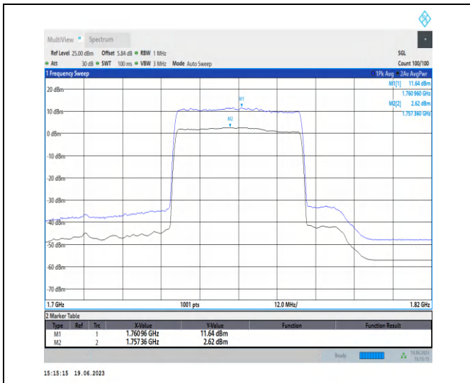
1-N66-PC3-15-40-H-1-DFT-256QAM-Outer_Full-216 @0-Ant3-9.02-100%-0.00-9.02-PASS-≤13
