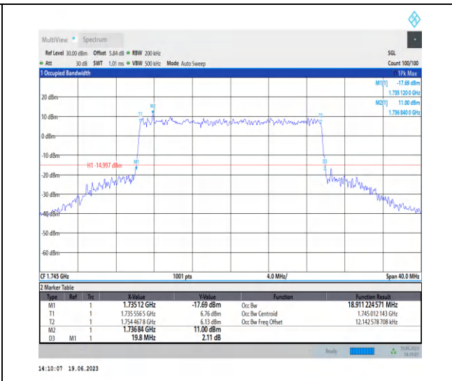
1-N66-PC3-15-20-M-8-CP-64QAM-Outer_Full-106 @-0-Ant3-18.911-19.800-<20-PASS
