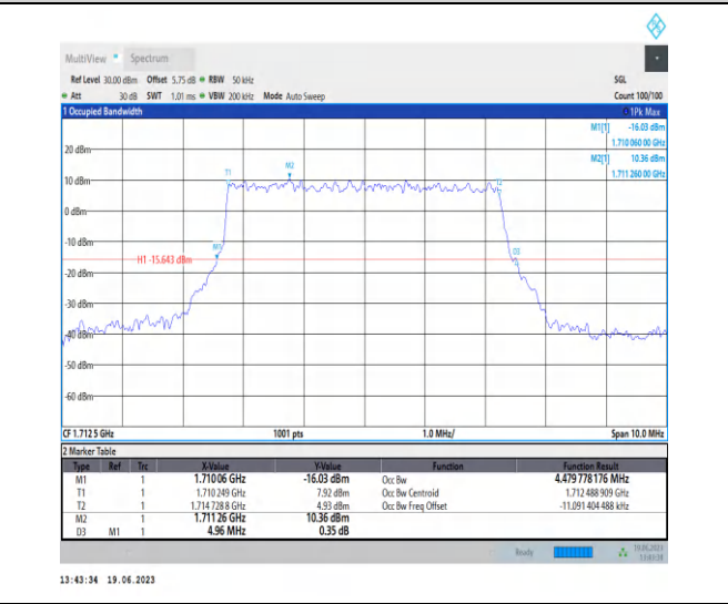
1-N66-PC3-15-5-L-4-DFT-64QAM-Outer_Full-25@0- Ant3-4.48-4.960- \leq 5 -PASS
