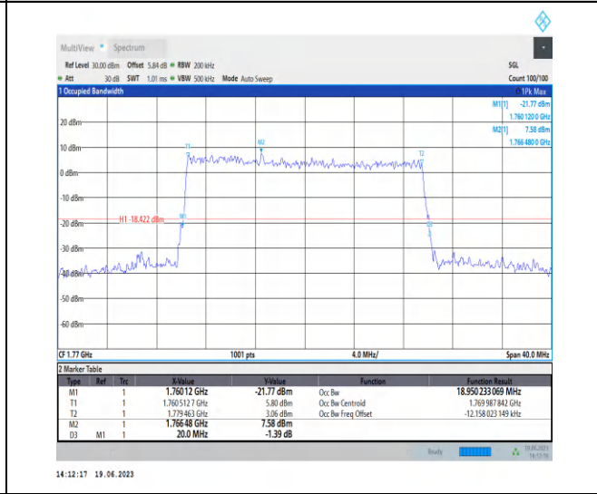
1-N66-PC3-15-20-H-9-CP-256QAM-Outer_Full-106@0 -Ant3-18.95-20.000-≤20-PASS
