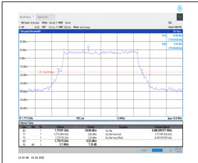
1-N66-PC3-15-5-H-7-CP-16QAM-Outer_Full-25@0- Ant3-4.487-5.100-≤5-PASS
