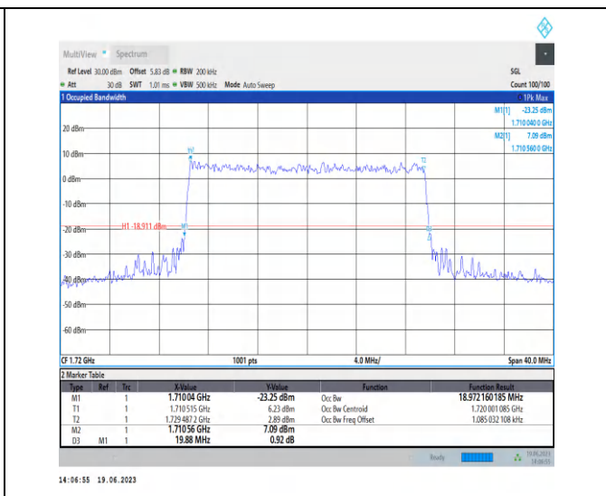
1-N66-PC3-15-20-L-9-CP-256QAM-Outer_Full-106 @0-Ant3-18.972-19.880-<math>\leq 20</math>-PASS
