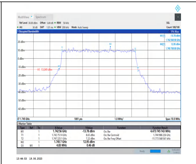
1-N66-PC3-15-5-M-1-DFT-QPSK-Outer_Full-25@0-Ant3-4.474-4.830-≤5-PASS
