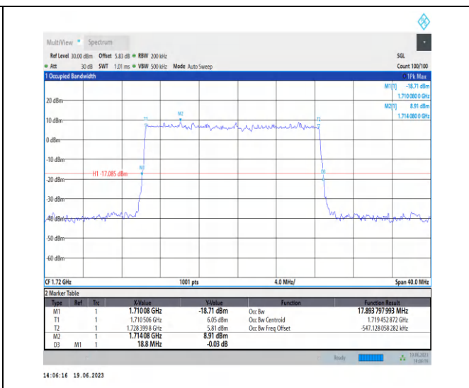
1-N66-PC3-15-20-L-5-DFT-256QAM-Outer_Full-100 @0-Ant3-17.894-18.800-≤20-PASS
