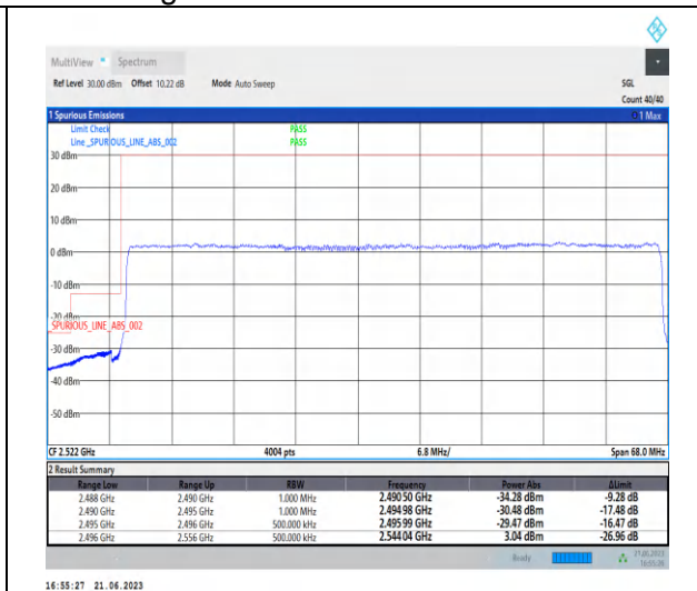
1-N41-PC3-30-60-L-3-DFT-PI2BPSK-Outer_Full-162@0-Ant0-1--PASS-see graph
