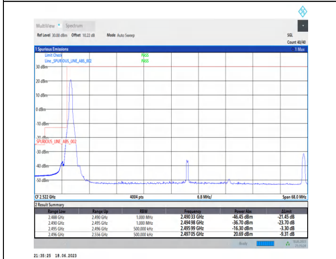
1-N41-PC3-30-60-L-4-CP-QPSK-Edge_1RB_Left-1@0-Ant0-1--PASS-see graph
