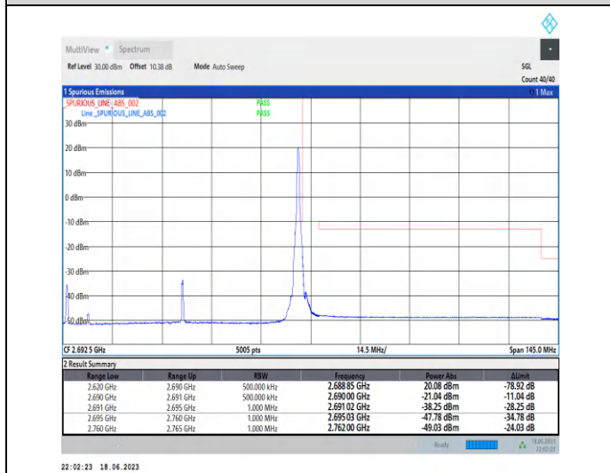
1-N41-PC3-30-70-H-5-CP-QPSK-Edge_1RB_Righ t-1@188-Ant0-1--PASS-see graph
