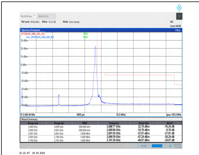
1-N41-PC3-30-50-H-2-DFT-PI2BPSK-Edge_1RB_Righ t-1@132-Ant0-1--PASS-see graph
