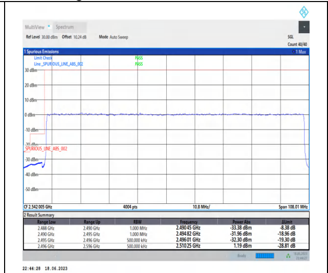
1-N41-PC3-30-100-L-3-DFT-PI2BPSK-Outer_Full-270@0-Ant0-1--PASS-see graph
