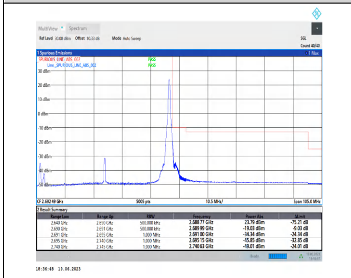
1-N41-PC2-30-50-H-2-CP-QPSK-Edge_1RB_Right-1@132-Ant0-1--PASS-see graph
