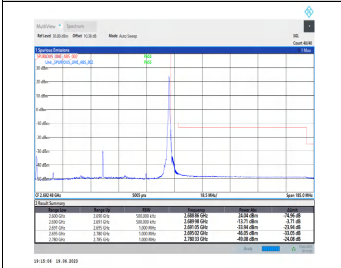
1-N41-PC2-30-90-H-2-CP-QPSK-Edge_1RB_Right-1 @244-Ant0-1--PASS-see graph
