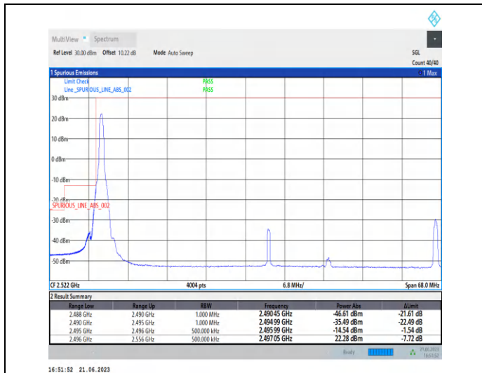
1-N41-PC3-30-60-L-1-DFT-PI2BPSK-Edge_1RB_Left-1@0-Ant0-1--PASS-see graph
