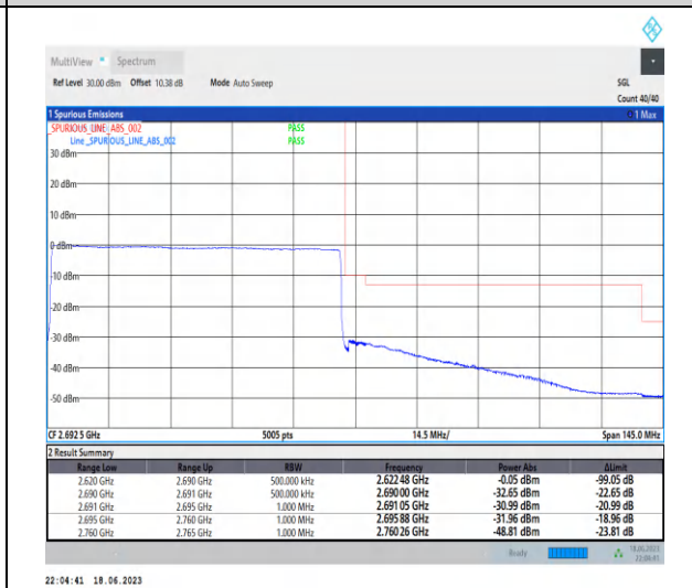
1-N41-PC3-30-70-H-6-CP-QPSK-Outer_Full-189 @0-Ant0-1--PASS-see graph
