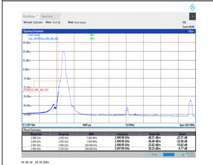
1-N41-PC3-30-30-L-4-CP-QPSK-Edge_1RB_Left-1@0-Ant0-1--PASS-see graph
