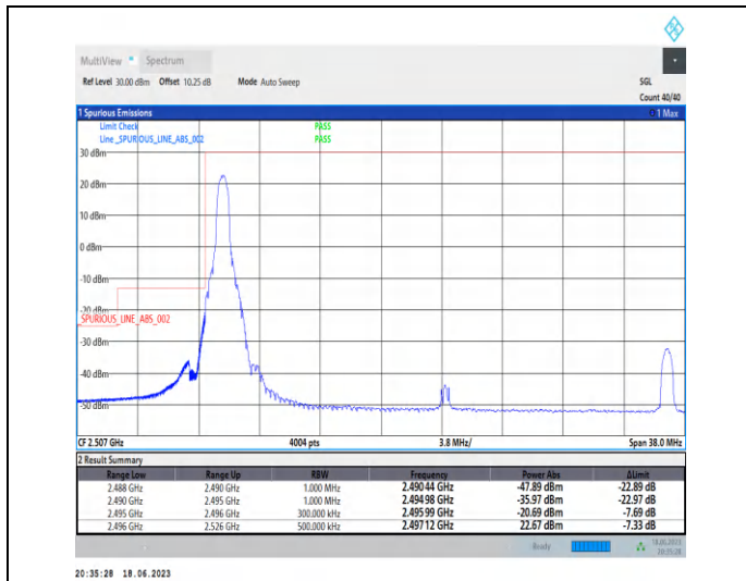
1-N41-PC3-30-30-L-1-DFT-PI2BPSK-Edge_1RB_Left-1@0-Ant0-1--PASS-see graph
