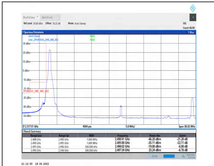
1-N41-PC3-30-50-L-1-DFT-PI2BPSK-Edge_1RB_Left-1@0-Ant0-1--PASS-see graph
