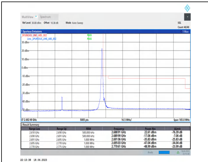
1-N41-PC3-30-80-H-2-DFT-PI2BPSK-Edge_1RB_Righ t-1@216-Ant0-1--PASS-see graph
