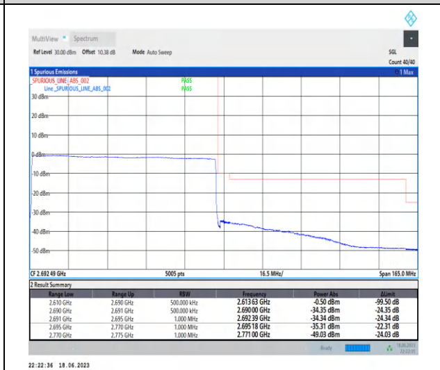
1-N41-PC3-30-80-H-6-CP-QPSK-Outer_Full-217 @0-Ant0-1--PASS-see graph
