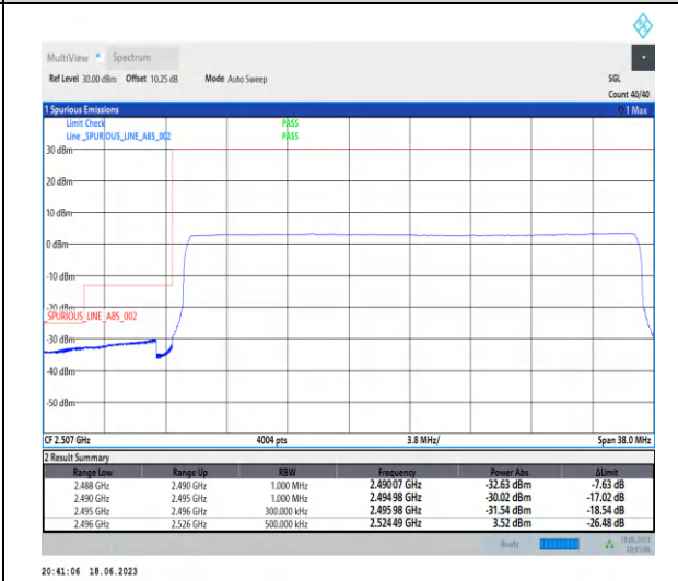
1-N41-PC3-30-30-L-6-CP-QPSK-Outer_Full-78@0-Ant0-1--PASS-see graph
