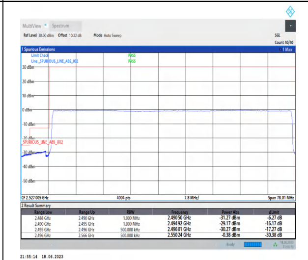
1-N41-PC3-30-70-L-6-CP-QPSK-Outer_Full-189@0-Ant0-1--PASS-see graph
