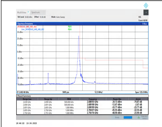
1-N41-PC2-30-60-H-2-CP-QPSK-Edge_1RB_Right-1 @161-Ant0-1--PASS-see graph
