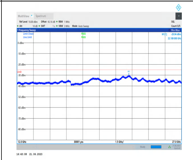
1-N41-PC3-30-100-M-1-N/A-DFT-PI2BPSK-Inner_1R B_Left-1@1-12000-27000-Ant0-22192.00--29.94--25- PASS
