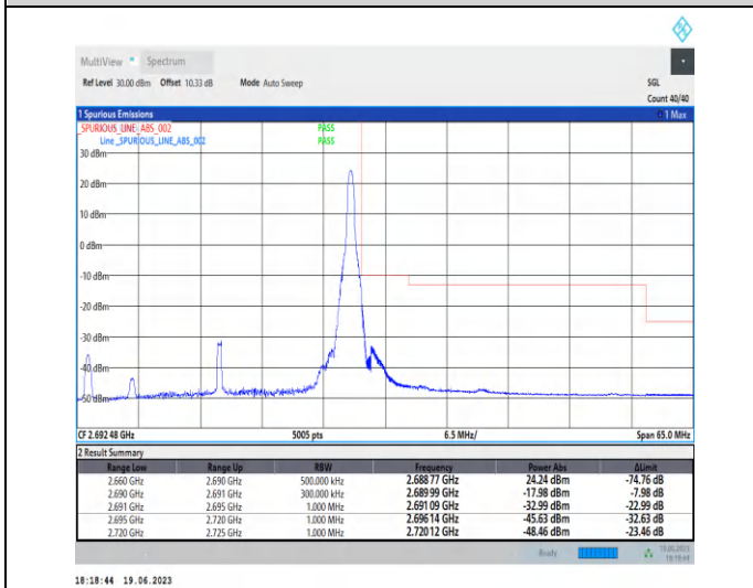
1-N41-PC2-30-30-H-2-CP-QPSK-Edge_1RB_Right-1 @77-Ant0-1--PASS-see graph
