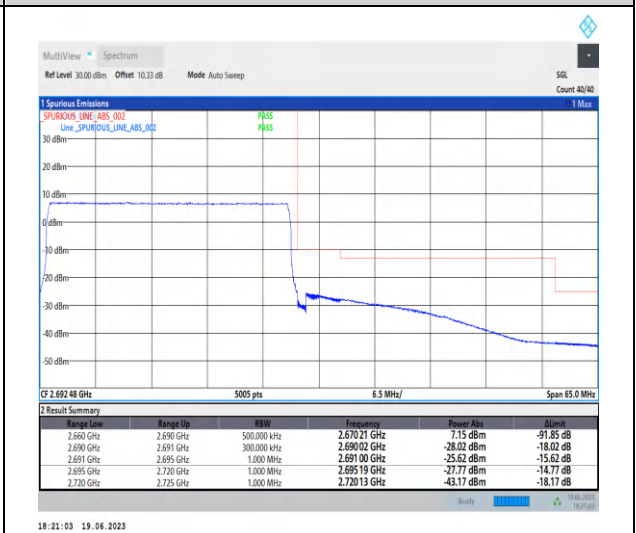
1-N41-PC2-30-30-H-3-CP-QPSK-Outer_Full-78@ 0-Ant0-1--PASS-see graph
