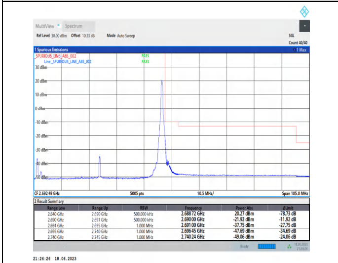
1-N41-PC3-30-50-H-5-CP-QPSK-Edge_1RB_Righ t-1 @132-Ant0-1--PASS-see graph
