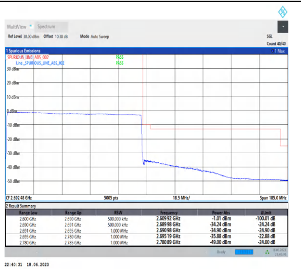
1-N41-PC3-30-90-H-6-CP-QPSK-Outer_Full-245 @0-Ant0-1--PASS-see graph
