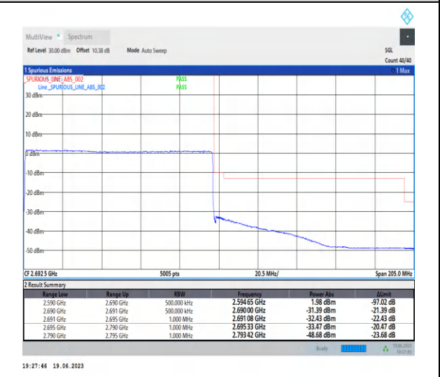
1-N41-PC2-30-100-H-3-CP-QPSK-Outer_Full-273 @ 0-Ant0-1--PASS-see graph
