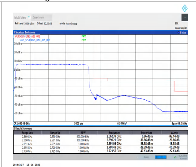
1-N41-PC3-30-30-H-3-DFT-PI2BPSK-Outer_Full-7 5@0-Ant0-1--PASS-see graph
