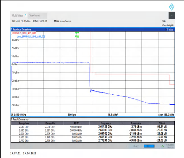
1-N41-PC2-30-80-H-3-CP-QPSK-Outer_Full-217 @0-Ant0-1--PASS-see graph
