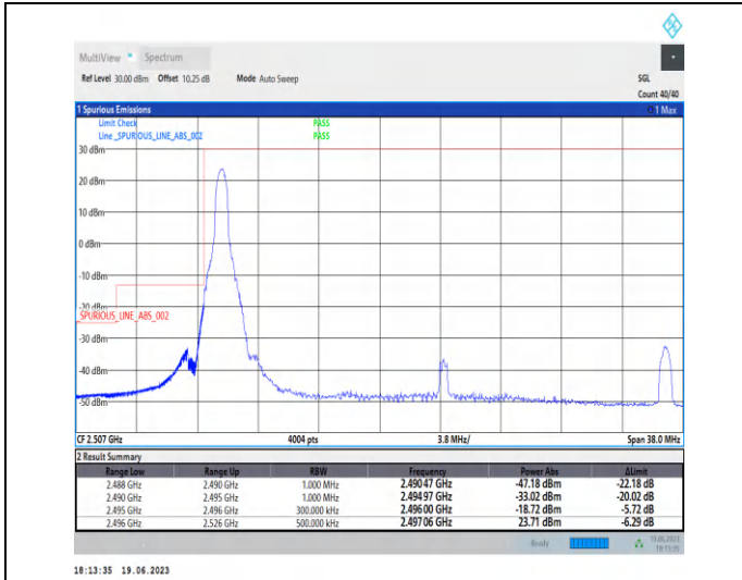
1-N41-PC2-30-30-L-1-CP-QPSK-Edge_1RB_Left-1@0 -Ant0-1--PASS-see graph
