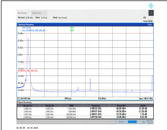
1-N41-PC3-30-100-L-1-DFT-PI2BPSK-Edge_1RB_Left -1@0-Ant0-1--PASS-see graph
