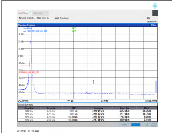
1-N41-PC3-30-90-L-4-CP-QPSK-Edge_1RB_Left-1@0-Ant0-1--PASS-see graph
