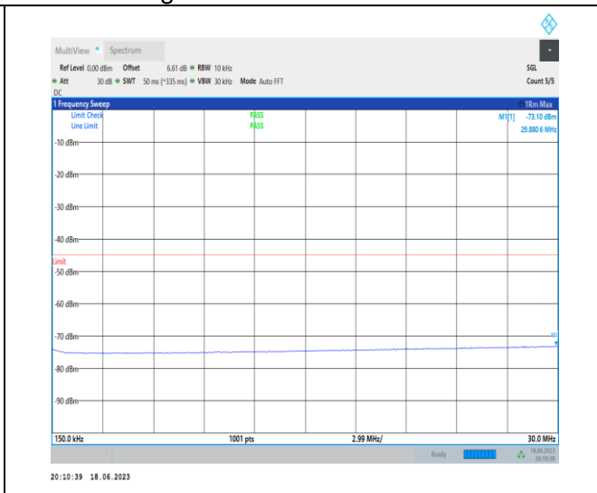
1-N41-PC3-30-100-H-1-N/A-DFT-PI2BPSK-Inner_1R B_Left-1@1-0.15-30-Ant0-29.88--73.10--45-PASS
