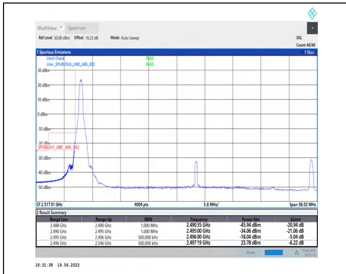
1-N41-PC2-30-50-L-1-CP-QPSK-Edge_1RB_Left-1@0-Ant0-1--PASS-see graph
