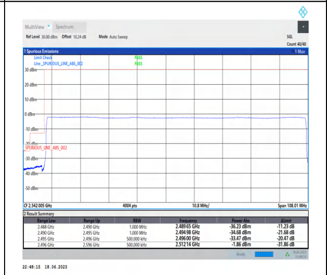
1-N41-PC3-30-100-L-6-CP-QPSK-Outer_Full-273@0-Ant0-1--PASS-see graph
