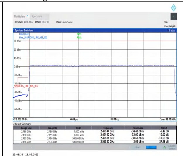
1-N41-PC3-30-80-L-3-DFT-PI2BPSK-Outer_Full-216@0-Ant0-1--PASS-see graph
