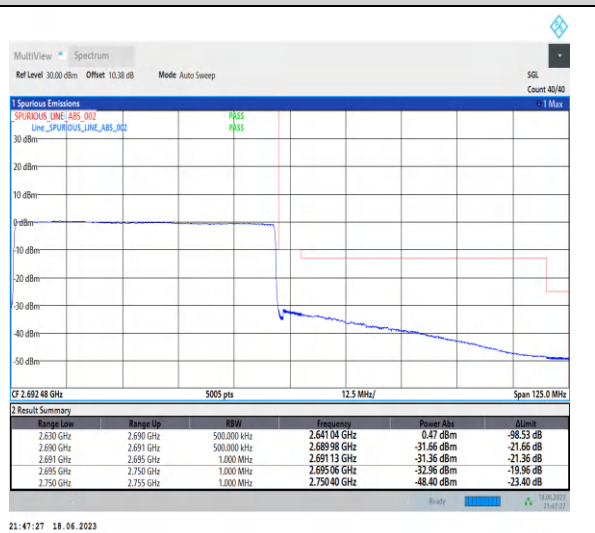
1-N41-PC3-30-60-H-6-CP-QPSK-Outer_Full-1 62 @0-Ant0-1--PASS-see graph
