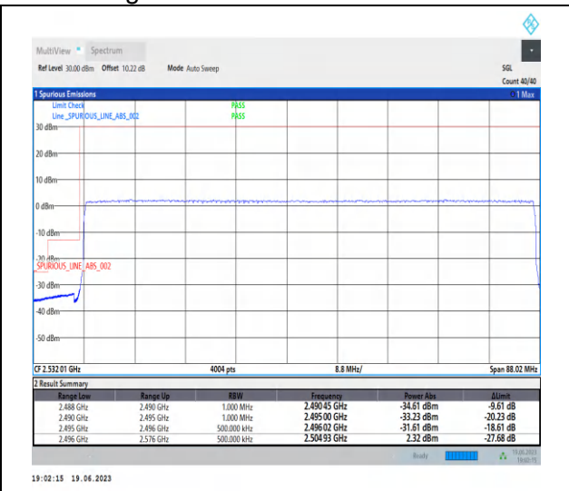
1-N41-PC2-30-80-L-3-CP-QPSK-Outer_Full-217 @0-Ant0-1--PASS-see graph
