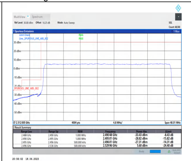
1-N41-PC3-30-40-L-3-DFT-PI2BPSK-Outer_Full-100@0-Ant0-1--PASS-see graph
