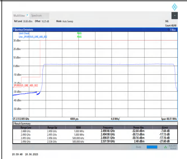
1-N41-PC3-30-40-L-6-CP-QPSK-Outer_Full-106@0-Ant0-1--PASS-see graph
