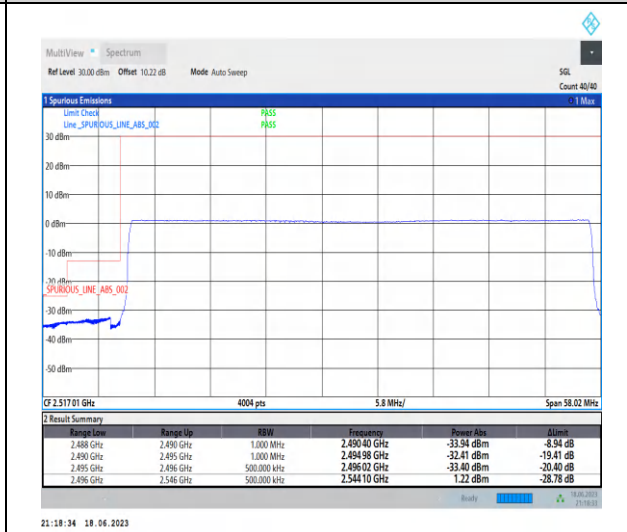
1-N41-PC3-30-50-L-6-CP-QPSK-Outer_Full-133@0-Ant0-1--PASS-see graph
