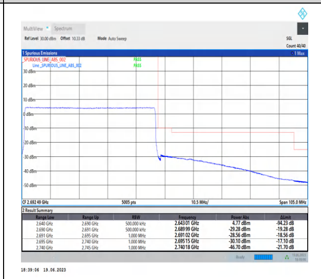
1-N41-PC2-30-50-H-3-CP-QPSK-Outer_Full-133@0-Ant0-1--PASS-see graph
