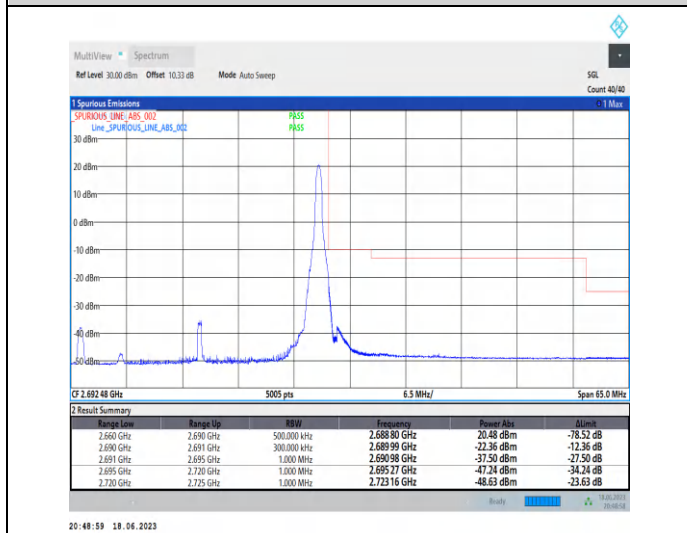
1-N41-PC3-30-30-H-5-CP-QPSK-Edge_1RB_Righ t-1@77-Ant0-1--PASS-see graph
