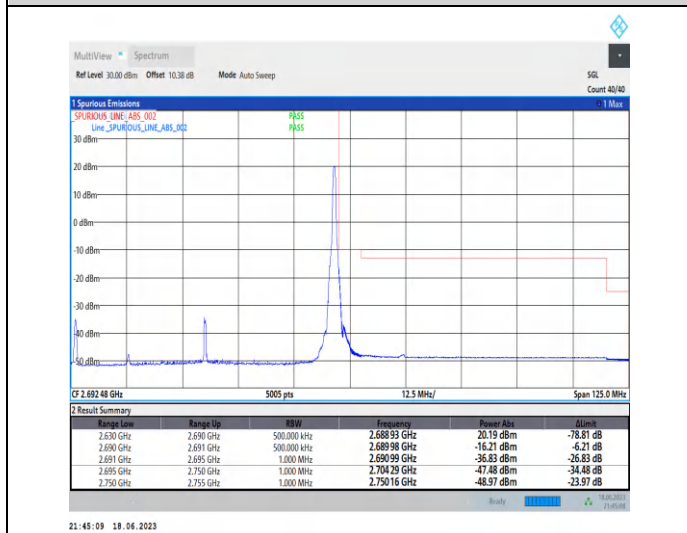
1-N41-PC3-30-60-H-5-CP-QPSK-Edge_1RB_Righ t-1 @161-Ant0-1--PASS-see graph
