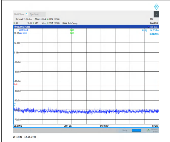
1-N41-PC3-30-100-H-1-N/A-DFT-PI2BPSK-Inner_1 RB_Left-1@1-30-1000-Ant0-38.25--56.77--35-PASS
