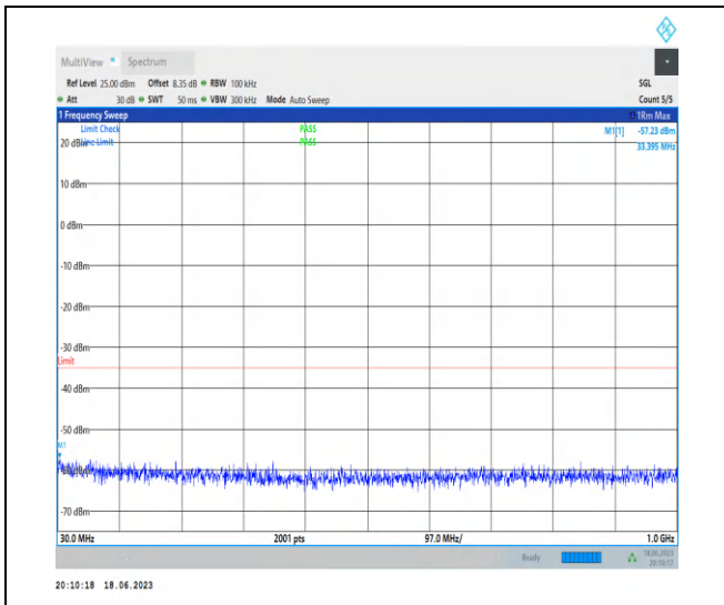
1-N41-PC3-30-100-M-1-N/A-DFT-PI2BPSK-Inner_1 RB_Left-1@1-30-1000-Ant0-33.40--57.23--35-PASS
