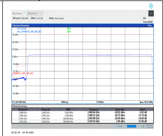
1-N41-PC2-30-70-L-3-CP-QPSK-Outer_Full-189 @0-Ant0-1--PASS-see graph
