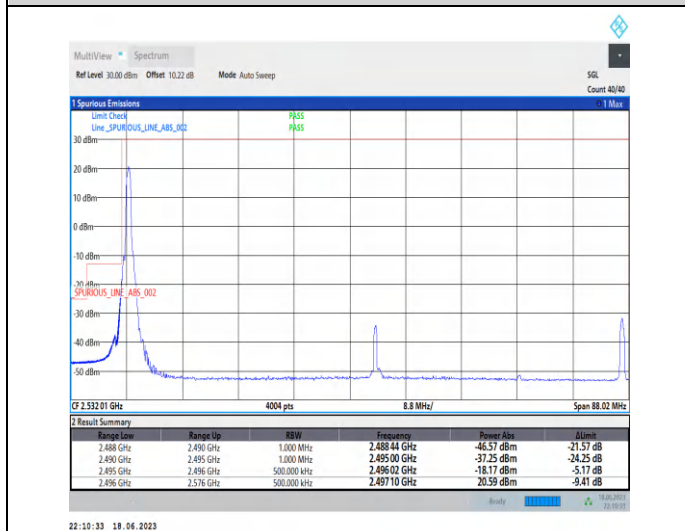
1-N41-PC3-30-80-L-4-CP-QPSK-Edge_1RB_Left-1@0-Ant0-1--PASS-see graph
