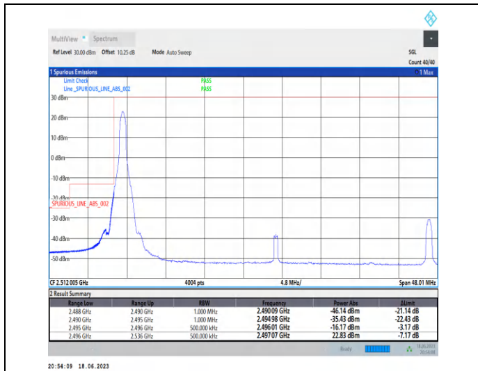
1-N41-PC3-30-40-L-1-DFT-PI2BPSK-Edge_1RB_Left-1@0-Ant0-1--PASS-see graph
