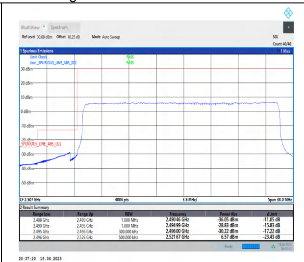
1-N41-PC3-30-30-L-3-DFT-PI2BPSK-Outer_Full-75@0-Ant0-1--PASS-see graph
