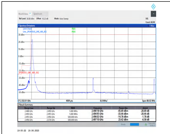
1-N41-PC2-30-80-L-1-CP-QPSK-Edge_1RB_Left-1@0 -Ant0-1--PASS-see graph
