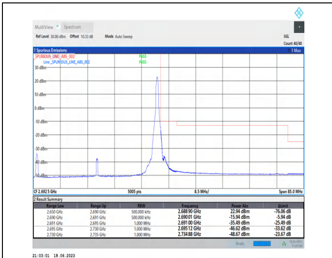
1-N41-PC3-30-40-H-2-DFT-PI2BPSK-Edge_1RB_Righ t-1@105-Ant0-1--PASS-see graph
