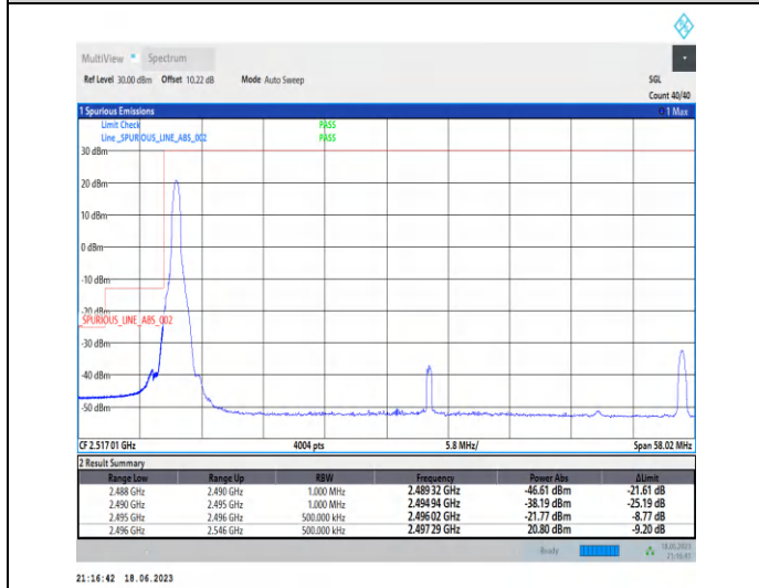
1-N41-PC3-30-50-L-4-CP-QPSK-Edge_1RB_Left-1@0-Ant0-1--PASS-see graph
