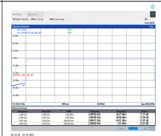
1-N41-PC3-30-80-L-6-CP-QPSK-Outer_Full-217@0-Ant0-1--PASS-see graph
