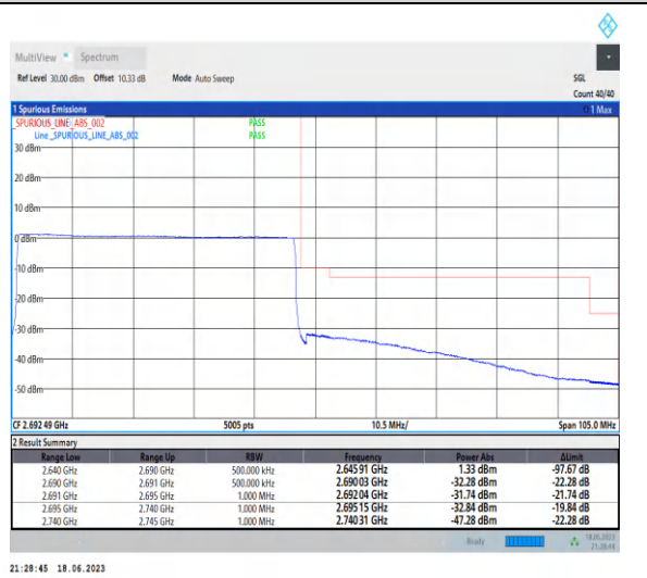
1-N41-PC3-30-50-H-6-CP-QPSK-Outer_Full-133 @0-Ant0-1--PASS-see graph
