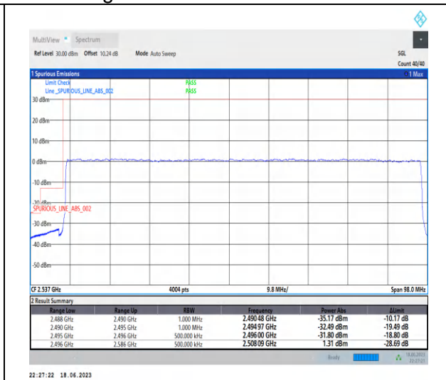
1-N41-PC3-30-90-L-3-DFT-PI2BPSK-Outer_Full-243@0-Ant0-1--PASS-see graph
