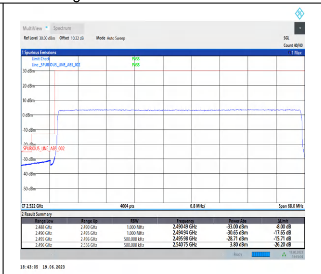
1-N41-PC2-30-60-L-3-CP-QPSK-Outer_Full-162 @0-Ant0-1--PASS-see graph
