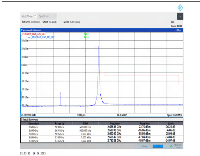
1-N41-PC3-30-90-H-2-DFT-PI2BPSK-Edge_1RB_Righ t-1@244-Ant0-1--PASS-see graph
