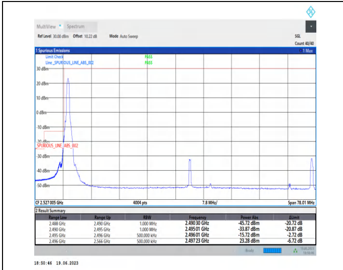
1-N41-PC2-30-70-L-1-CP-QPSK-Edge_1RB_Left-1@0 -Ant0-1--PASS-see graph
