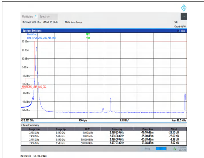
1-N41-PC3-30-90-L-1-DFT-PI2BPSK-Edge_1RB_Left-1@0-Ant0-1--PASS-see graph
