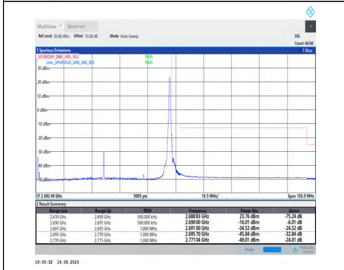
1-N41-PC2-30-80-H-2-CP-QPSK-Edge_1RB_Right-1 @216-Ant0-1--PASS-see graph
