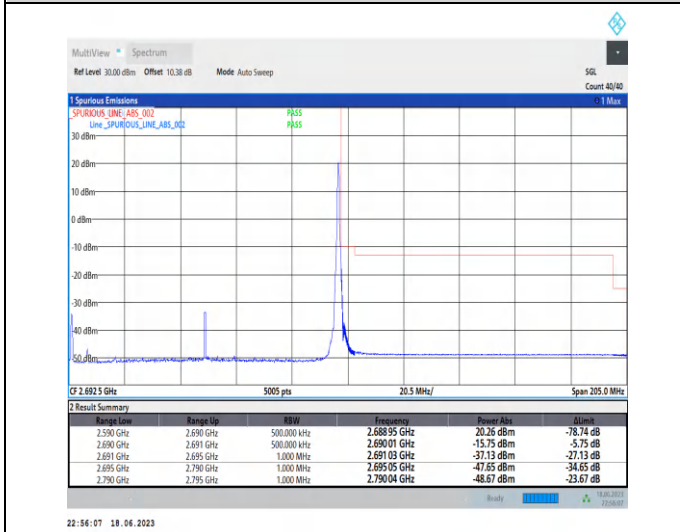
1-N41-PC3-30-100-H-5-CP-QPSK-Edge_1RB_Right-1 @272-Ant0-1--PASS-see graph
