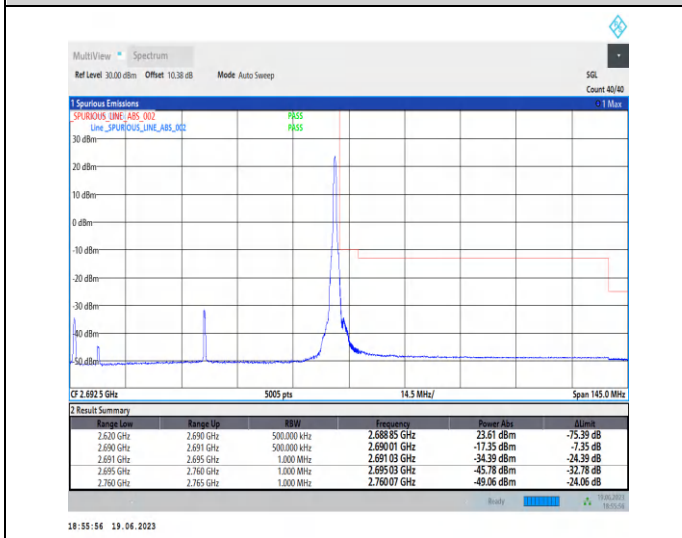
1-N41-PC2-30-70-H-2-CP-QPSK-Edge_1RB_Right-1 @188-Ant0-1--PASS-see graph
