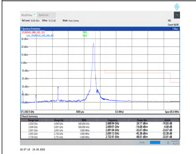
1-N41-PC2-30-40-H-2-CP-QPSK-Edge_1RB_Right-1@105-Ant0-1--PASS-see graph
