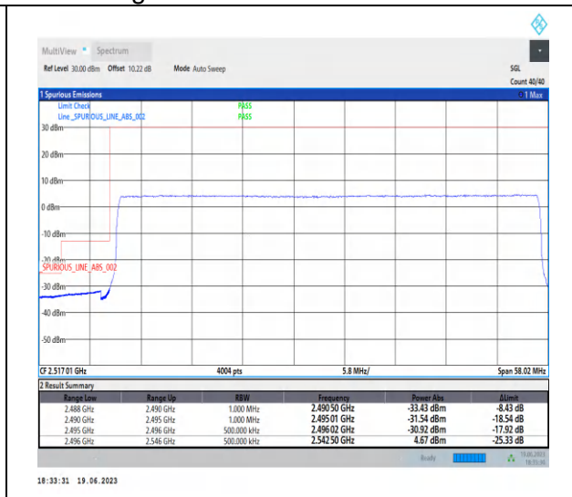
1-N41-PC2-30-50-L-3-CP-QPSK-Outer_Full-133@0-Ant0-1--PASS-see graph
