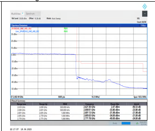
1-N41-PC3-30-80-H-3-DFT-PI2BPSK-Outer_Full-2 16@0-Ant0-1--PASS-see graph
