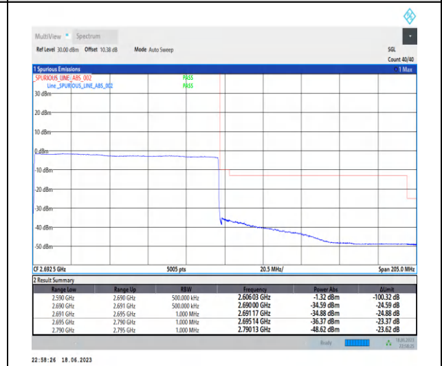
1-N41-PC3-30-100-H-6-CP-QPSK-Outer_Full-273 @0-Ant0-1--PASS-see graph
