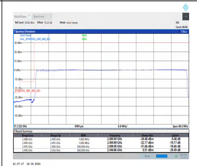
1-N41-PC3-30-60-L-6-CP-QPSK-Outer_Full-162@0-Ant0-1--PASS-see graph
