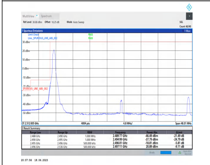
1-N41-PC3-30-40-L-4-CP-QPSK-Edge_1RB_Left-1@0-Ant0-1--PASS-see graph
