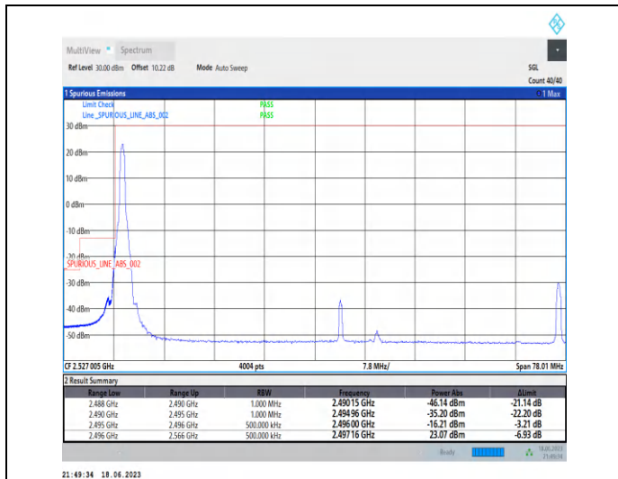
1-N41-PC3-30-70-L-1-DFT-PI2BPSK-Edge_1RB_Left-1@0-Ant0-1--PASS-see graph
