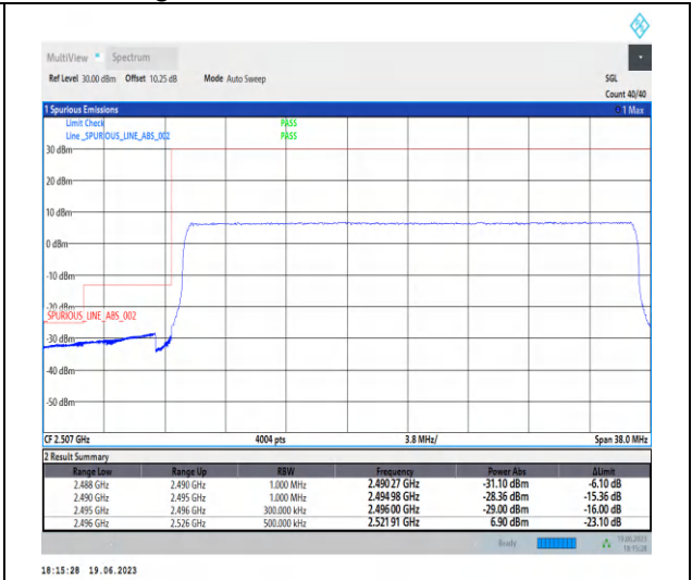
1-N41-PC2-30-30-L-3-CP-QPSK-Outer_Full-78@ 0-Ant0-1--PASS-see graph
