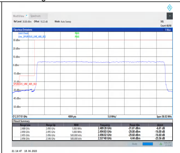
1-N41-PC3-30-50-L-3-DFT-PI2BPSK-Outer_Full-128@0-Ant0-1--PASS-see graph
