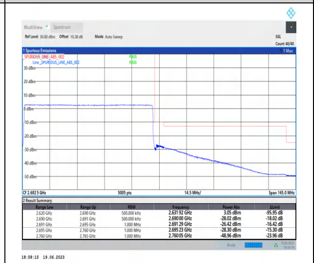
1-N41-PC2-30-70-H-3-CP-QPSK-Outer_Full-189 @0-Ant0-1--PASS-see graph
