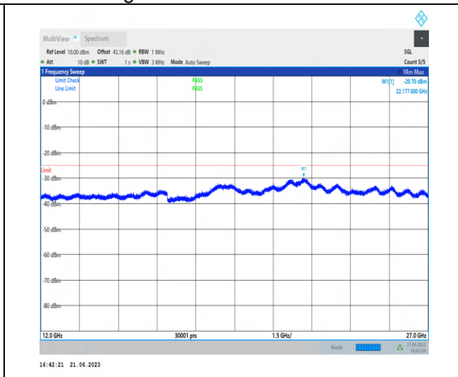
1-N41-PC3-30-100-L-1-N/A-DFT-PI2BPSK-Inner_1R B_Left-1@1-12000-27000-Ant0-22262.00--29.70--25 PASS
