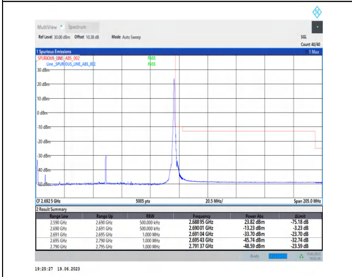
1-N41-PC2-30-100-H-2-CP-QPSK-Edge_1RB_Right-1 @ 272-Ant0-1--PASS-see graph
