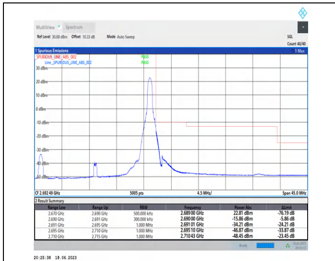
1-N41-PC3-30-20-H-2-DFT-PI2BPSK-Edge_1RB_Righ t-1@50-Ant0-1--PASS-see graph
