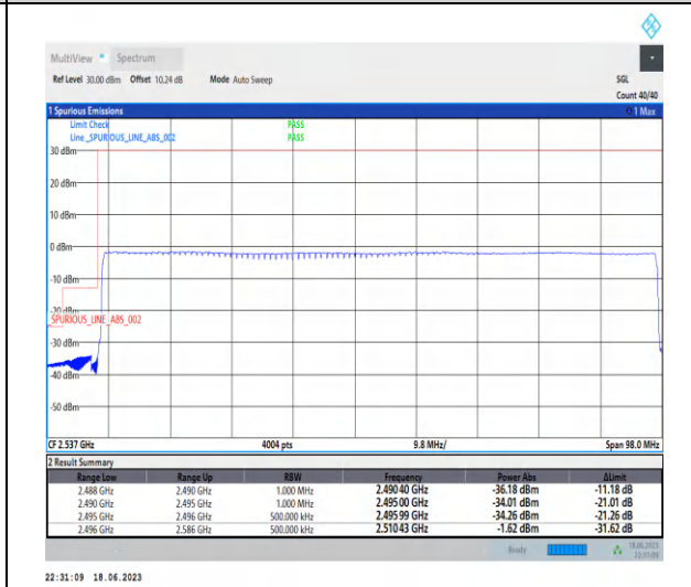
1-N41-PC3-30-90-L-6-CP-QPSK-Outer_Full-245@0-Ant0-1--PASS-see graph
