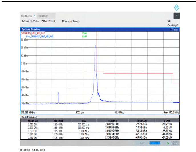
1-N41-PC3-30-60-H-2-DFT-PI2BPSK-Edge_1RB_Righ t-1@161-Ant0-1--PASS-see graph
