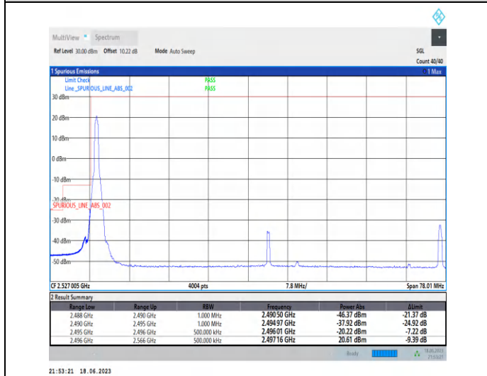
1-N41-PC3-30-70-L-4-CP-QPSK-Edge_1RB_Left-1@0-Ant0-1--PASS-see graph
