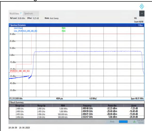
1-N41-PC2-30-40-L-3-CP-QPSK-Outer_Full-106@0-Ant0-1--PASS-see graph
