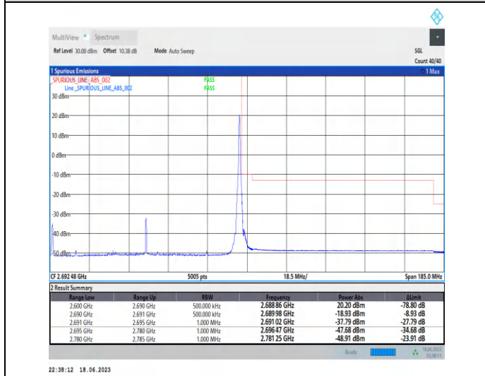
1-N41-PC3-30-90-H-5-CP-QPSK-Edge_1RB_Righ t-1@244-Ant0-1--PASS-see graph
