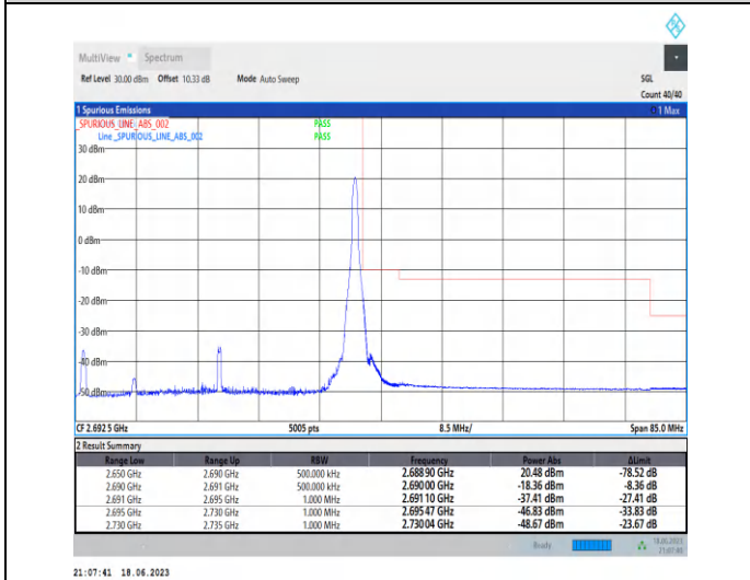
1-N41-PC3-30-40-H-5-CP-QPSK-Edge_1RB_Righ t-1@105-Ant0-1--PASS-see graph
