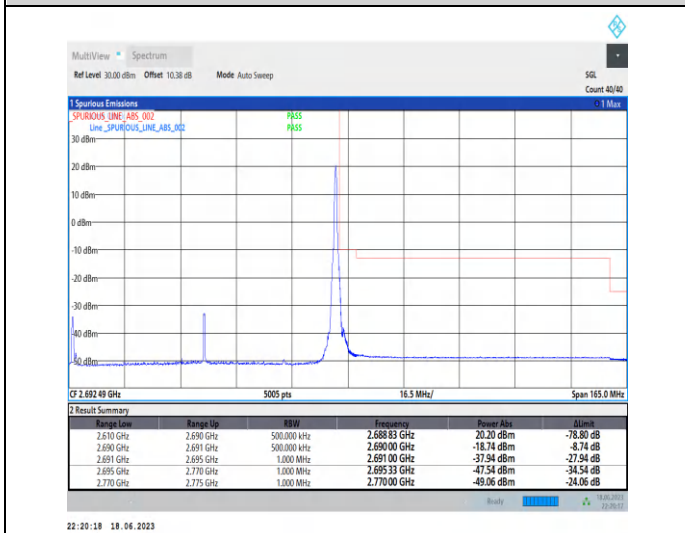
1-N41-PC3-30-80-H-5-CP-QPSK-Edge_1RB_Righ t-1@216-Ant0-1--PASS-see graph
