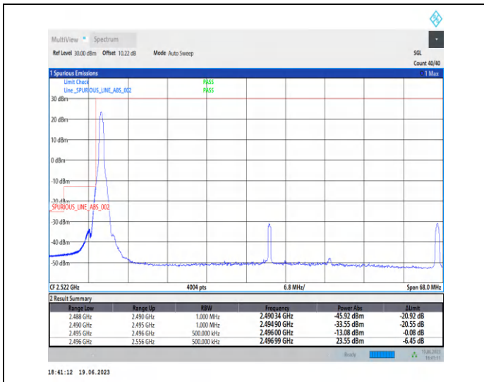
1-N41-PC2-30-60-L-1-CP-QPSK-Edge_1RB_Left-1@0 -Ant0-1--PASS-see graph
