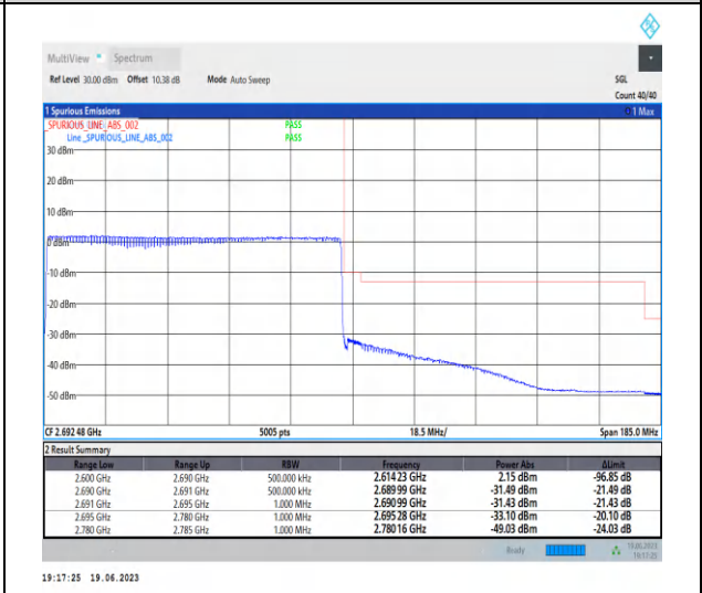
1-N41-PC2-30-90-H-3-CP-QPSK-Outer_Full-245 @0-Ant0-1--PASS-see graph
