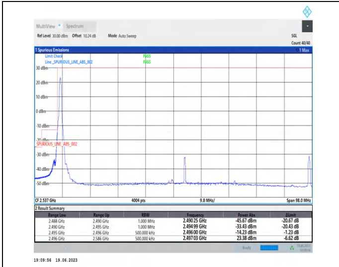
1-N41-PC2-30-90-L-1-CP-QPSK-Edge_1RB_Left-1@0 -Ant0-1--PASS-see graph
