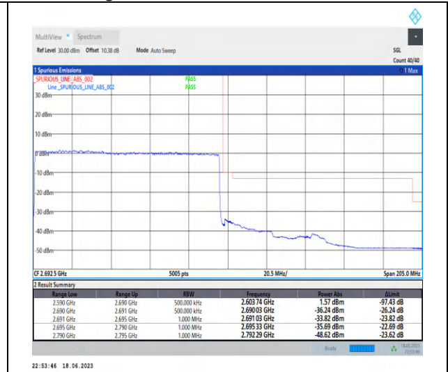
1-N41-PC3-30-100-H-3-DFT-PI2BPSK-Outer_Full-270@0-Ant0-1--PASS-see graph
