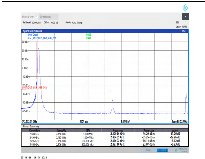
1-N41-PC3-30-80-L-1-DFT-PI2BPSK-Edge_1RB_Left-1@0-Ant0-1--PASS-see graph
