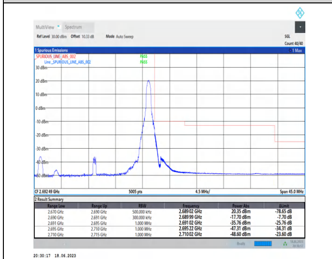
1-N41-PC3-30-20-H-5-CP-QPSK-Edge_1RB_Righ t-1@50-Ant0-1--PASS-see graph
