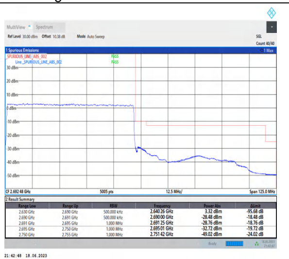
1-N41-PC3-30-60-H-3-DFT-PI2BPSK-Outer_Full-1 62@0-Ant0-1--PASS-see graph
