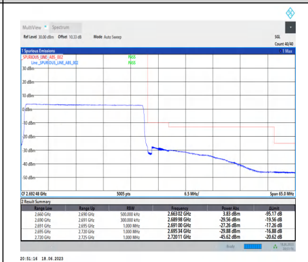
1-N41-PC3-30-30-H-6-CP-QPSK-Outer_Full-78@ 0-Ant0-1--PASS-see graph
