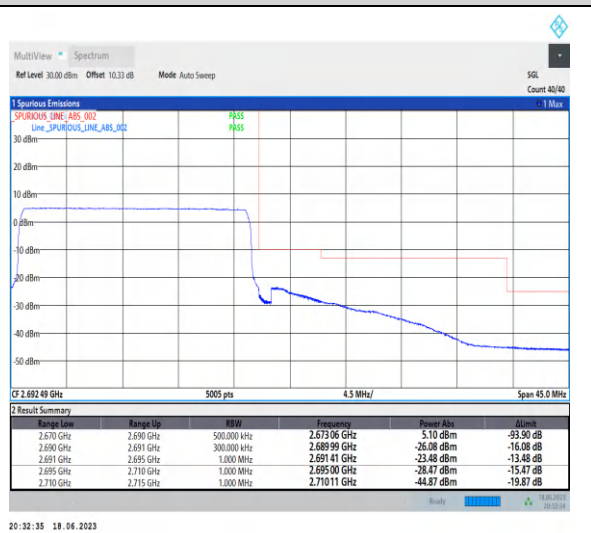
1-N41-PC3-30-20-H-6-CP-QPSK-Outer_Full-51 @0-Ant0-1--PASS-see graph
