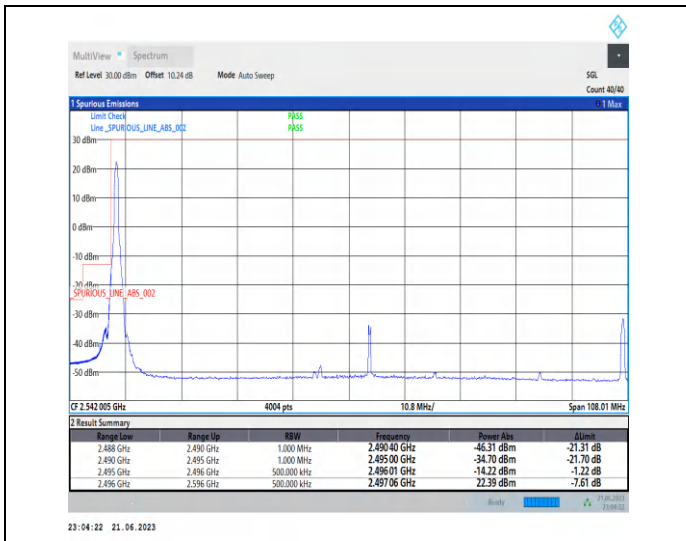
1-N41-PC2-30-100-L-1-CP-QPSK-Edge_1RB_Left-1 @ 0-Ant0-1--PASS-see graph
