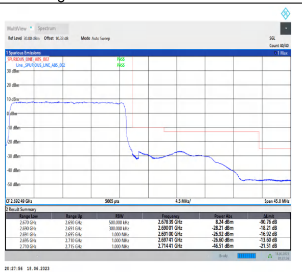
1-N41-PC3-30-20-H-3-DFT-PI2BPSK-Outer_Full-5 0@0-Ant0-1--PASS-see graph
