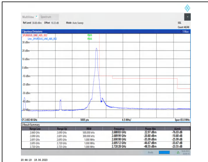
1-N41-PC3-30-30-H-2-DFT-PI2BPSK-Edge_1RB_Righ t-1@77-Ant0-1--PASS-see graph
