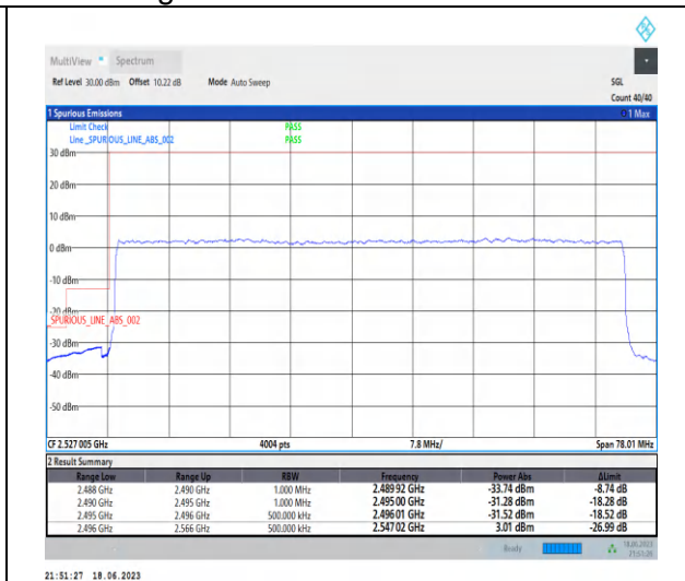
1-N41-PC3-30-70-L-3-DFT-PI2BPSK-Outer_Full-180@0-Ant0-1--PASS-see graph
