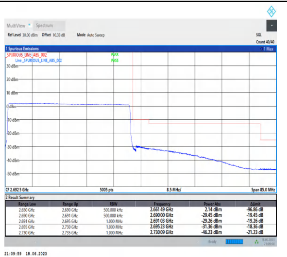
1-N41-PC3-30-40-H-6-CP-QPSK-Outer_Full-106 @0-Ant0-1--PASS-see graph
