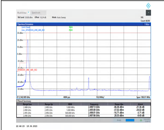
1-N41-PC3-30-100-L-4-CP-QPSK-Edge_1RB_Left1@0-Ant0-1--PASS-see graph
