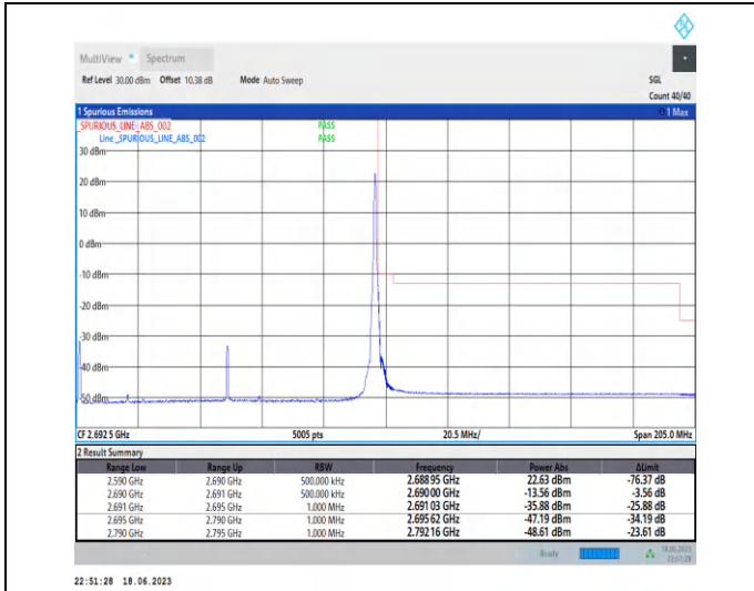
1-N41-PC3-30-100-H-2-DFT-PI2BPSK-Edge_1RB_Rig ht-1@272-Ant0-1--PASS-see graph
