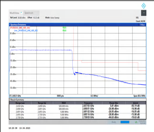
1-N41-PC2-30-40-H-3-CP-QPSK-Outer_Full-106@0-Ant0-1--PASS-see graph
