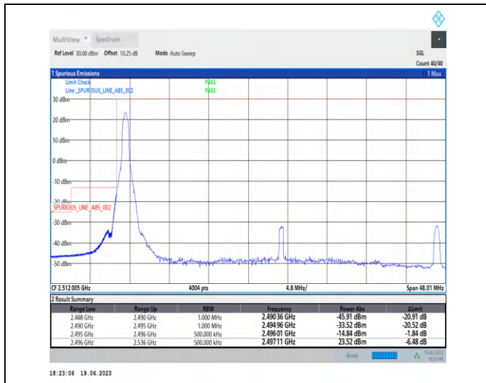
1-N41-PC2-30-40-L-1-CP-QPSK-Edge_1RB_Left-1@0-Ant0-1--PASS-see graph
