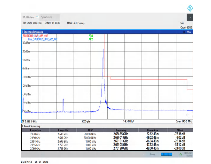
1-N41-PC3-30-70-H-2-DFT-PI2BPSK-Edge_1RB_Righ t-1@188-Ant0-1--PASS-see graph
