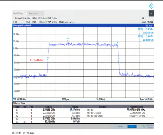
1-N41-PC3-30-80-M-9-CP-256QAM-Outer_Full-217@0 -Ant0-77.048-80.320-≤80-PASS
