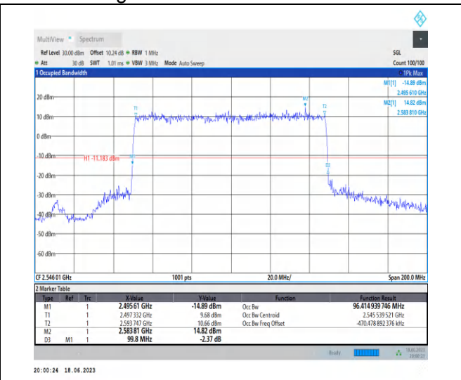
1-N41-PC3-30-100-L-2-DFT-QPSK-Outer_Full-270 @ 0-Ant0-96.415-99.800-≤100-PASS
