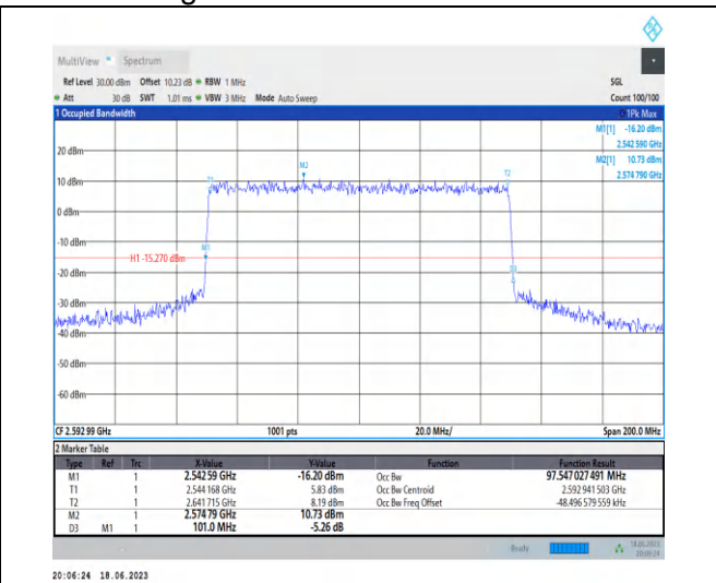
1-N41-PC3-30-100-M-6-CP-QPSK-Outer_Full-273 @ 0-Ant0-97.547-101.000-≤100-PASS
