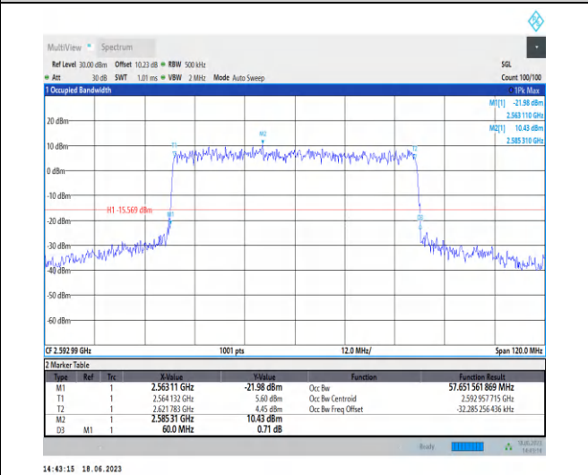
1-N41-PC3-30-60-M-7-CP-16QAM-Outer_Full-162 @ 0-Ant0-57.652-60.000-≤60-PASS
