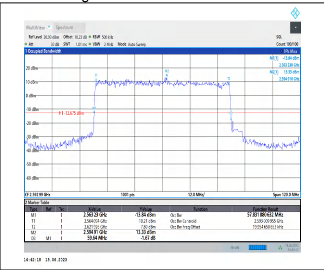
1-N41-PC3-30-60-M-1-DFT-PI2BPSK-Outer_Full-16 2@0-Ant0-57.832-59.640-≤60-PASS
