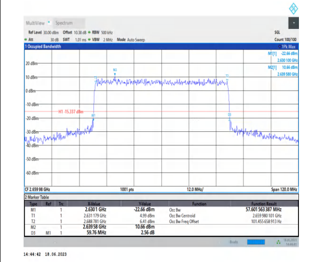
1-N41-PC3-30-60-H-6-CP-QPSK-Outer_Full-162 @ 0-Ant0-57.602-59.760-≤60-PASS
