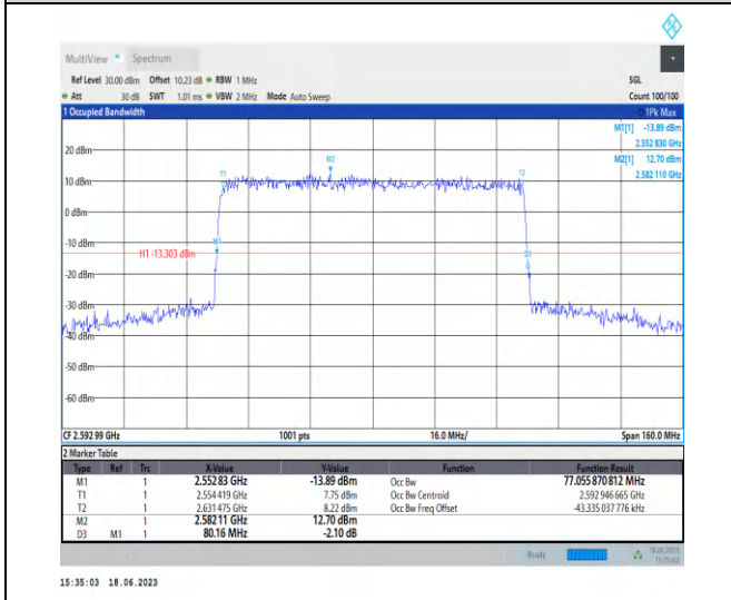
1-N41-PC3-30-80-M-4-DFT-64QAM-Outer_Full-216 @0-Ant0-77.056-80.160-≤80-PASS
