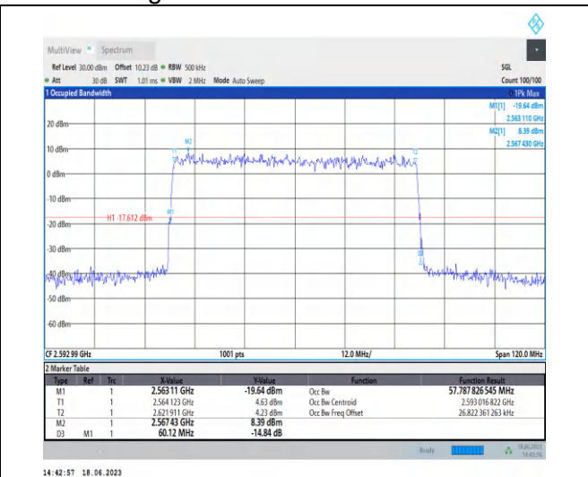
1-N41-PC3-30-60-M-5-DFT-256QAM-Outer_Full-162 @ 0-Ant0-57.788-60.120-≤60-PASS
