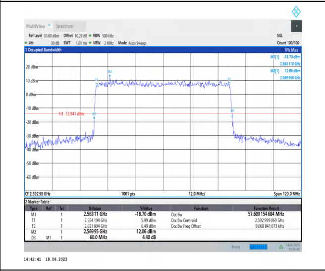
1-N41-PC3-30-60-M-3-DFT-16QAM-Outer_Full-162 @0-Ant0-57.609-60.000-≤60-PASS
