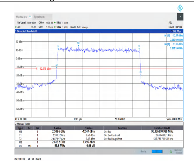
1-N41-PC3-30-100-H-1-DFT-PI2BPSK-Outer_Full-270 @0-Ant0-96.327-99.800-≤100-PASS
