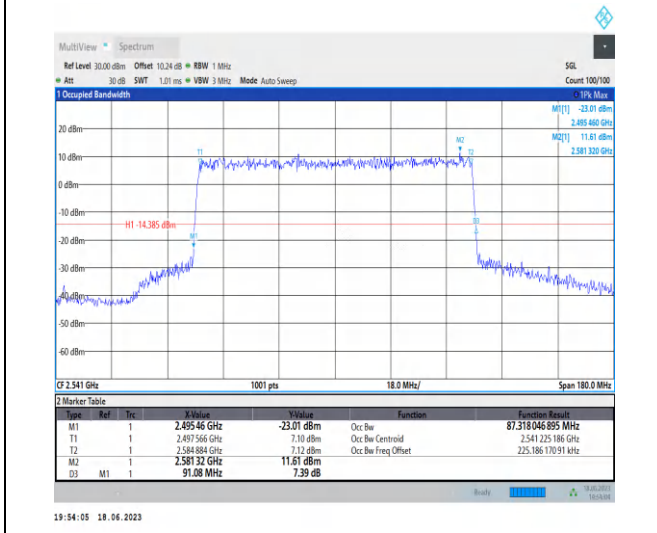
1-N41-PC3-30-90-L-6-CP-QPSK-Outer_Full-245 @ 0-Ant0-87.318-91.080-≤90-PASS
