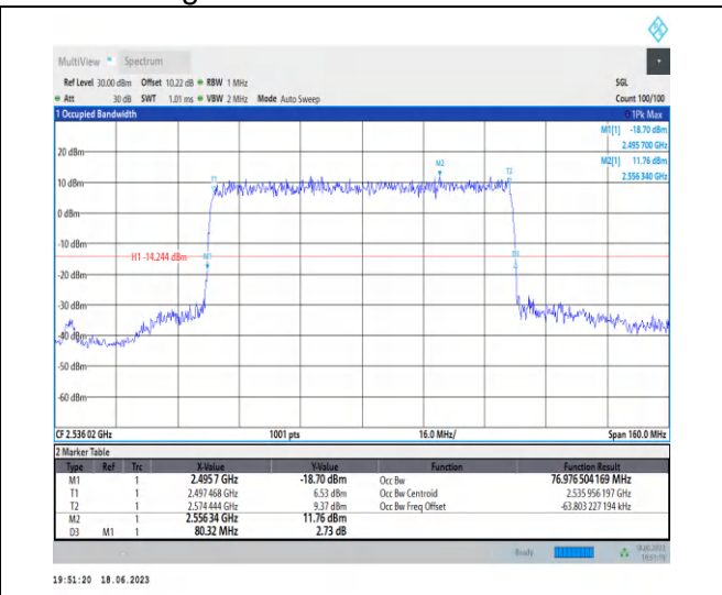
1-N41-PC3-30-80-L-4-DFT-64QAM-Outer_Full-216 @0-Ant0-76.977-80.320-≤80-PASS
