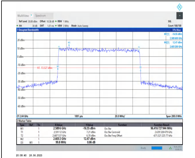
1-N41-PC3-30-100-H-4-DFT-64QAM-Outer_Full-270 @0-Ant0-96.417-99.800-≤100-PASS
