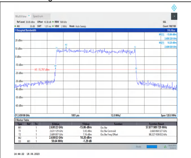
1-N41-PC3-30-60-H-4-DFT-64QAM-Outer_Full-162 @ 0-Ant0-57.878-59.640-≤60-PASS
