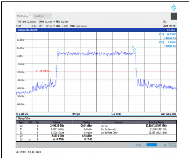
1-N41-PC3-30-60-L-9-CP-256QAM-Outer_Full-162 @0-Ant0-57.88-59.640-≤60-PASS
