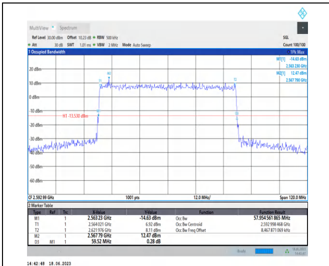
1-N41-PC3-30-60-M-4-DFT-64QAM-Outer_Full-162 @ 0-Ant0-57.955-59.520-≤60-PASS
