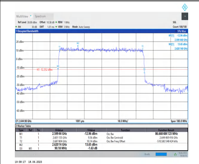
1-N41-PC3-30-90-H-1-DFT-Pl2BPSK-Outer_Full-243 @0-Ant0-86.668-90.180-≤90-PASS
