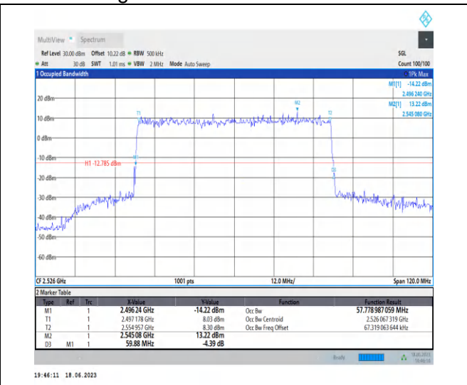
1-N41-PC3-30-60-L-2-DFT-QPSK-Outer_Full-162 @0-Ant0-57.779-59.880-≤60-PASS
