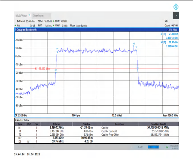
1-N41-PC3-30-60-L-4-DFT-64QAM-Outer_Full-162 @0-Ant0-57.77-59.760-≤60-PASS
