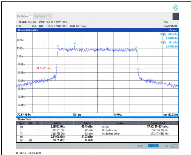
1-N41-PC3-30-90-H-6-CP-QPSK-Outer_Full-245@0 -Ant0-87.508-90.720-≤90-PASS
