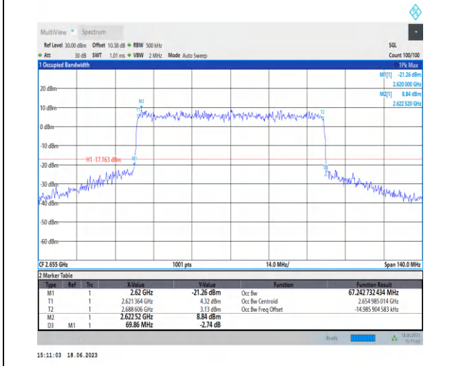
1-N41-PC3-30-70-H-6-CP-QPSK-Outer_Full-189@ 0-Ant0-67.243-69.860-≤70-PASS
