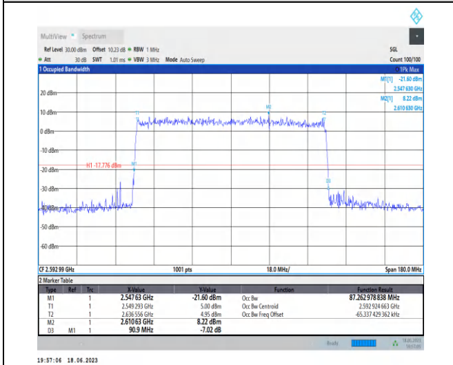
1-N41-PC3-30-90-M-9-CP-256QAM-Outer_Full-245 @0-Ant0-87.263-90.900-≤90-PASS
