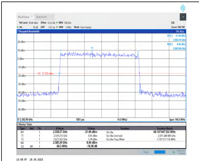
1-N41-PC3-30-70-M-5-DFT-256QAM-Outer_Full-180 @ 0-Ant0-64.148-66.500-≤70-PASS
