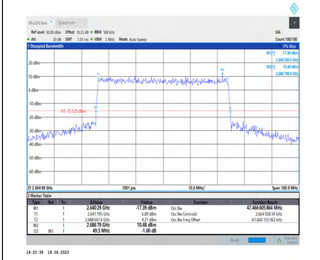
1-N41-PC3-30-50-H-8-CP-64QAM-Outer_Full-133@0 -Ant0-47.467-49.500-≤50-PASS
