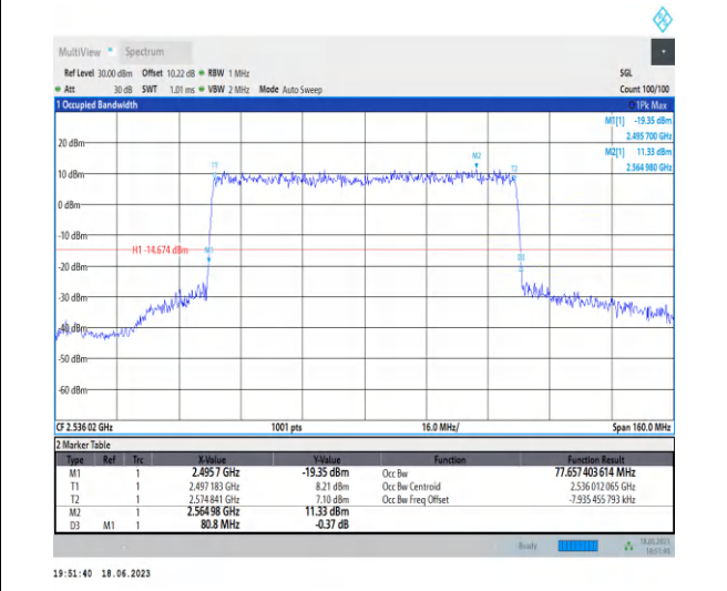
1-N41-PC3-30-80-L-6-CP-QPSK-Outer_Full-217 @0-Ant0-77.657-80.800-≤80-PASS
