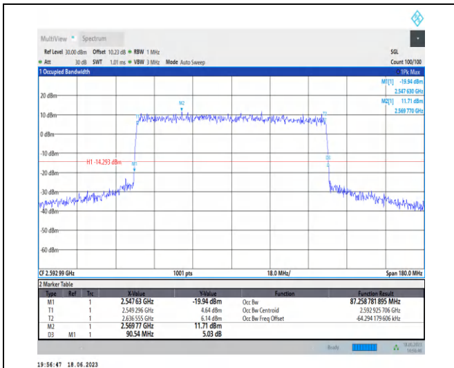
1-N41-PC3-30-90-M-7-CP-16QAM-Outer_Full-245@ 0-Ant0-87.259-90.540-≤90-PASS
