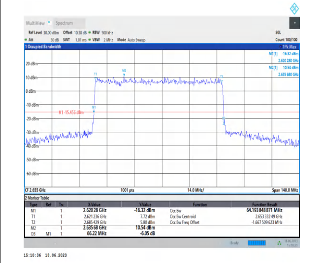
1-N41-PC3-30-70-H-3-DFT-16QAM-Outer_Full-180 @ 0-Ant0-64.194-66.220-≤70-PASS
