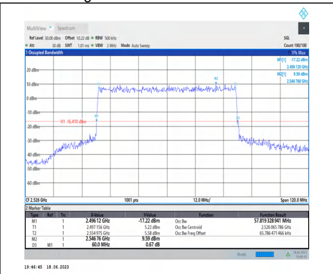
1-N41-PC3-30-60-L-6-CP-QPSK-Outer_Full-162 @ 0-Ant0-57.819-60.000-≤60-PASS
