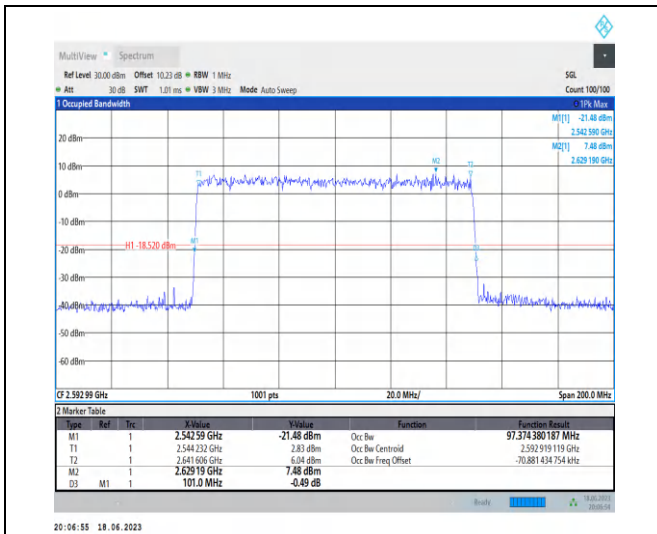
1-N41-PC3-30-100-M-9-CP-256QAM-Outer_Full-273 @0-Ant0-97.374-101.000-≤100-PASS
