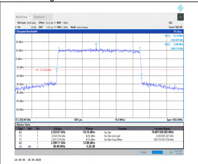
1-N41-PC3-30-80-M-3-DFT-16QAM-Outer_Full-216 @0-Ant0-76.898-80.480-≤80-PASS
