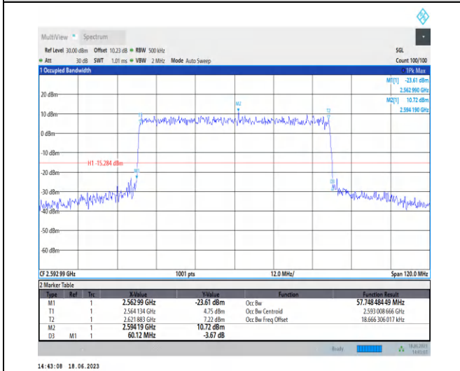
1-N41-PC3-30-60-M-6-CP-QPSK-Outer_Full-162 @ 0-Ant0-57.748-60.120-≤60-PASS
