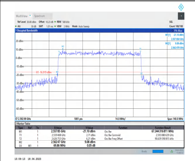
1-N41-PC3-30-70-M-8-CP-64QAM-Outer_Full-189 @ 0-Ant0-67.344-69.860-≤70-PASS
