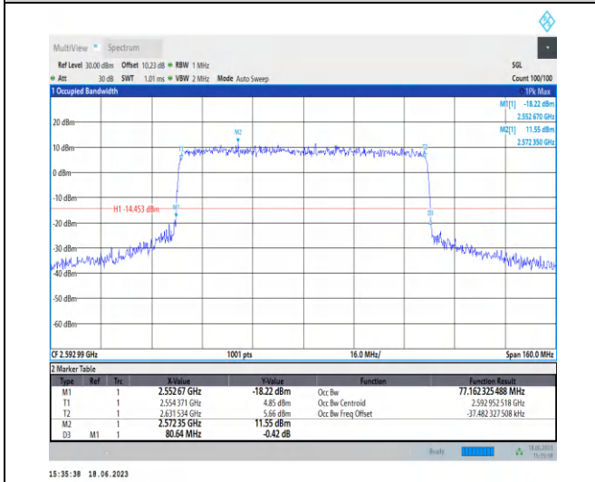
1-N41-PC3-30-80-M-8-CP-64QAM-Outer_Full-217@0 -Ant0-77.162-80.640-≤80-PASS
