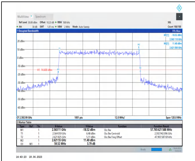
1-N41-PC3-30-60-M-8-CP-64QAM-Outer_Full-162@ 0-Ant0-57.766-59.520-≤60-PASS
