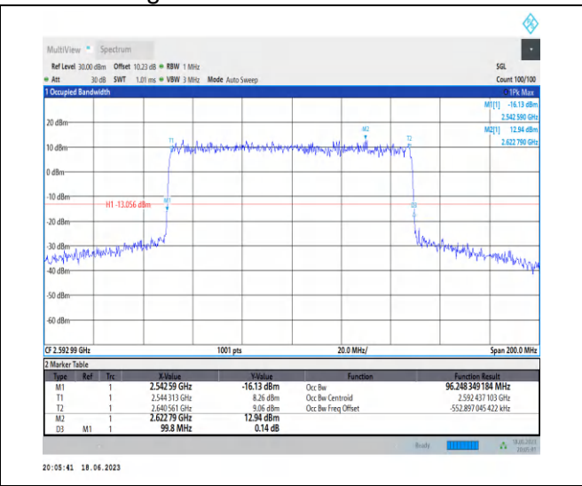
1-N41-PC3-30-100-M-2-DFT-QPSK-Outer_Full-270 @ 0-Ant0-96.248-99.800-≤100-PASS
