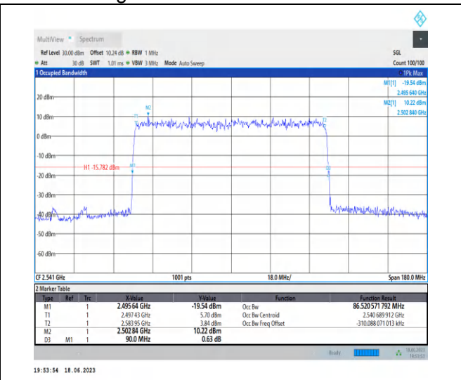
1-N41-PC3-30-90-L-5-DFT-256QAM-Outer_Full-243 @ 0-Ant0-86.521-90.000-≤90-PASS
