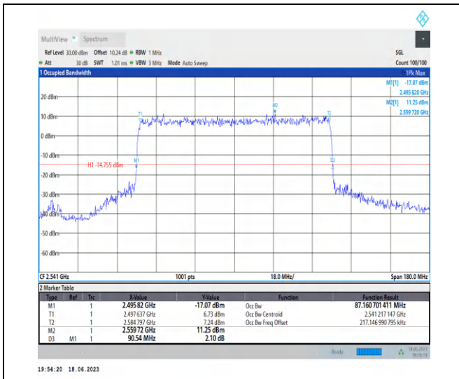
1-N41-PC3-30-90-L-8-CP-64QAM-Outer_Full-245@ 0-Ant0-87.161-90.540-≤90-PASS
