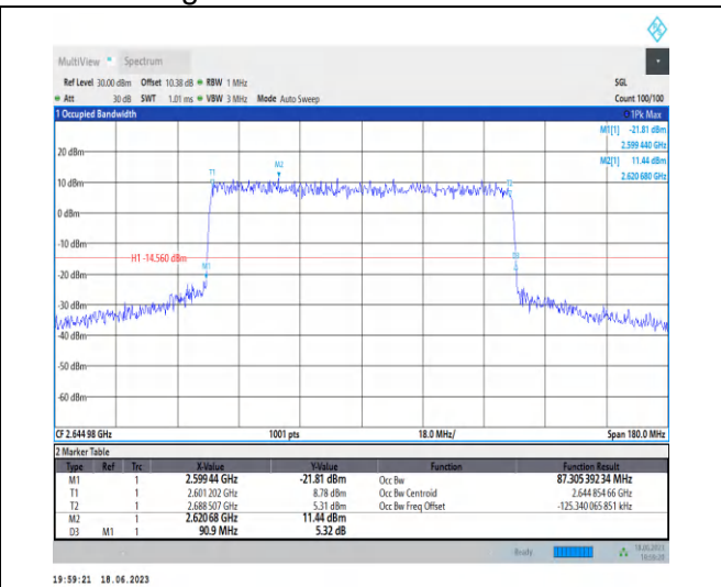
1-N41-PC3-30-90-H-7-CP-16QAM-Outer_Full-245@0 -Ant0-87.305-90.900-≤90-PASS
