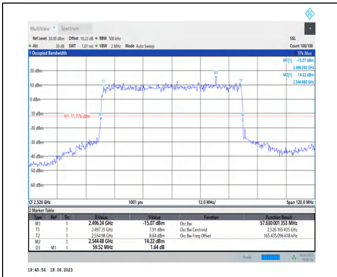
1-N41-PC3-30-60-L-1-DFT-PI2BPSK-Outer_Full-162 @0-Ant0-57.63-59.520-≤60-PASS
