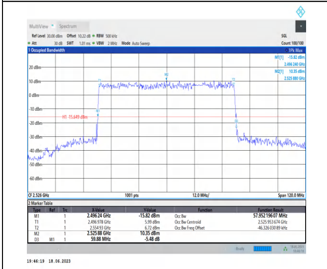
1-N41-PC3-30-60-L-3-DFT-16QAM-Outer_Full-162 @0-Ant0-57.952-59.880-≤60-PASS
