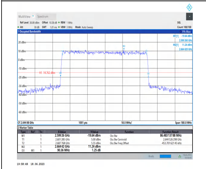
1-N41-PC3-30-90-H-4-DFT-64QAM-Outer_Full-243 @0-Ant0-86.483-90.360-≤90-PASS
