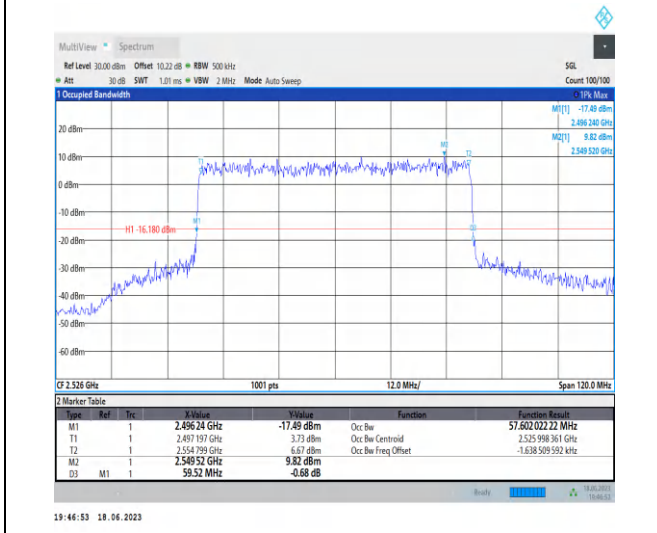
1-N41-PC3-30-60-L-7-CP-16QAM-Outer_Full-162 @ 0-Ant0-57.602-59.520-≤60-PASS
