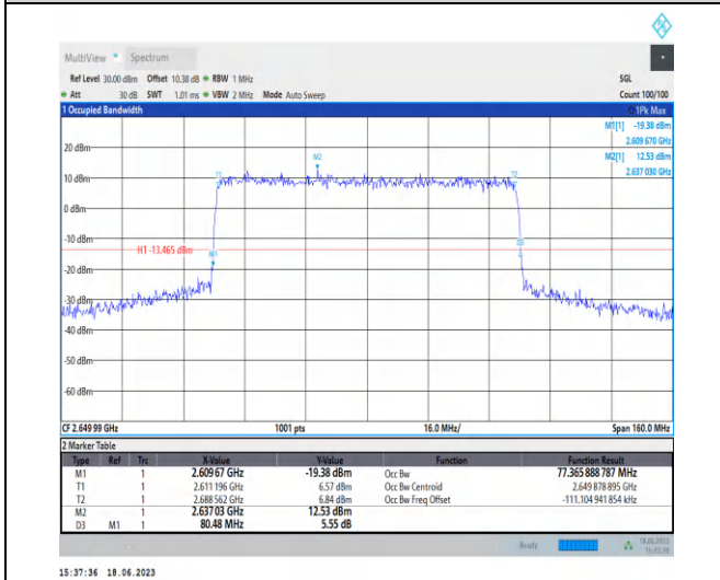
1-N41-PC3-30-80-H-7-CP-16QAM-Outer_Full-217 @ 0-Ant0-77.366-80.480-≤80-PASS
