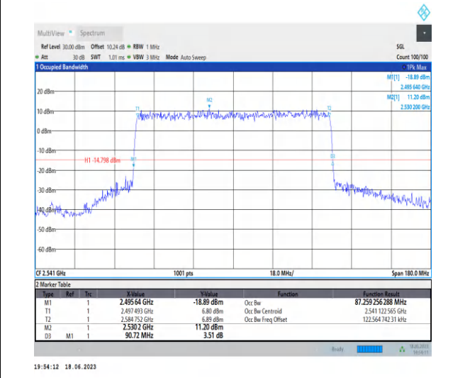
1-N41-PC3-30-90-L-7-CP-16QAM-Outer_Full-245 @ 0-Ant0-87.259-90.720-≤90-PASS
