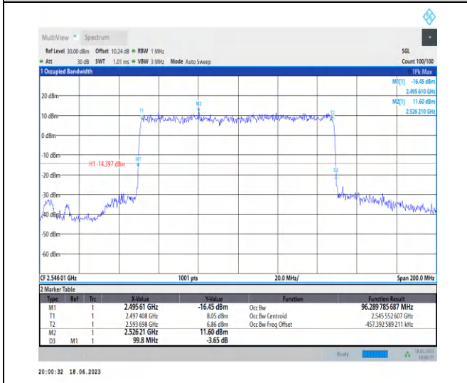
1-N41-PC3-30-100-L-3-DFT-16QAM-Outer_Full-270 @ 0-Ant0-96.29-99.800-≤100-PASS
