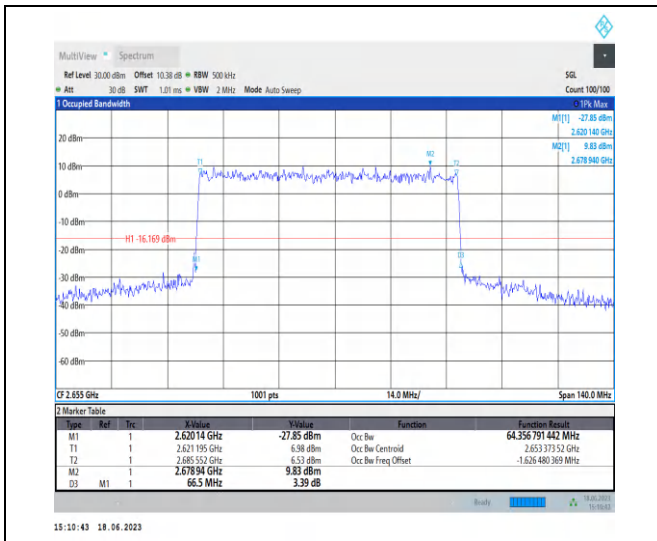
1-N41-PC3-30-70-H-4-DFT-64QAM-Outer_Full-180 @ 0-Ant0-64.357-66.500-≤70-PASS
