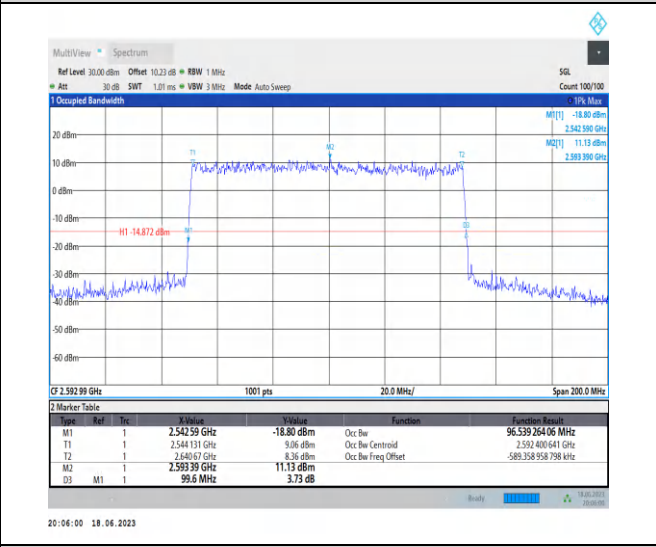
1-N41-PC3-30-100-M-4-DFT-64QAM-Outer_Full-270 @ 0-Ant0-96.539-99.600-≤100-PASS
