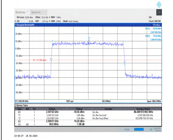
1-N41-PC3-30-90-M-5-DFT-256QAM-Outer_Full-243 @0-Ant0-86.47-90.000-≤90-PASS
