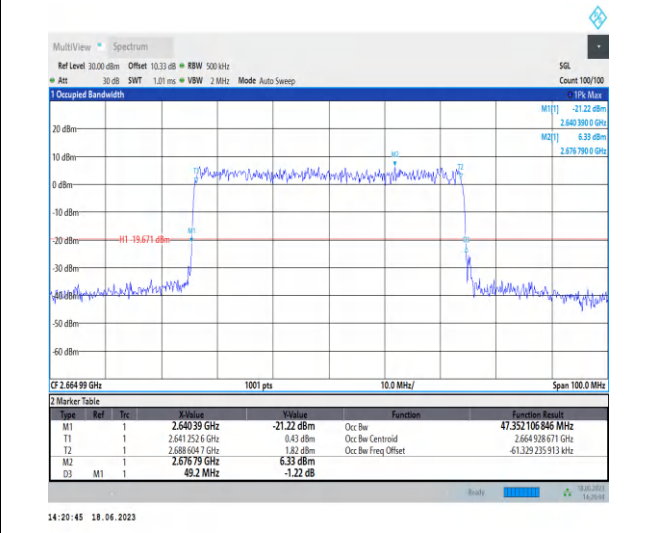
1-N41-PC3-30-50-H-9-CP-256QAM-Outer_Full-133@0 -Ant0-47.352-49.200-≤50-PASS
