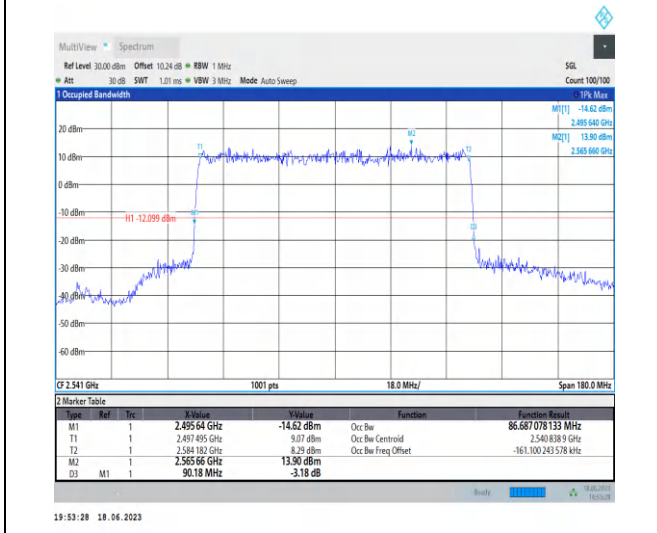
1-N41-PC3-30-90-L-2-DFT-QPSK-Outer_Full-243 @ 0-Ant0-86.687-90.180-≤90-PASS
