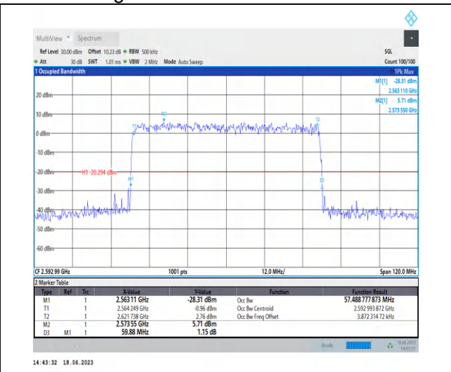
1-N41-PC3-30-60-M-9-CP-256QAM-Outer_Full-162 @0-Ant0-57.489-59.880-≤60-PASS
