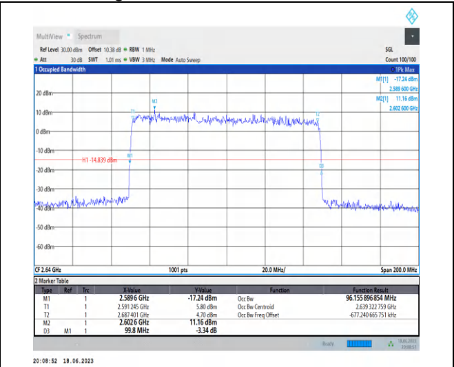
1-N41-PC3-30-100-H-5-DFT-256QAM-Outer_Full-270 @0-Ant0-96.156-99.800-≤100-PASS
