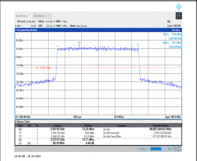
1-N41-PC3-30-90-M-2-DFT-QPSK-Outer_Full-243@ 0-Ant0-86.897-90.180-≤90-PASS
