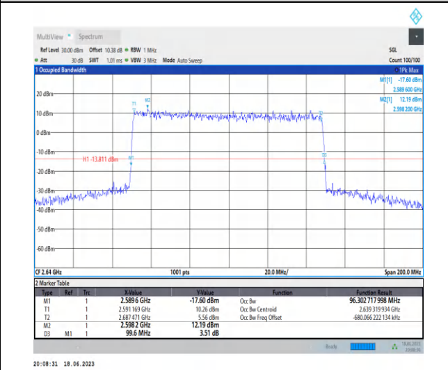
1-N41-PC3-30-100-H-3-DFT-16QAM-Outer_Full-270 @0-Ant0-96.303-99.600-≤100-PASS
