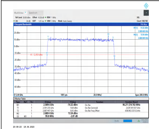
1-N41-PC3-30-100-H-2-DFT-QPSK-Outer_Full-270 @0-Ant0-96.211-99.800-≤100-PASS
