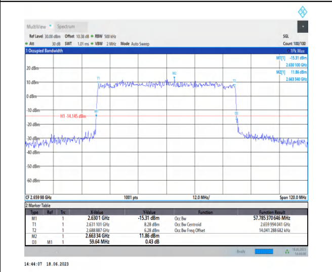
1-N41-PC3-30-60-H-2-DFT-QPSK-Outer_Full-162@ 0-Ant0-57.785-59.640-≤60-PASS
