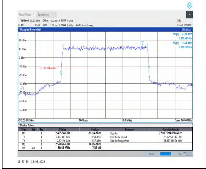
1-N41-PC3-30-80-L-1-DFT-PI2BPSK-Outer_Full-216 @0-Ant0-77.017-80.480-≤80-PASS
