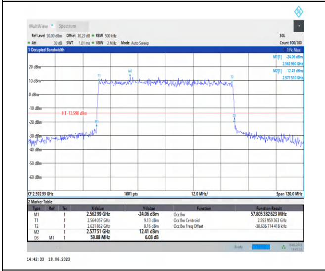
1-N41-PC3-30-60-M-2-DFT-QPSK-Outer_Full-162 @0-Ant0-57.805-59.880-≤60-PASS
