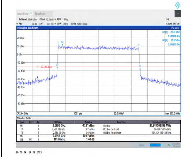
1-N41-PC3-30-100-H-6-CP-QPSK-Outer_Full-273 @0-Ant0-97.349-101.000-≤100-PASS
