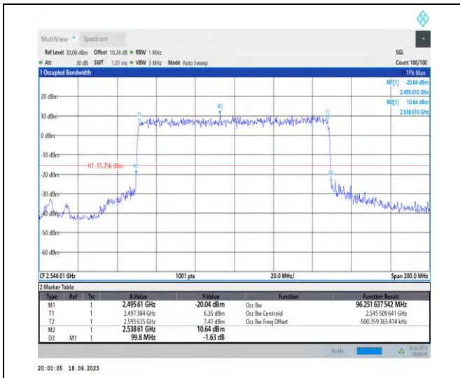
1-N41-PC3-30-100-L-1-DFT-PI2BPSK-Outer_Full-270 @ 0-Ant0-96.252-99.800-≤100-PASS
