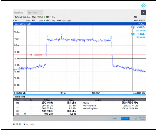
1-N41-PC3-30-100-M-3-DFT-16QAM-Outer_Full-270 @ 0-Ant0-96.399-99.800-≤100-PASS
