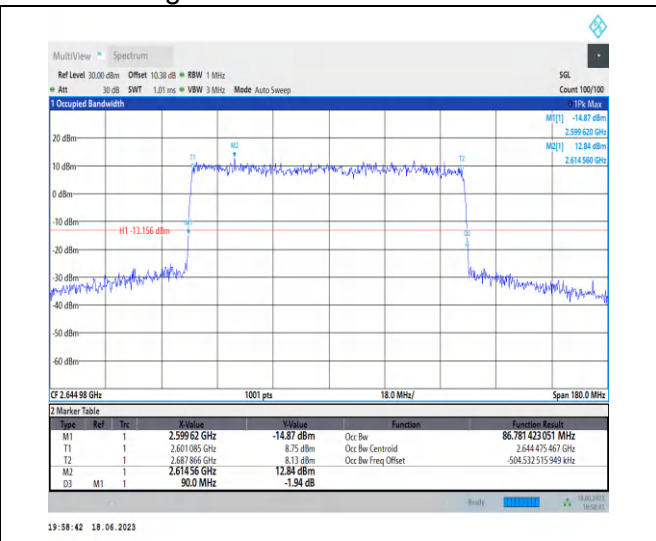
1-N41-PC3-30-90-H-3-DFT-16QAM-Outer_Full-243 @0-Ant0-86.781-90.000-≤90-PASS
