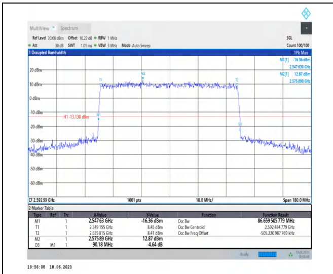
1-N41-PC3-30-90-M-3-DFT-16QAM-Outer_Full-243 @0-Ant0-86.66-90.180-≤90-PASS
