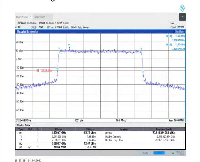
1-N41-PC3-30-80-H-6-CP-QPSK-Outer_Full-217 @ 0-Ant0-77.318-80.640-≤80-PASS
