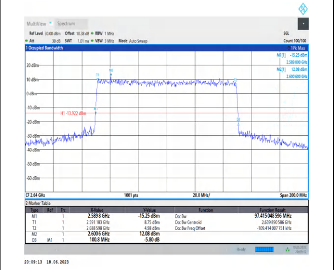
1-N41-PC3-30-100-H-7-CP-16QAM-Outer_Full-273 @0-Ant0-97.415-100.800-≤100-PASS
