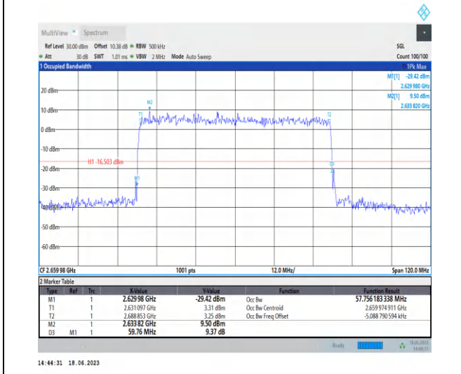
1-N41-PC3-30-60-H-5-DFT-256QAM-Outer_Full-162 @ 0-Ant0-57.756-59.760-≤60-PASS
