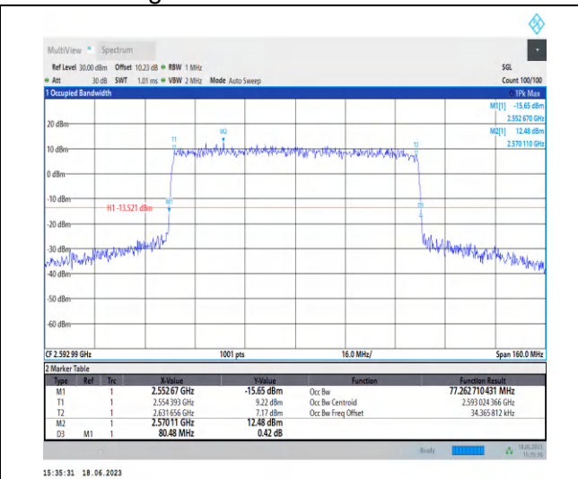
1-N41-PC3-30-80-M-7-CP-16QAM-Outer_Full-217@0 -Ant0-77.263-80.480-≤80-PASS
