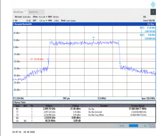
1-N41-PC3-30-60-L-8-CP-64QAM-Outer_Full-162 @ 0-Ant0-57.684-60.240-≤60-PASS
