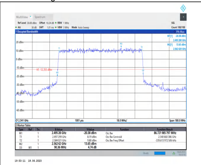
1-N41-PC3-30-90-L-1-DFT-PI2BPSK-Outer_Full-243 @ 0-Ant0-86.722-90.360-≤90-PASS
