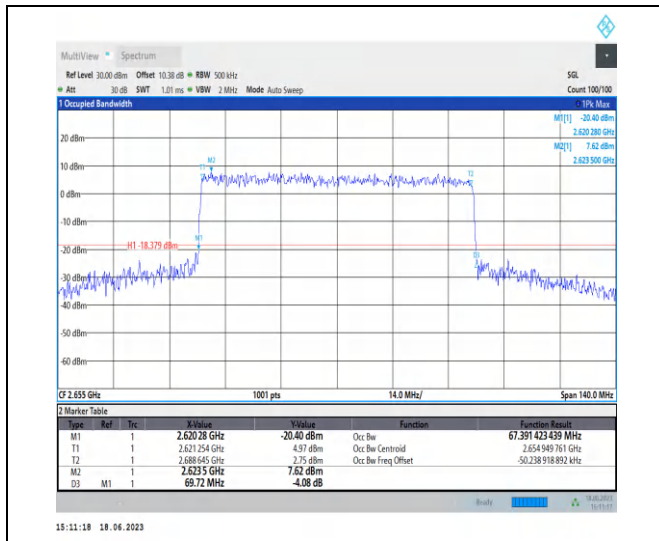
1-N41-PC3-30-70-H-8-CP-64QAM-Outer_Full-189@ 0-Ant0-67.391-69.720-≤70-PASS
