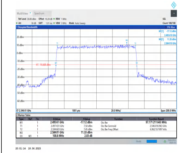
1-N41-PC3-30-100-L-7-CP-16QAM-Outer_Full-273 @0-Ant0-97.171-100.800-≤100-PASS
