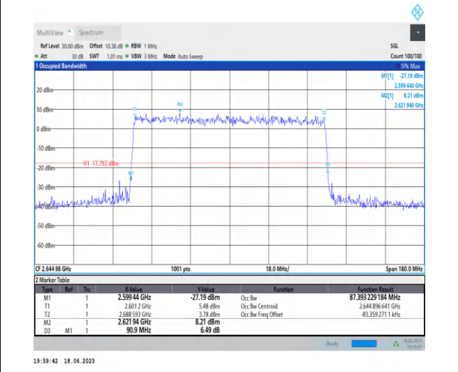
1-N41-PC3-30-90-H-9-CP-256QAM-Outer_Full-245@0 -Ant0-87.393-90.900-≤90-PASS
