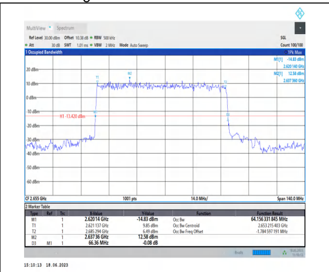
1-N41-PC3-30-70-H-1-DFT-PI2BPSK-Outer_Full-180 @ 0-Ant0-64.156-66.360-≤70-PASS
