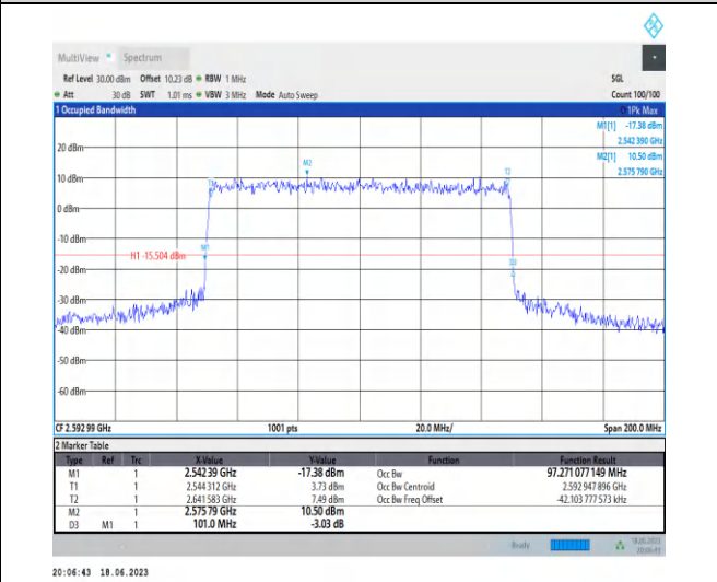
1-N41-PC3-30-100-M-8-CP-64QAM-Outer_Full-273 @ 0-Ant0-97.271-101.000-≤100-PASS
