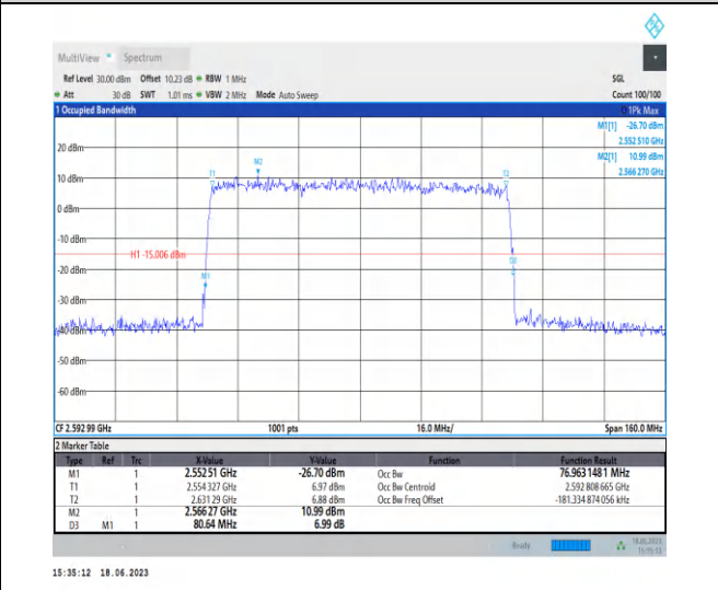
1-N41-PC3-30-80-M-5-DFT-256QAM-Outer_Full-216 @0-Ant0-76.963-80.640-≤80-PASS
