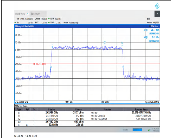
1-N41-PC3-30-60-H-9-CP-256QAM-Outer_Full-162 @0-Ant0-57.649-60.000-≤60-PASS
