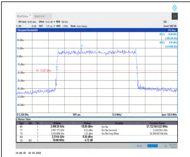
1-N41-PC3-30-60-L-5-DFT-256QAM-Outer_Full-162 @ 0-Ant0-57.723-59.880-≤60-PASS
