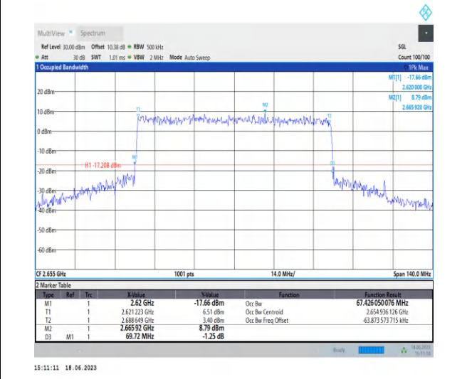
1-N41-PC3-30-70-H-7-CP-16QAM-Outer_Full-189@ 0-Ant0-67.426-69.720-≤70-PASS
