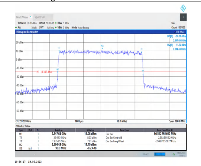
1-N41-PC3-30-90-M-4-DFT-64QAM-Outer_Full-243 @0-Ant0-86.513-90.000-≤90-PASS
