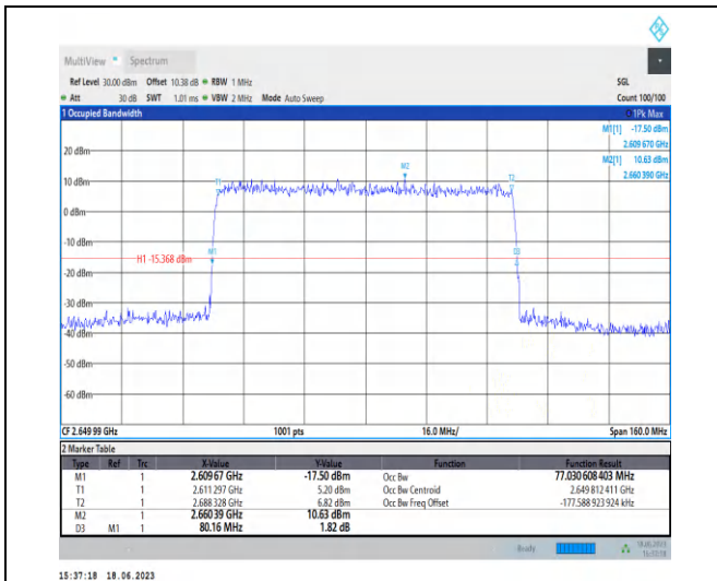
1-N41-PC3-30-80-H-5-DFT-256QAM-Outer_Full-216 @ 0-Ant0-77.031-80.160-≤80-PASS
