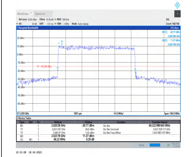
1-N41-PC3-30-70-H-2-DFT-QPSK-Outer_Full-180 @ 0-Ant0-64.223-66.220-≤70-PASS
