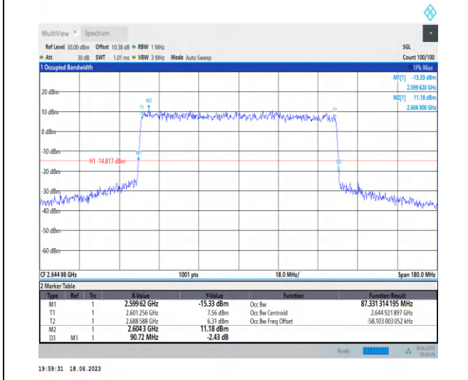
1-N41-PC3-30-90-H-8-CP-64QAM-Outer_Full-245@0 -Ant0-87.331-90.720-≤90-PASS
