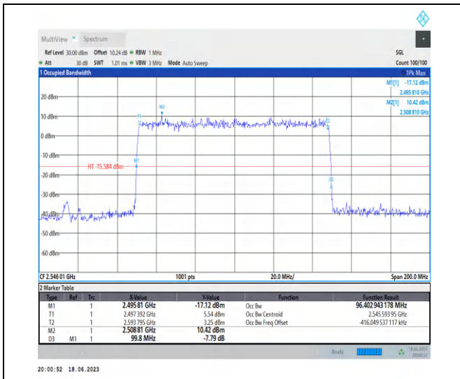
1-N41-PC3-30-100-L-5-DFT-256QAM-Outer_Full-27 @0-Ant0-96.403-99.800-≤100-PASS
