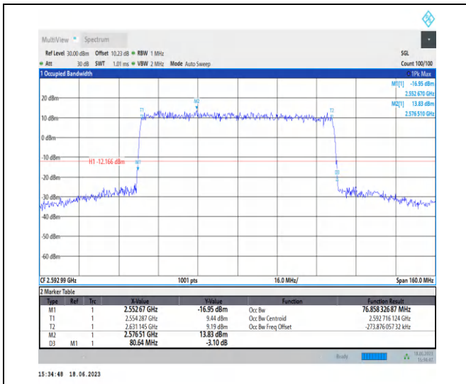
1-N41-PC3-30-80-M-2-DFT-QPSK-Outer_Full-216@ @0-Ant0-76.858-80.640-≤80-PASS
