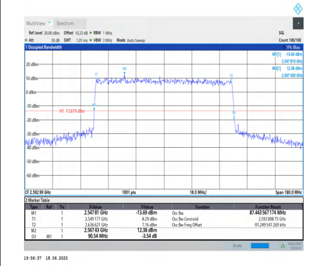
1-N41-PC3-30-90-M-6-CP-QPSK-Outer_Full-245 @0-Ant0-87.444-90.540-≤90-PASS
