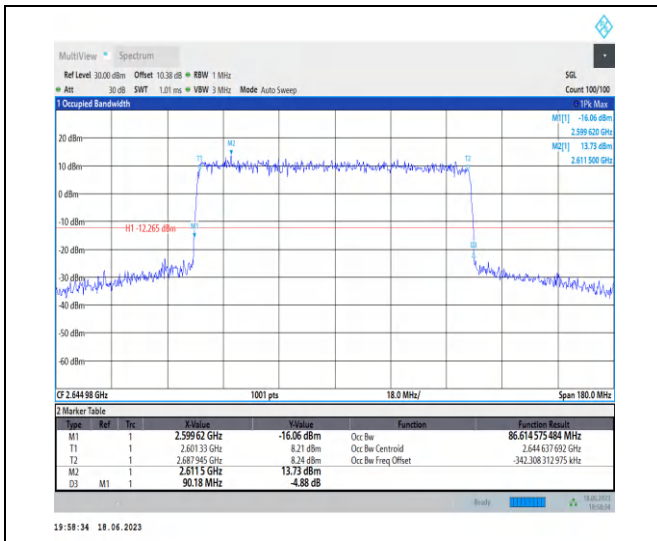
1-N41-PC3-30-90-H-2-DFT-QPSK-Outer_Full-243@ @0-Ant0-86.615-90.180-≤90-PASS
