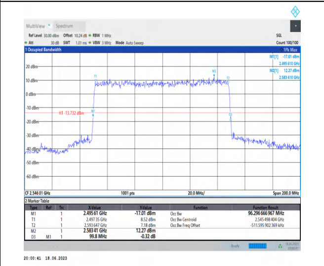
1-N41-PC3-30-100-L-4-DFT-64QAM-Outer_Full-270 @ 0-Ant0-96.297-99.800-≤100-PASS
