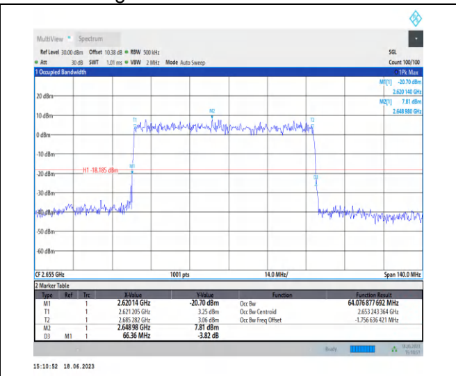
1-N41-PC3-30-70-H-5-DFT-256QAM-Outer_Full-180 @ 0-Ant0-64.077-66.360-≤70-PASS
