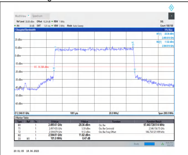
1-N41-PC3-30-100-L-6-CP-QPSK-Outer_Full-273@ @0-Ant0-97.444-101.000-≤100-PASS
