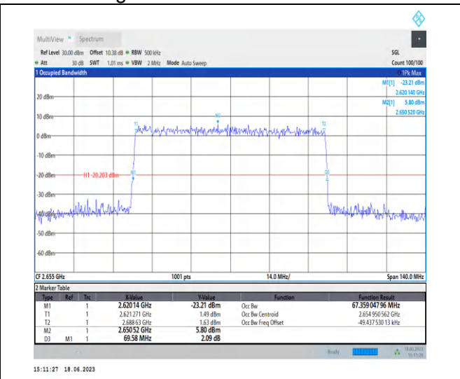
1-N41-PC3-30-70-H-9-CP-256QAM-Outer_Full-189 @0-Ant0-67.359-69.580-≤70-PASS
