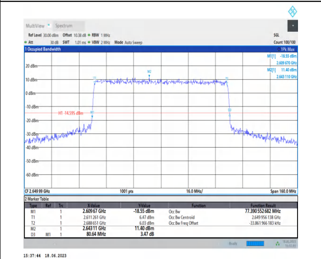
1-N41-PC3-30-80-H-8-CP-64QAM-Outer_Full-217 @ 0-Ant0-77.391-80.640-≤80-PASS
