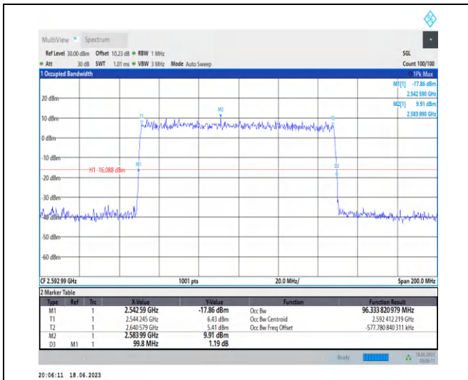
1-N41-PC3-30-100-M-5-DFT-256QAM-Outer_Full-27 @ 0-Ant0-96.334-99.800-≤100-PASS
