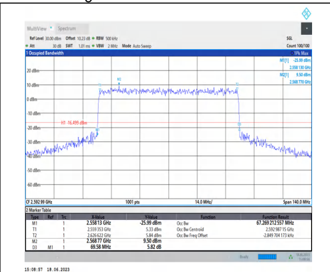
1-N41-PC3-30-70-M-6-CP-QPSK-Outer_Full-189 @ 0-Ant0-67.269-69.580-≤70-PASS
