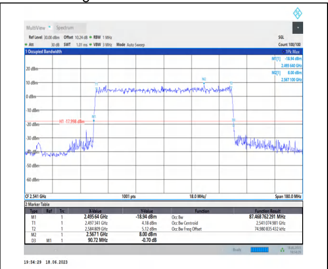
1-N41-PC3-30-90-L-9-CP-256QAM-Outer_Full-245 @0-Ant0-87.469-90.720-≤90-PASS
