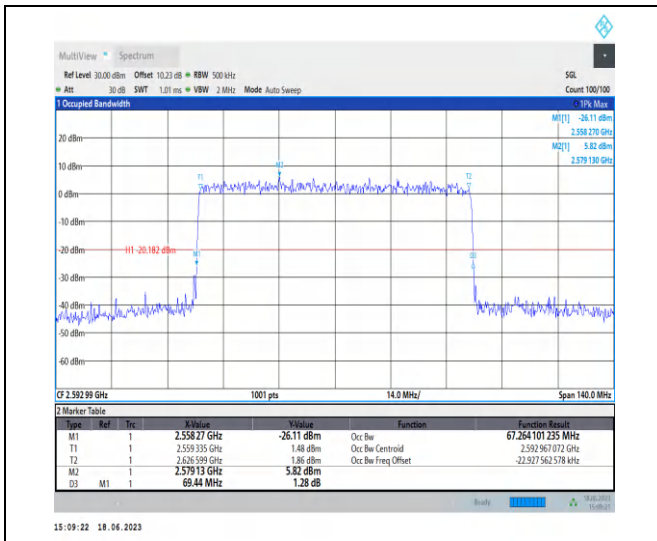
1-N41-PC3-30-70-M-9-CP-256QAM-Outer_Full-189 @ 0-Ant0-67.264-69.440-≤70-PASS
