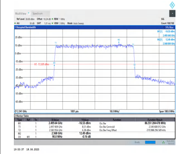
1-N41-PC3-30-90-L-3-DFT-16QAM-Outer_Full-243 @ 0-Ant0-86.551-90.000-≤90-PASS
