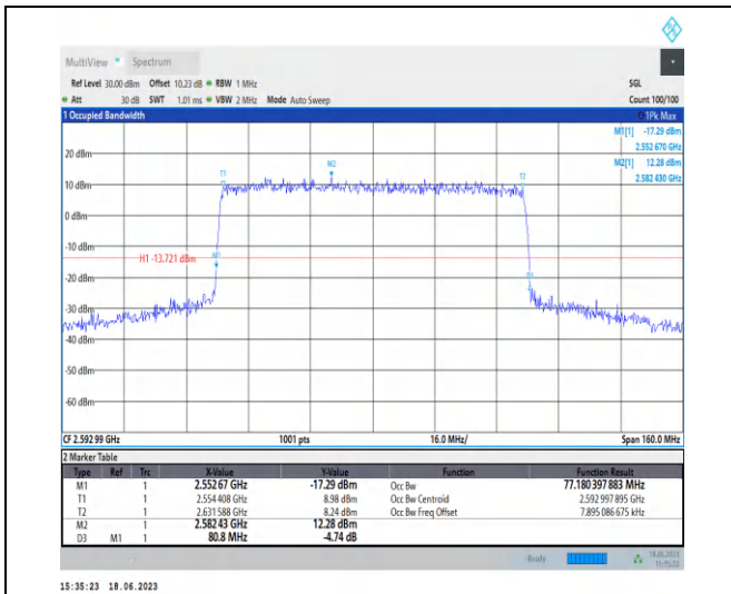
1-N41-PC3-30-80-M-6-CP-QPSK-Outer_Full-217@0 -Ant0-77.18-80.800-≤80-PASS
