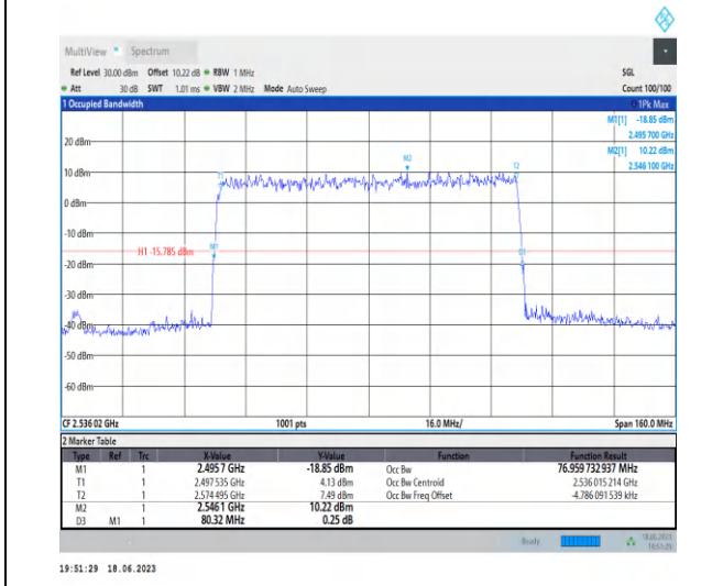
1-N41-PC3-30-80-L-5-DFT-256QAM-Outer_Full-216 @0-Ant0-76.96-80.320-≤80-PASS
