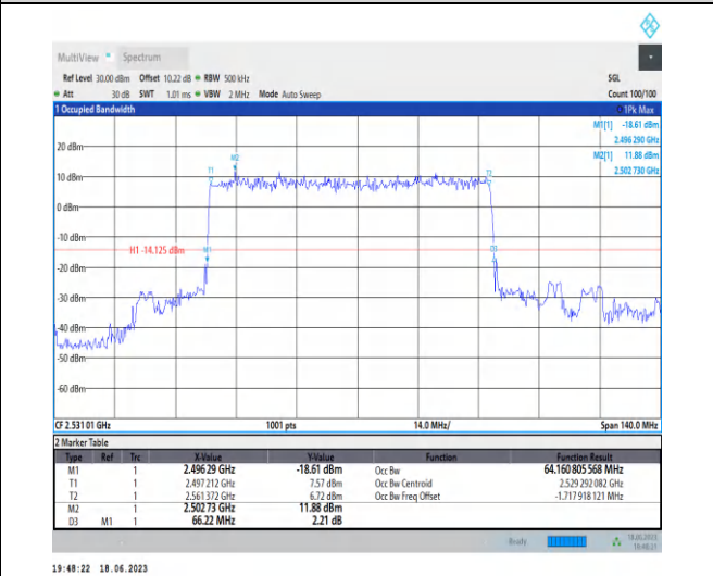
1-N41-PC3-30-70-L-1-DFT-PI2BPSK-Outer_Full-180 @0-Ant0-64.161-66.220-≤70-PASS
