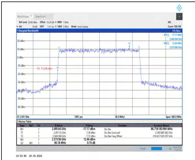
1-N41-PC3-30-90-L-4-DFT-64QAM-Outer_Full-243 @ 0-Ant0-86.718-90.180-≤90-PASS
