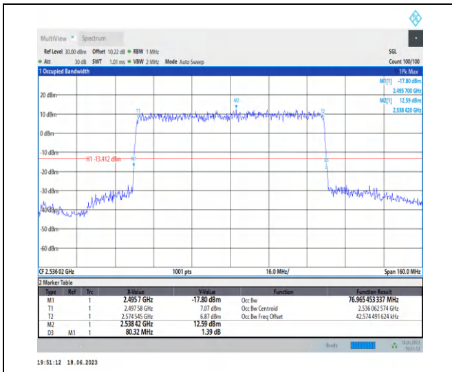
1-N41-PC3-30-80-L-3-DFT-16QAM-Outer_Full-216 @0-Ant0-76.965-80.320-≤80-PASS
