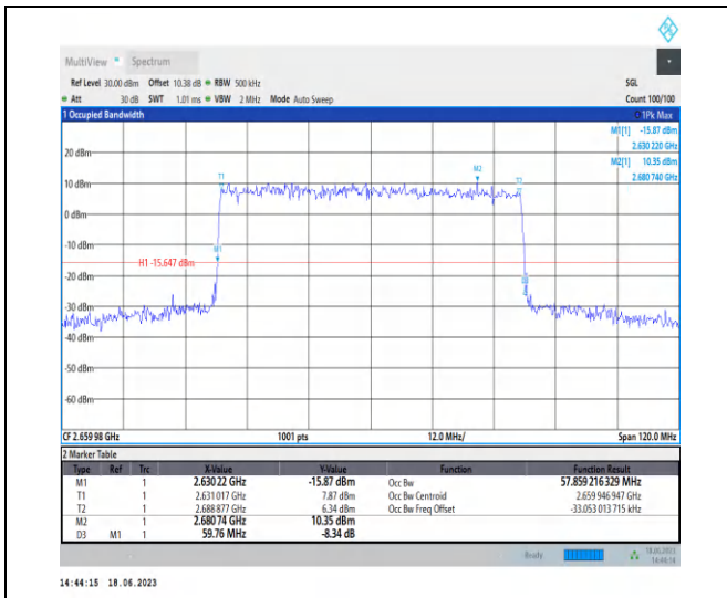
1-N41-PC3-30-60-H-3-DFT-16QAM-Outer_Full-162 @ 0-Ant0-57.859-59.760-≤60-PASS
