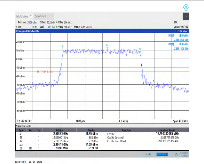
1-N41-PC3-30-20-M-3-DFT-16QAM-Outer_Full-50@ 0-Ant0-17.754-18.960-<=20-PASS
