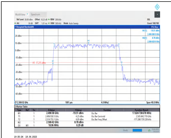
1-N41-PC3-30-20-L-5-DFT-256QAM-Outer_Full-50 @ 0-Ant0-17.825-18.960-≤20-PASS
