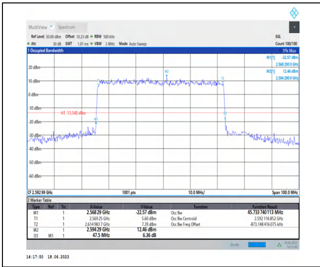
1-N41-PC3-30-50-M-3-DFT-16QAM-Outer_Full-128 @ 0-Ant0-45.734-47.500-≤50-PASS
