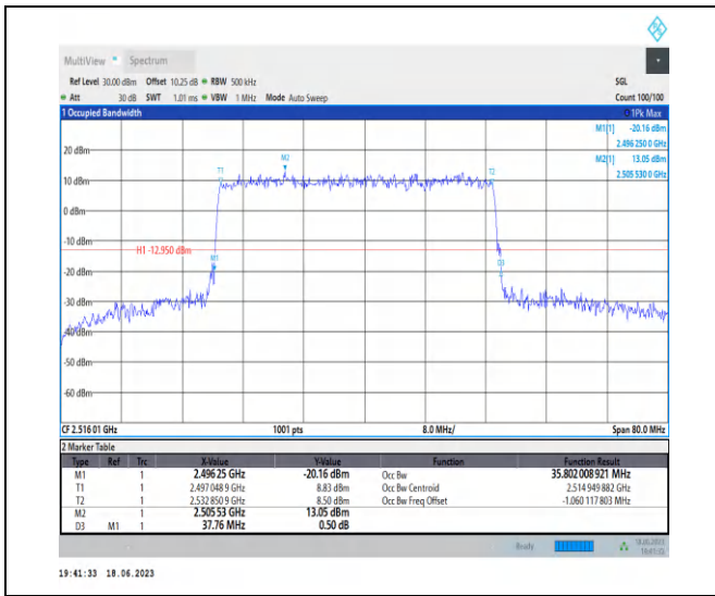
1-N41-PC3-30-40-L-3-DFT-16QAM-Outer_Full-100 @0-Ant0-35.802-37.760-≤40-PASS
