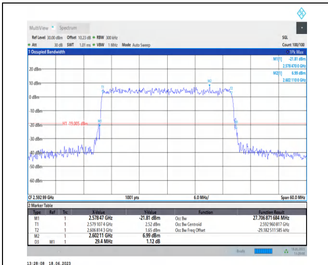
1-N41-PC3-30-30-M-9-CP-256QAM-Outer_Full-78@ 0-Ant0-27.707-29.400-≤30-PASS
