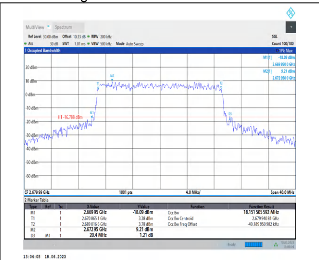
1-N41-PC3-30-20-H-8-CP-64QAM-Outer_Full-51@0 -Ant0-18.152-20.400-≤20-PASS
