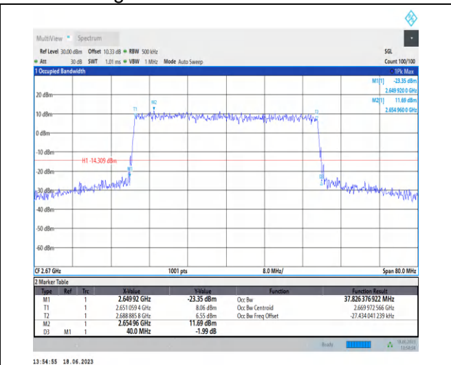
1-N41-PC3-30-40-H-6-CP-QPSK-Outer_Full-106 @ 0-Ant0-37.826-40.000-≤40-PASS
