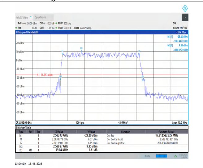
1-N41-PC3-30-20-M-5-DFT-256QAM-Outer_Full-50@ 0-Ant0-17.813-19.040-≤20-PASS
