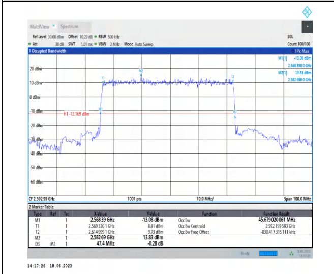
1-N41-PC3-30-50-M-1-DFT-PI2BPSK-Outer_Full-128 8@0-Ant0-45.679-47.400-≤50-PASS
