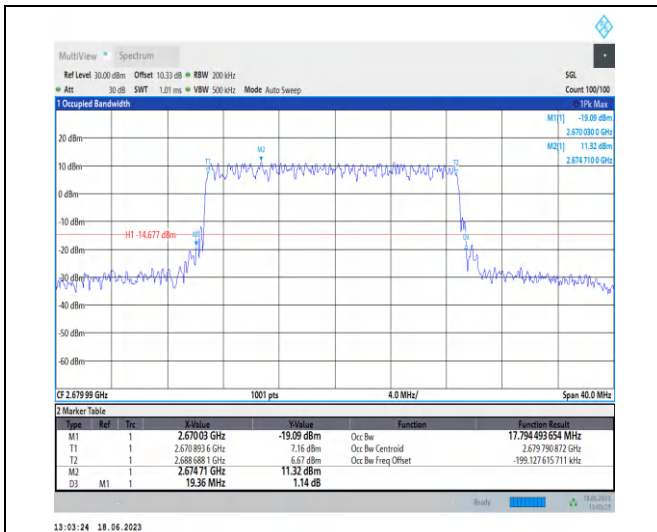
1-N41-PC3-30-20-H-3-DFT-16QAM-Outer_Full-50@ 0-Ant0-17.794-19.360-≤20-PASS
