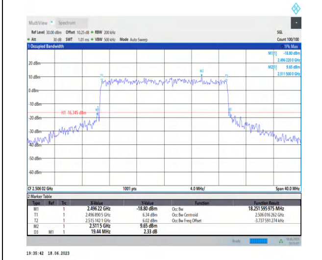
1-N41-PC3-30-20-L-7-CP-16QAM-Outer_Full-51 @ 0-Ant0-18.252-19.440-≤20-PASS
