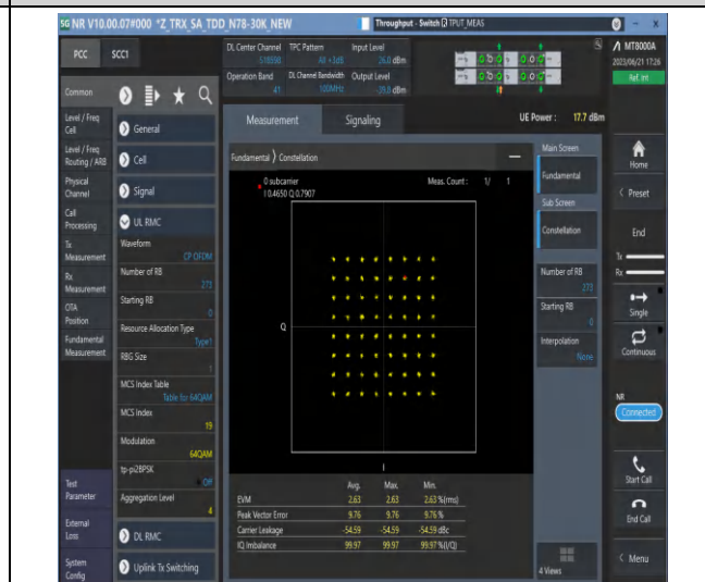
1-N41-PC3-30-100-M-8-CP-64QAM-Outer_Full-273 @0-Ant0-see graph-PASS
