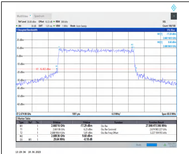
1-N41-PC3-30-30-H-8-CP-64QAM-Outer_Full-78@0 -Ant0-27.846-29.640-≤30-PASS
