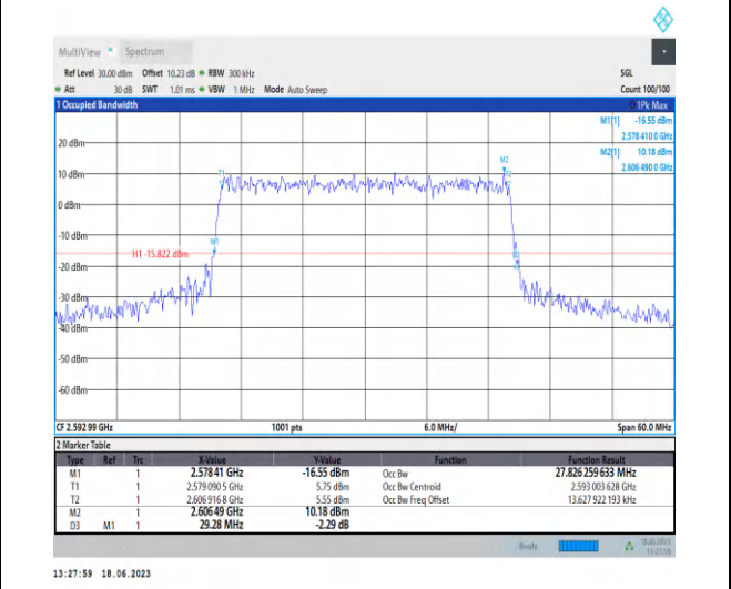
1-N41-PC3-30-30-M-8-CP-64QAM-Outer_Full-78 @ 0 -Ant0-27.826-29.280-≤30-PASS
