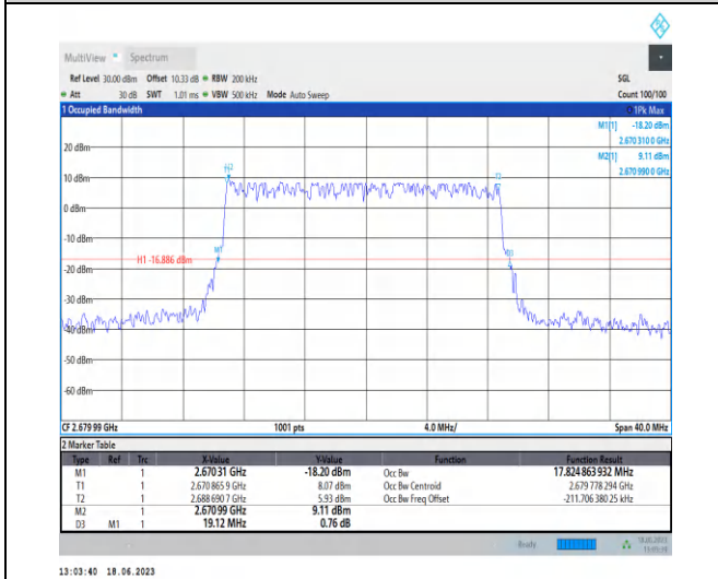
1-N41-PC3-30-20-H-5-DFT-256QAM-Outer_Full-50 @0-Ant0-17.825-19.120-≤20-PASS
