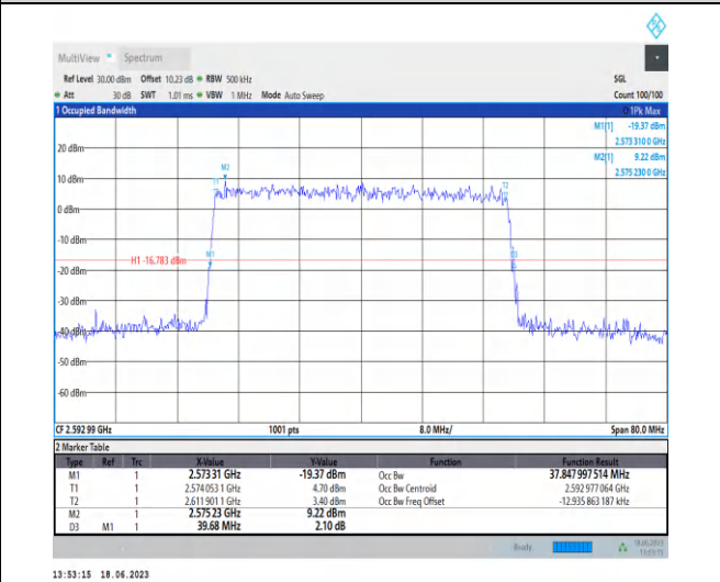
1-N41-PC3-30-40-M-9-CP-256QAM-Outer_Full-106@0 -Ant0-37.848-39.680-≤40-PASS
