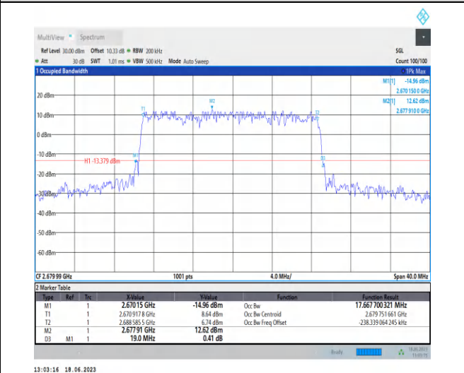
1-N41-PC3-30-20-H-2-DFT-QPSK-Outer_Full-50 @ 0-Ant0-17.668-19.000-≤20-PASS
