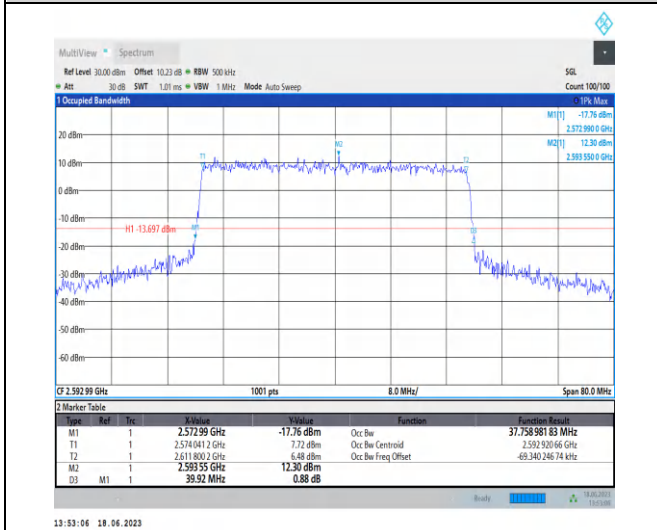
1-N41-PC3-30-40-M-8-CP-64QAM-Outer_Full-106@0 -Ant0-37.759-39.920-≤40-PASS
