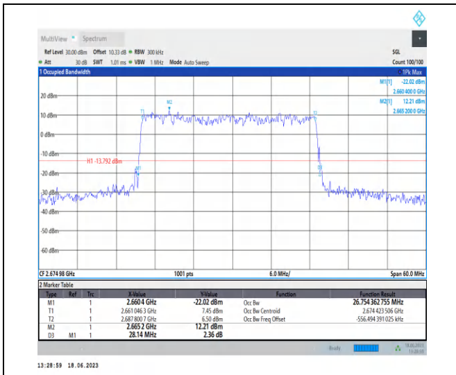
1-N41-PC3-30-30-H-4-DFT-64QAM-Outer_Full-75@ 0-Ant0-26.754-28.140-≤30-PASS
