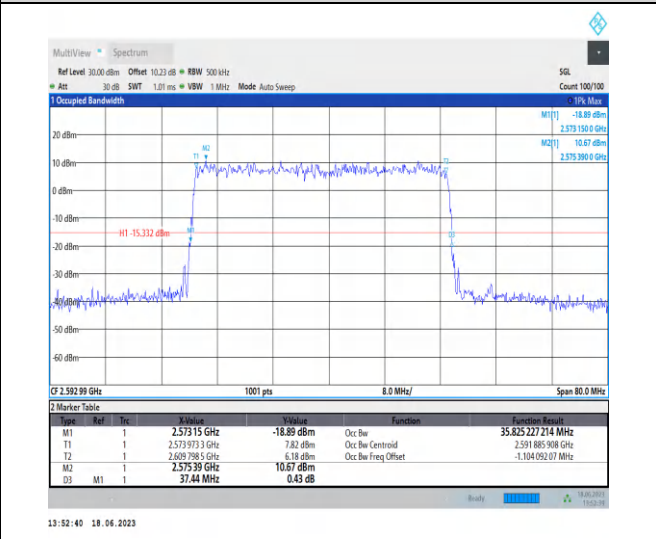
1-N41-PC3-30-40-M-5-DFT-256QAM-Outer_Full-100 @0-Ant0-35.825-37.440-≤40-PASS
