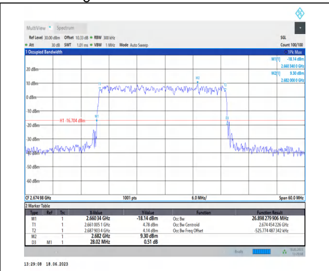
1-N41-PC3-30-30-H-5-DFT-256QAM-Outer_Full-75@ 0-Ant0-26.898-28.020-≤30-PASS
