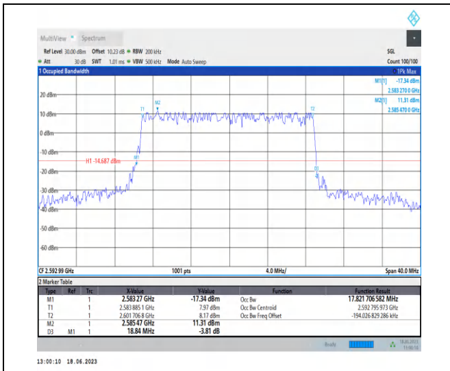
1-N41-PC3-30-20-M-4-DFT-64QAM-Outer_Full-50@ 0-Ant0-17.822-18.840-≤20-PASS
