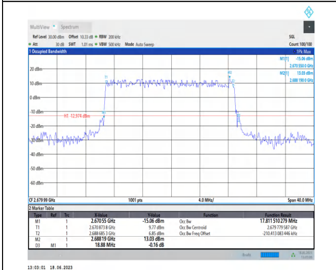
1-N41-PC3-30-20-H-1-DFT-PI2BPSK-Outer_Full-50 @ 0-Ant0-17.812-18.880-≤20-PASS
