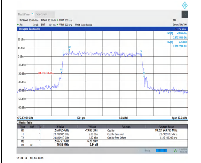
1-N41-PC3-30-20-H-9-CP-256QAM-Outer_Full-51@0 0-Ant0-18.201-19.360-≤20-PASS
