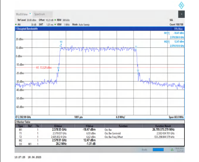
1-N41-PC3-30-30-M-4-DFT-64QAM-Outer_Full-75 @ 0-Ant0-26.795-28.200-≤30-PASS
