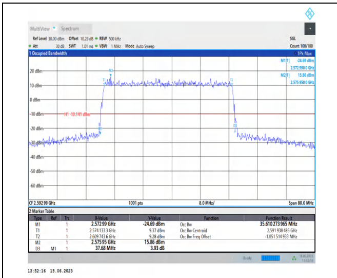
1-N41-PC3-30-40-M-2-DFT-QPSK-Outer_Full-100@ @0-Ant0-35.61-37.680-≤40-PASS
