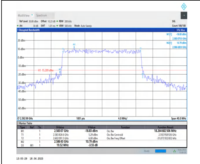
1-N41-PC3-30-20-M-6-CP-QPSK-Outer_Full-51@0- Ant0-18.265-19.520-≤20-PASS
