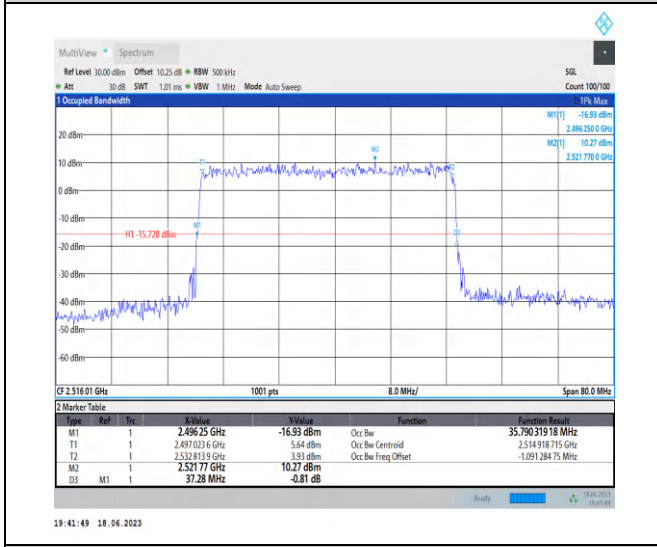
1-N41-PC3-30-40-L-5-DFT-256QAM-Outer_Full-100 @0-Ant0-35.79-37.280-≤40-PASS
