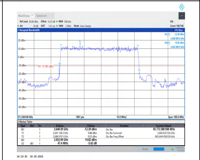
1-N41-PC3-30-50-H-1-DFT-PI2BPSK-Outer_Full-128 @0-Ant0-45.772-47.400-≤50-PASS
