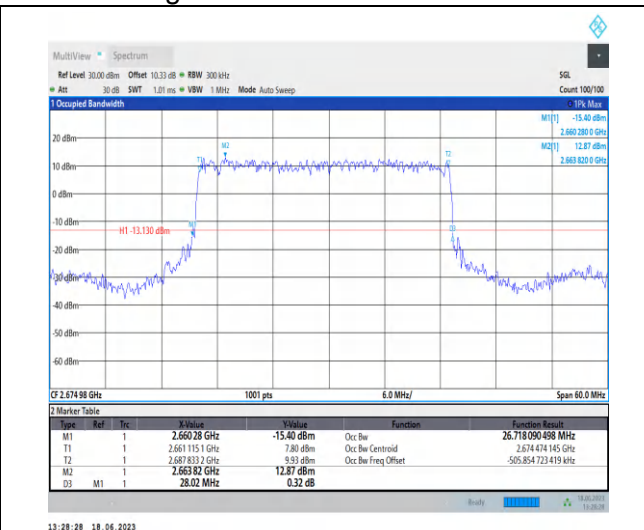
1-N41-PC3-30-30-H-1-DFT-PI2BPSK-Outer_Full-75@ 0-Ant0-26.718-28.020-≤30-PASS
