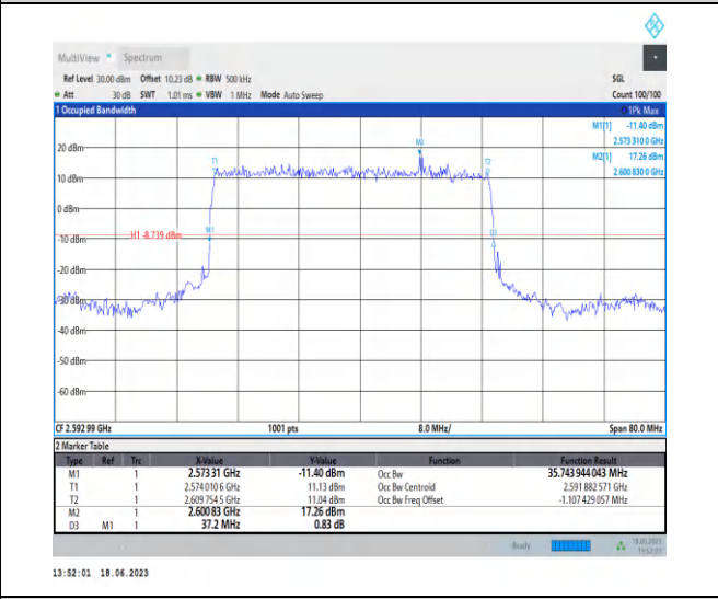
1-N41-PC3-30-40-M-1-DFT-PI2BPSK-Outer_Full-10 0@0-Ant0-35.744-37.200-≤40-PASS
