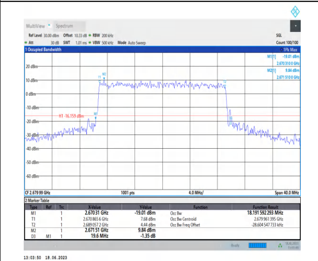
1-N41-PC3-30-20-H-6-CP-QPSK-Outer_Full-51@0- Ant0-18.192-19.600-≤20-PASS
