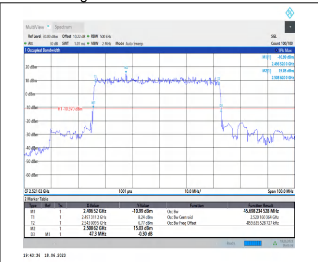
1-N41-PC3-30-50-L-1-DFT-PI2BPSK-Outer_Full-128 @ 0-Ant0-45.698-47.300-≤50-PASS
