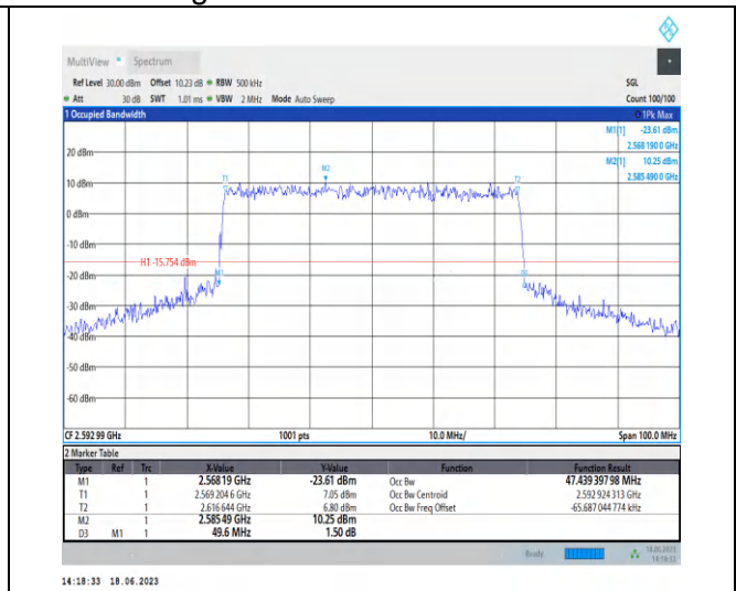
1-N41-PC3-30-50-M-8-CP-64QAM-Outer_Full-133@ 0-Ant0-47.439-49.600-≤50-PASS
