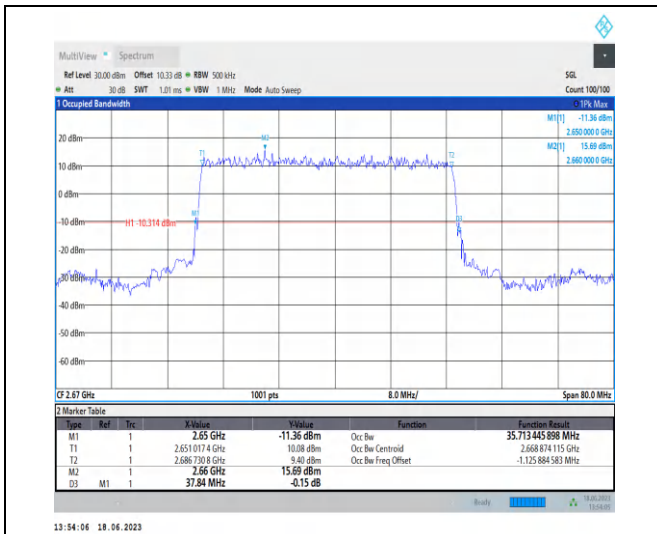
1-N41-PC3-30-40-H-1-DFT-PI2BPSK-Outer_Full-100@0-Ant0-35.713-37.840-≤40-PASS
