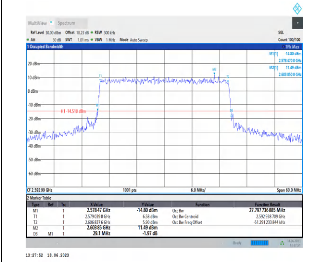
1-N41-PC3-30-30-M-7-CP-16QAM-Outer_Full-78 @ 0 -Ant0-27.798-29.100-≤30-PASS
