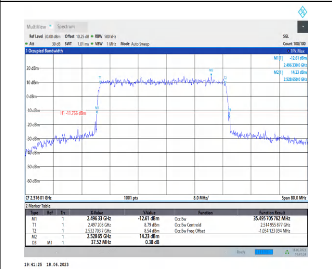
1-N41-PC3-30-40-L-2-DFT-QPSK-Outer_Full-100@0 -Ant0-35.496-37.520-≤40-PASS
