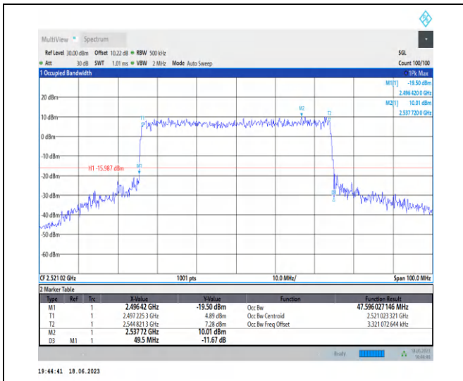
1-N41-PC3-30-50-L-8-CP-64QAM-Outer_Full-133@ 0-Ant0-47.596-49.500-≤50-PASS
