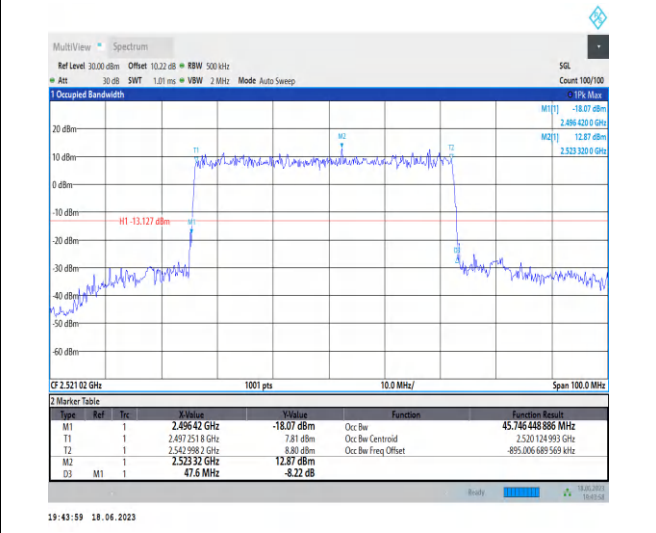
1-N41-PC3-30-50-L-3-DFT-16QAM-Outer_Full-128 @ 0-Ant0-45.746-47.600-≤50-PASS
