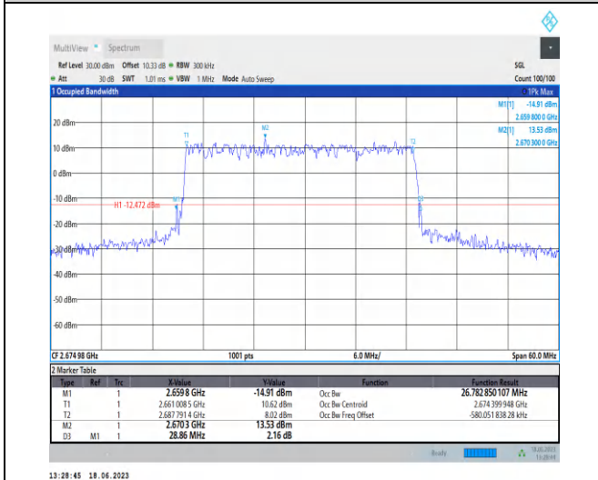
1-N41-PC3-30-30-H-2-DFT-QPSK-Outer_Full-75@0- Ant0-26.783-28.860-≤30-PASS
