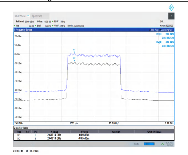
1-N41-PC3-30-100-H-2-CP-256QAM-Outer_Full-273 @0-Ant0-9.54-100%-0.00-9.54-PASS-≤13
