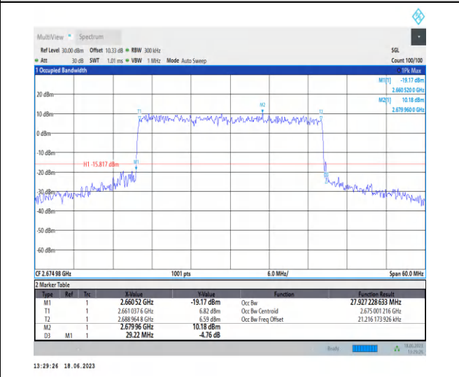
1-N41-PC3-30-30-H-7-CP-16QAM-Outer_Full-78@0- -Ant0-27.927-29.220-≤30-PASS
