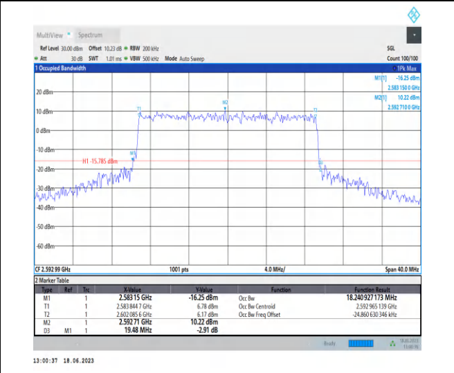
1-N41-PC3-30-20-M-7-CP-16QAM-Outer_Full-51@0- -Ant0-18.241-19.480-≤20-PASS
