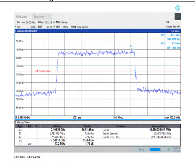
1-N41-PC3-30-50-L-5-DFT-256QAM-Outer_Full-128 @ 0-Ant0-45.65-47.200-≤50-PASS
