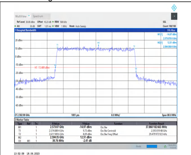
1-N41-PC3-30-40-M-7-CP-16QAM-Outer_Full-106@0 -Ant0-37.86-39.760-≤40-PASS
