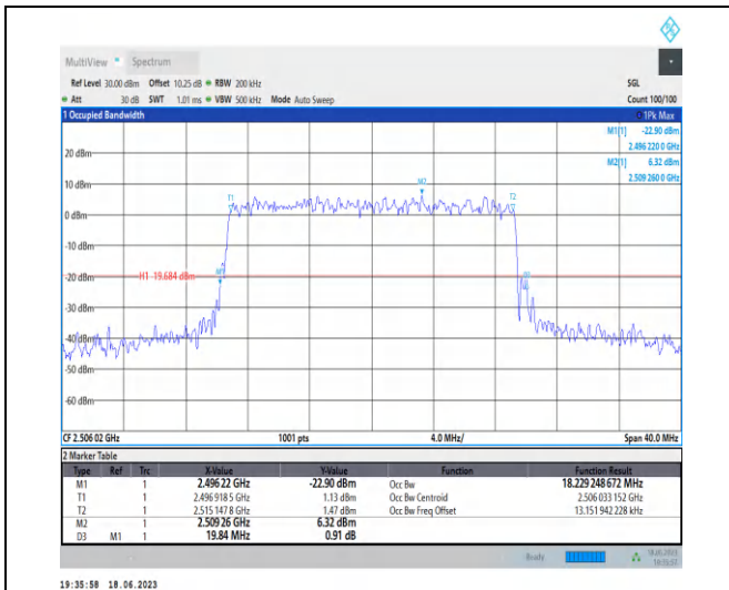
1-N41-PC3-30-20-L-9-CP-256QAM-Outer_Full-51@ 0-Ant0-18.229-19.840-<=20-PASS
