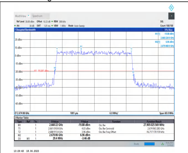
1-N41-PC3-30-30-H-9-CP-256QAM-Outer_Full-78@0 -Ant0-27.905-29.400-≤30-PASS
