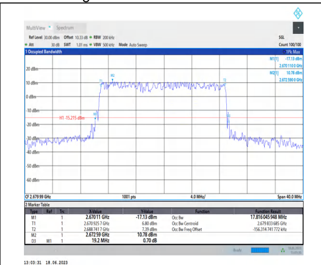
1-N41-PC3-30-20-H-4-DFT-64QAM-Outer_Full-50@ 0-Ant0-17.816-19.200-≤20-PASS
