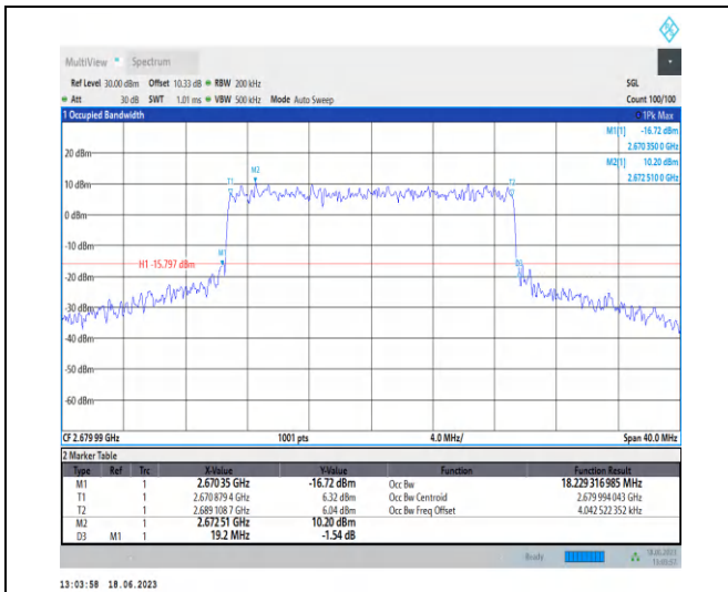
1-N41-PC3-30-20-H-7-CP-16QAM-Outer_Full-51@0 -Ant0-18.229-19.200-≤20-PASS
