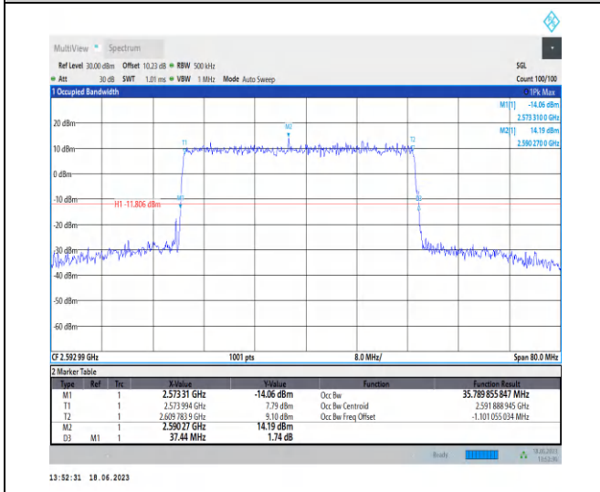
1-N41-PC3-30-40-M-4-DFT-64QAM-Outer_Full-100 @0-Ant0-35.79-37.440-≤40-PASS
