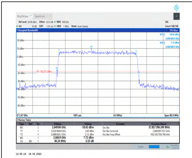
1-N41-PC3-30-40-H-9-CP-256QAM-Outer_Full-106 @ 0-Ant0-37.857-40.240-≤40-PASS
