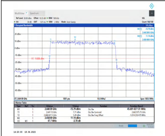
1-N41-PC3-30-50-H-4-DFT-64QAM-Outer_Full-128 @0-Ant0-45.691-47.700-≤50-PASS
