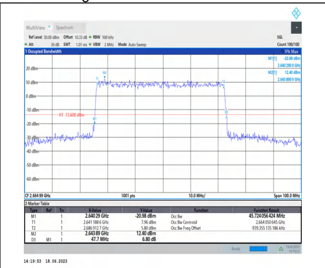
1-N41-PC3-30-50-H-3-DFT-16QAM-Outer_Full-128 @0-Ant0-45.724-47.700-≤50-PASS
