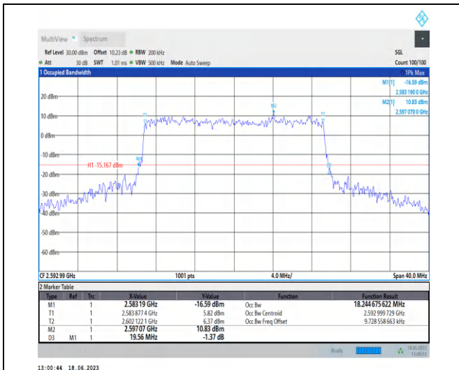
1-N41-PC3-30-20-M-8-CP-64QAM-Outer_Full-51 @ 0-Ant0-18.245-19.560-≤20-PASS
