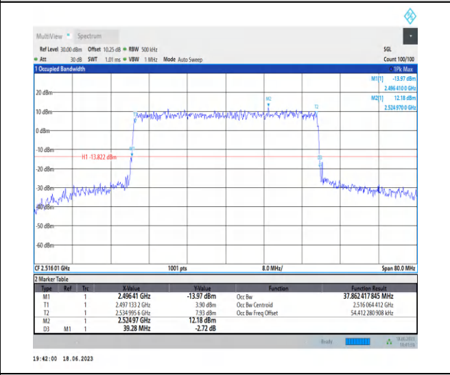
1-N41-PC3-30-40-L-6-CP-QPSK-Outer_Full-106 @0-Ant0-37.862-39.280-≤40-PASS
