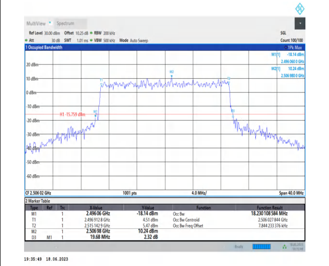
1-N41-PC3-30-20-L-8-CP-64QAM-Outer_Full-51 @ 0-Ant0-18.23-19.680-≤20-PASS
