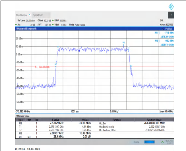
1-N41-PC3-30-30-M-5-DFT-256QAM-Outer_Full-75 @ 0-Ant0-26.639-28.500-≤30-PASS
