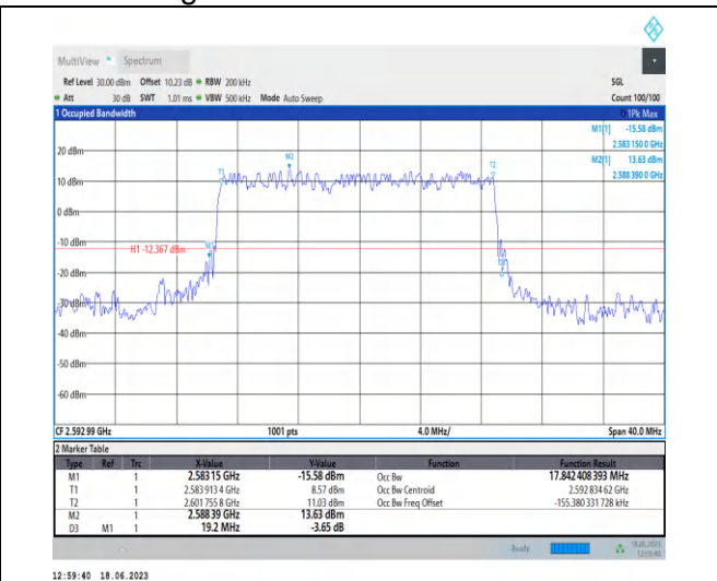
1-N41-PC3-30-20-M-1-DFT-PI2BPSK-Outer_Full-50@ 0-Ant0-17.842-19.200-<=20-PASS
