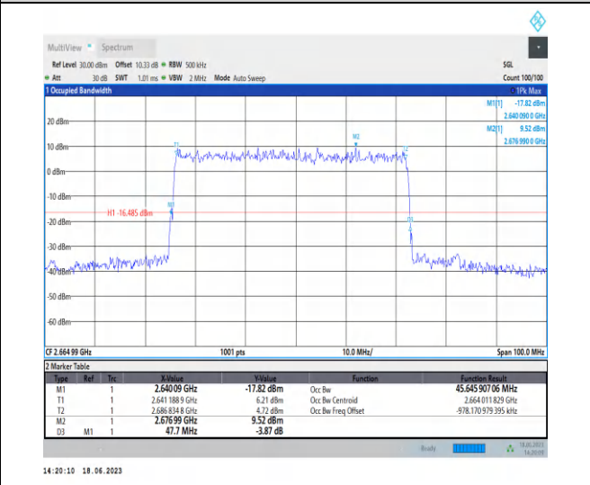
1-N41-PC3-30-50-H-5-DFT-256QAM-Outer_Full-128 @0-Ant0-45.646-47.700-≤50-PASS
