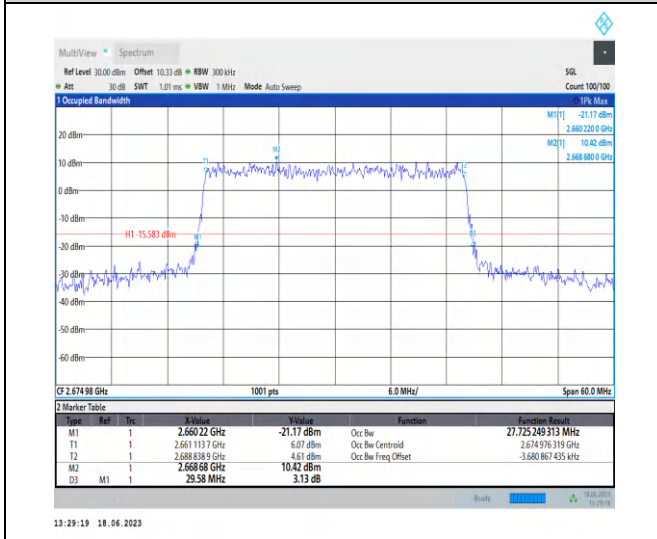
1-N41-PC3-30-30-H-6-CP-QPSK-Outer_Full-78@0- Ant0-27.725-29.580-≤30-PASS
