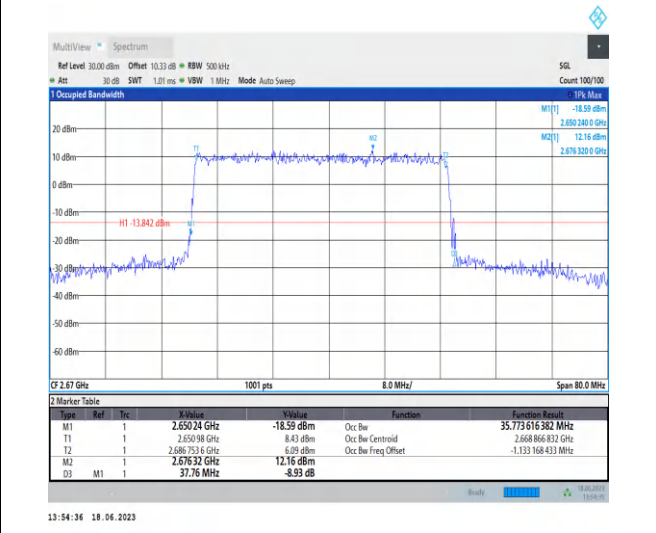
1-N41-PC3-30-40-H-4-DFT-64QAM-Outer_Full-100@0-Ant0-35.774-37.760-≤40-PASS
