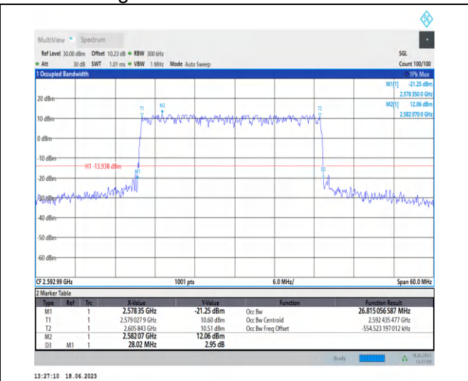
1-N41-PC3-30-30-M-2-DFT-QPSK-Outer_Full-75 @ 0-Ant0-26.815-28.020-≤30-PASS
