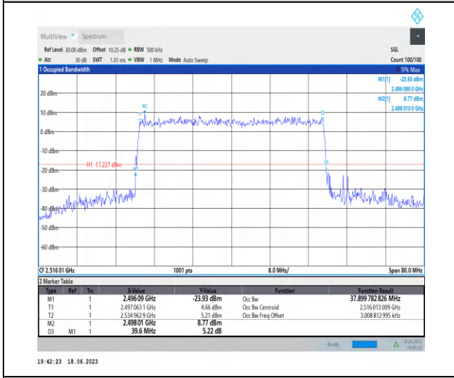
1-N41-PC3-30-40-L-9-CP-256QAM-Outer_Full-106 @0-Ant0-37.9-39.600-≤40-PASS
