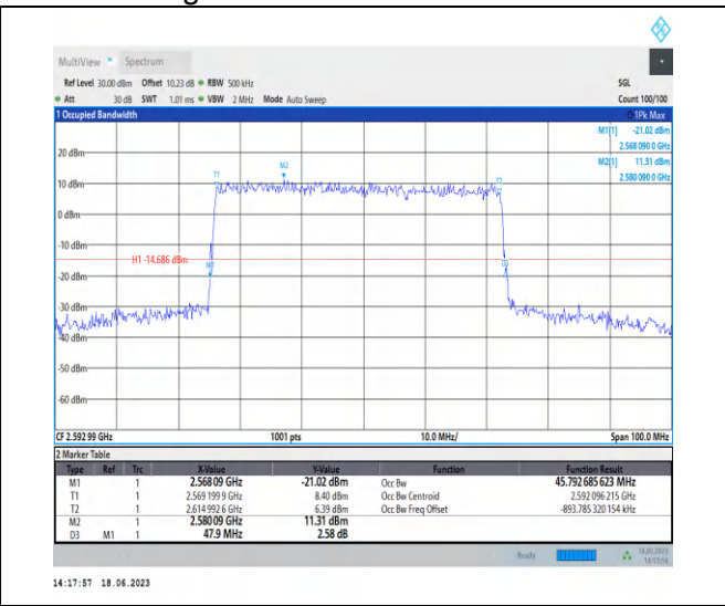
1-N41-PC3-30-50-M-4-DFT-64QAM-Outer_Full-128 @ 0-Ant0-45.793-47.900-≤50-PASS
