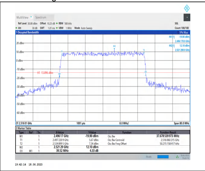
1-N41-PC3-30-40-L-8-CP-64QAM-Outer_Full-106@ 0-Ant0-37.679-39.520-≤40-PASS
