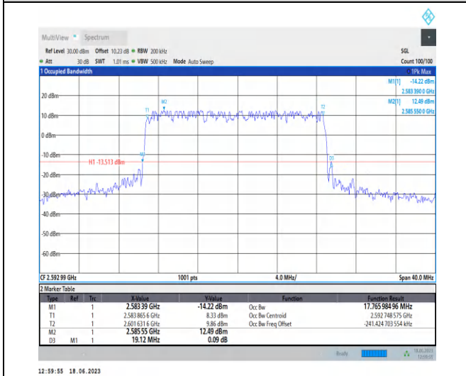
1-N41-PC3-30-20-M-2-DFT-QPSK-Outer_Full-50@0 -Ant0-17.766-19.120-<=20-PASS
