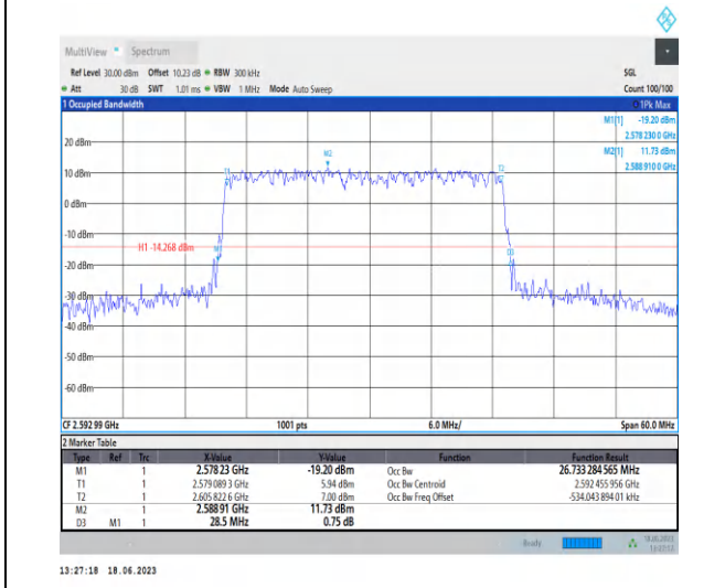
1-N41-PC3-30-30-M-3-DFT-16QAM-Outer_Full-75 @ 0-Ant0-26.733-28.500-≤30-PASS
