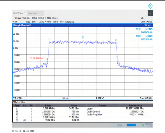
1-N41-PC3-30-40-H-8-CP-64QAM-Outer_Full-106 @ 0-Ant0-37.874-39.840-≤40-PASS
