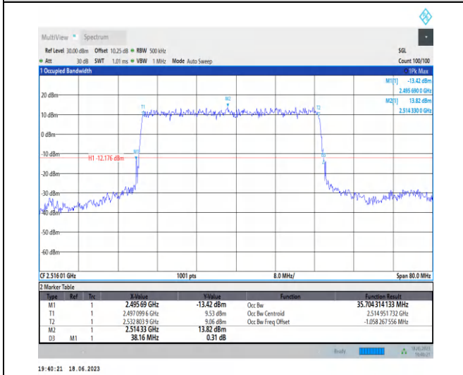
1-N41-PC3-30-40-L-1-DFT-PI2BPSK-Outer_Full-100@0 -Ant0-35.704-38.160-≤40-PASS
