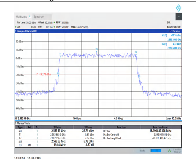
1-N41-PC3-30-20-M-9-CP-256QAM-Outer_Full-51 @ 0-Ant0-18.191-19.440-≤20-PASS
