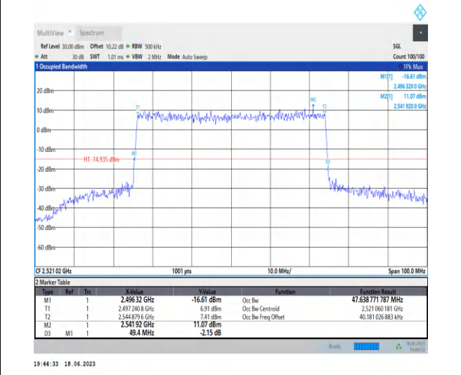
1-N41-PC3-30-50-L-7-CP-16QAM-Outer_Full-133 @ 0-Ant0-47.639-49.400-≤50-PASS
