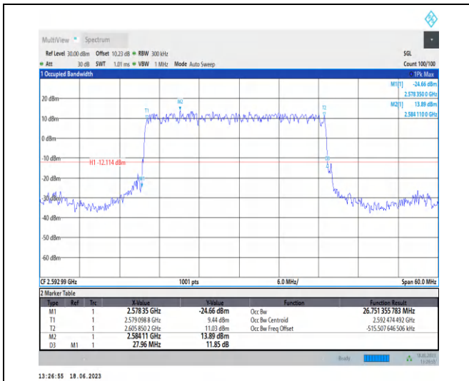
1-N41-PC3-30-30-M-1-DFT-PI2BPSK-Outer_Full-75 @ 0-Ant0-26.751-27.960-≤30-PASS
