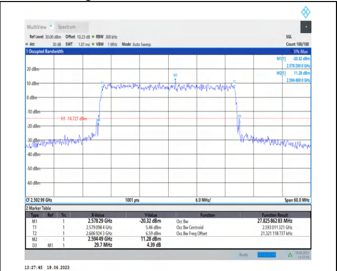
1-N41-PC3-30-30-M-6-CP-QPSK-Outer_Full-78 @ 0-Ant0-27.826-29.700-≤30-PASS
