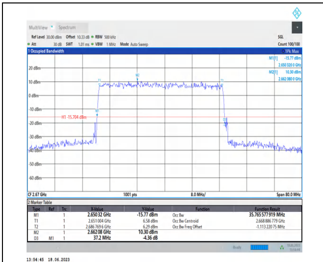
1-N41-PC3-30-40-H-5-DFT-256QAM-Outer_Full-100 @ 0-Ant0-35.766-37.200-≤40-PASS
