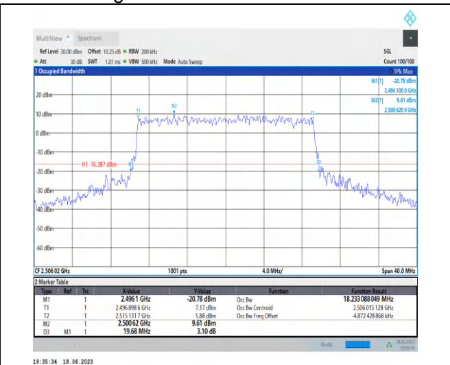
1-N41-PC3-30-20-L-6-CP-QPSK-Outer_Full-51 @ 0-Ant0-18.233-19.680-≤20-PASS
