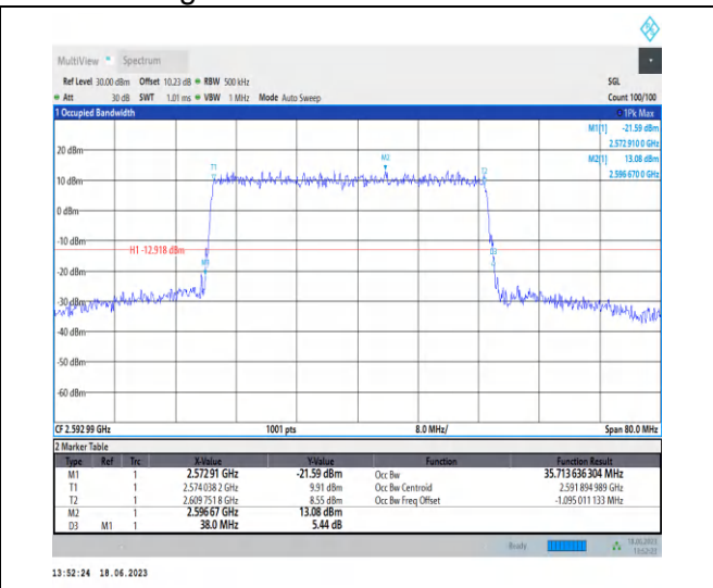
1-N41-PC3-30-40-M-3-DFT-16QAM-Outer_Full-100 @0-Ant0-35.714-38.000-≤40-PASS
