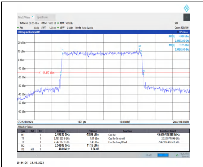
1-N41-PC3-30-50-L-4-DFT-64QAM-Outer_Full-128 @ 0-Ant0-45.676-48.000-≤50-PASS
