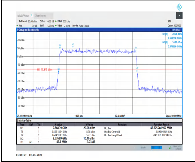
1-N41-PC3-30-50-M-5-DFT-256QAM-Outer_Full-128 @ 0-Ant0-45.725-47.300-≤50-PASS
