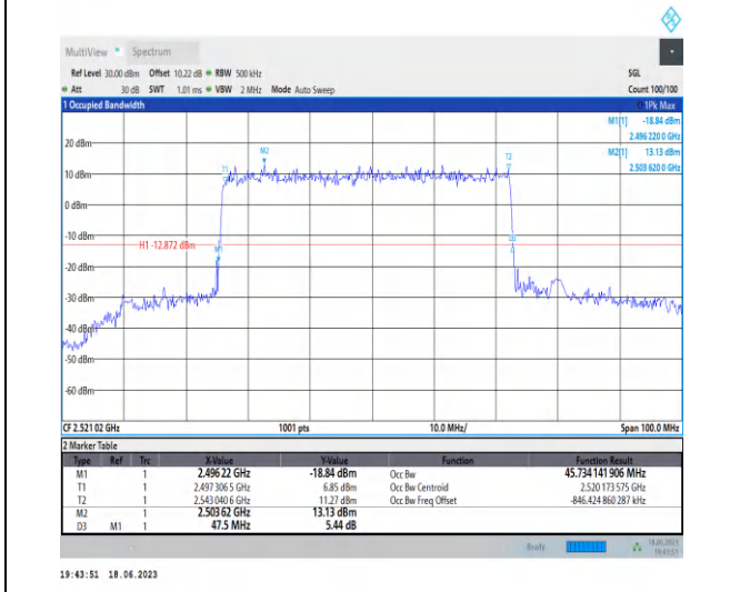
1-N41-PC3-30-50-L-2-DFT-QPSK-Outer_Full-128 @ 0-Ant0-45.734-47.500-≤50-PASS
