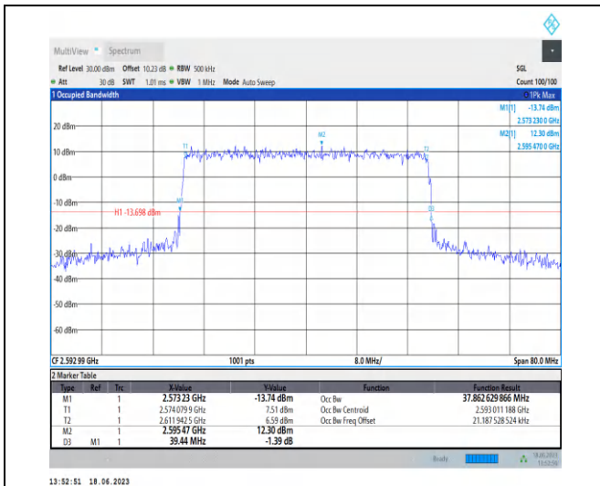
1-N41-PC3-30-40-M-6-CP-QPSK-Outer_Full-106@0 -Ant0-37.863-39.440-≤40-PASS
