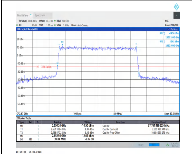
1-N41-PC3-30-40-H-7-CP-16QAM-Outer_Full-106 @ 0-Ant0-37.762-39.840-≤40-PASS
