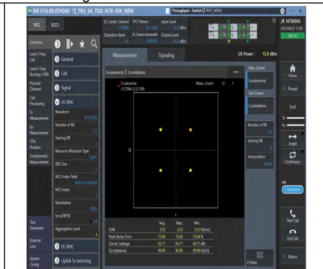
1-N41-PC3-30-100-M-6-CP-QPSK-Outer_Full-273 @0-Ant0-see graph-PASS
