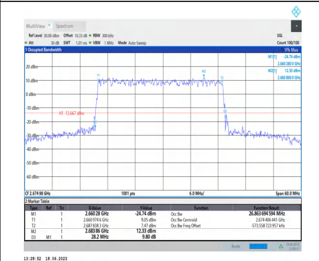
1-N41-PC3-30-30-H-3-DFT-16QAM-Outer_Full-75@ 0-Ant0-26.864-28.200-≤30-PASS
