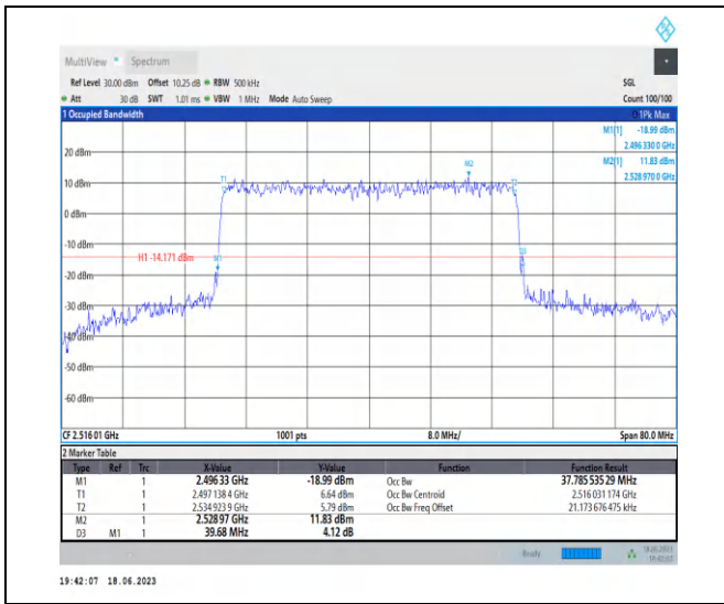
1-N41-PC3-30-40-L-7-CP-16QAM-Outer_Full-106@ 0-Ant0-37.786-39.680-≤40-PASS
