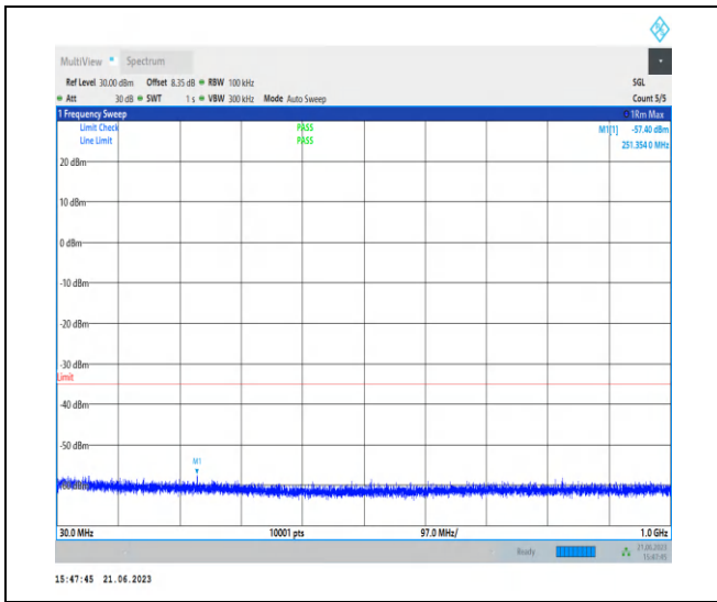
1-N38-PC2-30-40-M-1-N/A-DFT-QPSK-Edge_1RB_Left-1@0-30-1000-Ant0-36.98--57.40--35-PASS
