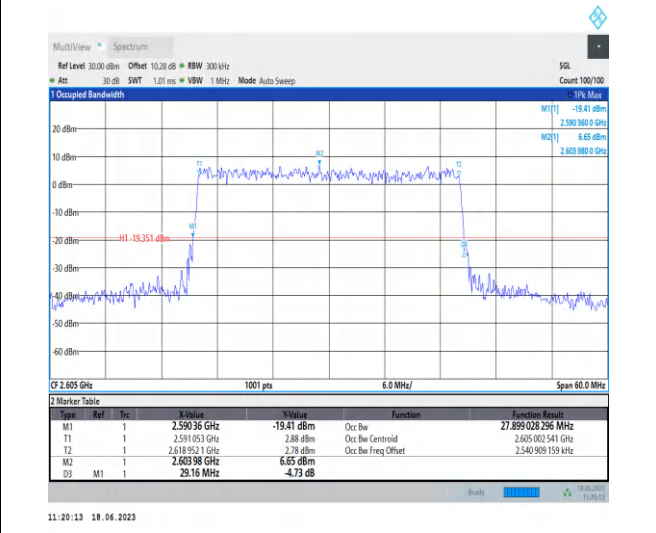
1-N38-PC3-30-30-H-9-CP-256QAM-Outer_Full-78@0-Ant0-27.899-29.160-≤30-PASS
