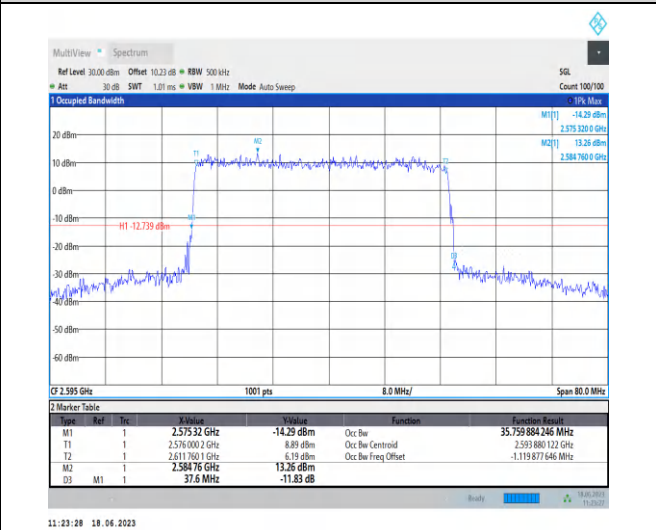
1-N38-PC3-30-40-M-3-DFT-16QAM-Outer_Full-100 @ 0-Ant0-35.76-37.600-≤40-PASS
