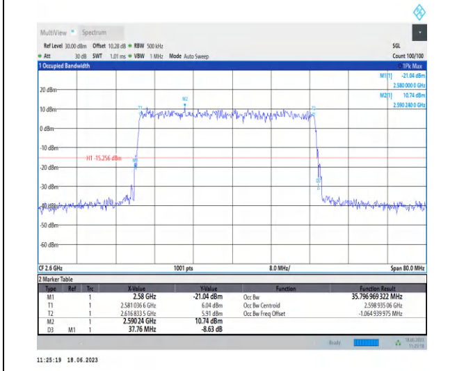
1-N38-PC3-30-40-H-5-DFT-256QAM-Outer_Full-100 @ 0-Ant0-35.797-37.760-≤40-PASS
