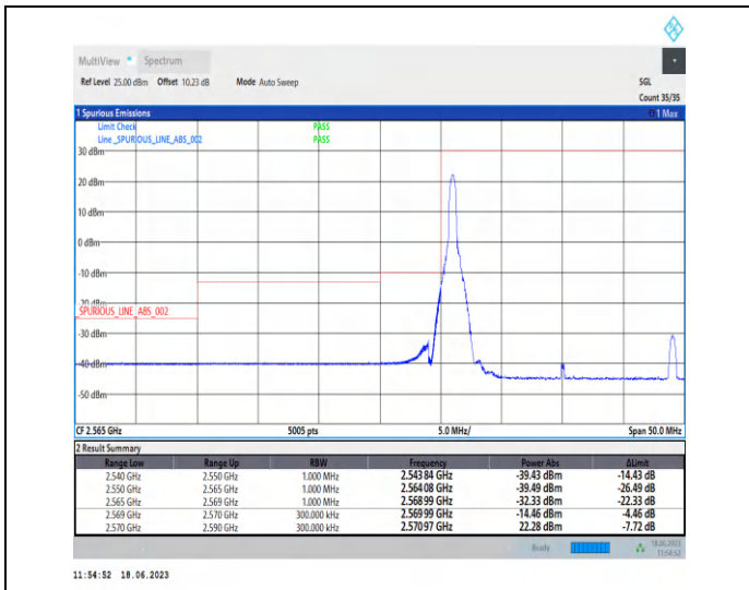
1-N38-PC3-30-20-L-1-DFT-PI2BPSK-Edge_1RB_Left-1@0-Ant0-1--PASS-see graph
