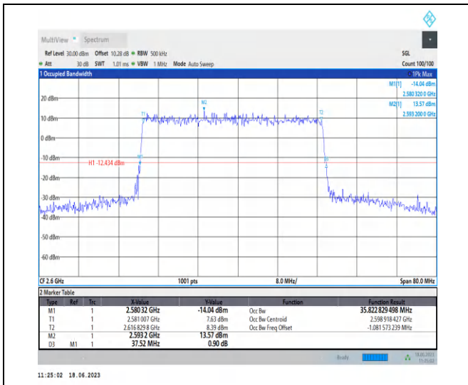
1-N38-PC3-30-40-H-3-DFT-16QAM-Outer_Full-100 @ 0-Ant0-35.823-37.520-≤40-PASS
