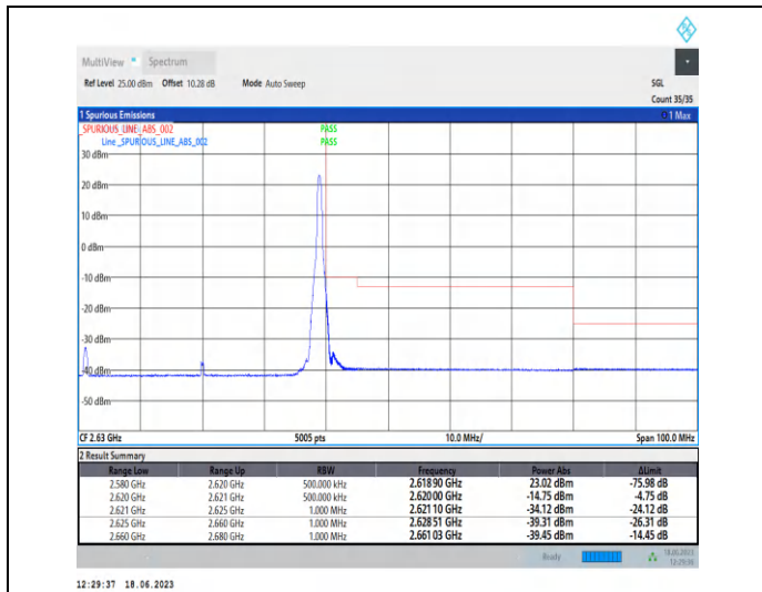
1-N38-PC3-30-40-H-2-DFT-PI2BPSK-Edge_1RB_Righ t-1@105-Ant0-1--PASS-see graph
