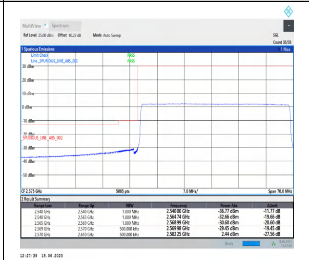
1-N38-PC3-30-40-L-6-CP-QPSK-Outer_Full-106@0-Ant0-1--PASS-see graph
