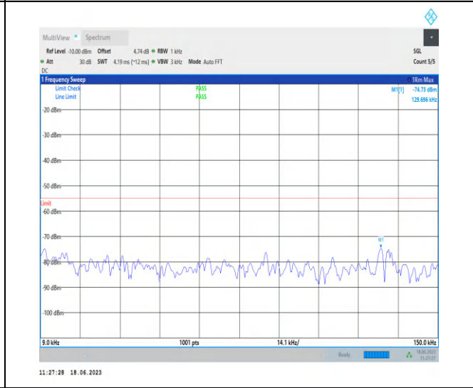
1-N38-PC3-30-40-H-1-N/A-DFT-PI2BPSK-Inner_1R B_Left-1@1-0.009-0.15-Ant0-0.13--74.73--55-PASS
