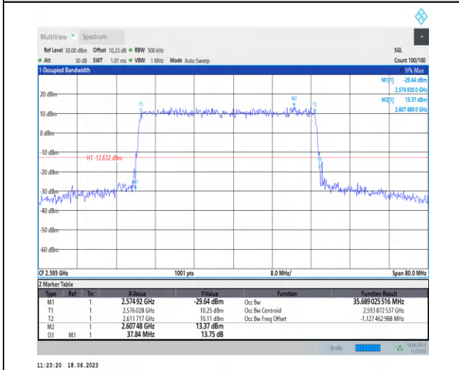
1-N38-PC3-30-40-M-2-DFT-QPSK-Outer_Full-100 @ 0-Ant0-35.689-37.840-≤40-PASS
