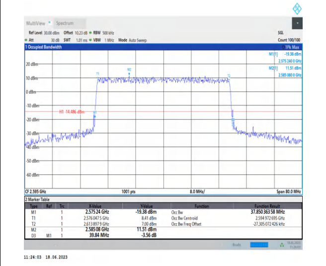
1-N38-PC3-30-40-M-7-CP-16QAM-Outer_Full-106 @ 0-Ant0-37.85-39.840-≤40-PASS
