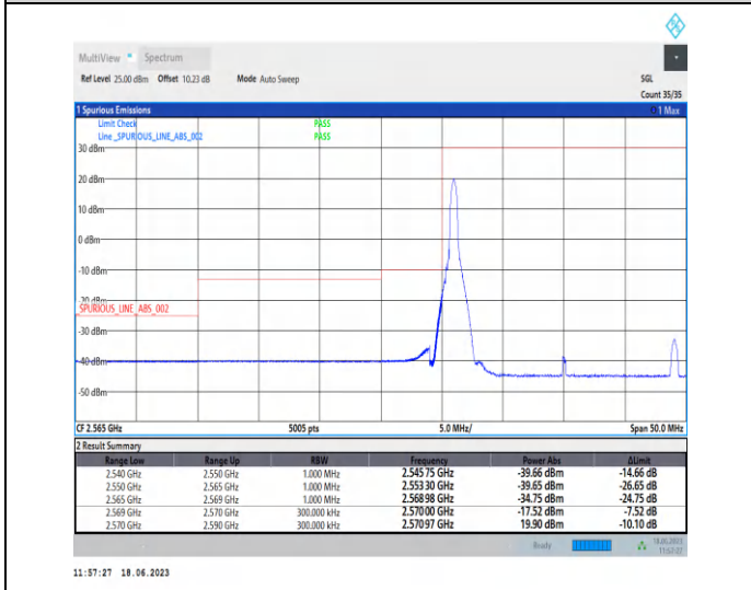
1-N38-PC3-30-20-L-4-CP-QPSK-Edge_1RB_Left-1@0-Ant0-1--PASS-see graph
