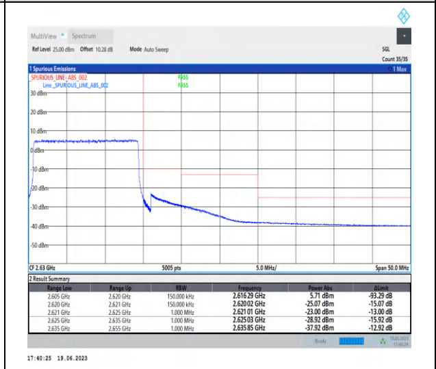
1-N38-PC2-30-15-H-3-CP-QPSK-Outer_Full-38@0-Ant0-1--PASS-see graph
