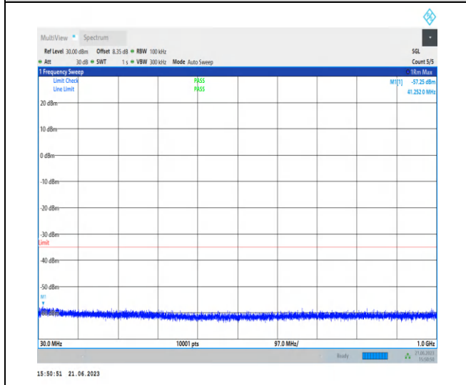
1-N38-PC2-30-40-H-1-N/A-DFT-QPSK-Edge_1RB_Left-1@0-30-1000-Ant0-41.25--57.25--35-PASS
