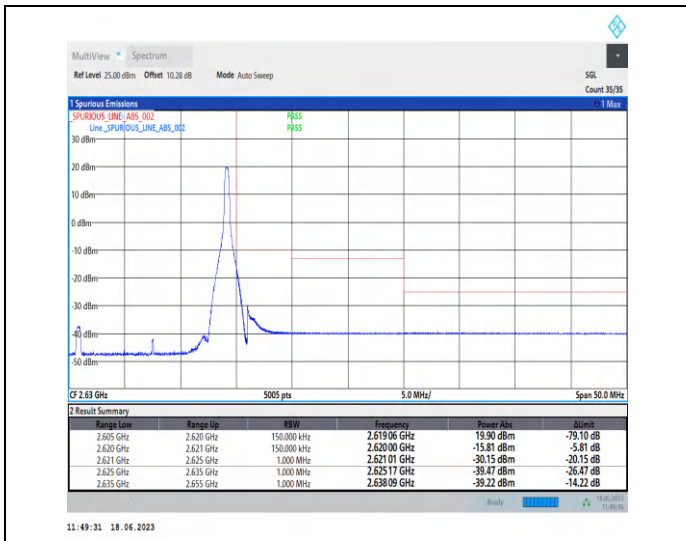
1-N38-PC3-30-15-H-2-DFT-PI2BPSK-Edge_1RB_Righ t-1@37-Ant0-1--PASS-see graph
