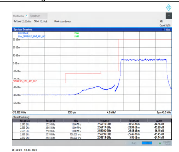
1-N38-PC3-30-15-L-3-DFT-PI2BPSK-Outer_Full-36@0-Ant0-1--PASS-see graph
