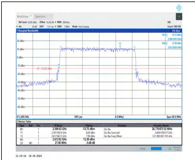
1-N38-PC3-30-30-H-2-DFT-QPSK-Outer_Full-75@0 -Ant0-26.771-27.960-≤30-PASS
