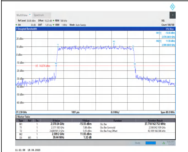
1-N38-PC3-30-40-L-7-CP-16QAM-Outer_Full-106 @ 0-Ant0-37.718-39.440-≤40-PASS
