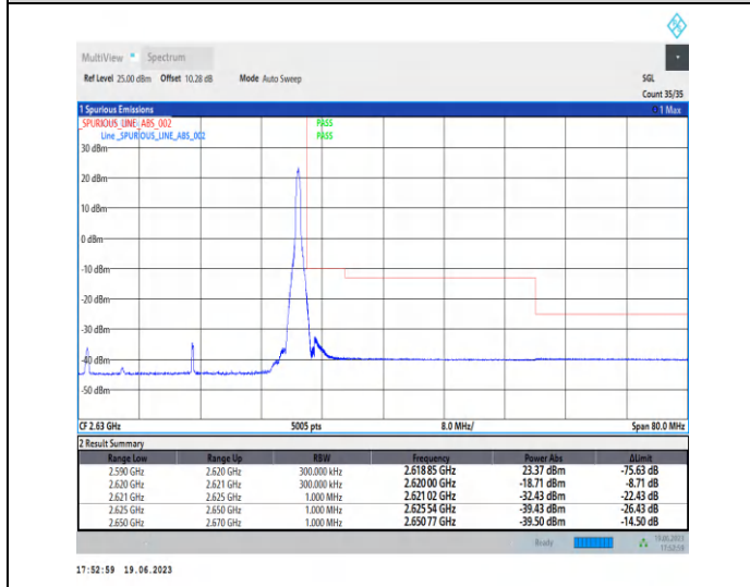
1-N38-PC2-30-30-H-2-CP-QPSK-Edge_1RB_Right-1@77-Ant0-1--PASS-see graph
