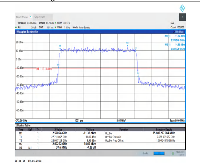
1-N38-PC3-30-40-L-2-DFT-QPSK-Outer_Full-100 @ 0-Ant0-35.606-37.600-≤40-PASS
