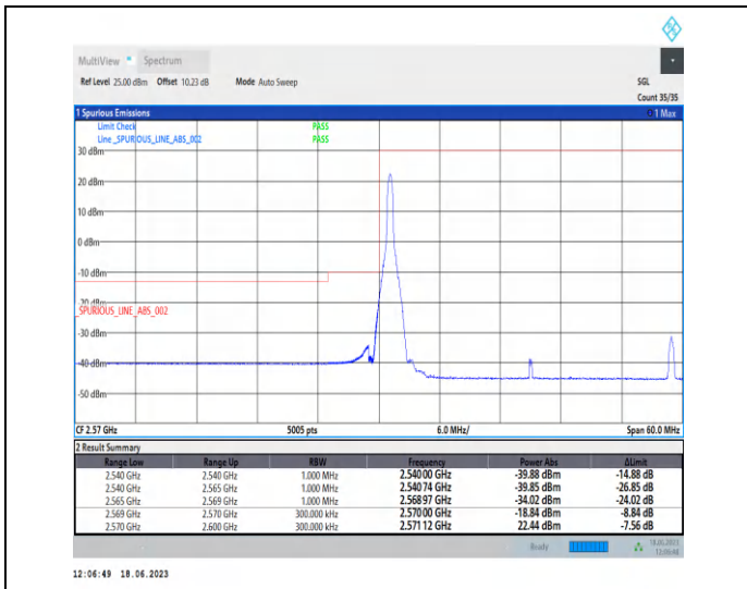
1-N38-PC3-30-30-L-1-DFT-PI2BPSK-Edge_1RB_Left-1@0-Ant0-1--PASS-see graph
