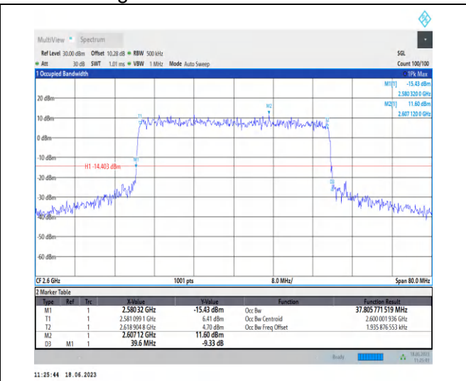
1-N38-PC3-30-40-H-8-CP-64QAM-Outer_Full-106@ 0-Ant0-37.806-39.600-≤40-PASS
