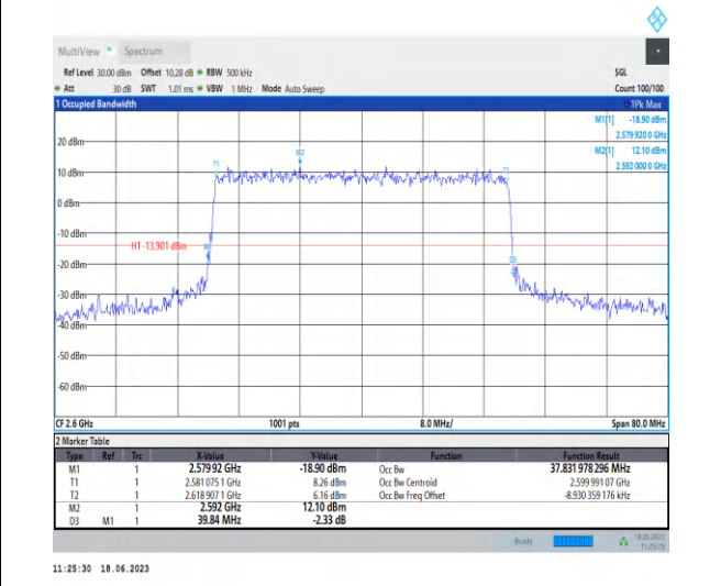
1-N38-PC3-30-40-H-6-CP-QPSK-Outer_Full-106 @ 0-Ant0-37.832-39.840-≤40-PASS
