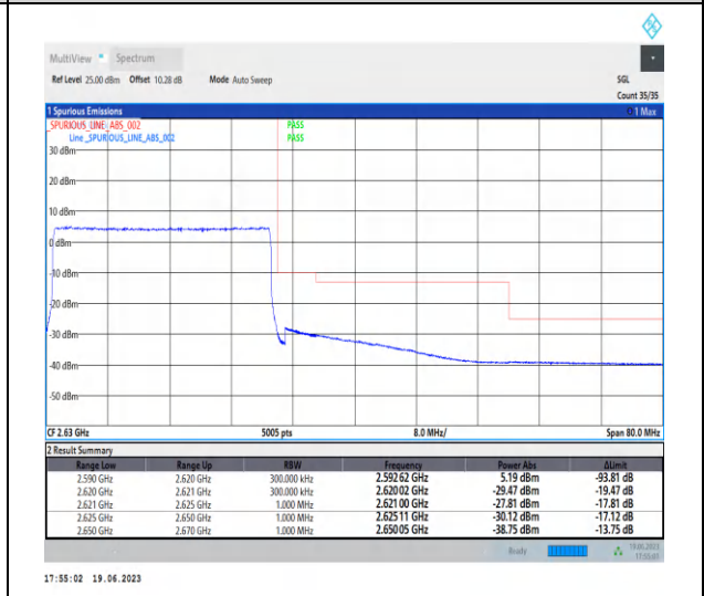
1-N38-PC2-30-30-H-3-CP-QPSK-Outer_Full-78@0-Ant0-1--PASS-see graph
