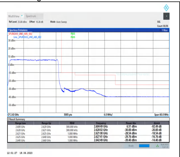
1-N38-PC3-30-20-H-3-DFT-PI2BPSK-Outer_Full-5 0@0-Ant0-1--PASS-see graph
