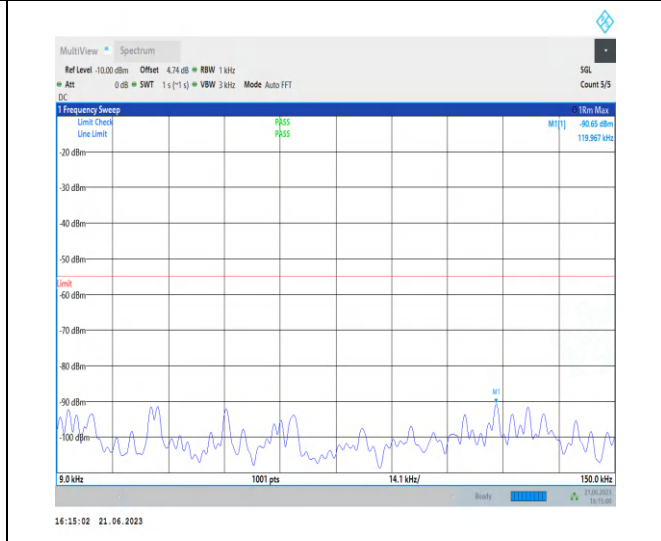
1-N38-PC3-30-40-M-1-DFT-PI2BPSK-Inner_1RB_Le ft-1 @ 1-0.009-0.15-Ant0-0.12--90.65--55-PASS
