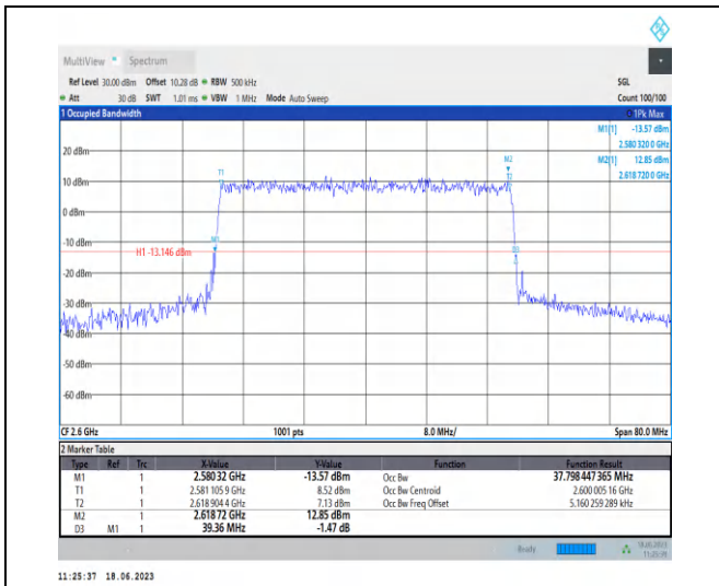
1-N38-PC3-30-40-H-7-CP-16QAM-Outer_Full-106@ 0-Ant0-37.798-39.360-≤40-PASS
