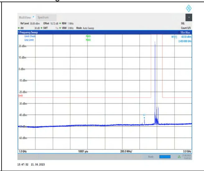
1-N38-PC2-30-40-M-1-N/A-DFT-QPSK-Edge_1RB_Left-1@0-1000-3000-Ant0-2755.40--43.53--25-PASS
