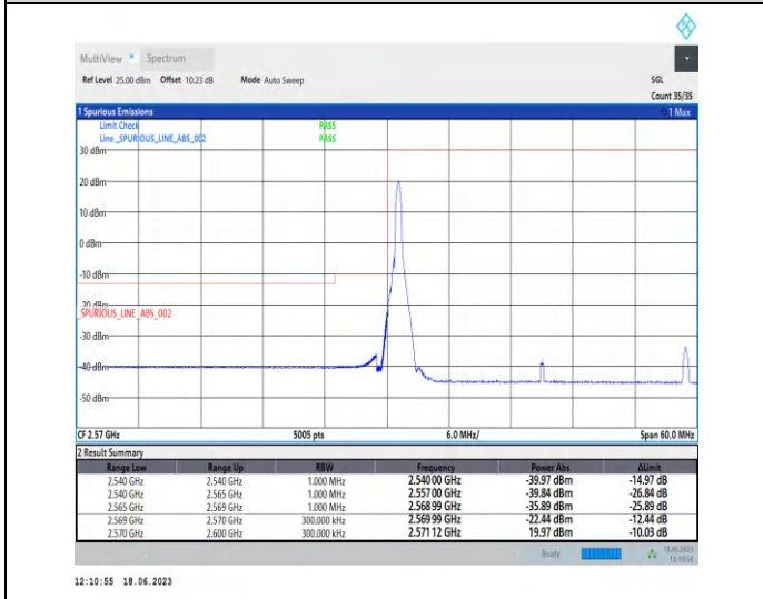
1-N38-PC3-30-30-L-4-CP-QPSK-Edge_1RB_Left-1@0-Ant0-1--PASS-see graph
