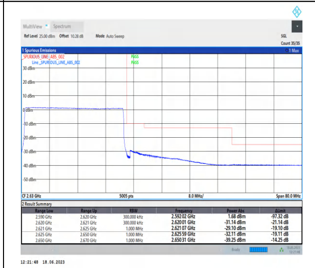
1-N38-PC3-30-30-H-6-CP-QPSK-Outer_Full-78@ 0-Ant0-1--PASS-see graph
