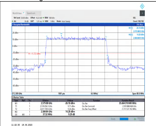
1-N38-PC3-30-40-M-1-DFT-PI2BPSK-Outer_Full-10 @ 0-Ant0-35.664-37.520-≤40-PASS
