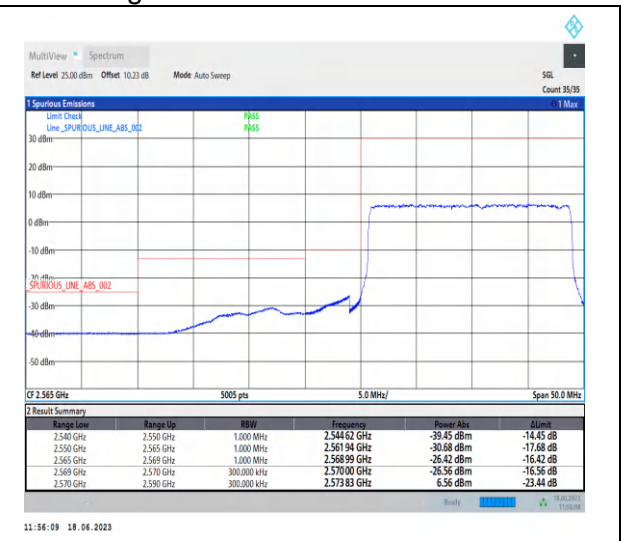
1-N38-PC3-30-20-L-3-DFT-PI2BPSK-Outer_Full-50@0-Ant0-1--PASS-see graph
