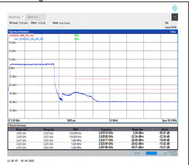
1-N38-PC3-30-15-H-3-DFT-PI2BPSK-Outer_Full-3 6@0-Ant0-1--PASS-see graph
