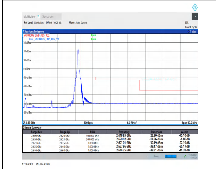
1-N38-PC2-30-20-H-2-CP-QPSK-Edge_1RB_Right-1@50-Ant0-1--PASS-see graph
