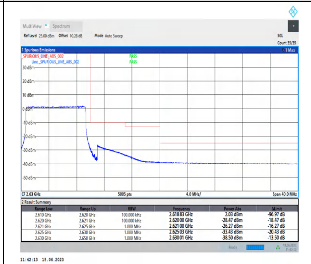
1-N38-PC3-30-10-H-6-CP-QPSK-Outer_Full-24 @0-Ant0-1--PASS-see graph
