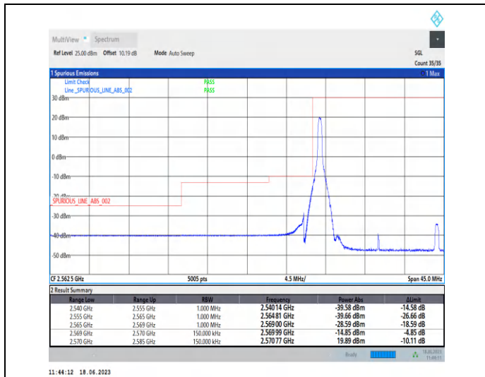
1-N38-PC3-30-15-L-1-DFT-PI2BPSK-Edge_1RB_Left-1@0-Ant0-1--PASS-see graph
