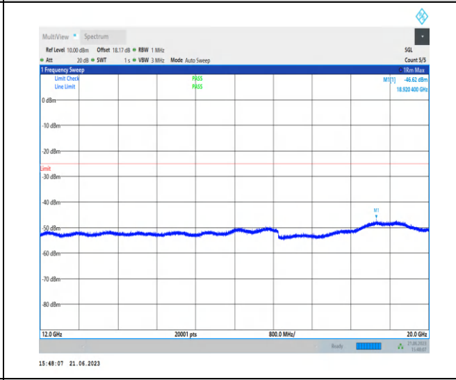
1-N38-PC2-30-40-M-1-N/A-DFT-QPSK-Edge_1RB_Left-1@0-12000-20000-Ant0-19328.80--46.62--25-PA SS
