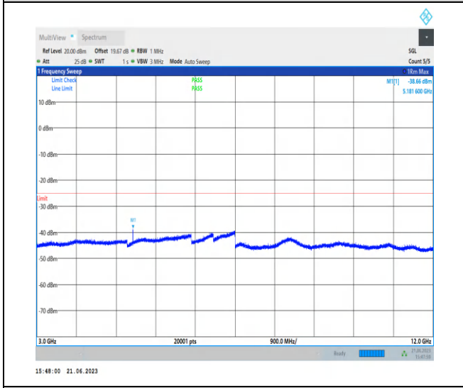
1-N38-PC2-30-40-M-1-N/A-DFT-QPSK-Edge_1RB_Left-1@0-3000-12000-Ant0-5219.40--38.66--25-PA SS
