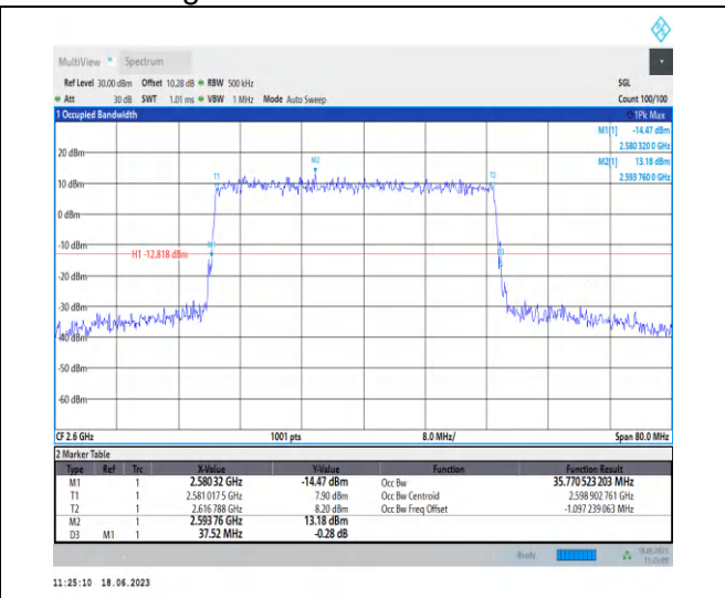
1-N38-PC3-30-40-H-4-DFT-64QAM-Outer_Full-100 @ 0-Ant0-35.771-37.520-≤40-PASS
