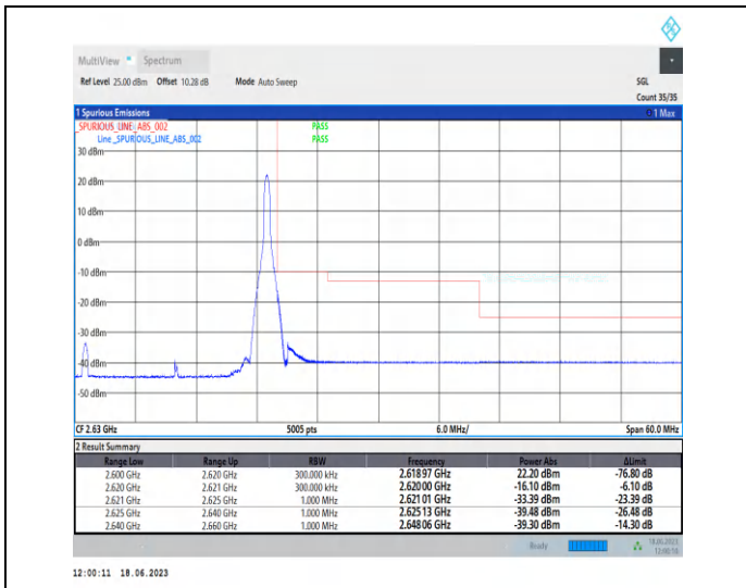
1-N38-PC3-30-20-H-2-DFT-PI2BPSK-Edge_1RB_Righ t-1@50-Ant0-1--PASS-see graph
