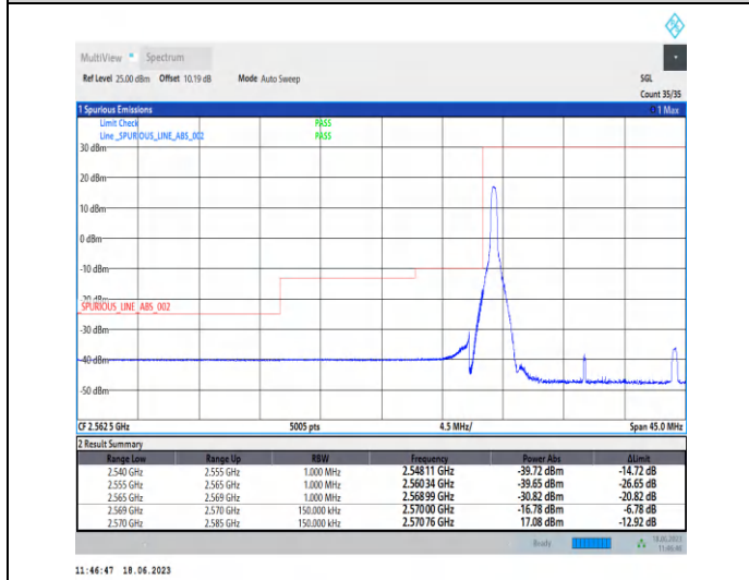
1-N38-PC3-30-15-L-4-CP-QPSK-Edge_1RB_Left-1@0-Ant0-1--PASS-see graph
