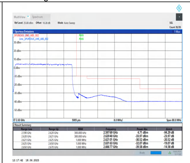
1-N38-PC3-30-30-H-3-DFT-PI2BPSK-Outer_Full-7 5@0-Ant0-1--PASS-see graph
