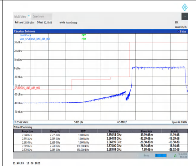
1-N38-PC3-30-15-L-6-CP-QPSK-Outer_Full-38@0-Ant0-1--PASS-see graph
