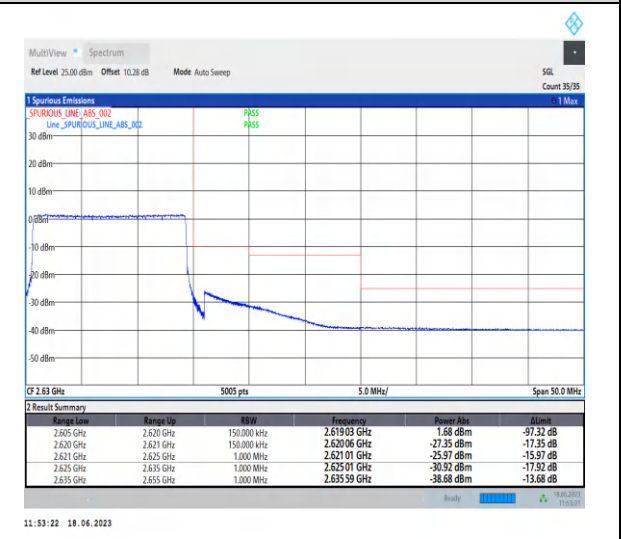
1-N38-PC3-30-15-H-6-CP-QPSK-Outer_Full-38 @0-Ant0-1--PASS-see graph
