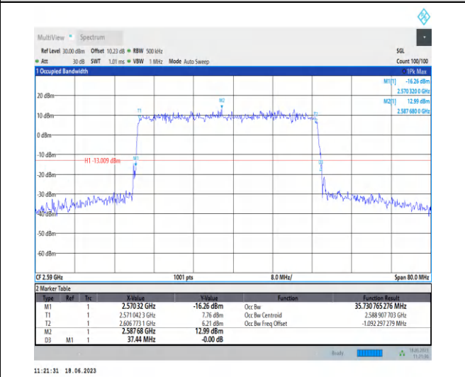
1-N38-PC3-30-40-L-4-DFT-64QAM-Outer_Full-100 @ 0-Ant0-35.731-37.440-≤40-PASS
