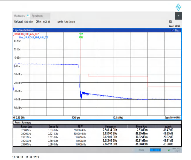
1-N38-PC3-30-40-H-6-CP-QPSK-Outer_Full-106 @0-Ant0-1--PASS-see graph
