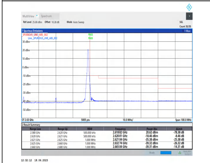
1-N38-PC3-30-40-H-5-CP-QPSK-Edge_1RB_Right-1 @105-Ant0-1--PASS-see graph
