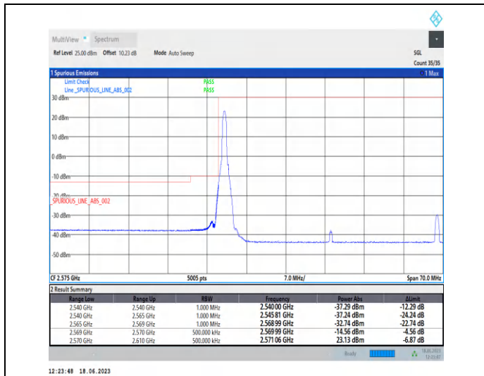
1-N38-PC3-30-40-L-1-DFT-PI2BPSK-Edge_1RB_Left-1@0-Ant0-1--PASS-see graph
