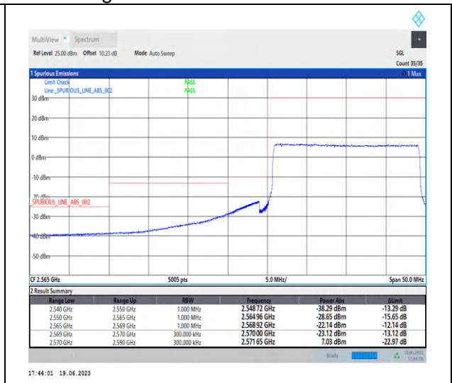
1-N38-PC2-30-20-L-3-CP-QPSK-Outer_Full-51@0-Ant0-1--PASS-see graph
