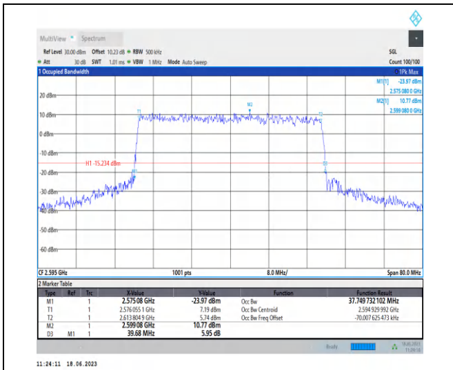
1-N38-PC3-30-40-M-8-CP-64QAM-Outer_Full-106@ 0-Ant0-37.75-39.680-≤40-PASS
