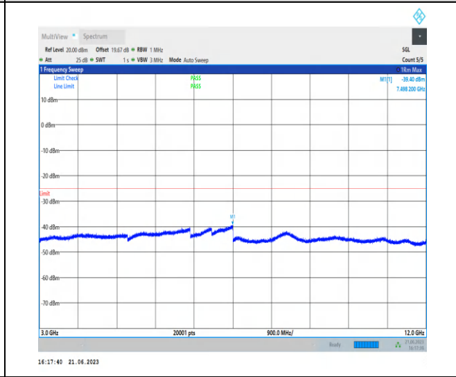
1-N38-PC3-30-40-H-1-N/A-DFT-PI2BPSK-Inner_1R B_Left-1@1-3000-12000-Ant0-7437.45--39.40--25-PASS
