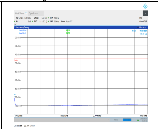
1-N38-PC2-30-40-H-1-N/A-DFT-QPSK-Edge_1RB_Left-1@0-0.15-30-Ant0-0.16--90.33--45-PASS
