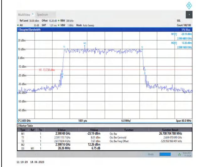
1-N38-PC3-30-30-H-4-DFT-64QAM-Outer_Full-75@0-Ant0-26.709-28.260-≤30-PASS
