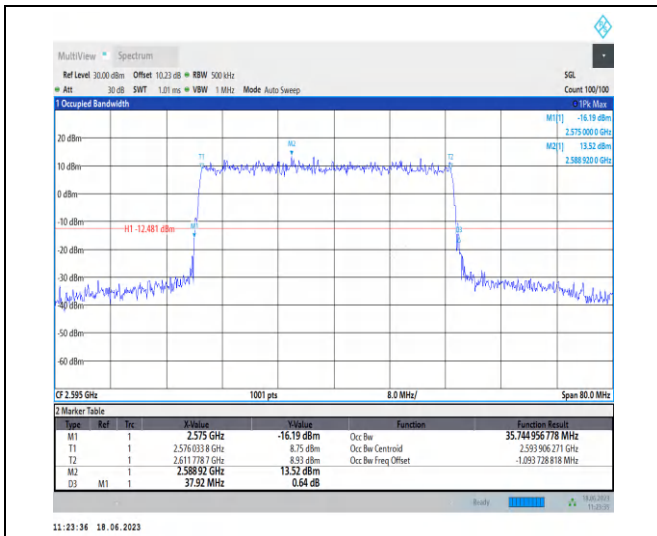
1-N38-PC3-30-40-M-4-DFT-64QAM-Outer_Full-100 @ 0-Ant0-35.745-37.920-≤40-PASS
