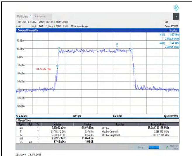
1-N38-PC3-30-40-L-5-DFT-256QAM-Outer_Full-100 @ 0-Ant0-35.783-37.440-≤40-PASS
