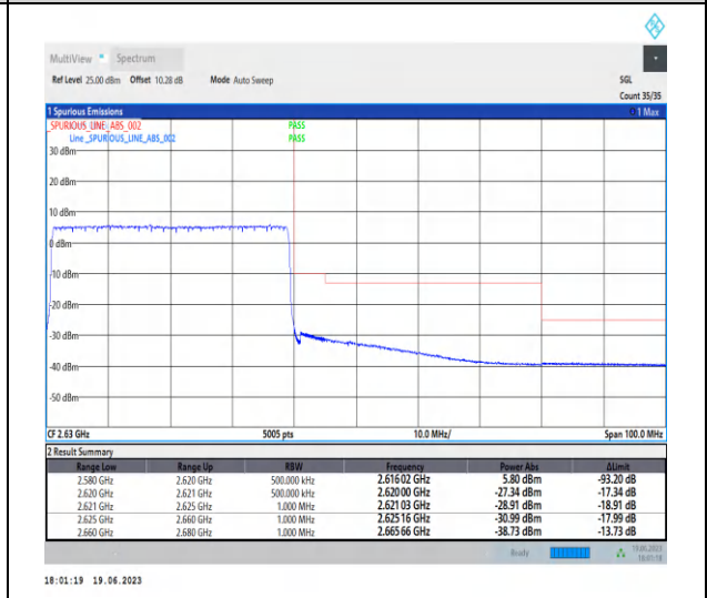
1-N38-PC2-30-40-H-3-CP-QPSK-Outer_Full-106@0-Ant0-1--PASS-see graph
