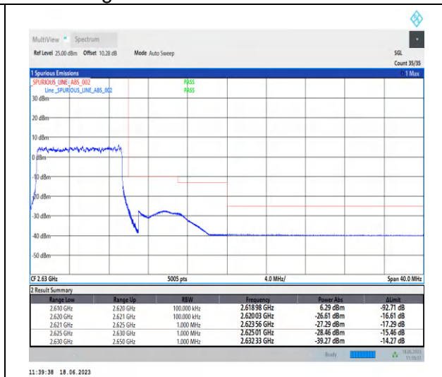
1-N38-PC3-30-10-H-3-DFT-PI2BPSK-Outer_Full-2 4@0-Ant0-1--PASS-see graph
