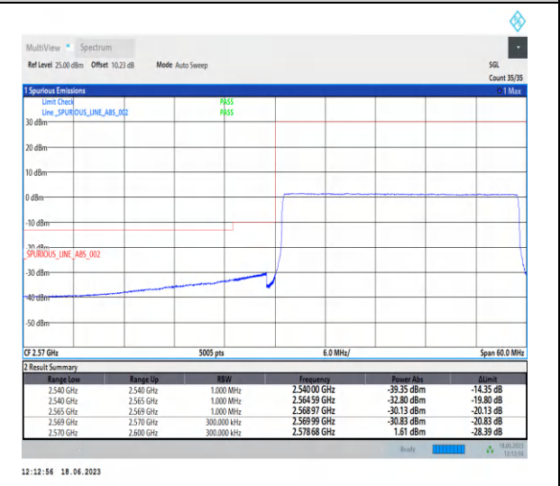
1-N38-PC3-30-30-L-6-CP-QPSK-Outer_Full-78@0-Ant0-1--PASS-see graph
