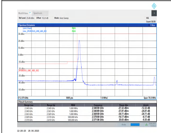
1-N38-PC3-30-40-L-4-CP-QPSK-Edge_1RB_Left-1@0-Ant0-1--PASS-see graph
