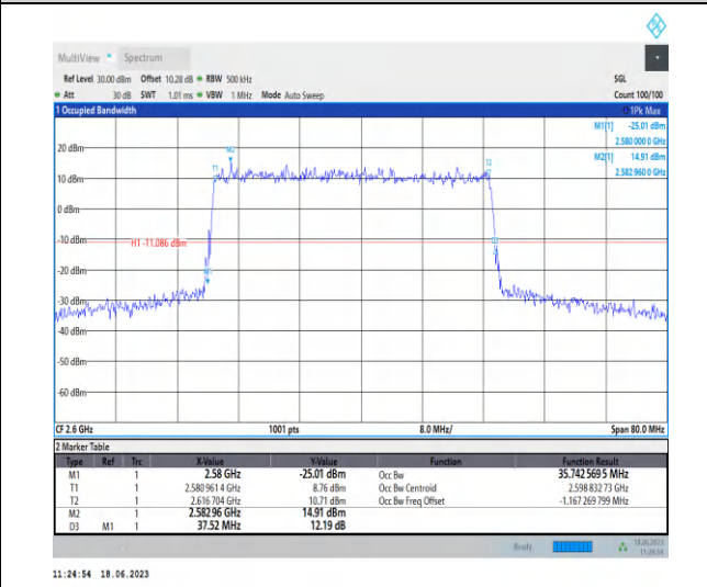
1-N38-PC3-30-40-H-2-DFT-QPSK-Outer_Full-100@ 0-Ant0-35.743-37.520-≤40-PASS
