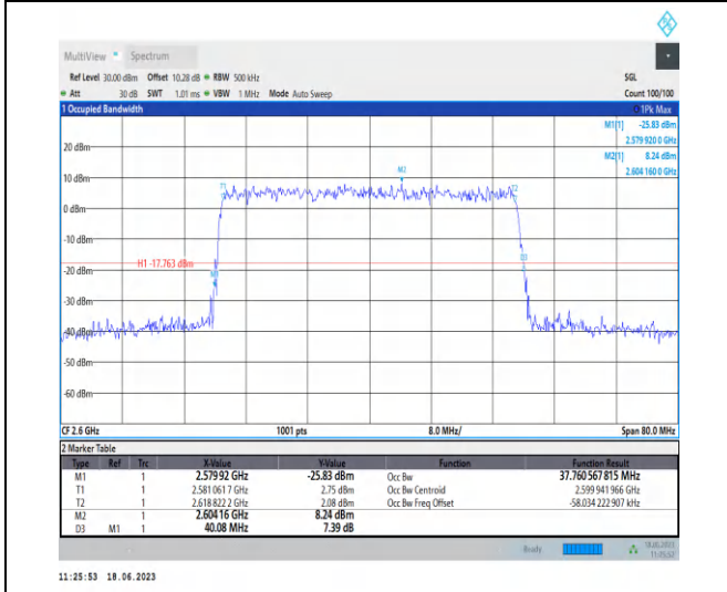
1-N38-PC3-30-40-H-9-CP-256QAM-Outer_Full-106 @0-Ant0-37.761-40.080-≤40-PASS
