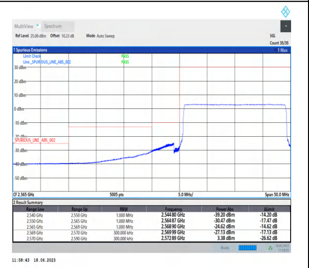
1-N38-PC3-30-20-L-6-CP-QPSK-Outer_Full-51@0-Ant0-1--PASS-see graph
