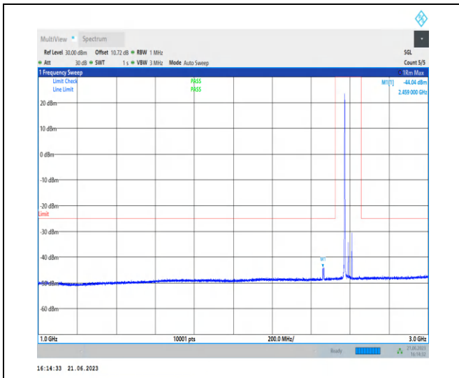
1-N38-PC3-30-40-L-1-N/A-DFT-PI2BPSK-Inner_1RB _Left-1 @ 1-1000-3000-Ant0-2413.50--44.04--25-PAS S
