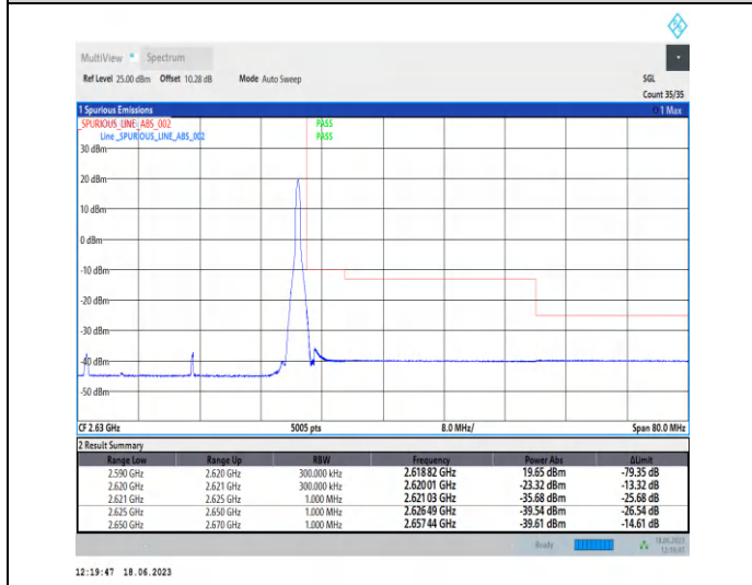
1-N38-PC3-30-30-H-5-CP-QPSK-Edge_1RB_Righ t-1@77-Ant0-1--PASS-see graph
