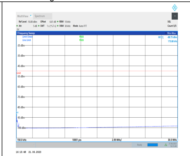
1-N38-PC3-30-40-M-1-N/A-DFT-PI2BPSK-Inner_1R B_Left-1@1-0.15-30-Ant0-27.61--88.73--45-PASS
