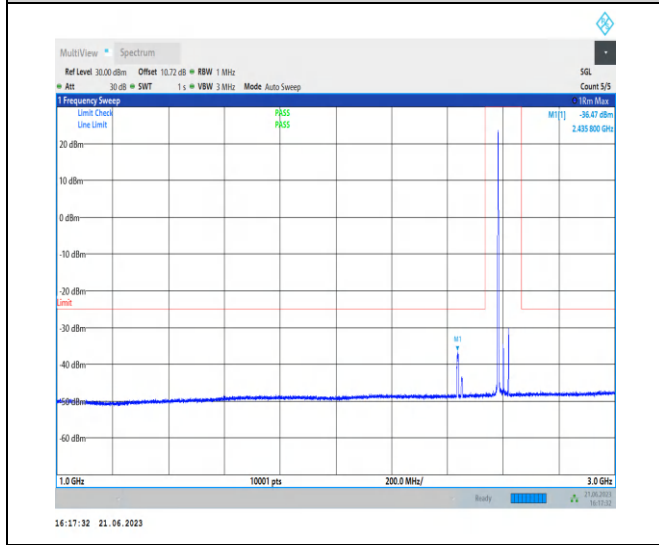
1-N38-PC3-30-40-H-1-N/A-DFT-PI2BPSK-Inner_1R B_Left-1@1-1000-3000-Ant0-2461.00--36.47--25-PASS
