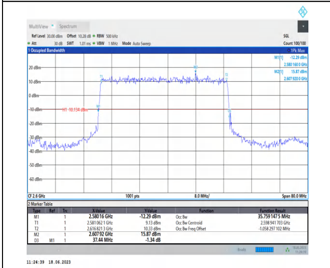
1-N38-PC3-30-40-H-1-DFT-PI2BPSK-Outer_Full-100@ 0@0-Ant0-35.759-37.440-≤40-PASS
