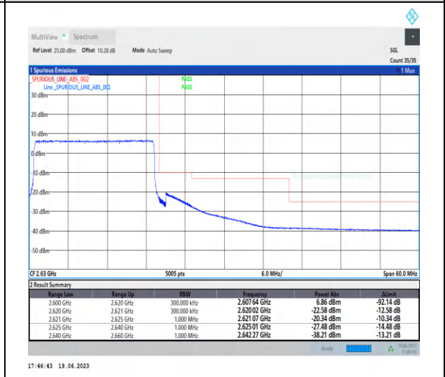
1-N38-PC2-30-20-H-3-CP-QPSK-Outer_Full-51@0-Ant0-1--PASS-see graph
