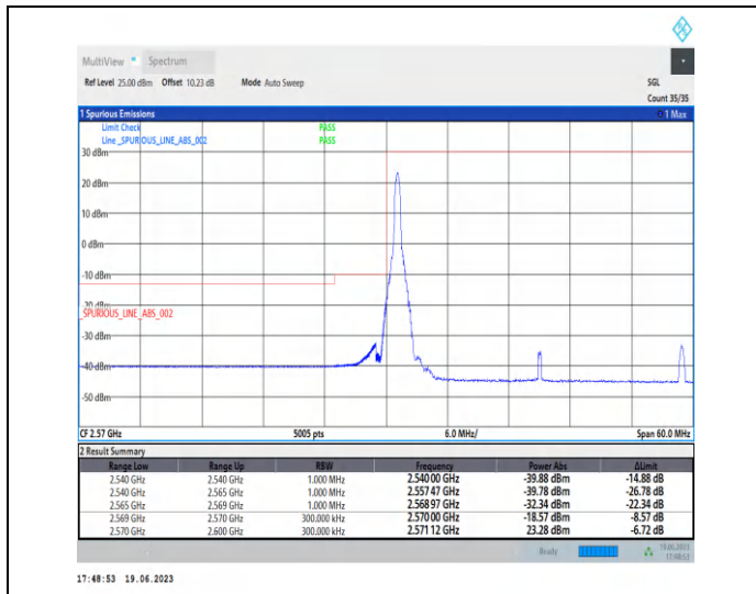
1-N38-PC2-30-30-L-1-CP-QPSK-Edge_1RB_Left-1@0-Ant0-1--PASS-see graph
