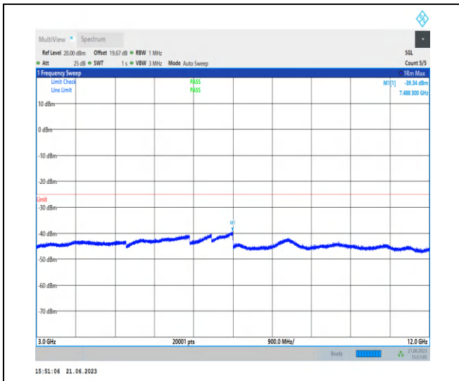
1-N38-PC2-30-40-H-1-N/A-DFT-QPSK-Edge_1RB_Left-1@0-3000-12000-Ant0-7488.30--39.34--25-PA SS
