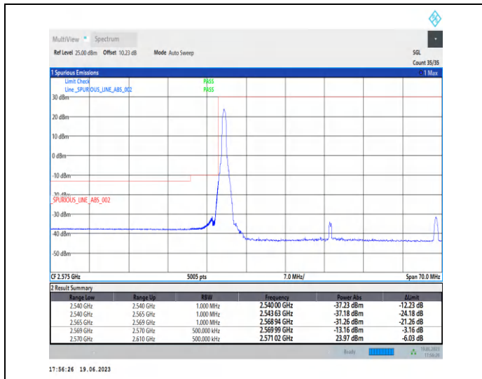
1-N38-PC2-30-40-L-1-CP-QPSK-Edge_1RB_Left-1@0-Ant0-1--PASS-see graph
