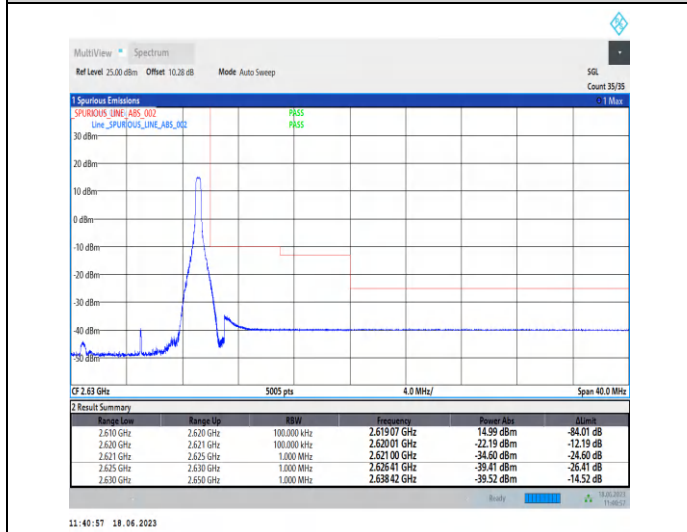
1-N38-PC3-30-10-H-5-CP-QPSK-Edge_1RB_Righ t-1@23-Ant0-1--PASS-see graph
