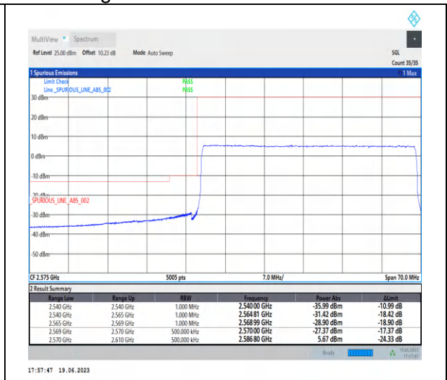
1-N38-PC2-30-40-L-3-CP-QPSK-Outer_Full-106@0-Ant0-1--PASS-see graph
