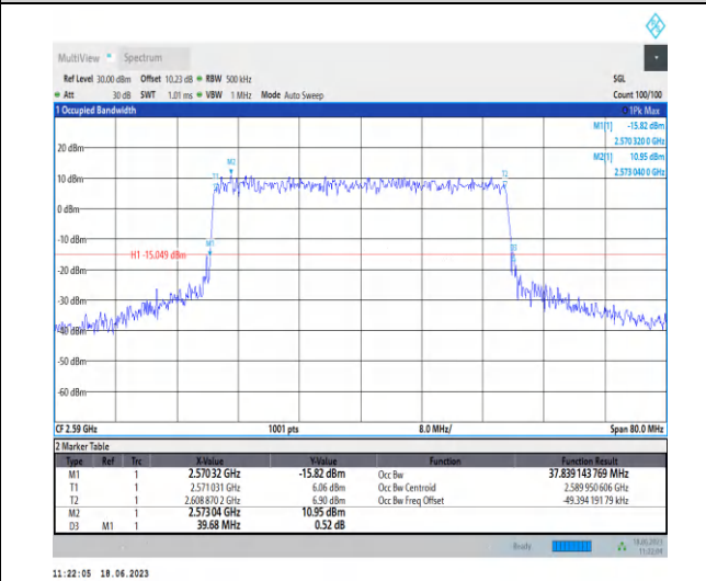
1-N38-PC3-30-40-L-8-CP-64QAM-Outer_Full-106 @ 0-Ant0-37.839-39.680-≤40-PASS
