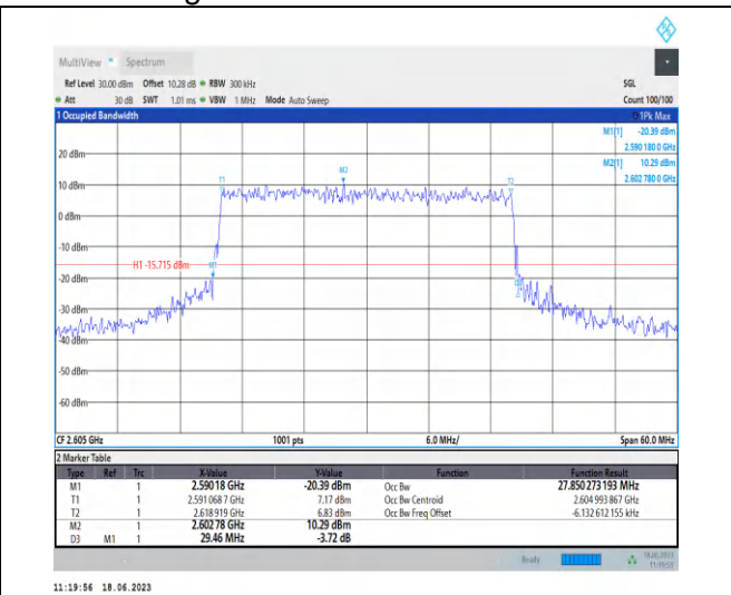
1-N38-PC3-30-30-H-7-CP-16QAM-Outer_Full-78@0-Ant0-27.85-29.460-≤30-PASS
