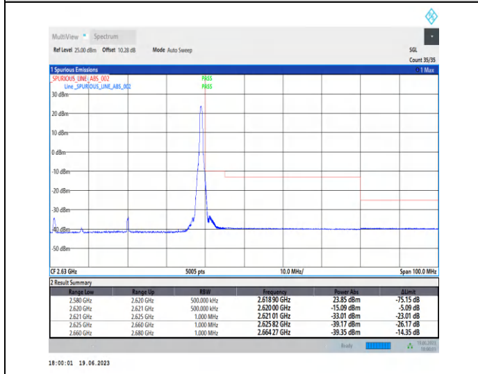
1-N38-PC2-30-40-H-2-CP-QPSK-Edge_1RB_Right-1@105-Ant0-1--PASS-see graph
