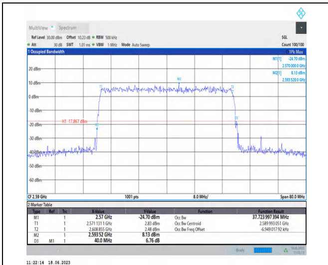
1-N38-PC3-30-40-L-9-CP-256QAM-Outer_Full-106 @ 0-Ant0-37.724-40.000-≤40-PASS
