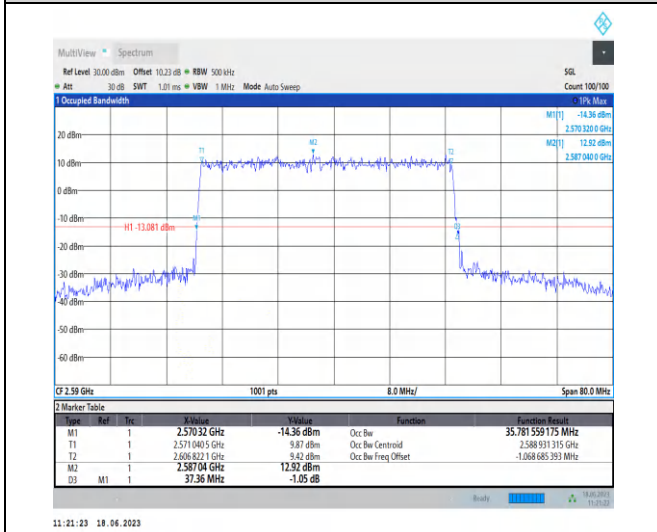
1-N38-PC3-30-40-L-3-DFT-16QAM-Outer_Full-100 @ 0-Ant0-35.782-37.360-≤40-PASS
