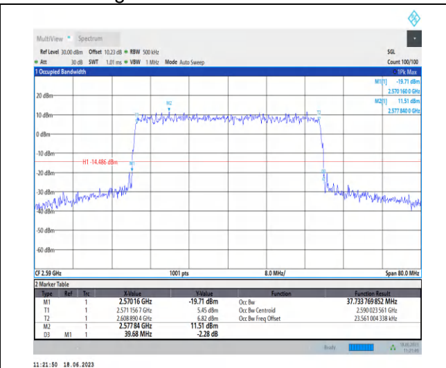
1-N38-PC3-30-40-L-6-CP-QPSK-Outer_Full-106 @ 0-Ant0-37.734-39.680-≤40-PASS
