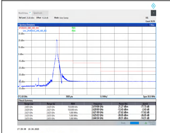
1-N38-PC2-30-15-H-2-CP-QPSK-Edge_1RB_Right-1@37-Ant0-1--PASS-see graph
