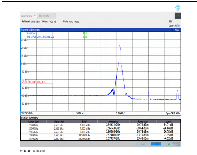
1-N38-PC2-30-20-L-1-CP-QPSK-Edge_1RB_Left-1@0-Ant0-1--PASS-see graph
