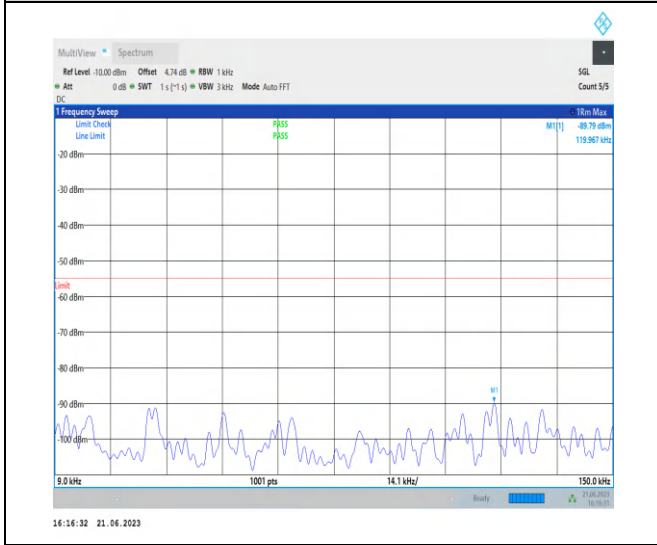
1-N38-PC3-30-40-H-1-DFT-PI2BPSK-Inner_1RB_Le ft-1@1-0.009-0.15-Ant0-0.12--89.79--55-PASS
