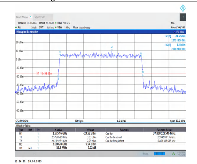
1-N38-PC3-30-40-M-9-CP-256QAM-Outer_Full-106 @0-Ant0-37.869-39.600-≤40-PASS
