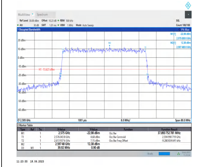
1-N38-PC3-30-40-M-6-CP-QPSK-Outer_Full-106 @ 0-Ant0-37.894-39.920-≤40-PASS
