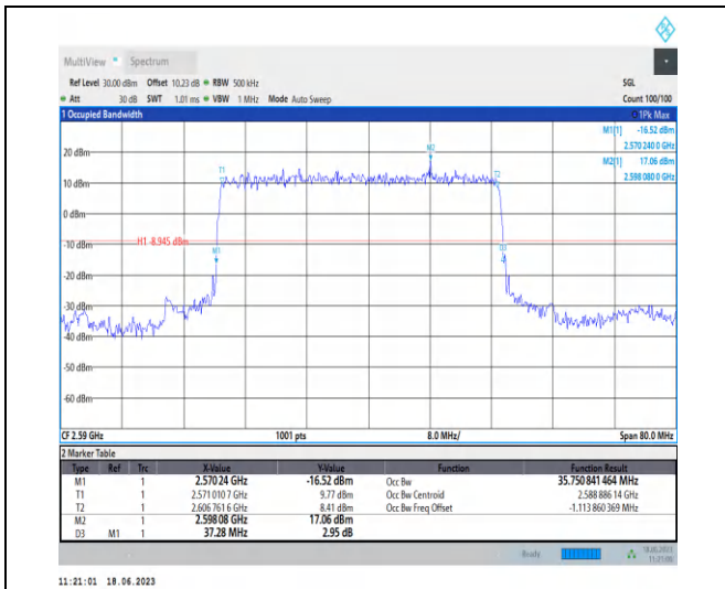
1-N38-PC3-30-40-L-1-DFT-PI2BPSK-Outer_Full-100 @ 0-Ant0-35.751-37.280-≤40-PASS
