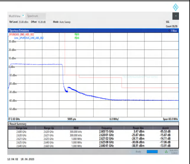
1-N38-PC3-30-20-H-6-CP-QPSK-Outer_Full-51 @ 0-Ant0-1--PASS-see graph
