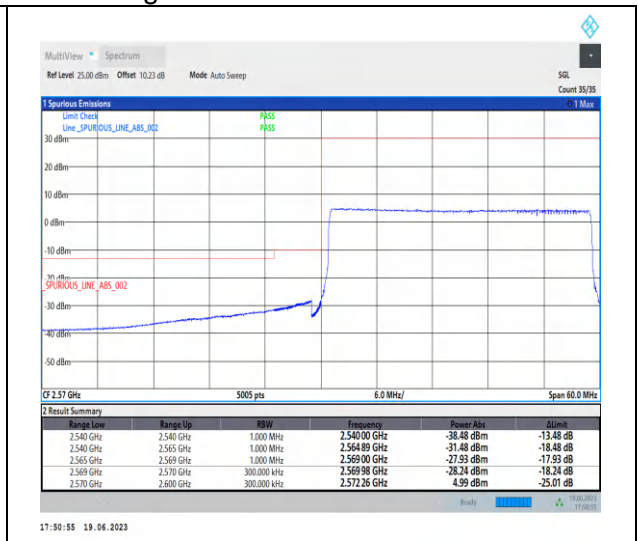
1-N38-PC2-30-30-L-3-CP-QPSK-Outer_Full-78@0-Ant0-1--PASS-see graph
