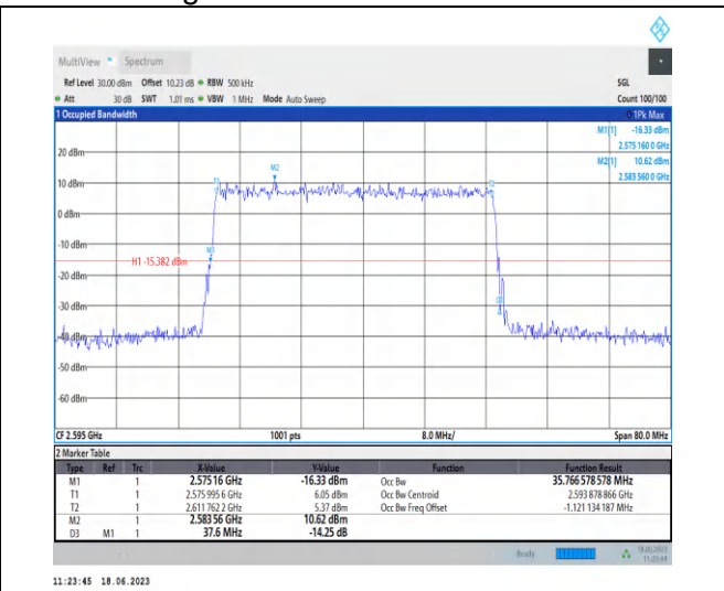
1-N38-PC3-30-40-M-5-DFT-256QAM-Outer_Full-100 @ 0-Ant0-35.767-37.600-≤40-PASS
