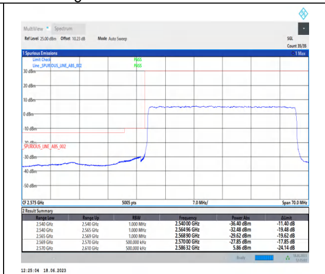
1-N38-PC3-30-40-L-3-DFT-PI2BPSK-Outer_Full-100@0-Ant0-1--PASS-see graph
