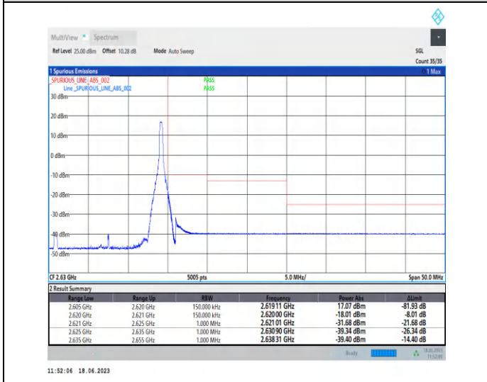
1-N38-PC3-30-15-H-5-CP-QPSK-Edge_1RB_Righ t-1@37-Ant0-1--PASS-see graph
