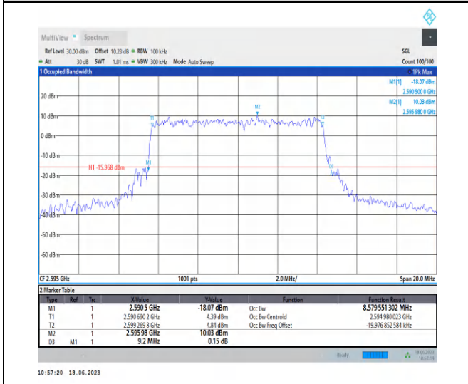
1-N38-PC3-30-10-M-6-CP-QPSK-Outer_Full-24@0- Ant0-8.58-9.200-≤10-PASS
