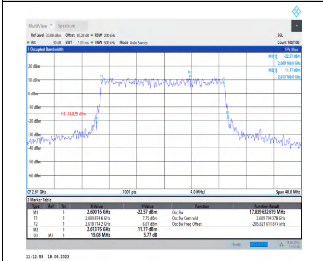
1-N38-PC3-30-20-H-3-DFT-16QAM-Outer_Full-50 @ 0-Ant0-17.84-19.080-≤20-PASS
