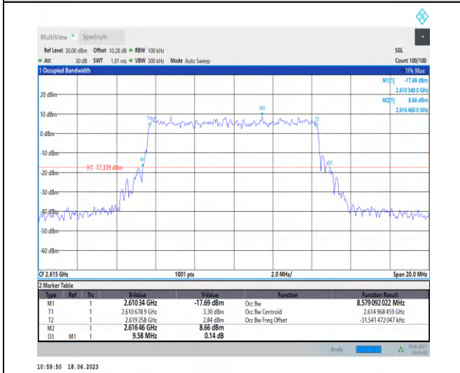
1-N38-PC3-30-10-H-5-DFT-256QAM-Outer_Full-24@0-Ant0-8.579-9.580-≤10-PASS
