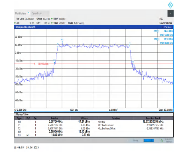
1-N38-PC3-30-15-M-8-CP-64QAM-Outer_Full-38 @ 0-Ant0-13.573-14.850-≤15-PASS
