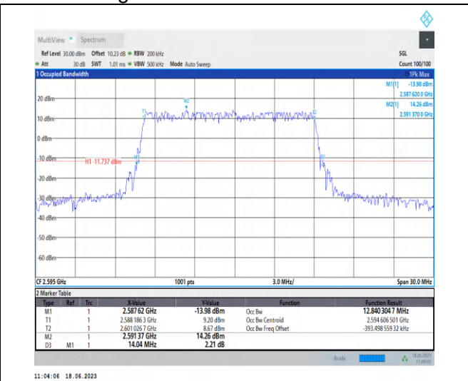
1-N38-PC3-30-15-M-2-DFT-QPSK-Outer_Full-36 @0-Ant0-12.84-14.040-≤15-PASS
