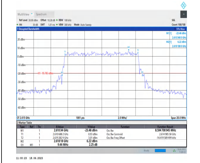
1-N38-PC3-30-10-H-9-CP-256QAM-Outer_Full-24@0 0-Ant0-8.595-9.440-≤10-PASS
