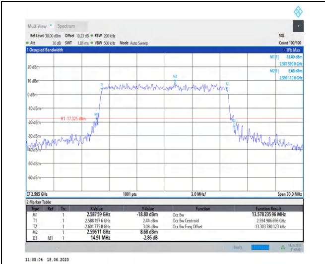
1-N38-PC3-30-15-M-9-CP-256QAM-Outer_Full-38@ 0-Ant0-13.578-14.910-≤15-PASS
