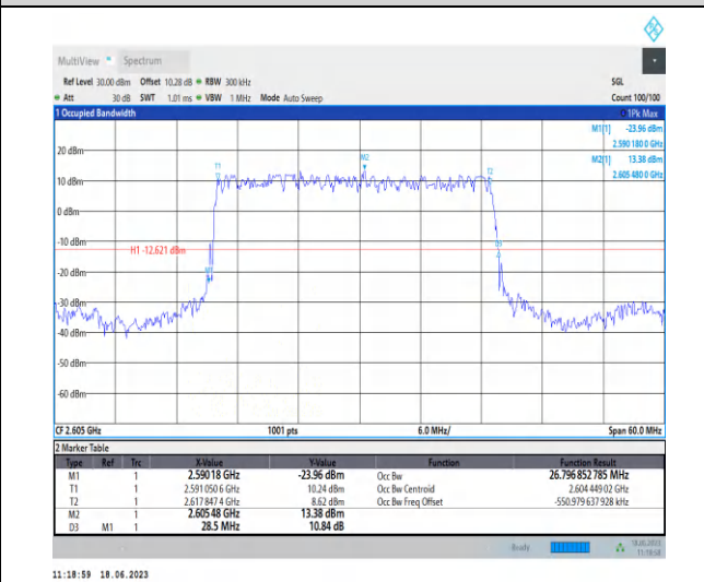
1-N38-PC3-30-30-H-1-DFT-PI2BPSK-Outer_Full-75@0 -Ant0-26.797-28.500-≤30-PASS
