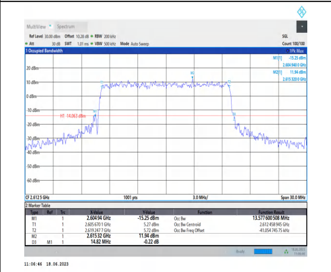
1-N38-PC3-30-15-H-7-CP-16QAM-Outer_Full-38@0- Ant0-13.578-14.820-≤15-PASS
