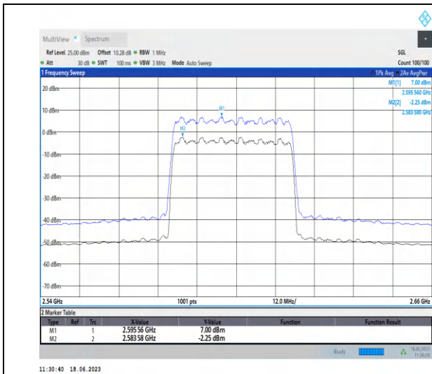
1-N38-PC3-30-40-H-1-DFT-256QAM-Outer_Full-100 @0-Ant0-9.25-100%-0.00-9.25-PASS-≤13
