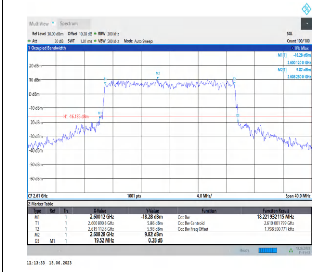
1-N38-PC3-30-20-H-7-CP-16QAM-Outer_Full-51 @ 0-Ant0-18.222-19.520-≤20-PASS
