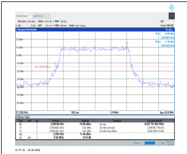
1-N38-PC3-30-10-M-4-DFT-64QAM-Outer_Full-24@ 0-Ant0-8.598-9.560-≤10-PASS
