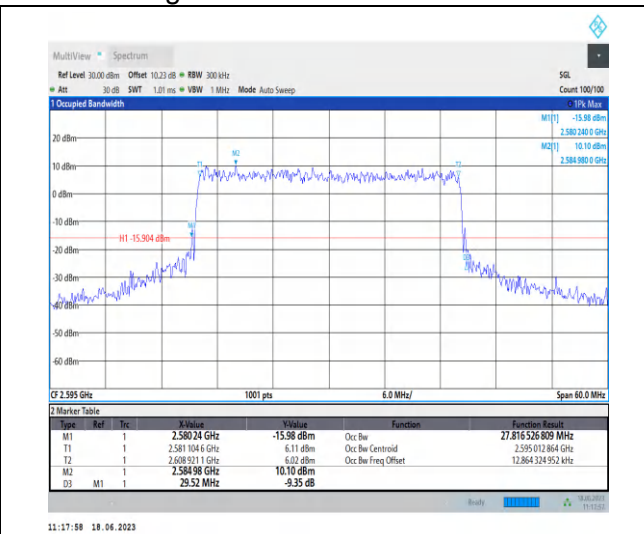
1-N38-PC3-30-30-M-8-CP-64QAM-Outer_Full-78@0 -Ant0-27.817-29.520-≤30-PASS
