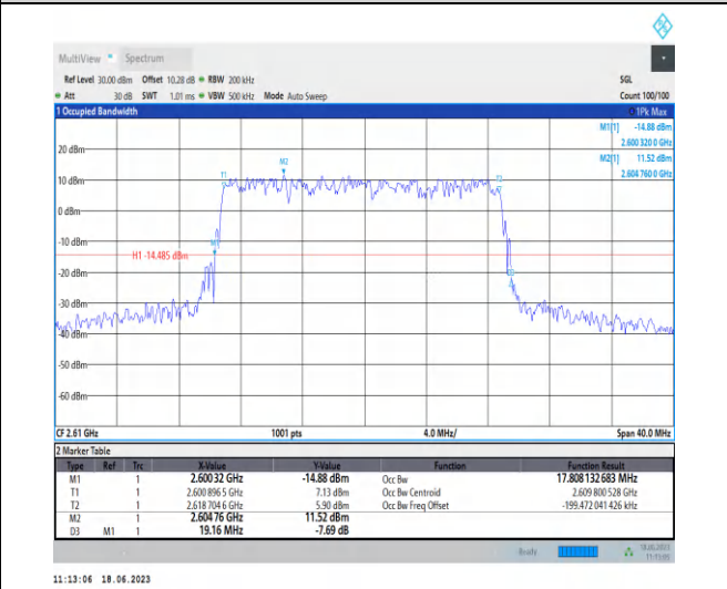
1-N38-PC3-30-20-H-4-DFT-64QAM-Outer_Full-50 @ 0-Ant0-17.808-19.160-≤20-PASS
