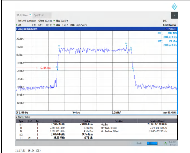
1-N38-PC3-30-30-M-5-DFT-256QAM-Outer_Full-75@ 0-Ant0-26.733-28.260-≤30-PASS
