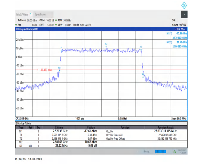
1-N38-PC3-30-30-L-7-CP-16QAM-Outer_Full-78@0-Ant0-27.833-29.220-≤30-PASS
