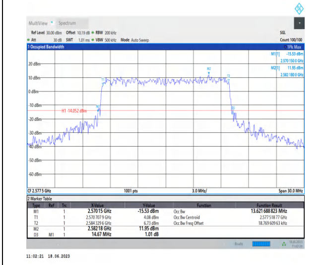
1-N38-PC3-30-15-L-8-CP-64QAM-Outer_Full-38@0-Ant0-13.622-14.670-≤15-PASS
