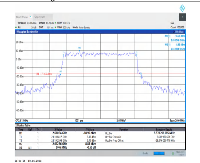
1-N38-PC3-30-10-H-8-CP-64QAM-Outer_Full-24@0 -Ant0-8.578-9.460-≤10-PASS
