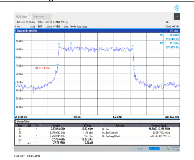
1-N38-PC3-30-30-L-1-DFT-PI2BPSK-Outer_Full-75 @ 0-Ant0-26.806-27.780-<=30-PASS
