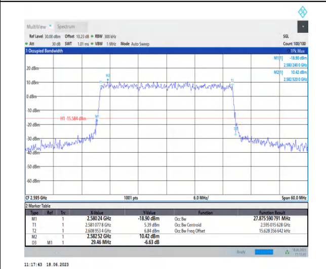
1-N38-PC3-30-30-M-6-CP-QPSK-Outer_Full-78@0- Ant0-27.876-29.460-≤30-PASS
