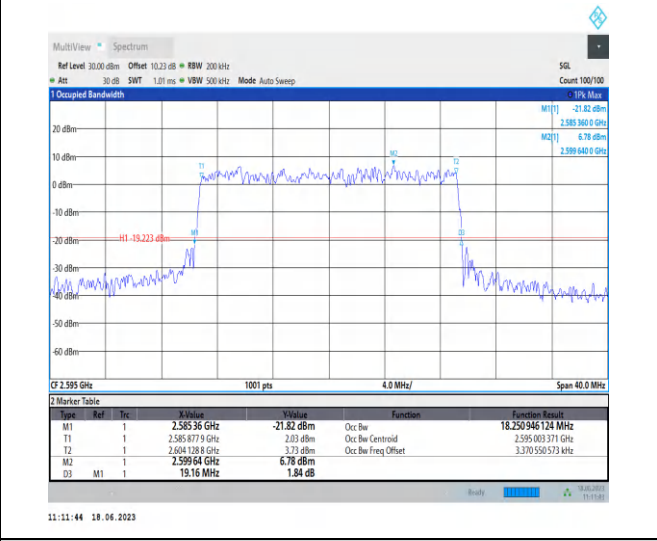
1-N38-PC3-30-20-M-9-CP-256QAM-Outer_Full-51@0-Ant0-18.251-19.160-<=20-PASS
