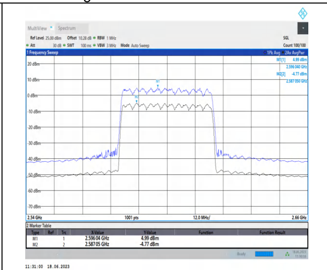
1-N38-PC3-30-40-H-2-CP-256QAM-Outer_Full-106 @0-Ant0-9.76-100%-0.00-9.76-PASS-≤13
