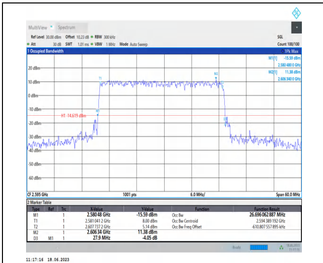
1-N38-PC3-30-30-M-3-DFT-16QAM-Outer_Full-75@ 0-Ant0-26.696-27.900-≤30-PASS
