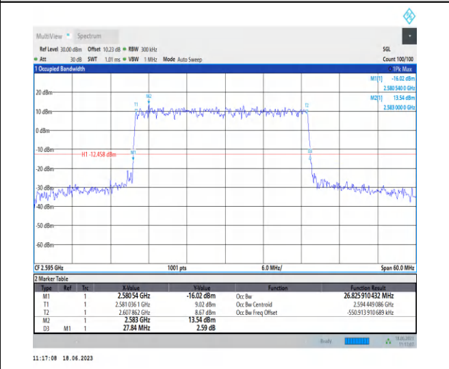
1-N38-PC3-30-30-M-2-DFT-QPSK-Outer_Full-75@0-Ant0-26.826-27.840-≤30-PASS
