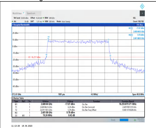
1-N38-PC3-30-20-H-6-CP-QPSK-Outer_Full-51 @ 0-Ant0-18.256-19.240-≤20-PASS
