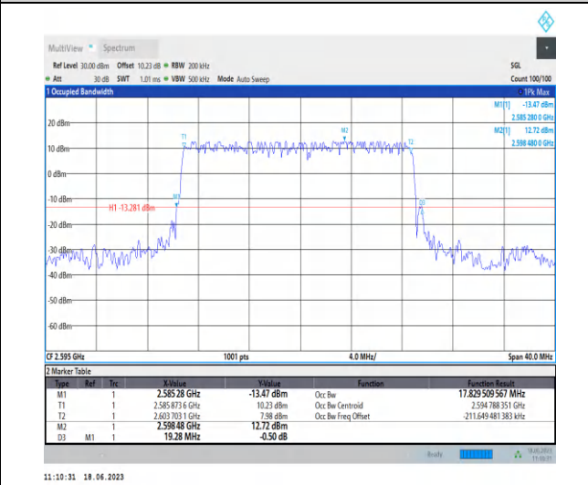
1-N38-PC3-30-20-M-1-DFT-PI2BPSK-Outer_Full-50@0-Ant0-17.83-19.280-≤20-PASS
