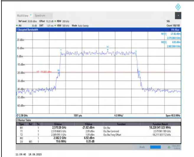
1-N38-PC3-30-20-L-9-CP-256QAM-Outer_Full-51@0-Ant0-18.227-19.600-≤20-PASS
