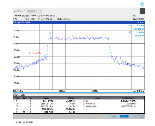
1-N38-PC3-30-15-M-7-CP-16QAM-Outer_Full-38 @ 0-Ant0-13.611-14.580-≤15-PASS
