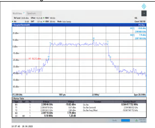
1-N38-PC3-30-10-M-9-CP-256QAM-Outer_Full-24@0-Ant0-8.564-9.180-≤10-PASS
