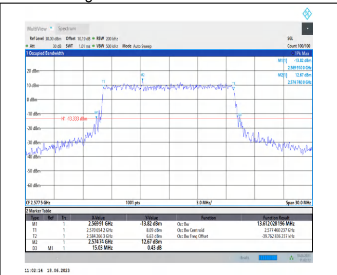
1-N38-PC3-30-15-L-7-CP-16QAM-Outer_Full-38@0-Ant0-13.612-15.030-≤15-PASS
