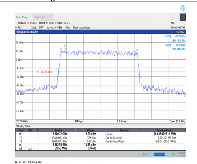
1-N38-PC3-30-30-M-4-DFT-64QAM-Outer_Full-75@ 0-Ant0-26.838-28.560-≤30-PASS
