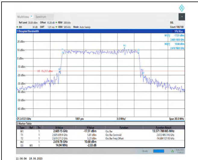
1-N38-PC3-30-15-H-8-CP-64QAM-Outer_Full-38@0 -Ant0-13.572-14.940-≤15-PASS
