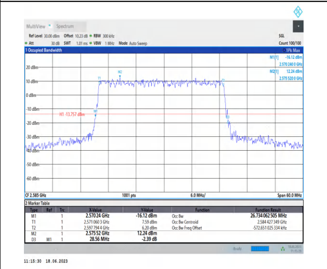
1-N38-PC3-30-30-L-3-DFT-16QAM-Outer_Full-75 @ 0-Ant0-26.734-28.560-<=30-PASS
