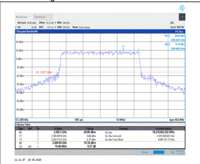
1-N38-PC3-30-20-M-7-CP-16QAM-Outer_Full-51@0-Ant0-18.217-19.480-<=20-PASS
