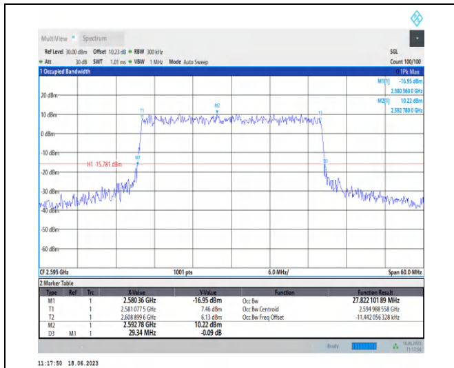
1-N38-PC3-30-30-M-7-CP-16QAM-Outer_Full-78@0 -Ant0-27.822-29.340-≤30-PASS
