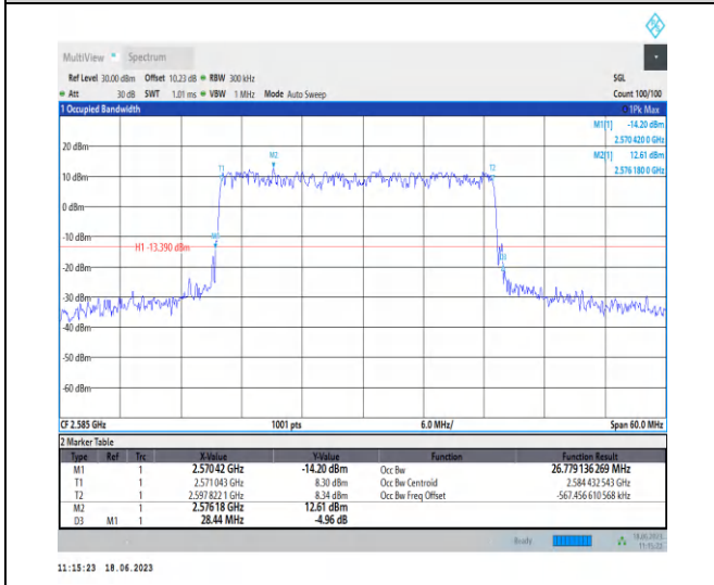
1-N38-PC3-30-30-L-2-DFT-QPSK-Outer_Full-75 @ 0- Ant0-26.779-28.440-<=30-PASS
