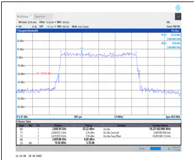
1-N38-PC3-30-20-H-9-CP-256QAM-Outer_Full-51 @ 0-Ant0-18.222-19.560-<=20-PASS
