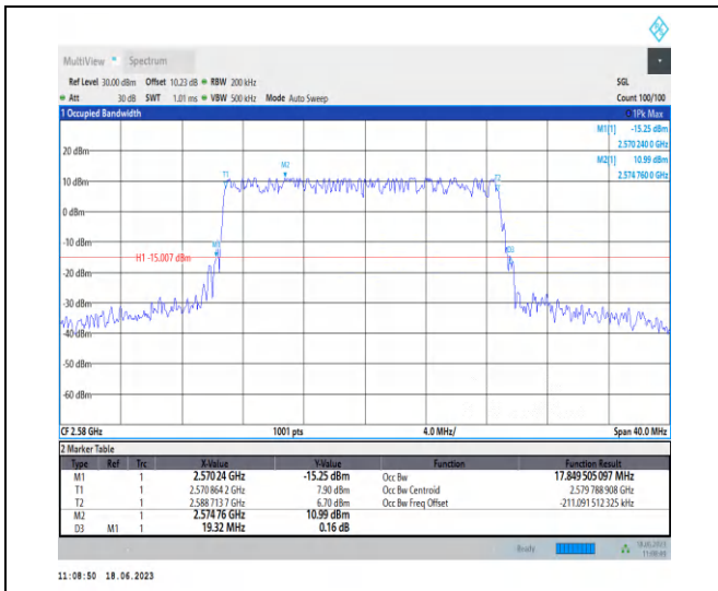
1-N38-PC3-30-20-L-3-DFT-16QAM-Outer_Full-50@0-Ant0-17.85-19.320-≤20-PASS
