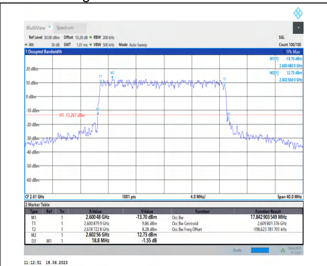
1-N38-PC3-30-20-H-2-DFT-QPSK-Outer_Full-50 @ 0-Ant0-17.843-18.800-≤20-PASS
