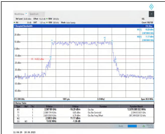
1-N38-PC3-30-15-M-5-DFT-256QAM-Outer_Full-36 @ 0-Ant0-12.877-13.920-≤15-PASS
