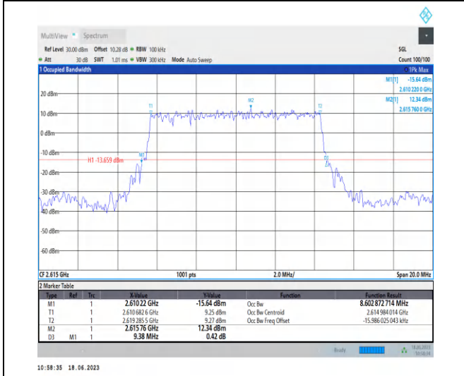
1-N38-PC3-30-10-H-1-DFT-PI2BPSK-Outer_Full-24@0-Ant0-8.603-9.380-≤10-PASS
