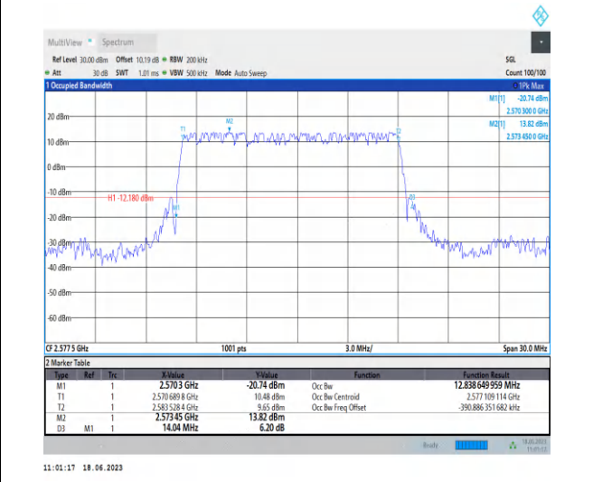
1-N38-PC3-30-15-L-1-DFT-PI2BPSK-Outer_Full-36@0 -Ant0-12.839-14.040-≤15-PASS
