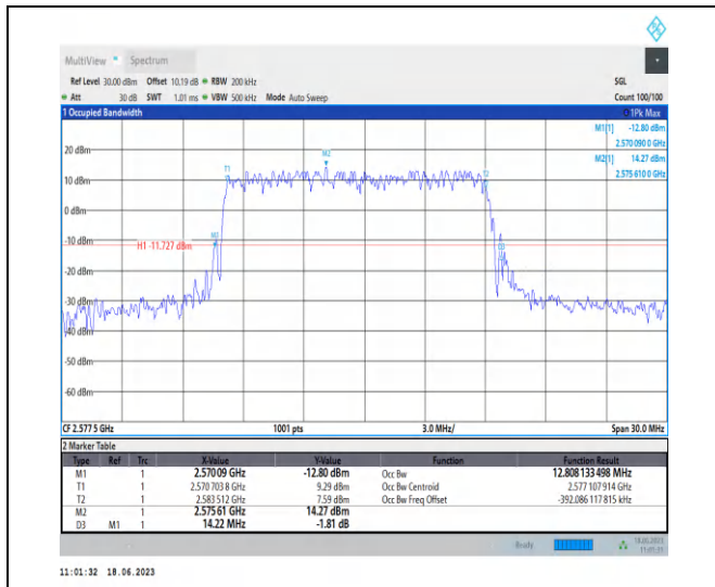
1-N38-PC3-30-15-L-2-DFT-QPSK-Outer_Full-36@0-Ant0-12.808-14.220-≤15-PASS
