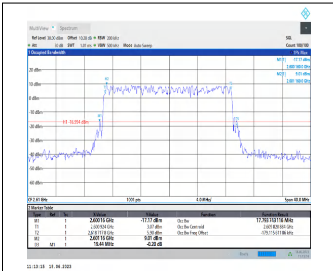
1-N38-PC3-30-20-H-5-DFT-256QAM-Outer_Full-50 @ 0-Ant0-17.794-19.440-≤20-PASS
