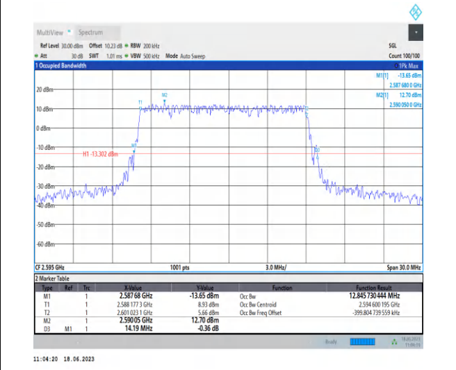
1-N38-PC3-30-15-M-4-DFT-64QAM-Outer_Full-36 @0-Ant0-12.846-14.190-≤15-PASS
