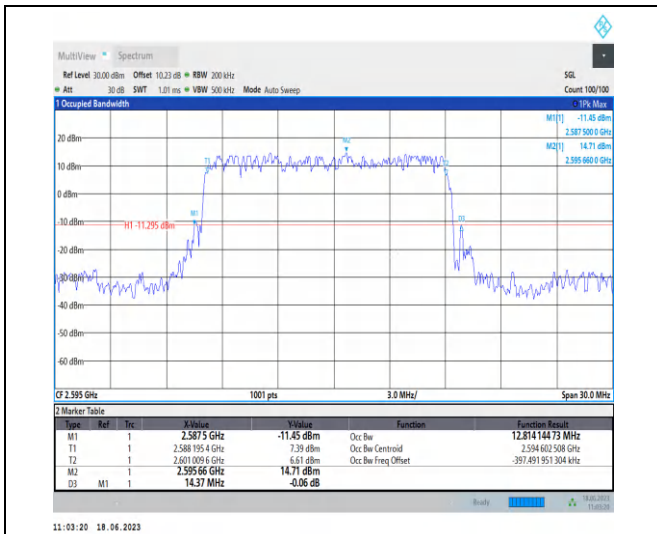
1-N38-PC3-30-15-M-1-DFT-PI2BPSK-Outer_Full-36 @0-Ant0-12.814-14.370-≤15-PASS
