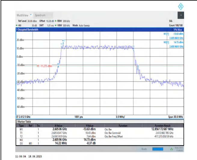
1-N38-PC3-30-15-H-2-DFT-QPSK-Outer_Full-36@0 -Ant0-12.856-14.220-≤15-PASS
