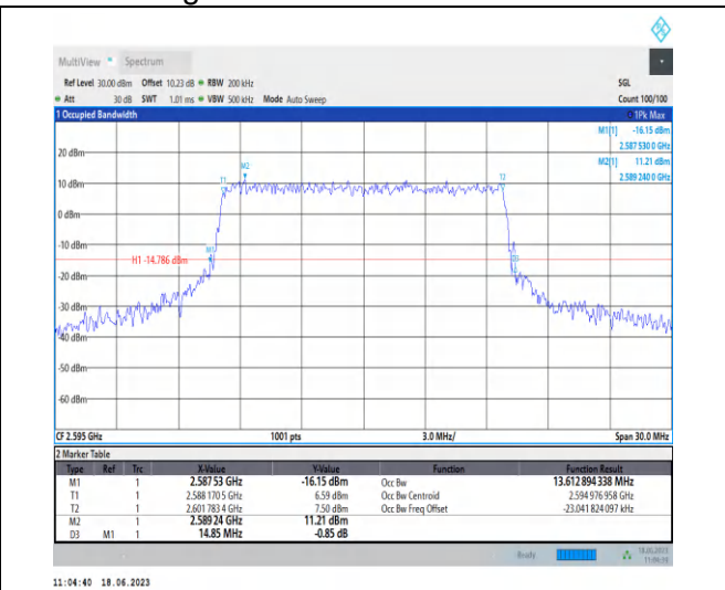
1-N38-PC3-30-15-M-6-CP-QPSK-Outer_Full-38 @ 0-Ant0-13.613-14.850-≤15-PASS
