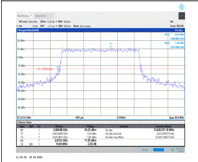
1-N38-PC3-30-15-H-6-CP-QPSK-Outer_Full-38@0- Ant0-13.62-14.940-≤15-PASS
