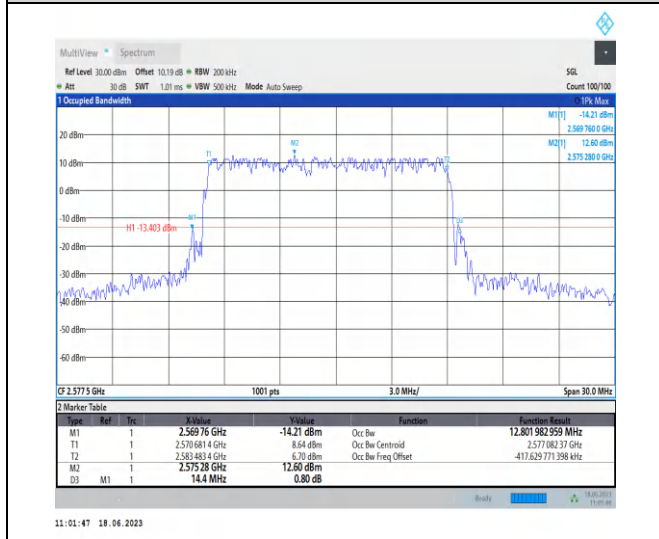
1-N38-PC3-30-15-L-4-DFT-64QAM-Outer_Full-36@0-Ant0-12.802-14.400-≤15-PASS
