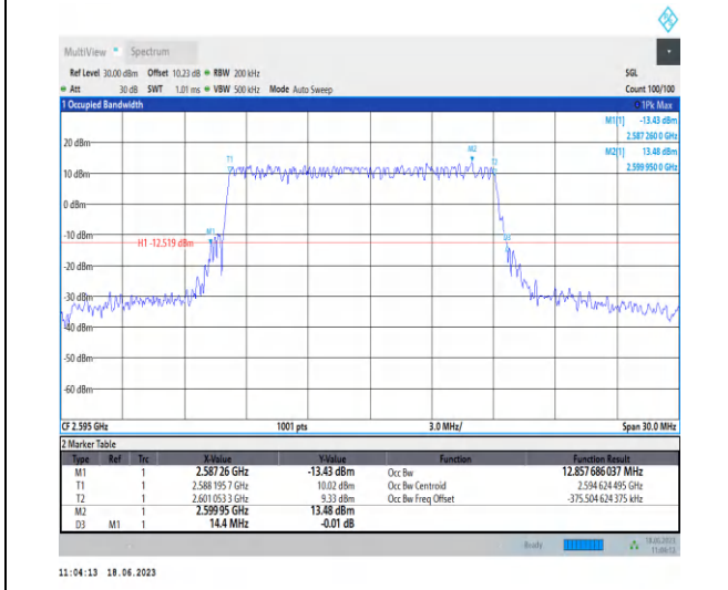
1-N38-PC3-30-15-M-3-DFT-16QAM-Outer_Full-36 @0-Ant0-12.858-14.400-≤15-PASS
