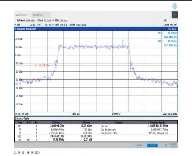
1-N38-PC3-30-15-H-3-DFT-16QAM-Outer_Full-36@ 0-Ant0-12.865-14.160-≤15-PASS
