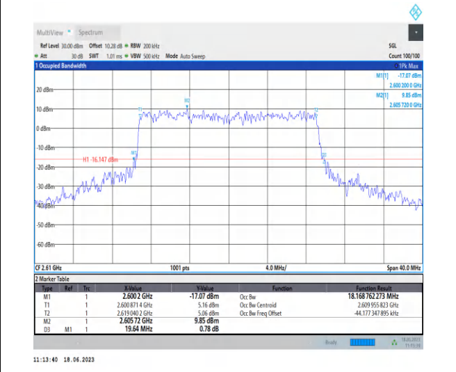
1-N38-PC3-30-20-H-8-CP-64QAM-Outer_Full-51 @ 0-Ant0-18.169-19.640-≤20-PASS
