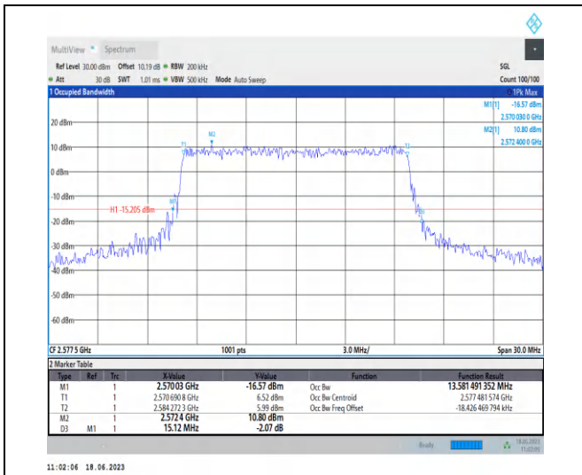
1-N38-PC3-30-15-L-6-CP-QPSK-Outer_Full-38@0-Ant0-13.581-15.120-≤15-PASS
