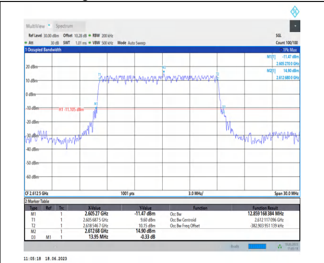
1-N38-PC3-30-15-H-1-DFT-PI2BPSK-Outer_Full-36@ 0-Ant0-12.859-13.950-≤15-PASS
