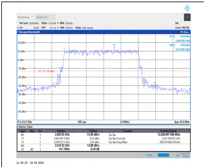
1-N38-PC3-30-15-H-4-DFT-64QAM-Outer_Full-36@ 0-Ant0-12.836-14.100-≤15-PASS
