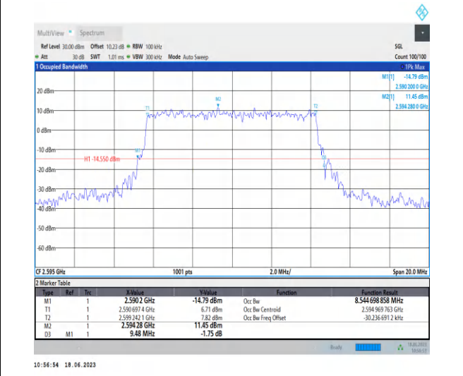
1-N38-PC3-30-10-M-3-DFT-16QAM-Outer_Full-24@0-Ant0-8.545-9.480-≤10-PASS
