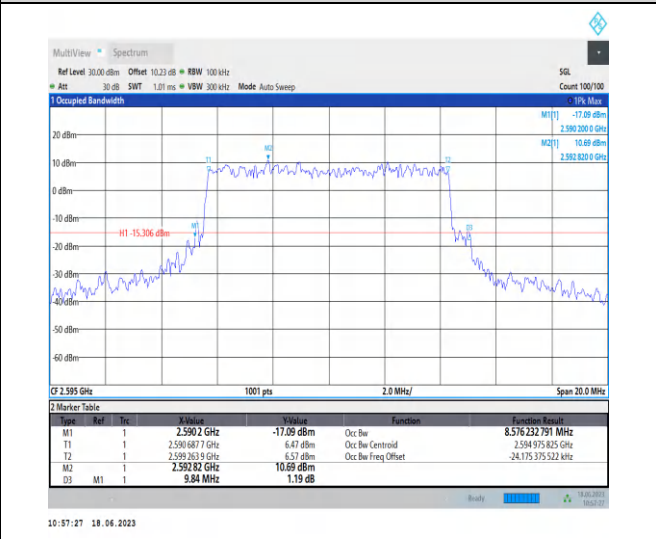
1-N38-PC3-30-10-M-7-CP-16QAM-Outer_Full-24@0- -Ant0-8.576-9.840-≤10-PASS
