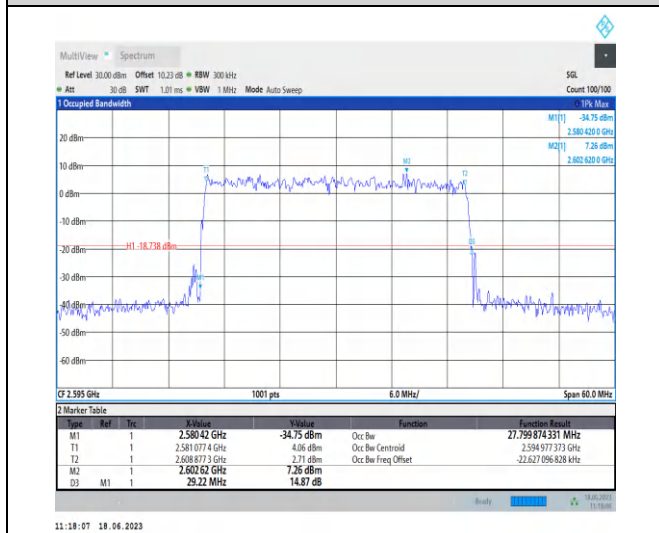
1-N38-PC3-30-30-M-9-CP-256QAM-Outer_Full-78@0 -Ant0-27.8-29.220-≤30-PASS
