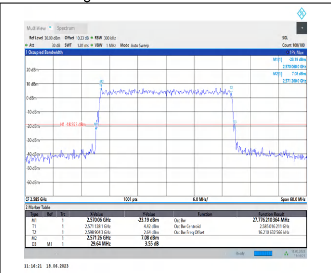
1-N38-PC3-30-30-L-9-CP-256QAM-Outer_Full-78@0-Ant0-27.776-29.640-≤30-PASS
