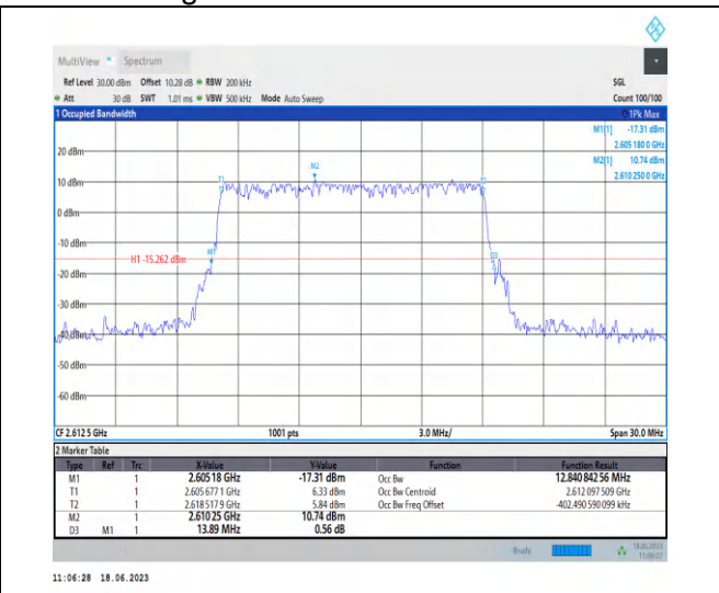
1-N38-PC3-30-15-H-5-DFT-256QAM-Outer_Full-36@ 0-Ant0-12.841-13.890-≤15-PASS
