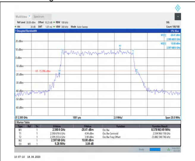
1-N38-PC3-30-10-M-5-DFT-256QAM-Outer_Full-24 @0-Ant0-8.579-9.280-≤10-PASS
