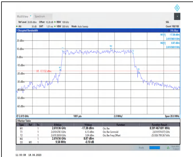
1-N38-PC3-30-10-H-7-CP-16QAM-Outer_Full-24@0 -Ant0-8.591-9.580-≤10-PASS
