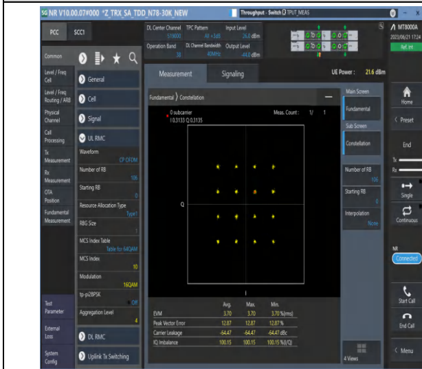
1-N38-PC3-30-40-M-7-CP-16QAM-Outer_Full-106 @0-Ant0-see graph-PASS
