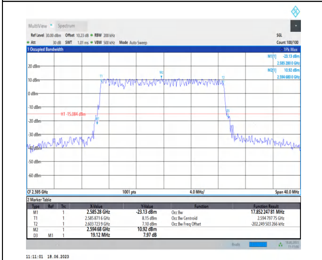
1-N38-PC3-30-20-M-4-DFT-64QAM-Outer_Full-50@0-Ant0-17.852-19.120-≤20-PASS
