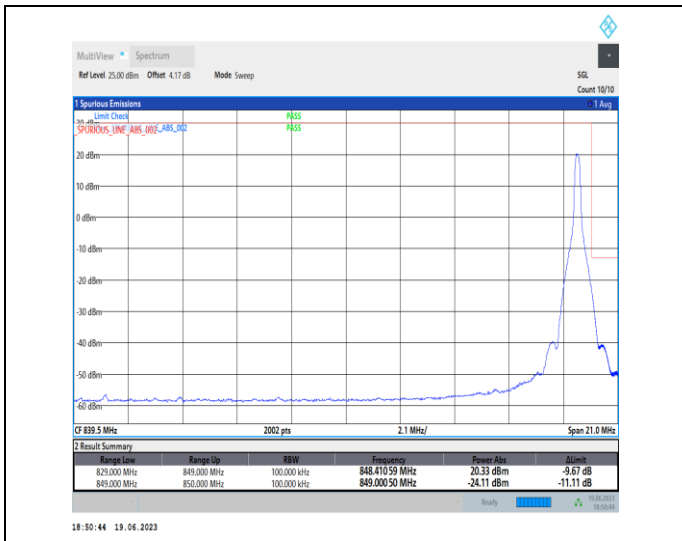
1-N26-824-849-PC3-15-20-H-2-DFT-PI2BPSK-Edge_1 RB_Right-1@105-Ant0-1-seegraph-PASS-see graph
