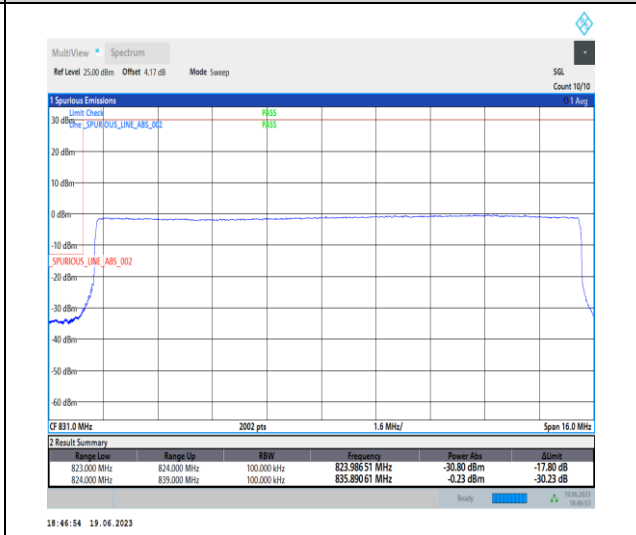
1-N26-824-849-PC3-15-15-L-6-CP-QPSK-Outer_Full-79@0-Ant0-1-seegraph-PASS-see graph
