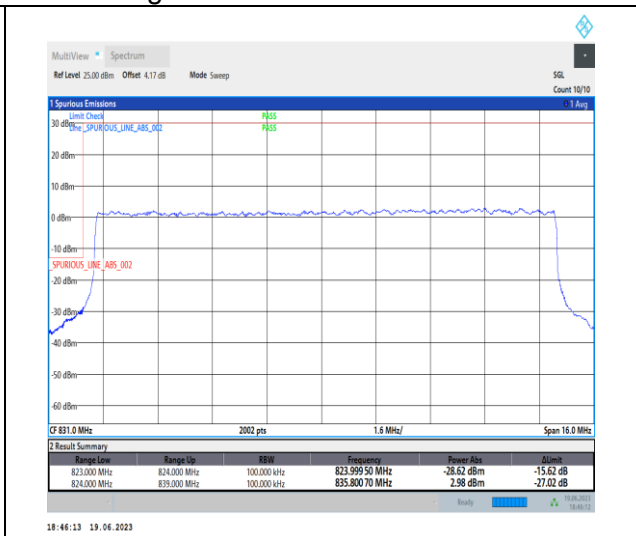
1-N26-824-849-PC3-15-15-L-3-DFT-PI2BPSK-Outer_Full-75@0-Ant0-1-seegraph-PASS-see graph
