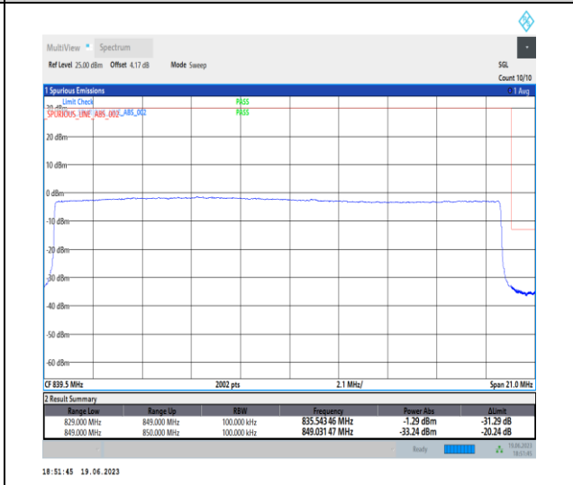
1-N26-824-849-PC3-15-20-H-6-CP-QPSK-Outer_Full-106@0-Ant0-1-seegraph-PASS-see graph
