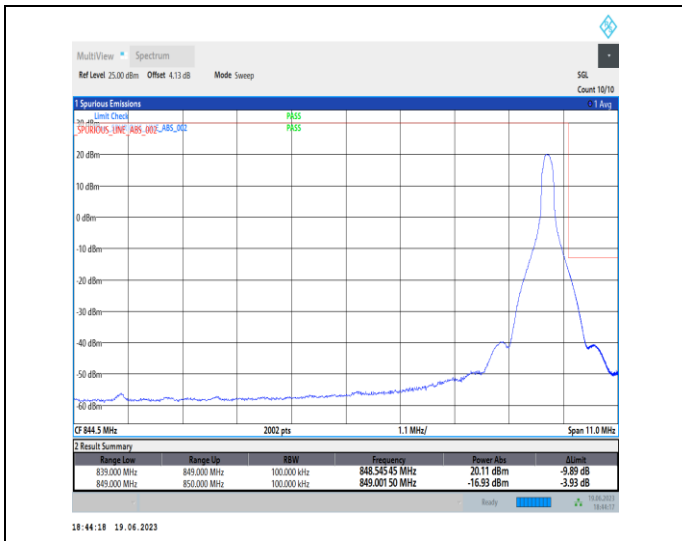
1-N26-824-849-PC3-15-10-H-2-DFT-PI2BPSK-Edge_1_RB_Right-1@51-Ant0-1-seegraph-PASS-see graph
