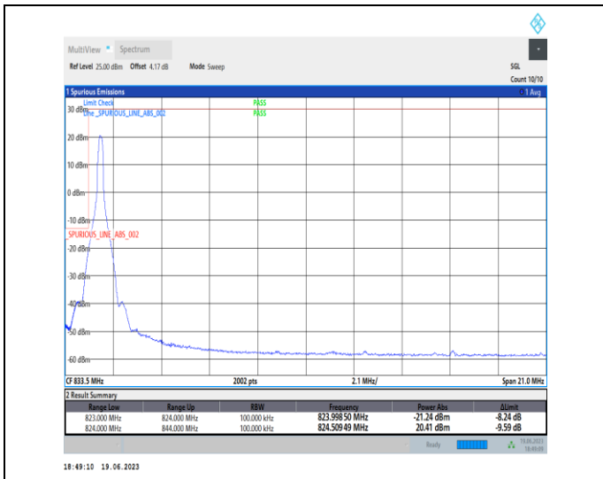
1-N26-824-849-PC3-15-20-L-1-DFT-PI2BPSK-Edge_1 RB_Left-1@0-Ant0-1-seegraph-PASS-see graph
