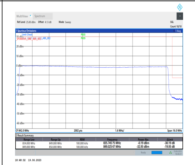
1-N26-824-849-PC3-15-15-H-6-CP-QPSK-Outer_Full-79@0-Ant0-1-seegraph-PASS-see graph
