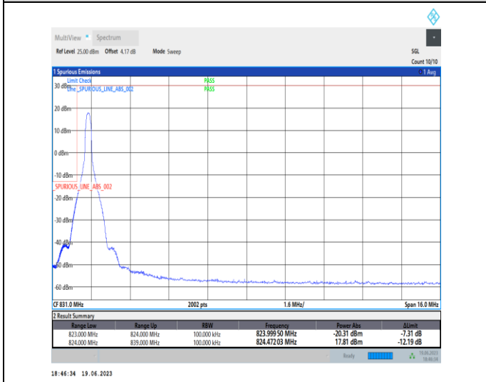
1-N26-824-849-PC3-15-15-L-4-CP-QPSK-Edge_1RB_Left-1@0-Ant0-1-seegraph-PASS-see graph
