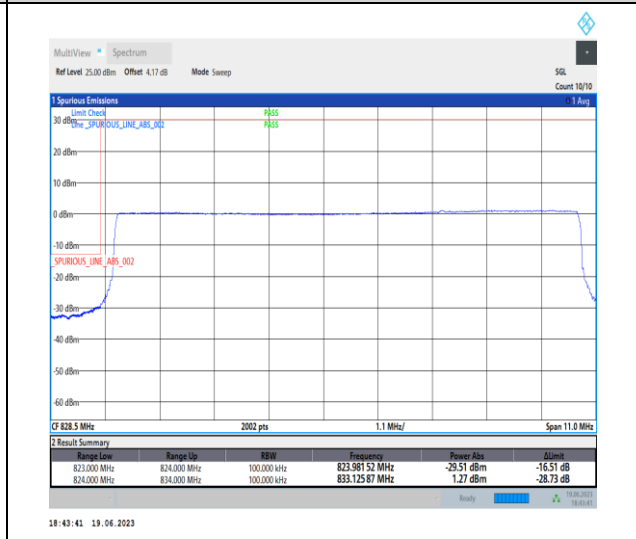
1-N26-824-849-PC3-15-10-L-6-CP-QPSK-Outer_Full-52@0-Ant0-1-seegraph-PASS-see graph
