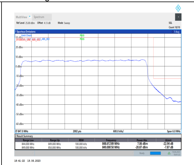
1-N26-824-849-PC3-15-5-H-3-DFT-PI2BPSK-Outer_Full-25@0-Ant0-1-seegraph-PASS-see graph
