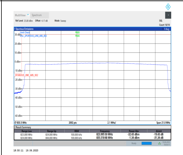
1-N26-824-849-PC3-15-20-L-6-CP-QPSK-Outer_Full-106@0-Ant0-1-seegraph-PASS-see graph
