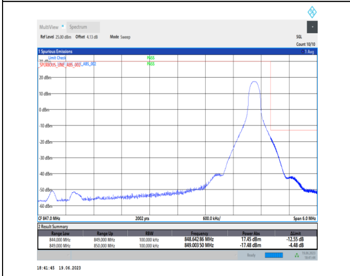
1-N26-824-849-PC3-15-5-H-5-CP-QPSK-Edge_1RB_Right-1@24-Ant0-1-seegraph-PASS-see graph
