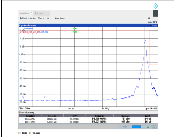
1-N26-824-849-PC3-15-15-H-5-CP-QPSK-Edge_1RB_Right-1@78-Ant0-1-seegraph-PASS-see graph
