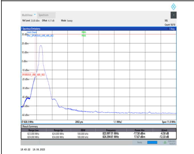
1-N26-824-849-PC3-15-10-L-4-CP-QPSK-Edge_1RB_Left-1@0-Ant0-1-seegraph-PASS-see graph
