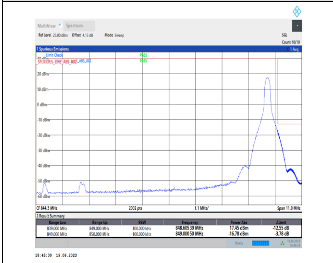
1-N26-824-849-PC3-15-10-H-5-CP-QPSK-Edge_1RB_Right-1@51-Ant0-1-seegraph-PASS-see graph
