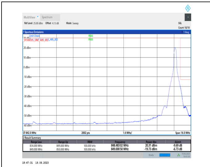
1-N26-824-849-PC3-15-15-H-2-DFT-PI2BPSK-Edge_1_RB_Right-1@78-Ant0-1-seegraph-PASS-see graph
