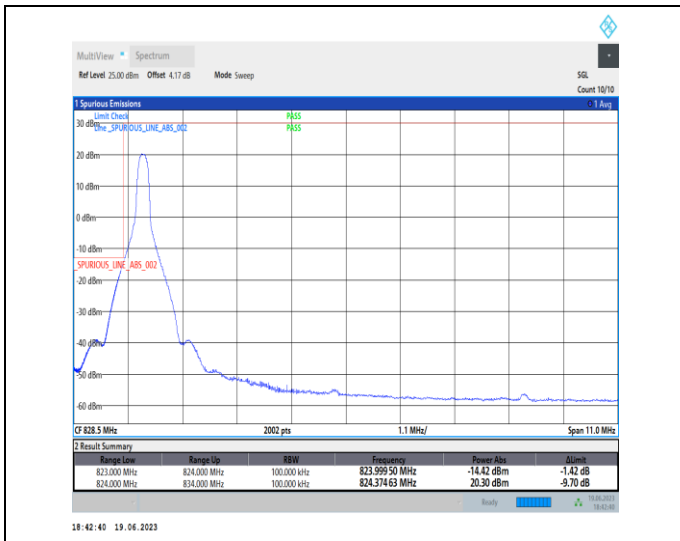
1-N26-824-849-PC3-15-10-L-1-DFT-PI2BPSK-Edge_1 RB_Left-1@0-Ant0-1-seegraph-PASS-see graph
