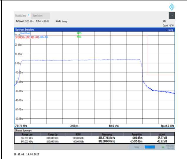
1-N26-824-849-PC3-15-5-H-6-CP-QPSK-Outer_Full-25@0-Ant0-1-seegraph-PASS-see graph
