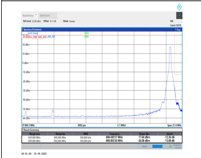
1-N26-824-849-PC3-15-20-H-5-CP-QPSK-Edge_1RB_Right-1@105-Ant0-1-seegraph-PASS-see graph
