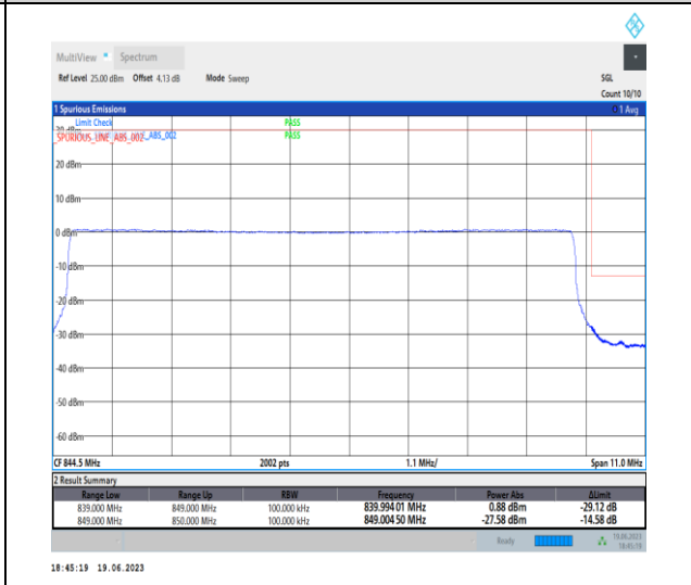
1-N26-824-849-PC3-15-10-H-6-CP-QPSK-Outer_Full-52@0-Ant0-1-seegraph-PASS-see graph
