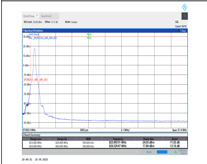
1-N26-824-849-PC3-15-20-L-4-CP-QPSK-Edge_1RB_Left-1@0-Ant0-1-seegraph-PASS-see graph
