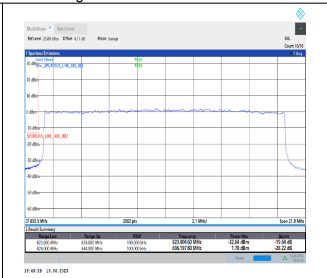
1-N26-824-849-PC3-15-20-L-3-DFT-PI2BPSK-Outer_Full-100@0-Ant0-1-seegraph-PASS-see graph
