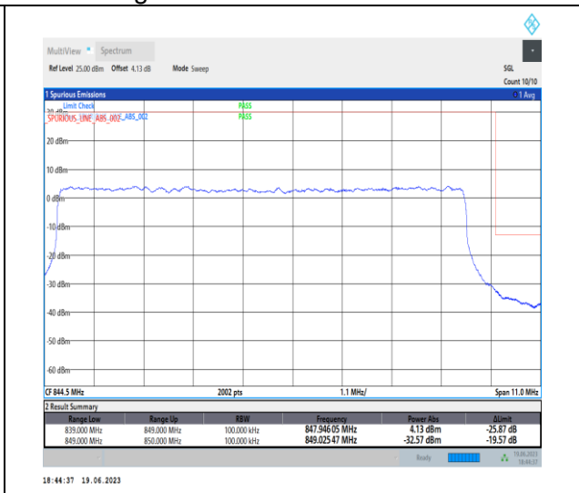
1-N26-824-849-PC3-15-10-H-3-DFT-PI2BPSK-Outer_Full-50@0-Ant0-1-seegraph-PASS-see graph
