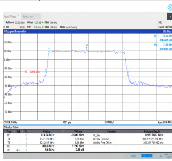
1-N26-814-824-PC3-15-10-M-3-DFT-16QAM-Outer_ Full-50@0-Ant0-8.924-9.600-≤10-PASS
