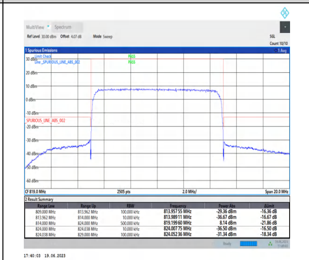
1-N26-814-824-PC3-15-10-L-6-CP-QPSK-Outer_F ull-52@0-Ant0-1--PASS-see graph
