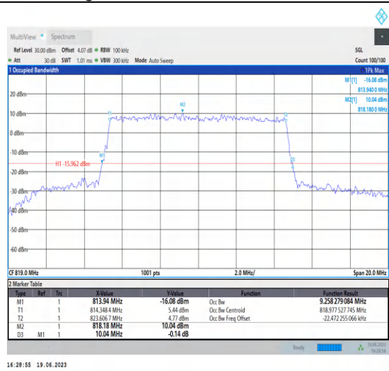
1-N26-814-824-PC3-15-10-M-7-CP-16QAM-Outer_Full I-52@0-Ant0-9.258-10.040-≤10-PASS
