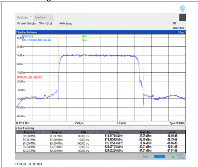
1-N26-814-824-PC3-15-10-L-3-DFT-PI2BPSK-Out er_Full-50@0-Ant0-1--PASS-see graph
