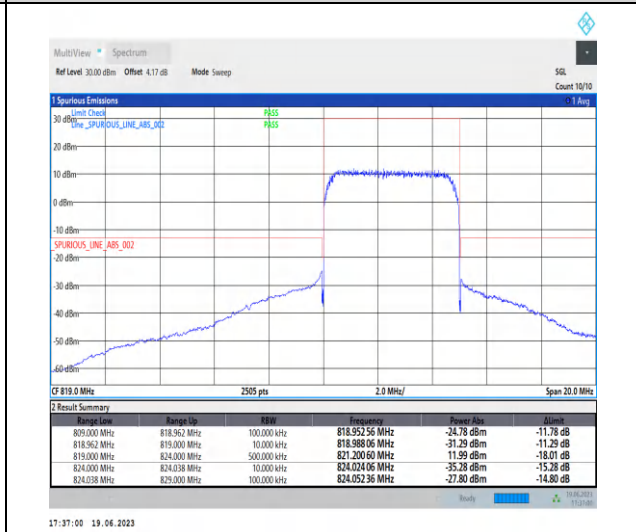
1-N26-814-824-PC3-15-5-H-6-CP-QPSK-Outer_Full-25@0-Ant0-1--PASS-see graph
