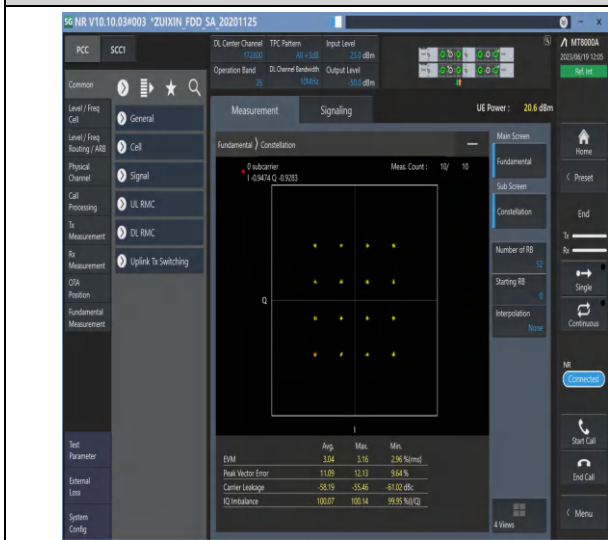
1-N26-814-824-PC3-15-10-M-7-CP-16QAM-Outer_Full-52@0-Ant0-see graph-PASS
