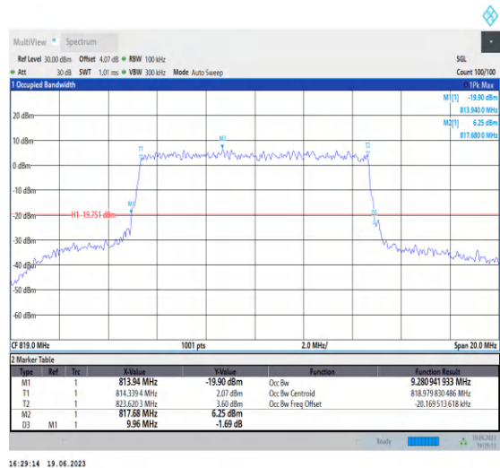
1-N26-814-824-PC3-15-10-M-9-CP-256QAM-Outer_Full I-52@0-Ant0-9.281-9.960-≤10-PASS
