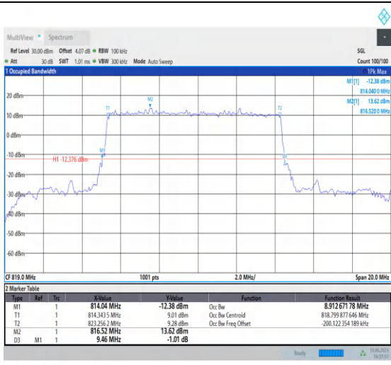
1-N26-814-824-PC3-15-10-M-2-DFT-PI2BPSK-Outer _Full-50@0-Ant0-8.913-9.460-≤10-PASS
