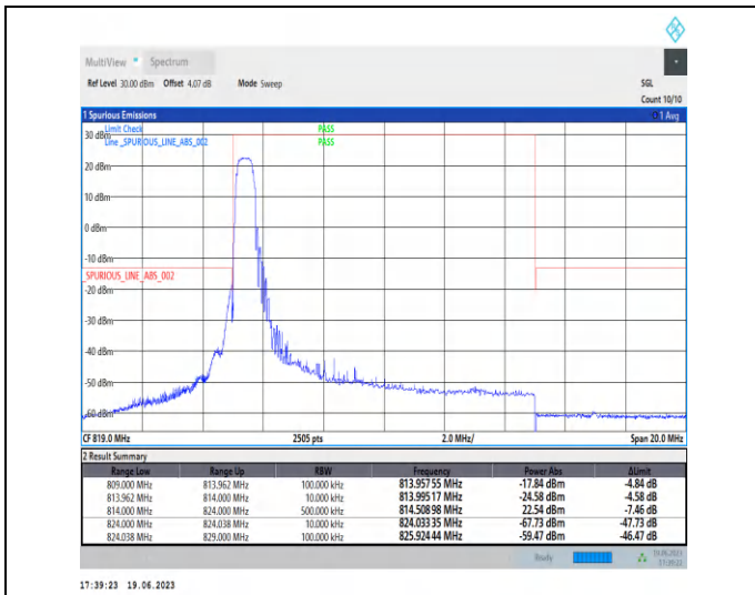
1-N26-814-824-PC3-15-10-L-1-DFT-PI2BPSK-Edge_1 RB_Left-1@0-Ant0-1--PASS-see graph
