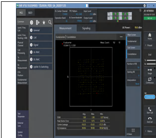
1-N26-814-824-PC3-15-10-M-5-DFT-256QAM-Outer_Full-50@0-Ant0-see graph-PASS
