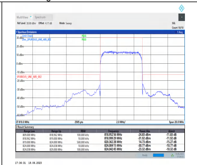
1-N26-814-824-PC3-15-5-H-3-DFT-PI2BPSK-Outer_Full-25@0-Ant0-1--PASS-see graph
