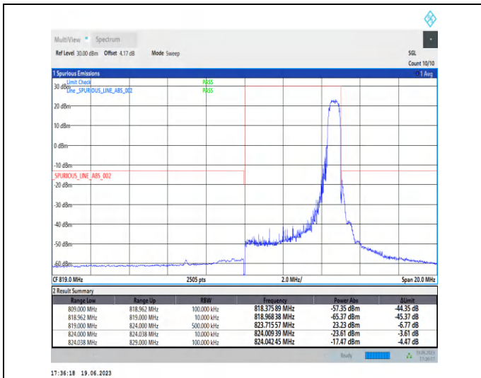
1-N26-814-824-PC3-15-5-H-2-DFT-PI2BPSK-Edge_1 RB_Right-1@24-Ant0-1--PASS-see graph
