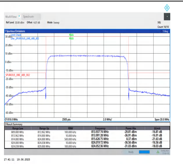
1-N26-814-824-PC3-15-10-H-6-CP-QPSK-Outer_Full-52@0-Ant0-1--PASS-see graph
