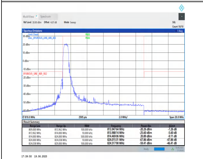
1-N26-814-824-PC3-15-10-L-4-CP-QPSK-Edge_1RB_Left-1@0-Ant0-1--PASS-see graph
