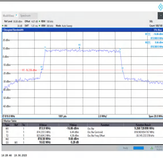
1-N26-814-824-PC3-15-10-M-6-CP-QPSK-Outer_Ful I-52@0-Ant0-9.269-10.020-≤10-PASS
