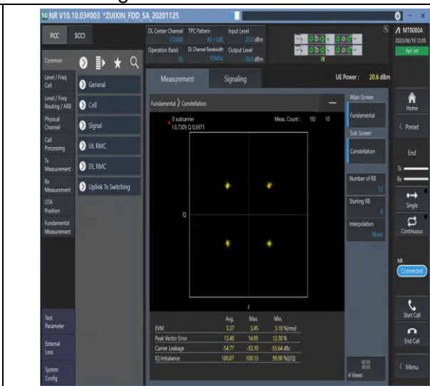
1-N26-814-824-PC3-15-10-M-6-CP-QPSK-Outer_Full-52@0-Ant0-see graph-PASS
