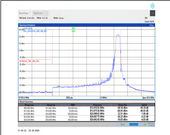
1-N26-814-824-PC3-15-10-H-2-DFT-PI2BPSK-Edge_1 RB_Right-1@51-Ant0-1--PASS-see graph
