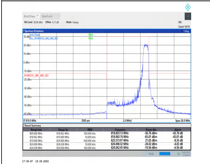
1-N26-814-824-PC3-15-5-H-5-CP-QPSK-Edge_1RB_Right-1@24-Ant0-1--PASS-see graph
