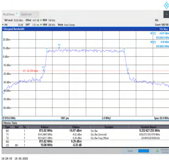
1-N26-814-824-PC3-15-10-M-8-CP-64QAM-Outer_Full I-52@0-Ant0-9.253-10.080-≤10-PASS
