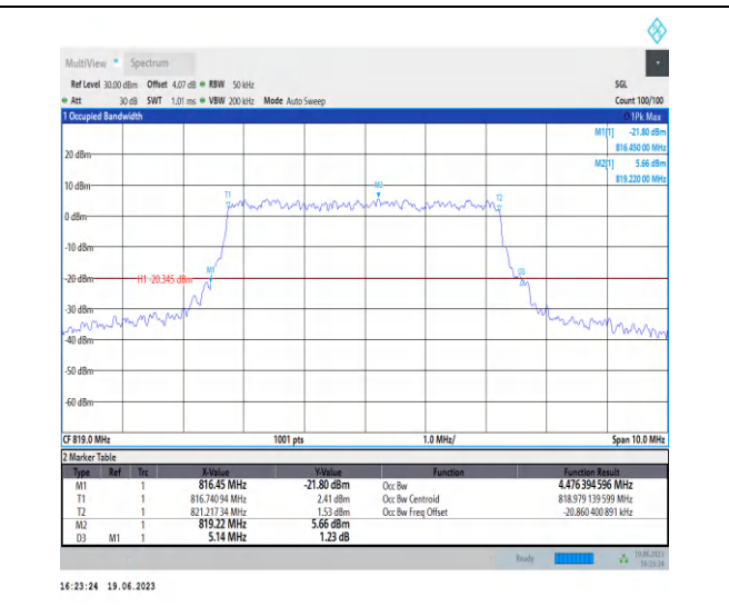
1-N26-814-824-PC3-15-5-M-9-CP-256QAM-Outer_F ull-25@0-Ant0-4.476-5.140-<math>\leq</math>5-PASS
