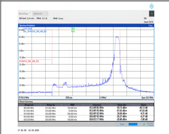
1-N26-814-824-PC3-15-10-H-5-CP-QPSK-Edge_1RB_Right-1@51-Ant0-1--PASS-see graph
