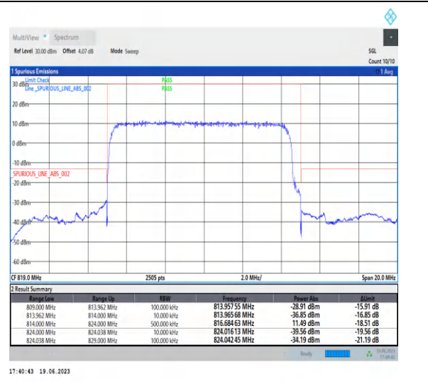
1-N26-814-824-PC3-15-10-H-3-DFT-PI2BPSK-Out_er_Full-50@0-Ant0-1--PASS-see graph
