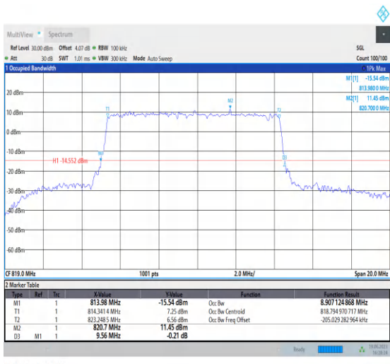
1-N26-814-824-PC3-15-10-M-4-DFT-64QAM-Outer_ Full-50@0-Ant0-8.907-9.560-≤10-PASS
