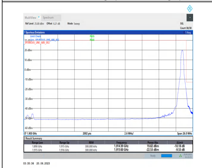
1-N25-PC3-15-25-H-5-CP-QPSK-Edge_1RB_Right-1@132-Ant3-1-seegraph-PASS-see graph
