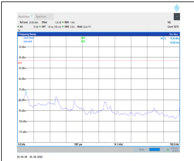
1-N25-PC3-15-40-H-1-DFT-PI2BPSK-Inner_1RB_L eft-1 @ 1-0.009-0.15-Ant3-0.02--74.36--43-PASS
