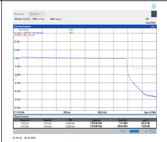
1-N25-PC3-15-5-H-6-CP-QPSK-Outer_Full-25@0-Ant3-1-seegraph-PASS-see graph
