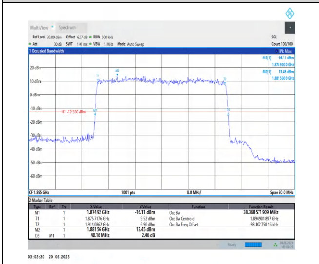
1-N25-PC3-15-40-H-3-DFT-16QAM-Outer_Full-216 @0-Ant3-38.369-40.160-<40-PASS
