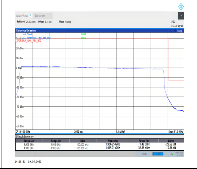
1-N25-PC3-15-10-H-6-CP-QPSK-Outer_Full-52@0-Ant3-1-seegraph-PASS-see graph
