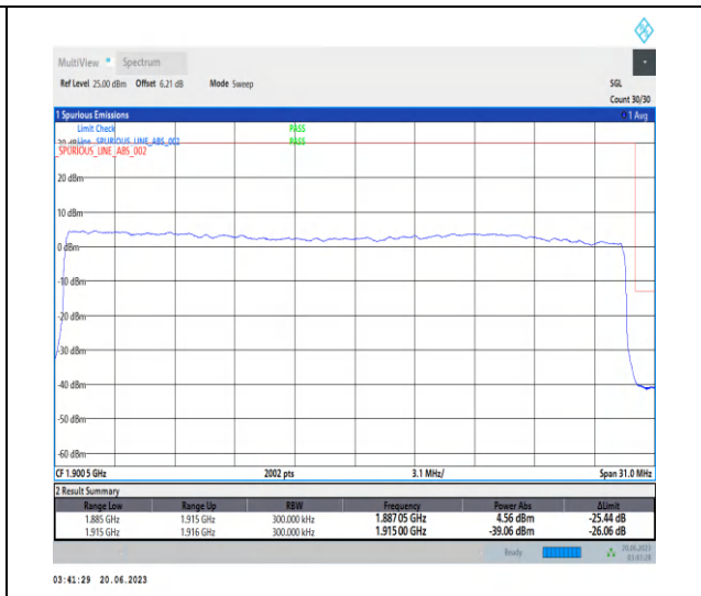
1-N25-PC3-15-30-H-3-DFT-PI2BPSK-Outer_Full-160@0-Ant3-1-seegraph-PASS-see graph
