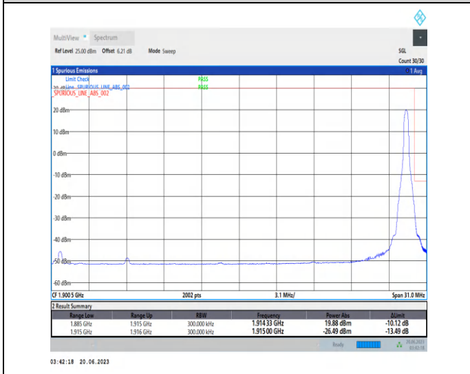
1-N25-PC3-15-30-H-5-CP-QPSK-Edge_1RB_Right-1@159-Ant3-1-seegraph-PASS-see graph
