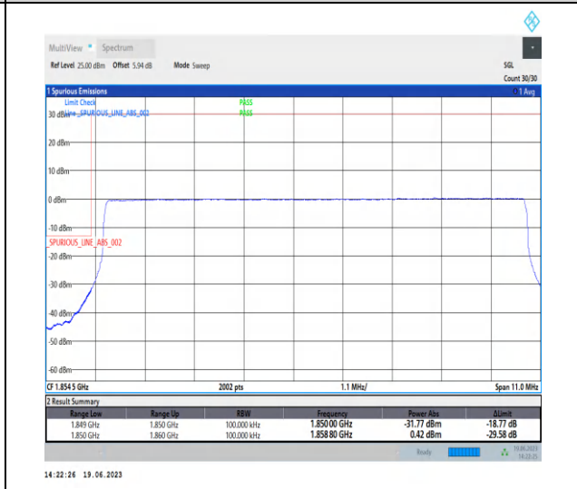
1-N25-PC3-15-10-L-6-CP-QPSK-Outer_Full-52@0-Ant3-1-seegraph-PASS-see graph
