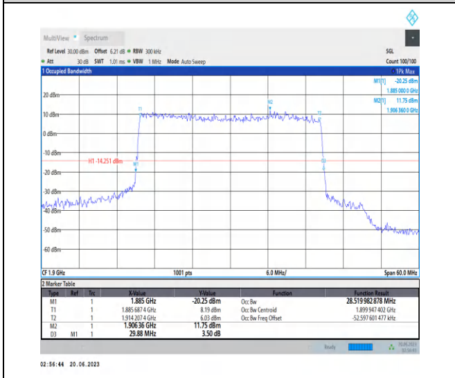
1-N25-PC3-15-30-H-6-CP-QPSK-Outer_Full-160@0 -Ant3-28.52-29.880-<30-PASS
