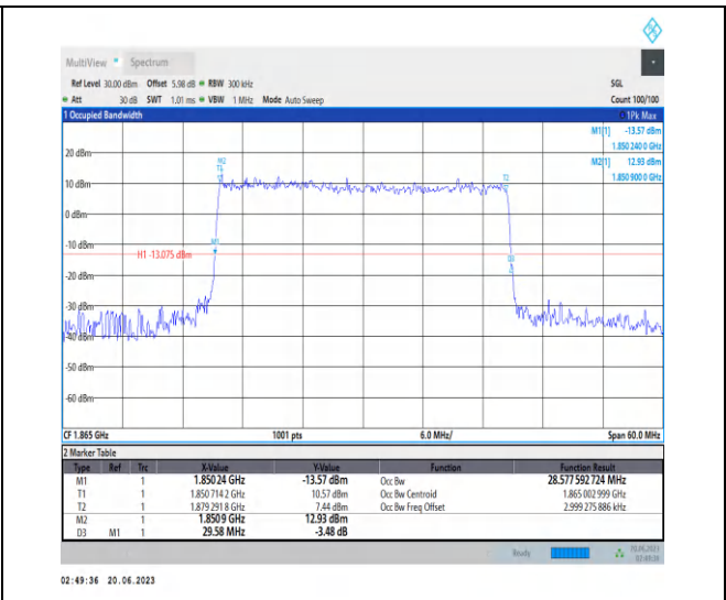
1-N25-PC3-15-30-L-3-DFT-16QAM-Outter_Full-160 @0-Ant3-28.578-29.580-<30-PASS
