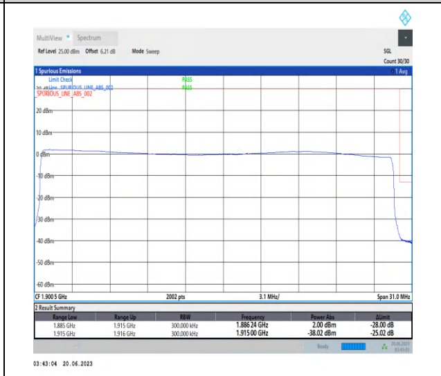
1-N25-PC3-15-30-H-6-CP-QPSK-Outer_Full-160@0-Ant3-1-seegraph-PASS-see graph
