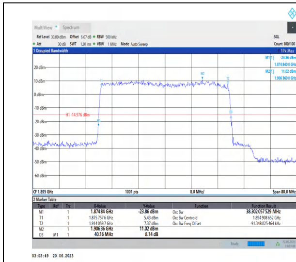
1-N25-PC3-15-40-H-5-DFT-256QAM-Outer_Full-216 @0-Ant3-38.302-40.160-≤40-PASS
