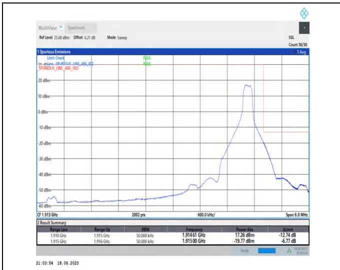
1-N25-PC3-15-5-H-2-DFT-PI2BPSK-Edge_1RB_Right -1@24-Ant3-1-seegraph-PASS-see graph
