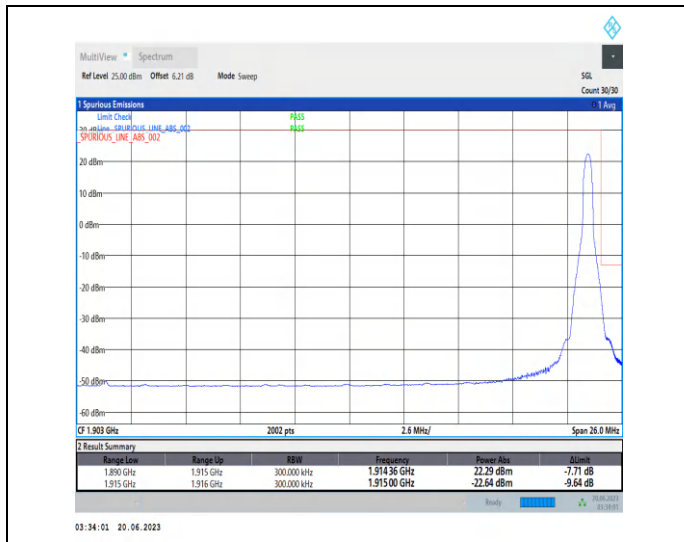
1-N25-PC3-15-25-H-2-DFT-PI2BPSK-Edge_1RB_Right-t-1@132-Ant3-1-seegraph-PASS-see graph
