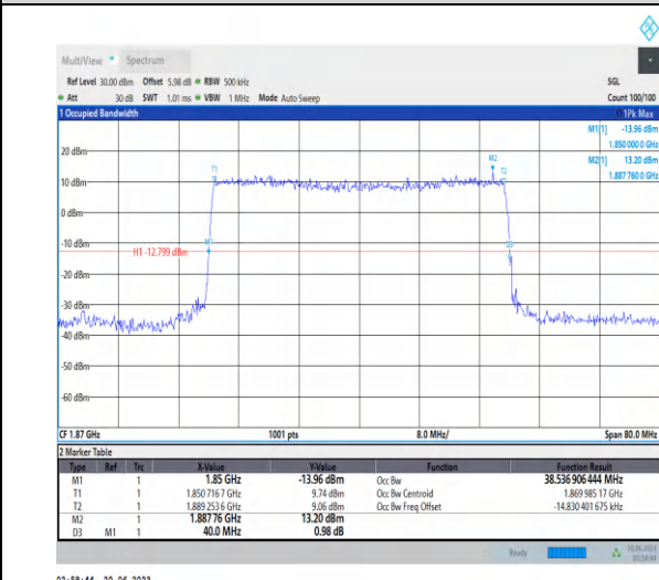
1-N25-PC3-15-40-L-6-CP-QPSK-Outer_Full-216@0 -Ant3-38.537-40.000-<40-PASS
