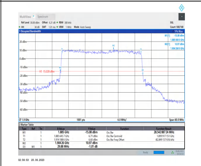
1-N25-PC3-15-30-H-7-CP-16QAM-Outer_Full-160@0 0-Ant3-28.543-29.880-<30-PASS
