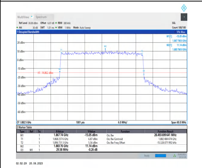
1-N25-PC3-15-30-M-8-CP-64QAM-Outer_Full-160 @0-Ant3-28.494-29.580-≤30-PASS
