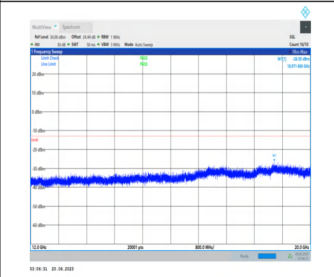
1-N25-PC3-15-40-M-1-DFT-PI2BPSK-Inner_1RB_L ef t-1 @ 1-12000-20000-Ant3-18971.60--26.55--13-PASS
