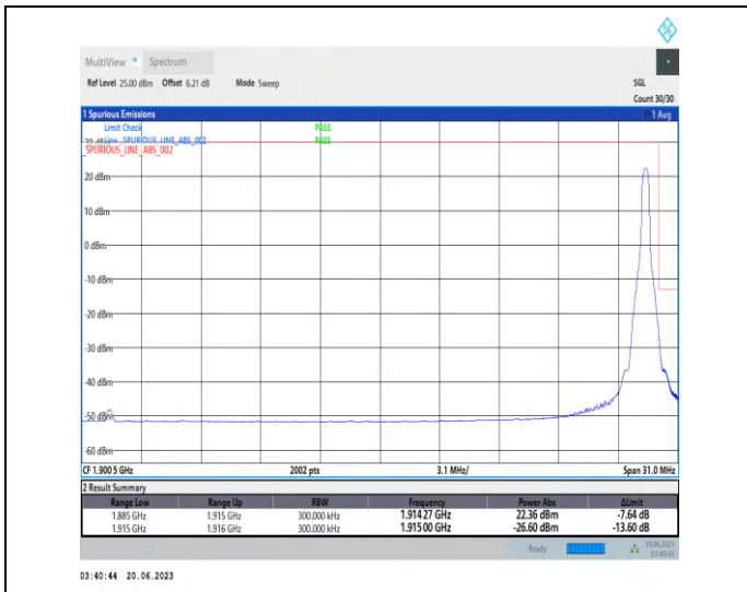
1-N25-PC3-15-30-H-2-DFT-PI2BPSK-Edge_1RB_Right-t-1@159-Ant3-1-seegraph-PASS-see graph
