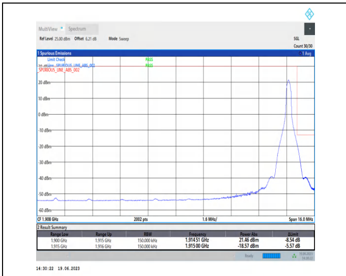
1-N25-PC3-15-15-H-2-DFT-PI2BPSK-Edge_1RB_Right-t-1@78-Ant3-1-seegraph-PASS-see graph
