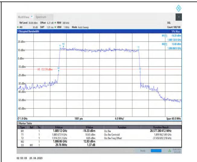
1-N25-PC3-15-30-H-1-DFT-QPSK-Outer_Full-160@ 0-Ant3-28.577-29.760-<30-PASS
