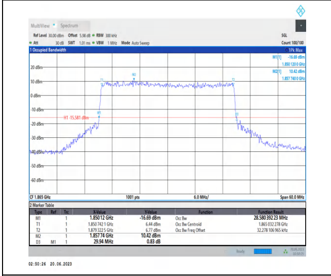
1-N25-PC3-15-30-L-8-CP-64QAM-Outer_Full-160@0 -Ant3-28.58-29.940-≤30-PASS
