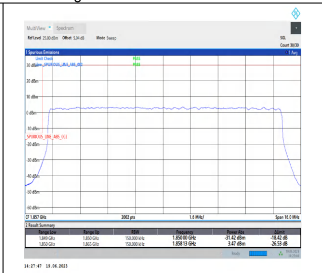
1-N25-PC3-15-15-L-3-DFT-PI2BPSK-Outer_Full-75@0-Ant3-1-seegraph-PASS-see graph
