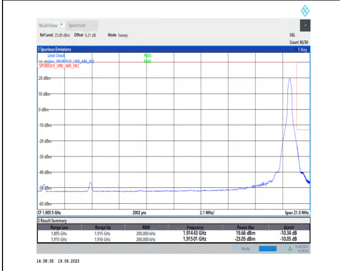
1-N25-PC3-15-20-H-5-CP-QPSK-Edge_1RB_Right-1@105-Ant3-1-seegraph-PASS-see graph
