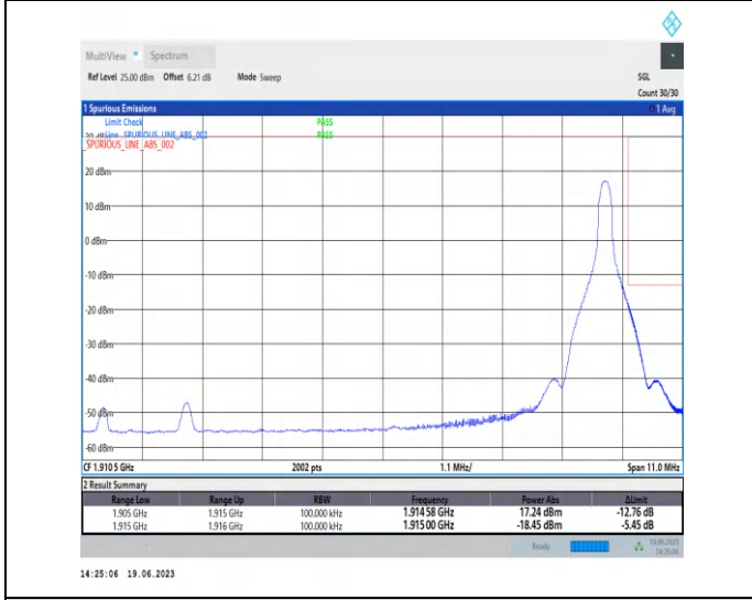
1-N25-PC3-15-10-H-5-CP-QPSK-Edge_1RB_Right-1@51-Ant3-1-seegraph-PASS-see graph
