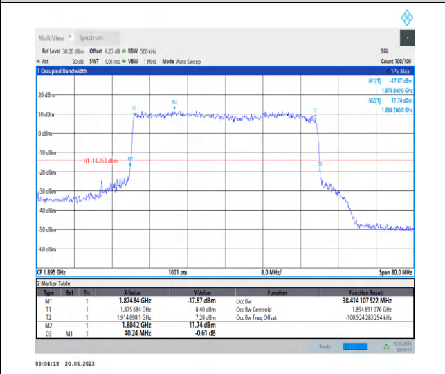
1-N25-PC3-15-40-H-8-CP-64QAM-Outer_Full-216 @0-Ant3-38.414-40.240-≤40-PASS
