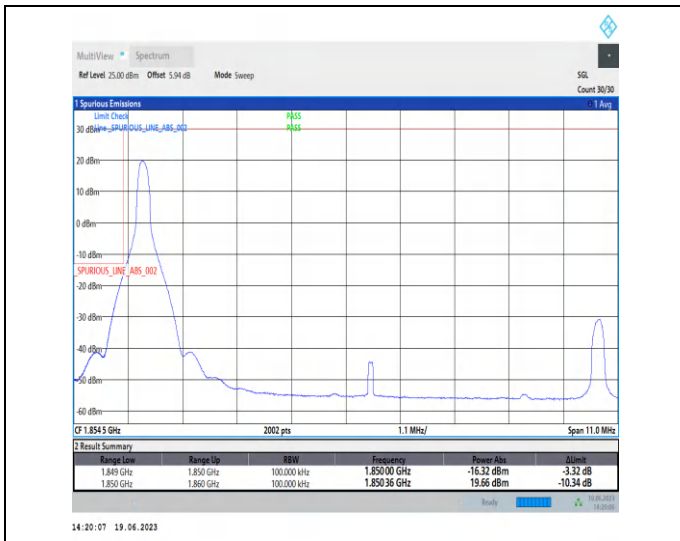
1-N25-PC3-15-10-L-1-DFT-PI2BPSK-Edge_1RB_Left-1@0-Ant3-1-seegraph-PASS-see graph
