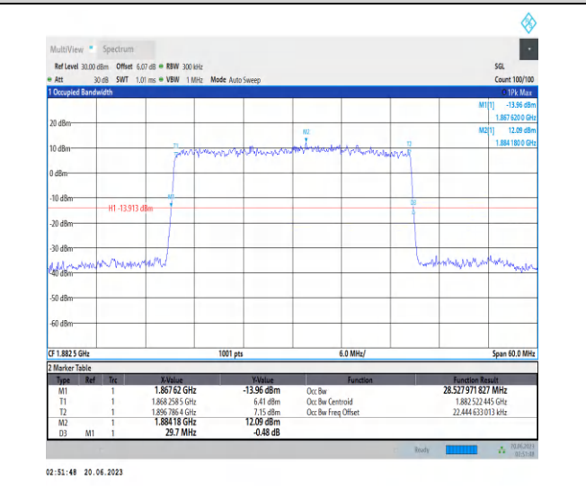
1-N25-PC3-15-30-M-4-DFT-64QAM-Outer_Full-160 @0-Ant3-28.528-29.700-≤30-PASS
