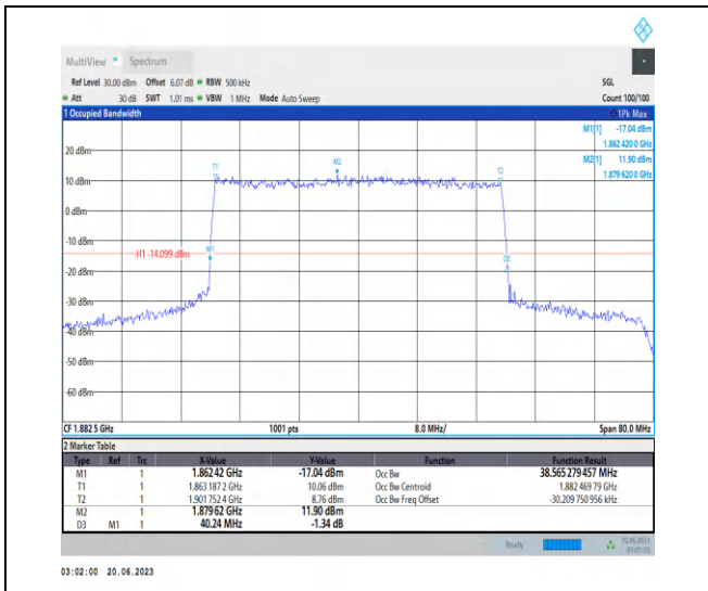
1-N25-PC3-15-40-M-6-CP-QPSK-Outer_Full-216@ 0-Ant3-38.565-40.240-≤40-PASS
