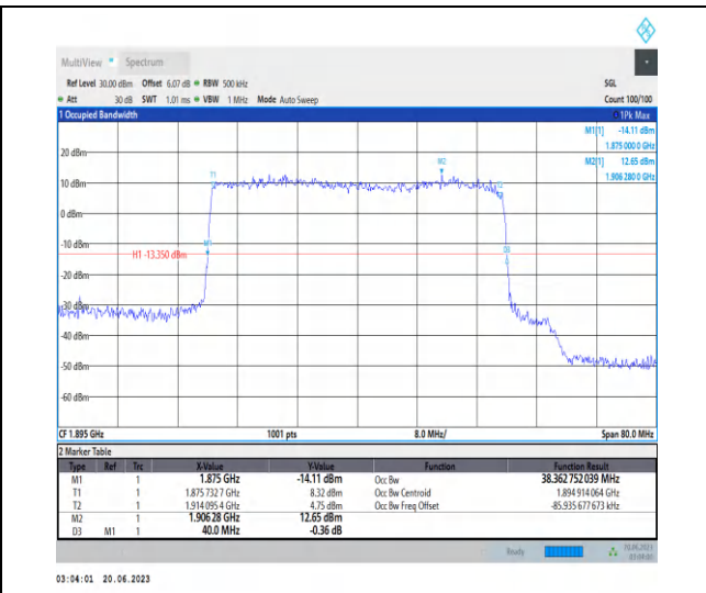
1-N25-PC3-15-40-H-6-CP-QPSK-Outer_Full-216@ 0-Ant3-38.363-40.000-≤40-PASS
