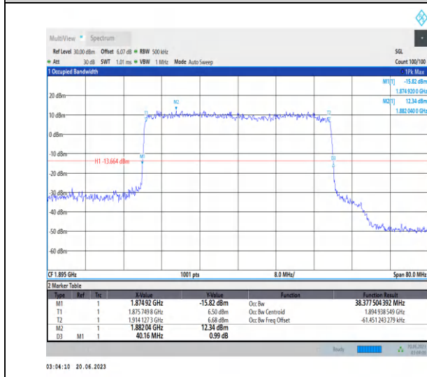
1-N25-PC3-15-40-H-7-CP-16QAM-Outer_Full-216@0 -Ant3-38.378-40.160-≤40-PASS
