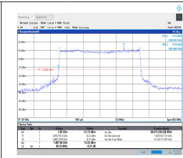
1-N25-PC3-15-40-L-8-CP-64QAM-Outer_Full-216@ 0-Ant3-38.613-40.160-≤40-PASS
