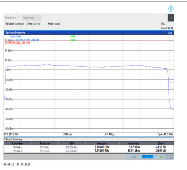
1-N25-PC3-15-40-H-3-DFT-PI2BPSK-Outer_Full-216@0-Ant3-1-seegraph-PASS-see graph
