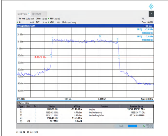
1-N25-PC3-15-30-H-2-DFT-PI2BPSK-Outer_Full-160 @0-Ant3-28.549-29.700-<30-PASS
