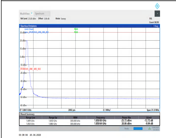
1-N25-PC3-15-30-L-4-CP-QPSK-Edge_1RB_Left-1@0-Ant3-1-seegrph-PASS-see graph
