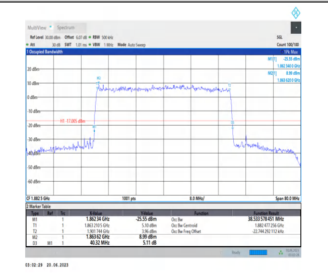
1-N25-PC3-15-40-M-9-CP-256QAM-Outer_Full-216 @0-Ant3-38.534-40.320-≤40-PASS
