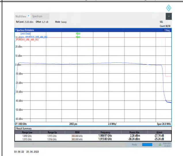
1-N25-PC3-15-25-H-6-CP-QPSK-Outer_Full-133@0-Ant3-1-seegraph-PASS-see graph
