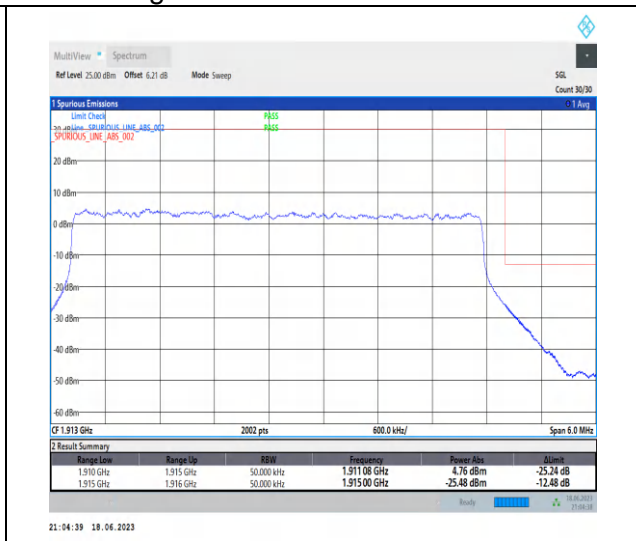
1-N25-PC3-15-5-H-3-DFT-PI2BPSK-Outer_Full-25 @0-Ant3-1-seegraph-PASS-see graph
