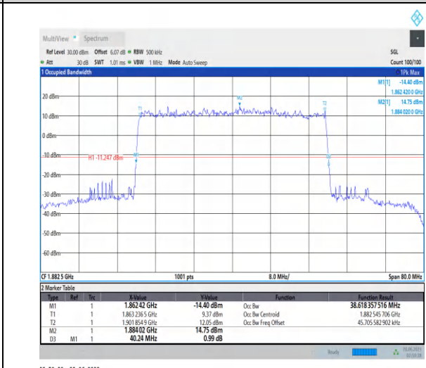
1-N25-PC3-15-40-M-1-DFT-QPSK-Outer_Full-216@ 0-Ant3-38.618-40.240-≤40-PASS
