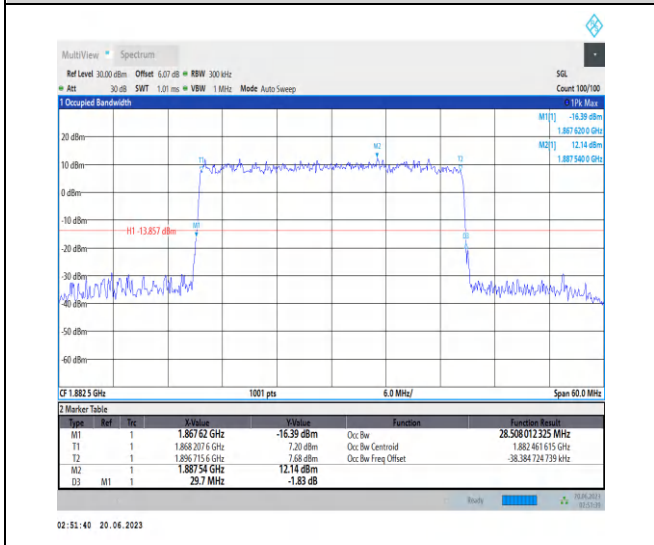
1-N25-PC3-15-30-M-3-DFT-16QAM-Outer_Full-160 @0-Ant3-28.508-29.700-≤30-PASS
