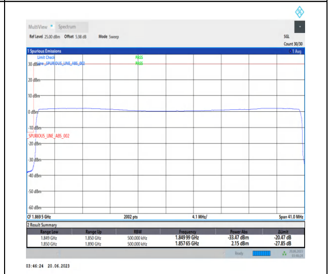
1-N25-PC3-15-40-L-6-CP-QPSK-Outer_Full-216@0-Ant3-1-seegrph-PASS-see graph
