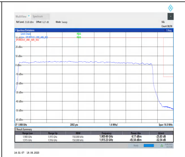
1-N25-PC3-15-15-H-3-DFT-PI2BPSK-Outer_Full-75@0-Ant3-1-seegraph-PASS-see graph
