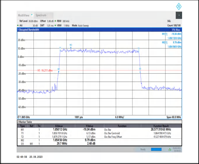
1-N25-PC3-15-30-L-5-DFT-256QAM-Outter_Full-160 @0-Ant3-28.577-29.700-<30-PASS
