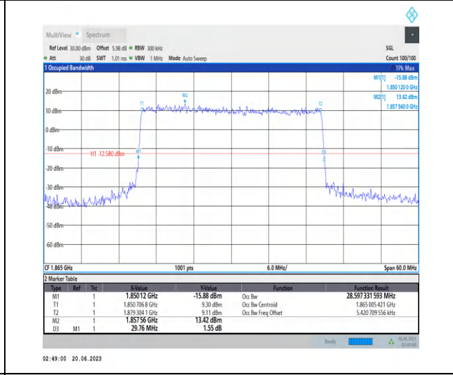
1-N25-PC3-15-30-L-1-DFT-QPSK-Outer_Full-160@ 0-Ant3-28.597-29.760-<=30-PASS
