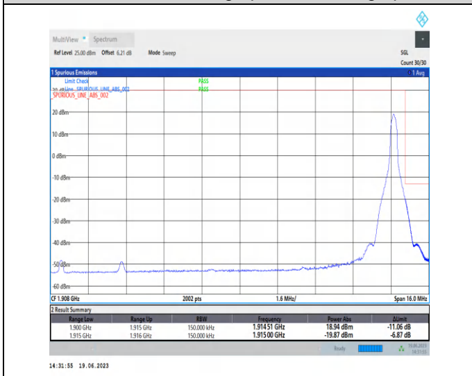
1-N25-PC3-15-15-H-5-CP-QPSK-Edge_1RB_Right-1@78-Ant3-1-seegraph-PASS-see graph
