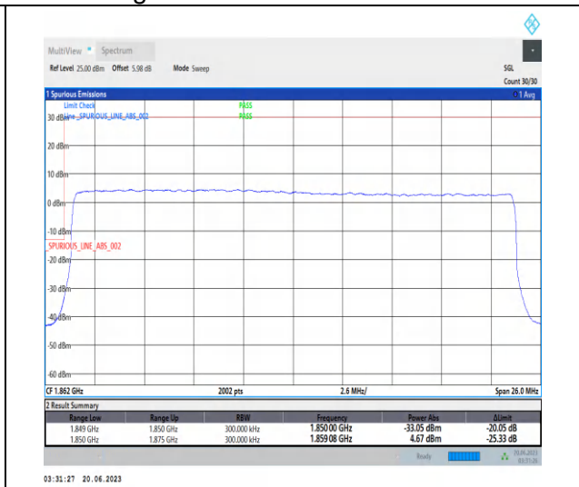
1-N25-PC3-15-25-L-3-DFT-PI2BPSK-Outer_Full-1 28@0-Ant3-1-seegrph-PASS-see graph
