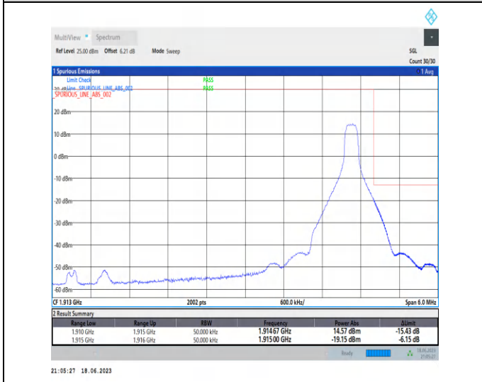
1-N25-PC3-15-5-H-5-CP-QPSK-Edge_1RB_Right-1@ 24-Ant3-1-seegraph-PASS-see graph
