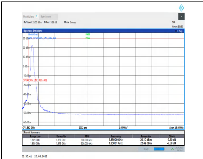
1-N25-PC3-15-25-L-1-DFT-PI2BPSK-Edge_1RB_Left-1@0-Ant3-1-seegrph-PASS-see graph
