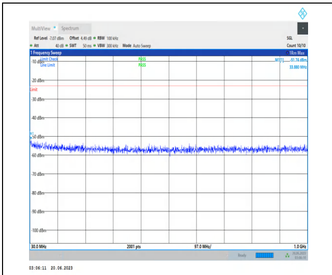
1-N25-PC3-15-40-M-1-DFT-PI2BPSK-Inner_1RB_L eft-1 @ 1-30-1000-Ant3-33.88--51.74--23-PASS
