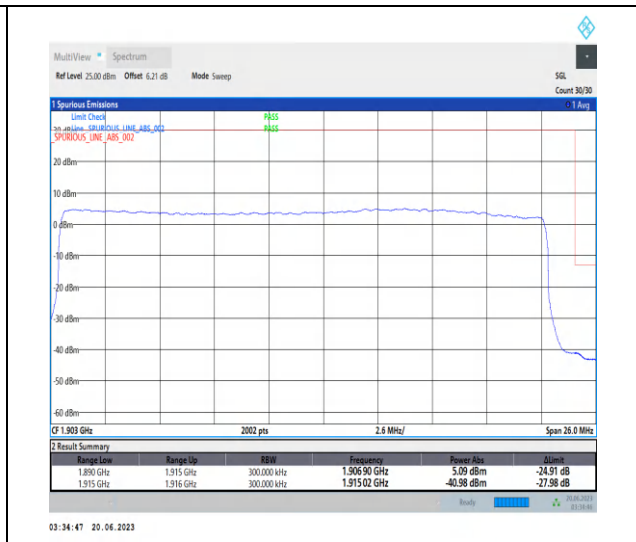
1-N25-PC3-15-25-H-3-DFT-PI2BPSK-Outer_Full-128@0-Ant3-1-seegraph-PASS-see graph
