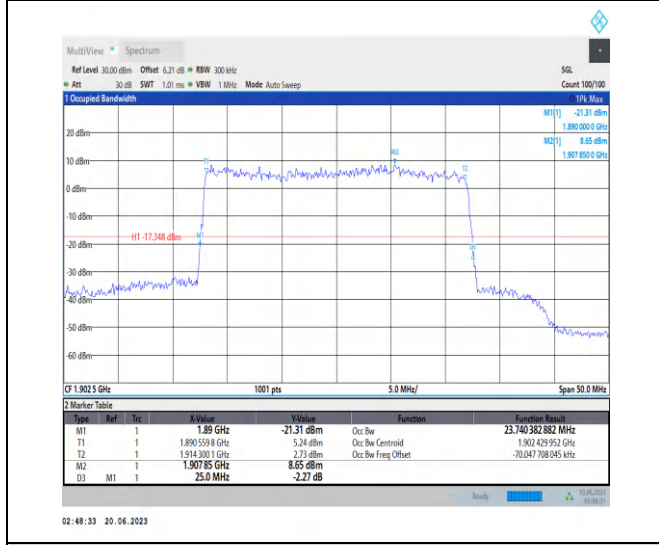
1-N25-PC3-15-25-H-9-CP-256QAM-Outer_Full-133 @0-Ant3-23.74-25.000-<=25-PASS
