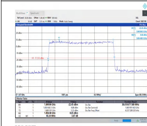
1-N25-PC3-15-40-L-9-CP-256QAM-Outer_Full-216 @0-Ant3-38.619-40.240-≤40-PASS
