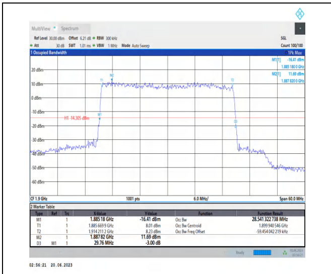
1-N25-PC3-15-30-H-4-DFT-64QAM-Outer_Full-160 @0-Ant3-28.541-29.760-<30-PASS
