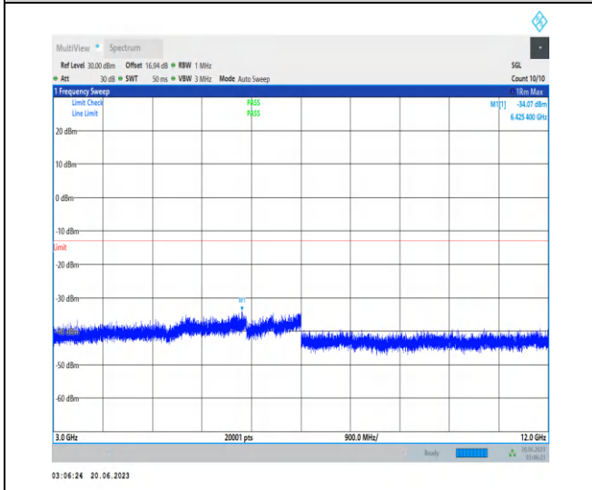
1-N25-PC3-15-40-M-1-DFT-PI2BPSK-Inner_1RB_L eft-1 @ 1-3000-12000-Ant3-6425.40--34.07--13-PAS S
