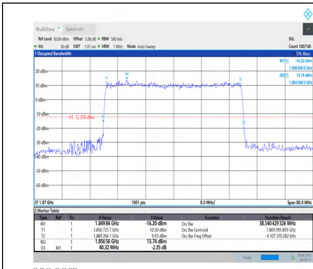
1-N25-PC3-15-40-L-3-DFT-16QAM-Outer_Full-216@ 0-Ant3-38.54-40.320-<40-PASS
