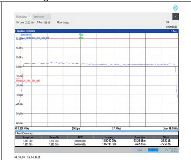
1-N25-PC3-15-30-L-3-DFT-PI2BPSK-Outer_Full-160@0-Ant3-1-seegrph-PASS-see graph
