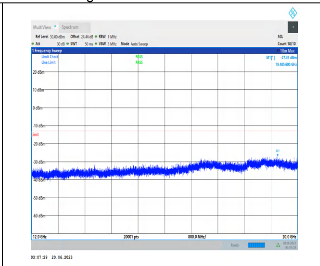
1-N25-PC3-15-40-H-1-DFT-PI2BPSK-Inner_1RB_L ef t-1 @ 1-12000-20000-Ant3-19405.60--27.31--13-PASS
