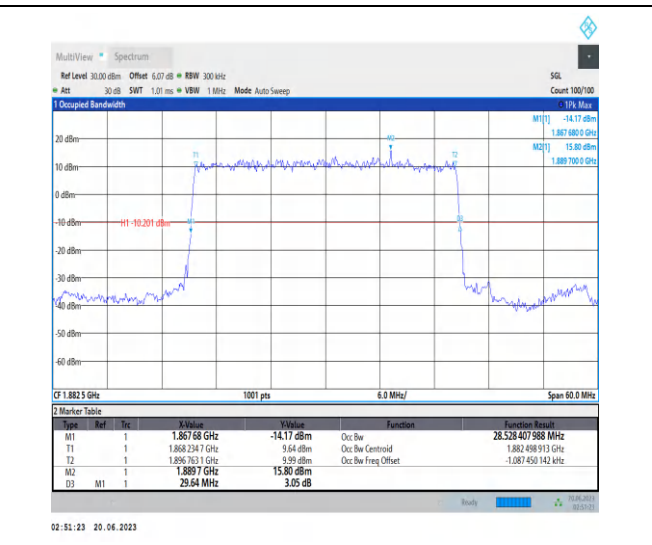
1-N25-PC3-15-30-M-2-DFT-PI2BPSK-Outer_Full-160 @0-Ant3-28.528-29.640-≤30-PASS
