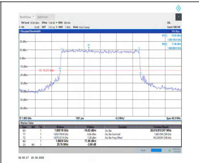
1-N25-PC3-15-30-L-7-CP-16QAM-Outer_Full-160@0 -Ant3-28.617-29.760-≤30-PASS
