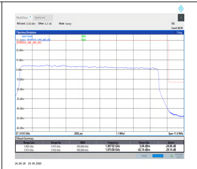
1-N25-PC3-15-10-H-3-DFT-PI2BPSK-Outer_Full-50@0-Ant3-1-seegraph-PASS-see graph
