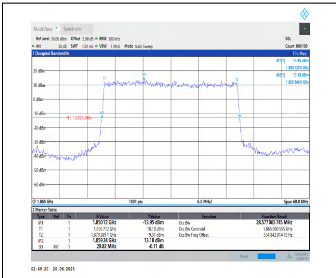
1-N25-PC3-15-30-L-2-DFT-PI2BPSK-Outter_Full-160 @0-Ant3-28.577-29.820-<30-PASS
