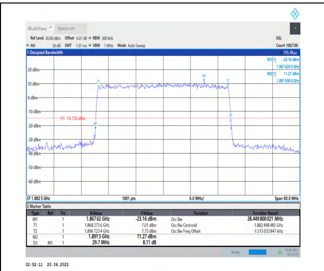
1-N25-PC3-15-30-M-6-CP-QPSK-Outer_Full-160 @0-Ant3-28.45-29.700-≤30-PASS
