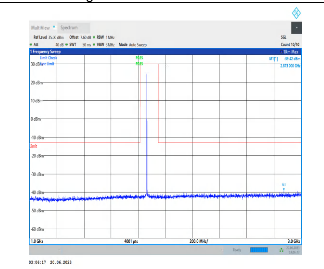
1-N25-PC3-15-40-M-1-DFT-PI2BPSK-Inner_1RB_L ef t-1 @ 1-1000-3000-Ant3-2873.00--39.42--13-PASS
