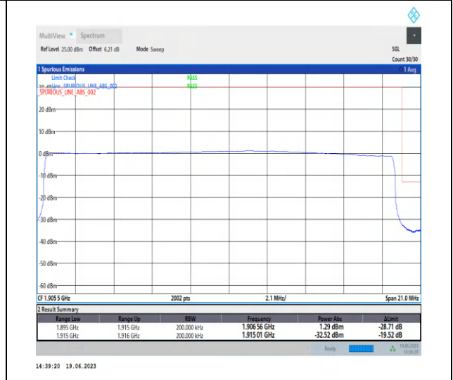
1-N25-PC3-15-20-H-6-CP-QPSK-Outer_Full-106@0-Ant3-1-seegraph-PASS-see graph
