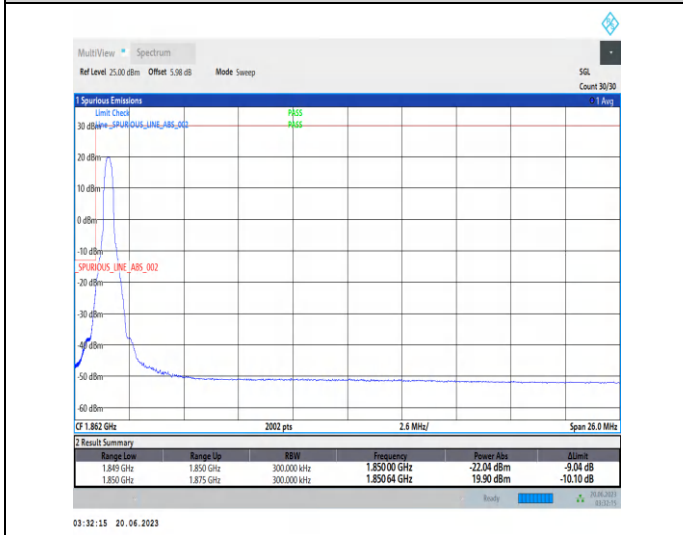
1-N25-PC3-15-25-L-4-CP-QPSK-Edge_1RB_Left-1@0-Ant3-1-seegrph-PASS-see graph
