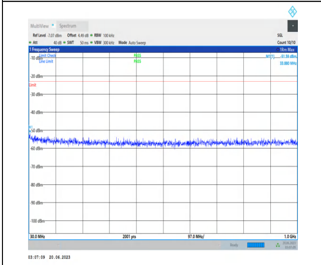
1-N25-PC3-15-40-H-1-DFT-PI2BPSK-Inner_1RB_L eft-1 @ 1-30-1000-Ant3-33.88--51.59--23-PASS
