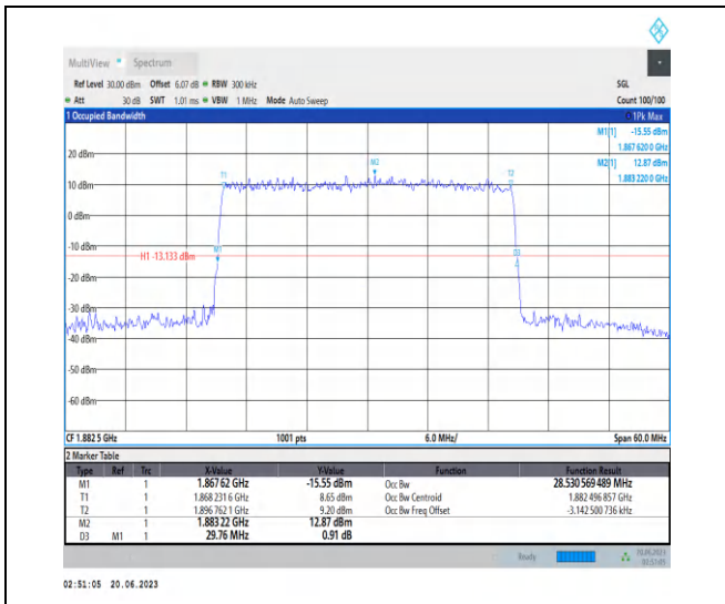
1-N25-PC3-15-30-M-1-DFT-QPSK-Outer_Full-160@ 0-Ant3-28.531-29.760-≤30-PASS
