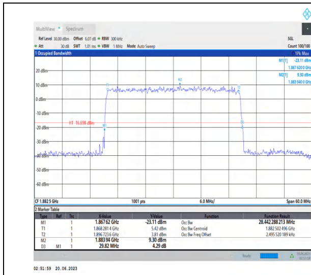
1-N25-PC3-15-30-M-5-DFT-256QAM-Outer_Full-160 @0-Ant3-28.442-29.820-≤30-PASS
