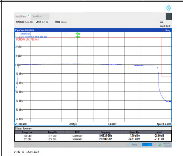
1-N25-PC3-15-15-H-6-CP-QPSK-Outer_Full-79@0-Ant3-1-seegraph-PASS-see graph
