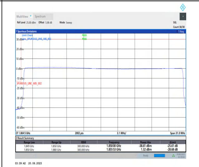
1-N25-PC3-15-30-L-6-CP-QPSK-Outer_Full-160@0-Ant3-1-seegrph-PASS-see graph
