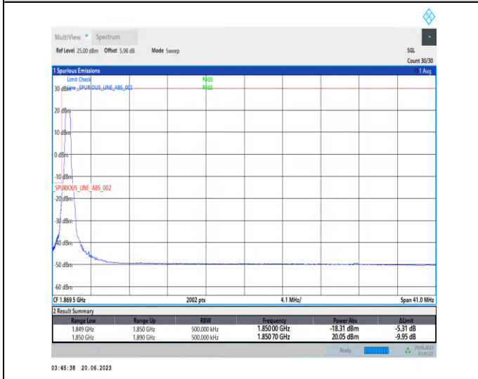
1-N25-PC3-15-40-L-4-CP-QPSK-Edge_1RB_Left-1@0-Ant3-1-seegrph-PASS-see graph
