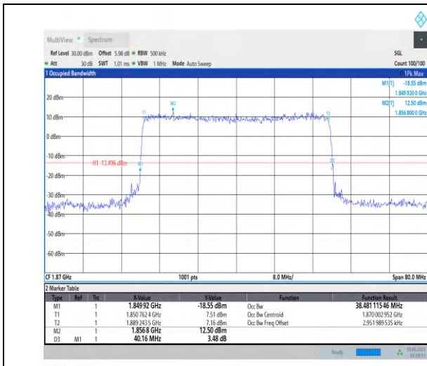
1-N25-PC3-15-40-L-7-CP-16QAM-Outer_Full-216@ 0-Ant3-38.481-40.160-≤40-PASS
