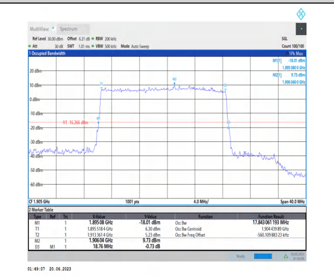
1-N25-PC3-15-20-H-5-DFT-256QAM-Outer_Full-100 @0-Ant3-17.843-18.760-<20-PASS
