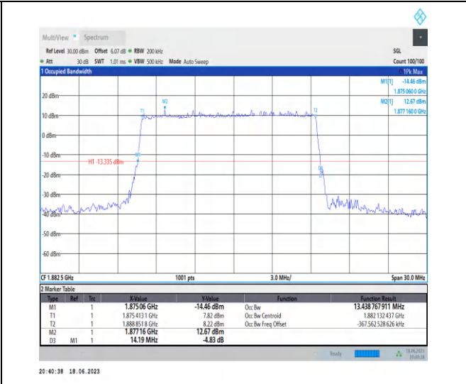
1-N25-PC3-15-15-M-3-DFT-16QAM-Outer_Full-75@ 0-Ant3-13.439-14.190≤15-PASS
