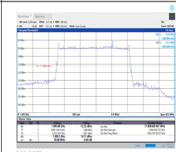
1-N25-PC3-15-20-H-1-DFT-QPSK-Outer_Full-100@ -0-Ant3-17.839-18.680-<20-PASS
