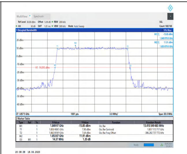
1-N25-PC3-15-15-L-4-DFT-64QAM-Outer_Full-75@0 0-Ant3-13.41-14.370-≤15-PASS
