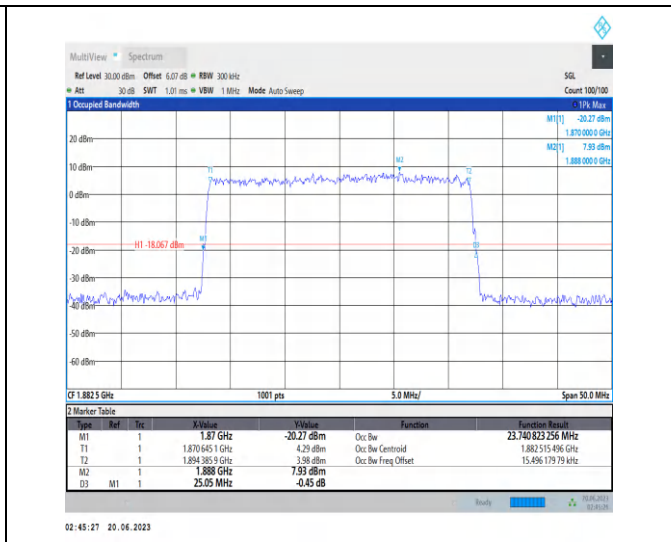
1-N25-PC3-15-25-M-9-CP-256QAM-Outer_Full-133 @0-Ant3-23.741-25.050-<25-PASS
