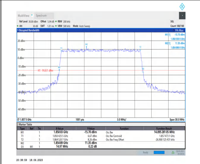
1-N25-PC3-15-15-L-6-CP-QPSK-Outer_Full-79@0 Ant3-14.095-14.970-≤15-PASS
