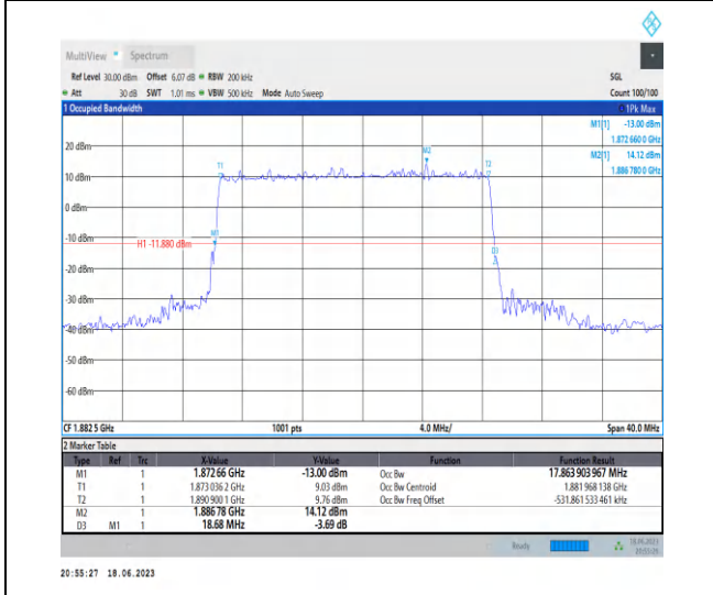
1-N25-PC3-15-20-M-1-DFT-QPSK-Outer_Full-100 @0-Ant3-17.864-18.680-≤20-PASS
