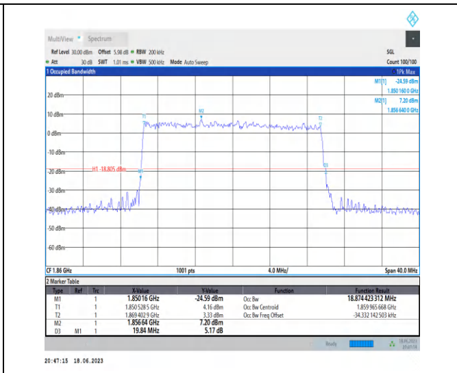
1-N25-PC3-15-20-L-9-CP-256QAM-Outer_Full-106 @0-Ant3-18.874-19.840-≤20-PASS
