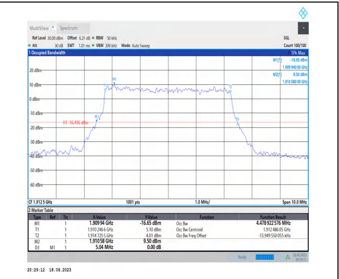
1-N25-PC3-15-5-H-8-CP-64QAM-Outer_Full-25@0- Ant3-4.479-5.040-≤5-PASS
