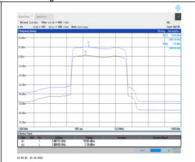
1-N25-PC3-15-40-H-2-CP-256QAM-Outer_Full-216 @0-Ant3-9.77-100%-0.00-9.77-PASS-≤13
