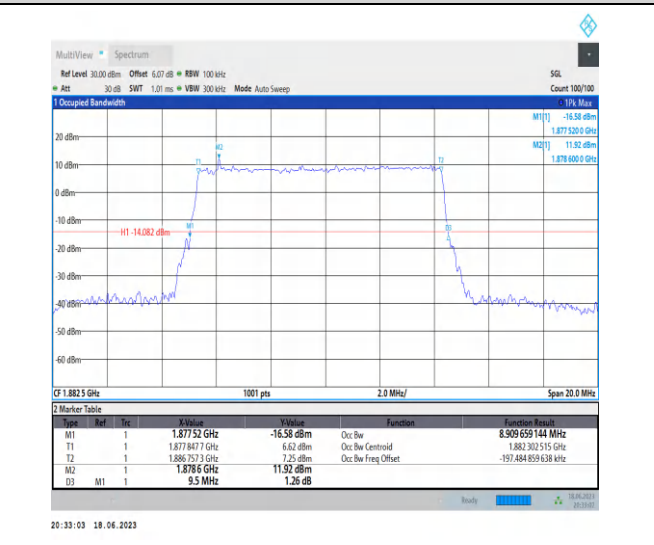
1-N25-PC3-15-10-M-4-DFT-64QAM-Outter_Full-50@0 @0-Ant3-8.91-9.500-≤10-PASS
