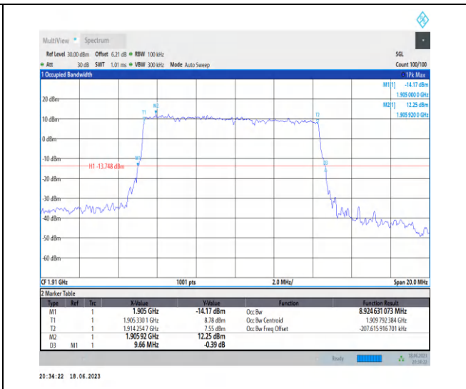
1-N25-PC3-15-10-H-1-DFT-QPSK-Outer_Full-50@0 -Ant3-8.925-9.660-≤10-PASS
