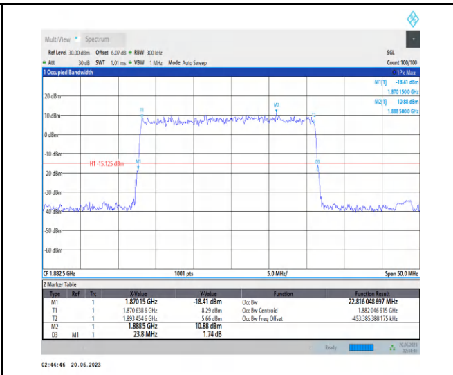
1-N25-PC3-15-25-M-5-DFT-256QAM-Outer_Full-128 @0-Ant3-22.816-23.800-<25-PASS
