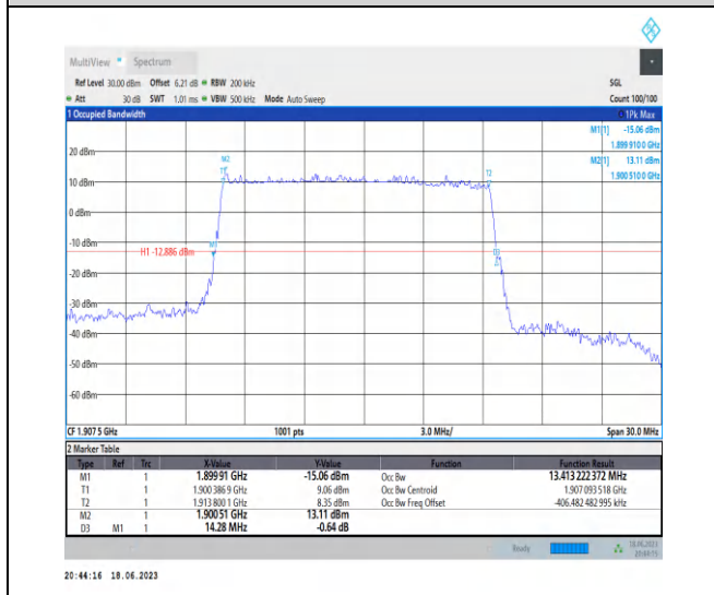
1-N25-PC3-15-15-H-3-DFT-16QAM-Outter_Full-75@ 0-Ant3-13.413-14.280-≤15-PASS
