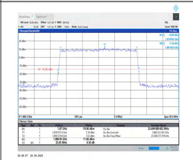
1-N25-PC3-15-25-M-7-CP-16QAM-Outer_Full-133@0 0-Ant3-23.695-25.050-<25-PASS
