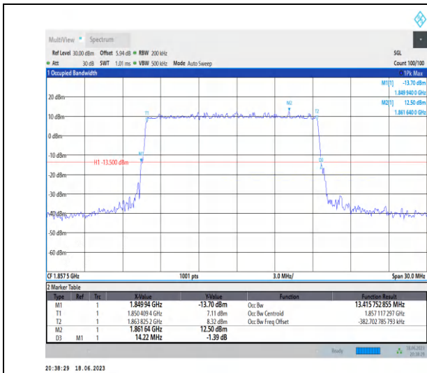
1-N25-PC3-15-15-L-3-DFT-16QAM-Outer_Full-75@0 -Ant3-13.416-14.220-≤15-PASS
