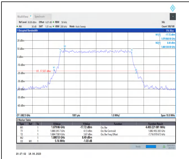
1-N25-PC3-15-5-M-8-CP-64QAM-Outer_Full-25@0 -Ant3-4.493-5.160-≤5-PASS
