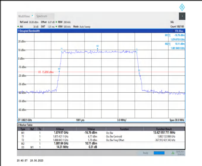
1-N25-PC3-15-15-M-5-DFT-256QAM-Outer_Full-75 @0-Ant3-13.422-14.310≤15-PASS
