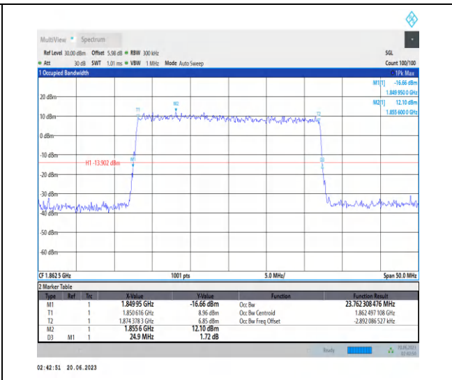
1-N25-PC3-15-25-L-6-CP-QPSK-Outer_Full-133@0 -Ant3-23.762-24.900-≤25-PASS
