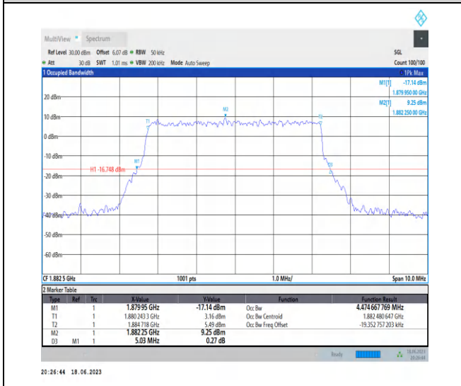
1-N25-PC3-15-5-M-6-CP-QPSK-Outer_Full-25@0-A nt3-4.475-5.030-≤5-PASS
