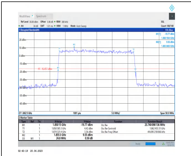
1-N25-PC3-15-25-L-9-CP-256QAM-Outer_Full-133@ 0-Ant3-23.74-24.800-<=25-PASS
