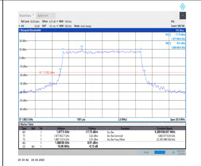
1-N25-PC3-15-10-M-8-CP-64QAM-Outer_Full-52 @0-Ant3-9.29-10.080-≤10-PASS
