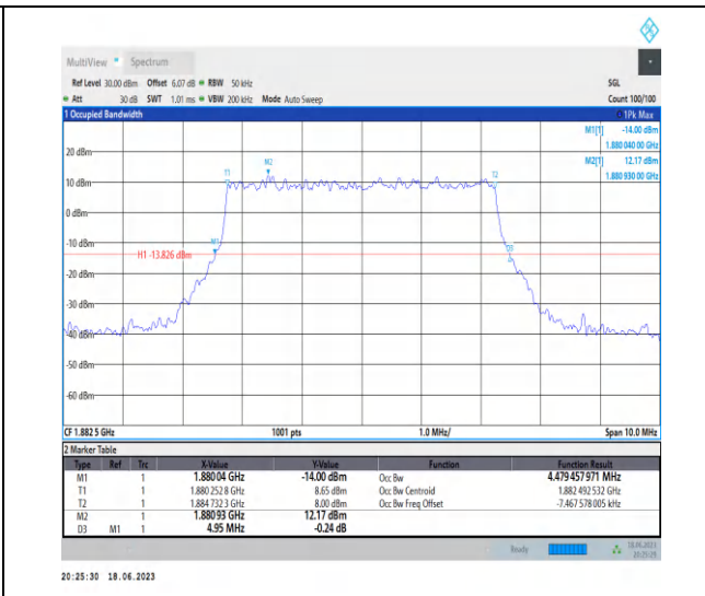
1-N25-PC3-15-5-M-1-DFT-QPSK-Outer_Full-25@0- Ant3-4.479-4.950-≤5-PASS
