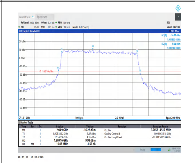
1-N25-PC3-15-10-H-7-CP-16QAM-Outer_Full-52@0- Ant3-9.266-10.080-≤10-PASS
