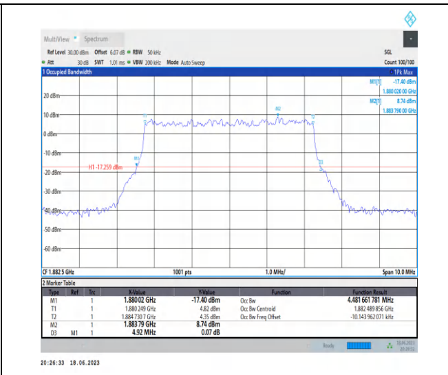
1-N25-PC3-15-5-M-5-DFT-256QAM-Outer_Full-25@ 0-Ant3-4.482-4.920-≤5-PASS
