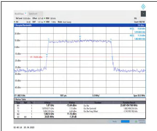
1-N25-PC3-15-25-M-8-CP-64QAM-Outer_Full-133 @0-Ant3-23.681-24.850-<25-PASS
