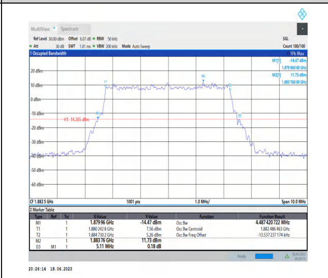
1-N25-PC3-15-5-M-3-DFT-16QAM-Outer_Full-25@0- -Ant3-4.487-5.110-≤5-PASS
