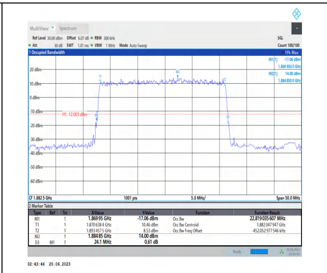
1-N25-PC3-15-25-M-1-DFT-QPSK-Outer_Full-128@ 0-Ant3-22.819-24.100-<=25-PASS
