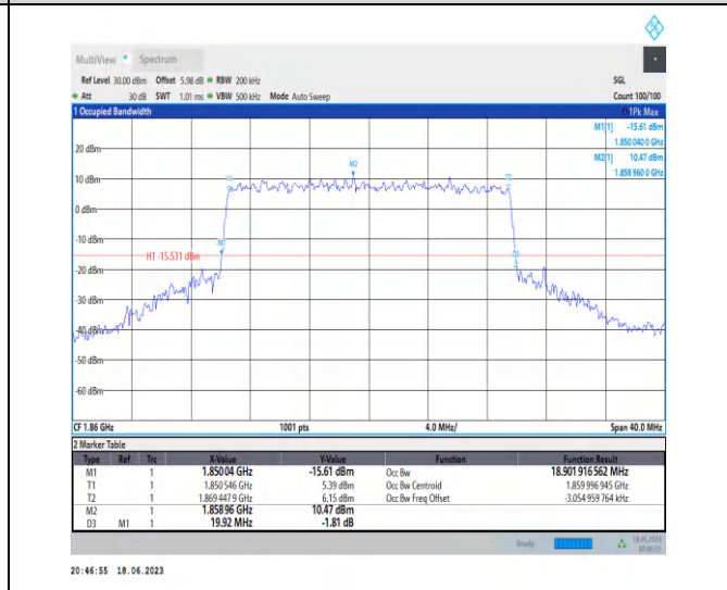
1-N25-PC3-15-20-L-7-CP-16QAM-Outer_Full-106@0 -Ant3-18.902-19.920-≤20-PASS
