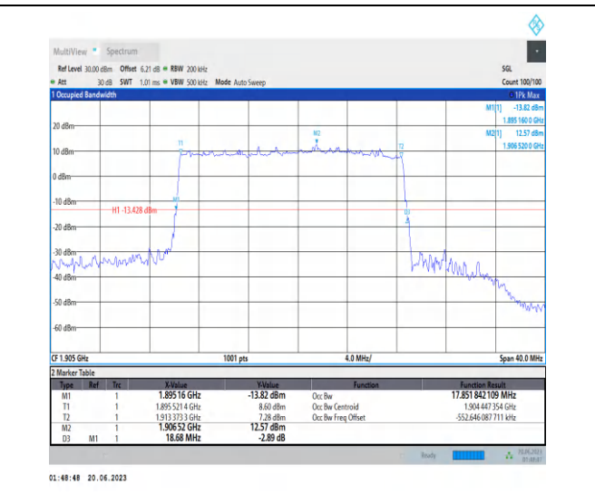
1-N25-PC3-15-20-H-3-DFT-16QAM-Outer_Full-100 @0-Ant3-17.852-18.680-<20-PASS
