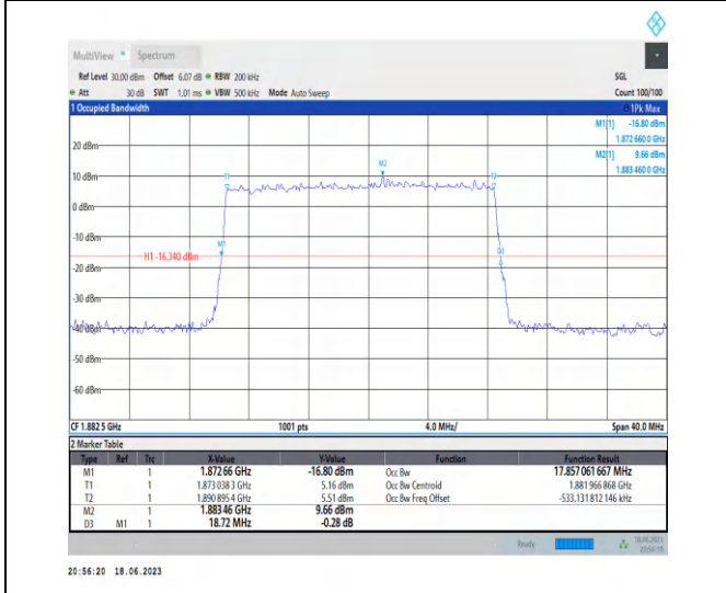
1-N25-PC3-15-20-M-5-DFT-256QAM-Outer_Full-100 @0-Ant3-17.857-18.720-<20-PASS
