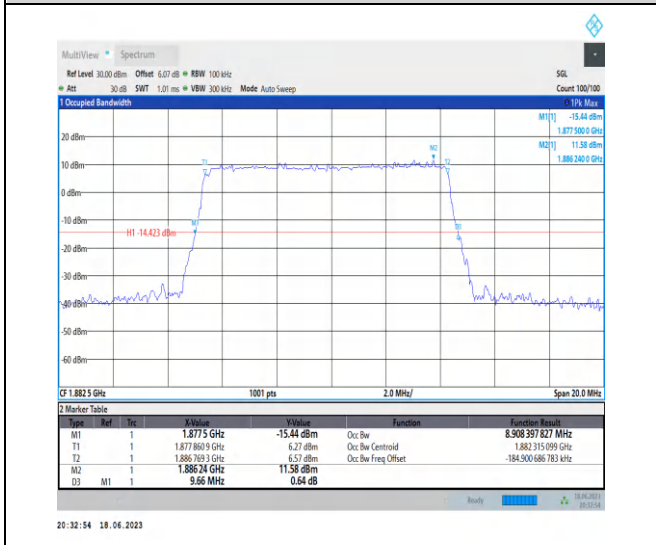
1-N25-PC3-15-10-M-3-DFT-16QAM-Outter_Full-50@0 @0-Ant3-8.908-9.660-≤10-PASS
