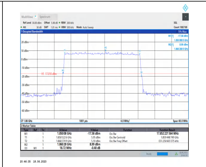
1-N25-PC3-15-20-L-5-DFT-256QAM-Outer_Full-100 @0-Ant3-17.852-18.720-≤20-PASS
