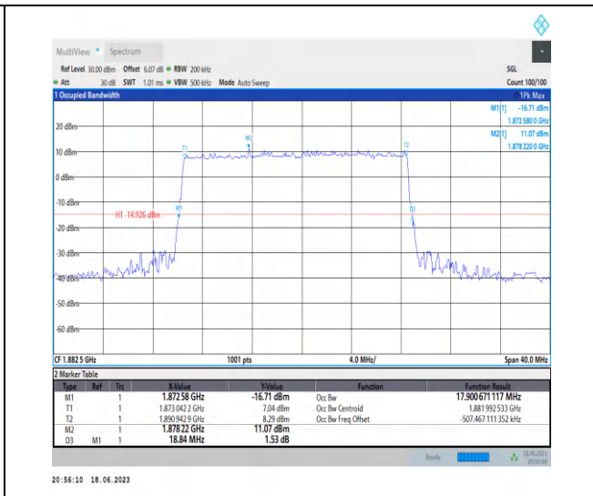
1-N25-PC3-15-20-M-4-DFT-64QAM-Outer_Full-100 @0-Ant3-17.901-18.840-<20-PASS
