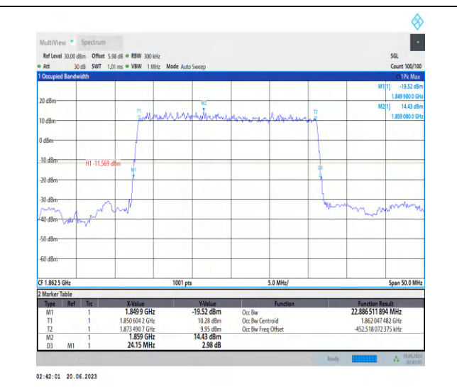
1-N25-PC3-15-25-L-2-DFT-PI2BPSK-Outer_Full-128@ 0-Ant3-22.887-24.150-≤25-PASS
