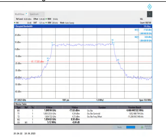
1-N25-PC3-15-5-L-6-CP-QPSK-Outer_Full-25@0-An t3-4.466-5.120-≤5-PASS
