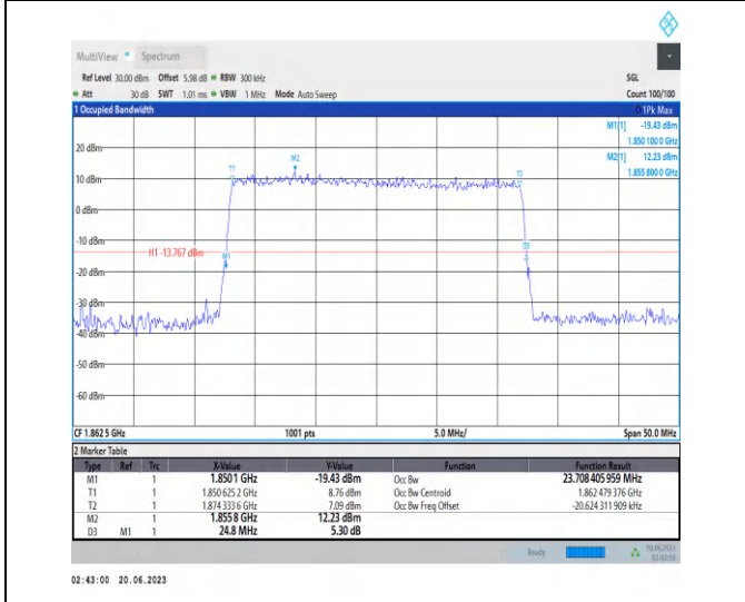
1-N25-PC3-15-25-L-7-CP-16QAM-Outer_Full-133@0 -Ant3-23.708-24.800-≤25-PASS
