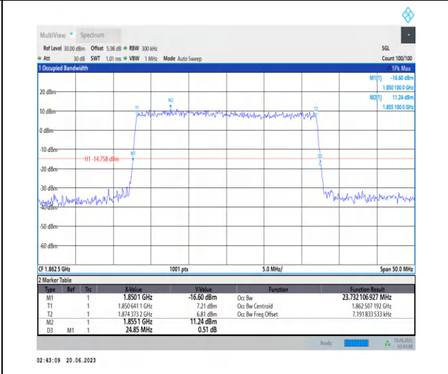
1-N25-PC3-15-25-L-8-CP-64QAM-Outer_Full-133@0 -Ant3-23.732-24.850-≤25-PASS
