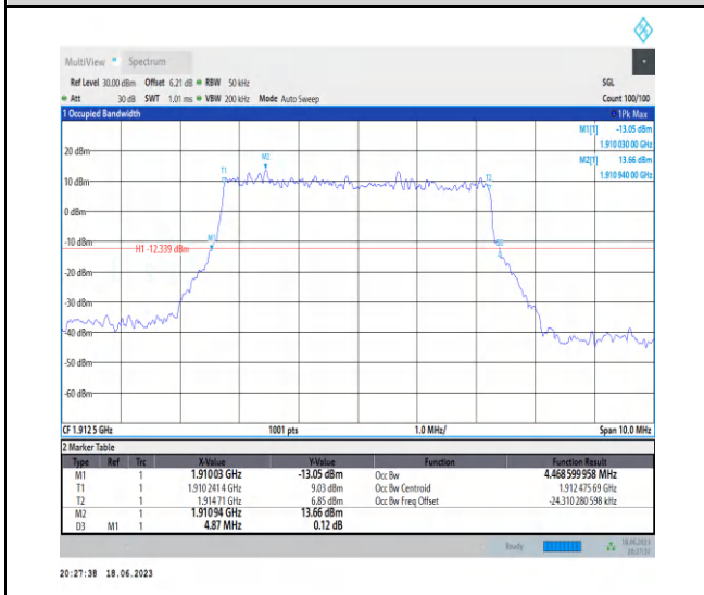
1-N25-PC3-15-5-H-1-DFT-QPSK-Outer_Full-25@0- Ant3-4.469-4.870-≤5-PASS
