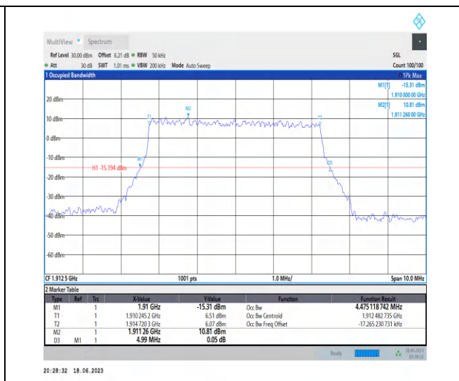
1-N25-PC3-15-5-H-4-DFT-64QAM-Outer_Full-25@0 -Ant3-4.475-4.990-≤5-PASS
