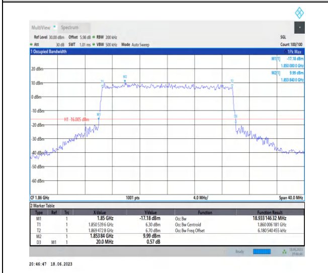
1-N25-PC3-15-20-L-6-CP-QPSK-Outer_Full-106@0 -Ant3-18.933-20.000-≤20-PASS
