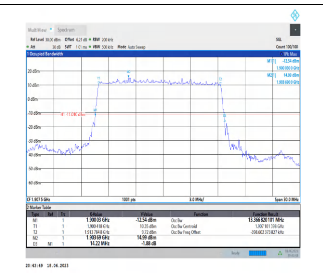
1-N25-PC3-15-15-H-2-DFT-PI2BPSK-Outter_Full-75@ @0-Ant3-13.367-14.220-≤15-PASS
