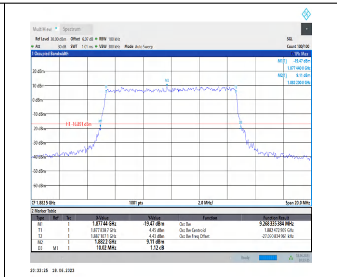
1-N25-PC3-15-10-M-6-CP-QPSK-Outer_Full-52 @0-Ant3-9.268-10.020-≤10-PASS
