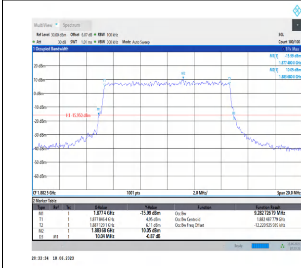
1-N25-PC3-15-10-M-7-CP-16QAM-Outer_Full-52 @0-Ant3-9.283-10.040-≤10-PASS
