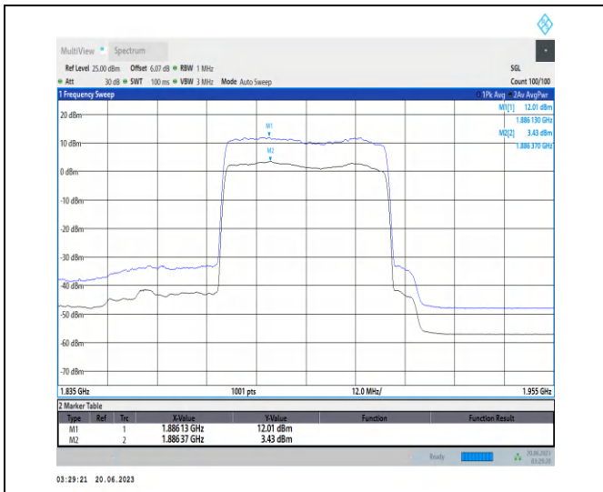
1-N25-PC3-15-40-H-1-DFT-256QAM-Outer_Full-216 @0-Ant3-8.58-100%-0.00-8.58-PASS-≤13
