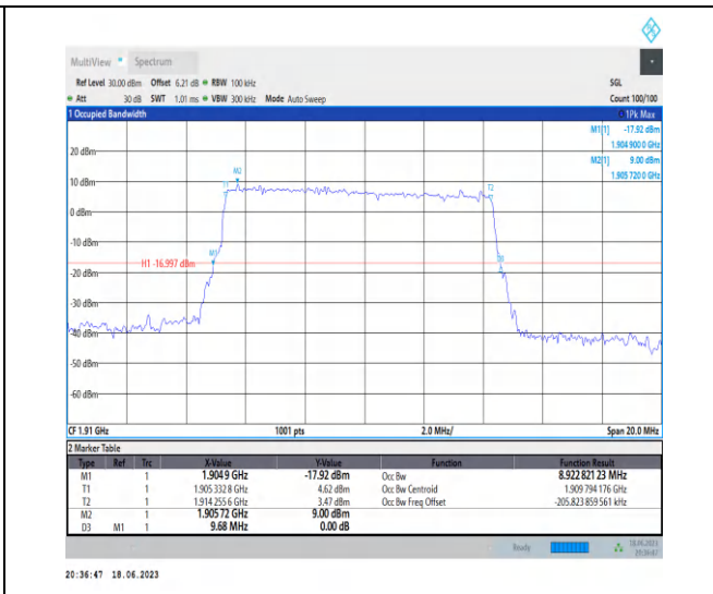
1-N25-PC3-15-10-H-5-DFT-256QAM-Outer_Full-50 @0-Ant3-8.923-9.680-≤10-PASS
