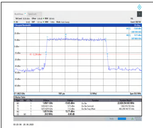
1-N25-PC3-15-25-L-1-DFT-QPSK-Outer_Full-128@ 0-Ant3-22.826-24.000-≤25-PASS
