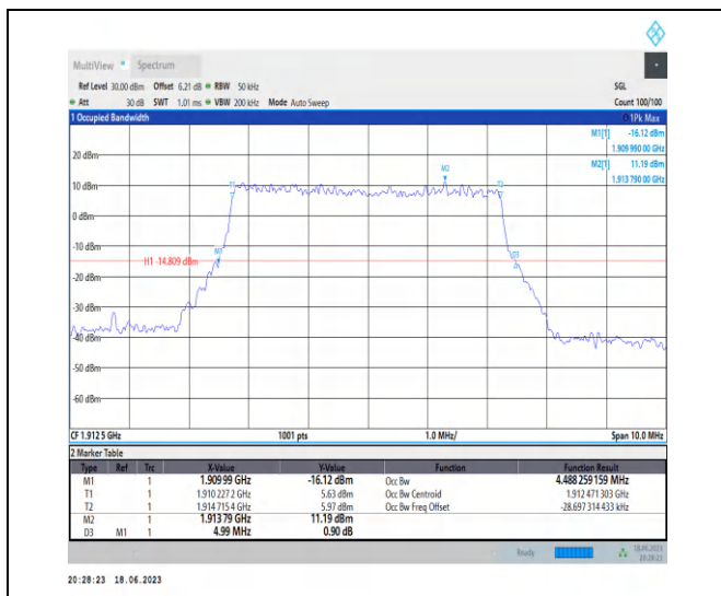
1-N25-PC3-15-5-H-3-DFT-16QAM-Outer_Full-25@0 -Ant3-4.488-4.990-≤5-PASS
