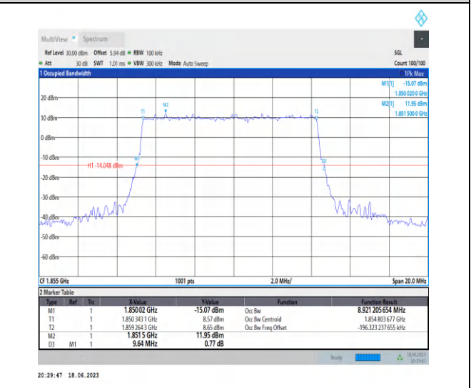
1-N25-PC3-15-10-L-1-DFT-QPSK-Outer_Full-50@0- Ant3-8.921-9.640-≤10-PASS
