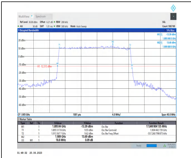
1-N25-PC3-15-20-H-2-DFT-PI2BPSK-Outer_Full-10 @0-Ant3-17.85-18.800-<20-PASS
