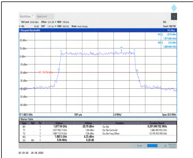
1-N25-PC3-15-10-M-9-CP-256QAM-Outer_Full-52@ 0-Ant3-9.291-9.940-≤10-PASS
