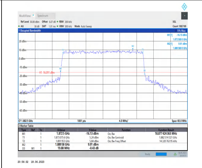
1-N25-PC3-15-20-M-6-CP-QPSK-Outer_Full-106 @0-Ant3-18.877-19.880-<20-PASS
