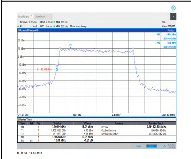
1-N25-PC3-15-10-H-6-CP-QPSK-Outer_Full-52@0- Ant3-9.265-10.040-≤10-PASS
