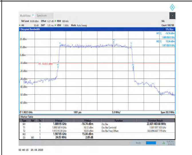
1-N25-PC3-15-25-H-2-DFT-P12BPSK-Outer_Full-128 @0-Ant3-22.831-24.050-<25-PASS
