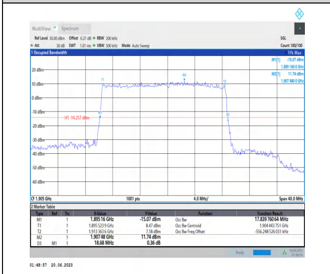
1-N25-PC3-15-20-H-4-DFT-64QAM-Outer_Full-100 @0-Ant3-17.84-18.680-<20-PASS
