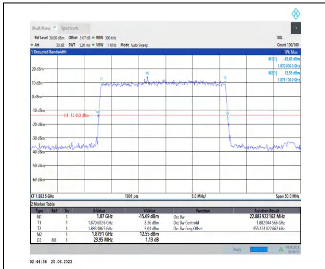
1-N25-PC3-15-25-M-4-DFT-64QAM-Outer_Full-128 @0-Ant3-22.884-23.950-<25-PASS
