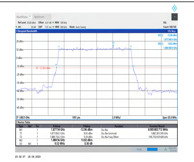
1-N25-PC3-15-10-M-2-DFT-PI2BPSK-Outter_Full-50@0 @0-Ant3-8.906-9.520-≤10-PASS
