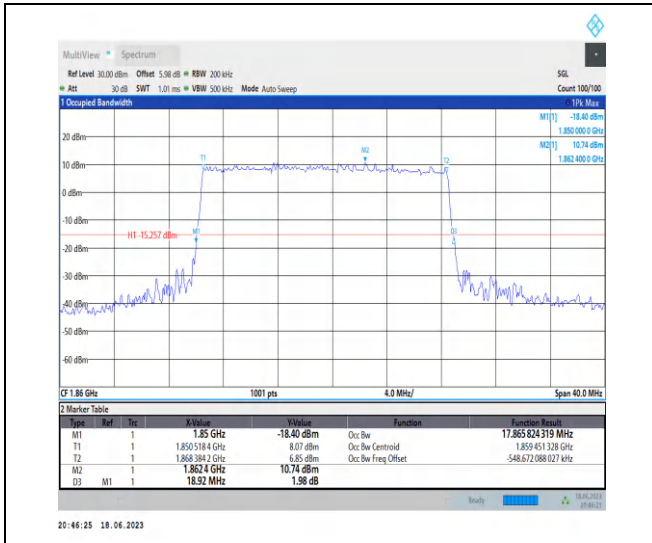
1-N25-PC3-15-20-L-4-DFT-64QAM-Outer_Full-100 @0-Ant3-17.866-18.920-≤20-PASS
