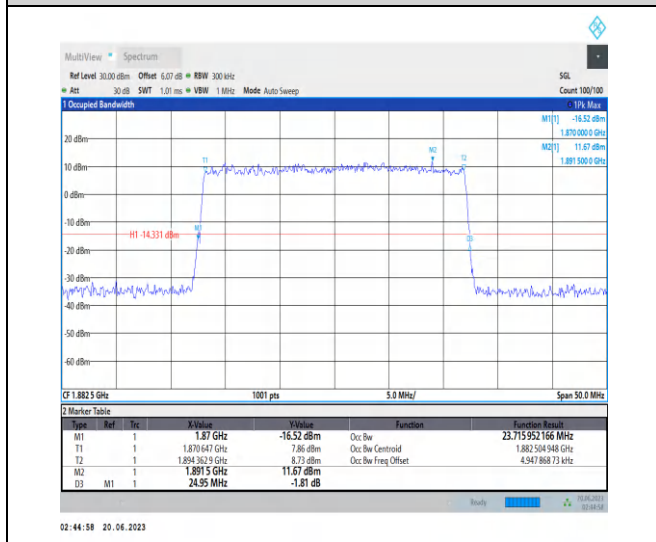
1-N25-PC3-15-25-M-6-CP-QPSK-Outer_Full-133@0 -Ant3-23.716-24.950-<25-PASS
