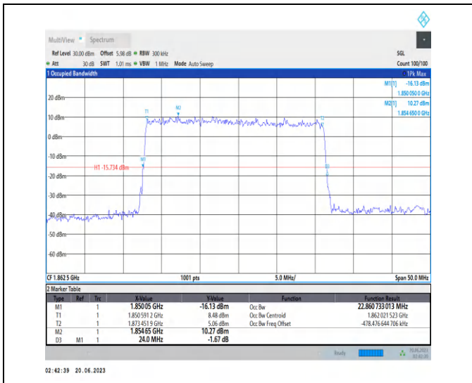
1-N25-PC3-15-25-L-5-DFT-256QAM-Outer_Full-128 @0-Ant3-22.861-24.000-≤25-PASS
