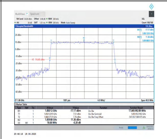
1-N25-PC3-15-20-L-3-DFT-16QAM-Outer_Full-100 @0-Ant3-17.846-18.680-<=20-PASS
