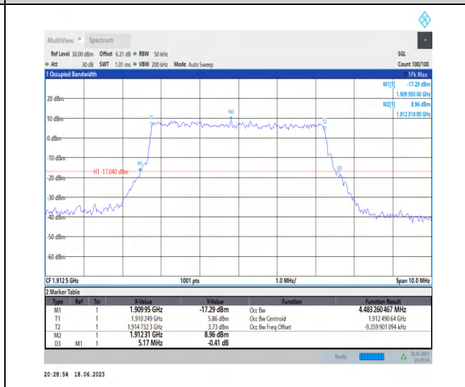
1-N25-PC3-15-5-H-6-CP-QPSK-Outer_Full-25@0-A Ant3-4.483-5.170-≤5-PASS
