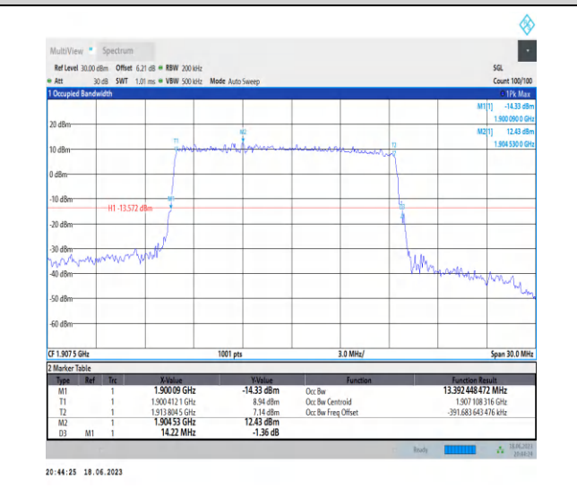
1-N25-PC3-15-15-H-4-DFT-64QAM-Outter_Full-75@ 0-Ant3-13.392-14.220-≤15-PASS
