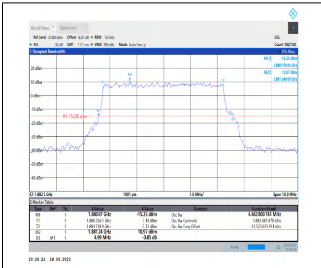
1-N25-PC3-15-5-M-4-DFT-64QAM-Outer_Full-25@0 -Ant3-4.463-4.990-≤5-PASS
