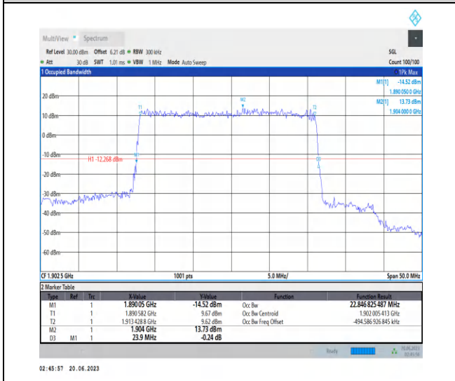
1-N25-PC3-15-25-H-1-DFT-QPSK-Outer_Full-128@ 0-Ant3-22.847-23.900-<25-PASS
