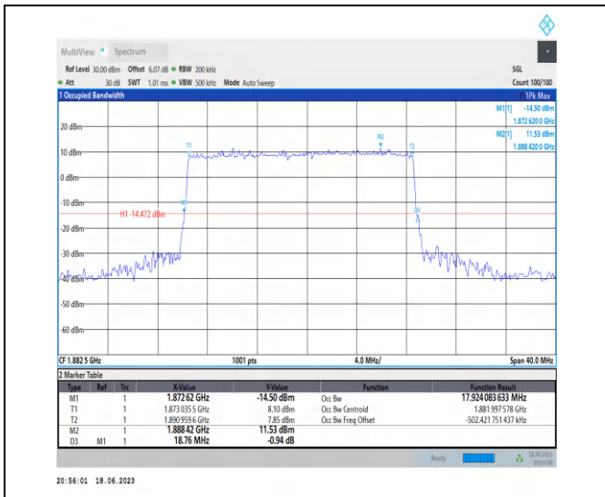
1-N25-PC3-15-20-M-3-DFT-16QAM-Outer_Full-100 @0-Ant3-17.924-18.760-<20-PASS
