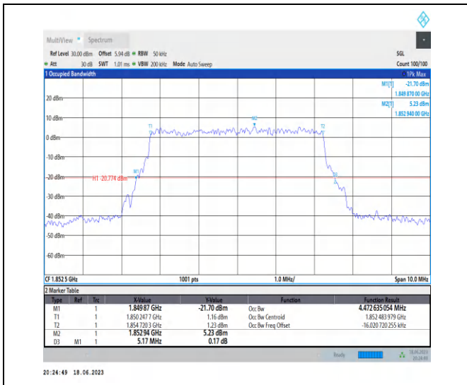
1-N25-PC3-15-5-L-9-CP-256QAM-Outer_Full-25@0- Ant3-4.473-5.170-≤5-PASS
