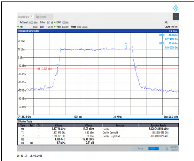
1-N25-PC3-15-10-M-1-DFT-QPSK-Outter_Full-50@0 -Ant3-8.92-9.700-≤10-PASS
