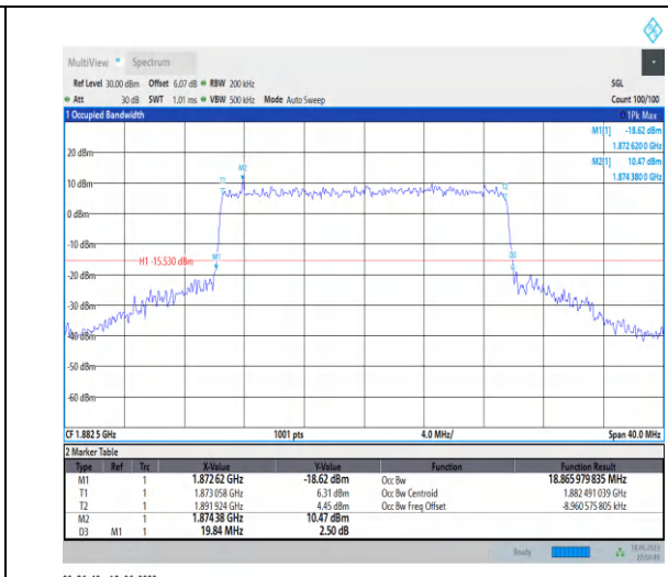
1-N25-PC3-15-20-M-8-CP-64QAM-Outer_Full-106@ -0-Ant3-18.866-19.840-<20-PASS
