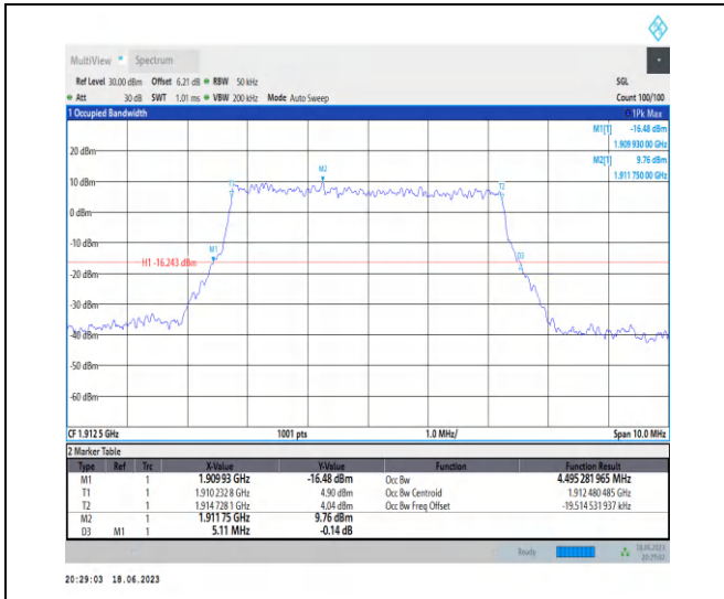
1-N25-PC3-15-5-H-7-CP-16QAM-Outer_Full-25@0- Ant3-4.495-5.110-≤5-PASS
