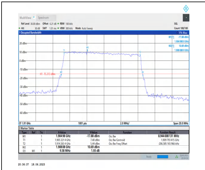
1-N25-PC3-15-10-H-4-DFT-64QAM-Outer_Full-50@ 0-Ant3-8.944-9.580-≤10-PASS
