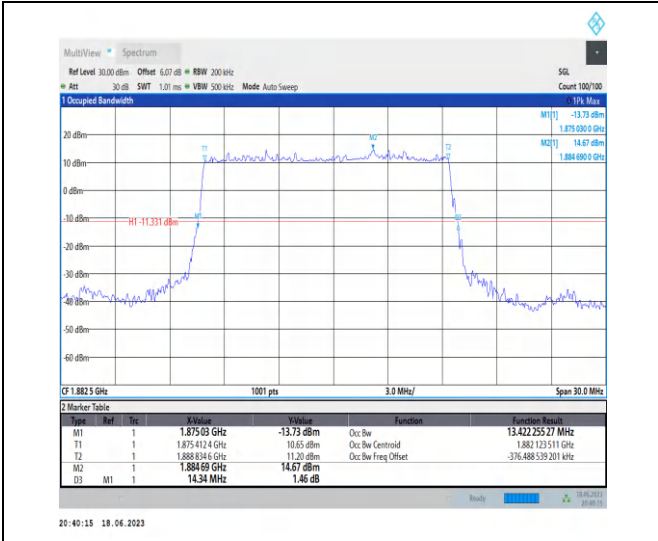
1-N25-PC3-15-15-M-2-DFT-PI2BPSK-Outer_Full-75 @0-Ant3-13.422-14.340≤15-PASS
