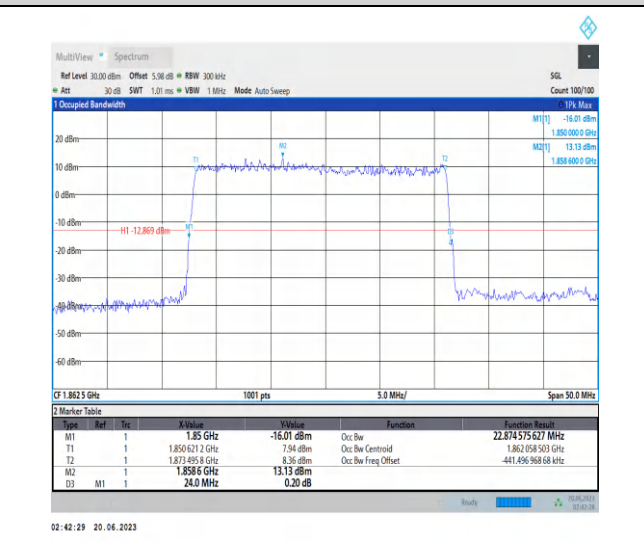
1-N25-PC3-15-25-L-4-DFT-64QAM-Outer_Full-128@ 0-Ant3-22.875-24.000-≤25-PASS
