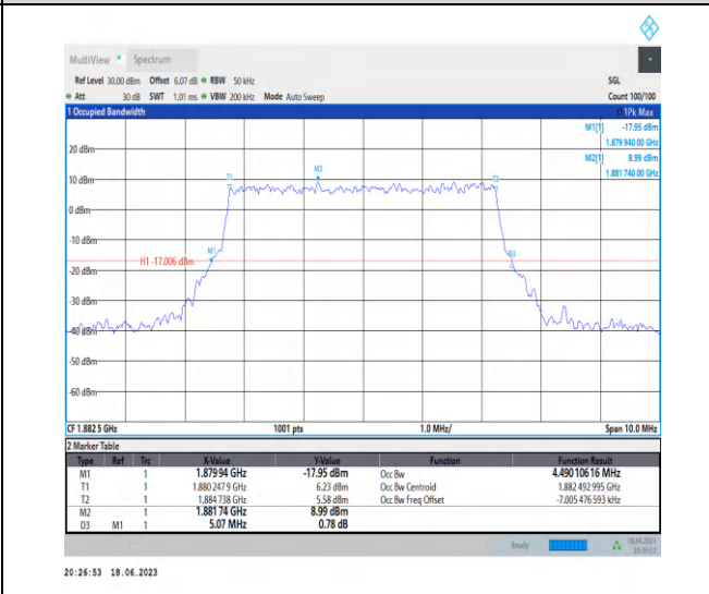
1-N25-PC3-15-5-M-7-CP-16QAM-Outer_Full-25@0- Ant3-4.49-5.070-≤5-PASS
