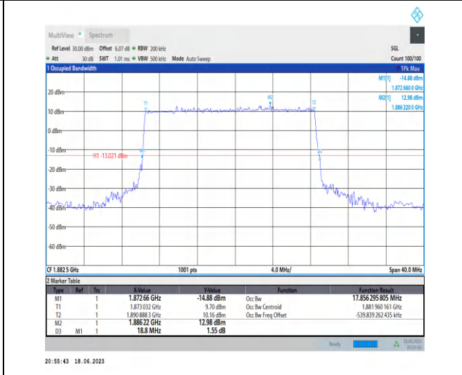
1-N25-PC3-15-20-M-2-DFT-PI2BPSK-Outer_Full-100 @0-Ant3-17.856-18.800-≤20-PASS
