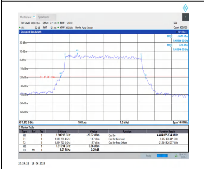
1-N25-PC3-15-5-H-9-CP-256QAM-Outer_Full-25@0 -Ant3-4.484-5.010-≤5-PASS
