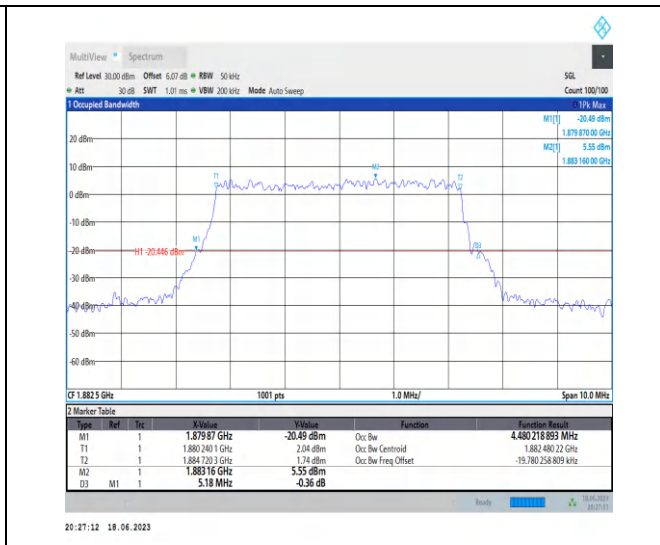
1-N25-PC3-15-5-M-9-CP-256QAM-Outer_Full-25@0- Ant3-4.48-5.180-≤5-PASS
