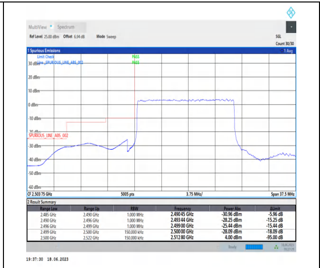
1-N7-PC3-15-15-L-3-DFT-PI2BPSK-Outer_Full-75 @0-Ant0-1--PASS-see graph
