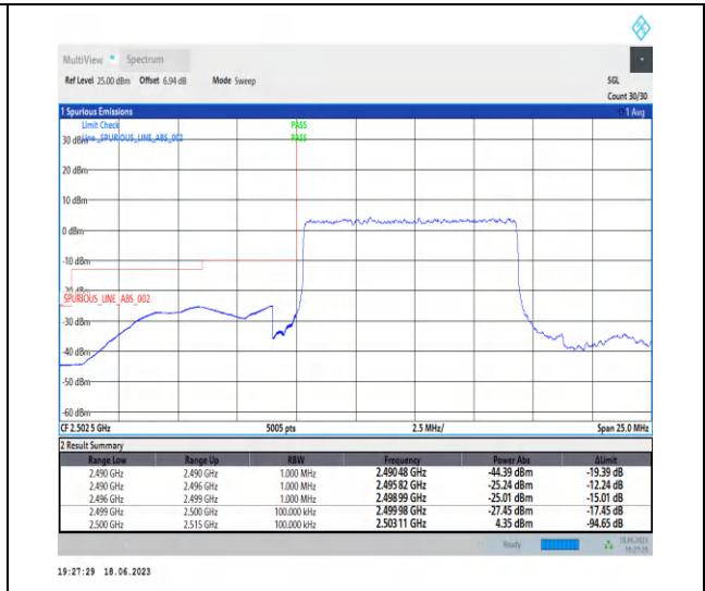
1-N7-PC3-15-10-L-3-DFT-PI2BPSK-Outer_Full-50 @0-Ant0-1--PASS-see graph
