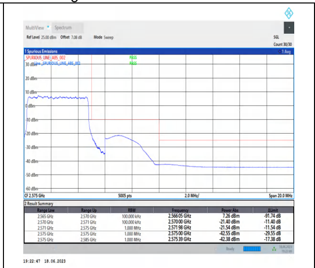
1-N7-PC3-15-5-H-3-DFT-PI2BPSK-Outer_Full-25 @0-Ant0-1--PASS-see graph
