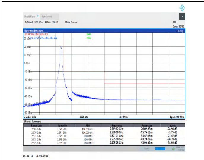
1-N7-PC3-15-5-H-2-DFT-PI2BPSK-Edge_1RB_Right-1 @24-Ant0-1--PASS-see graph
