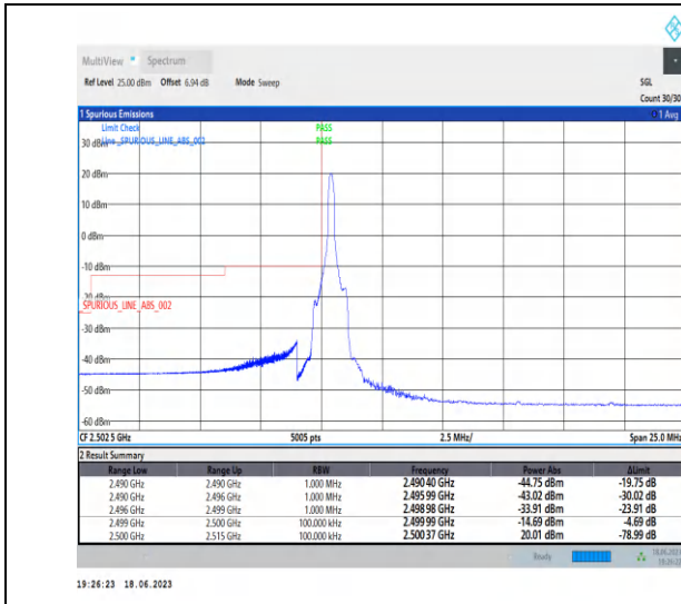
1-N7-PC3-15-10-L-1-DFT-PI2BPSK-Edge_1RB_Left-1 @0-Ant0-1--PASS-see graph
