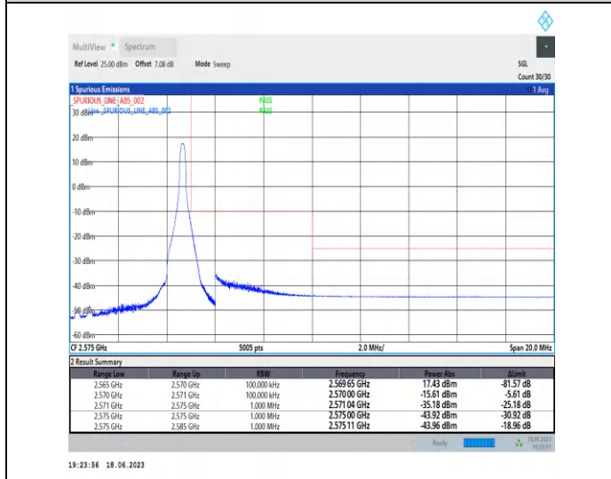
1-N7-PC3-15-5-H-5-CP-QPSK-Edge_1RB_Right-1 @24-Ant0-1--PASS-see graph
