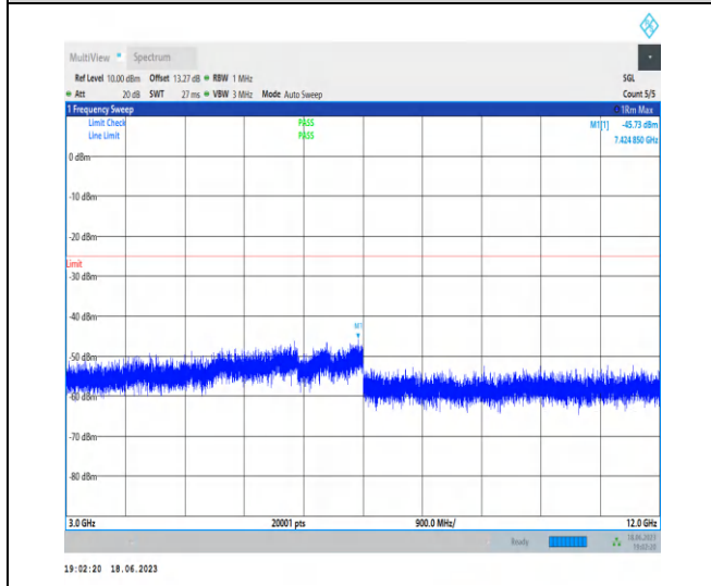
1-N7-PC3-15-40-M-1-DFT-PI2BPSK-Inner_1RB_Lef t-1 @ 1-3000-12000-Ant0-7424.85--45.73--25-PASS
