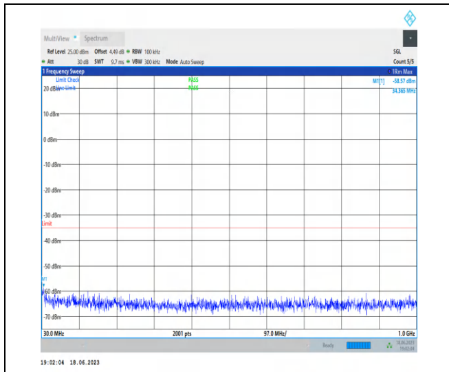
1-N7-PC3-15-40-M-1-DFT-PI2BPSK-Inner_1RB_Lef t-1 @ 1-30-1000-Ant0-34.37--58.57--35-PASS
