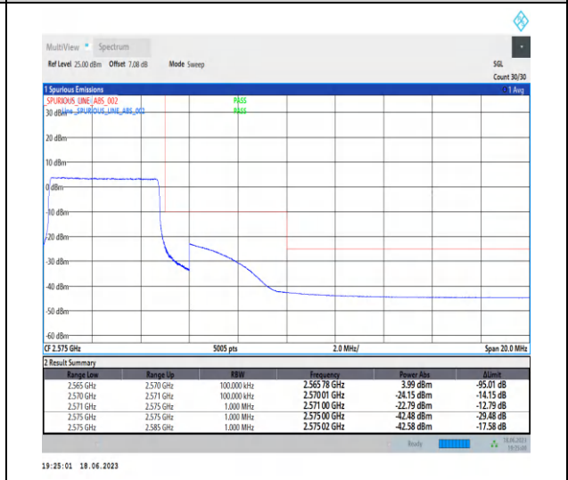
1-N7-PC3-15-5-H-6-CP-QPSK-Outer_Full-25 @0-Ant0-1--PASS-see graph
