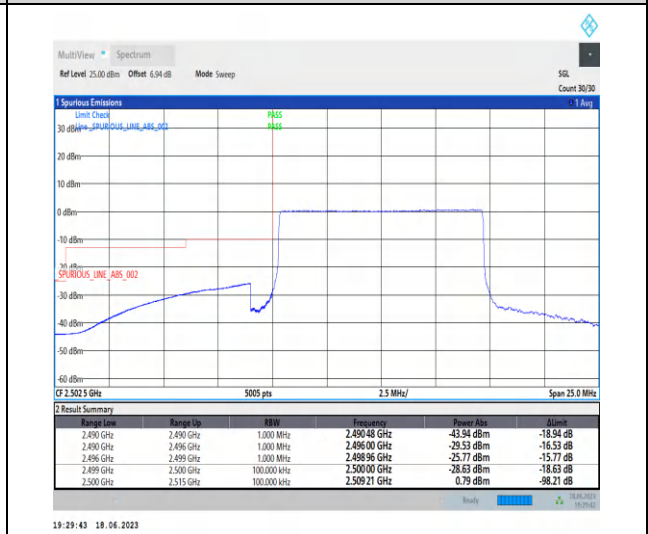
1-N7-PC3-15-10-L-6-CP-QPSK-Outer_Full-52 @0-Ant0-1--PASS-see graph
