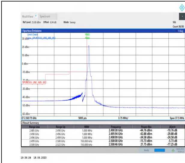
1-N7-PC3-15-15-L-1-DFT-PI2BPSK-Edge_1RB_Left-1 @0-Ant0-1--PASS-see graph
