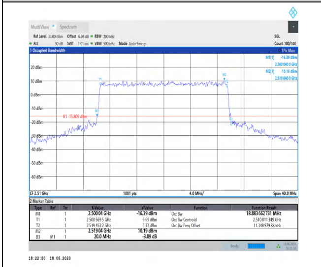
1-N7-PC3-15-20-L-6-CP-QPSK-Outer_Full-106@0- Ant0-18.884-20.000-≤20-PASS
