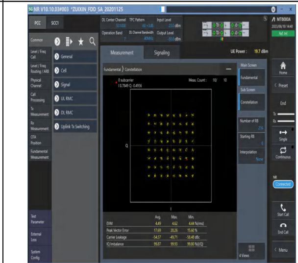
1-N7-PC3-15-40-M-8-CP-64QAM-Outer_Full-216@0-Ant0-see graph-PASS
