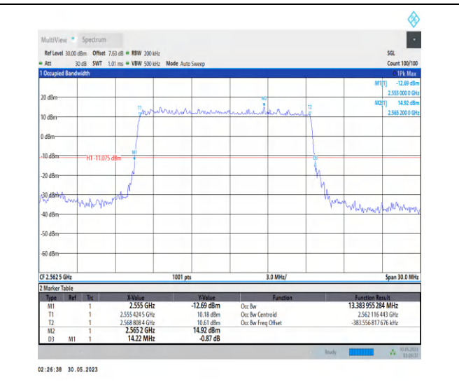
1-N7-PC3-15-15-H-2-DFT-PI2BPSK-Outer_Full-75@0-Ant0-13.384-14.22-≤15-PASS
