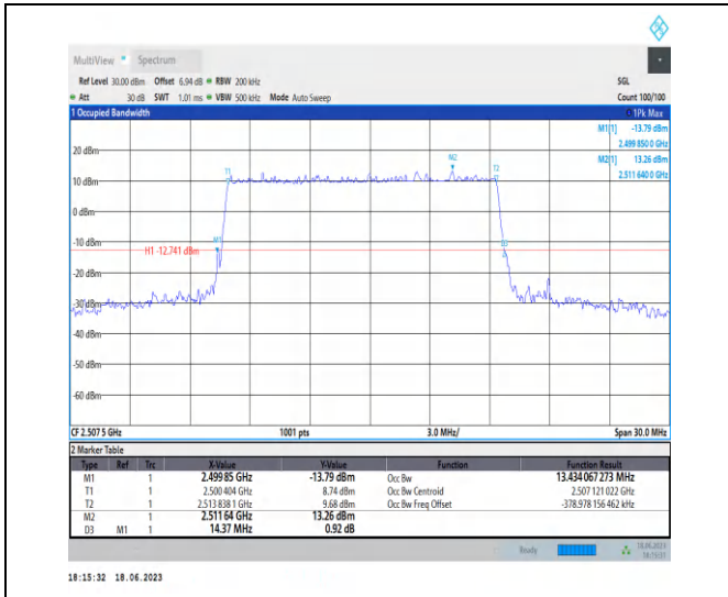
1-N7-PC3-15-15-L-3-DFT-16QAM-Outer_Full-75@0-Ant0-13.434-14.370-≤15-PASS
