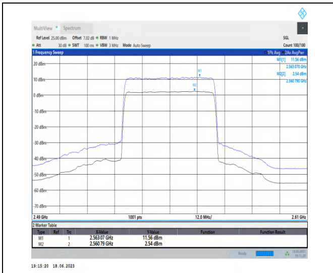
1-N7-PC3-15-40-H-1-DFT-256QAM-Outer_Full-216 @0-Ant0-9.02-100%-0.00-9.02-PASS-≤13
