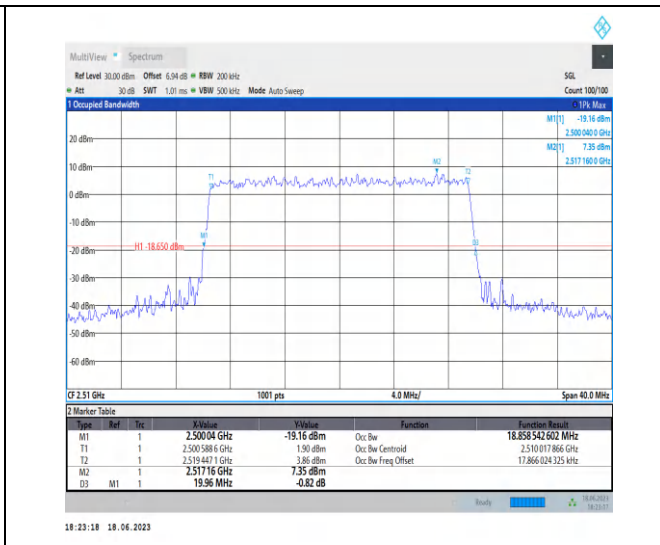
1-N7-PC3-15-20-L-9-CP-256QAM-Outer_Full-106@0 -Ant0-18.859-19.960-≤20-PASS
