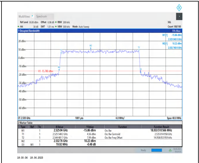
1-N7-PC3-15-20-M-8-CP-64QAM-Outer_Full-106@0 -Ant0-18.934-19.920-<=20-PASS
