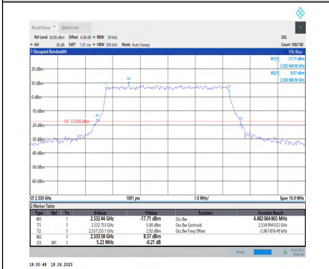
1-N7-PC3-15-5-M-6-CP-QPSK-Outer_Full-25@0-Ant0-4.482-5.220-≤5-PASS
