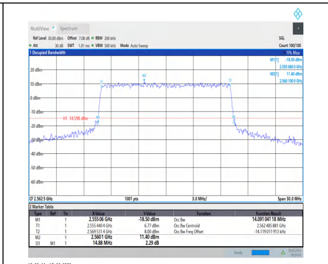
1-N7-PC3-15-15-H-6-CP-QPSK-Outer_Full-79@0-A Ant0-14.091-14.880-≤15-PASS
