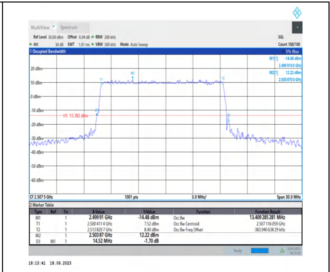
1-N7-PC3-15-15-L-4-DFT-64QAM-Outer_Full-75@0-Ant0-13.409-14.520-≤15-PASS
