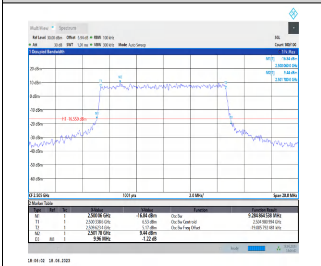
1-N7-PC3-15-10-L-8-CP-64QAM-Outer_Full-52@0-A Ant0-9.285-9.960≤10-PASS
