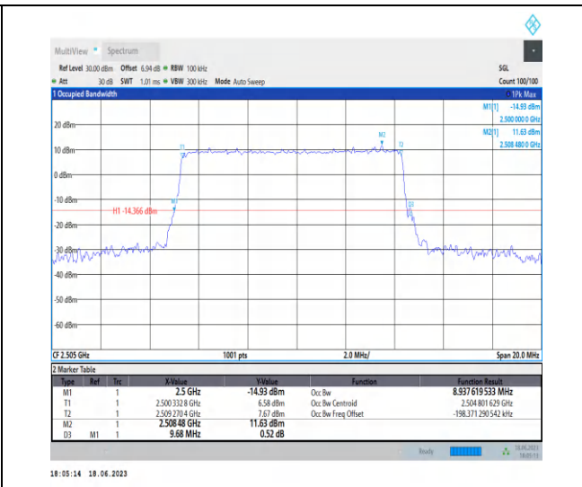
1-N7-PC3-15-10-L-3-DFT-16QAM-Outer_Full-50@0- Ant0-8.938-9.680-≤10-PASS
