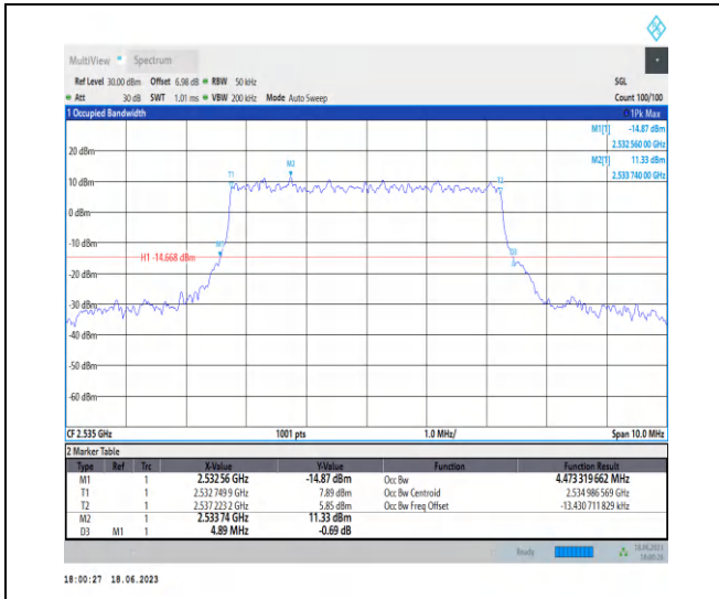
1-N7-PC3-15-5-M-4-DFT-64QAM-Outer_Full-25@0-Ant0-4.473-4.890-≤5-PASS
