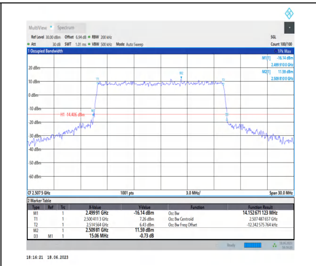
1-N7-PC3-15-15-L-8-CP-64QAM-Outer_Full-79@0- Ant0-14.153-15.060-≤15-PASS
