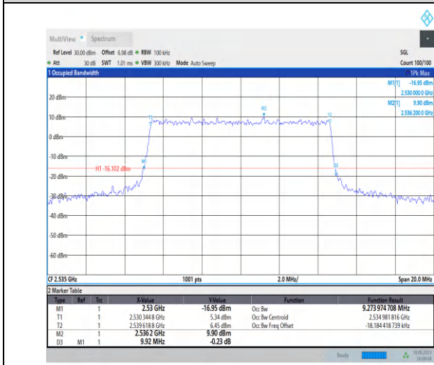
1-N7-PC3-15-10-M-5-DFT-256QAM-Outer_Full-50@0 -Ant0-8.926-9.640-≤10-PASS
