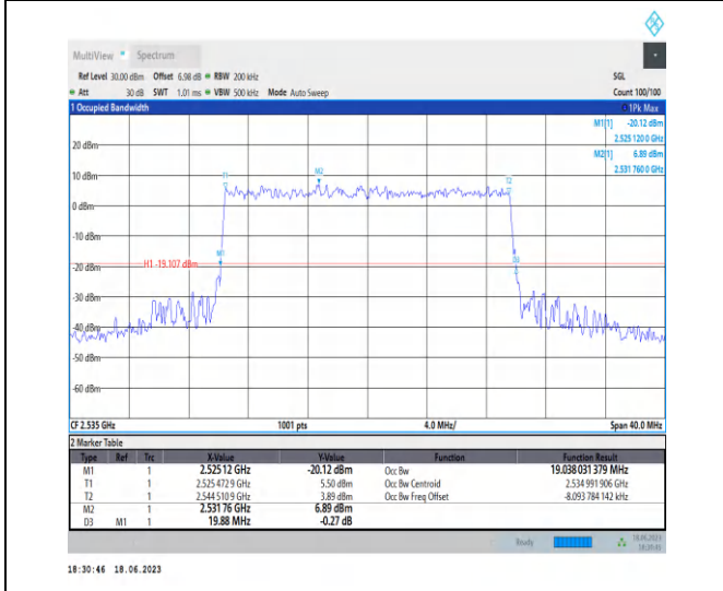
1-N7-PC3-15-20-M-9-CP-256QAM-Outer_Full-106@0 -Ant0-19.038-19.880-<=20-PASS
