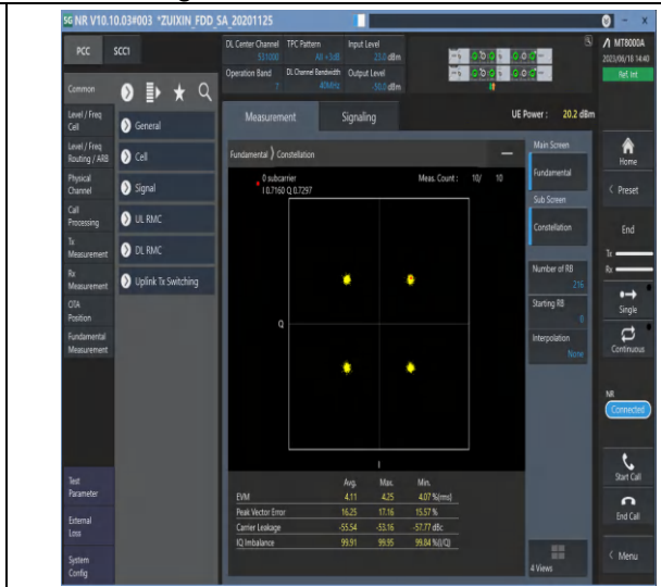
1-N7-PC3-15-40-M-6-CP-QPSK-Outer_Full-216@0-Ant0-see graph-PASS
