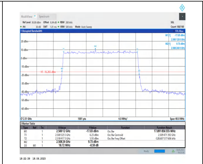
1-N7-PC3-15-20-L-5-DFT-256QAM-Outer_Full-100@ 0-Ant0-17.892-18.720-≤20-PASS
