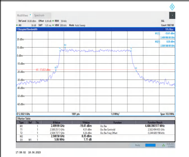
1-N7-PC3-15-5-L-8-CP-64QAM-Outer_Full-25@0-Ant0-4.486-5.060-≤5-PASS
