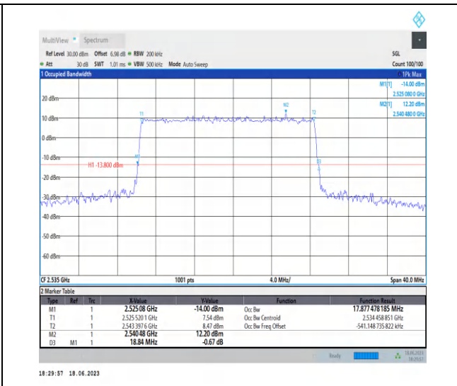
1-N7-PC3-15-20-M-4-DFT-64QAM-Outer_Full-100@ 0-Ant0-17.877-18.840-≤20-PASS
