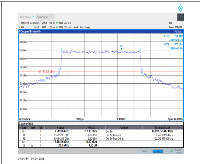
1-N7-PC3-15-20-H-7-CP-16QAM-Outer_Full-106@0-Ant0-18.897-20.000-<20-PASS
