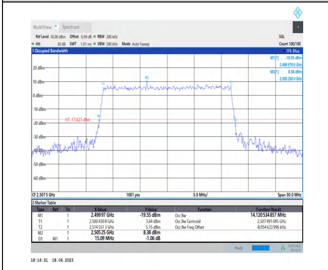
1-N7-PC3-15-15-L-9-CP-256QAM-Outer_Full-79@0- Ant0-14.121-15.090-≤15-PASS
