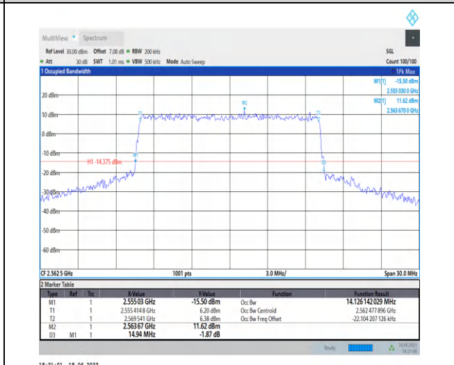
1-N7-PC3-15-15-H-8-CP-64QAM-Outer_Full-79@0-A Ant0-14.126-14.940-≤15-PASS
