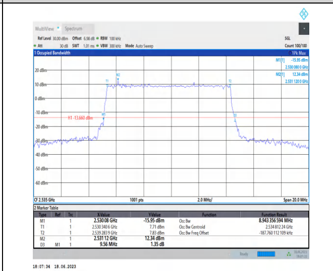
1-N7-PC3-15-10-M-4-DFT-64QAM-Outer_Full-50@0-Ant0-8.943-9.560-≤10-PASS
