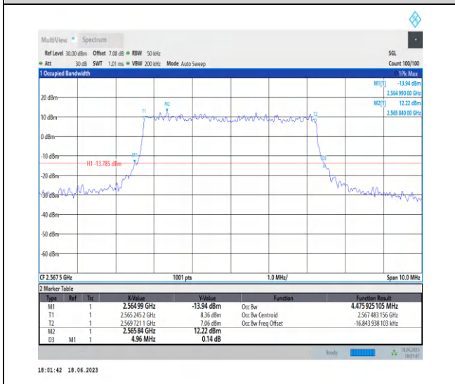
1-N7-PC3-15-5-H-1-DFT-QPSK-Outer_Full-25@0-A nt0-4.476-4.960-≤5-PASS
