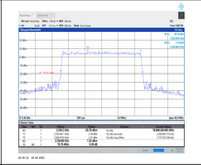
1-N7-PC3-15-20-H-9-CP-256QAM-Outer_Full-106@0-Ant0-18.848-19.760-<20-PASS
