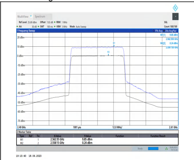
1-N7-PC3-15-40-H-2-CP-256QAM-Outer_Full-216 @0-Ant0-9.61-100%-0.00-9.61-PASS-≤13
