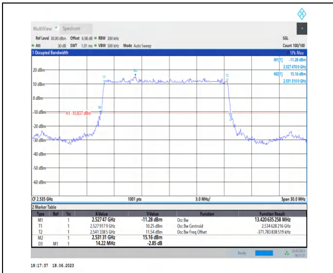
1-N7-PC3-15-15-M-2-DFT-PI2BPSK-Outer_Full-75@ 0-Ant0-13.421-14.220-≤15-PASS
