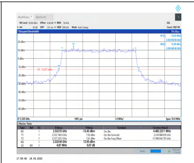
1-N7-PC3-15-5-M-1-DFT-QPSK-Outer_Full-25@0-A Ant0-4.482-4.870-≤5-PASS
