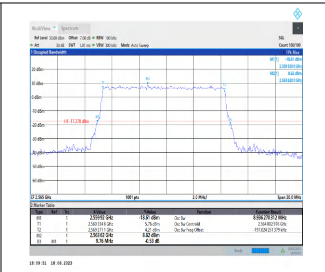
1-N7-PC3-15-10-H-5-DFT-256QAM-Outer_Full-50@0 0-Ant0-8.936-9.760-≤10-PASS
