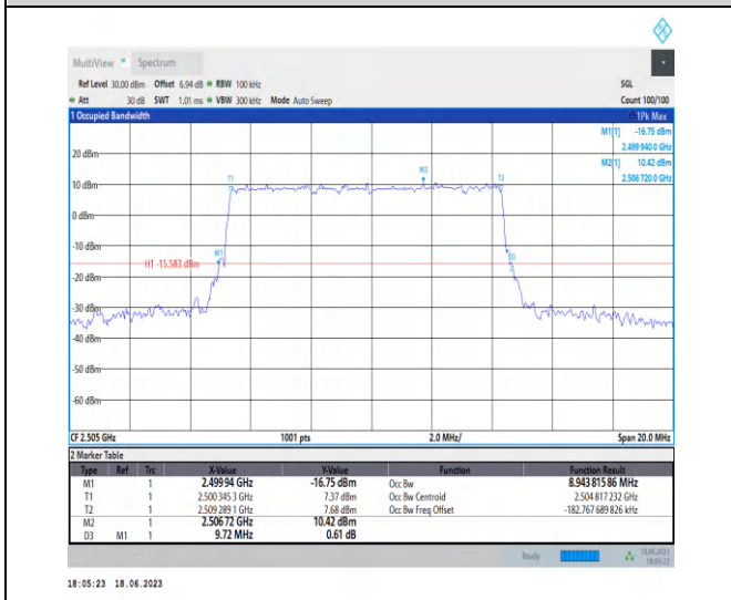
1-N7-PC3-15-10-L-4-DFT-64QAM-Outer_Full-50@0- Ant0-8.944-9.720-≤10-PASS
