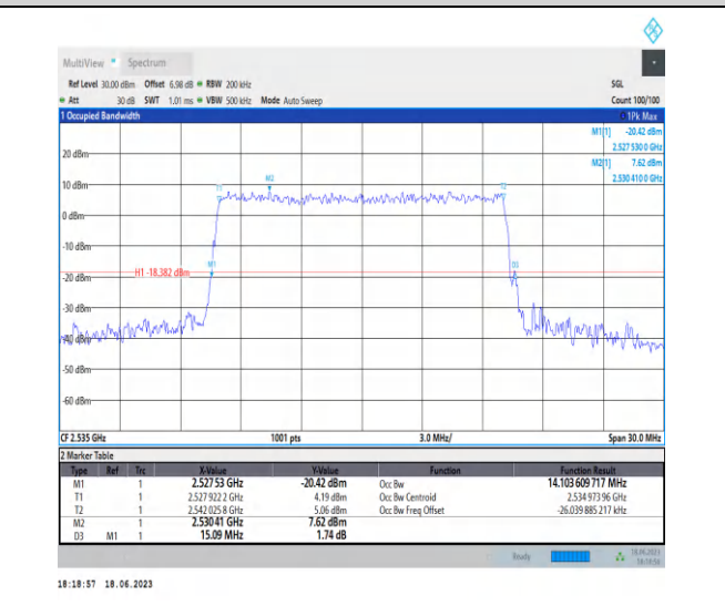
1-N7-PC3-15-15-M-9-CP-256QAM-Outer_Full-79@0- -Ant0-14.104-15.090-≤15-PASS
