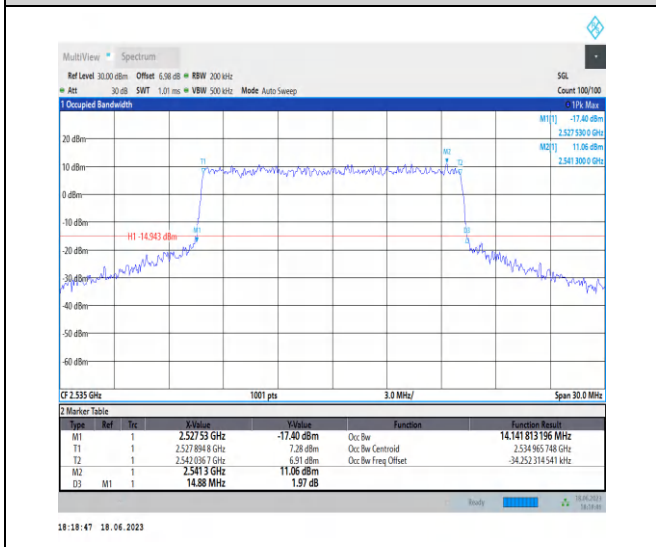
1-N7-PC3-15-15-M-8-CP-64QAM-Outer_Full-79@0- Ant0-14.142-14.880-≤15-PASS
