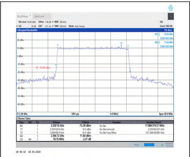
1-N7-PC3-15-20-H-3-DFT-16QAM-Outer_Full-100@0-Ant0-17.885-18.760-<=20-PASS
