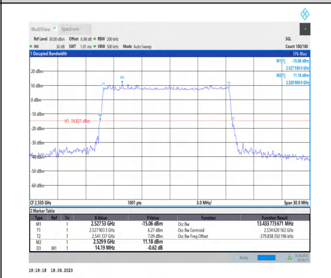
1-N7-PC3-15-15-M-5-DFT-256QAM-Outer_Full-75@ 0-Ant0-13.434-14.190-≤15-PASS
