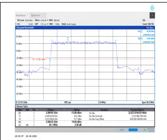
1-N7-PC3-15-25-L-2-DFT-PI2BPSK-Outer_Full-128@0-Ant0-22.872-24.100-≤25-PASS
