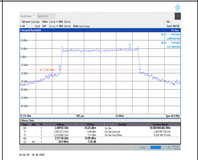
1-N7-PC3-15-20-L-7-CP-16QAM-Outer_Full-106@0- Ant0-18.945-20.000-≤20-PASS
