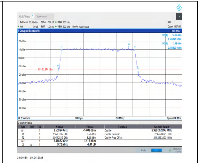
1-N7-PC3-15-10-H-1-DFT-QPSK-Outer_Full-50@0-Ant0-8.929-9.720-≤10-PASS
