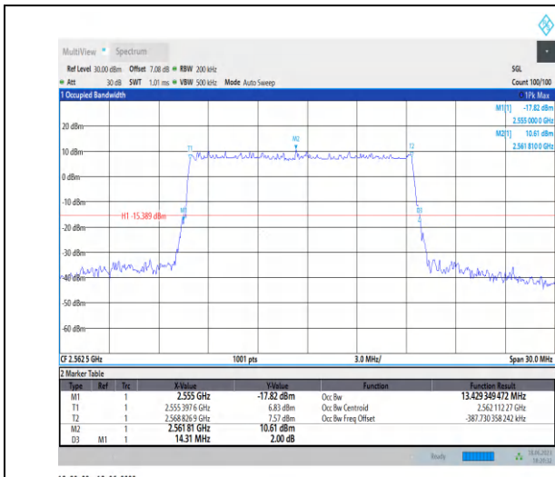
1-N7-PC3-15-15-H-5-DFT-256QAM-Outer_Full-75@0-A -Ant0-13.429-14.310-≤15-PASS
