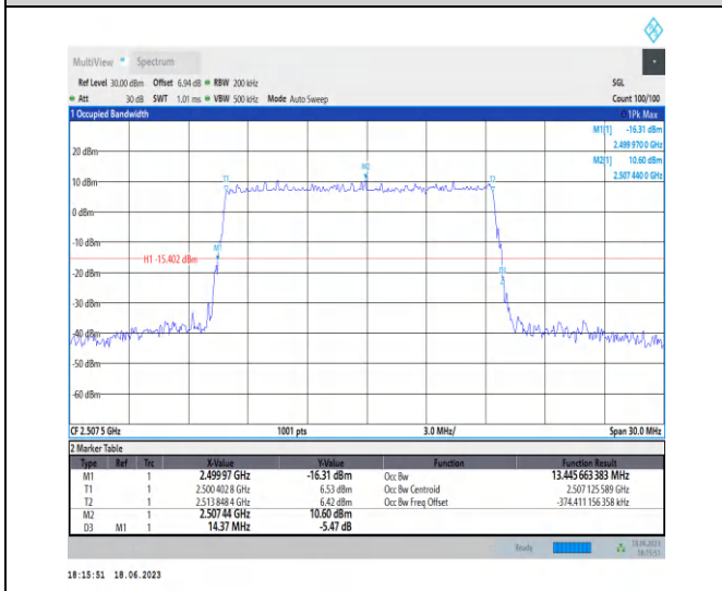
1-N7-PC3-15-15-L-5-DFT-256QAM-Outer_Full-75@0-Ant0-13.446-14.370-≤15-PASS
