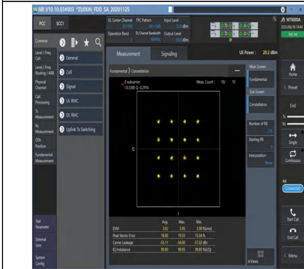
1-N7-PC3-15-40-M-7-CP-16QAM-Outer_Full-216@0-Ant0-see graph-PASS
