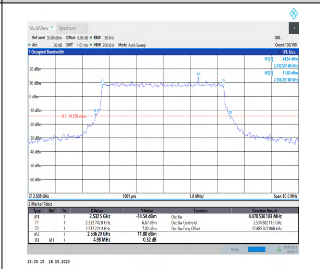
1-N7-PC3-15-5-M-3-DFT-16QAM-Outer_Full-25@0-A Ant0-4.479-4.980-≤5-PASS
