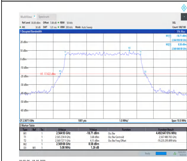
1-N7-PC3-15-5-H-5-DFT-256QAM-Outer_Full-25@0-A Ant0-4.493-5.080 \leq 5 -PASS
