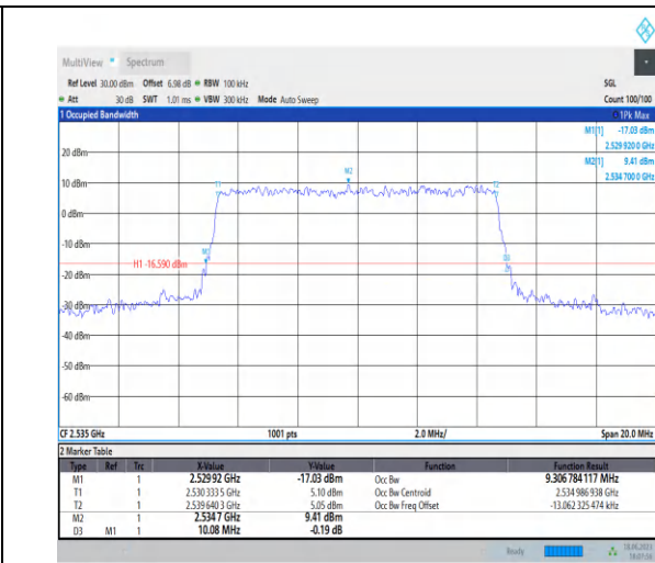
1-N7-PC3-15-10-M-6-CP-QPSK-Outer_Full-52@0- Ant0-9.307-10.080-≤10-PASS
