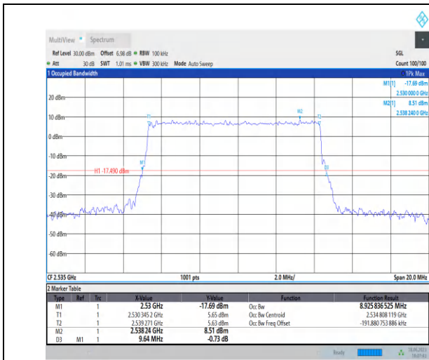
1-N7-PC3-15-10-M-5-DFT-256QAM-Outer_Full-50@0 -Ant0-8.926-9.640-≤10-PASS
