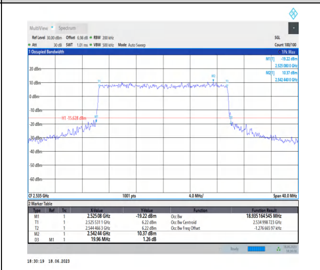
1-N7-PC3-15-20-M-6-CP-QPSK-Outer_Full-106@0- Ant0-18.935-19.960-≤20-PASS
