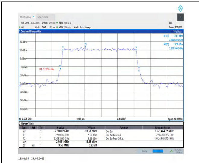
1-N7-PC3-15-10-L-2-DFT-PI2BPSK-Outer_Full-50@ 0-Ant0-8.921-9.560-≤10-PASS
