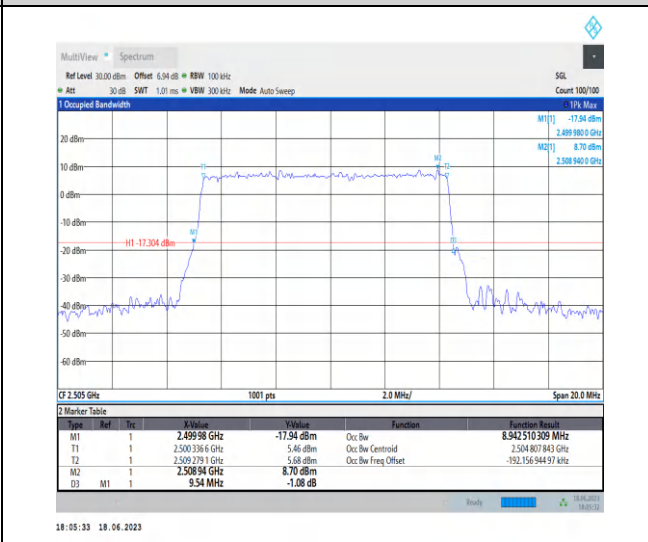
1-N7-PC3-15-10-L-5-DFT-256QAM-Outer_Full-50@ 0-Ant0-8.943-9.540-≤10-PASS
