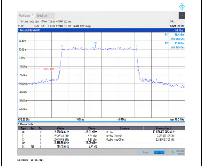
1-N7-PC3-15-20-H-1-DFT-QPSK-Outer_Full-100@0 -Ant0-17.873-18.720-<=20-PASS
