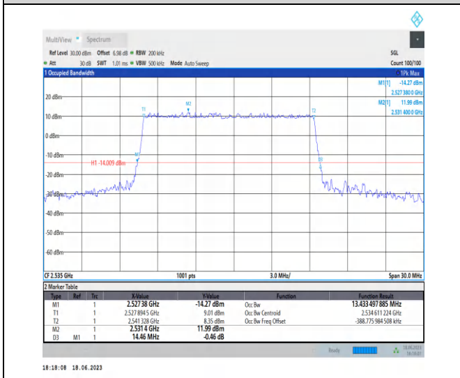
1-N7-PC3-15-15-M-4-DFT-64QAM-Outer_Full-75@0 -Ant0-13.433-14.460-≤15-PASS
