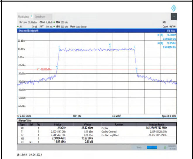
1-N7-PC3-15-15-L-6-CP-QPSK-Outer_Full-79@0-Ant0-14.127-14.970-≤15-PASS
