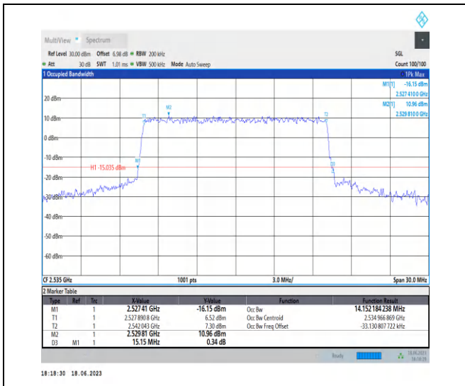
1-N7-PC3-15-15-M-6-CP-QPSK-Outer_Full-79@0-A Ant0-14.152-15.150-≤15-PASS
