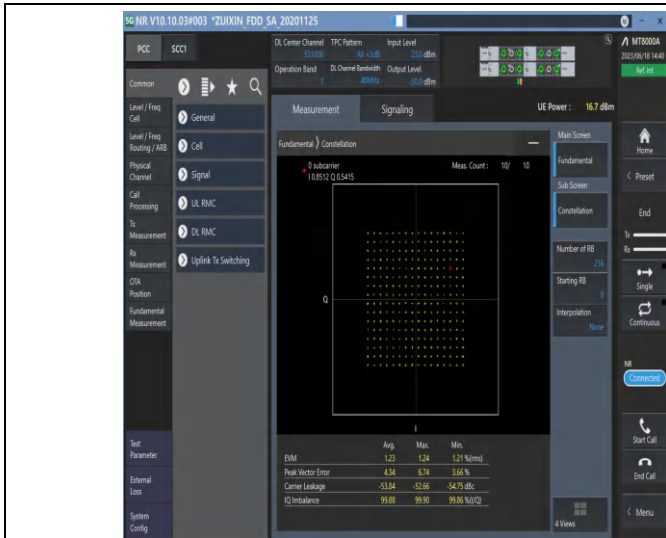
1-N7-PC3-15-40-M-9-CP-256QAM-Outer_Full-216@0-Ant0-see graph-PASS
