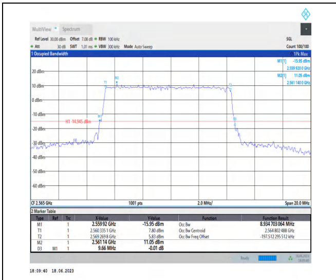
1-N7-PC3-15-10-H-4-DFT-64QAM-Outer_Full-50@0 -Ant0-8.935-9.660-≤10-PASS
