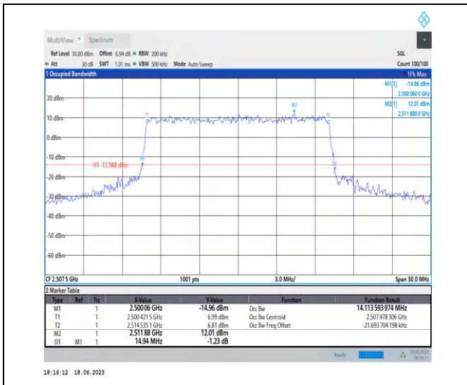
1-N7-PC3-15-15-L-7-CP-16QAM-Outer_Full-79@0-A Ant0-14.114-14.940-≤15-PASS
