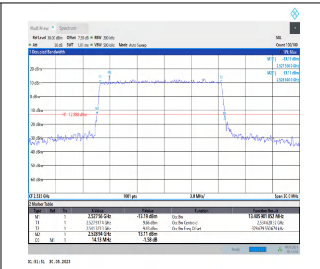
1-N7-PC3-15-15-M-3-DFT-16QAM-Outer_Full-75@0 -Ant0-13.406-14.13-≤15-PASS
