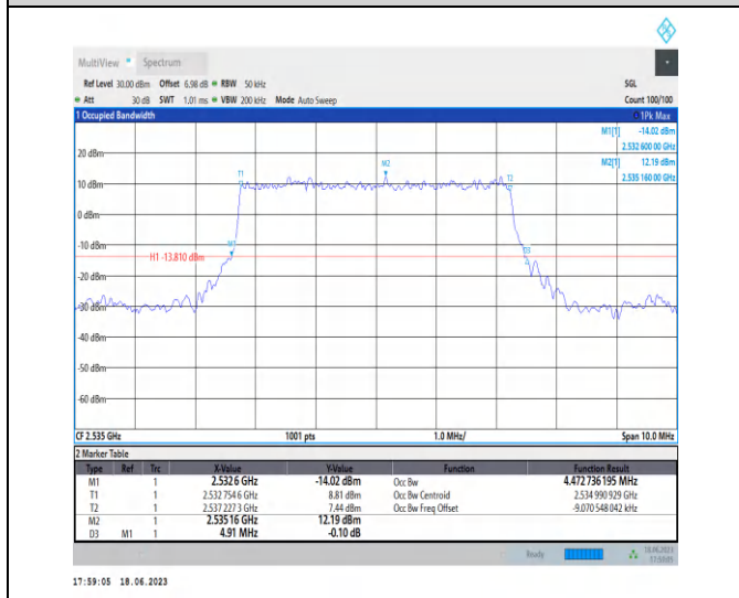
1-N7-PC3-15-5-M-2-DFT-PI2BPSK-Outer_Full-25@0-A Ant0-4.473-4.910-≤5-PASS
