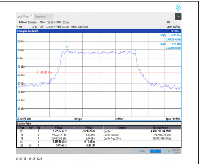
1-N7-PC3-15-5-H-8-CP-64QAM-Outer_Full-25@0-A nt0-4.489-5.010-≤5-PASS
