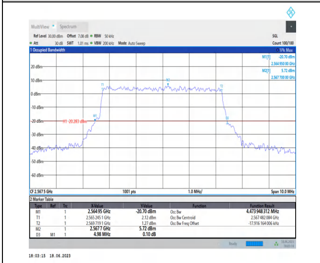
1-N7-PC3-15-5-H-9-CP-256QAM-Outer_Full-25@0-A Ant0-4.474-4.980-≤5-PASS
