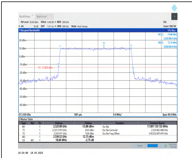
1-N7-PC3-15-20-M-3-DFT-16QAM-Outer_Full-100@ 0-Ant0-17.891-18.840-≤20-PASS
