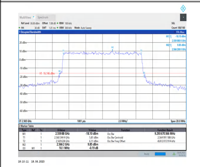
1-N7-PC3-15-10-H-7-CP-16QAM-Outer_Full-52@0- Ant0-9.294-10.100-≤10-PASS
