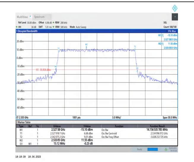
1-N7-PC3-15-15-M-7-CP-16QAM-Outer_Full-79@0- Ant0-14.157-15.120-≤15-PASS
