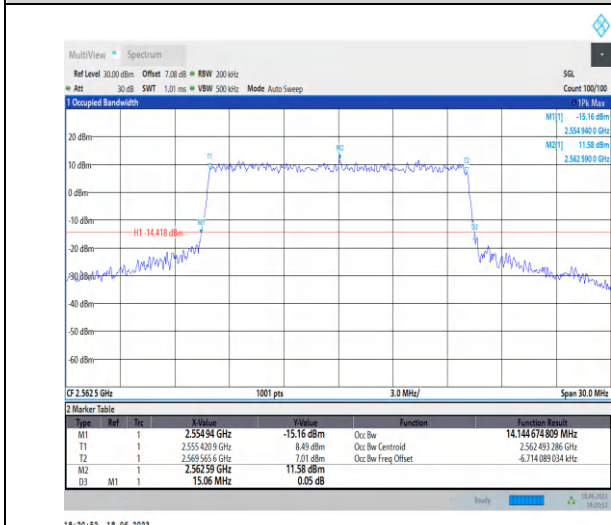
1-N7-PC3-15-15-H-7-CP-16QAM-Outer_Full-79@0-A Ant0-14.145-15.060-≤15-PASS
