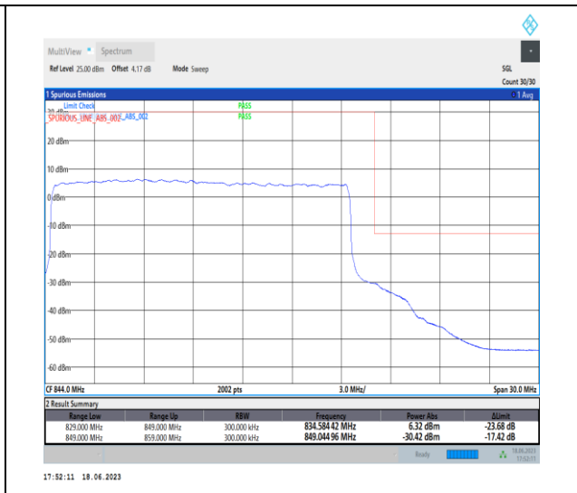
1-N5-PC3-15-20-H-3-DFT-PI2BPSK-Outer_Full-100@0-Ant0-1-seegraph-PASS-see graph
