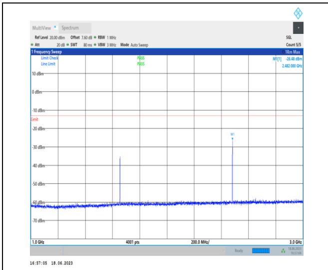
1-N5-PC3-15-20-M-1-DFT-PI2BPSK-Inner_1RB_Left -1 @ 1-1000-3000-Ant0-2482.00--26.48--13-PASS
