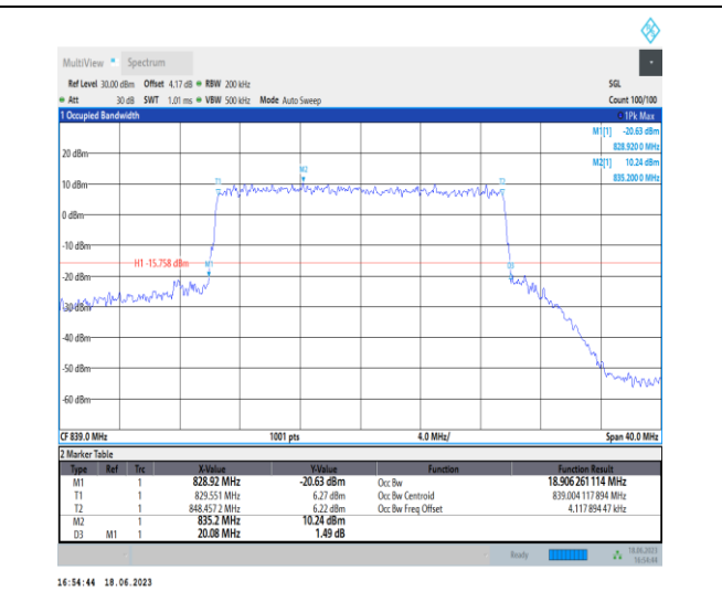
1-N5-PC3-15-20-H-7-CP-16QAM-Outer_Full-106@0-Ant0-18.906-20.080-<20-PASS
