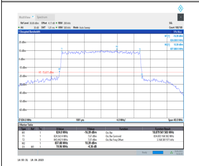
1-N5-PC3-15-20-L-6-CP-QPSK-Outer_Full-106@0- Ant0-18.88-19.960-≤20-PASS
