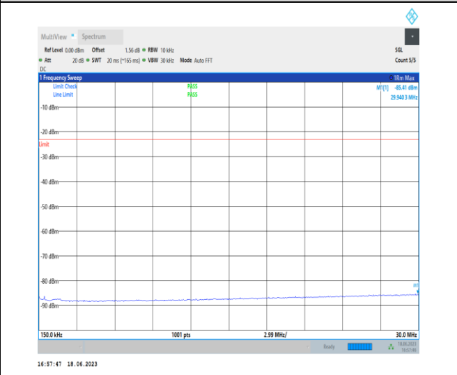
1-N5-PC3-15-20-H-1-DFT-PI2BPSK-Inner_1RB_Left -1 @ 1-0.15-30-Ant0-29.94--85.41--23-PASS
