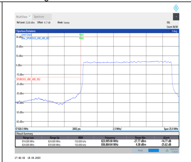
1-N5-PC3-15-15-L-3-DFT-PI2BPSK-Outer_Full-75 @0-Ant0-1-seegraph-PASS-see graph
