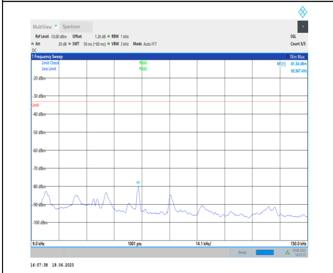
1-N5-PC3-15-20-H-1-DFT-PI2BPSK-Inner_1RB_Left -1 @ 1-0.009-0.15-Ant0-0.06--81.34--33-PASS
