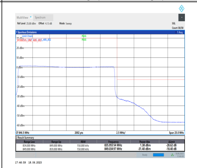
1-N5-PC3-15-15-H-6-CP-QPSK-Outer_Full-79@0- Ant0-1-seegraph-PASS-see graph
