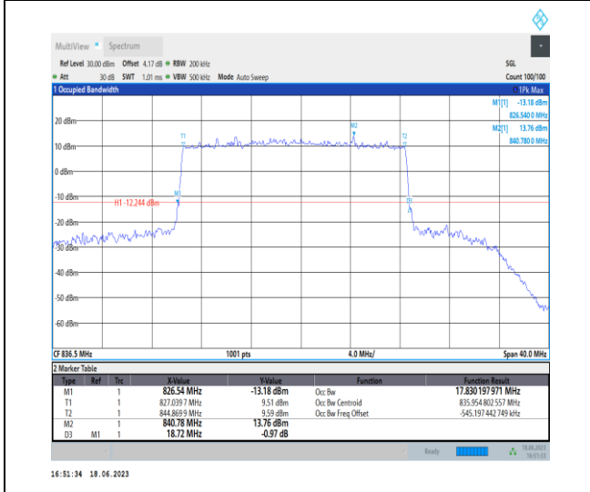
1-N5-PC3-15-20-M-1-DFT-QPSK-Outer_Full-100@0-Ant0-17.83-18.720-≤20-PASS
