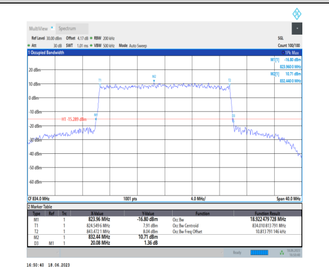
1-N5-PC3-15-20-L-7-CP-16QAM-Outer_Full-106@0- Ant0-18.922-20.080-≤20-PASS
