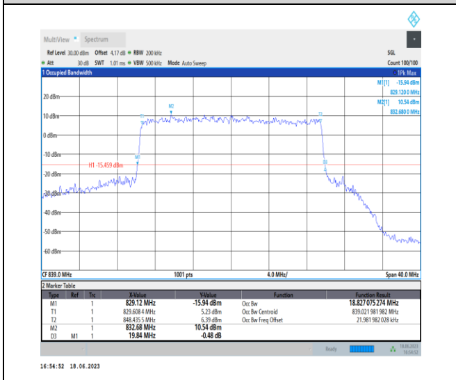
1-N5-PC3-15-20-H-8-CP-64QAM-Outer_Full-106@0-Ant0-18.827-19.840-<20-PASS
