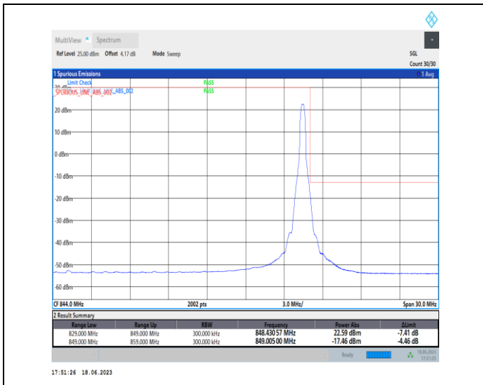
1-N5-PC3-15-20-H-2-DFT-PI2BPSK-Edge_1RB_Right-1@105-Ant0-1-seegraph-PASS-see graph
