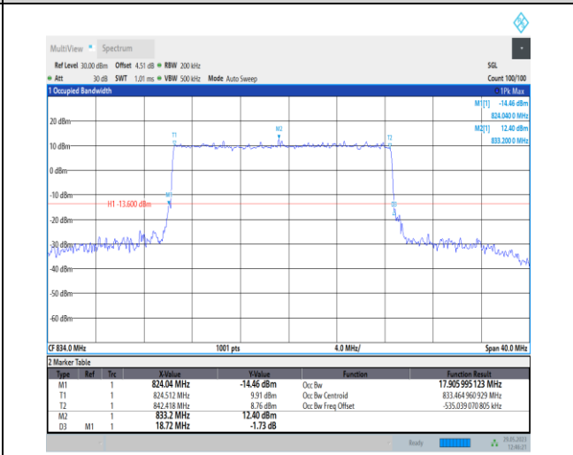
1-N5-PC3-15-20-L-1-DFT-QPSK-Outer_Full-100@0-Ant0-17.823-18.760-≤20-PASS
