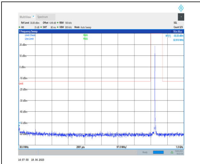
1-N5-PC3-15-20-H-1-DFT-PI2BPSK-Inner_1RB_Left -1 @ 1-30-1000-Ant0-32.91--53.33--13-PASS
