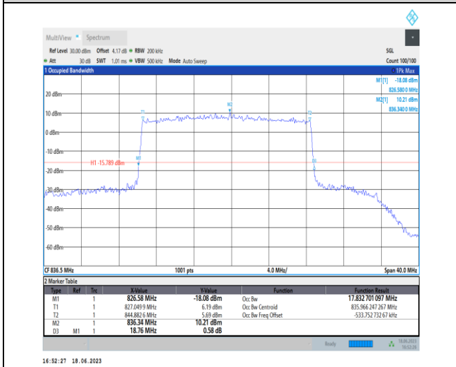
1-N5-PC3-15-20-M-5-DFT-256QAM-Outer_Full-100 @0-Ant0-17.833-18.760-<20-PASS
