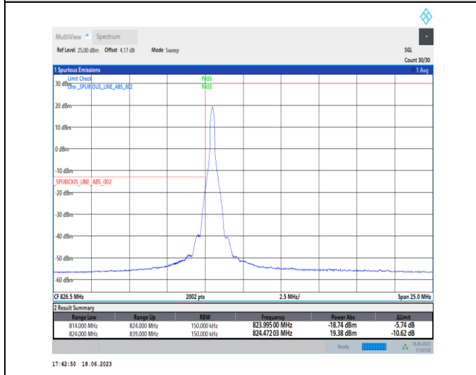
1-N5-PC3-15-15-L-4-CP-QPSK-Edge_1RB_Left-1@0-Ant0-1-seegraph-PASS-see graph
