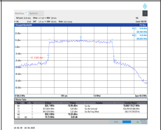
1-N5-PC3-15-20-M-6-CP-QPSK-Outer_Full-106@0- Ant0-18.86-19.720-<20-PASS
