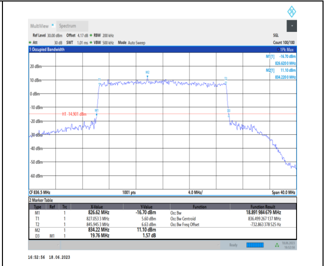
1-N5-PC3-15-20-M-8-CP-64QAM-Outer_Full-106@0 0-Ant0-18.892-19.760-≤20-PASS
