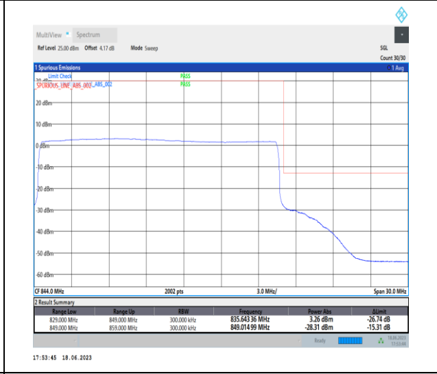
1-N5-PC3-15-20-H-6-CP-QPSK-Outer_Full-106@0-Ant0-1-seegraph-PASS-see graph
