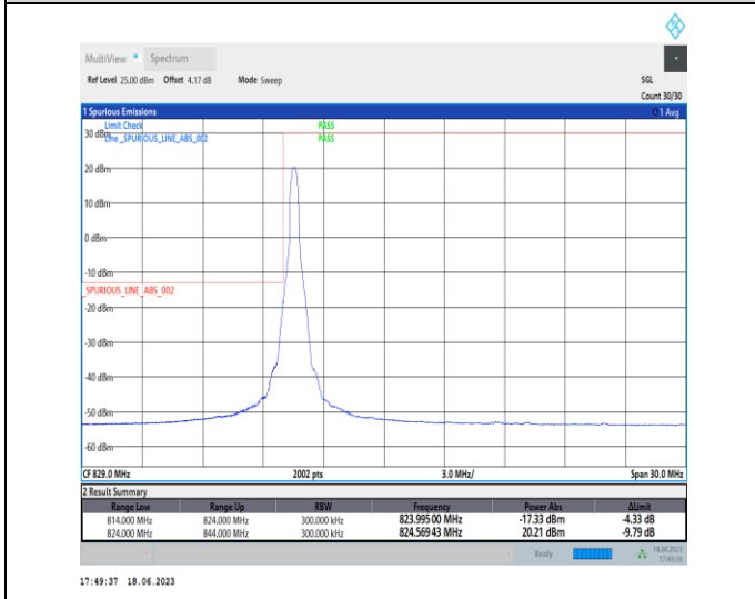
1-N5-PC3-15-20-L-4-CP-QPSK-Edge_1RB_Left-1@0-Ant0-1-seegraph-PASS-see graph
