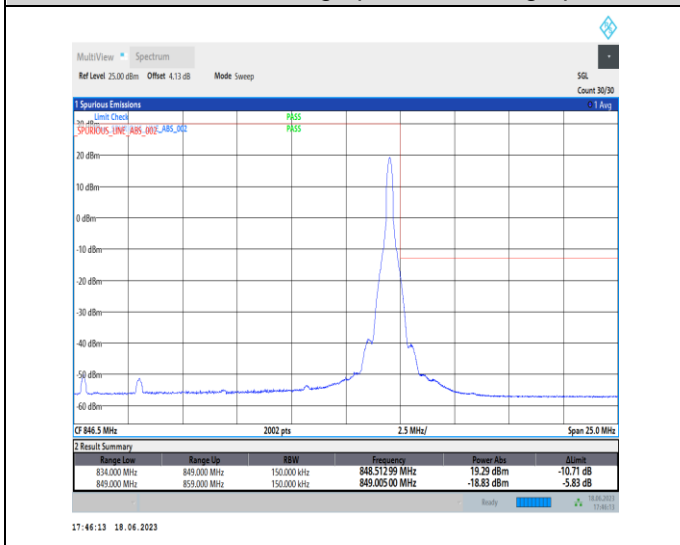
1-N5-PC3-15-15-H-5-CP-QPSK-Edge_1RB_Right-1@ 78-Ant0-1-seegraph-PASS-see graph
