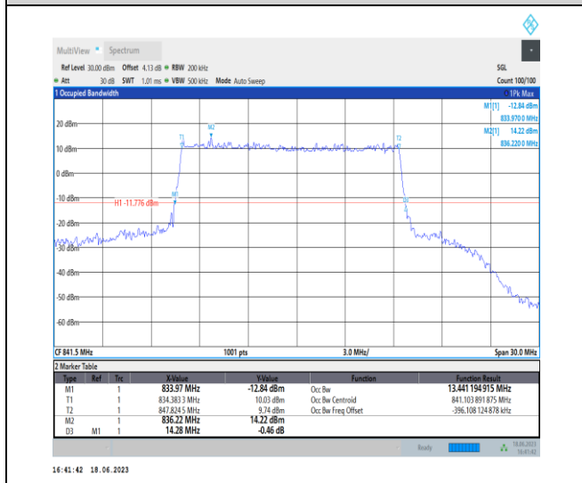
1-N5-PC3-15-15-H-3-DFT-16QAM-Outer_Full-75@0-Ant0-13.441-14.280-≤15-PASS
