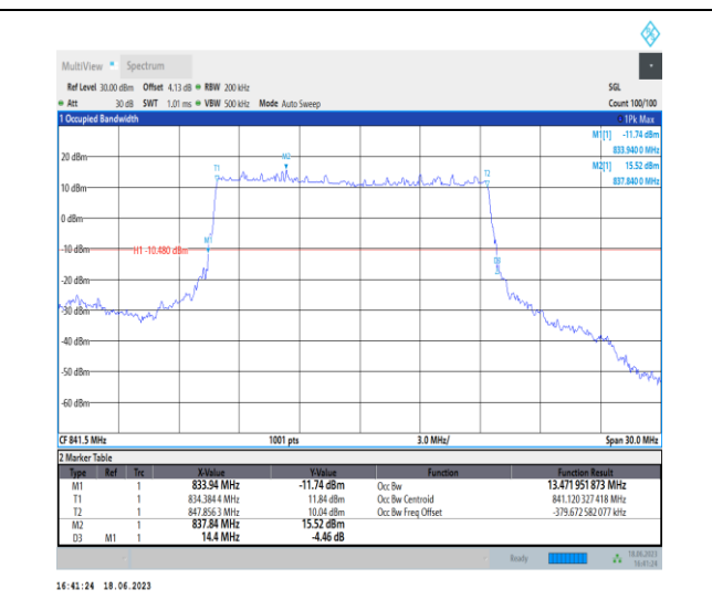
1-N5-PC3-15-15-H-2-DFT-PI2BPSK-Outer_Full-75@0-Ant0-13.472-14.400-≤15-PASS
