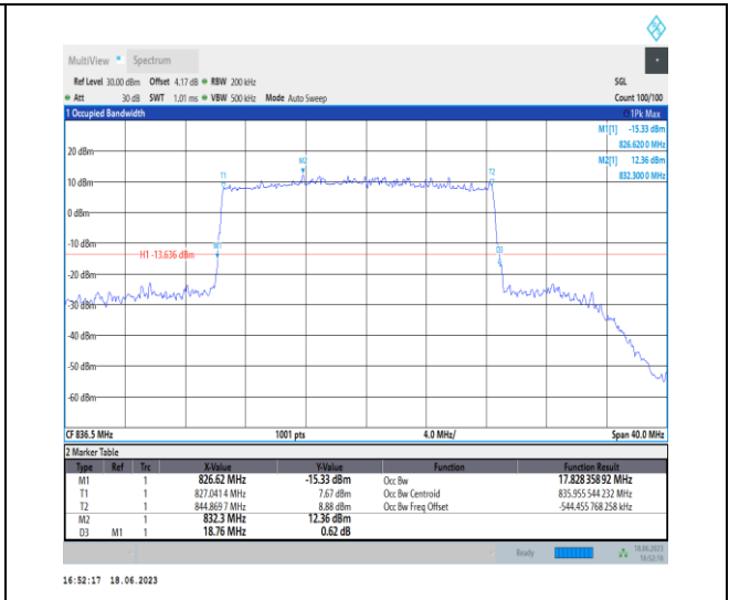
1-N5-PC3-15-20-M-4-DFT-64QAM-Outer_Full-100@ 0-Ant0-17.828-18.760-<20-PASS
