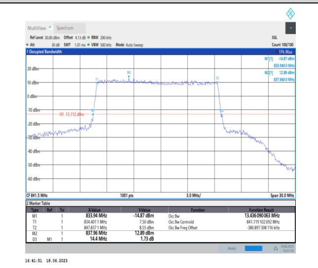
1-N5-PC3-15-15-H-4-DFT-64QAM-Outer_Full-75@0-Ant0-13.436-14.400-≤15-PASS
