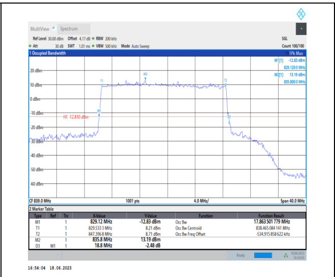
1-N5-PC3-15-20-H-3-DFT-16QAM-Outer_Full-100 @ 0-Ant0-17.864-18.800-<=20-PASS
