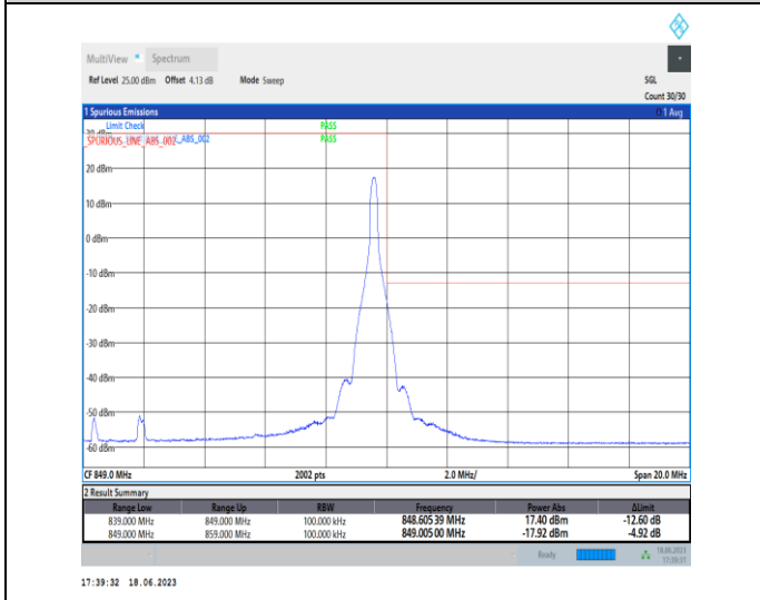
1-N5-PC3-15-10-H-5-CP-QPSK-Edge_1RB_Right-1@51-Ant0-1-seegraph-PASS-see graph
