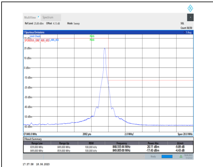
1-N5-PC3-15-10-H-2-DFT-PI2BPSK-Edge_1RB_Right-1@51-Ant0-1-seegraph-PASS-see graph
