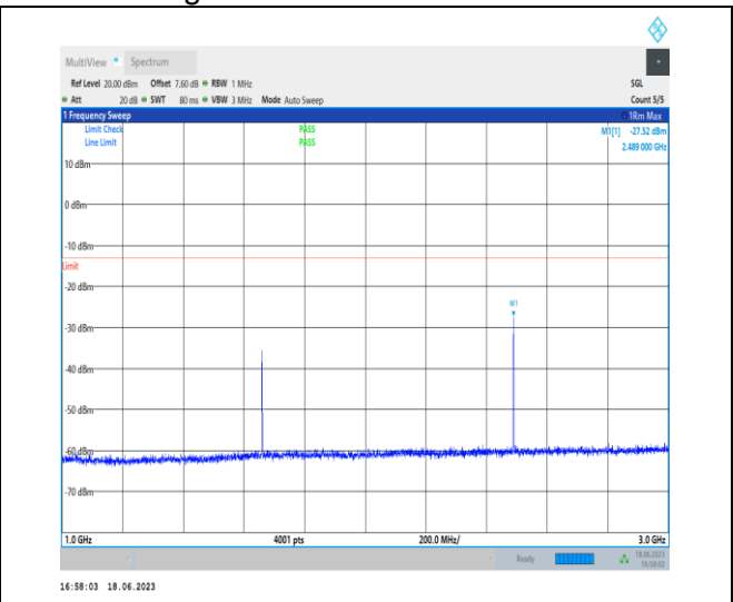
1-N5-PC3-15-20-H-1-DFT-PI2BPSK-Inner_1RB_Left -1 @ 1-1000-3000-Ant0-2489.00--27.52--13-PASS
