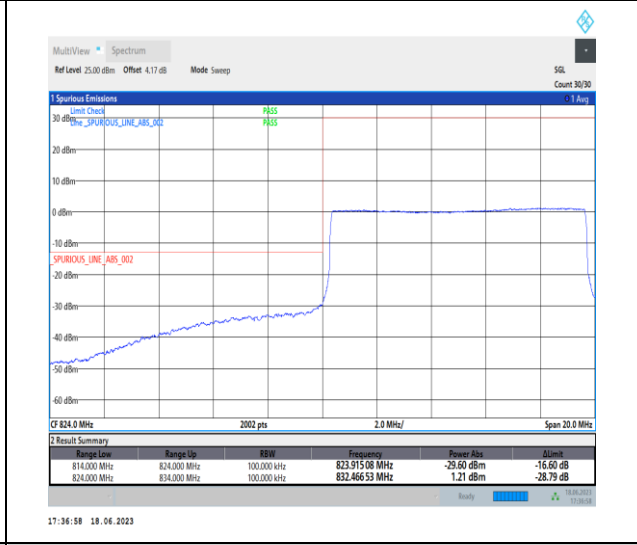
1-N5-PC3-15-10-L-6-CP-QPSK-Outer_Full-52 @0-Ant0-1-seegraph-PASS-see graph
