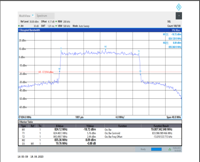
1-N5-PC3-15-20-L-9-CP-256QAM-Outer_Full-106@0-Ant0-19.007-19.760-≤20-PASS
