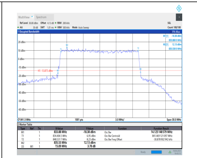
1-N5-PC3-15-15-H-6-CP-QPSK-Outer_Full-79@0-Ant0-14.125-15.090-≤15-PASS
