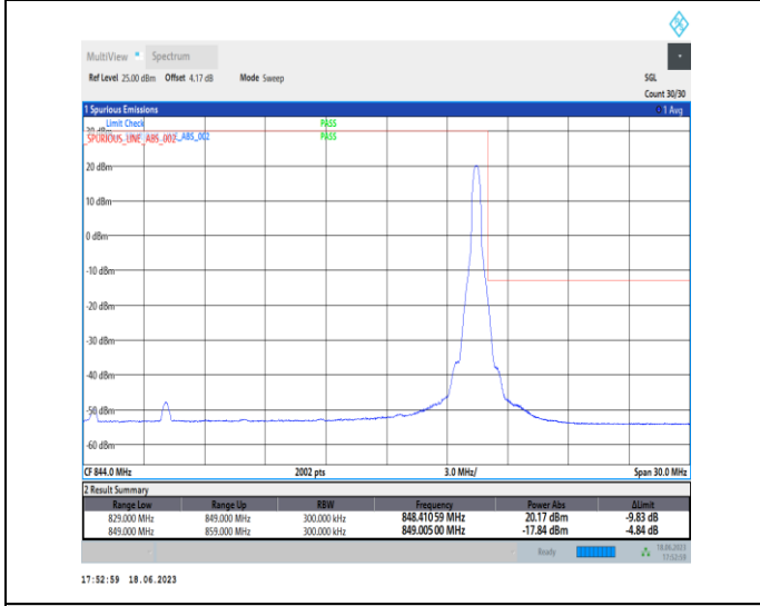
1-N5-PC3-15-20-H-5-CP-QPSK-Edge_1RB_Right-1@105-Ant0-1-seegraph-PASS-see graph
