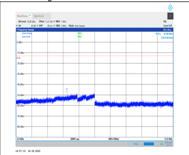
1-N5-PC3-15-20-M-1-DFT-PI2BPSK-Inner_1RB_Left -1 @ 1-3000-12000-Ant0-5918.70--47.88--13-PASS
