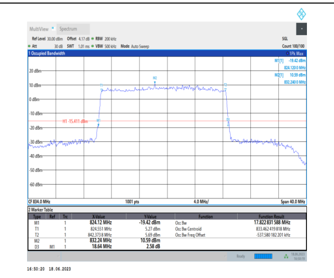
1-N5-PC3-15-20-L-5-DFT-256QAM-Outer_Full-100@ 0-Ant0-17.823-18.640-≤20-PASS
