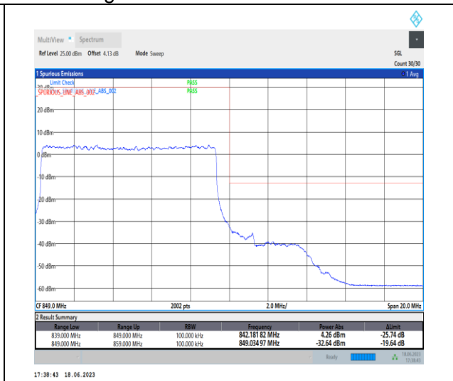
1-N5-PC3-15-10-H-3-DFT-PI2BPSK-Outer_Full-50@0-Ant0-1-seegraph-PASS-see graph
