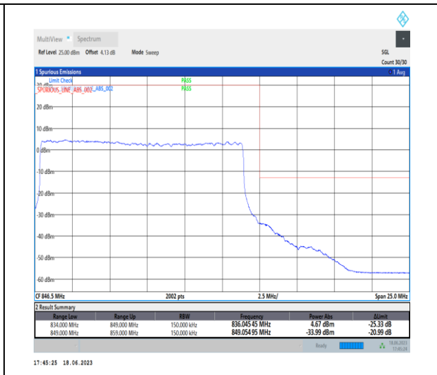
1-N5-PC3-15-15-H-3-DFT-PI2BPSK-Outer_Full-75 @0-Ant0-1-seegraph-PASS-see graph
