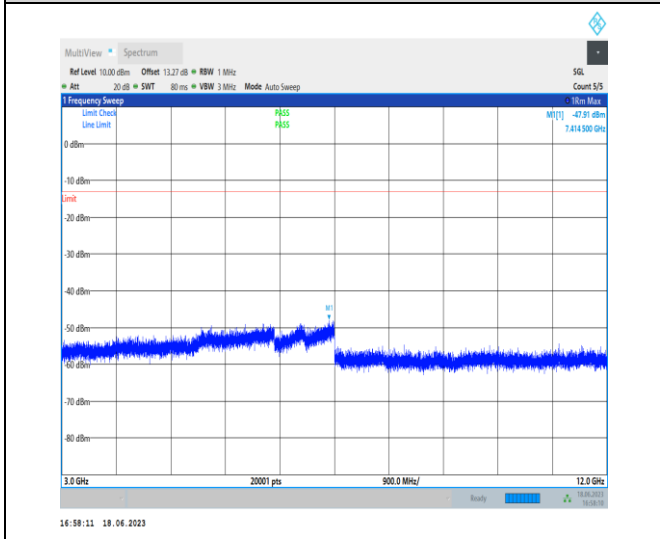
1-N5-PC3-15-20-H-1-DFT-PI2BPSK-Inner_1RB_Left -1 @ 1-3000-12000-Ant0-7414.50--47.91--13-PASS
