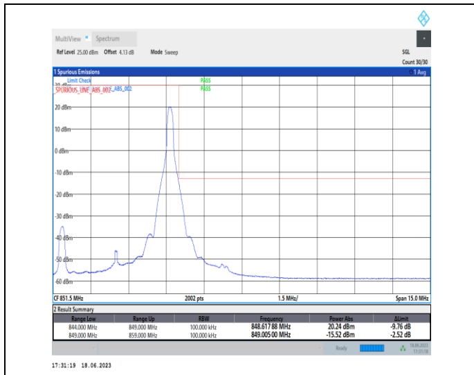
1-N5-PC3-15-5-H-2-DFT-PI2BPSK-Edge_1RB_Right-1 @24-Ant0-1-seegraph-PASS-see graph
