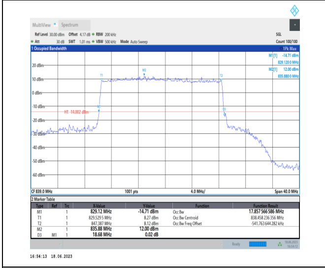
1-N5-PC3-15-20-H-4-DFT-64QAM-Outer_Full-100 @ 0-Ant0-17.858-18.680-<=20-PASS
