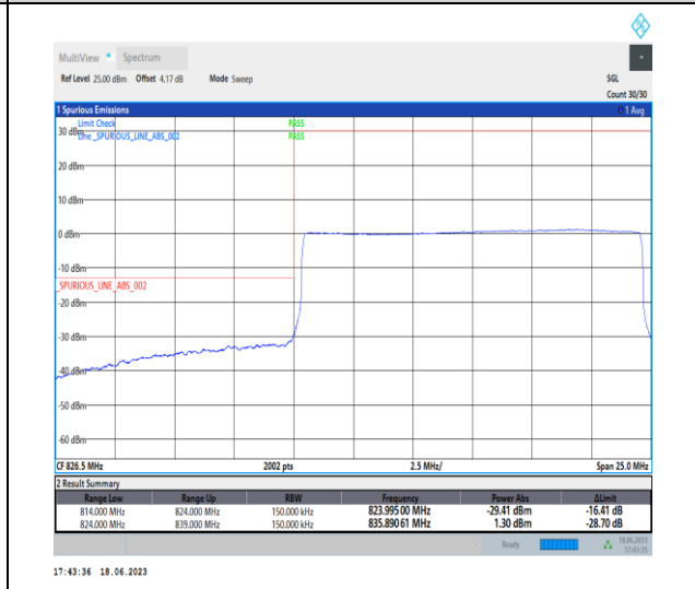
1-N5-PC3-15-15-L-6-CP-QPSK-Outer_Full-79@0-Ant0-1-seegraph-PASS-see graph
