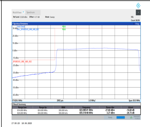
1-N5-PC3-15-20-L-6-CP-QPSK-Outer_Full-106@0-Ant0-1-seegraph-PASS-see graph
