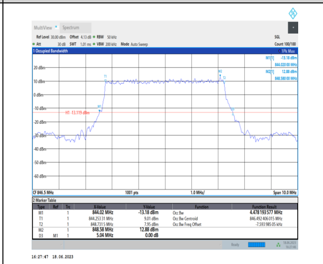
1-N5-PC3-15-5-H-2-DFT-PI2BPSK-Outer_Full-25@0-A Ant0-4.478-5.040<math>\leq 5</math>-PASS
