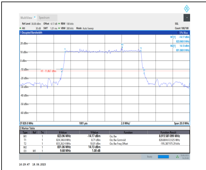
1-N5-PC3-15-10-L-2-DFT-PI2BPSK-Outer_Full-50@ 0-Ant0-8.916-9.680-<=10-PASS
