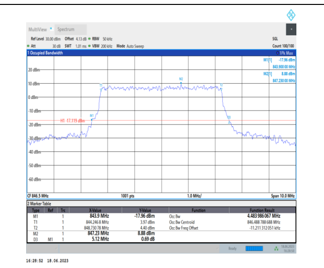
1-N5-PC3-15-5-H-8-CP-64QAM-Outer_Full-25@0-A nt0-4.484-5.120-≤5-PASS
