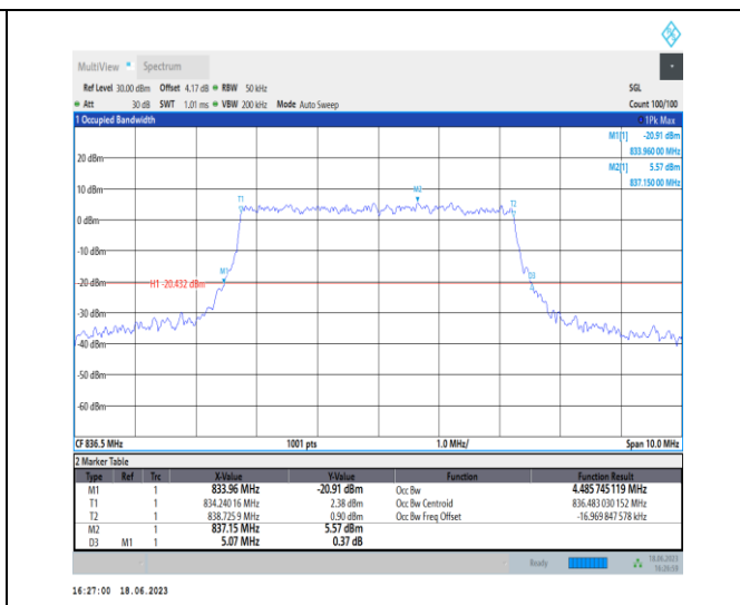
1-N5-PC3-15-5-M-9-CP-256QAM-Outer_Full-25@0-A nt0-4.486-5.070<math>\leq 5</math>-PASS
