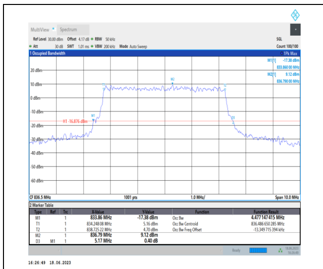
1-N5-PC3-15-5-M-8-CP-64QAM-Outer_Full-25@0-A Ant0-4.477-5.170<math>\leq 5</math>-PASS
