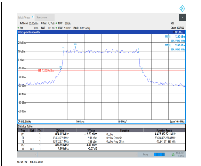
1-N5-PC3-15-5-M-1-DFT-QPSK-Outer_Full-25@0-A Ant0-4.477-4.880-≤5-PASS
