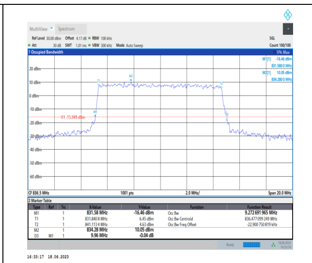
1-N5-PC3-15-10-M-6-CP-QPSK-Outer_Full-52@0- Ant0-9.273-9.960-≤10-PASS
