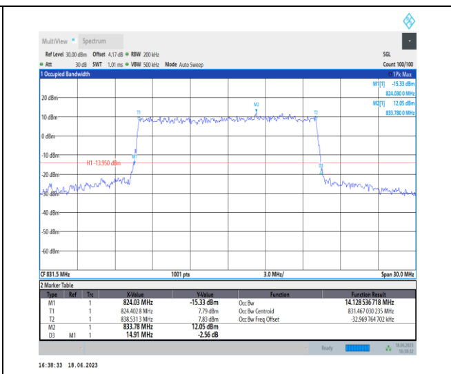
1-N5-PC3-15-15-L-8-CP-64QAM-Outer_Full-79@0- Ant0-14.129-14.910-≤15-PASS
