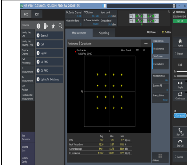
1-N5-PC3-15-20-M-7-CP-16QAM-Outer_Full-106@0-Ant0-see graph-PASS
