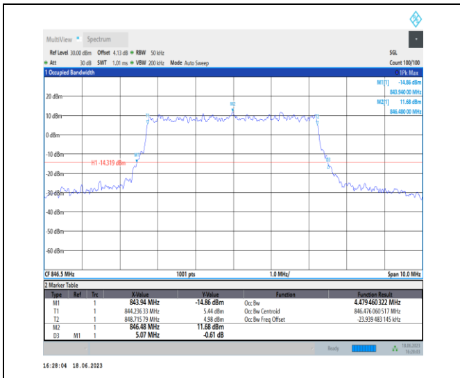
1-N5-PC3-15-5-H-3-DFT-16QAM-Outer_Full-25@0-A Ant0-4.479-5.070-≤5-PASS
