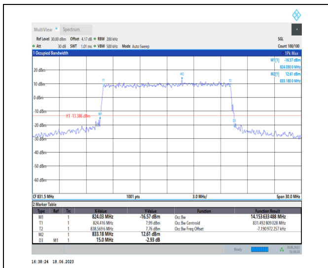
1-N5-PC3-15-15-L-7-CP-16QAM-Outer_Full-79@0-A Ant0-14.154-15.000-≤15-PASS
