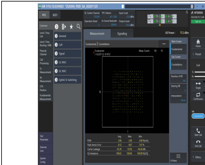
1-N5-PC3-15-20-M-9-CP-256QAM-Outer_Full-106@0-Ant0-see graph-PASS
