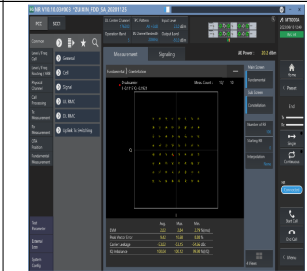
1-N5-PC3-15-20-M-8-CP-64QAM-Outer_Full-106@0-Ant0-see graph-PASS
