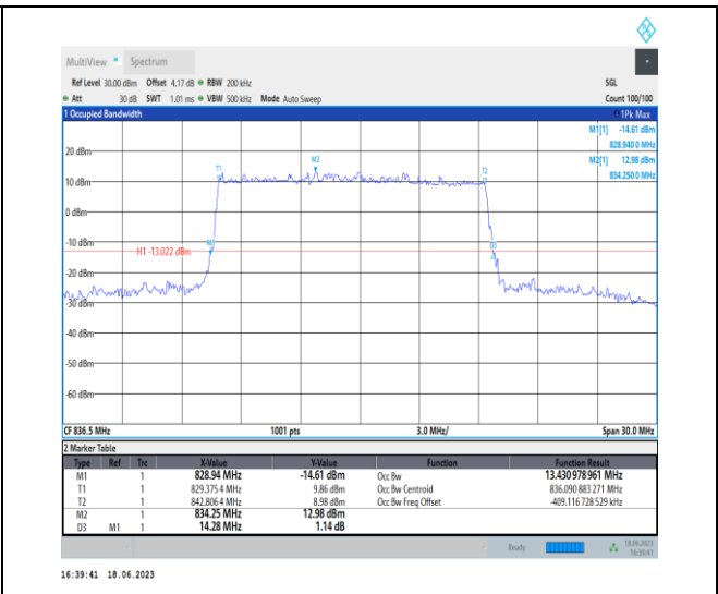
1-N5-PC3-15-15-M-3-DFT-16QAM-Outer_Full-75@0 -Ant0-13.431-14.280≤15-PASS
