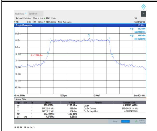
1-N5-PC3-15-5-H-1-DFT-QPSK-Outer_Full-25@0-A nt0-4.469-4.870<math>\leq 5</math>-PASS
