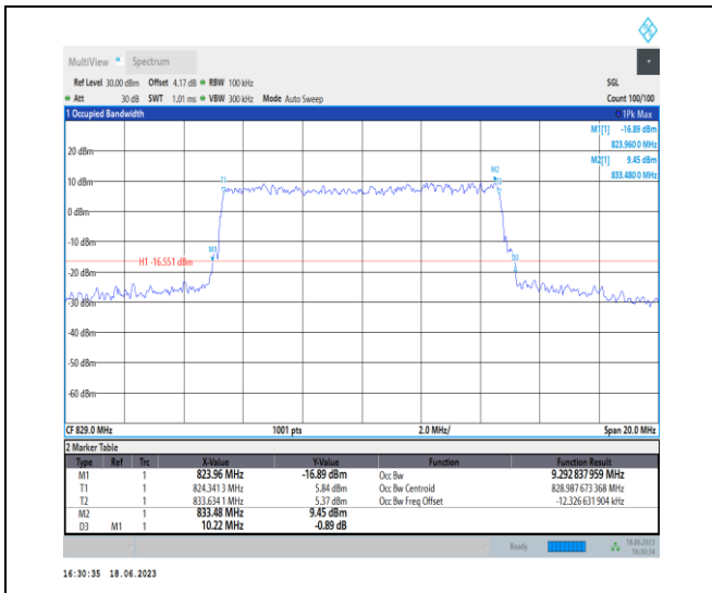
1-N5-PC3-15-10-L-6-CP-QPSK-Outer_Full-52@0-A Ant0-9.293-10.220-≤10-PASS
