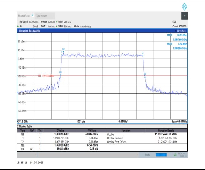
1-N2-PC3-15-20-H-9-CP-256QAM-Outer_Full-106@0-Ant3-19.011-19.840-<=20-PASS
