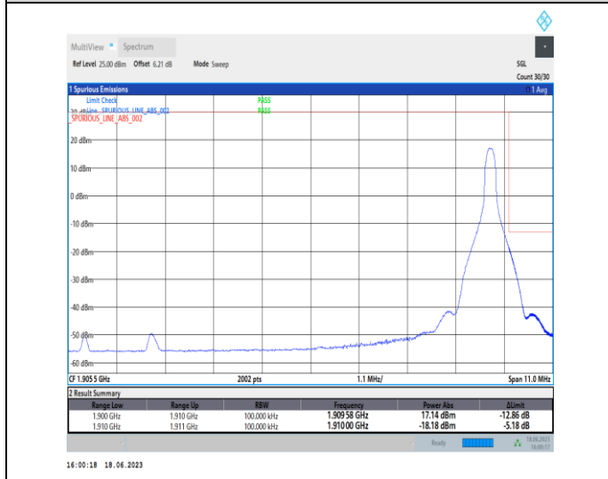
1-N2-PC3-15-10-H-5-CP-QPSK-Edge_1RB_Right-1@51-Ant3-1-seegraph-PASS-see graph
