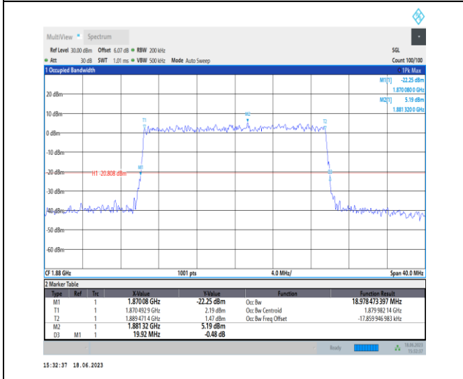
1-N2-PC3-15-20-M-9-CP-256QAM-Outer_Full-106@0 -Ant3-18.978-19.920-≤20-PASS
