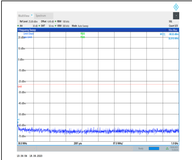
1-N2-PC3-15-20-M-1-DFT-PI2BPSK-Inner_1RB_Left-t-1 @ 1-30-1000-Ant3-32.91--58.32--23-PASS
