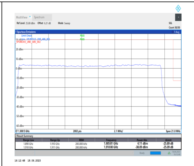
1-N2-PC3-15-20-H-3-DFT-PI2BPSK-Outer_Full-100@0-Ant3-1-seegraph-PASS-see graph
