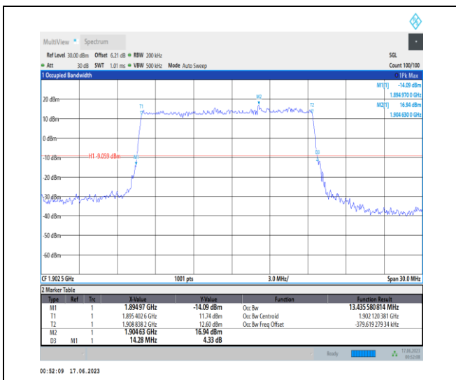
1-N2-PC3-15-15-H-1-DFT-QPSK-Outer_Full-75@0-Ant3-13.436-14.280≤15-PASS
