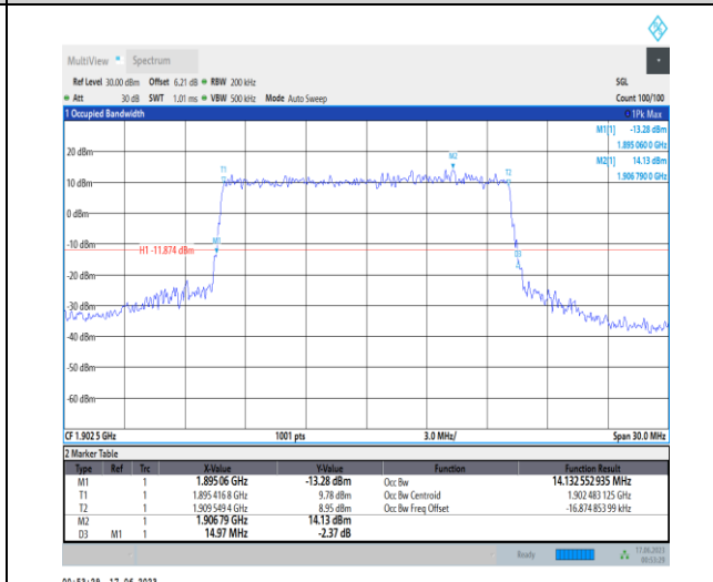
1-N2-PC3-15-15-H-8-CP-64QAM-Outer_Full-79@0-A Ant3-14.133-14.970-≤15-PASS
