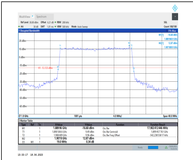
1-N2-PC3-15-20-H-2-DFT-PI2BPSK-Outer_Full-100@0-Ant3-17.902-19.000-<=20-PASS
