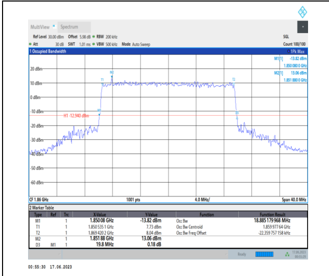
1-N2-PC3-15-20-L-8-CP-64QAM-Outer_Full-106@ 0-Ant3-18.885-19.800-≤20-PASS
