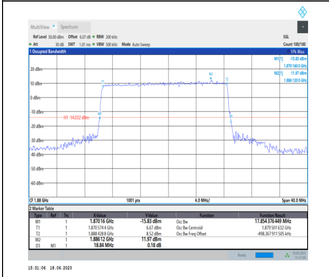
1-N2-PC3-15-20-M-1-DFT-QPSK-Outer_Full-100@ 0-Ant3-17.854-18.840-≤20-PASS
