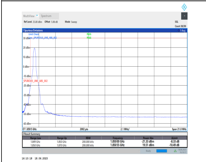
1-N2-PC3-15-20-L-4-CP-QPSK-Edge_1RB_Left-1@0-Ant3-1-seegraph-PASS-see graph
