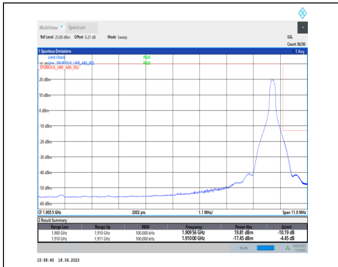
1-N2-PC3-15-10-H-2-DFT-PI2BPSK-Edge_1RB_Right-1@51-Ant3-1-seegraph-PASS-see graph
