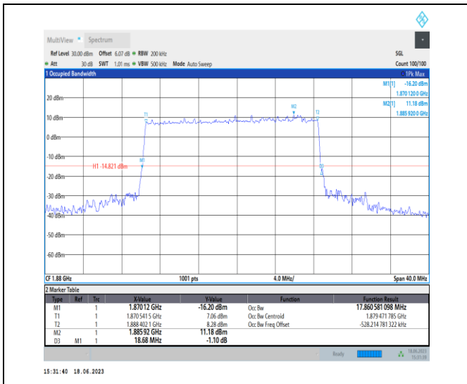
1-N2-PC3-15-20-M-3-DFT-16QAM-Outer_Full-100@ 0-Ant3-17.861-18.680-≤20-PASS
