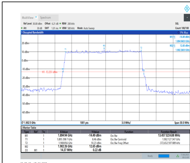
1-N2-PC3-15-15-H-5-DFT-256QAM-Outer_Full-75@0-A -Ant3-13.457-14.370-≤15-PASS
