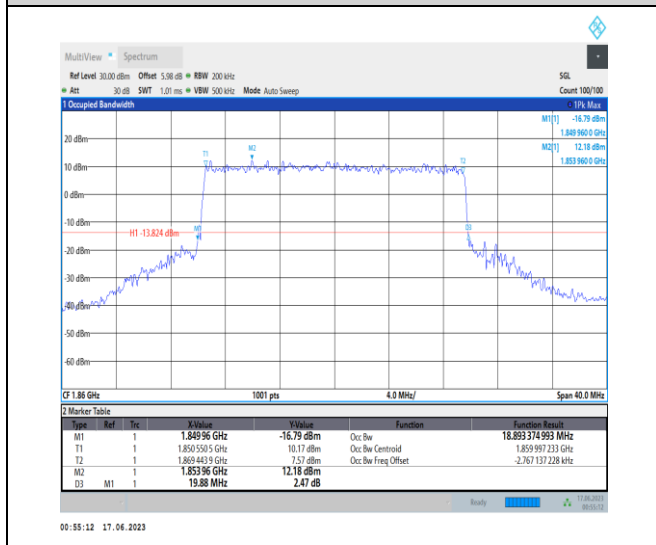
1-N2-PC3-15-20-L-6-CP-QPSK-Outer_Full-106@0- Ant3-18.893-19.880-≤20-PASS
