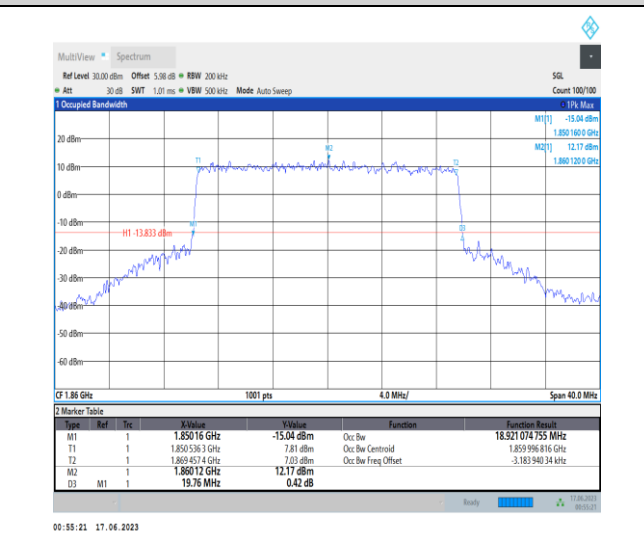
1-N2-PC3-15-20-L-7-CP-16QAM-Outer_Full-106@0- Ant3-18.921-19.760-≤20-PASS
