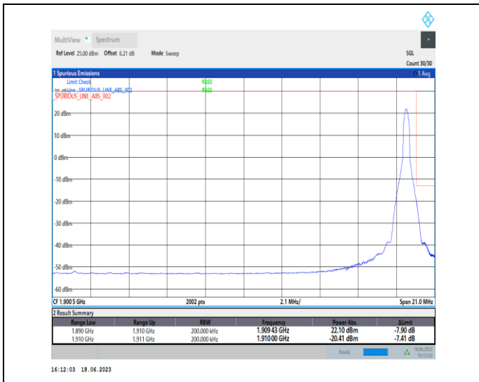
1-N2-PC3-15-20-H-2-DFT-PI2BPSK-Edge_1RB_Right-1@105-Ant3-1-seegraph-PASS-see graph
