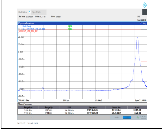
1-N2-PC3-15-20-H-5-CP-QPSK-Edge_1RB_Right-1@105-Ant3-1-seegraph-PASS-see graph
