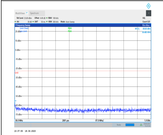
1-N2-PC3-15-20-H-1-DFT-PI2BPSK-Inner_1RB_Lef t-1@1-30-1000-Ant3-30.49--58.65--23-PASS
