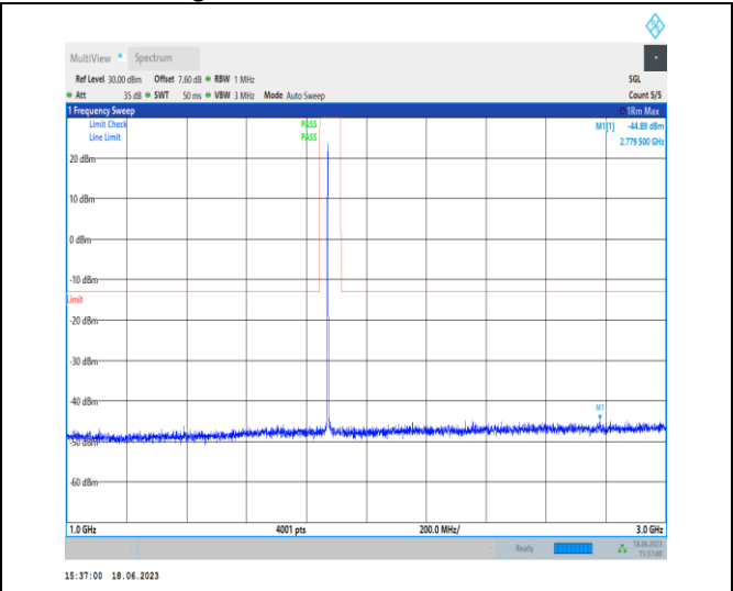
1-N2-PC3-15-20-M-1-DFT-PI2BPSK-Inner_1RB_Left-1 @ 1-1000-3000-Ant3-2779.50--44.89--13-PASS
