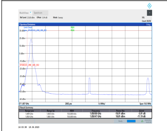
1-N2-PC3-15-15-L-4-CP-QPSK-Edge_1RB_Left-1@0-Ant3-1-seegraph-PASS-see graph
