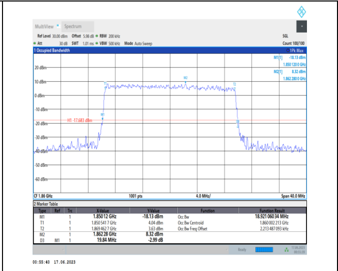
1-N2-PC3-15-20-L-9-CP-256QAM-Outer_Full-106@0 -Ant3-18.921-19.840-≤20-PASS
