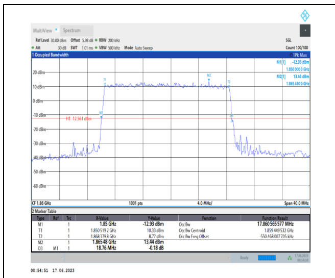
1-N2-PC3-15-20-L-4-DFT-64QAM-Outer_Full-100@ 0-Ant3-17.861-18.760-≤20-PASS
