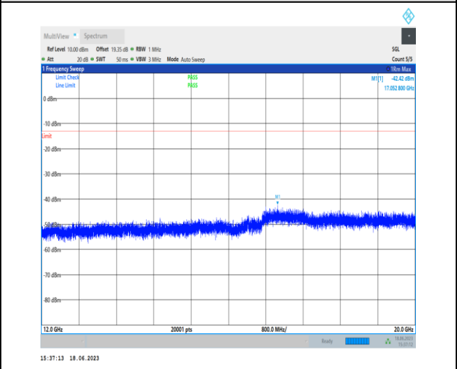
1-N2-PC3-15-20-M-1-DFT-PI2BPSK-Inner_1RB_Left-1 @ 1-12000-20000-Ant3-17052.80--42.42--13-PASS
