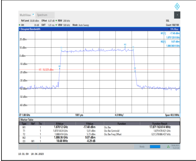
1-N2-PC3-15-20-M-5-DFT-256QAM-Outer_Full-100 @0-Ant3-17.871-18.680-≤20-PASS
