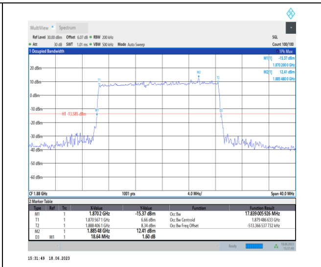
1-N2-PC3-15-20-M-4-DFT-64QAM-Outer_Full-100@ 0-Ant3-17.839-18.640-≤20-PASS
