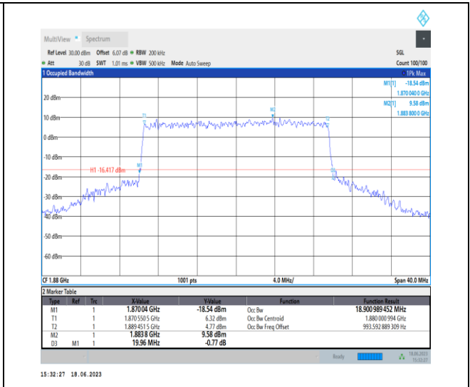
1-N2-PC3-15-20-M-8-CP-64QAM-Outer_Full-106@0 -Ant3-18.901-19.960-≤20-PASS
