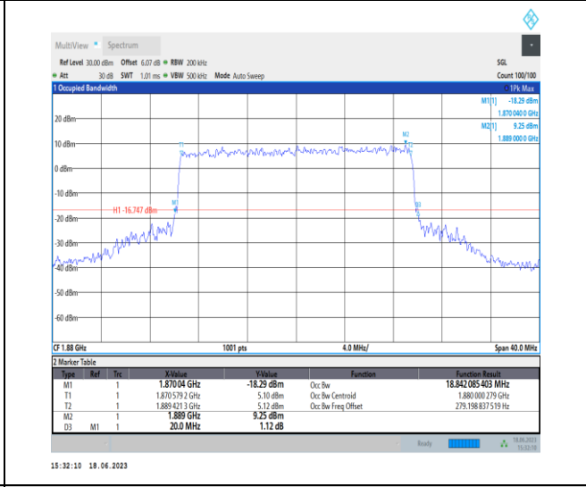
1-N2-PC3-15-20-M-6-CP-QPSK-Outer_Full-106@0- Ant3-18.842-20.000-≤20-PASS
