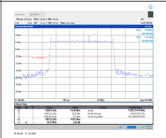
1-N2-PC3-15-20-L-3-DFT-16QAM-Outer_Full-100@0-Ant3-17.851-18.720-<=20-PASS
