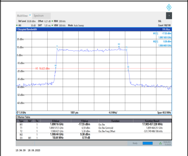
1-N2-PC3-15-20-H-5-DFT-256QAM-Outer_Full-100@0-Ant3-17.905-18.640-<=20-PASS
