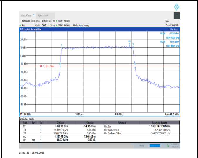
1-N2-PC3-15-20-M-2-DFT-PI2BPSK-Outer_Full-100 @0-Ant3-17.867-18.720-≤20-PASS
