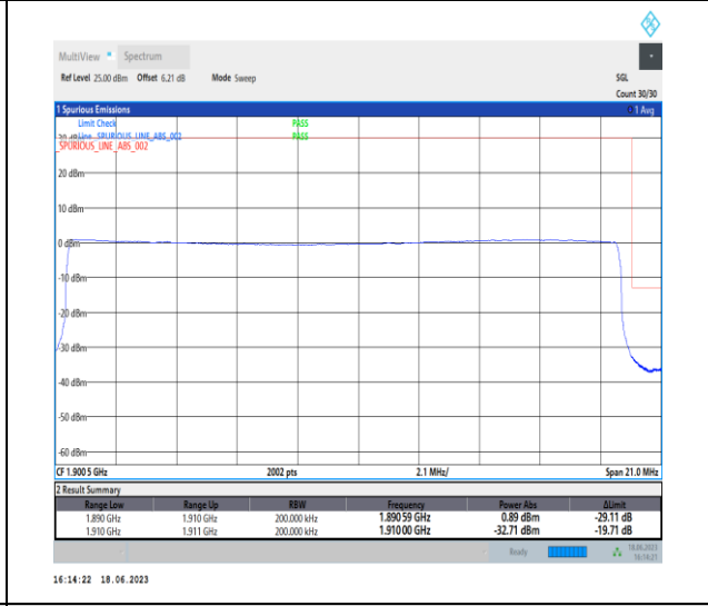
1-N2-PC3-15-20-H-6-CP-QPSK-Outer_Full-106@0-Ant3-1-seegraph-PASS-see graph
