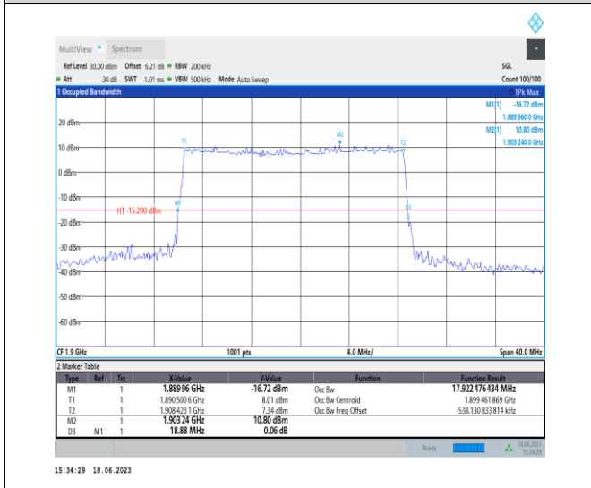
1-N2-PC3-15-20-H-4-DFT-64QAM-Outer_Full-100@0-Ant3-17.922-18.880-<=20-PASS
