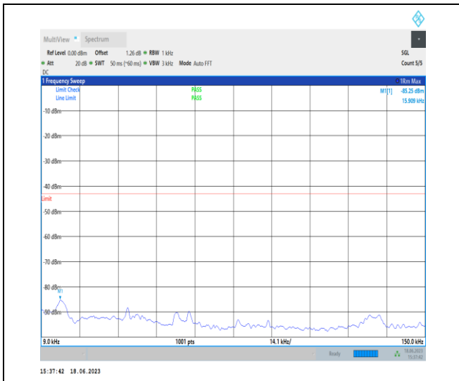
1-N2-PC3-15-20-H-1-DFT-PI2BPSK-Inner_1RB_Lef t-1@1-0.009-0.15-Ant3-0.02--85.25--43-PASS
