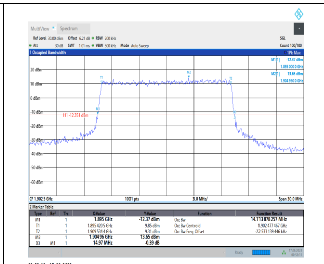
1-N2-PC3-15-15-H-6-CP-QPSK-Outer_Full-79@0-A Ant3-14.114-14.970-≤15-PASS
