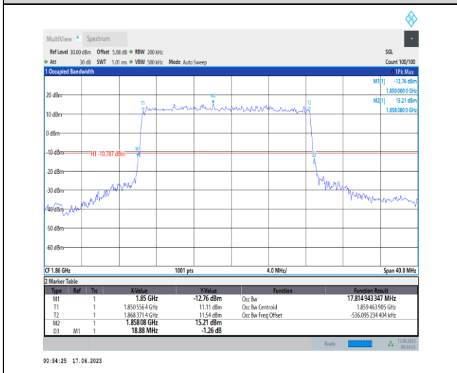
1-N2-PC3-15-20-L-2-DFT-PI2BPSK-Outer_Full-100@0-Ant3-17.815-18.880-<=20-PASS
