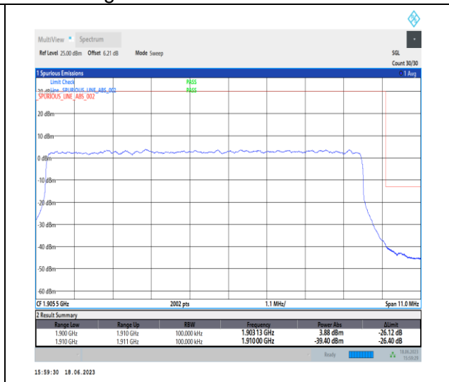
1-N2-PC3-15-10-H-3-DFT-PI2BPSK-Outer_Full-50@0-Ant3-1-seegraph-PASS-see graph
