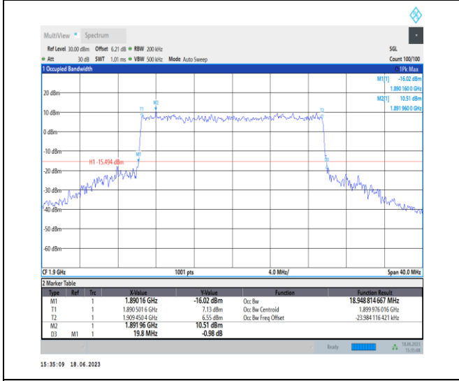
1-N2-PC3-15-20-H-8-CP-64QAM-Outer_Full-106@0-Ant3-18.949-19.800-<=20-PASS
