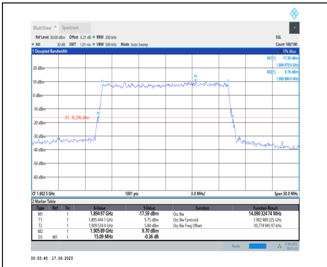
1-N2-PC3-15-15-H-9-CP-256QAM-Outer_Full-79@0-Ant3-14.09-15.090-<=15-PASS
