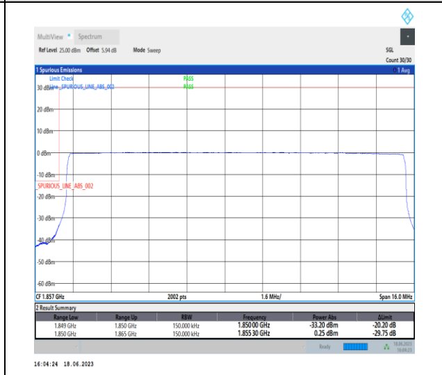
1-N2-PC3-15-15-L-6-CP-QPSK-Outer_Full-79@0-Ant3-1-seegraph-PASS-see graph
