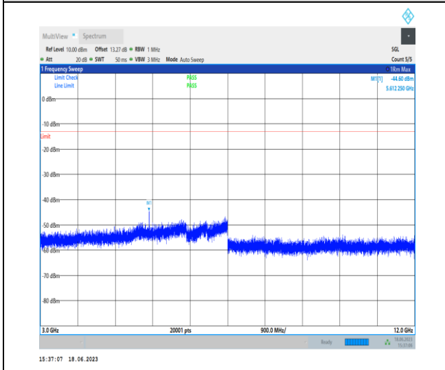
1-N2-PC3-15-20-M-1-DFT-PI2BPSK-Inner_1RB_Left-t-1 @ 1-3000-12000-Ant3-5612.25--44.60--13-PASS
