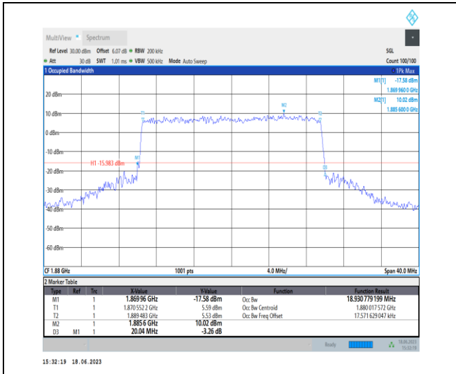
1-N2-PC3-15-20-M-7-CP-16QAM-Outer_Full-106@0 -Ant3-18.931-20.040-≤20-PASS
