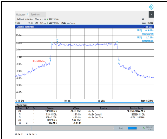
1-N2-PC3-15-20-H-6-CP-QPSK-Outer_Full-106@0-Ant3-18.898-19.840-<=20-PASS
