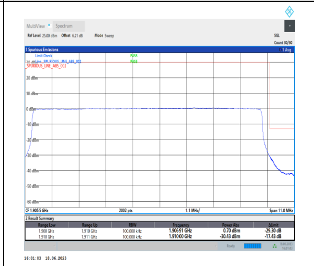
1-N2-PC3-15-10-H-6-CP-QPSK-Outer_Full-52@0-Ant3-1-seegraph-PASS-see graph
