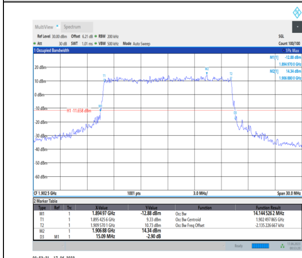
1-N2-PC3-15-15-H-7-CP-16QAM-Outer_Full-79@0-A Ant3-14.145-15.090-≤15-PASS
