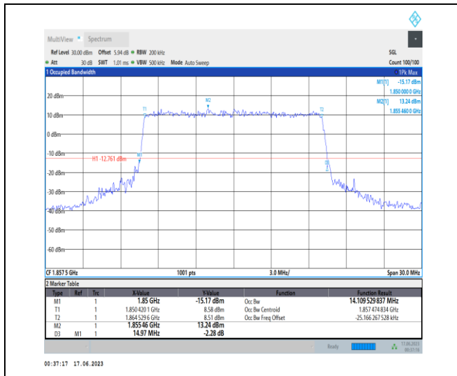
1-N2-PC3-15-15-L-7-CP-16QAM-Outer_Full-79@0-A Ant3-14.11-14.970≤15-PASS
