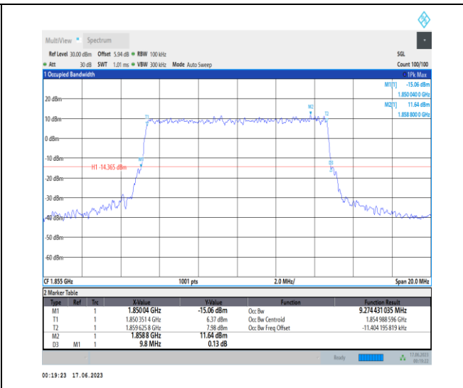
1-N2-PC3-15-10-L-7-CP-16QAM-Outer_Full-52@0-A Ant3-9.274-9.800-≤10-PASS
