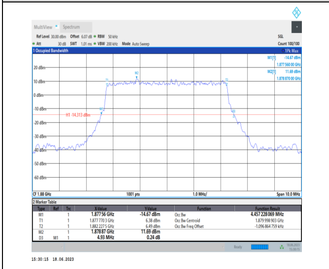
1-N2-PC3-15-5-M-2-DFT-PI2BPSK-Outer_Full-25@0 -Ant3-4.457-4.930-≤5-PASS
