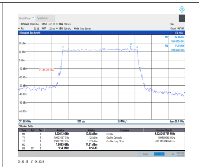
1-N2-PC3-15-10-H-1-DFT-QPSK-Outer_Full-50@0-Ant3-8.928-9.540-<=10-PASS
