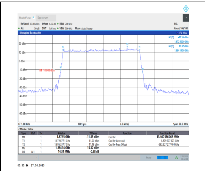
1-N2-PC3-15-15-M-3-DFT-16QAM-Outer_Full-75@0 -Ant3-13.461-14.340≤15-PASS
