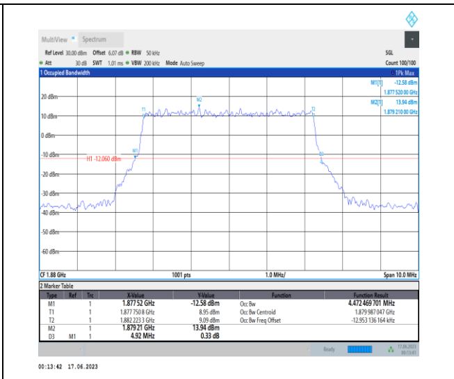
1-N2-PC3-15-5-M-1-DFT-QPSK-Outer_Full-25@0-A nt3-4.472-4.920-≤5-PASS
