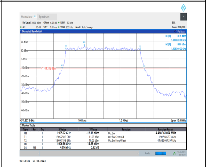
1-N2-PC3-15-5-H-2-DFT-PI2BPSK-Outer_Full-25@0-A Ant3-4.469-4.950-≤5-PASS
