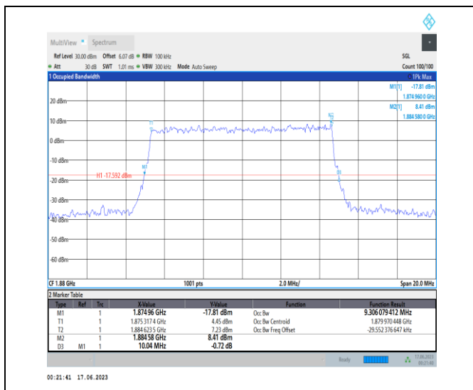
1-N2-PC3-15-10-M-9-CP-256QAM-Outer_Full-52@0-Ant3-9.306-10.040-<=10-PASS
