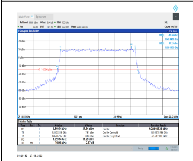
1-N2-PC3-15-10-L-8-CP-64QAM-Outer_Full-52@0-A Ant3-9.289-10.060-≤10-PASS
