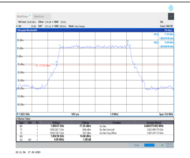
1-N2-PC3-15-5-L-2-DFT-PI2BPSK-Outer_Full-25@0 -Ant3-4.465-4.940-≤5-PASS
