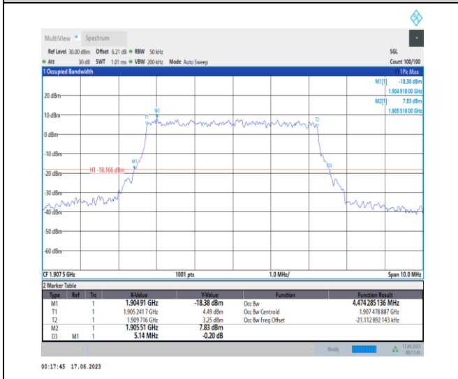
1-N2-PC3-15-5-H-9-CP-256QAM-Outer_Full-25@0-A Ant3-4.474-5.140-≤5-PASS
