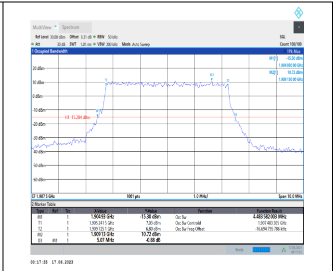
1-N2-PC3-15-5-H-8-CP-64QAM-Outer_Full-25@0-A nt3-4.484-5.070-≤5-PASS
