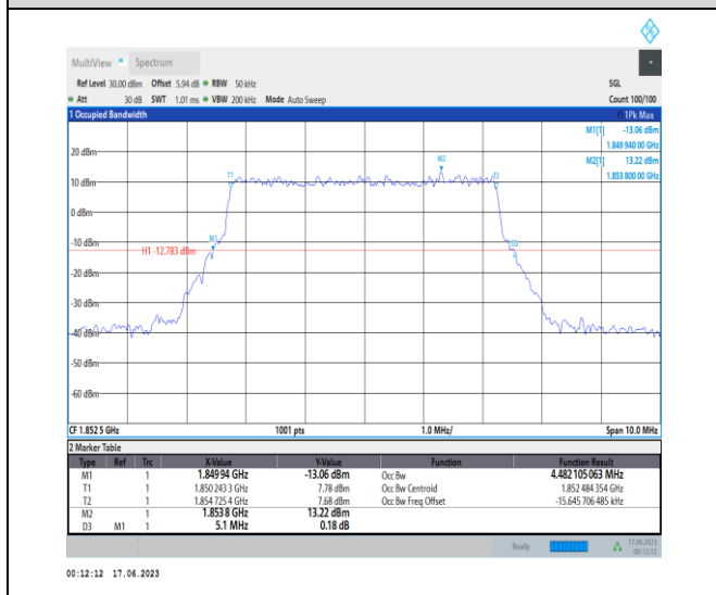
1-N2-PC3-15-5-L-3-DFT-16QAM-Outer_Full-25@0-Ant3-4.482-5.100-≤5-PASS
