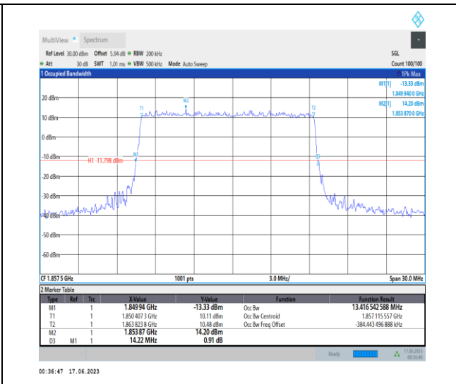
1-N2-PC3-15-15-L-4-DFT-64QAM-Outer_Full-75@0-Ant3-13.417-14.220-≤15-PASS
