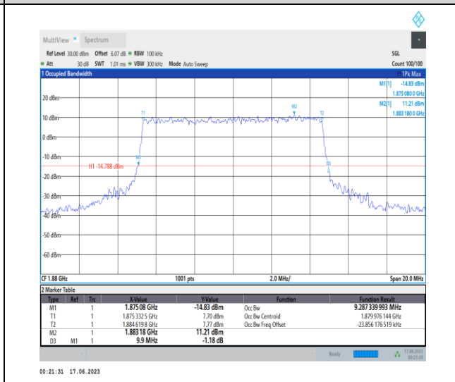
1-N2-PC3-15-10-M-8-CP-64QAM-Outer_Full-52@0- Ant3-9.287-9.900-≤10-PASS
