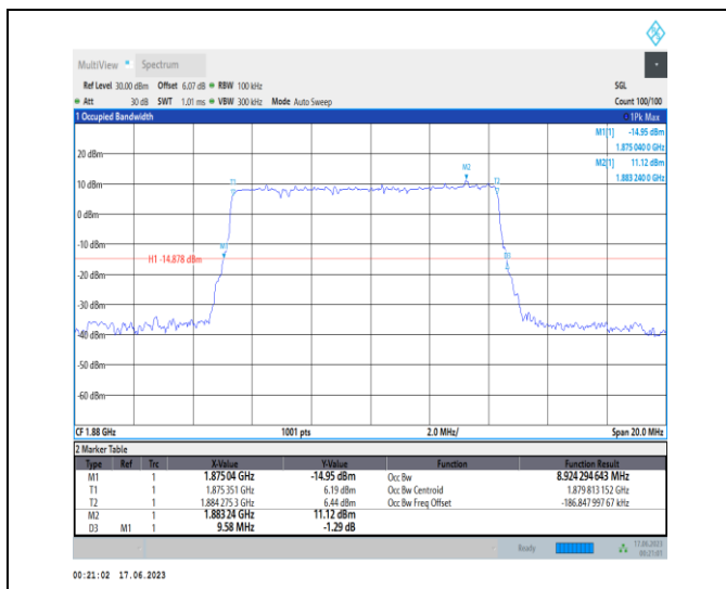
1-N2-PC3-15-10-M-5-DFT-256QAM-Outer_Full-50@ 0-Ant3-8.924-9.580-≤10-PASS
