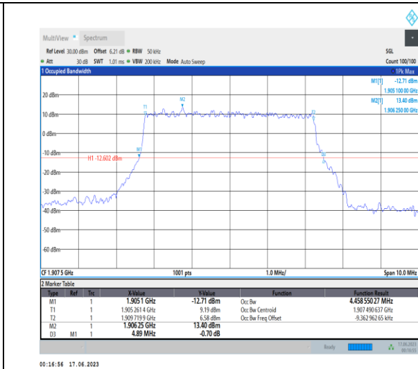
1-N2-PC3-15-5-H-4-DFT-64QAM-Outer_Full-25@0- Ant3-4.459-4.890-≤5-PASS
