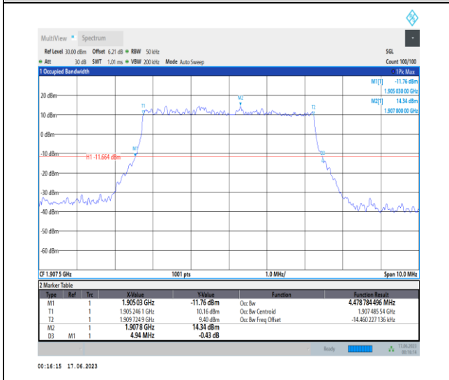
1-N2-PC3-15-5-H-1-DFT-QPSK-Outer_Full-25@0-A Ant3-4.479-4.940-≤5-PASS
