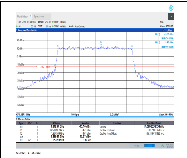
1-N2-PC3-15-15-L-8-CP-64QAM-Outer_Full-79@0- Ant3-14.09-15.090≤15-PASS
