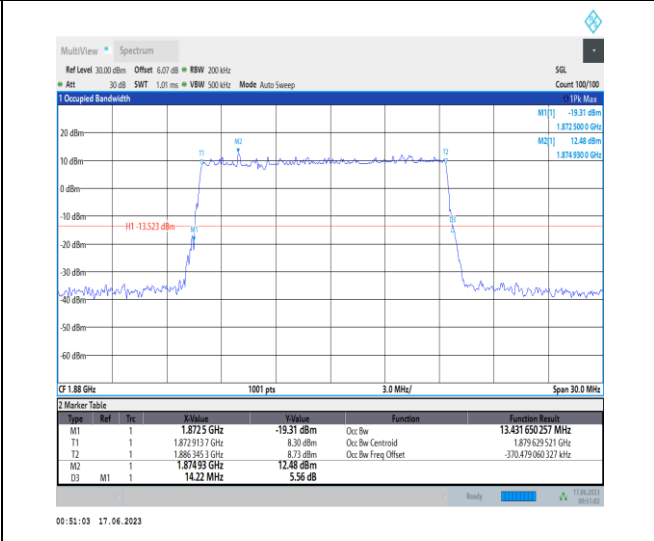
1-N2-PC3-15-15-M-5-DFT-256QAM-Outer_Full-75@ 0-Ant3-13.432-14.220≤15-PASS
