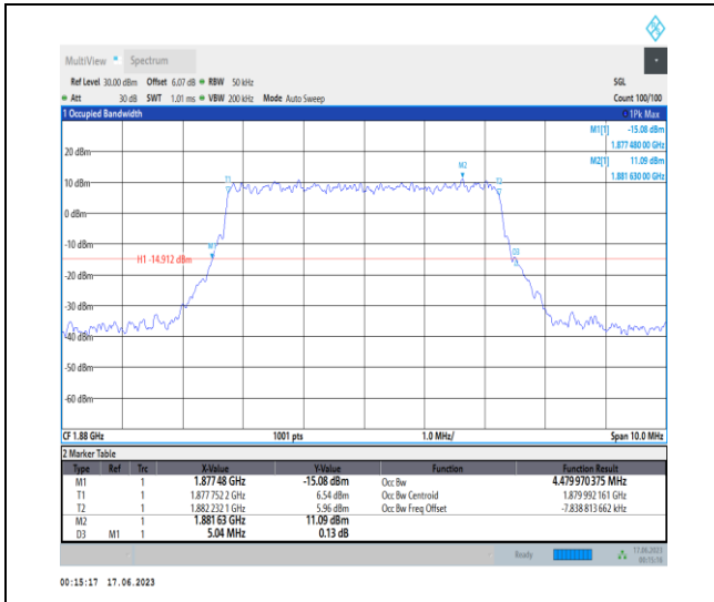
1-N2-PC3-15-5-M-8-CP-64QAM-Outer_Full-25@0-A Ant3-4.48-5.040-≤5-PASS
