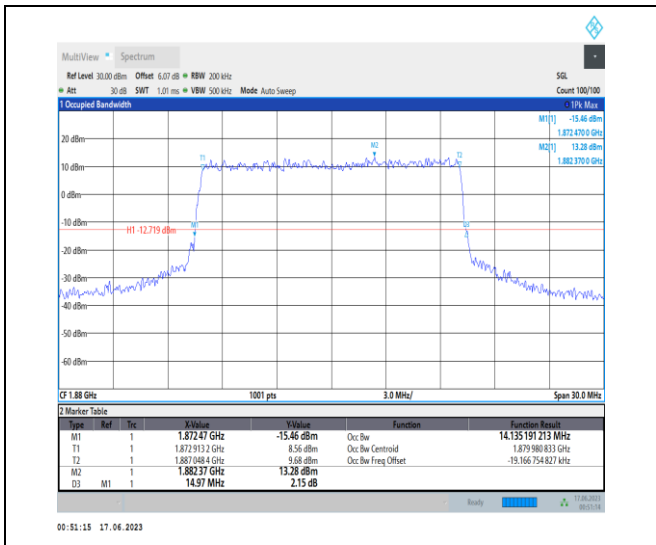
1-N2-PC3-15-15-M-6-CP-QPSK-Outer_Full-79@0-Ant3-14.135-14.970-≤15-PASS
