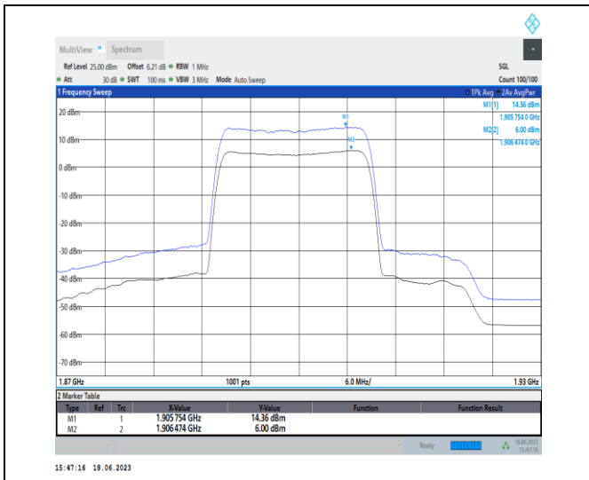
1-N2-PC3-15-20-H-1-DFT-256QAM-Outer_Full-100 @0-Ant3-8.36-100%-0.00-8.36-PASS-≤13
