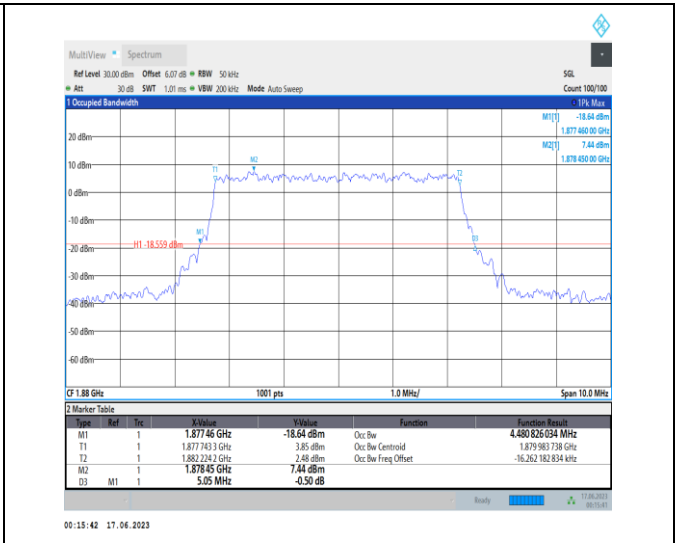
1-N2-PC3-15-5-M-9-CP-256QAM-Outer_Full-25@0-A Ant3-4.481-5.050-≤5-PASS
