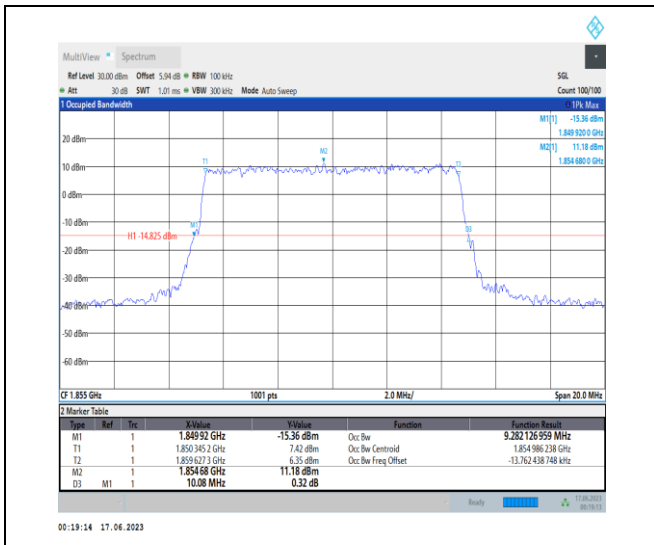
1-N2-PC3-15-10-L-6-CP-QPSK-Outer_Full-52@0-A Ant3-9.282-10.080-≤10-PASS
