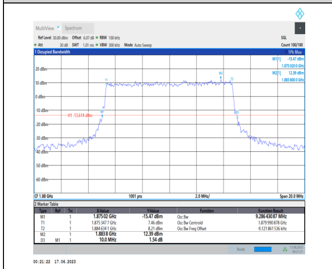
1-N2-PC3-15-10-M-7-CP-16QAM-Outer_Full-52@0-A nt3-9.286-10.000-≤10-PASS
