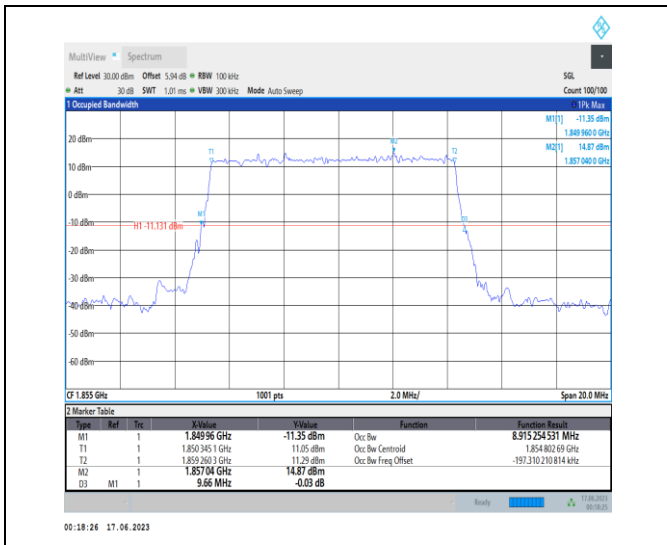
1-N2-PC3-15-10-L-2-DFT-PI2BPSK-Outer_Full-50@0-Ant3-8.915-9.660-≤10-PASS
