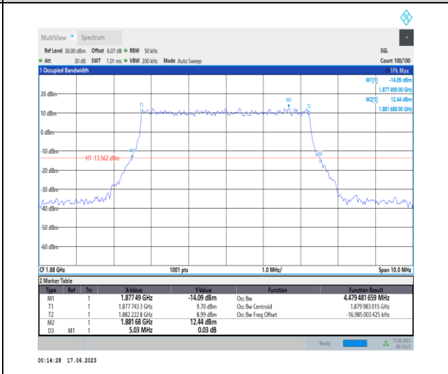
1-N2-PC3-15-5-M-3-DFT-16QAM-Outer_Full-25@0 Ant3-4.479-5.030-≤5-PASS
