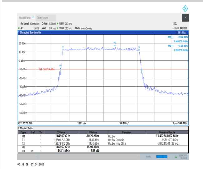
1-N2-PC3-15-15-L-1-DFT-QPSK-Outer_Full-75@0-Ant3-13.403-14.310-≤15-PASS
