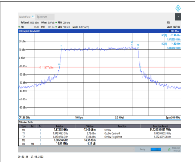
1-N2-PC3-15-15-M-7-CP-16QAM-Outer_Full-79@0-Ant3-14.125-14.970-≤15-PASS
