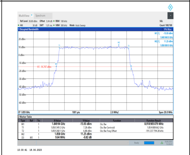
1-N2-PC3-15-10-L-1-DFT-QPSK-Outer_Full-50@0-A nt3-8.919-9.640-≤10-PASS
