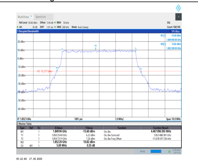
1-N2-PC3-15-5-L-6-CP-QPSK-Outer_Full-25@0-Ant3-4.467-5.090-≤5-PASS
