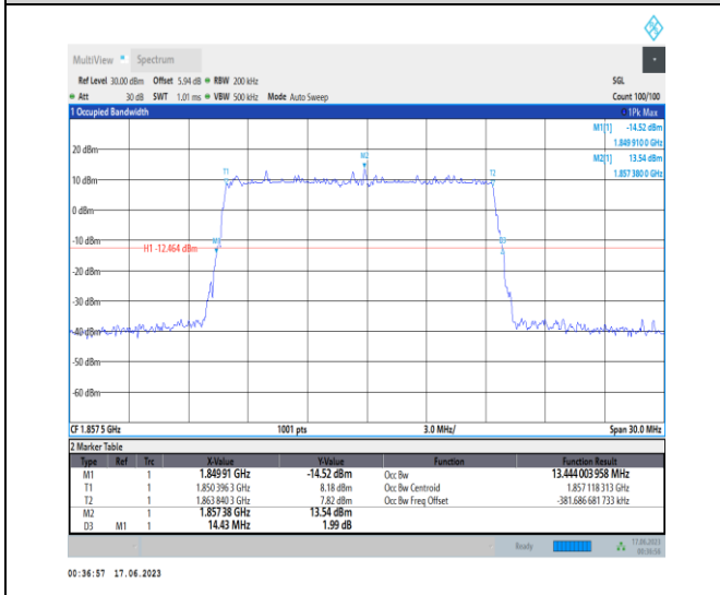
1-N2-PC3-15-15-L-5-DFT-256QAM-Outer_Full-75@0-Ant3-13.444-14.430-≤15-PASS
