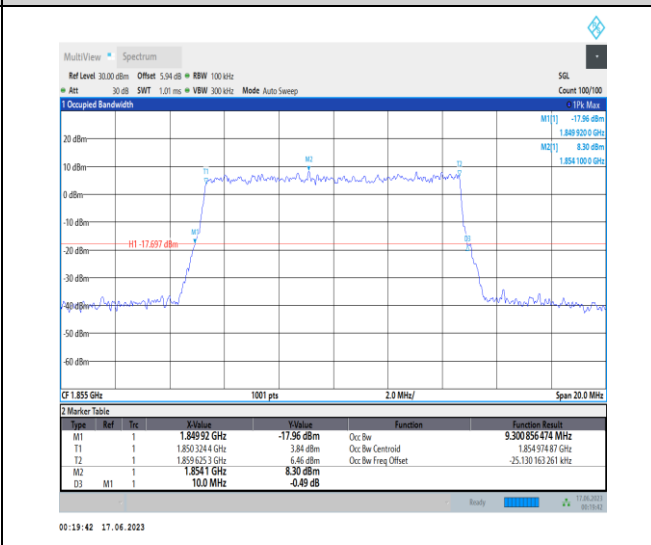
1-N2-PC3-15-10-L-9-CP-256QAM-Outer_Full-52@0-A Ant3-9.301-10.000-≤10-PASS
