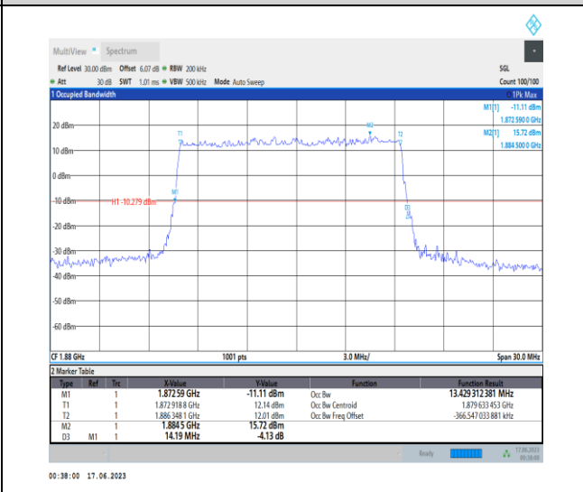
1-N2-PC3-15-15-M-1-DFT-QPSK-Outer_Full-75@0- Ant3-13.429-14.190≤15-PASS
