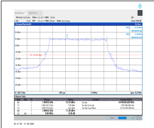
1-N2-PC3-15-5-H-7-CP-16QAM-Outer_Full-25@0-A nt3-4.479-5.090-≤5-PASS
