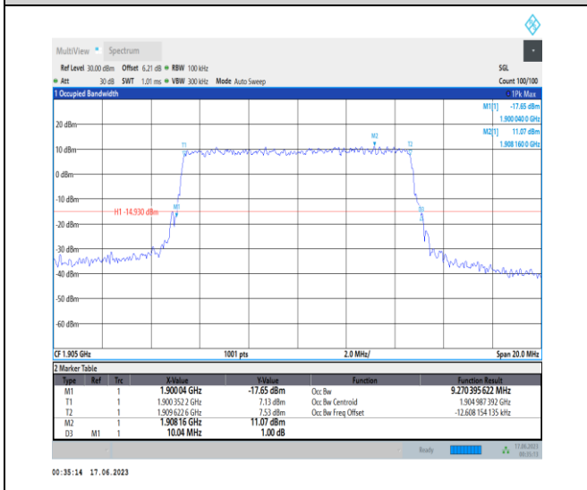
1-N2-PC3-15-10-H-6-CP-QPSK-Outer_Full-52@0-A nt3-9.27-10.040-≤10-PASS
