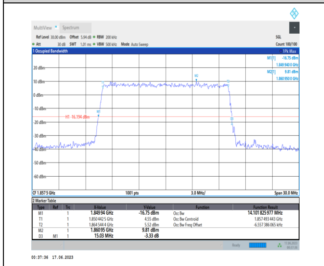
1-N2-PC3-15-15-L-9-CP-256QAM-Outer_Full-79@0- Ant3-14.102-15.030≤15-PASS
