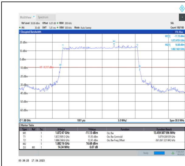
1-N2-PC3-15-15-M-2-DFT-PI2BPSK-Outer_Full-75@ 0-Ant3-13.459-14.340≤15-PASS
