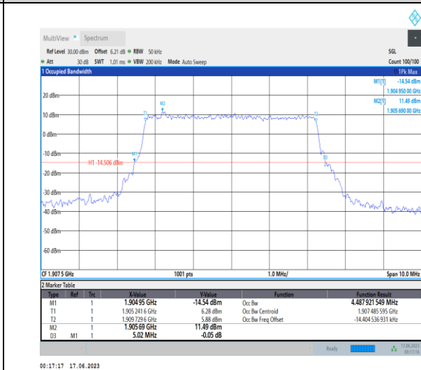
1-N2-PC3-15-5-H-6-CP-QPSK-Outer_Full-25@0-An t3-4.488-5.020-≤5-PASS
