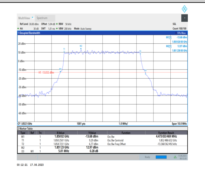
1-N2-PC3-15-5-L-4-DFT-64QAM-Outer_Full-25@0-A nt3-4.473-5.010-≤5-PASS
