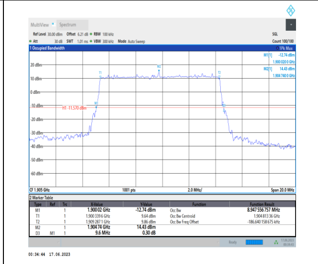
1-N2-PC3-15-10-H-3-DFT-16QAM-Outer_Full-50@0-Ant3-8.948-9.600-<=10-PASS
