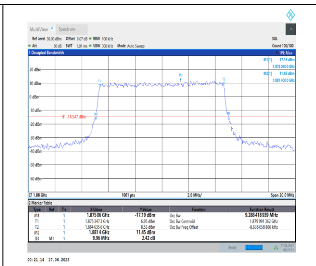
1-N2-PC3-15-10-M-6-CP-QPSK-Outer_Full-52@0- Ant3-9.288-9.960-≤10-PASS
