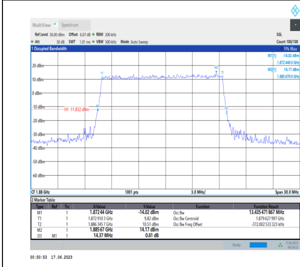
1-N2-PC3-15-15-M-4-DFT-64QAM-Outer_Full-75@0 -Ant3-13.435-14.370≤15-PASS
