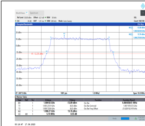
1-N2-PC3-15-5-H-3-DFT-16QAM-Outer_Full-25@0-A Ant3-4.485-5.140-≤5-PASS
