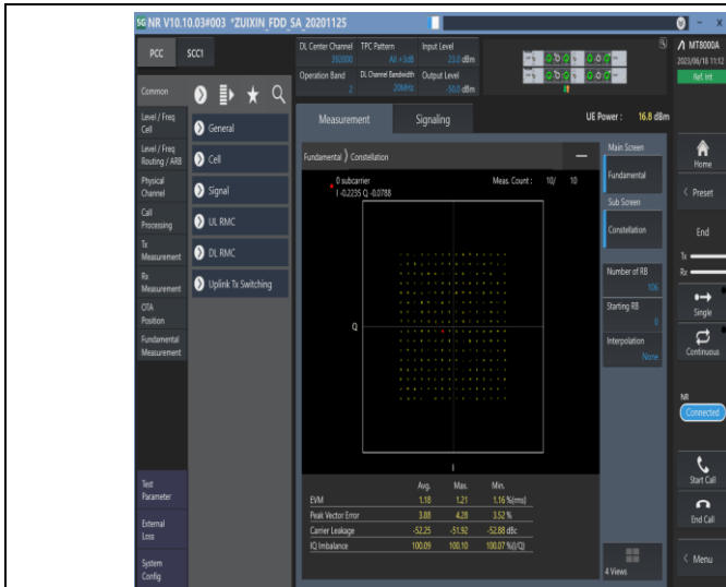
1-N2-PC3-15-20-M-9-CP-256QAM-Outer_Full-106@0-Ant3-see graph-PASS
