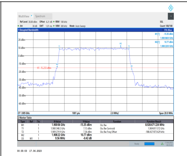
1-N2-PC3-15-10-H-5-DFT-256QAM-Outer_Full-50@0 0-Ant3-8.927-9.560-≤10-PASS
