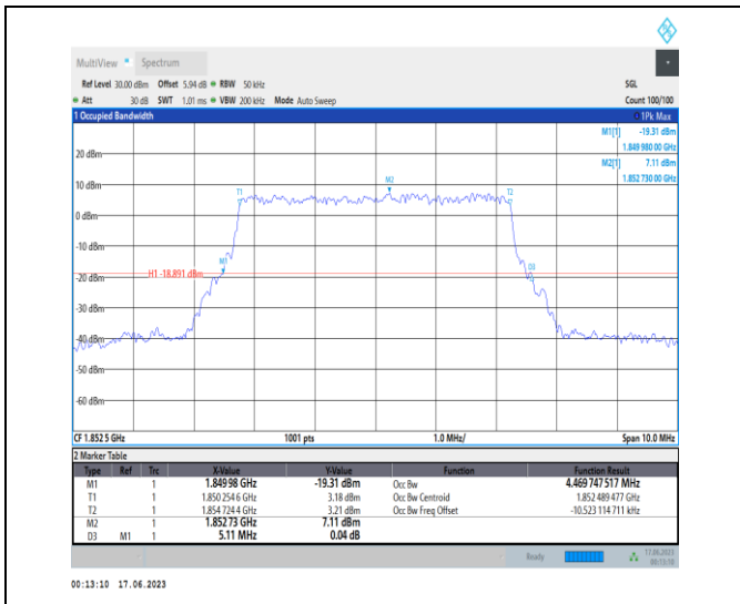
1-N2-PC3-15-5-L-9-CP-256QAM-Outer_Full-25@0-A nt3-4.47-5.110-≤5-PASS
