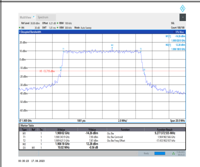
1-N2-PC3-15-10-H-7-CP-16QAM-Outer_Full-52@0- Ant3-9.277-10.020-≤10-PASS
