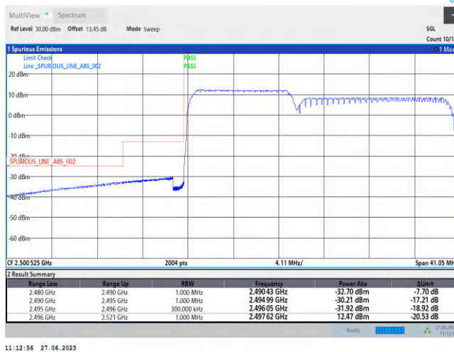
41-41-10MHz-15MHz-QPSK-QPSK-39703-39823-50RB#0-75RB#0
