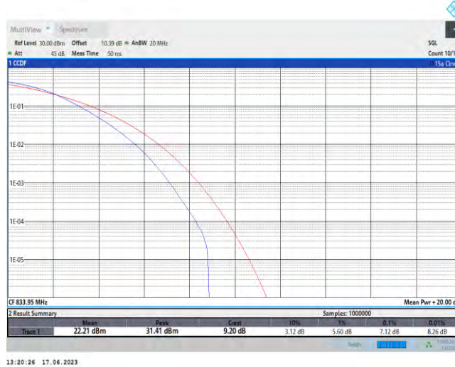
5-5-10MHz-10MHz-QPSK-QPSK-20476-20575-50RB#0-50RB#0
