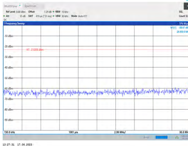
5-5-10MHz-10MHz-QPSK-QPSK-20450-20549-1RB#0-0RB#0-0.15~30MHz
