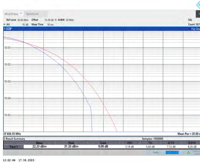
5-5-10MHz-10MHz-QPSK-QPSK-20476-20575-50RB#0-50RB#0
