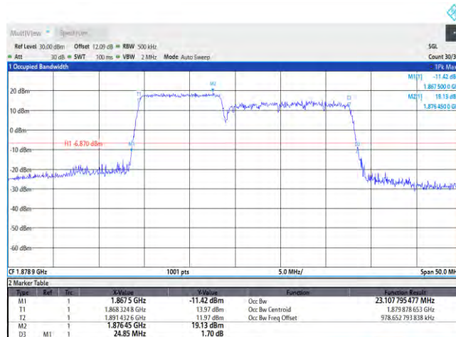
2-2-10MHz-15MHz-QPSK-QPSK-18829-18949-50RB#0-75RB#0
