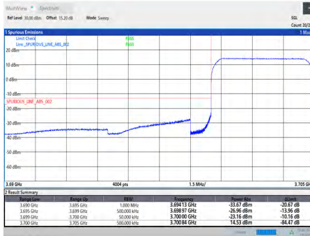
Band43-5MHz-QPSK-44615-25RB#0
