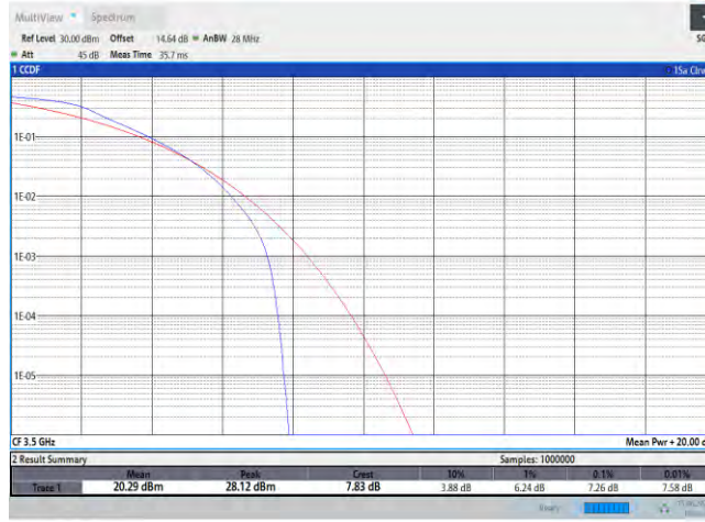
Band42-20MHz-QPSK-42590-100RB#0
