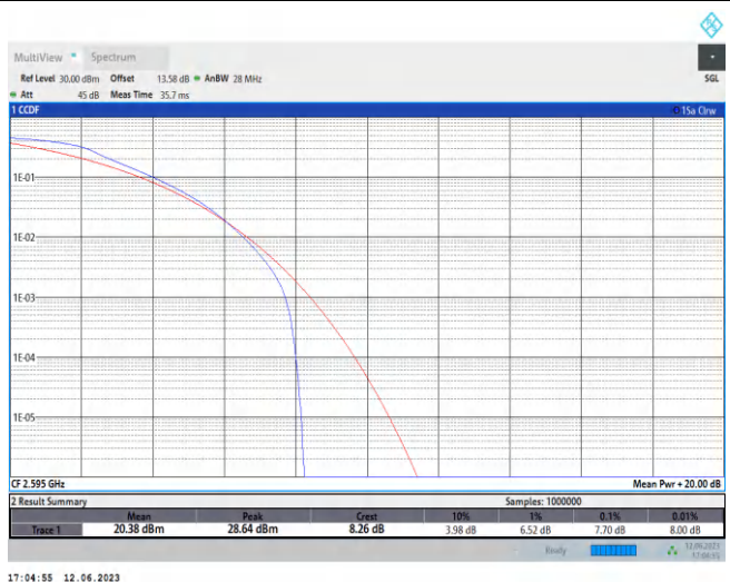
Band38-20MHz-QPSK-38000-100RB#0
