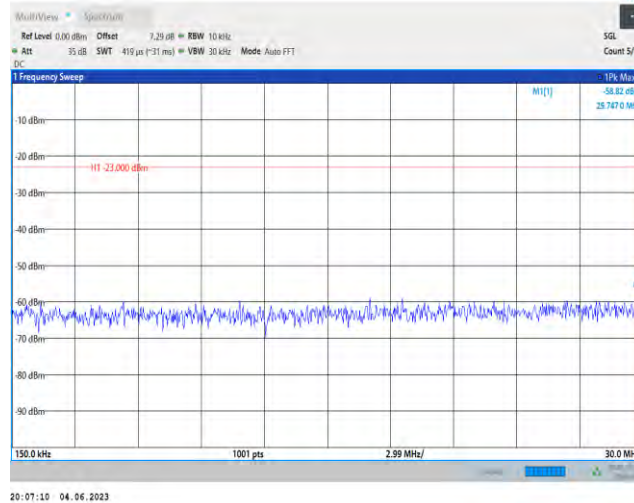
Band26-15MHz-QPSK-26865-1RB#0-Range2:0.15~30MHz
