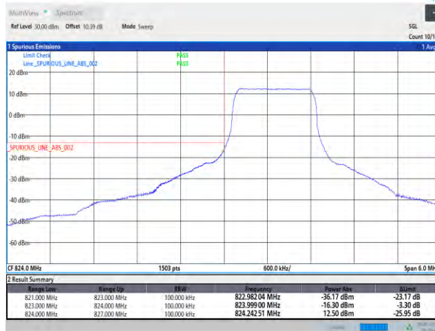
Band26-1.4MHz-QPSK-26797-6RB#0
