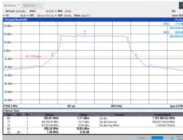
Band26-1.4MHz-QPSK-26915-6RB#0
