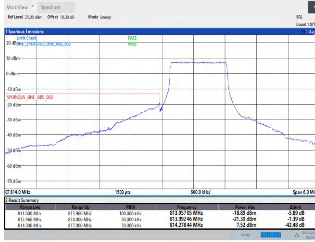
Band26-1.4MHz-QPSK-26697-6RB#0
