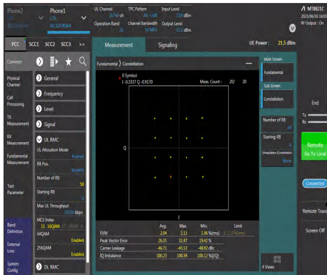
Band26-10MHz-16QAM-26740-50RB#0
