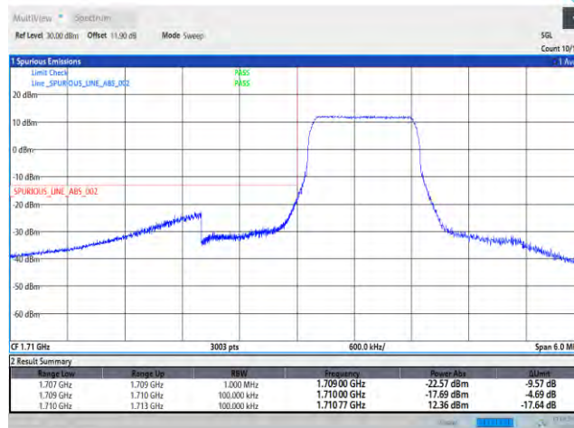
Band4-1.4MHz-QPSK-19957-6RB#0
