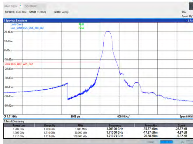
Band4-1.4MHz-QPSK-19957-6RB#0
