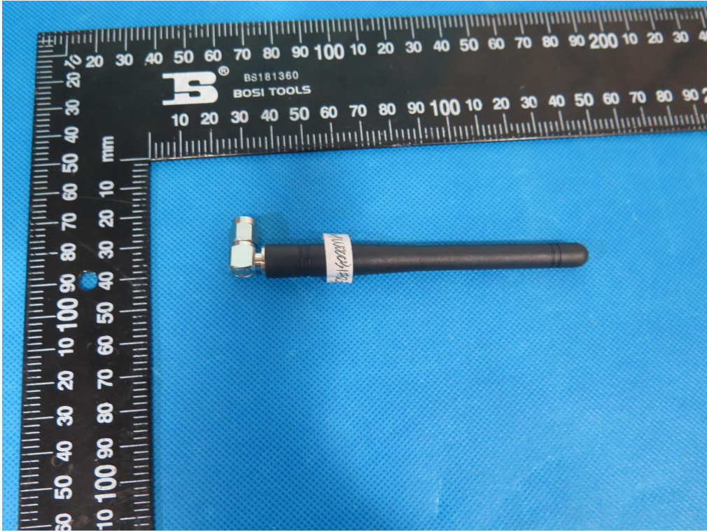
Main ANT
