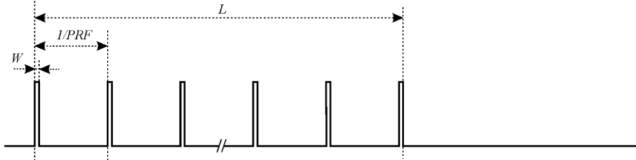
Figure 1: General structure of a single burst/constant PRF based radar test signal
