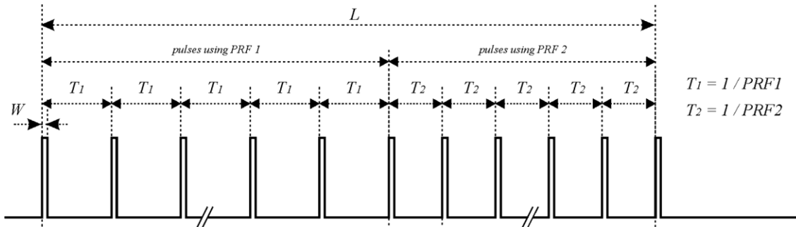
Figure 4: General structure of a single burst/package based staggered PRF radar test signal
