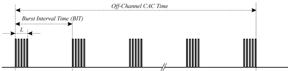
Figure 5: General structure of a multiple burst/package based staggered PRF based radar test signal
