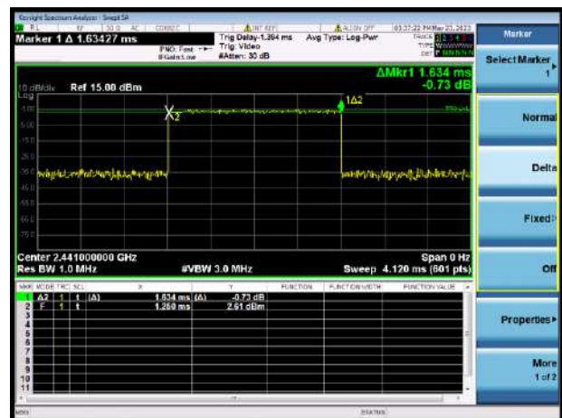
8-DPSK DH3
