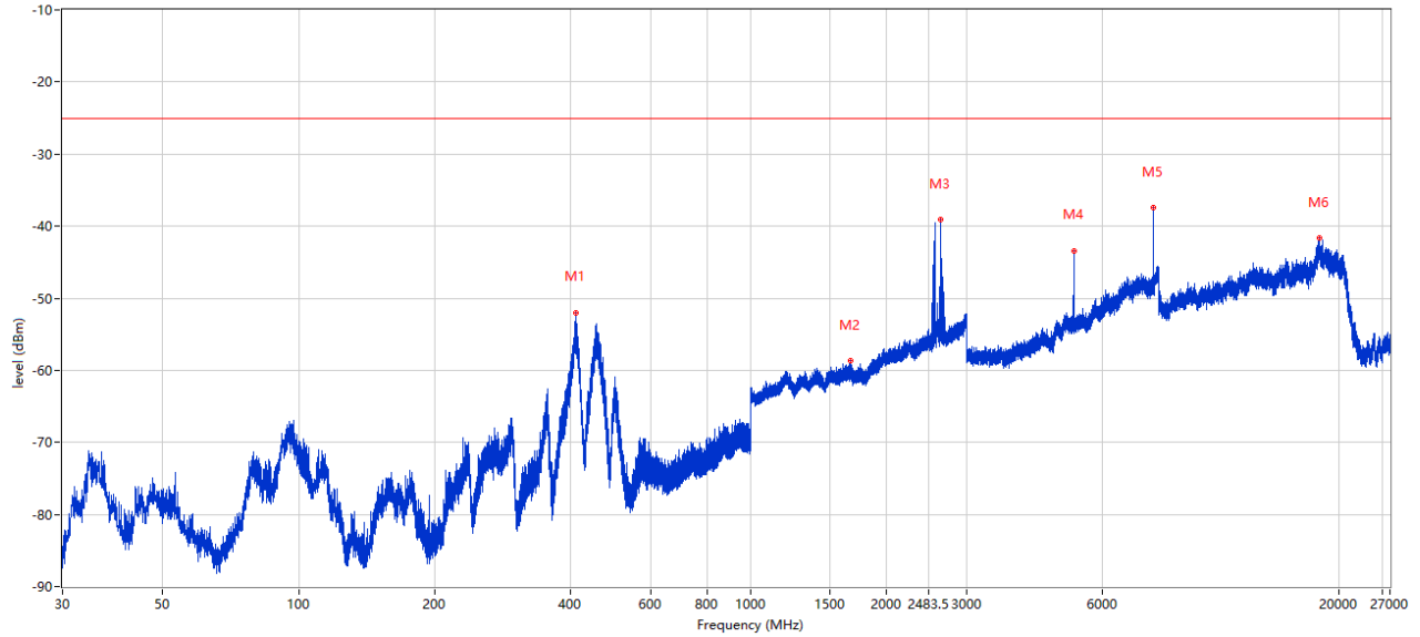
RSE (RF) _FCC PART22&24&27-RSE_LTE Band 38 & 41(mid) _2570-2620_30MHz-27GHz
