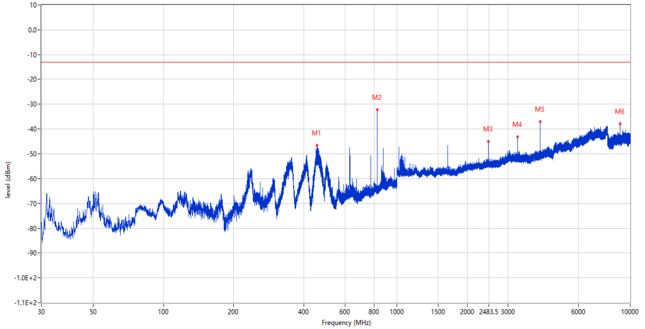
RSE (RF) _FCC PART22&24&27-RSE_GSM 850 & CDMA BC0 & WCDMA Band5 & LTE Band 5 & 26_814-849_30MHz-10GHz
