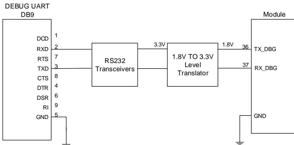
Figure 10 DEBUG serial port connection diagram
