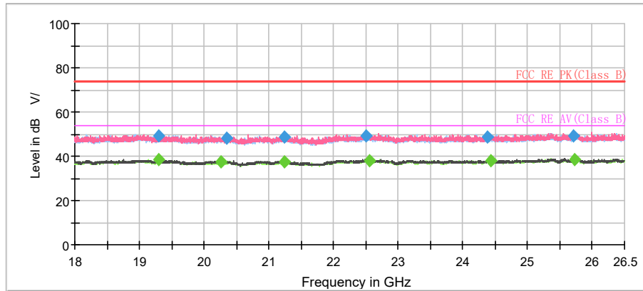
Radiates Emission from 18GHz to 26.5GHz
