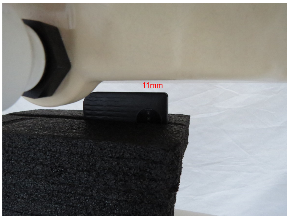
Picture 8: Left Edge, the distance from EUT to the bottom of the Phantom is 11mm
