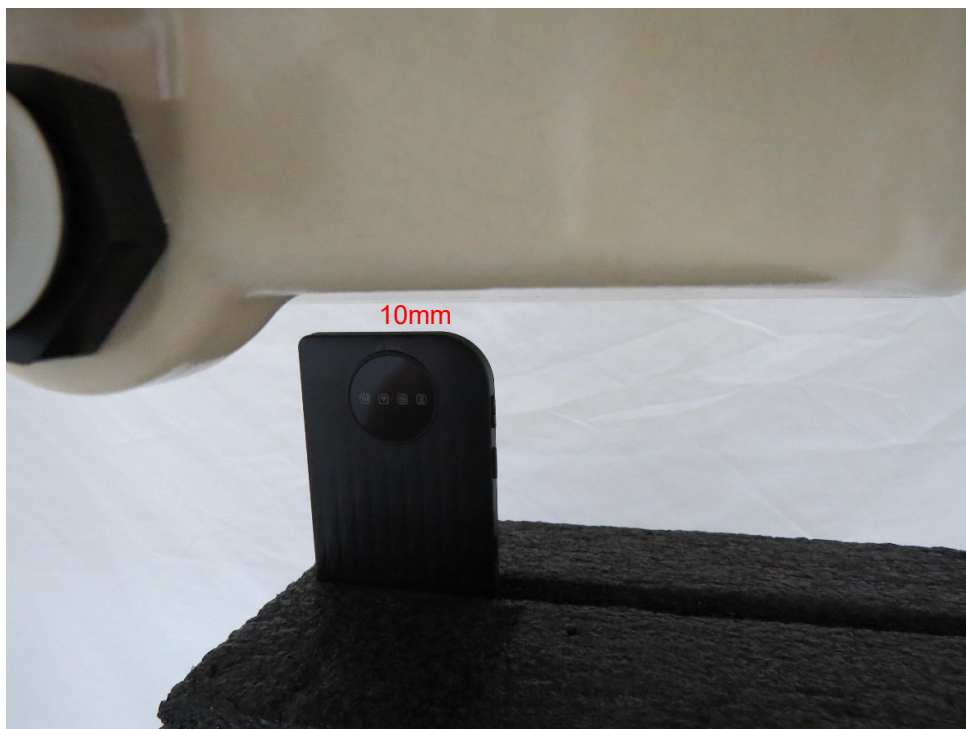
Picture 5: Top Edge, the distance from EUT to the bottom of the Phantom is 10mm
