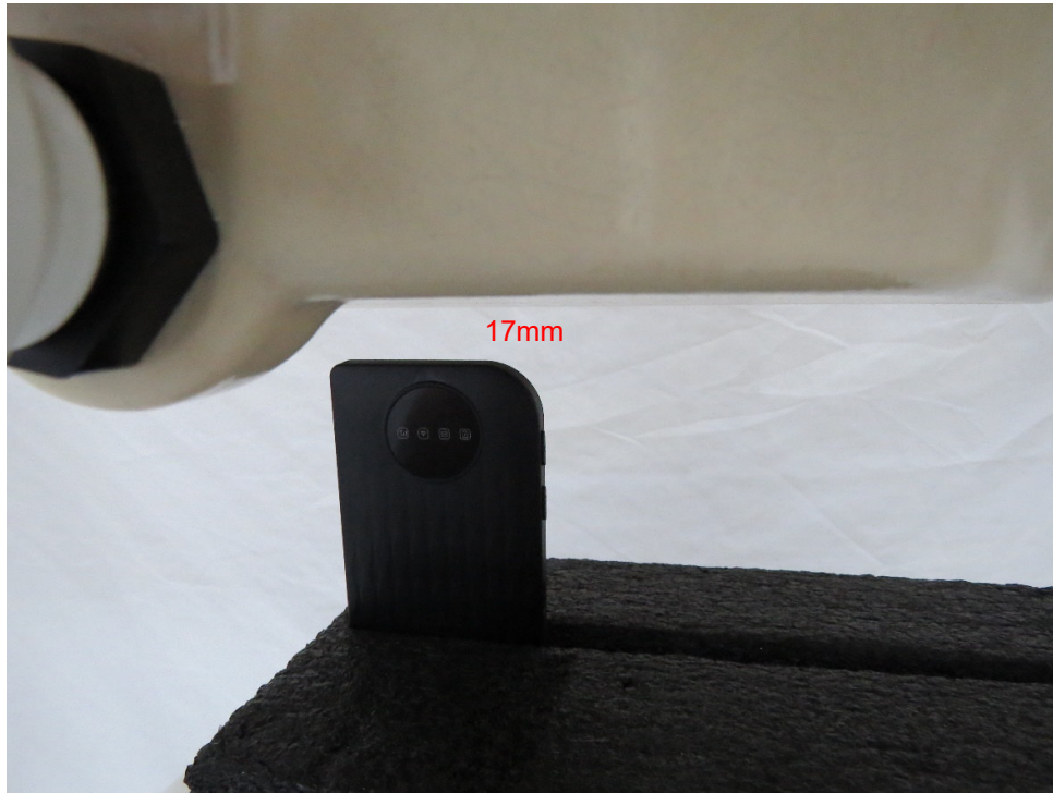
Picture 9: Top Edge, the distance from EUT to the bottom of the Phantom is 17mm
