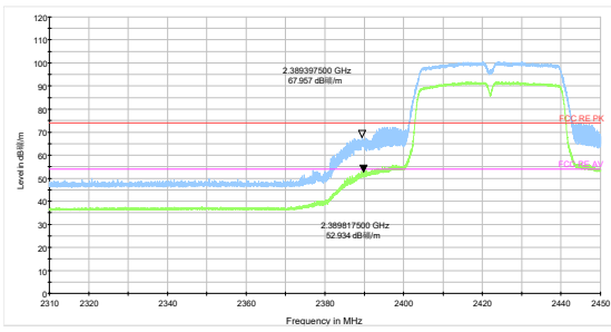
802.11n HT20 -Channel 3 Peak+ Average
