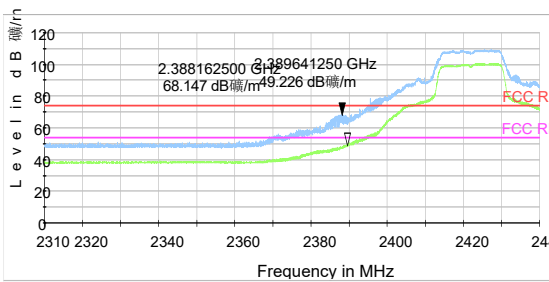
802.11g-Channel 3 Peak+ Average
