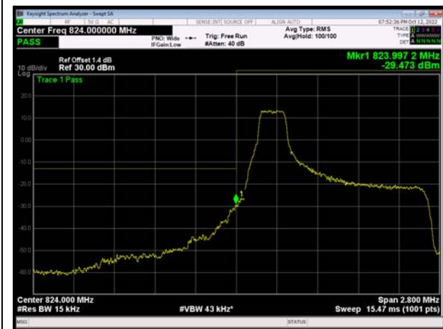
LTE Band 5 QPSK 1.4MHz CH-Low 100%RB
