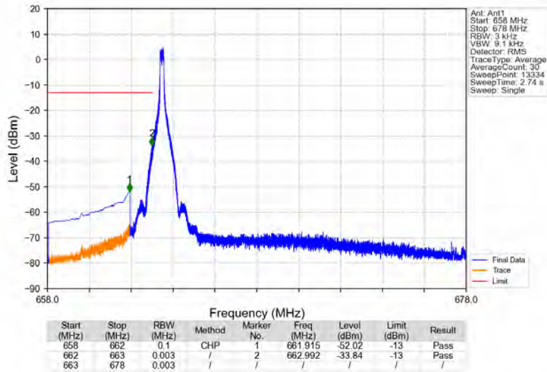
n71_15kHz_SISO_NTNV_15MHz_CP-OFDM QPSK_670.5MHz_Edge_1RB_Left
