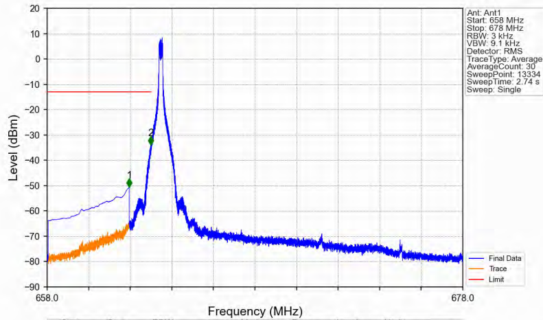
n71_15kHz_SISO_NTNV_15MHz_DFT-s-OFDM QPSK_670.5MHz_Edge_1RB_Left
