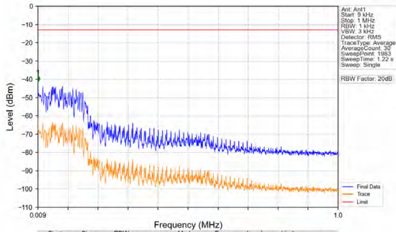
n71_15kHz_SISO_NTNV_15MHz_DFT-s-OFDM QPSK_690.5MHz_Edge_1RB_Right
