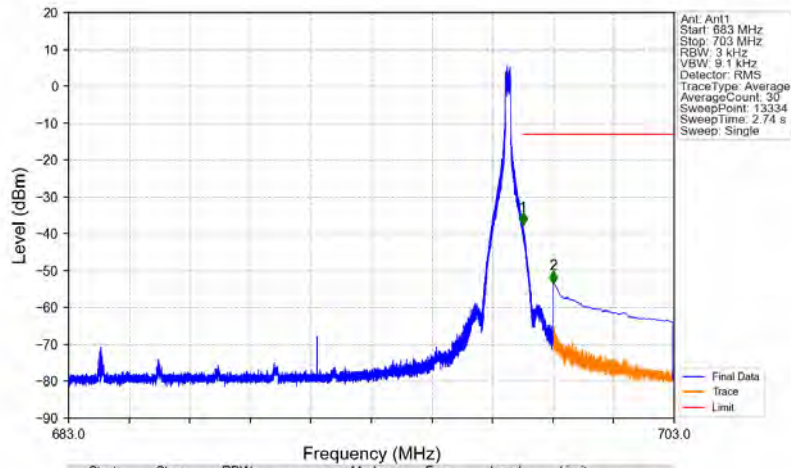
n71_15kHz_SISO_NTNV_15MHz_DFT-s-OFDM PI/2 BPSK 690.5MHz_Edge_1RB_Right
