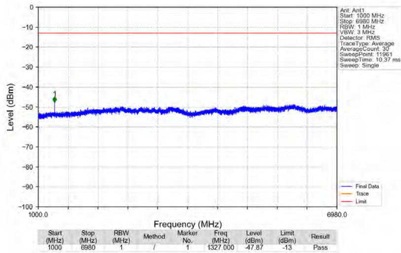
n71_15kHz_SISO_NTNV_15MHz_DFT-s-OFDM QPSK_670.5MHz_Edge_1RB_Left
