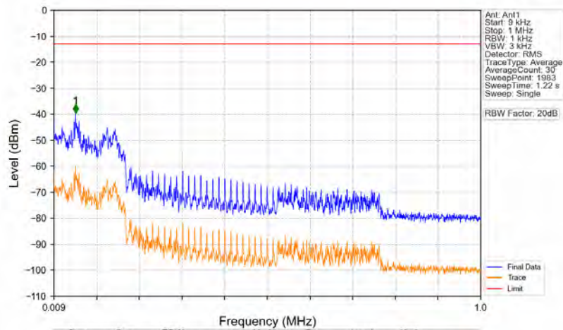
n71_15kHz_SISO_NTNV_10MHz_DFT-s-OFDM PI/2 BPSK_693MHz_Edge_1RB_Right
