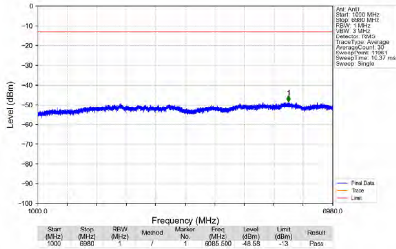
n71_15kHz_SISO_NTNV_15MHz_DFT-s-OFDM PI/2 BPSK_690.5MHz_Edge_1RB_Right
