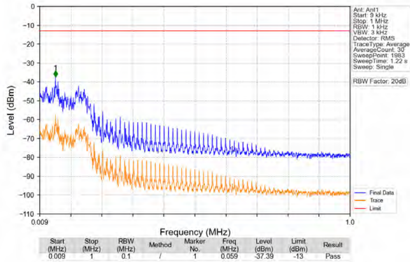
n71_15kHz_SISO_NTV_10MHz_DFT-s-OFDM PI/2 BPSK_680.5MHz_Edge_1RB_Left
