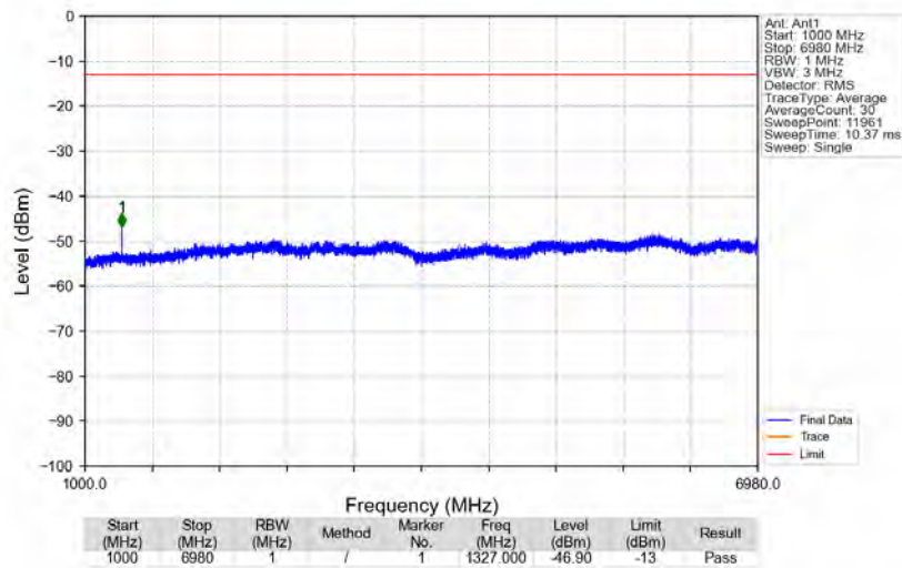
n71_15kHz_SISO_NTNV_15MHz_DFT-s-OFDM PI/2 BPSK_670.5MHz_Edge_1RB_Left
