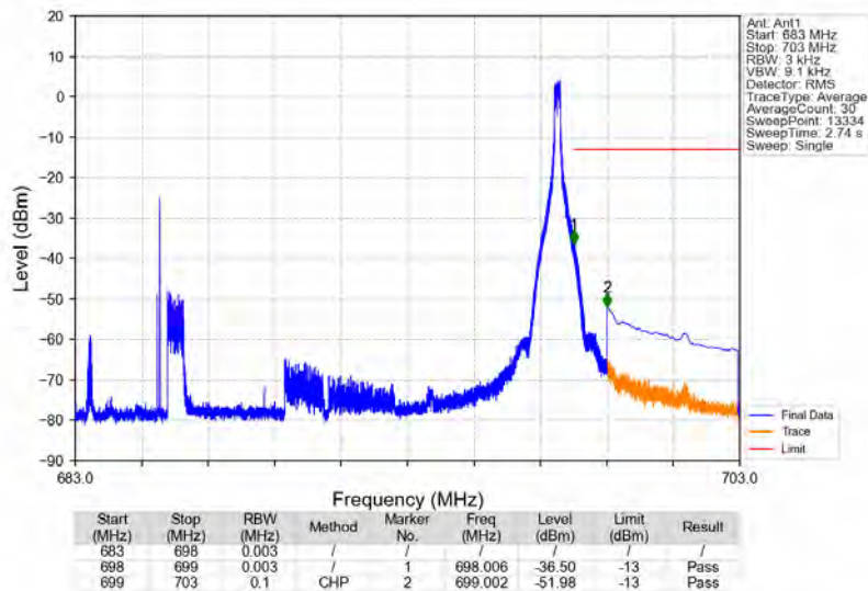
n71_15kHz_SISO_NTV_15MHz_CP-OFDM_QPSK_690.5MHz_Edge_1RB_Right
