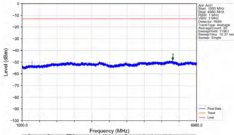
n71_15kHz_SISO_NTNV_20MHz_DFT-s-OFDM QPSK_680.5MHz_Edge_1RB_Left
