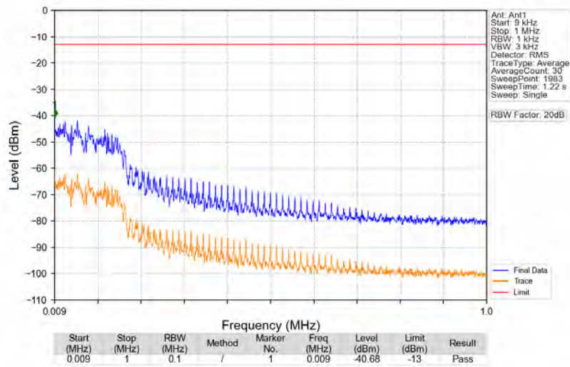
n71_15kHz_SISO_NTNV_15MHz_CP-OFDM QPSK_670.5MHz_Edge_1RB_Left
