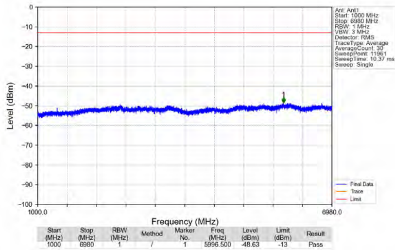
n71_15kHz_SISO_NTNV_10MHz_CP-OFDM QPSK_693MHz_Edge_1RB_Right
