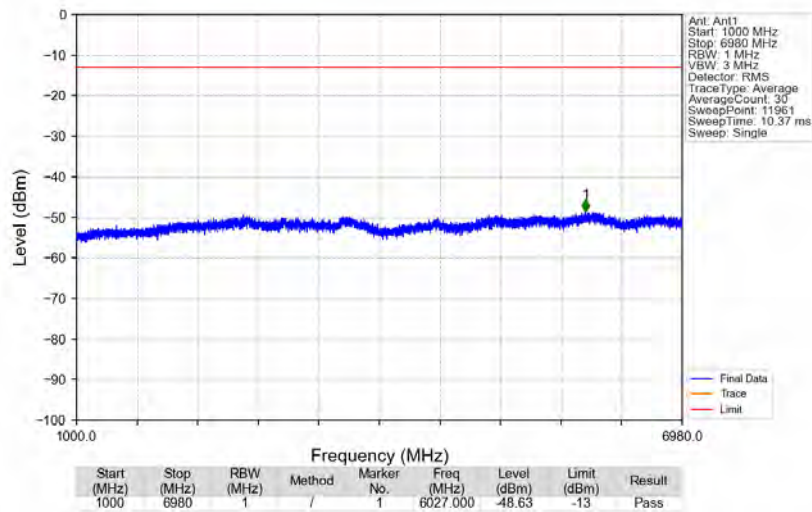
n71_15kHz_SISO_NTNV_15MHz_CP-OFDM QPSK_690.5MHz_Edge_1RB_Right
