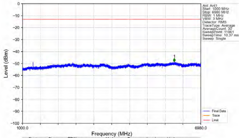
n71_15kHz_SISO_NTNV_10MHz_DFT-s-OFDM PI/2 BPSK_680.5MHz_Edge_1RB_Left
