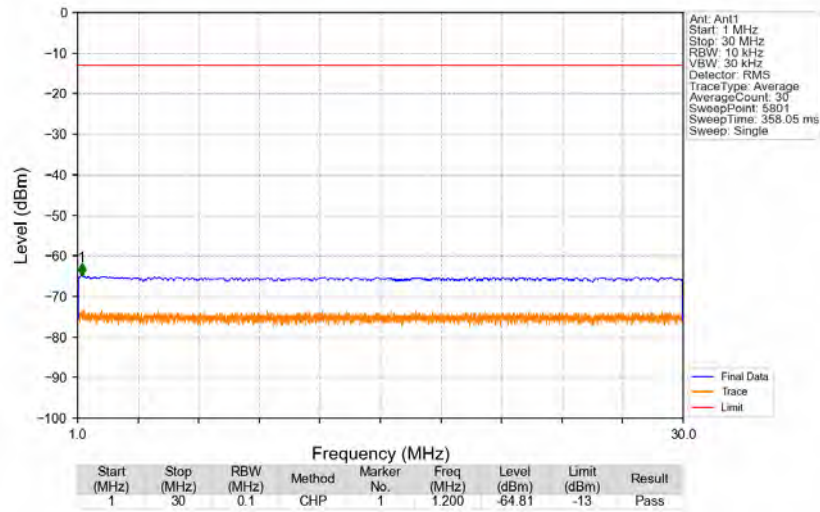
n71_15kHz_SISO_NTNV_15MHz_CP-OFDM QPSK_670.5MHz_Edge_1RB_Left
