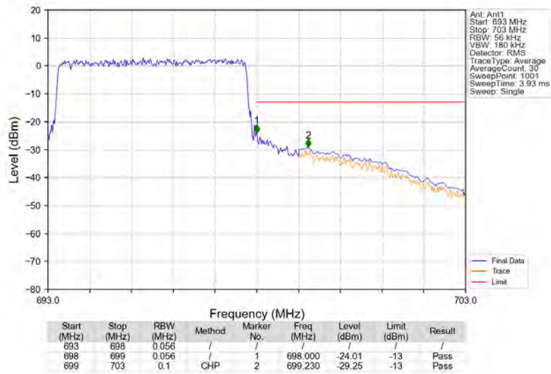
n71_15kHz_SISO_NTNV_5MHz_CP-OFDM QPSK_695.5MHz_Outer_Full
