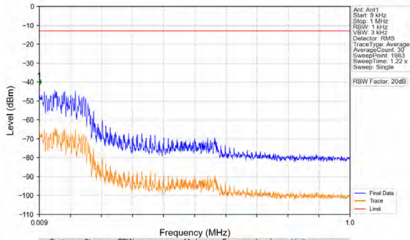
n71_15kHz_SISO_NTNV_15MHz_DFT-s-OFDM QPSK_670.5MHz_Edge_1RB_Left
