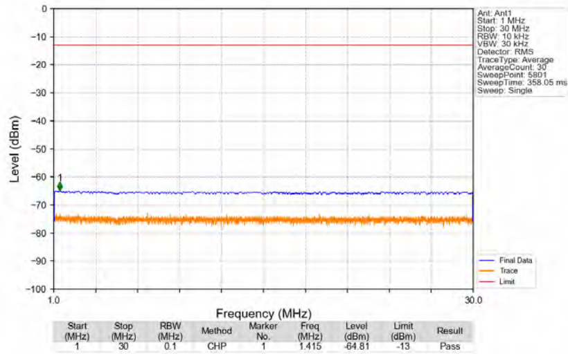
n71_15kHz_SISO_NTNV_15MHz_DFT-s-OFDM QPSK_670.5MHz_Edge_1RB_Left
