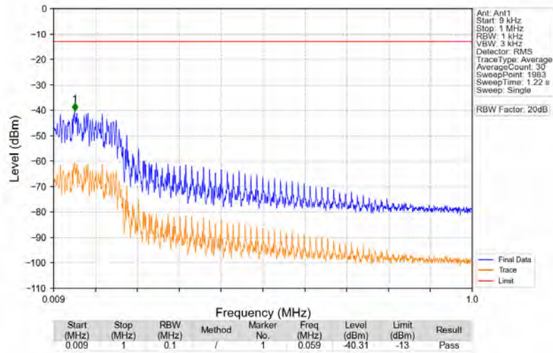
n71_15kHz_SISO_NTNV_15MHz_DFT-s-OFDM QPSK_680.5MHz_Edge_1RB_Left
