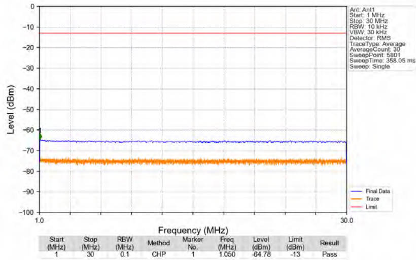
n71_15kHz_SISO_NTNV_10MHz_DFT-s-OFDM QPSK_693MHz_Edge_1RB_Right
