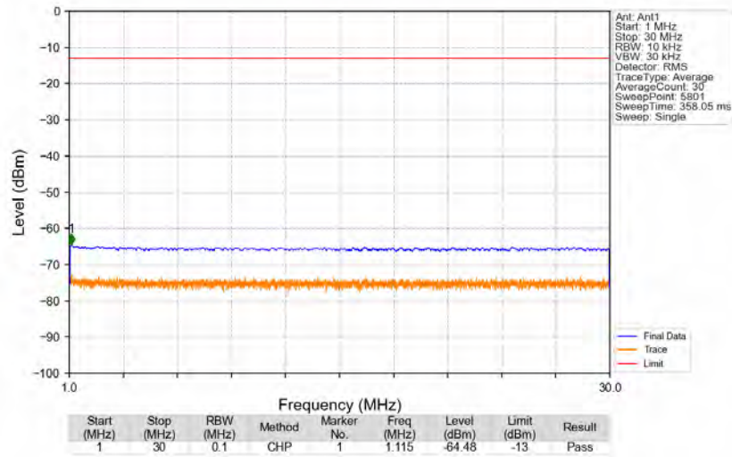
n71_15kHz_SISO_NTNV_15MHz_CP-OFDM QPSK_690.5MHz_Edge_1RB_Right
