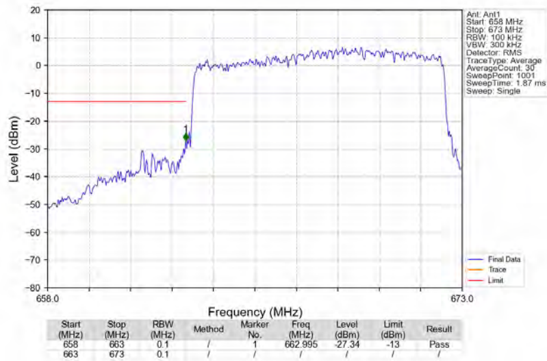
n71_15kHz_SISO_NTNV_10MHz_DFT-s-OFDM PI/2 BPSK_668MHz_Outer_Full
