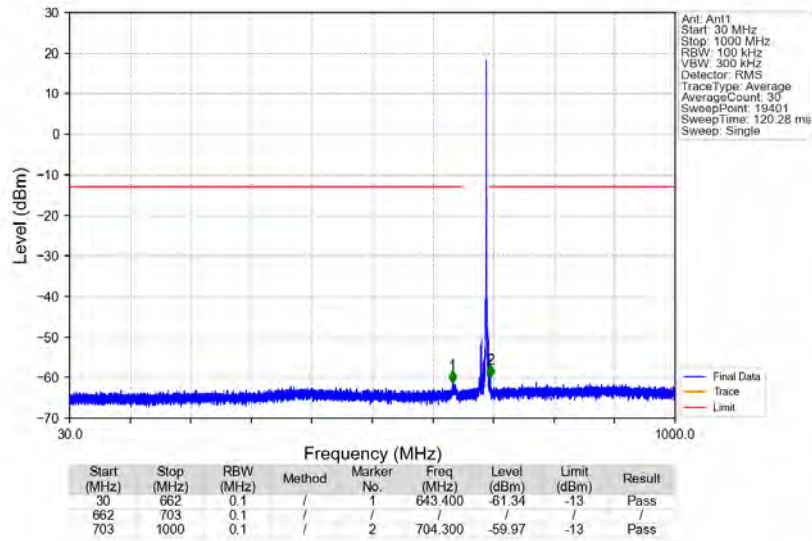
n71_15kHz_SISO_NTNV_10MHz_CP-OFDM QPSK_693MHz_Edge_1RB_Right
