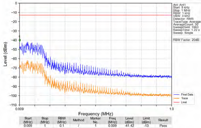
n71_15kHz_SISO_NTV_10MHz_DFT-s-OFDM_QPSK_668MHz_Edge_1RB_Left
