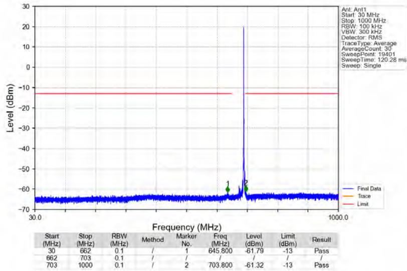
n71_15kHz_SISO_NTNV_15MHz_DFT-s-OFDM QPSK_690.5MHz_Edge_1RB_Right
