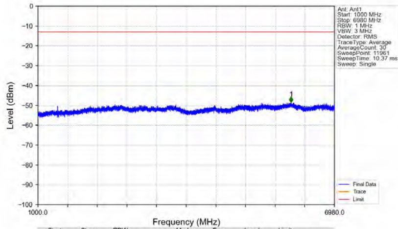
n71_15kHz_SISO_NTNV_10MHz_DFT-s-OFDM PI/2 BPSK_693MHz_Edge_1RB_Right
