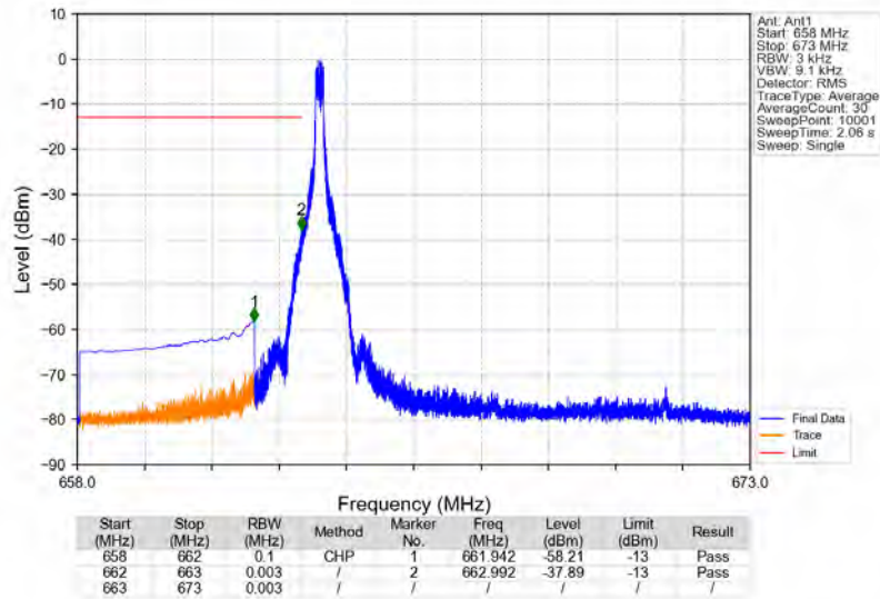
n71_15kHz_SISO_NTV_10MHz_DFT-s-OFDM_QPSK_668MHz_Edge_1RB_Left
