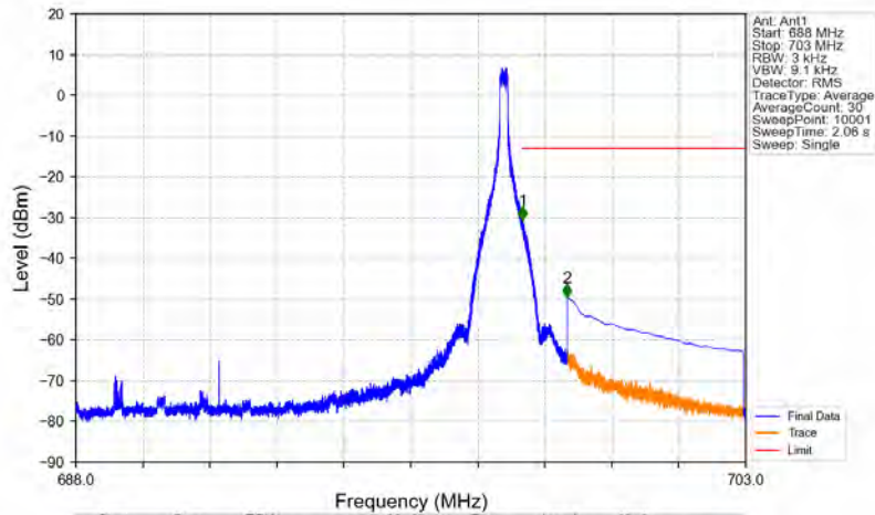
n71_15kHz_SISO_NTNV_10MHz_DFT-s-OFDM QPSK_693MHz_Edge_1RB_Right
