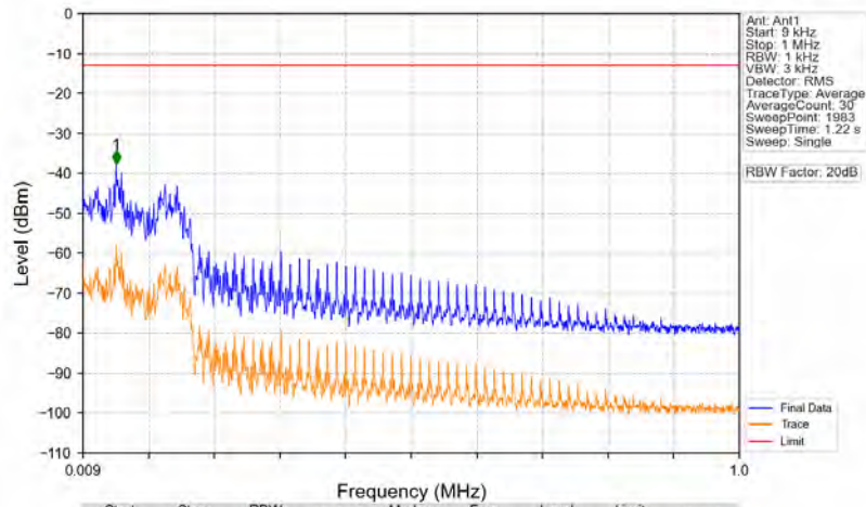
n71_15kHz_SISO_NTNV_15MHz_DFT-s-OFDM PI/2 BPSK 690.5MHz_Edge_1RB_Right
