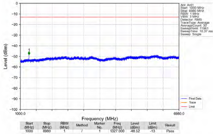
n71_15kHz_SISO_NTNV_10MHz_DFT-s-OFDM QPSK_668MHz_Edge_1RB_Left
