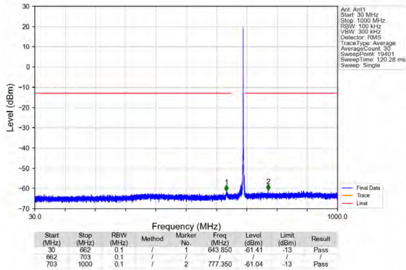
n71_15kHz_SISO_NTNV_10MHz_DFT-s-OFDM QPSK_693MHz_Edge_1RB_Right
