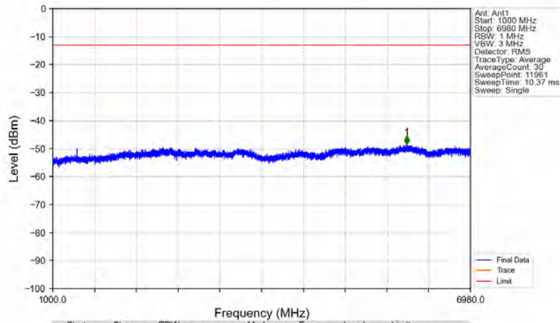
n71_15kHz_SISO_NTNV_15MHz_DFT-s-OFDM QPSK_680.5MHz_Edge_1RB_Left
