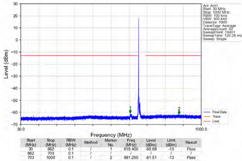
n71_15kHz_SISO_NTNV_10MHz_DFT-s-OFDM_QPSK_668MHz_Edge_1RB_Left
