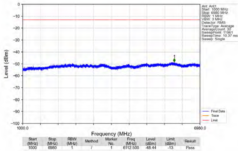
n71_15kHz_SISO_NTNV_10MHz_CP-OFDM QPSK_680.5MHz_Edge_1RB_Left
