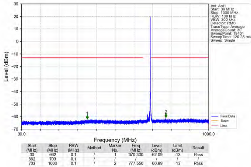
n71_15kHz_SISO_NTNV_15MHz_DFT-s-OFDM PI/2 BPSK_690.5MHz_Edge_1RB_Right
