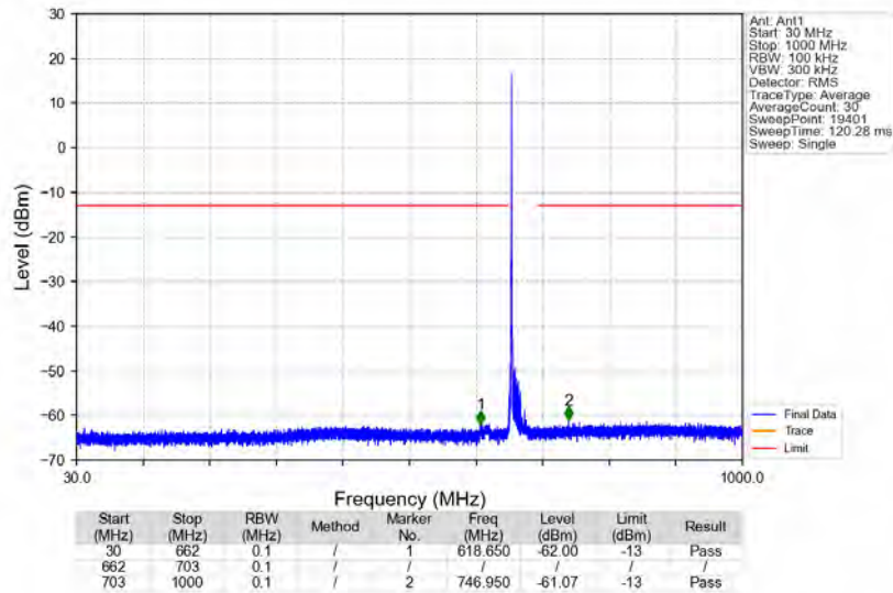
n71_15kHz_SISO_NTNV_15MHz_CP-OFDM QPSK_670.5MHz_Edge_1RB_Left
