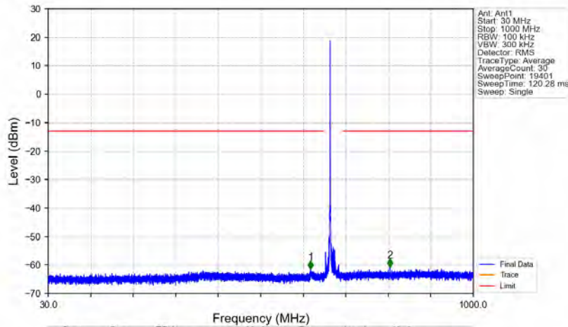
n71_15kHz_SISO_NTNV_15MHz_DFT-s-OFDM QPSK_680.5MHz_Edge_1RB_Left
