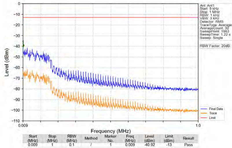
n71_15kHz_SISO_NTNV_15MHz_CP-OFDM QPSK_680.5MHz_Edge_1RB_Left
