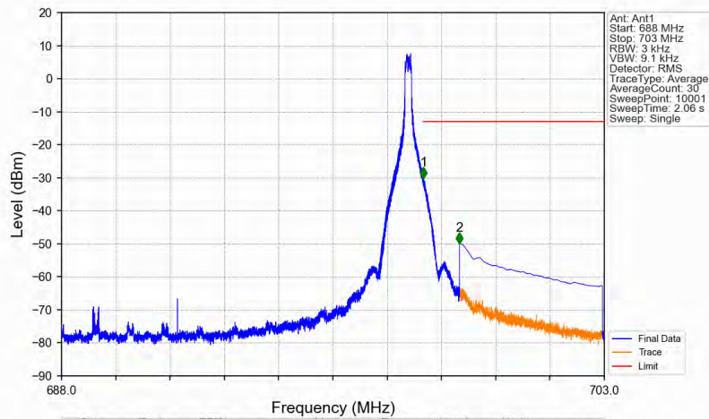
n71_15kHz_SISO_NTNV_10MHz_DFT-s-OFDM PI/2 BPSK_693MHz_Edge_1RB_Right
