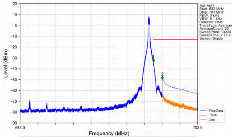
n71_15kHz_SISO_NTNV_15MHz_DFT-s-OFDM QPSK_690.5MHz_Edge_1RB_Right
