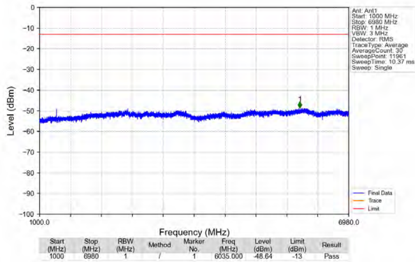
n71_15kHz_SISO_NTNV_15MHz_CP-OFDM QPSK_670.5MHz_Edge_1RB_Left
