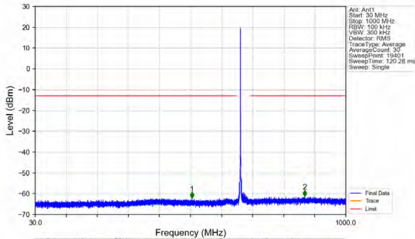
n71_15kHz_SISO_NTNV_20MHz_DFT-s-OFDM QPSK_680.5MHz_Edge_1RB_Left
