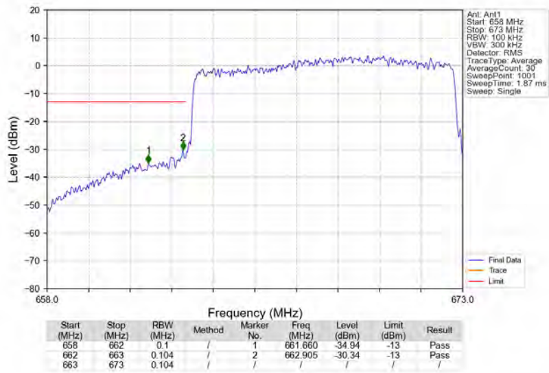
n71_15kHz_SISO_NTNV_10MHz_CP-OFDM QPSK_668MHz_Outer_Full
