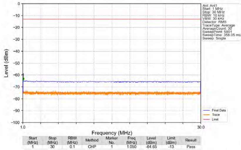
n71_15kHz_SISO_NTNV_15MHz_DFT-s-OFDM PI/2 BPSK_680.5MHz_Edge_1RB_Left
