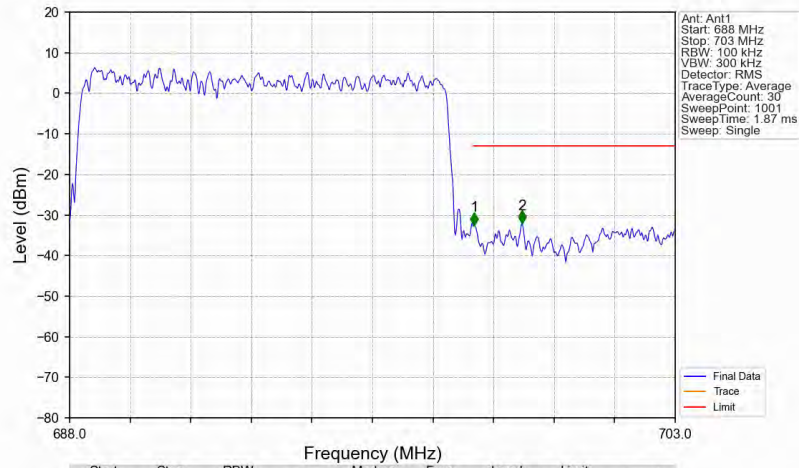
n71_15kHz_SISO_NTNV_10MHz_DFT-s-OFDM PI/2 BPSK_693MHz_Outer_Full
