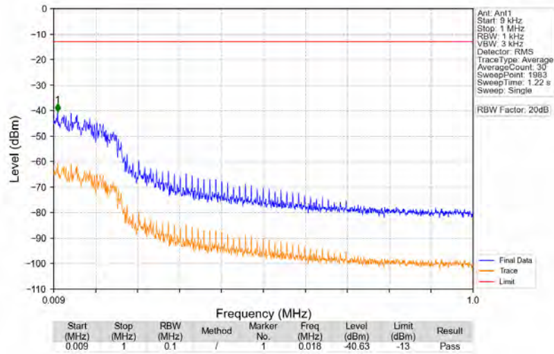
n71_15kHz_SISO_NTNV_10MHz_CP-OFDM QPSK_680.5MHz_Edge_1RB_Left
