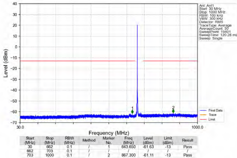
n71_15kHz_SISO_NTNV_20MHz_DFT-s-OFDM PI/2 BPSK_680.5MHz_Edge_1RB_Left
