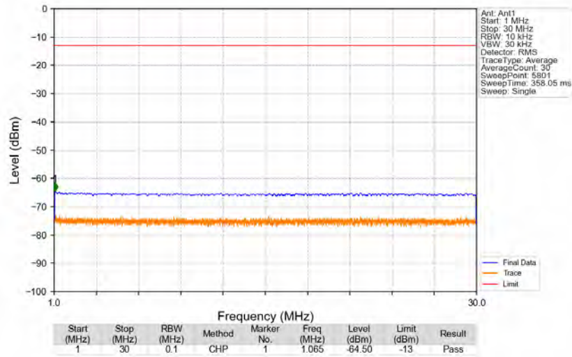
n71_15kHz_SISO_NTNV_10MHz_DFT-s-OFDM_QPSK_668MHz_Edge_1RB_Left
