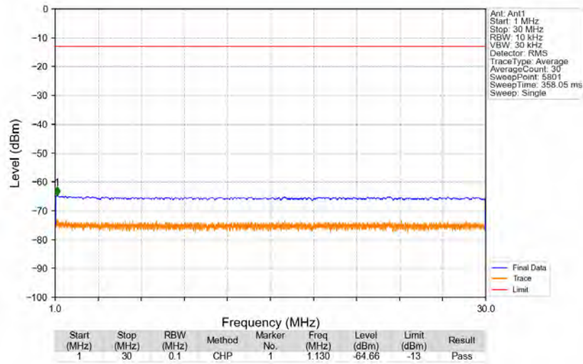
n71_15kHz_SISO_NTNV_10MHz_CP-OFDM QPSK_680.5MHz_Edge_1RB_Left
