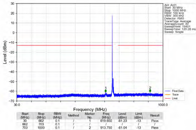
n71_15kHz_SISO_NTNV_10MHz_CP-OFDM QPSK_668MHz_Edge_1RB_Left
