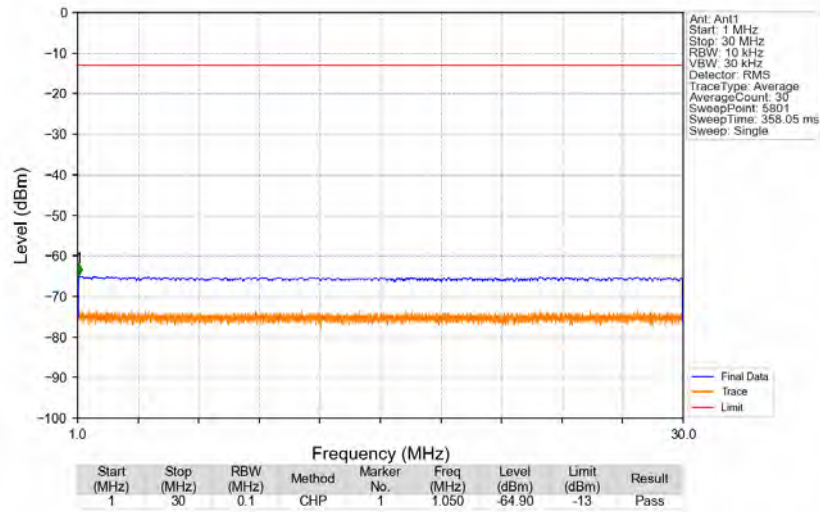
n71_15kHz_SISO_NTNV_15MHz_DFT-s-OFDM QPSK_690.5MHz_Edge_1RB_Right
