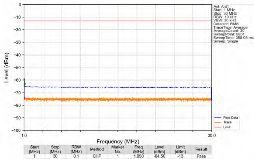
n71_15kHz_SISO_NTNV_10MHz_DFT-s-OFDM QPSK_680.5MHz_Edge_1RB_Left
