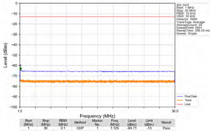
n71_15kHz_SISO_NTNV_10MHz_CP-OFDM QPSK_693MHz_Edge_1RB_Right
