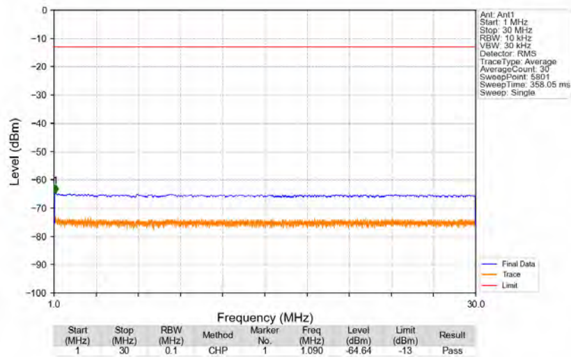
n71_15kHz_SISO_NTNV_20MHz_DFT-s-OFDM QPSK_680.5MHz_Edge_1RB_Left
