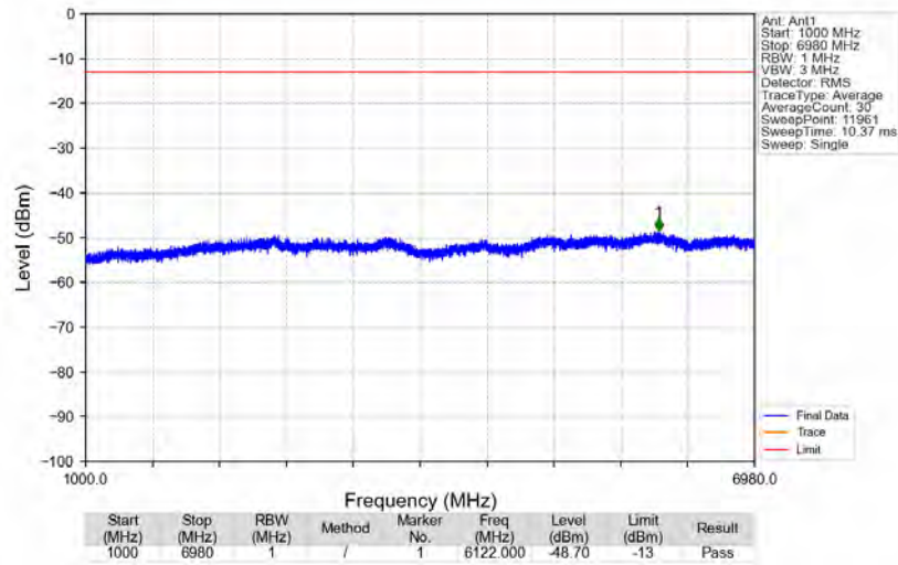
n71_15kHz_SISO_NTNV_5MHz_CP-OFDM QPSK_695.5MHz_Edge_1RB_Right
