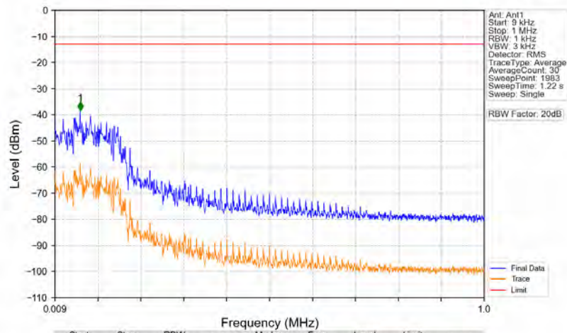
n71_15kHz_SISO_NTNV_10MHz_DFT-s-OFDM QPSK_693MHz_Edge_1RB_Right
