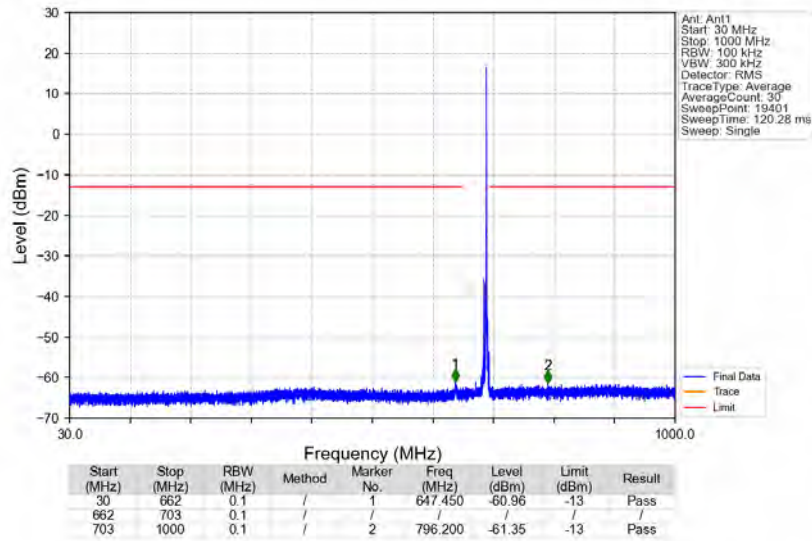
n71_15kHz_SISO_NTNV_5MHz_CP-OFDM QPSK_695.5MHz_Edge_1RB_Right
