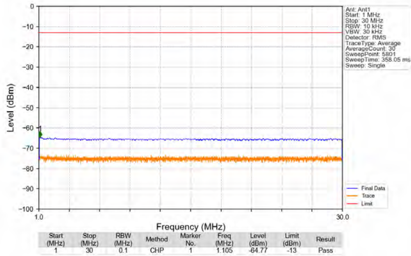
n71_15kHz_SISO_NTNV_15MHz_DFT-s-OFDM QPSK_680.5MHz_Edge_1RB_Left
