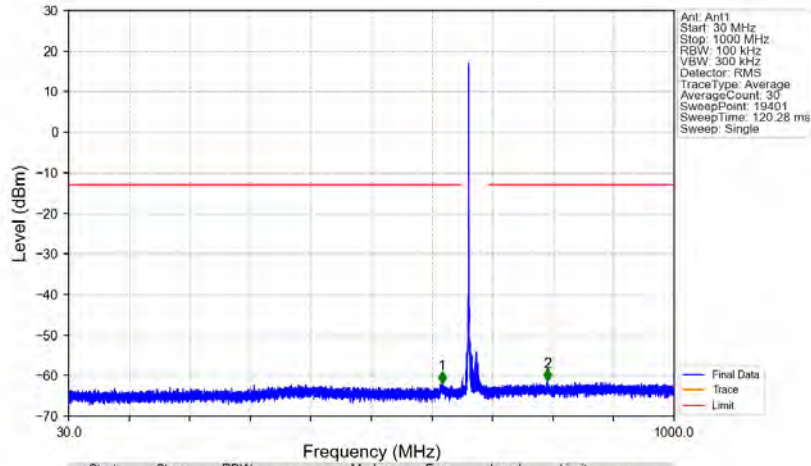
n71_15kHz_SISO_NTNV_20MHz_CP-OFDM QPSK_680.5MHz_Edge_1RB_Left
