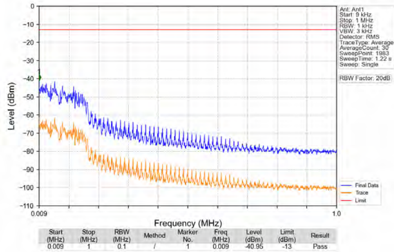
n71_15kHz_SISO_NTNV_20MHz_CP-OFDM QPSK_680.5MHz_Edge_1RB_Left
