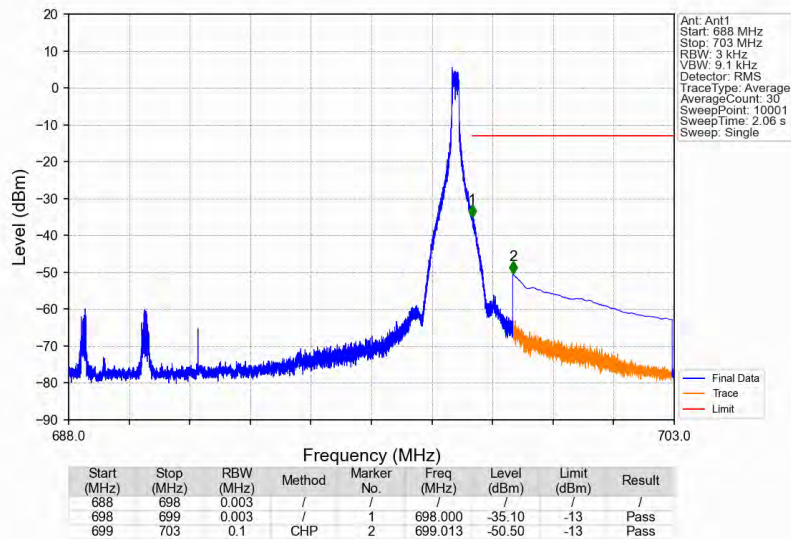
n71_15kHz_SISO_NTNV_10MHz_CP-OFDM QPSK_693MHz_Edge_1RB_Right
