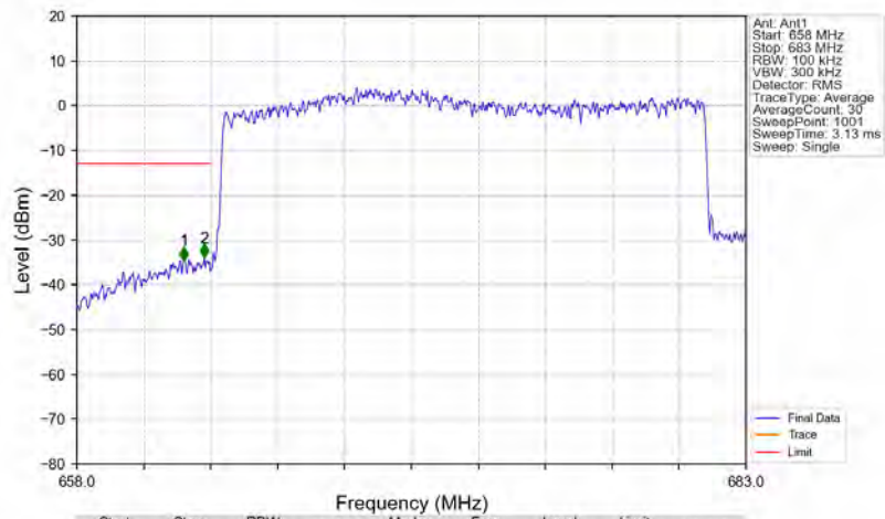
n71_15kHz_SISO_NTNV_20MHz_DFT-s-OFDM PI/2 BPSK_673MHz_Outer_Full
