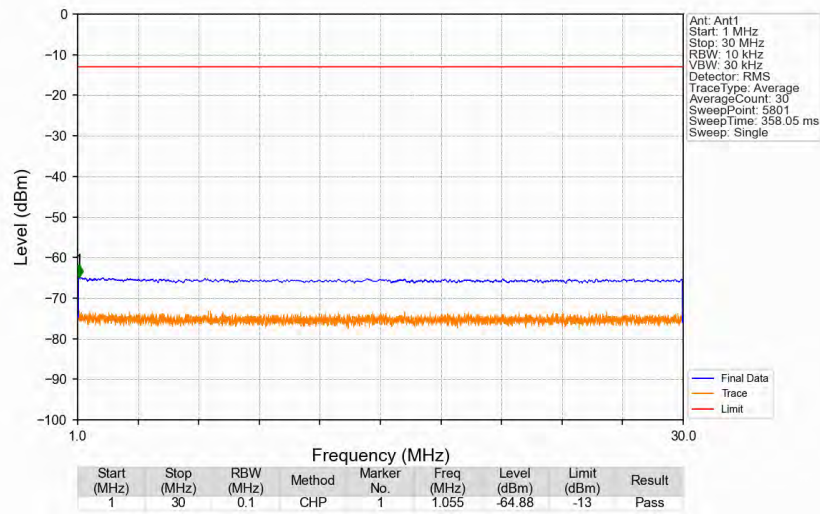
n71_15kHz_SISO_NTNV_10MHz_CP-OFDM QPSK_668MHz_Edge_1RB_Left
