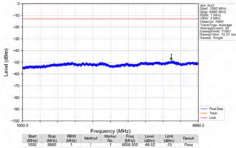
n71_15kHz_SISO_NTNV_10MHz_CP-OFDM QPSK_668MHz_Edge_1RB_Left
