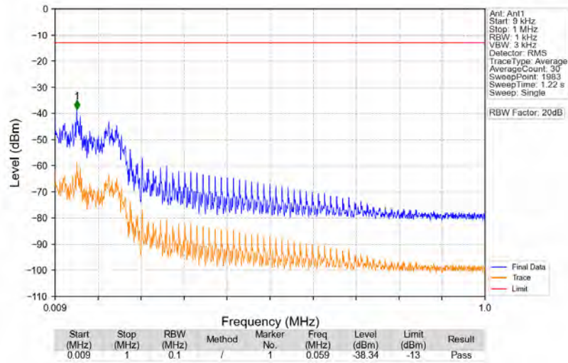
n71_15kHz_SISO_NTNV_15MHz_DFT-s-OFDM PI/2 BPSK_680.5MHz_Edge_1RB_Left
