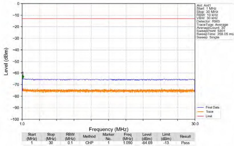
n71_15kHz_SISO_NTNV_5MHz_CP-OFDM QPSK_695.5MHz_Edge_1RB_Right
