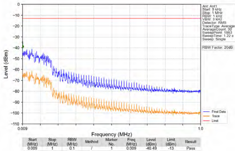
n71_15kHz_SISO_NTV_15MHz_CP-OFDM_QPSK_690.5MHz_Edge_1RB_Right
