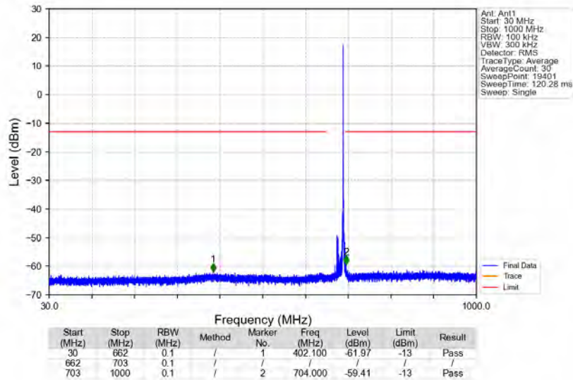
n71_15kHz_SISO_NTNV_15MHz_CP-OFDM QPSK_690.5MHz_Edge_1RB_Right
