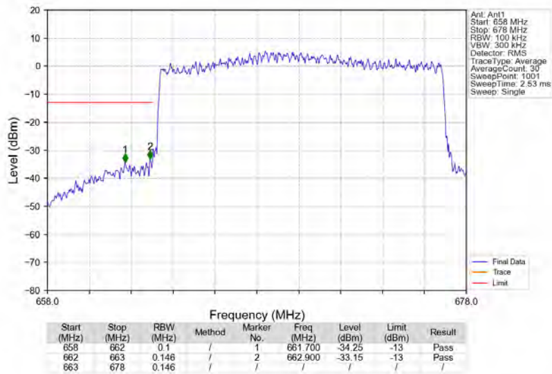
n71_15kHz_SISO_NTNV_15MHz_DFT-s-OFDM PI/2 BPSK_670.5MHz_Outer_Full
